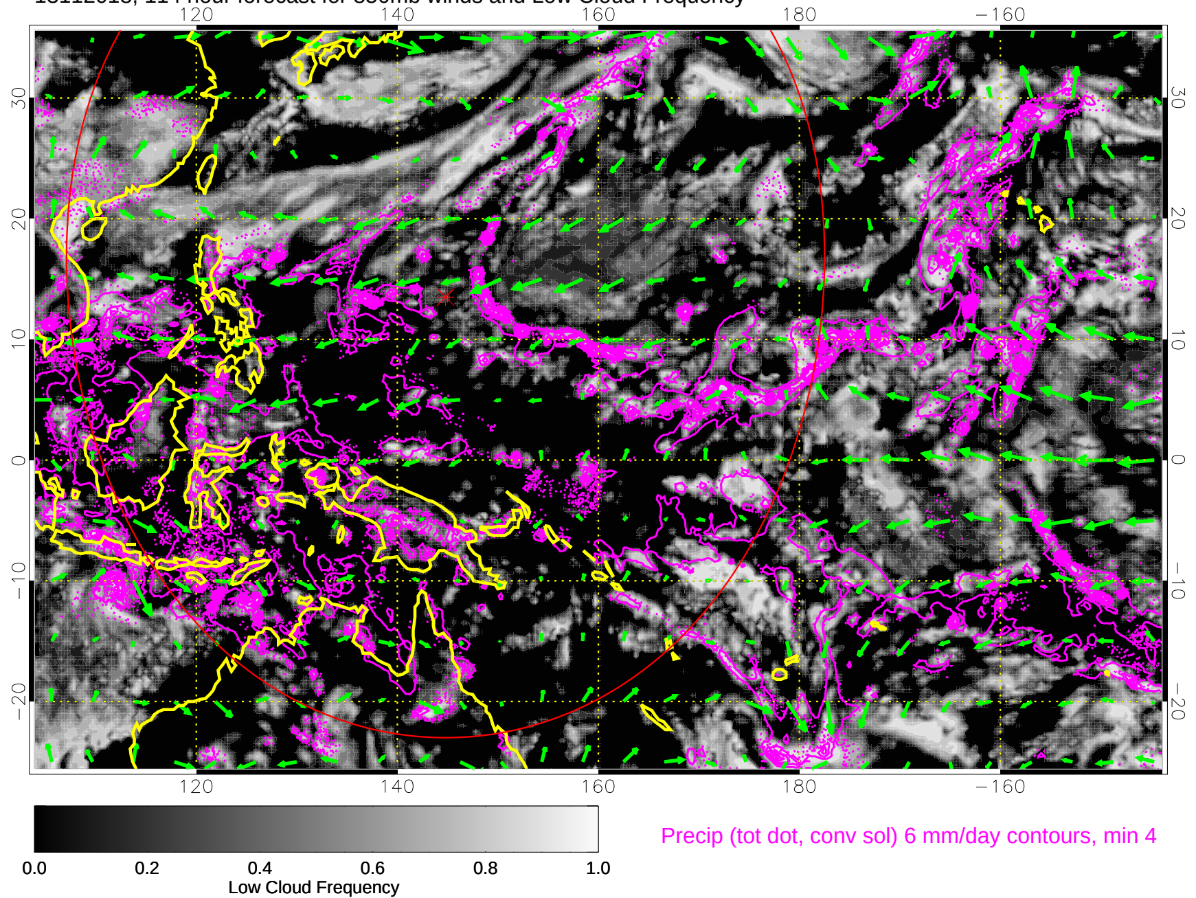
13112018, 114 hour forecast for 850mb winds and Low Cloud Frequency
