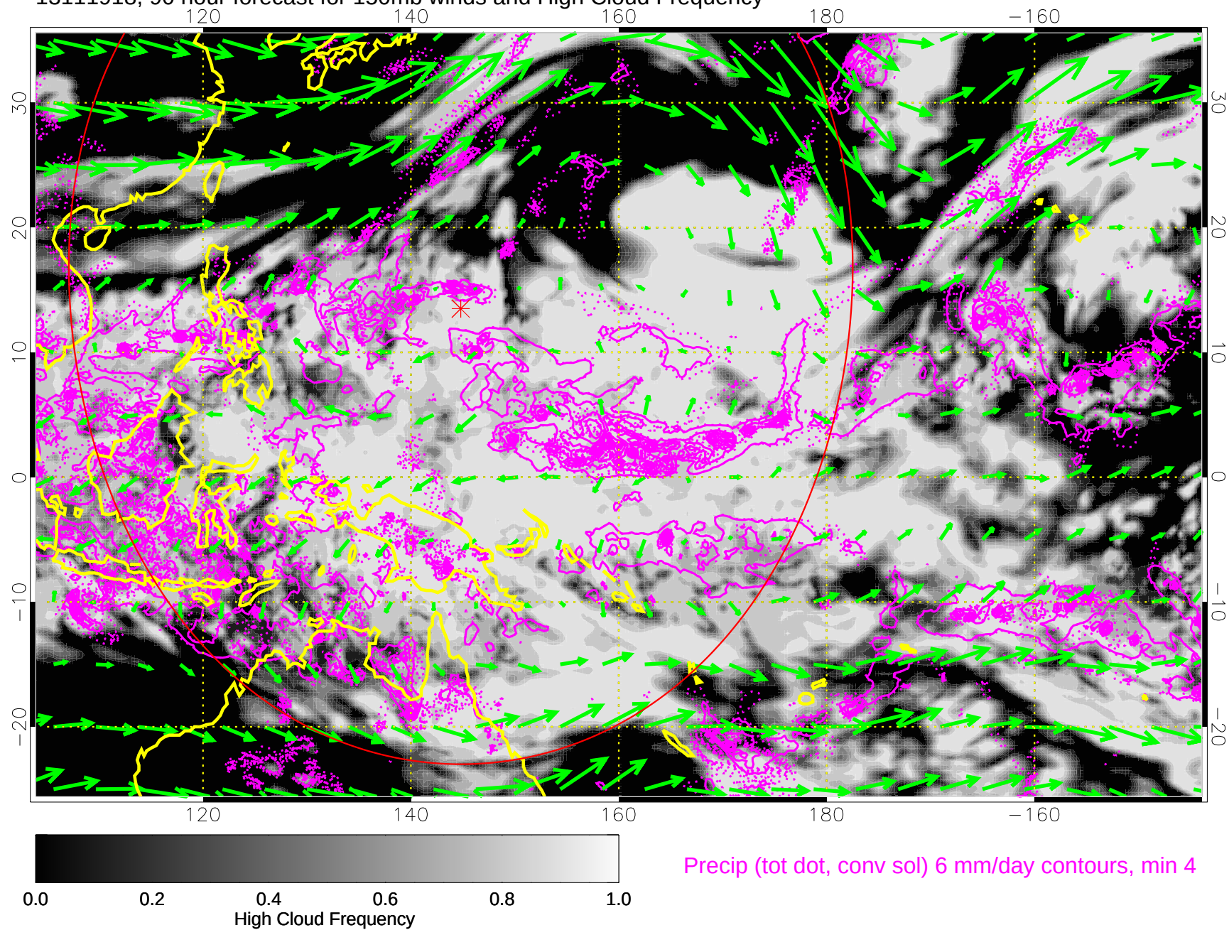
13111918, 90 hour forecast for 150mb winds and High Cloud Frequency
