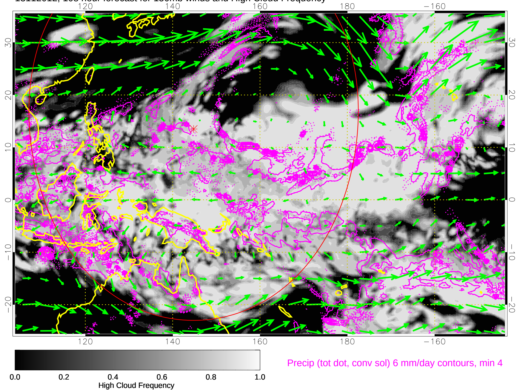
13112012, 108 hour forecast for 150mb winds and High Cloud Frequency
