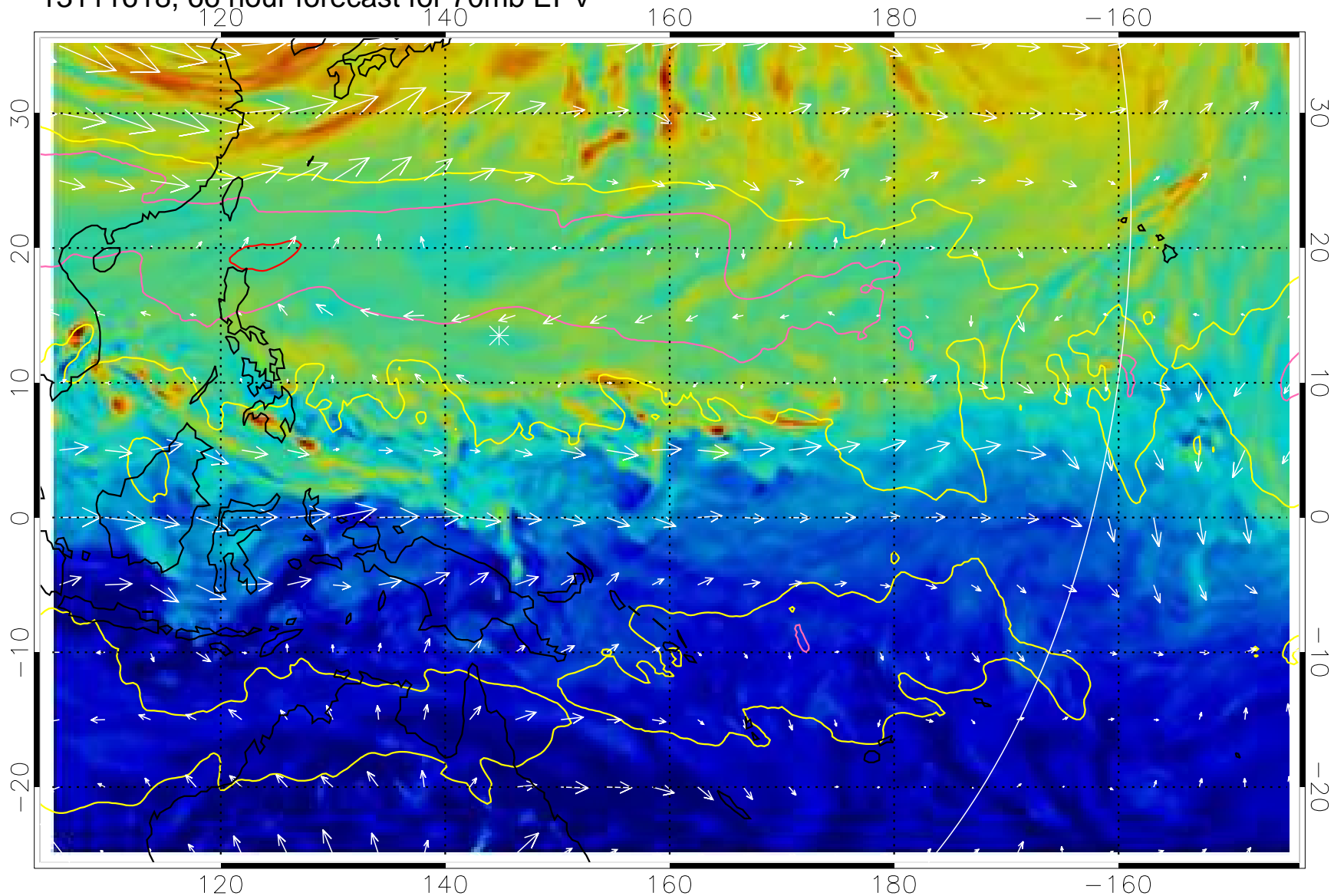
13111618, 66 hour forecast for 70mb EPV
