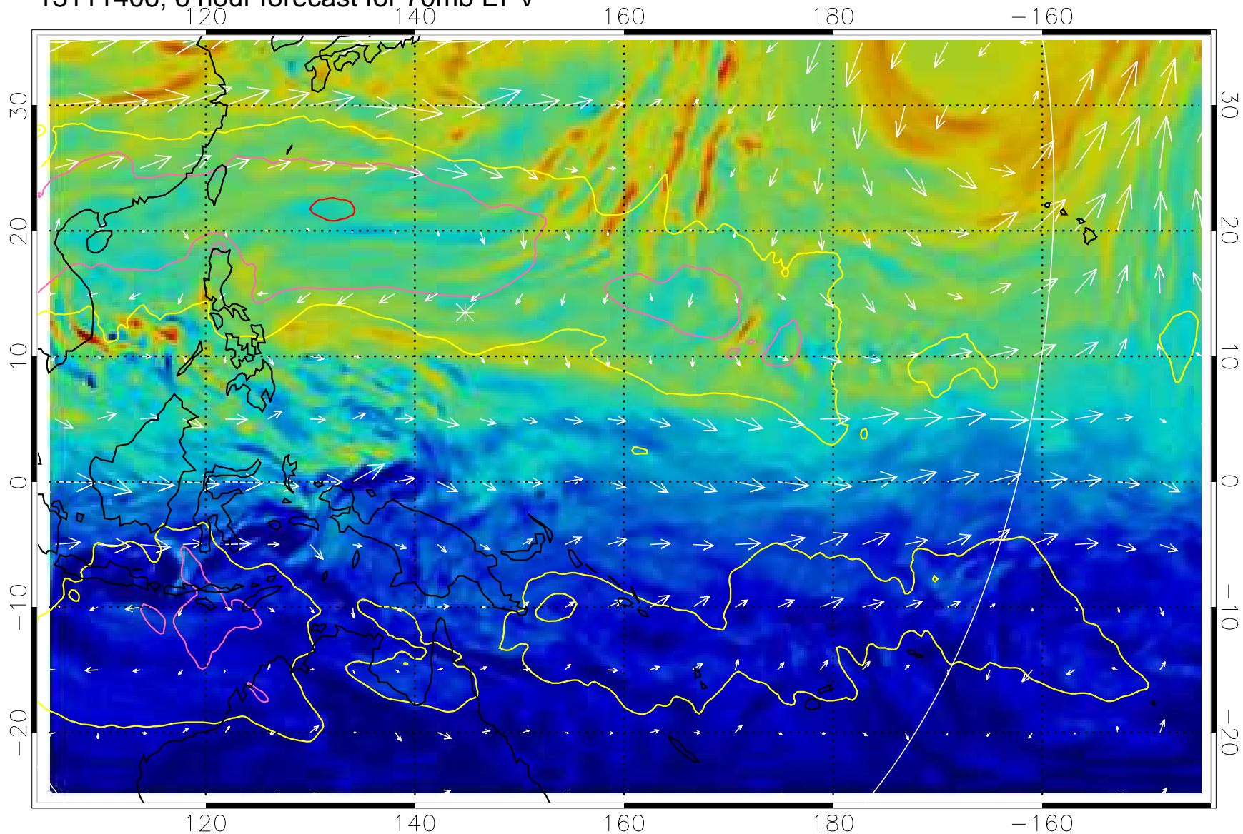
13111406, 6 hour forecast for 70mb EPV
