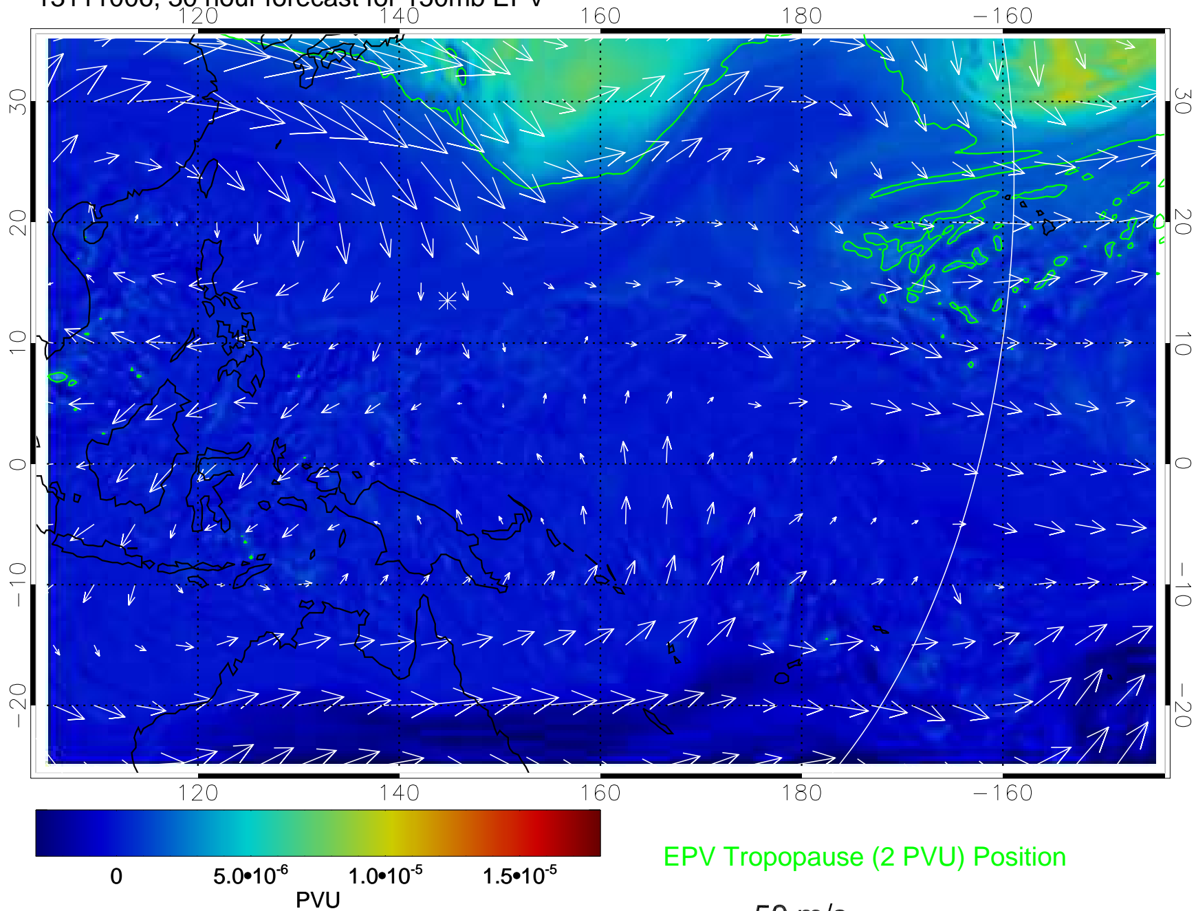
13111006, 30 hour forecast for 150mb EPV
