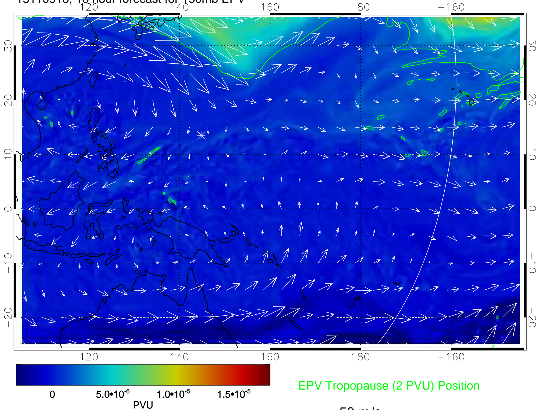
13110918, 18 hour forecast for 150mb EPV
