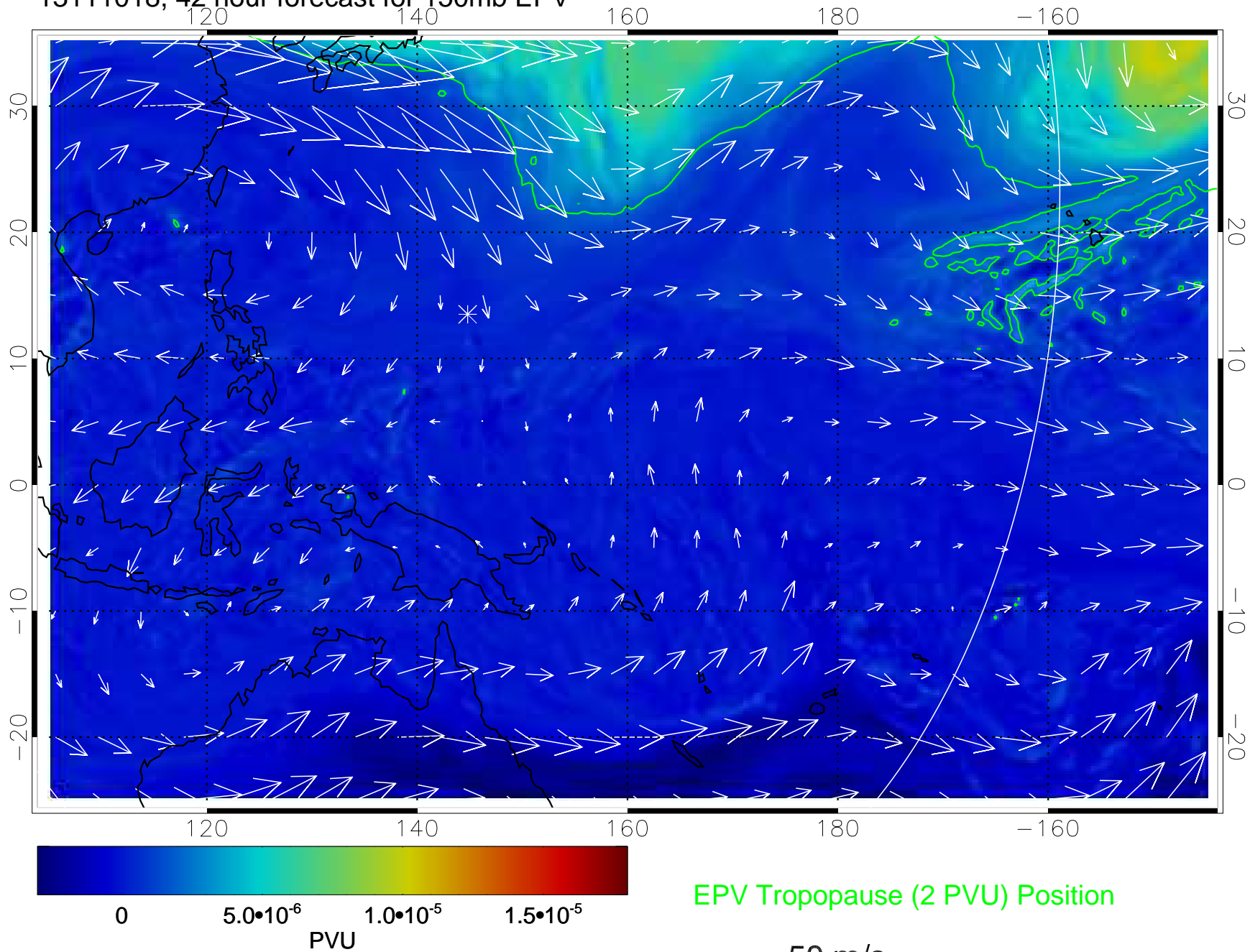
13111018, 42 hour forecast for 150mb EPV
