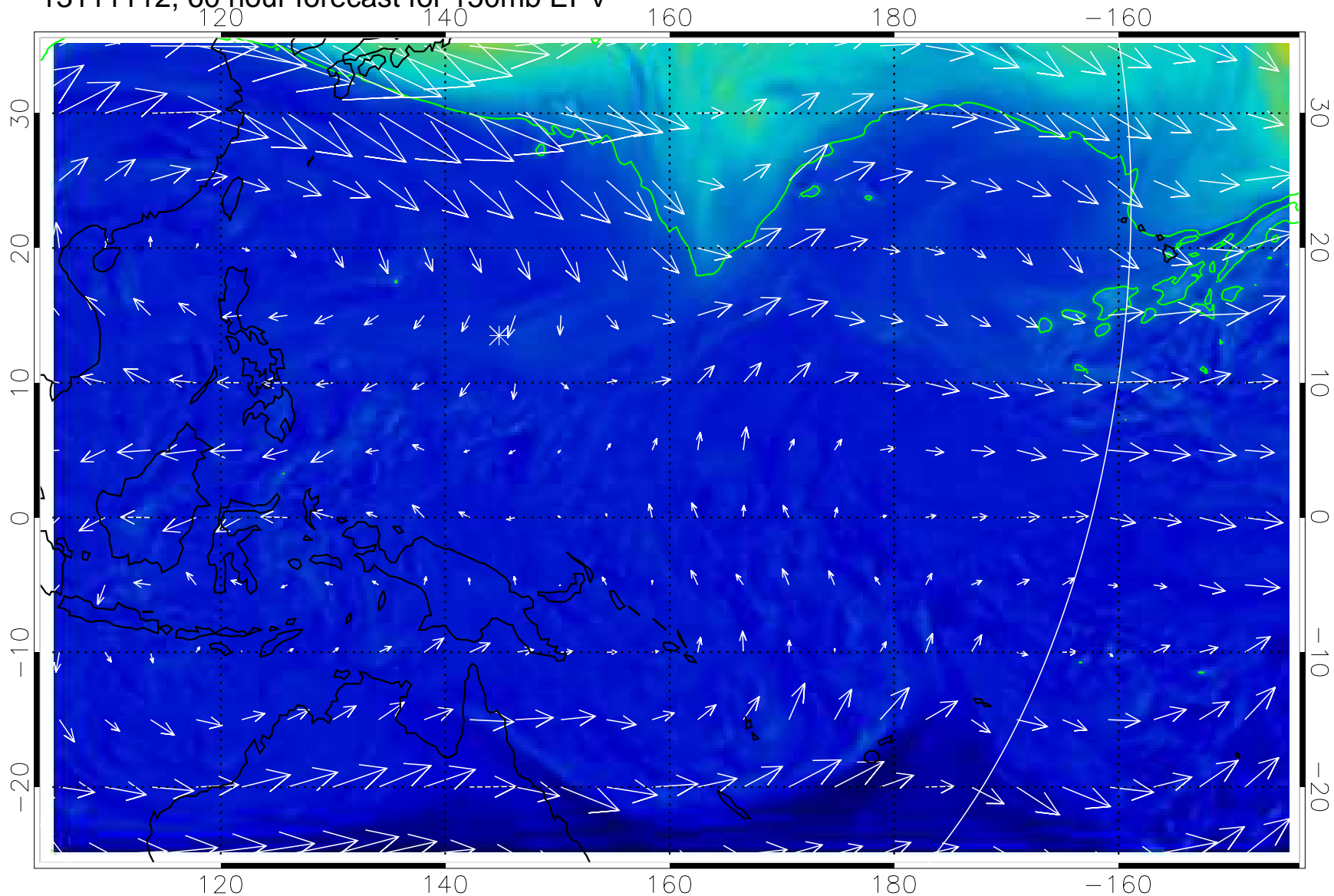
13111112, 60 hour forecast for 150mb EPV
