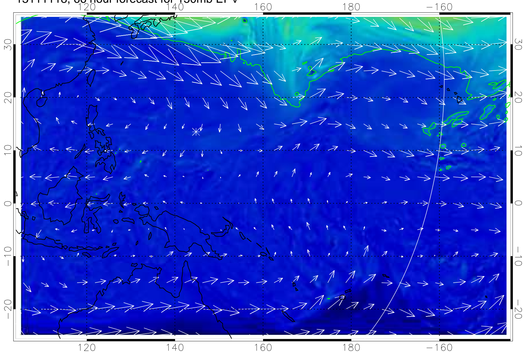
13111118, 66 hour forecast for 150mb EPV
