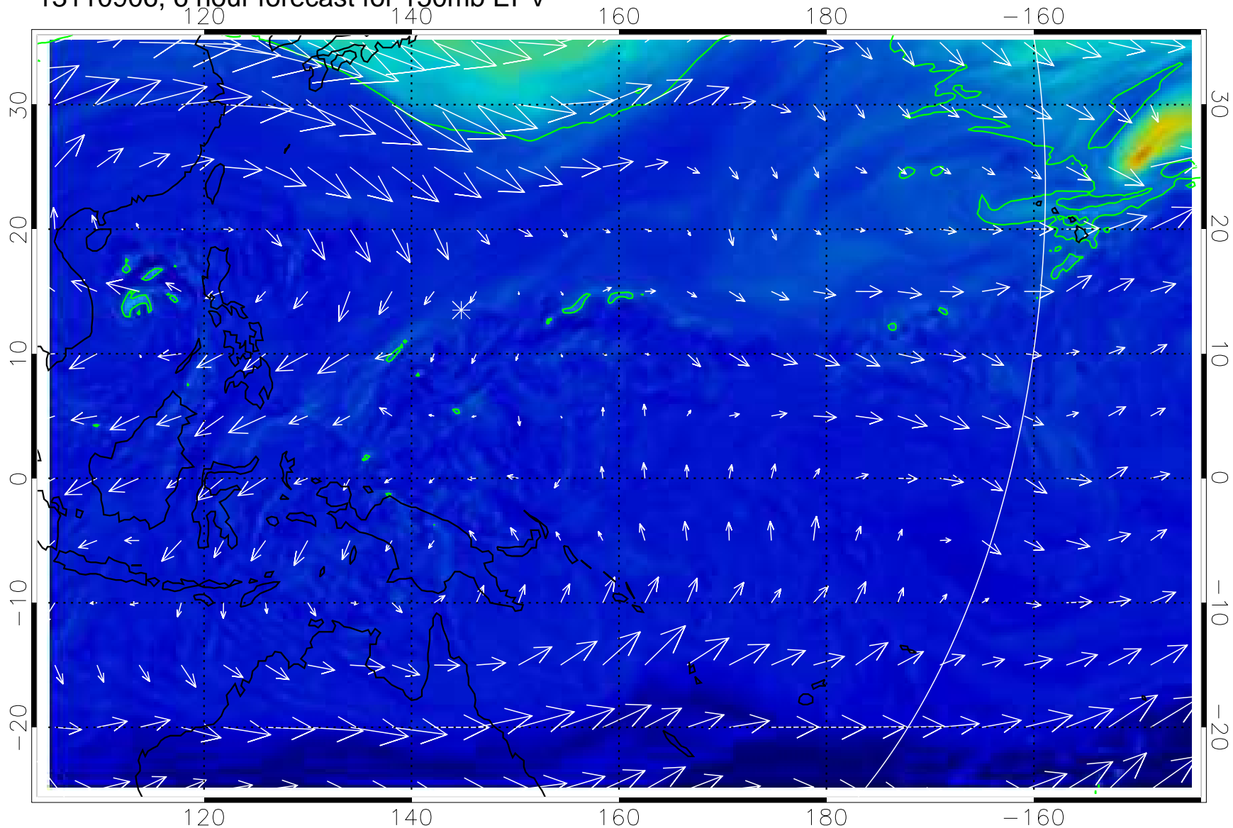
13110906, 6 hour forecast for 150mb EPV
