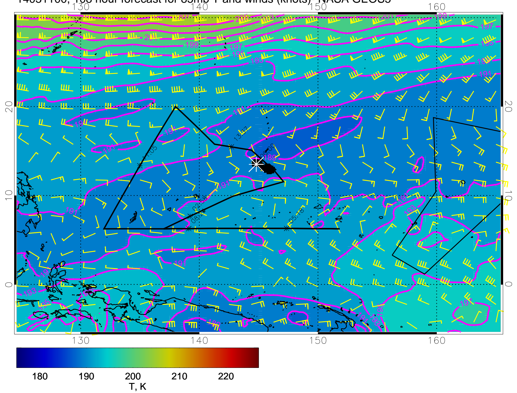
14031100, 108 hour forecast for 85mb T and winds (knots)- NASA GEOS5
