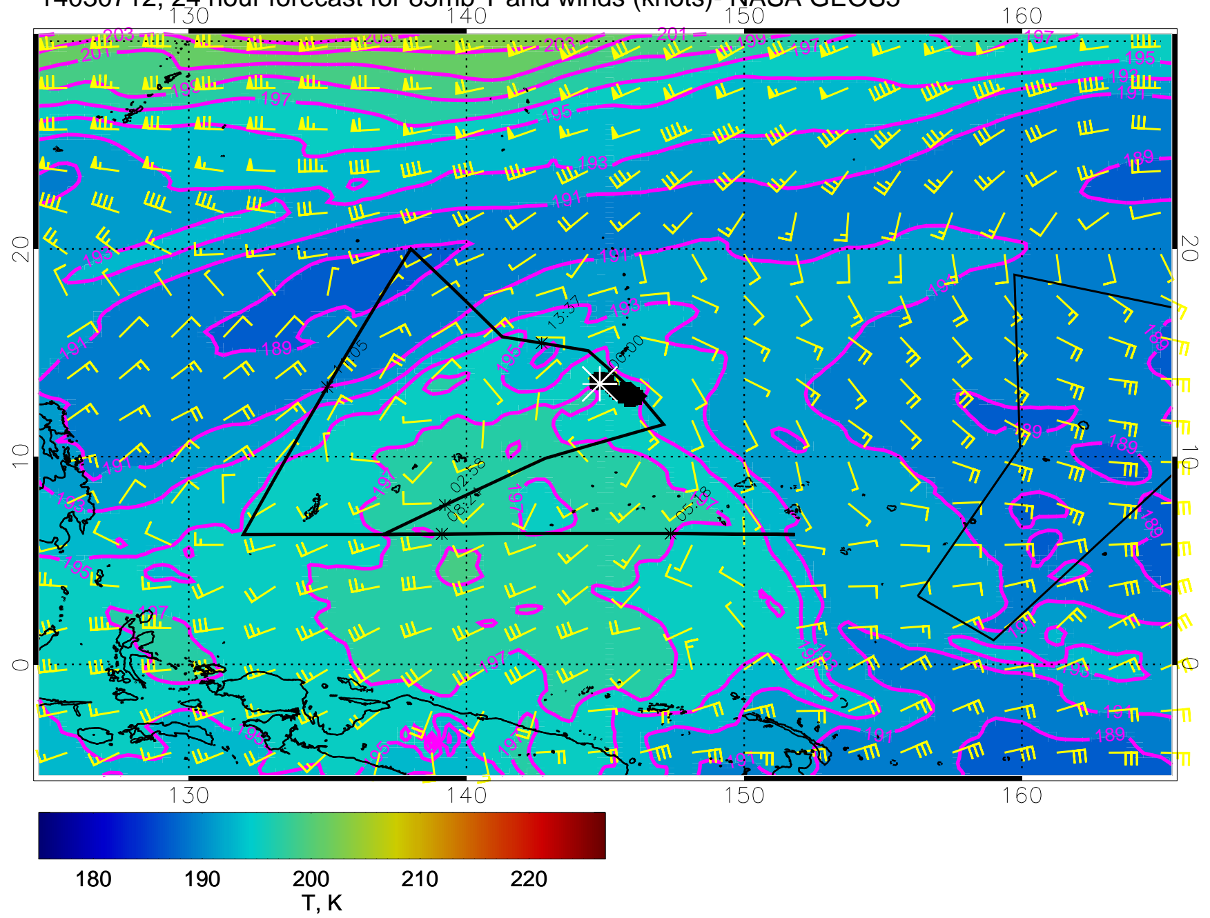
14030712, 24 hour forecast for 85mb T and winds (knots)- NASA GEOS5
