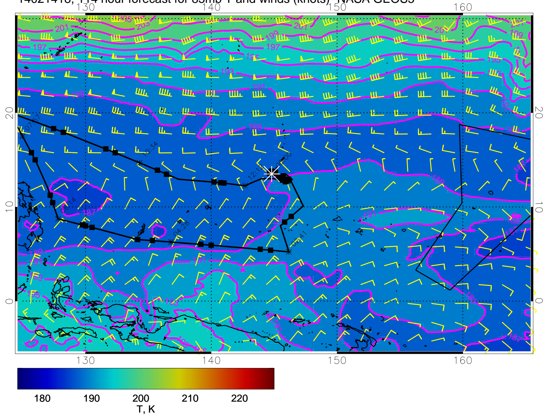
14021418, 114 hour forecast for 85mb T and winds (knots)- NASA GEOS5
