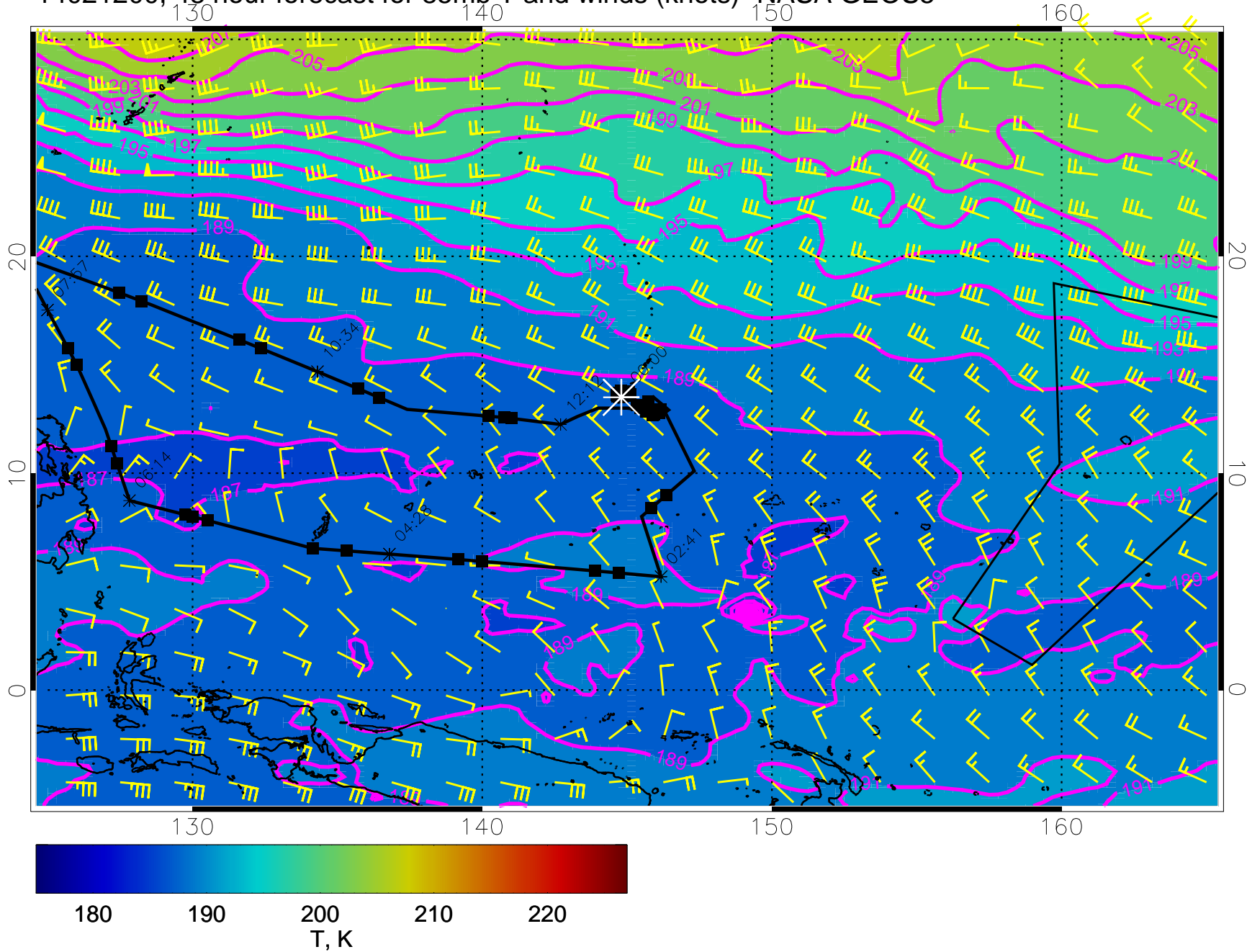
14021200, 48 hour forecast for 85mb T and winds (knots)- NASA GEOS5
