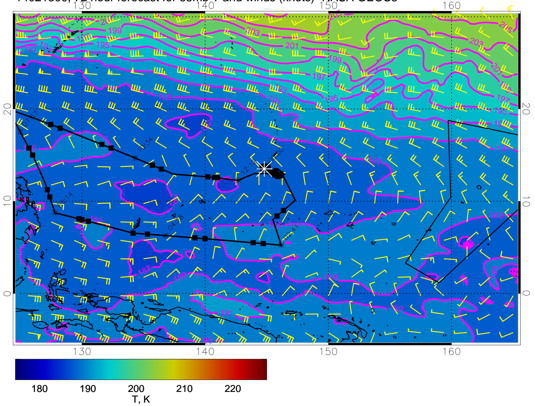
14021300, 72 hour forecast for 85mb T and winds (knots)- NASA GEOS5
