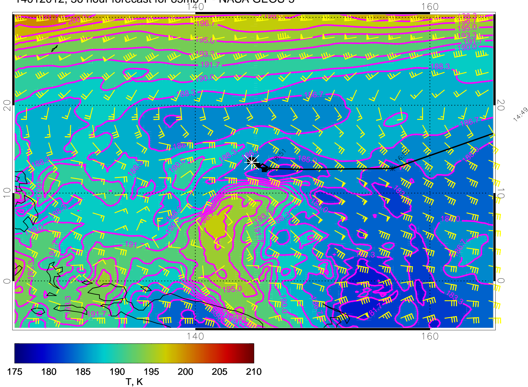
14012012, 36 hour forecast for 85mb T - NASA GEOS-5
