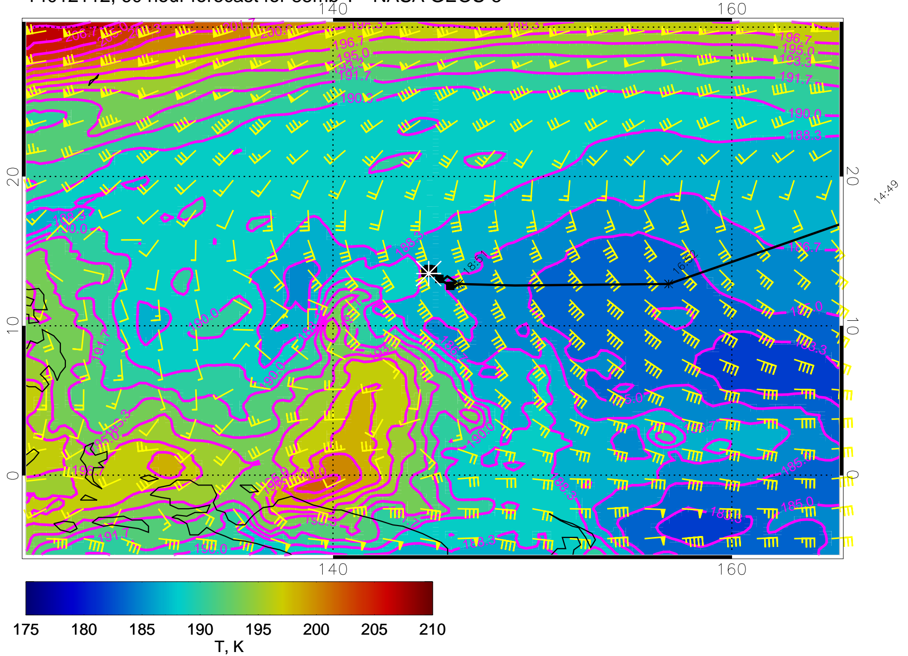
14012112, 60 hour forecast for 85mb T - NASA GEOS-5
