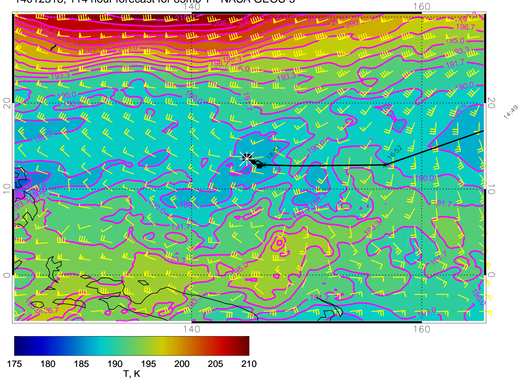
14012318, 114 hour forecast for 85mb T - NASA GEOS-5
