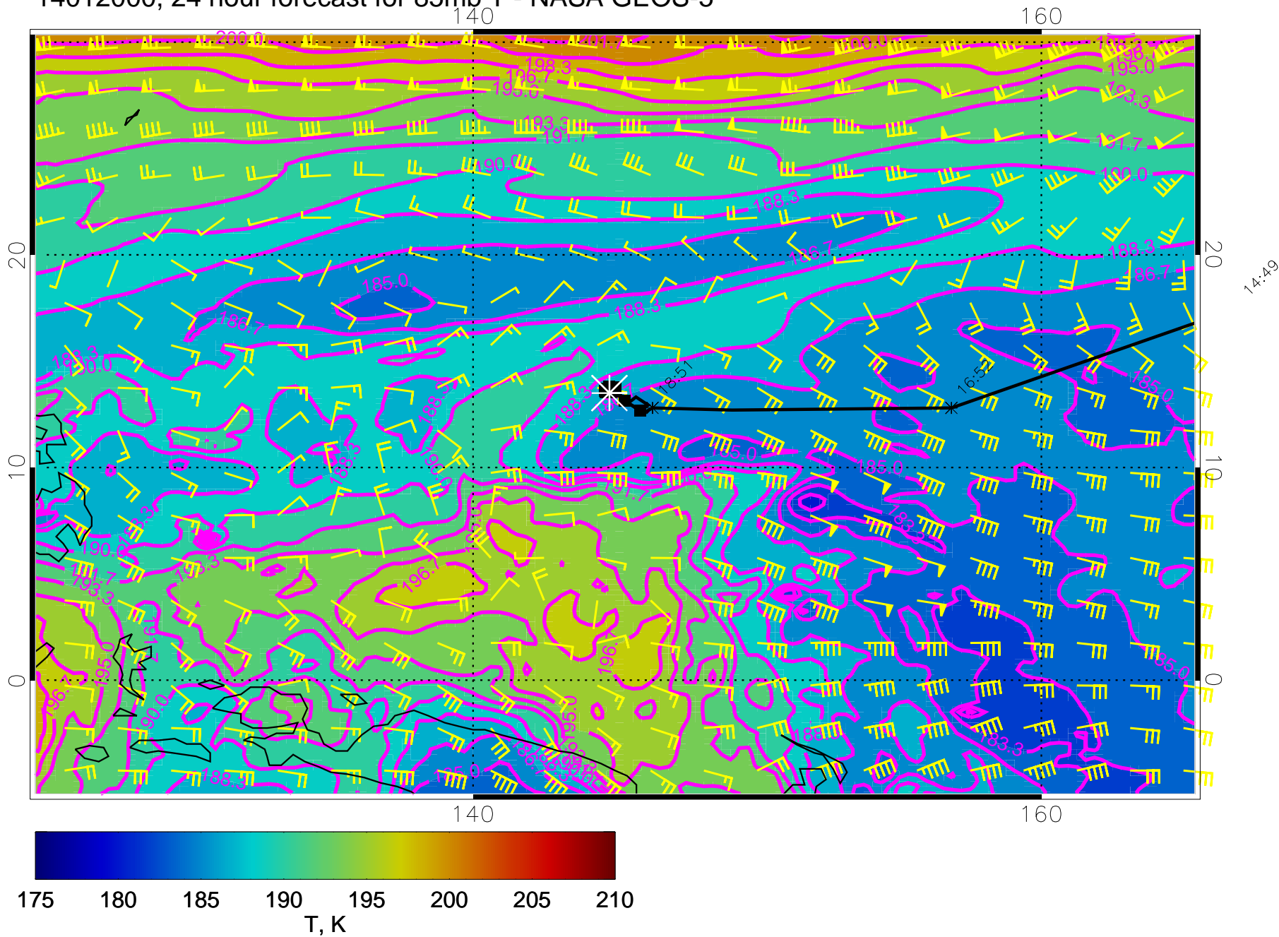
14012000, 24 hour forecast for 85mb T - NASA GEOS-5
