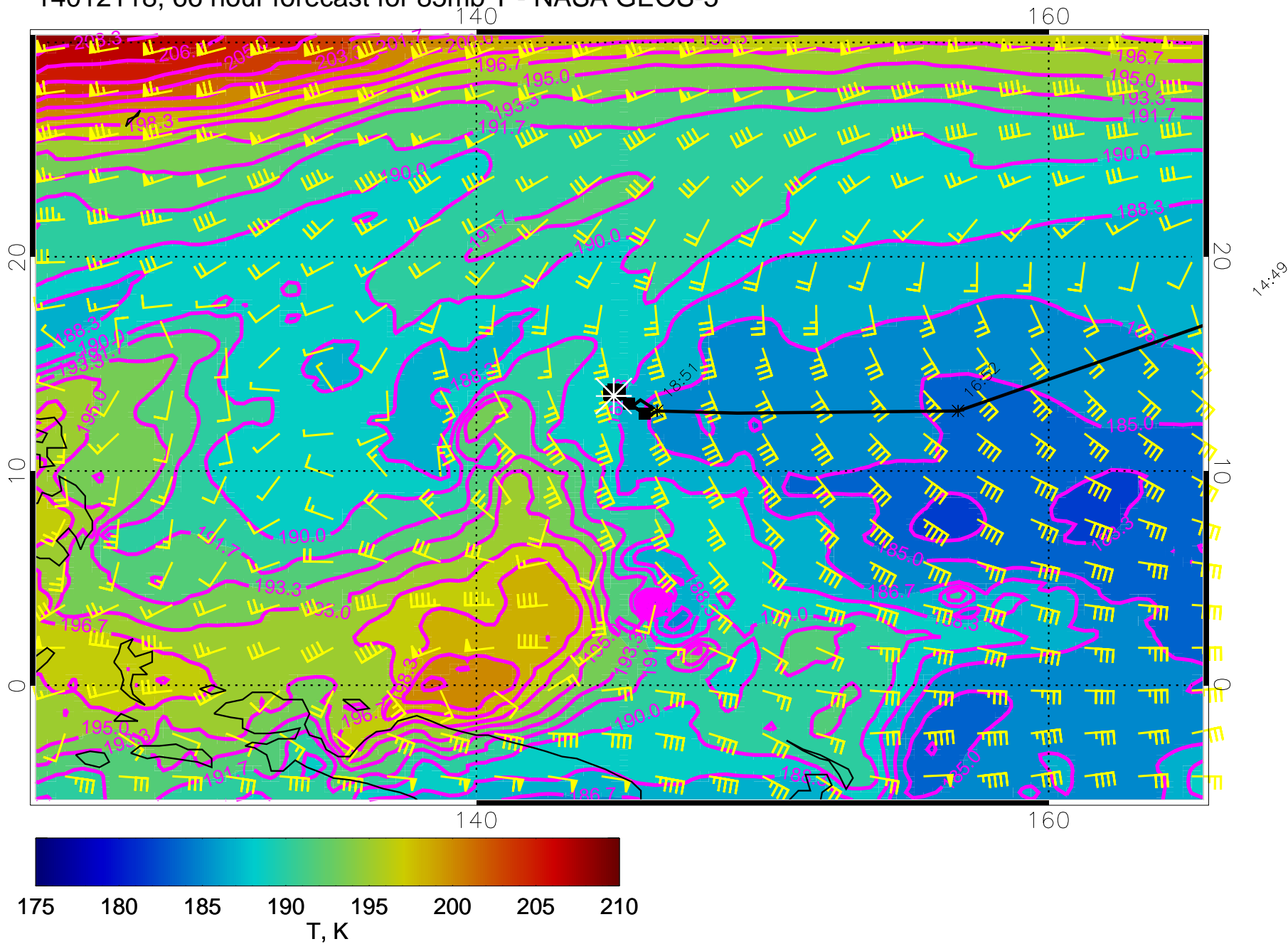
14012118, 66 hour forecast for 85mb T - NASA GEOS-5
