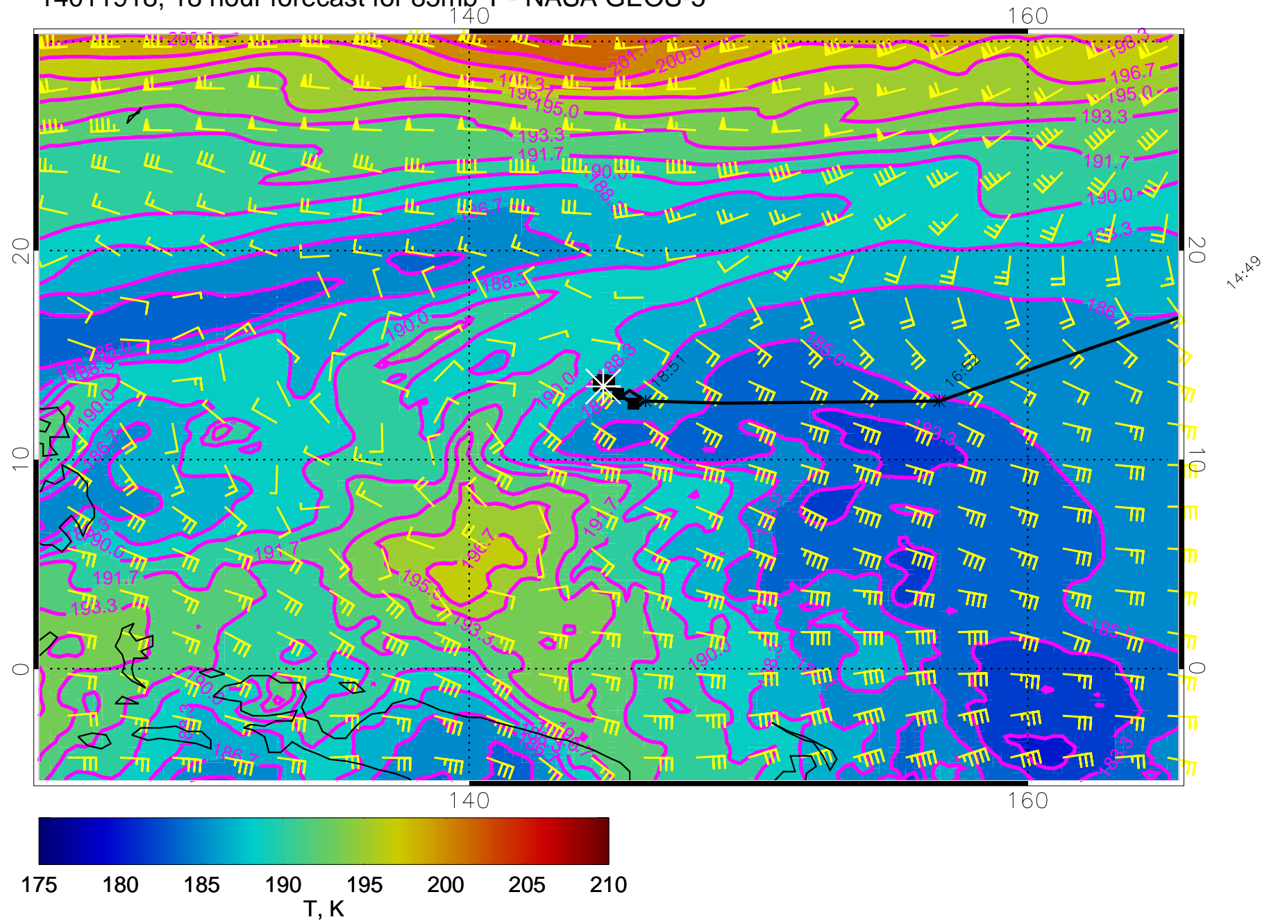
14011918, 18 hour forecast for 85mb T - NASA GEOS-5
