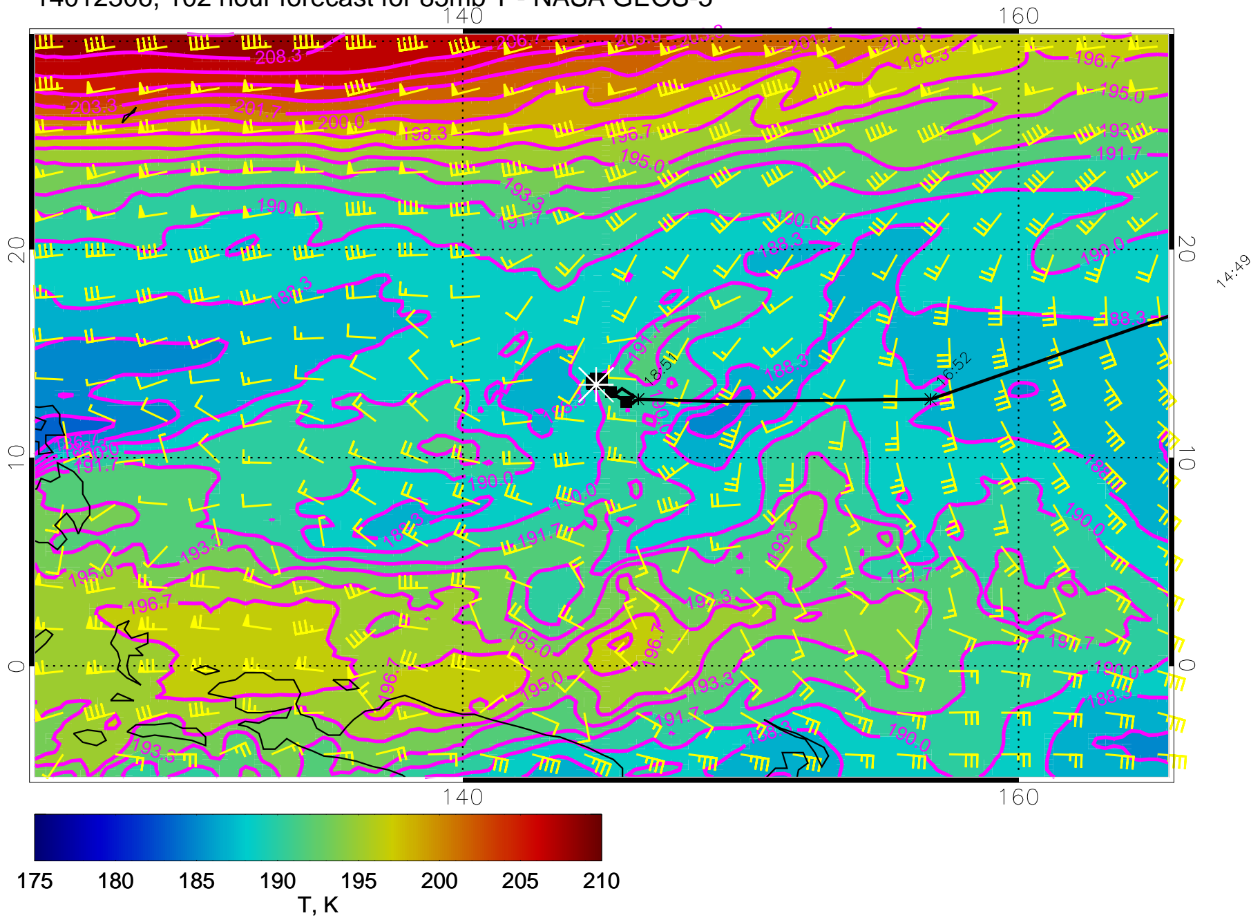
14012306, 102 hour forecast for 85mb T - NASA GEOS-5
