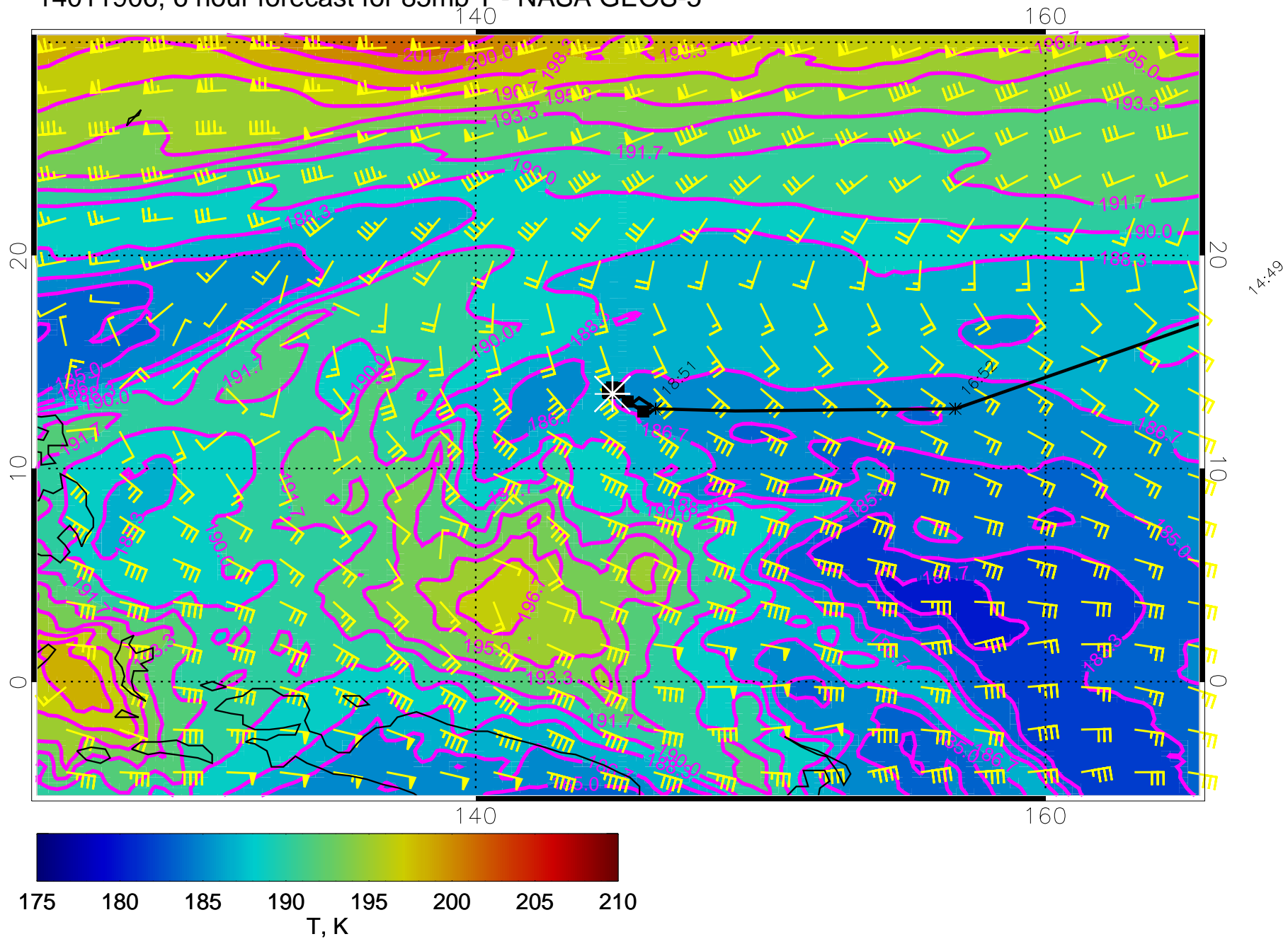
14011906, 6 hour forecast for 85mb T - NASA GEOS-5
