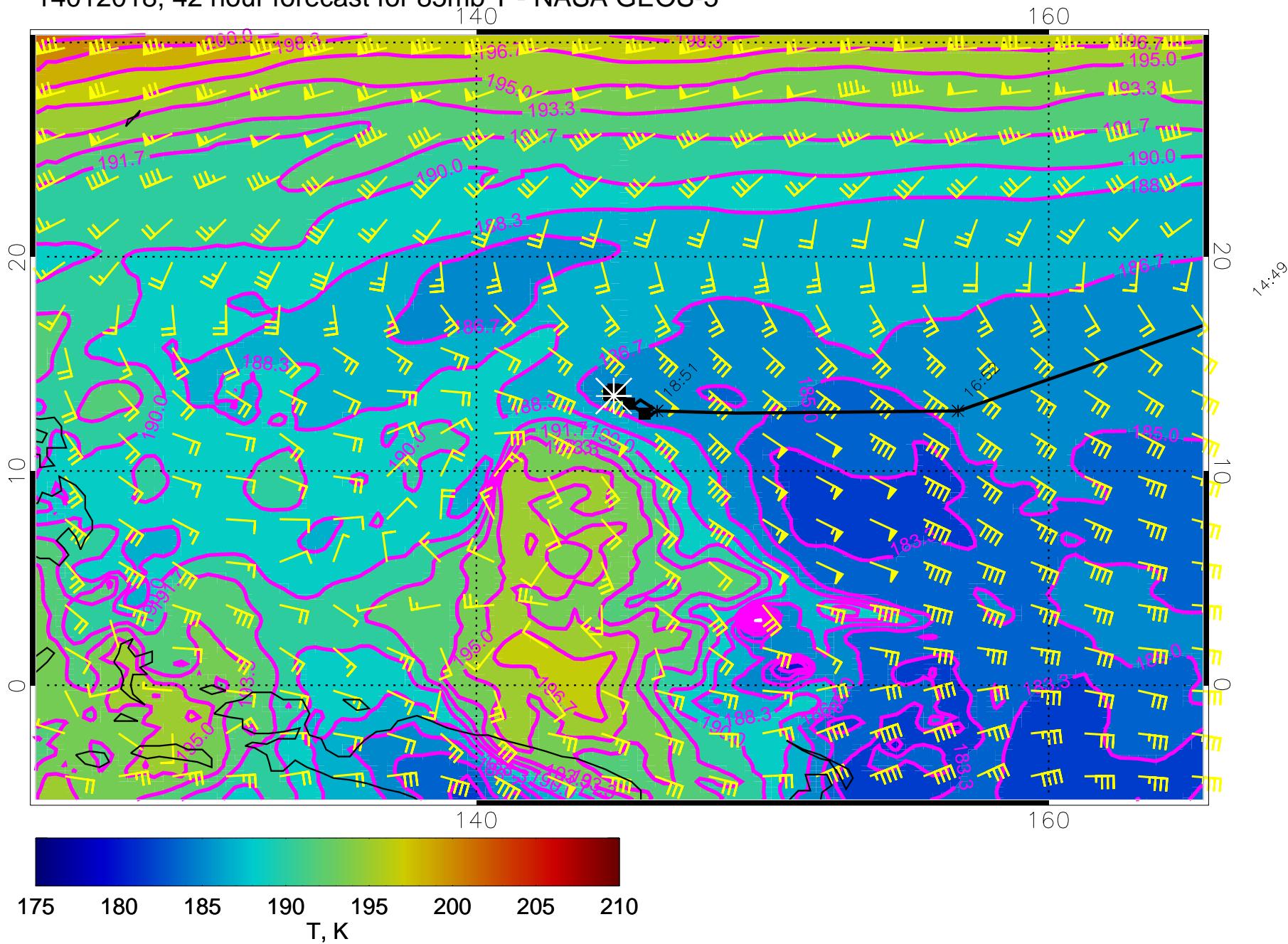
14012018, 42 hour forecast for 85mb T - NASA GEOS-5
