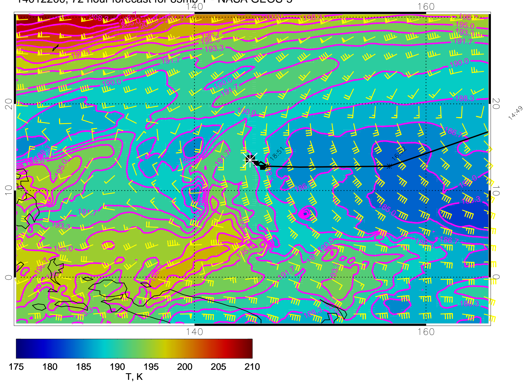
14012200, 72 hour forecast for 85mb T - NASA GEOS-5
