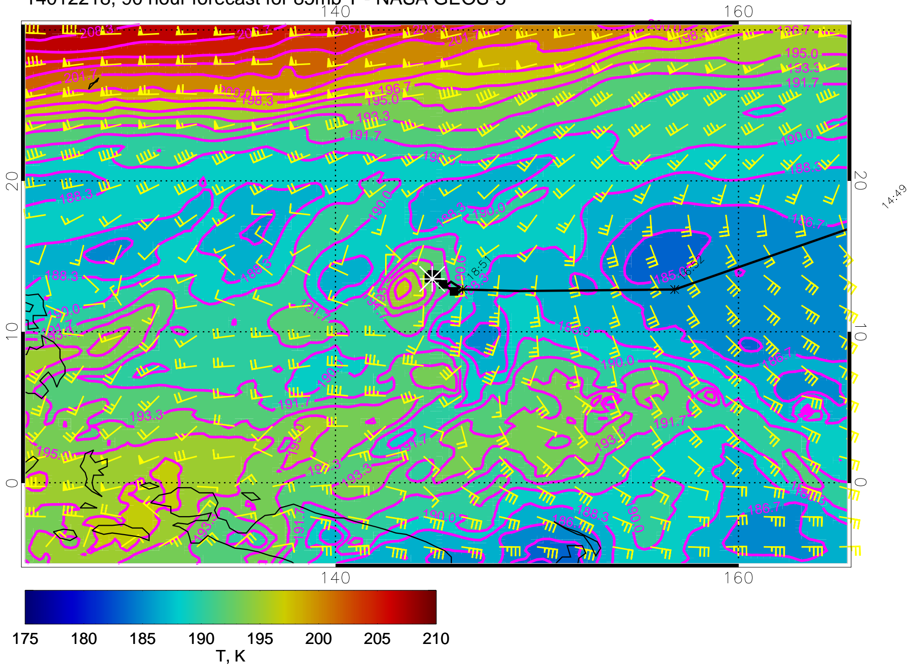
14012218, 90 hour forecast for 85mb T - NASA GEOS-5
