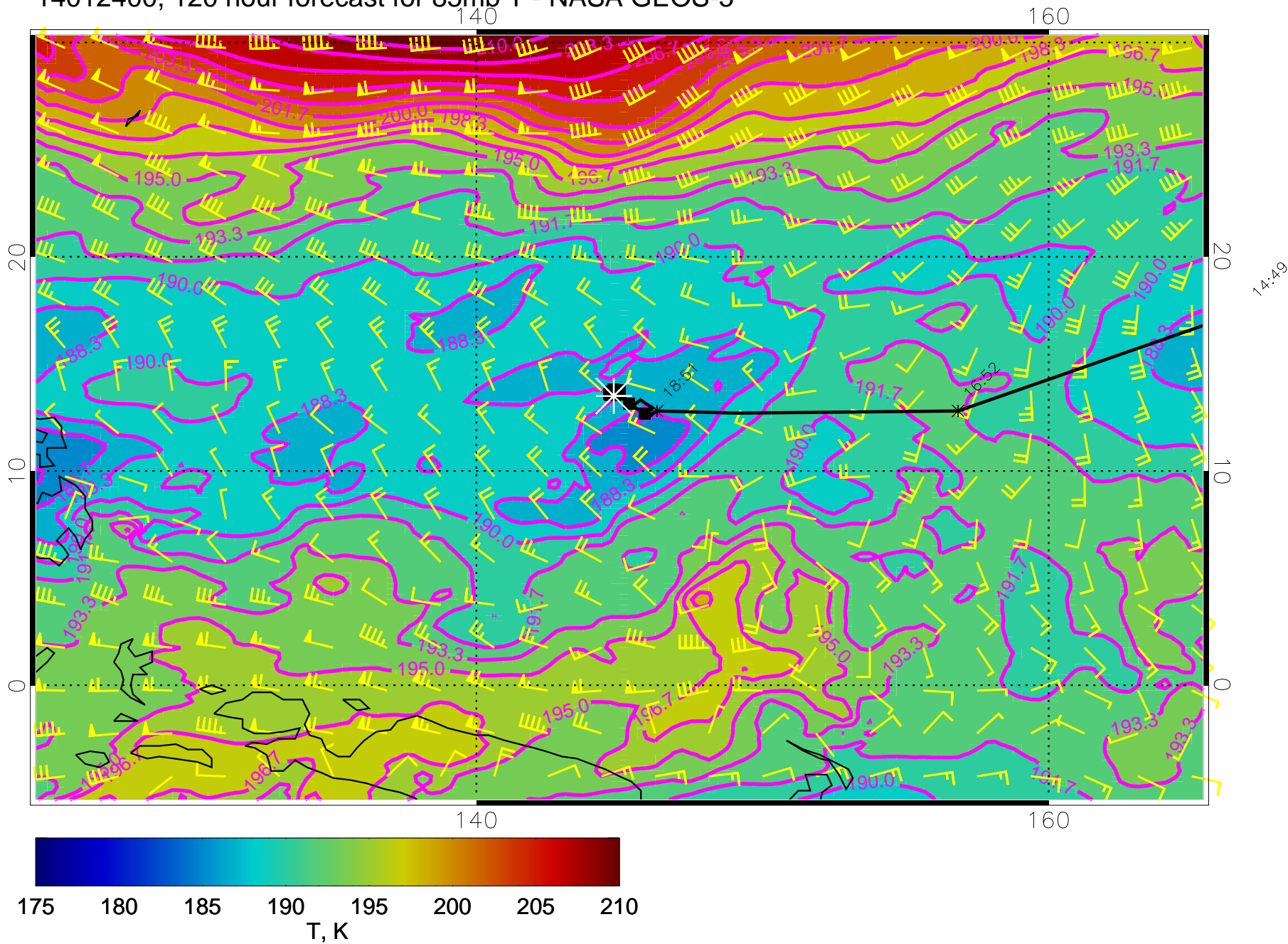
14012400, 120 hour forecast for 85mb T - NASA GEOS-5
