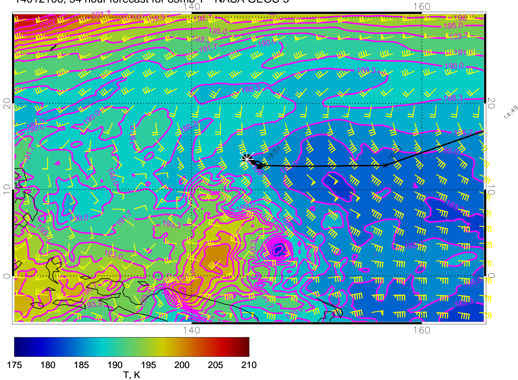
14012106, 54 hour forecast for 85mb T - NASA GEOS-5
