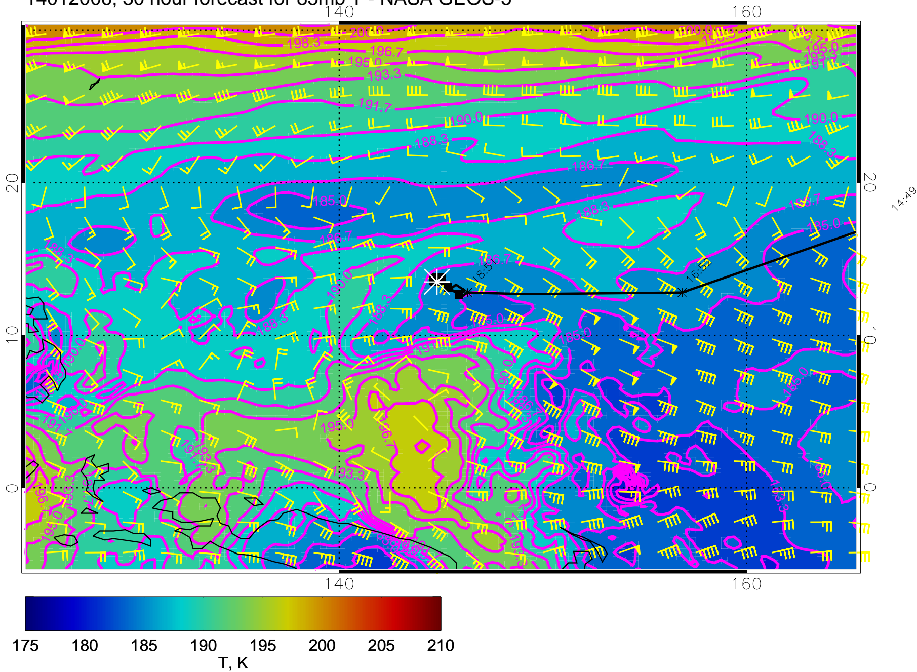
14012006, 30 hour forecast for 85mb T - NASA GEOS-5
