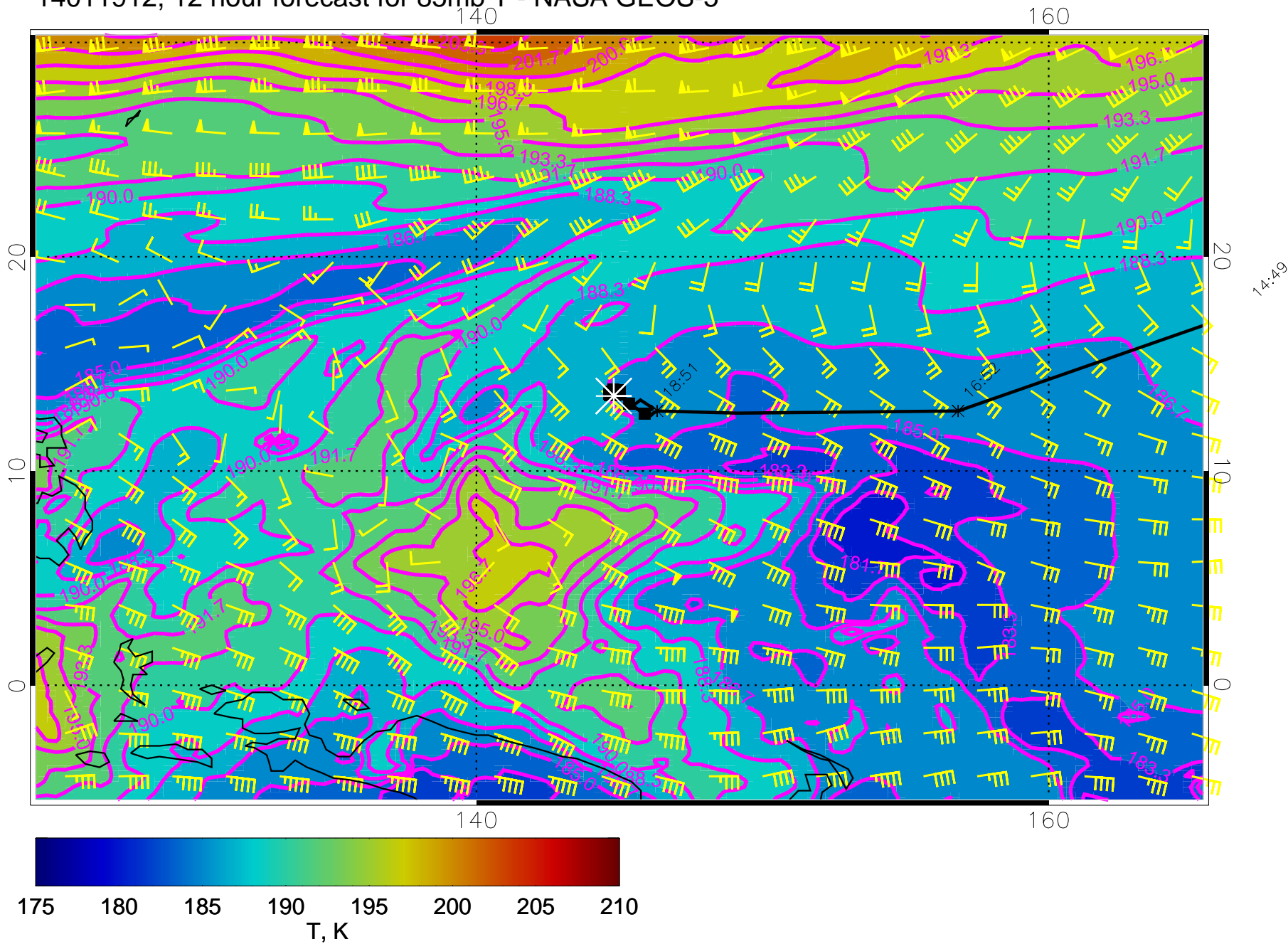
14011912, 12 hour forecast for 85mb T - NASA GEOS-5
