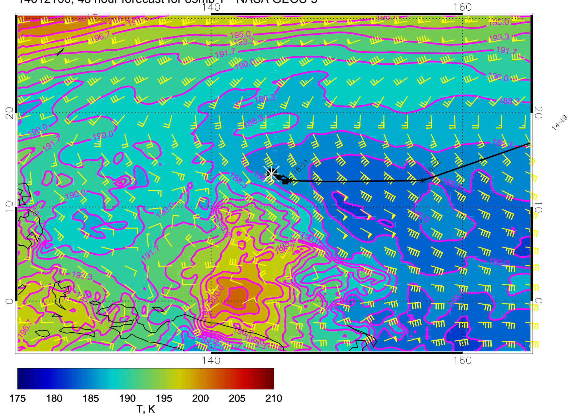
14012100, 48 hour forecast for 85mb T - NASA GEOS-5
