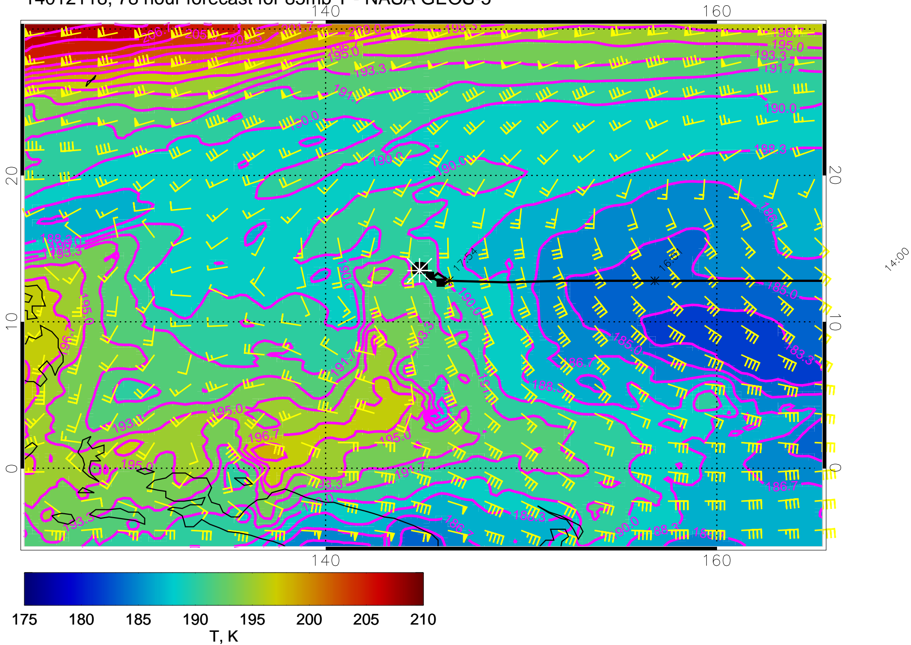
14012118, 78 hour forecast for 85mb T - NASA GEOS-5
