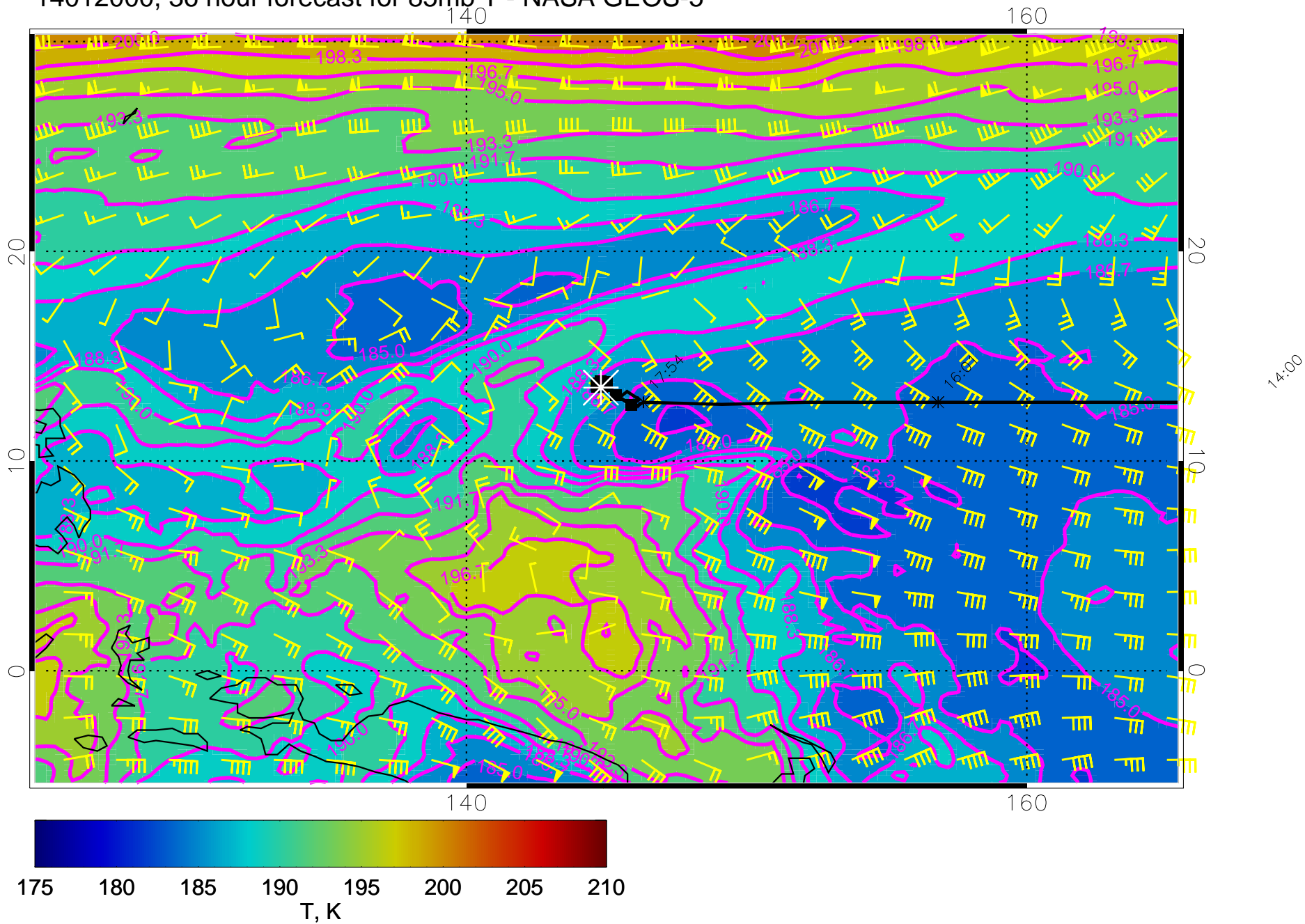
14012000, 36 hour forecast for 85mb T - NASA GEOS-5
