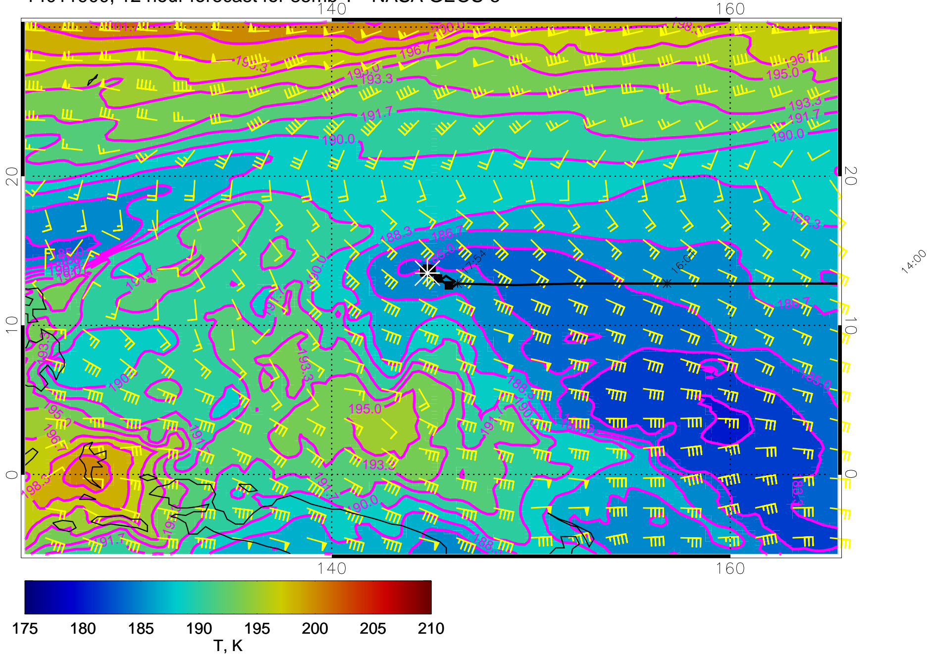
14011900, 12 hour forecast for 85mb T - NASA GEOS-5
