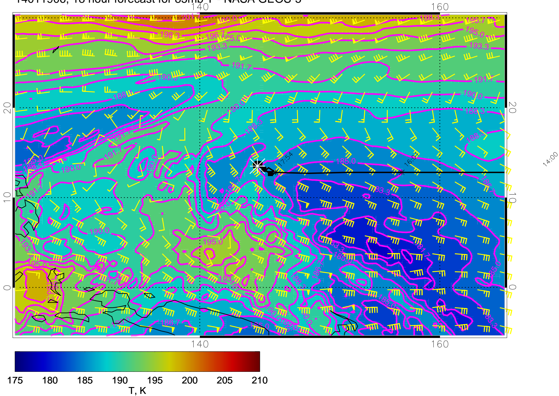
14011906, 18 hour forecast for 85mb T - NASA GEOS-5
