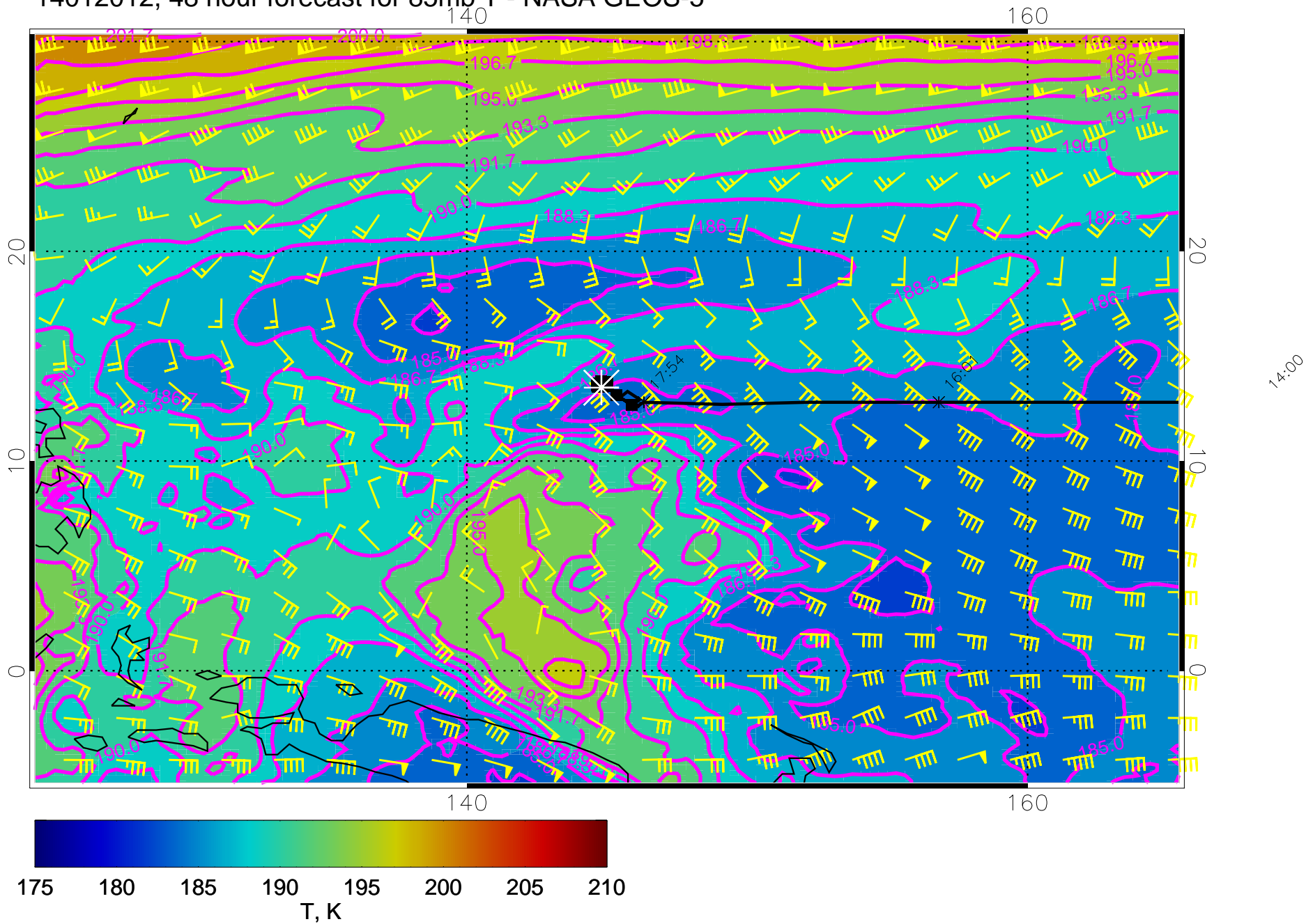
14012012, 48 hour forecast for 85mb T - NASA GEOS-5
