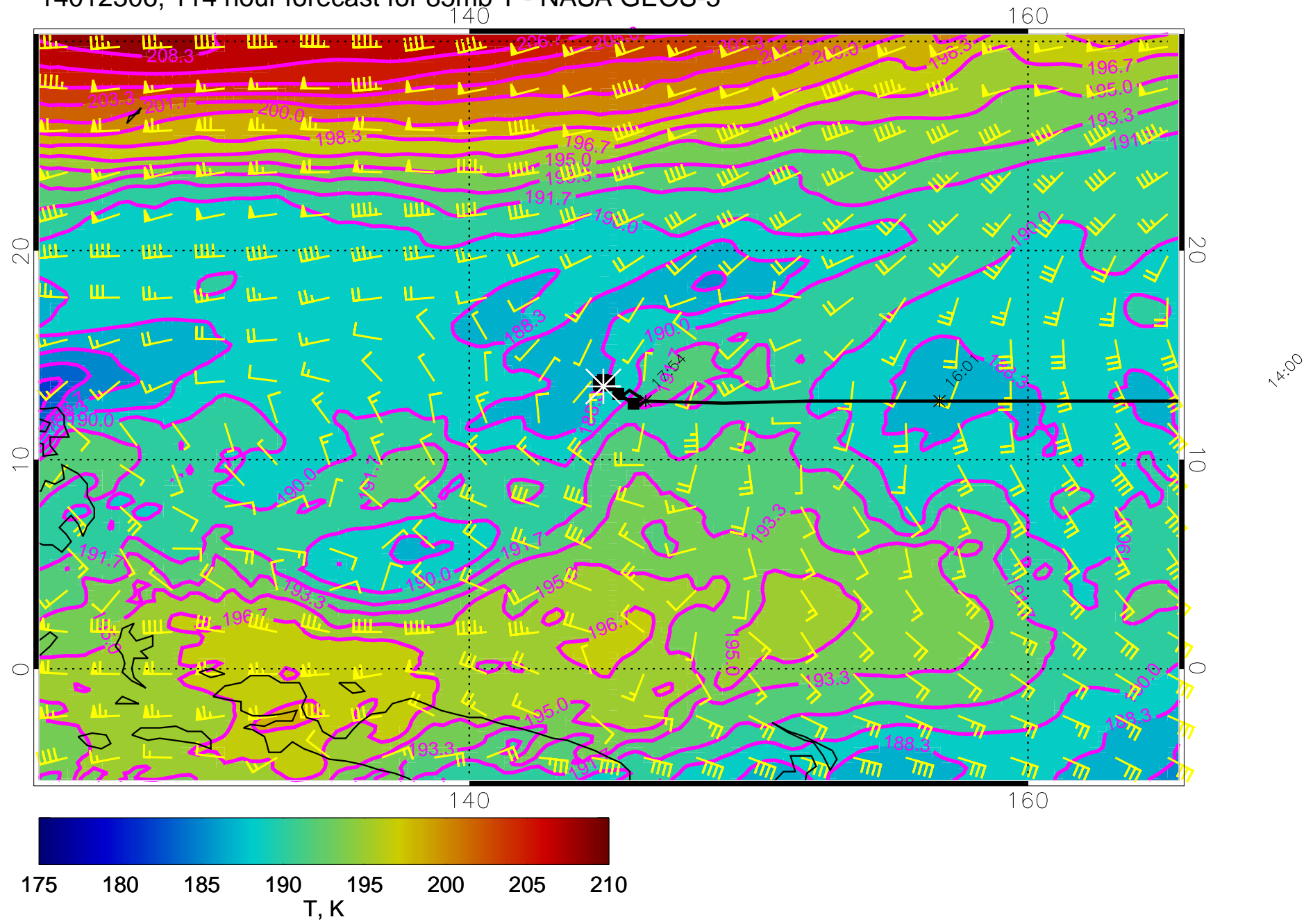
14012306, 114 hour forecast for 85mb T - NASA GEOS-5
