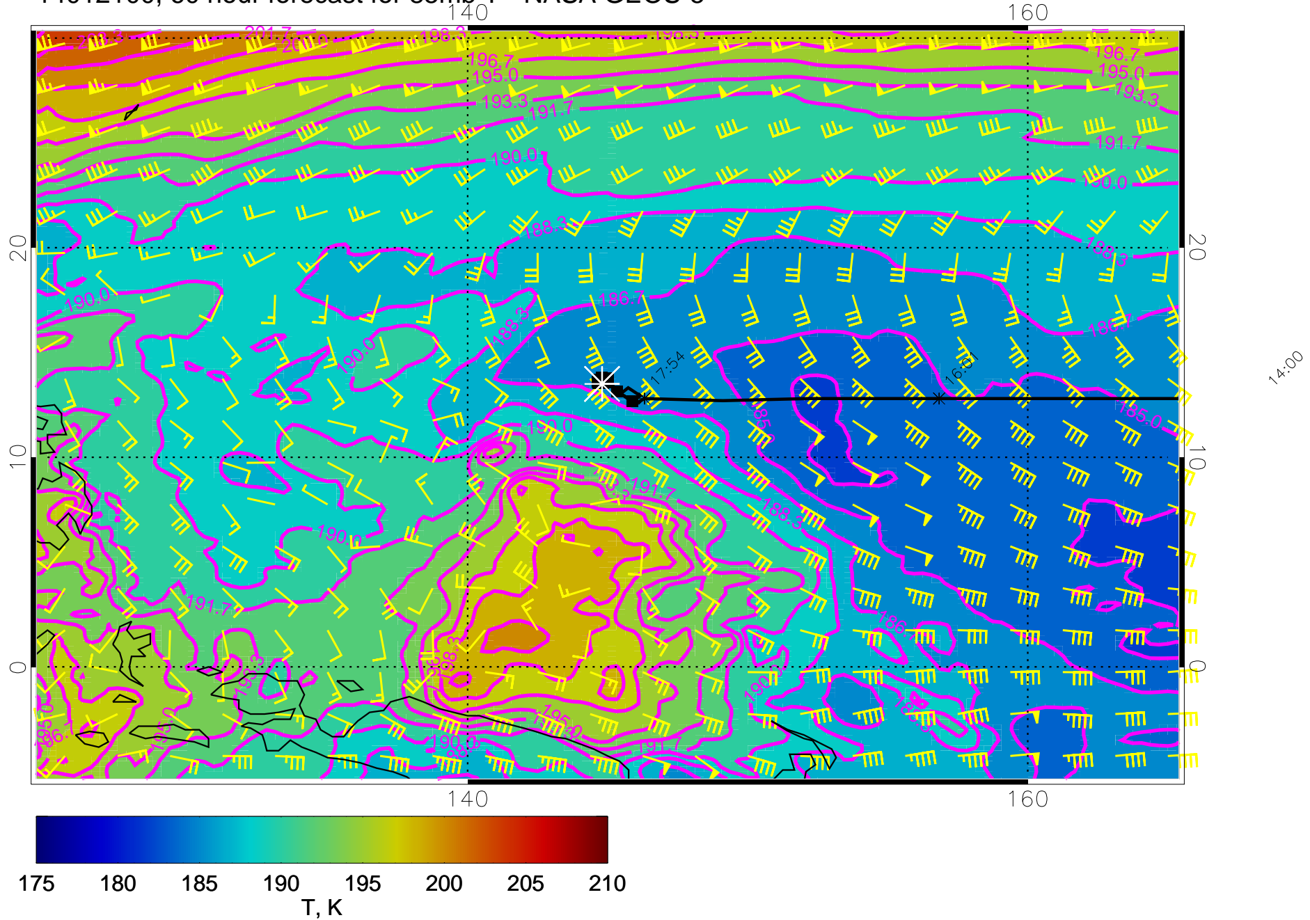
14012100, 60 hour forecast for 85mb T - NASA GEOS-5
