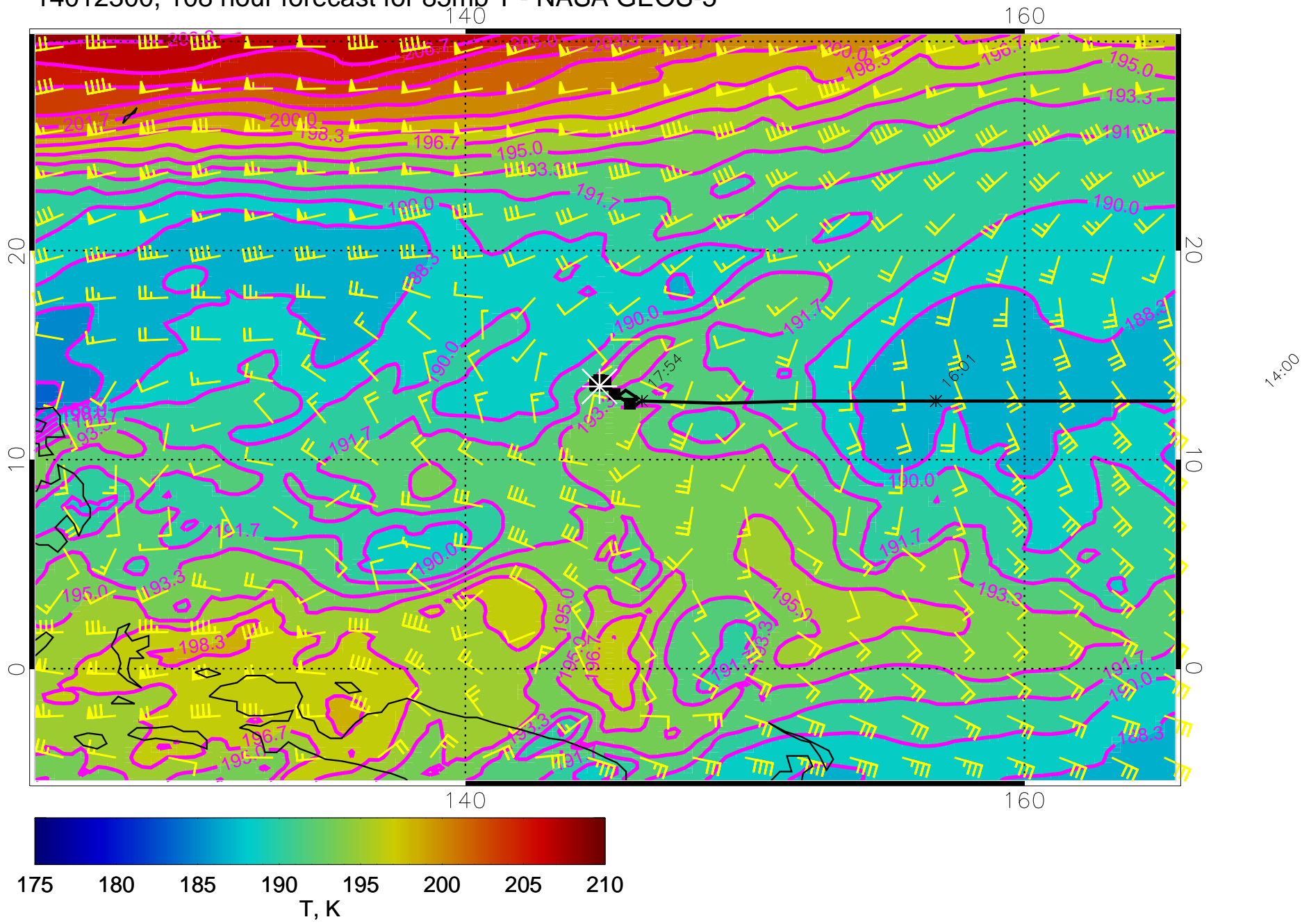
14012300, 108 hour forecast for 85mb T - NASA GEOS-5
