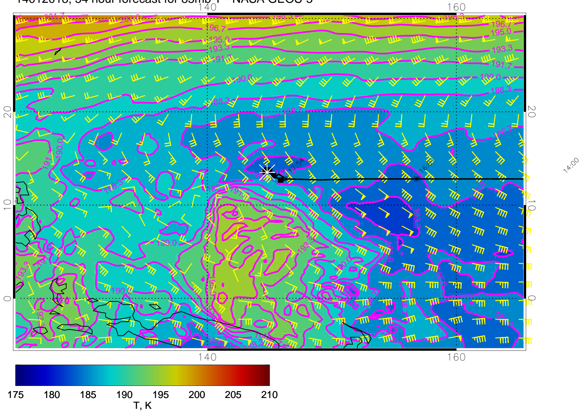
14012018, 54 hour forecast for 85mb T - NASA GEOS-5
