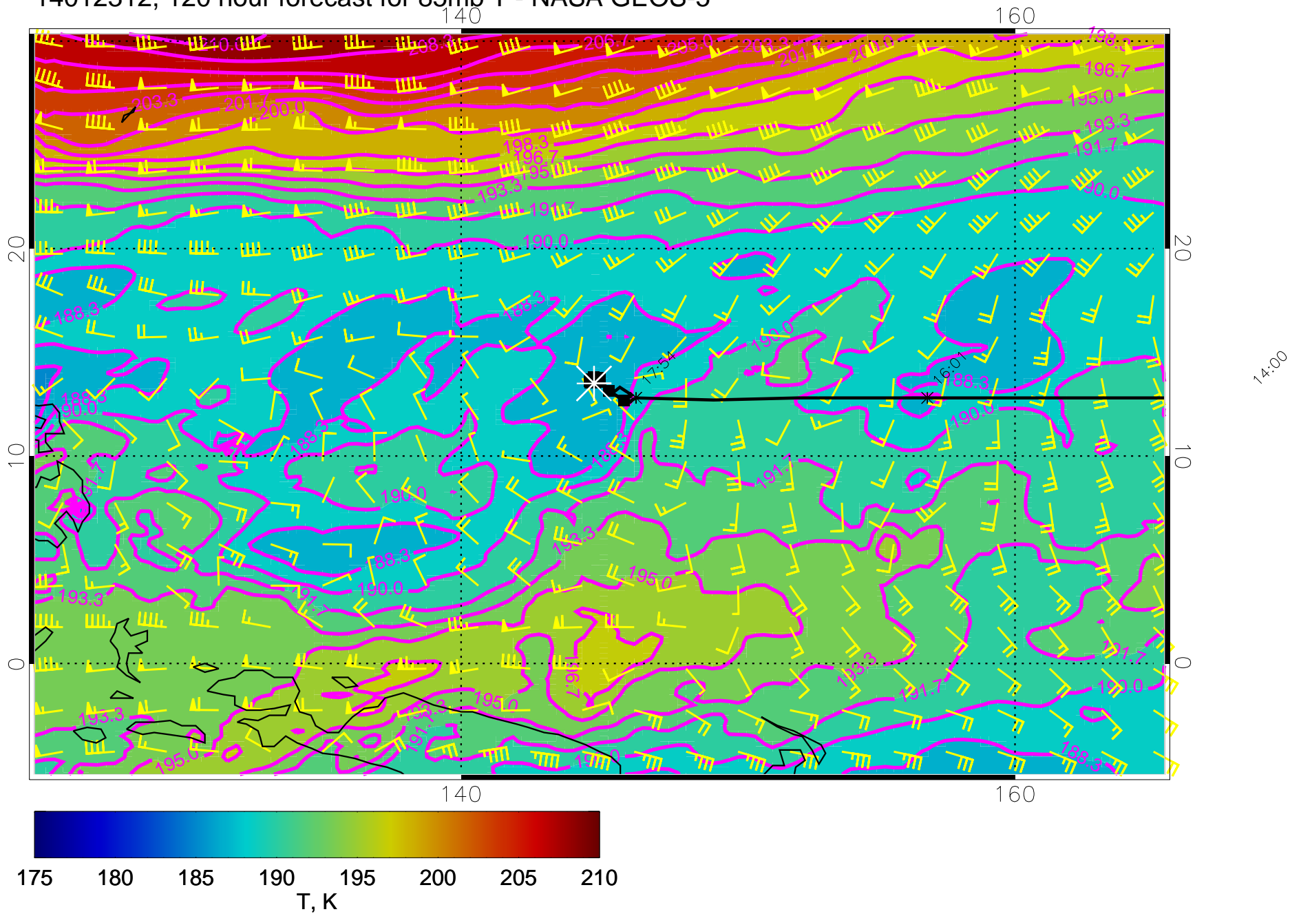
14012312, 120 hour forecast for 85mb T - NASA GEOS-5
