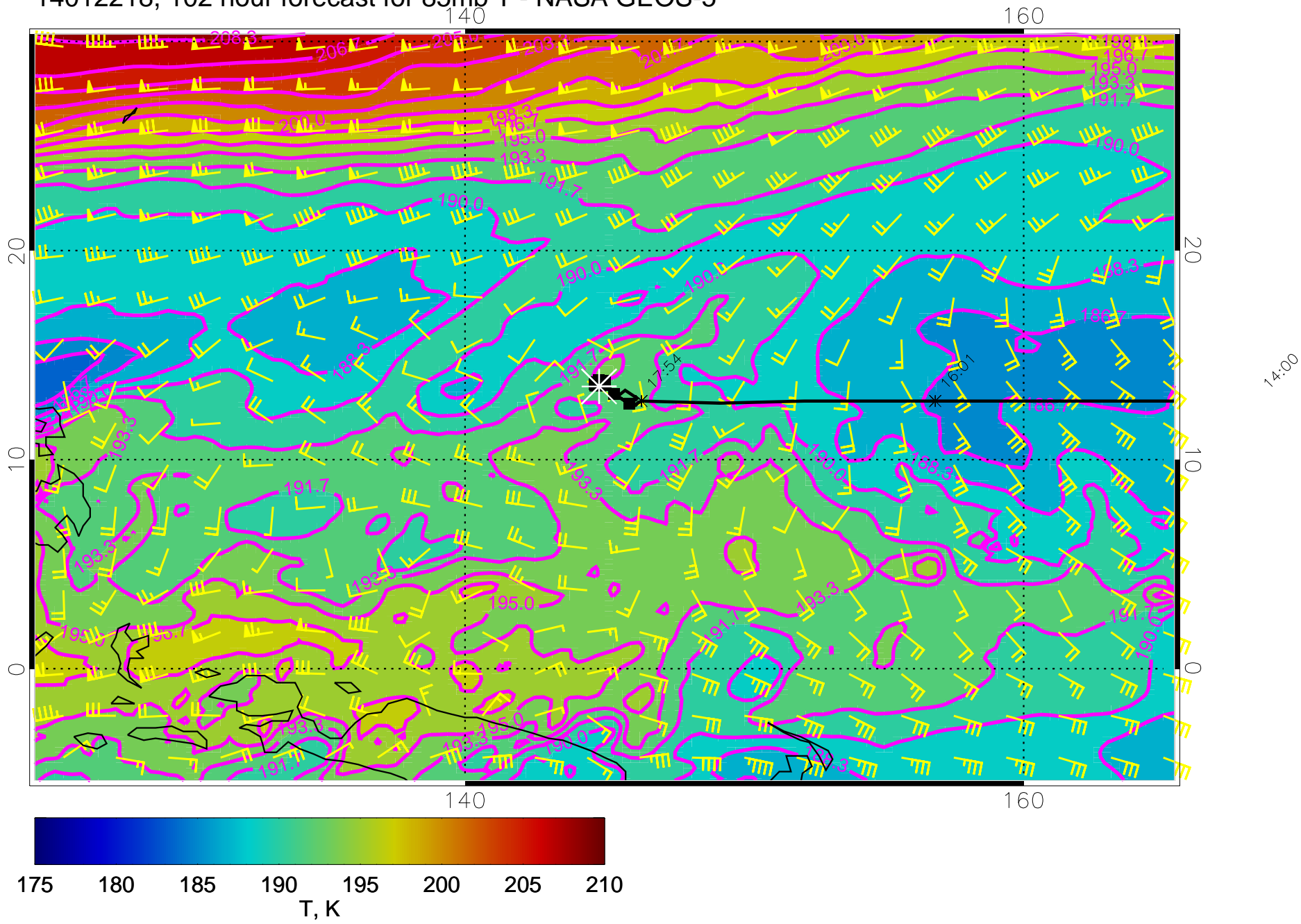
14012218, 102 hour forecast for 85mb T - NASA GEOS-5
