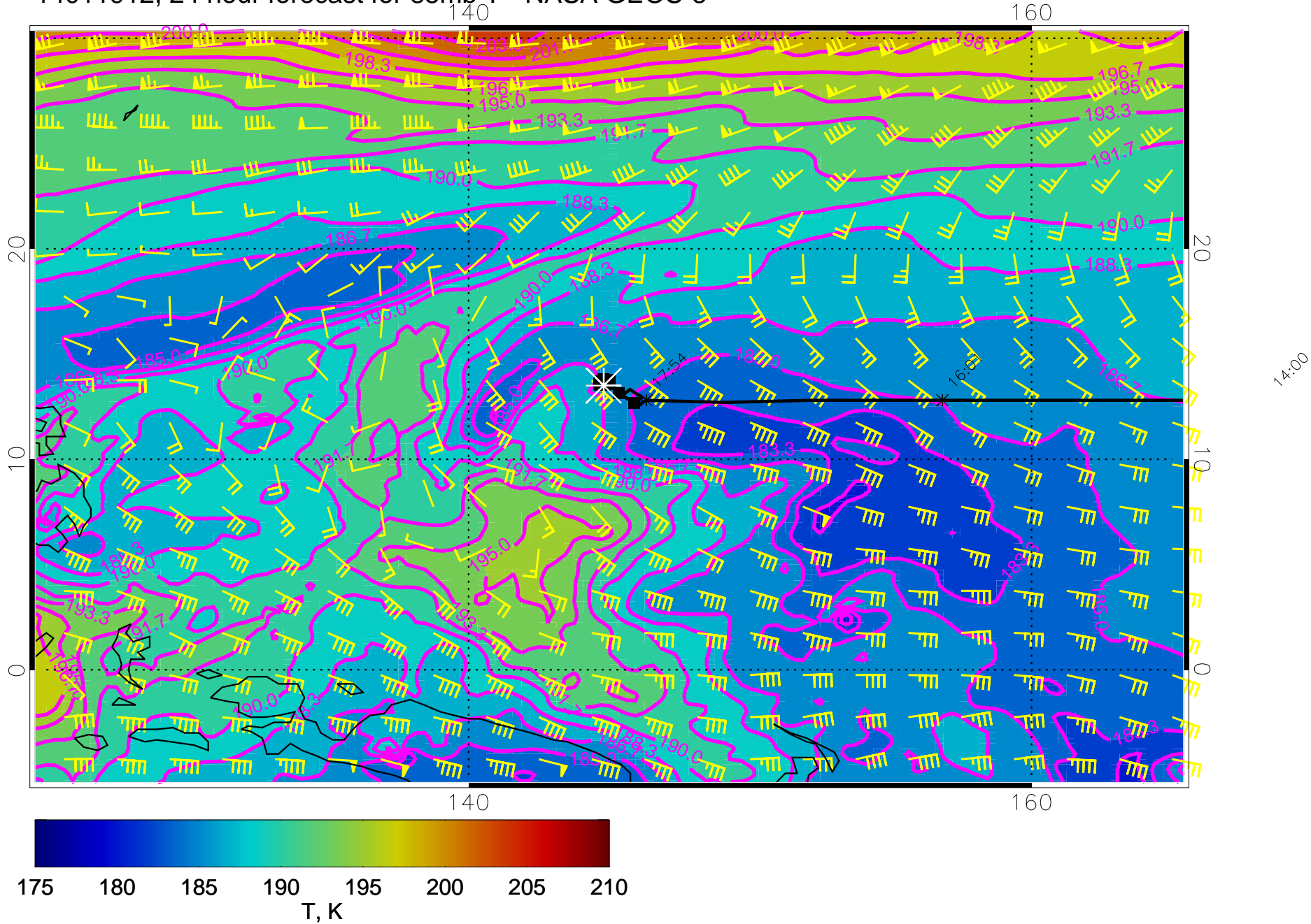
14011912, 24 hour forecast for 85mb T - NASA GEOS-5
