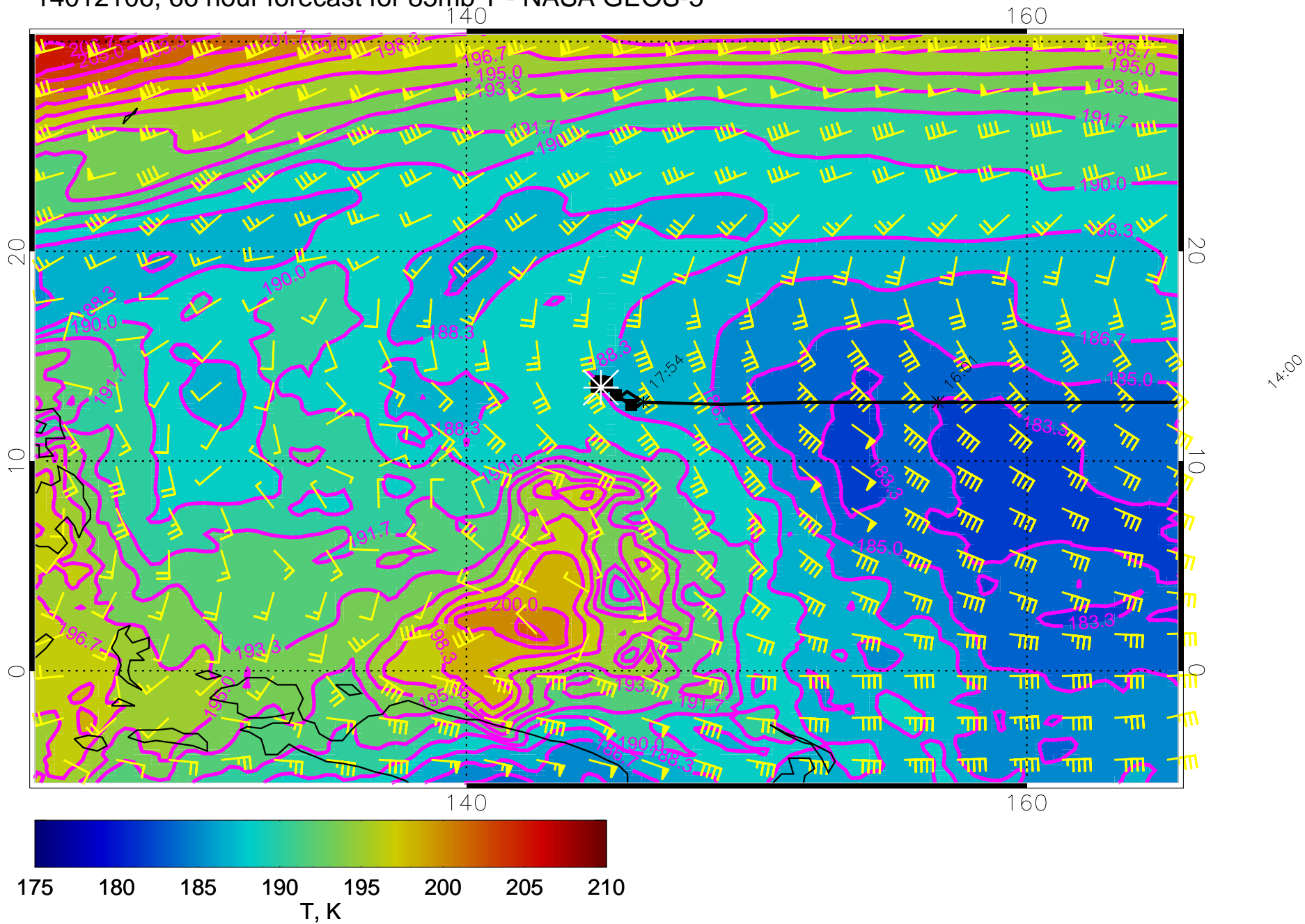
14012106, 66 hour forecast for 85mb T - NASA GEOS-5
