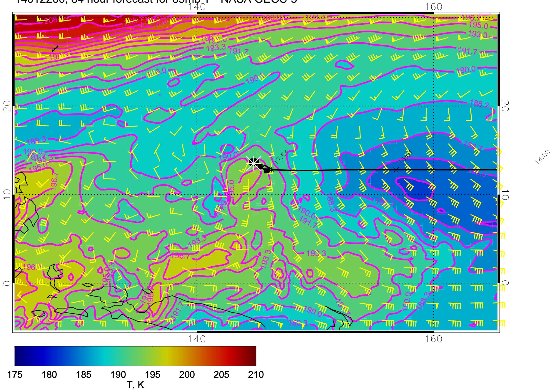
14012200, 84 hour forecast for 85mb T - NASA GEOS-5
