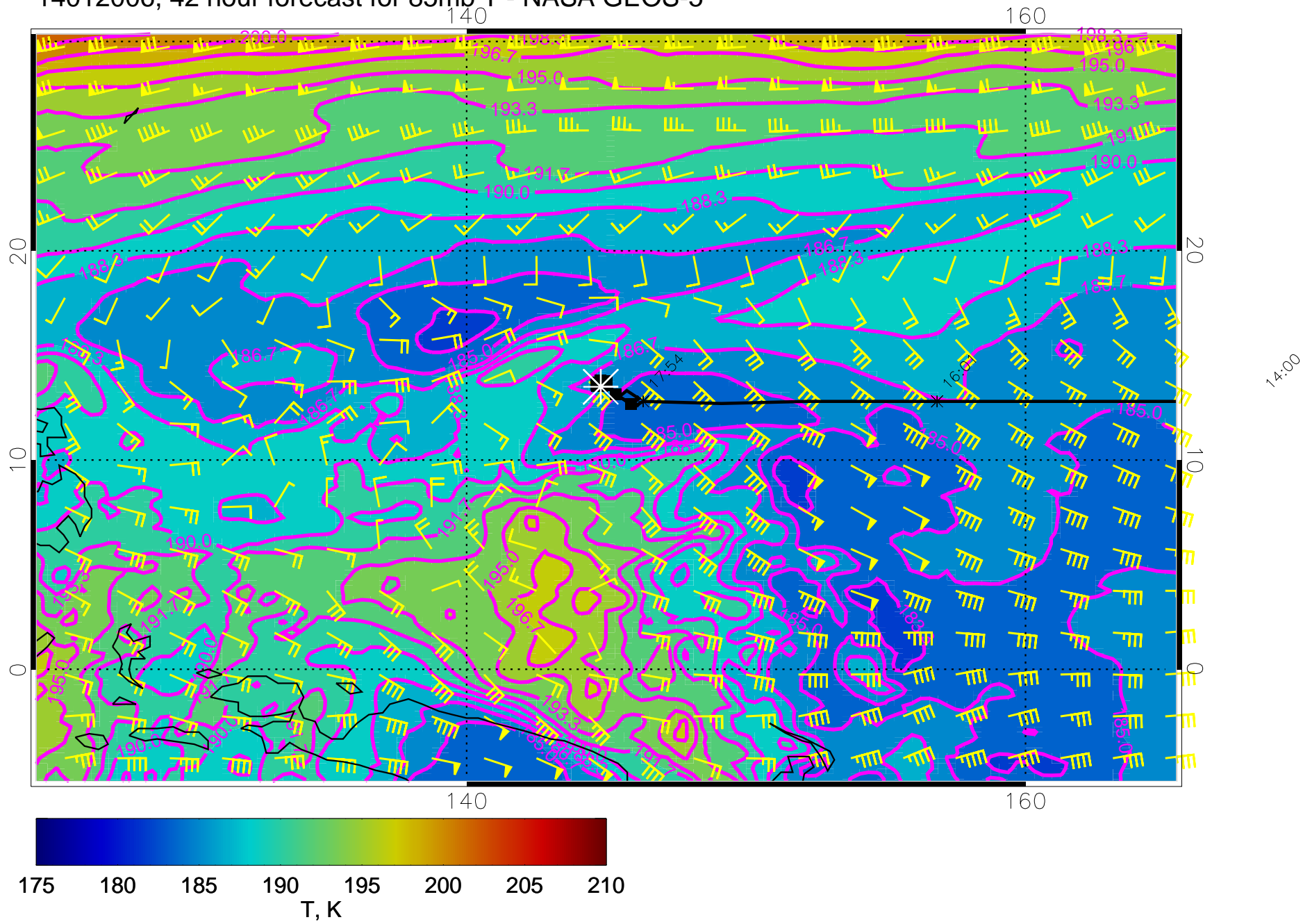
14012006, 42 hour forecast for 85mb T - NASA GEOS-5
