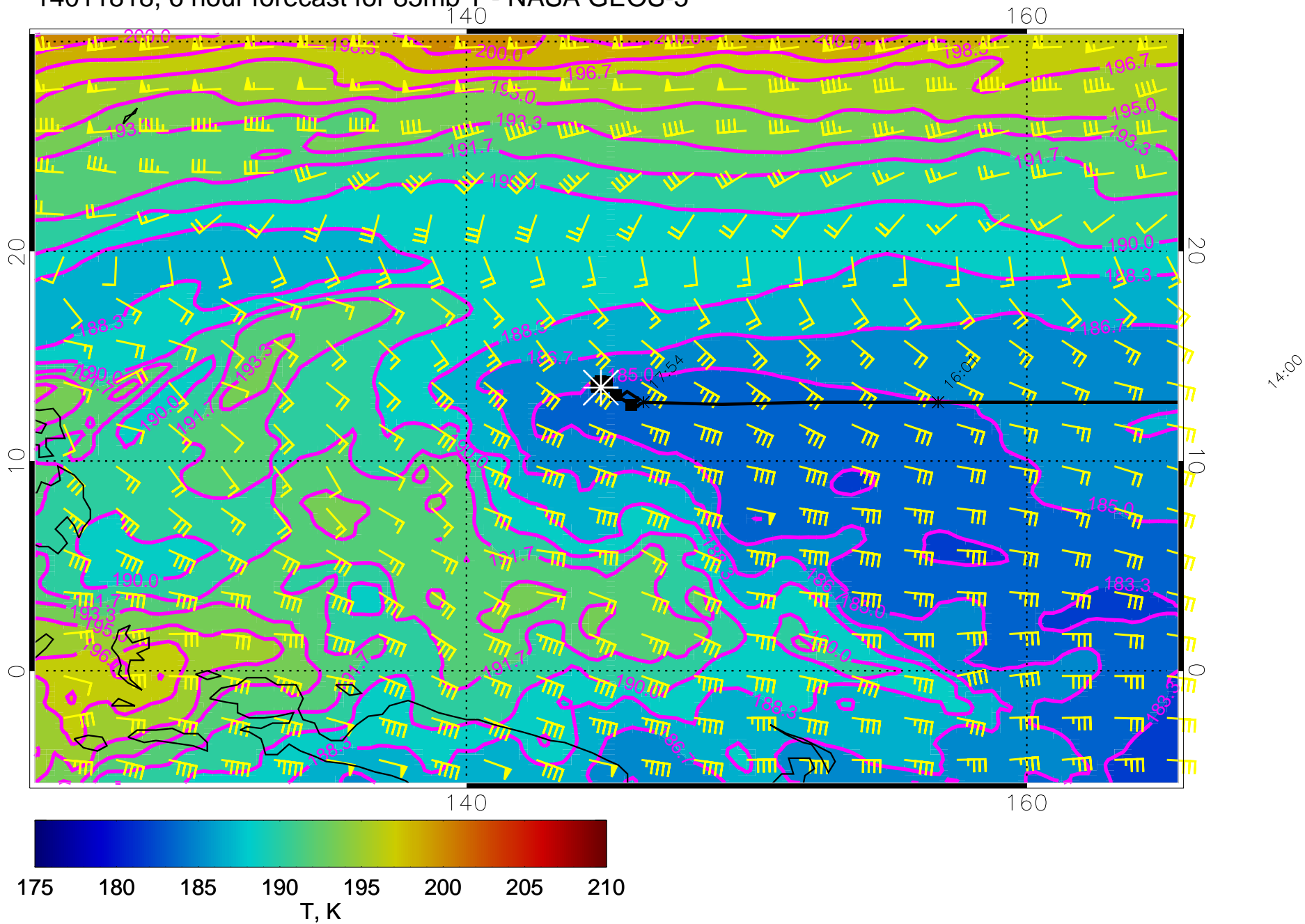
14011818, 6 hour forecast for 85mb T - NASA GEOS-5
