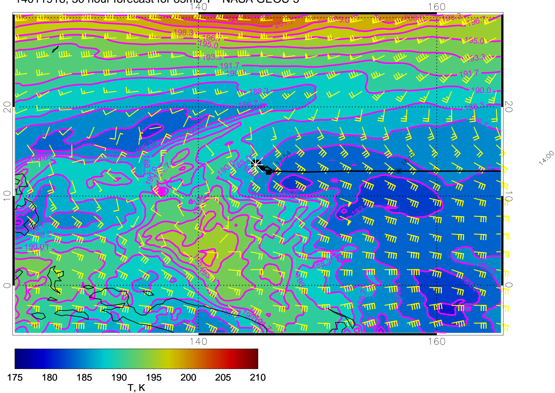
14011918, 30 hour forecast for 85mb T - NASA GEOS-5
