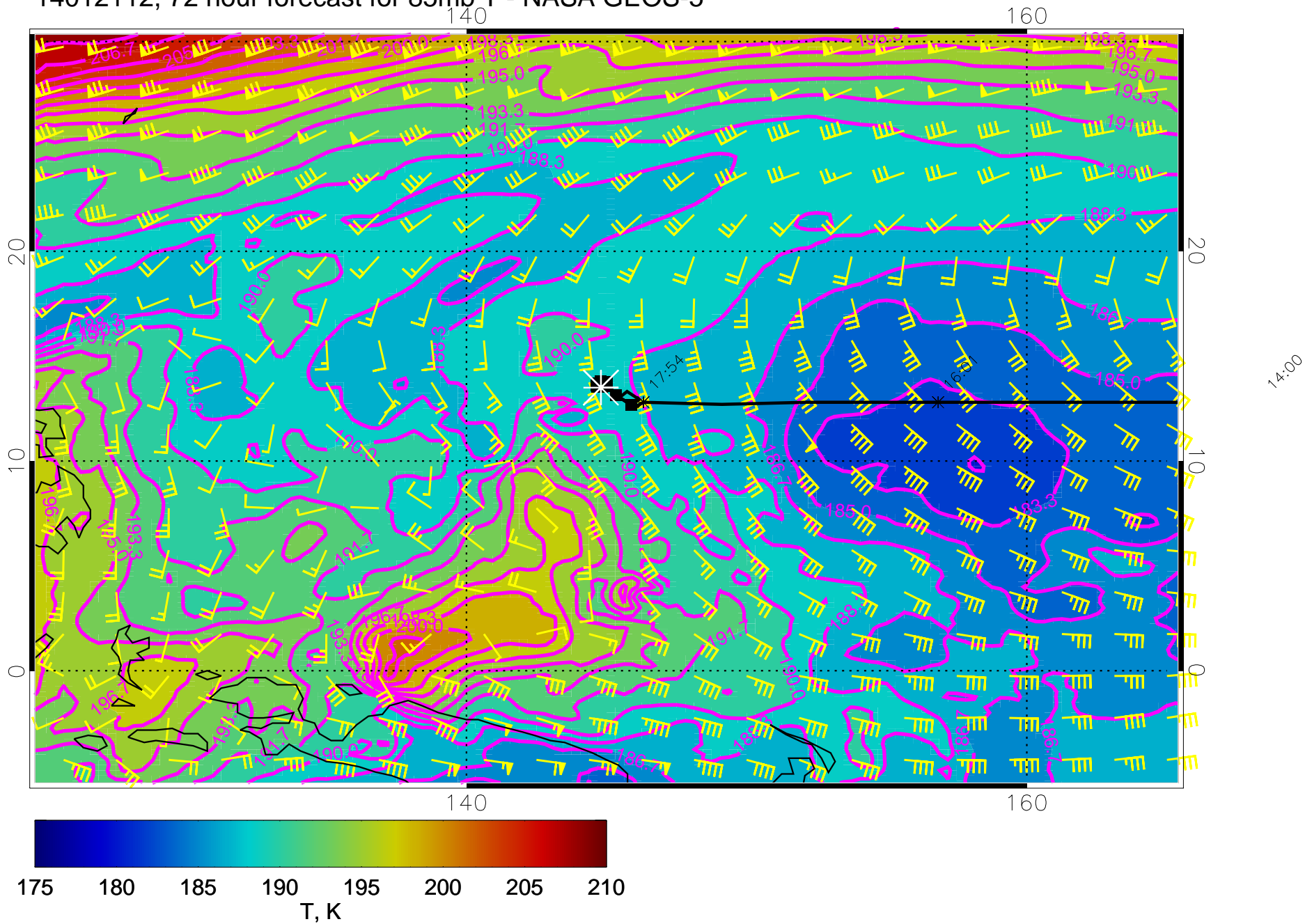
14012112, 72 hour forecast for 85mb T - NASA GEOS-5
