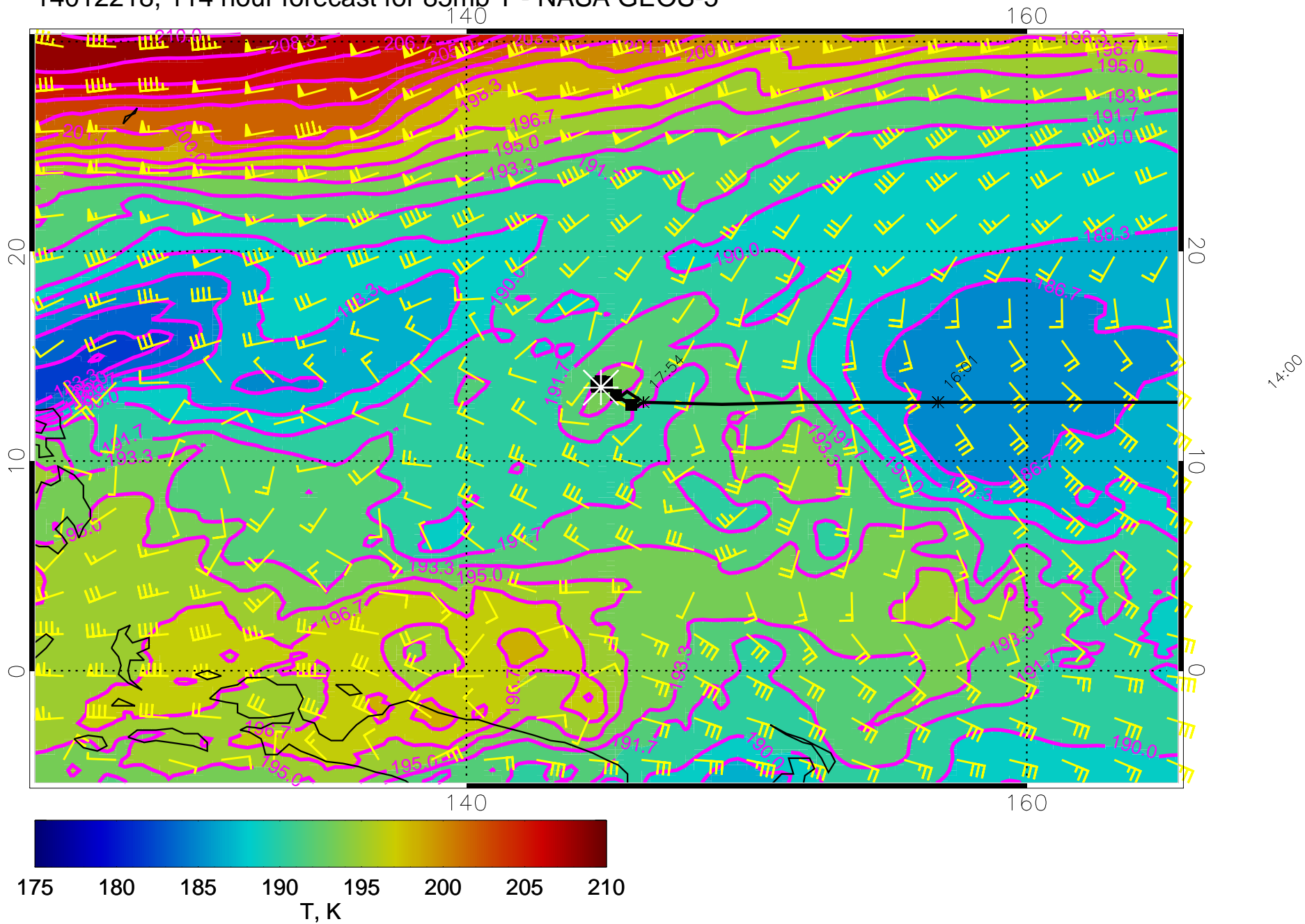
14012218, 114 hour forecast for 85mb T - NASA GEOS-5
