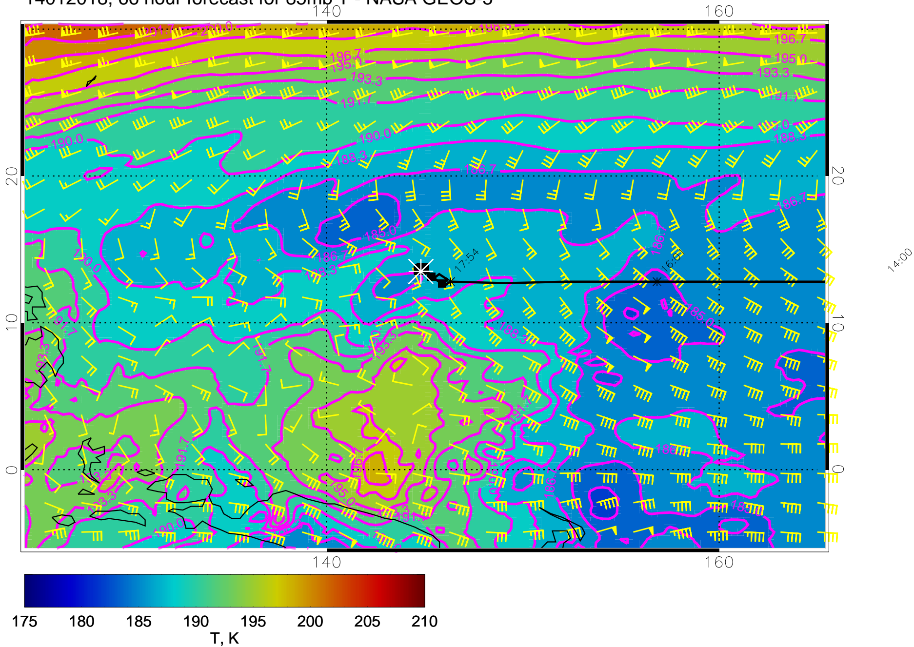
14012018, 66 hour forecast for 85mb T - NASA GEOS-5
