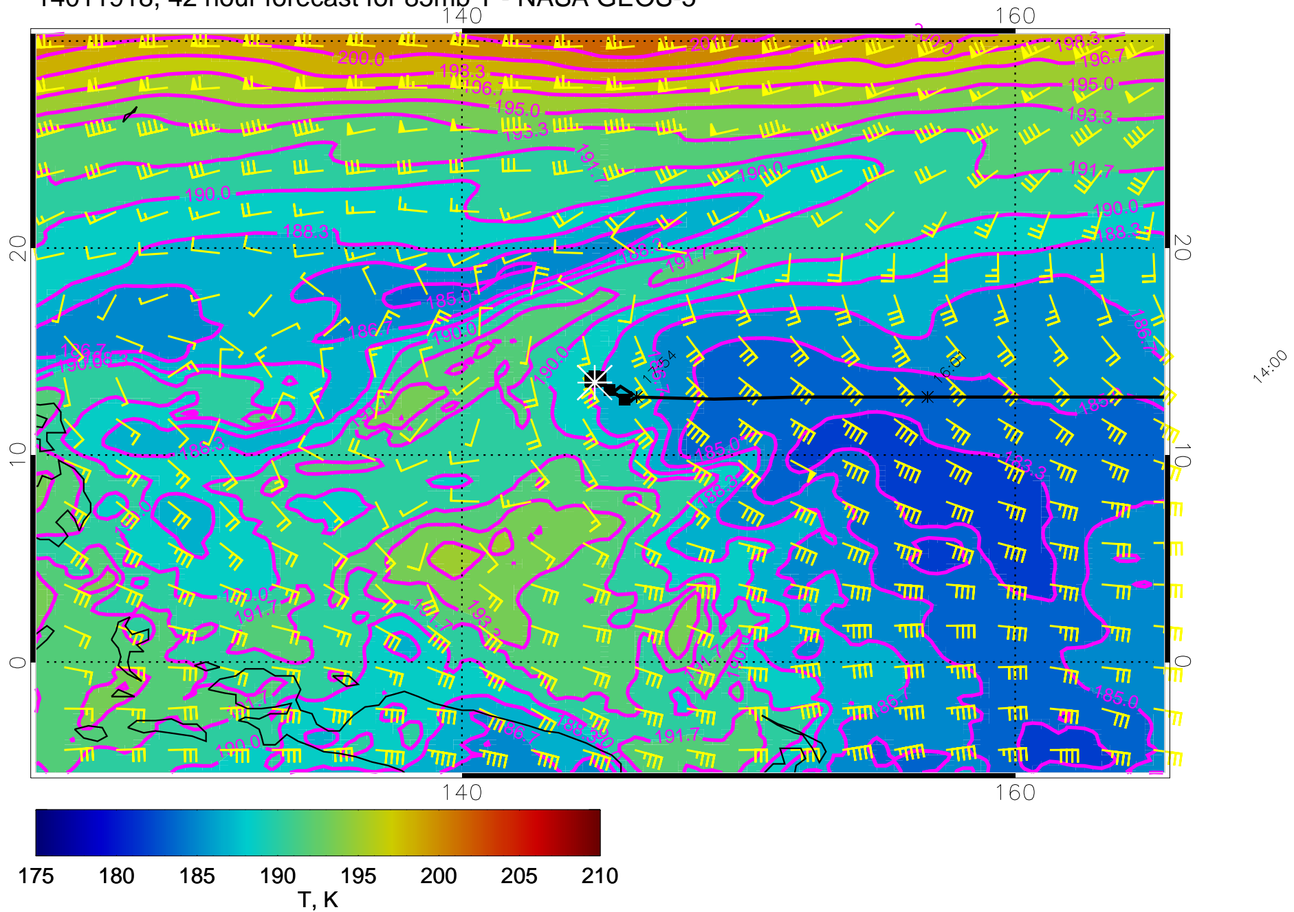
14011918, 42 hour forecast for 85mb T - NASA GEOS-5
