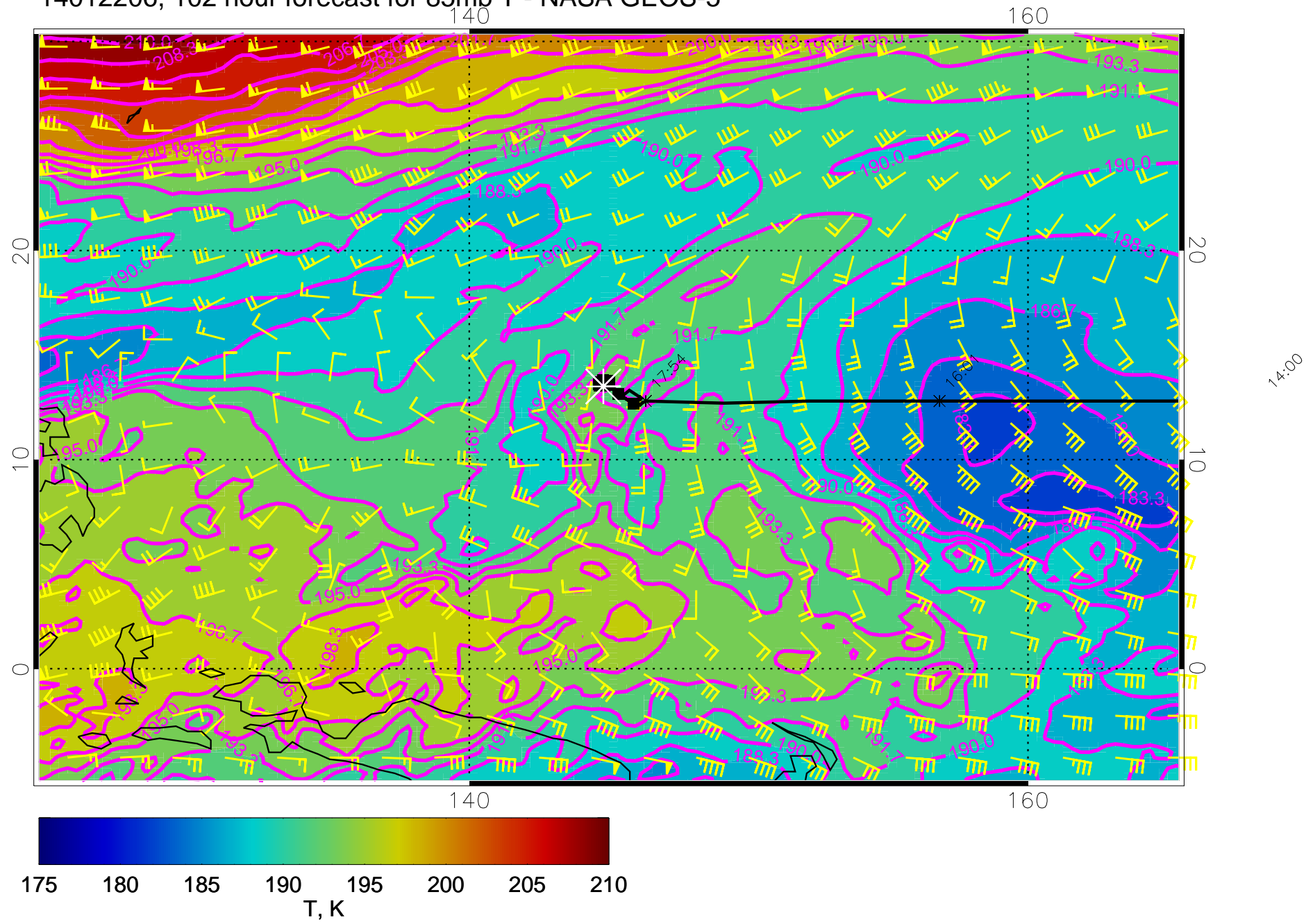
14012206, 102 hour forecast for 85mb T - NASA GEOS-5
