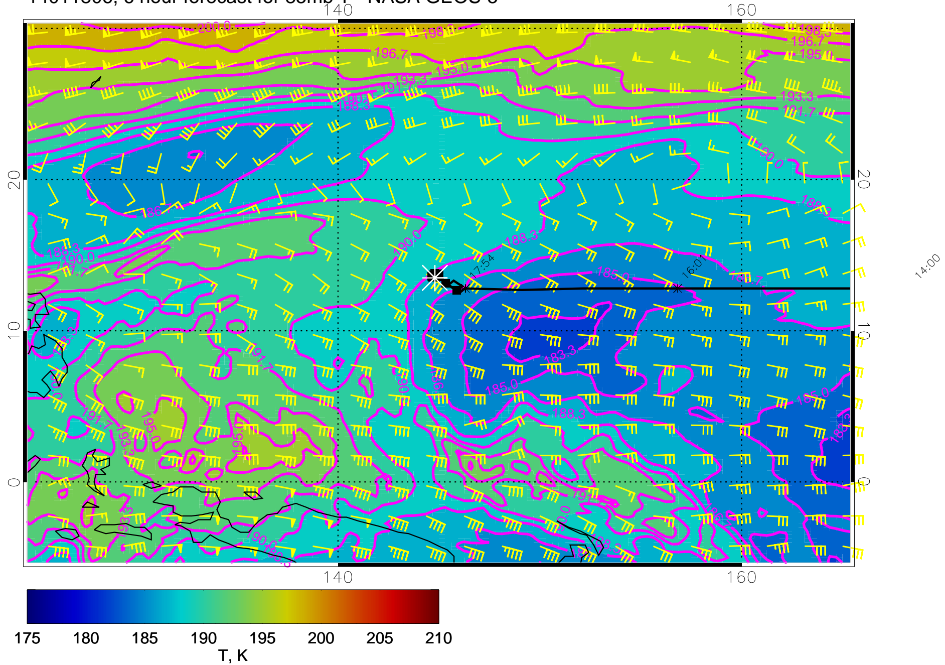
14011806, 6 hour forecast for 85mb T - NASA GEOS-5
