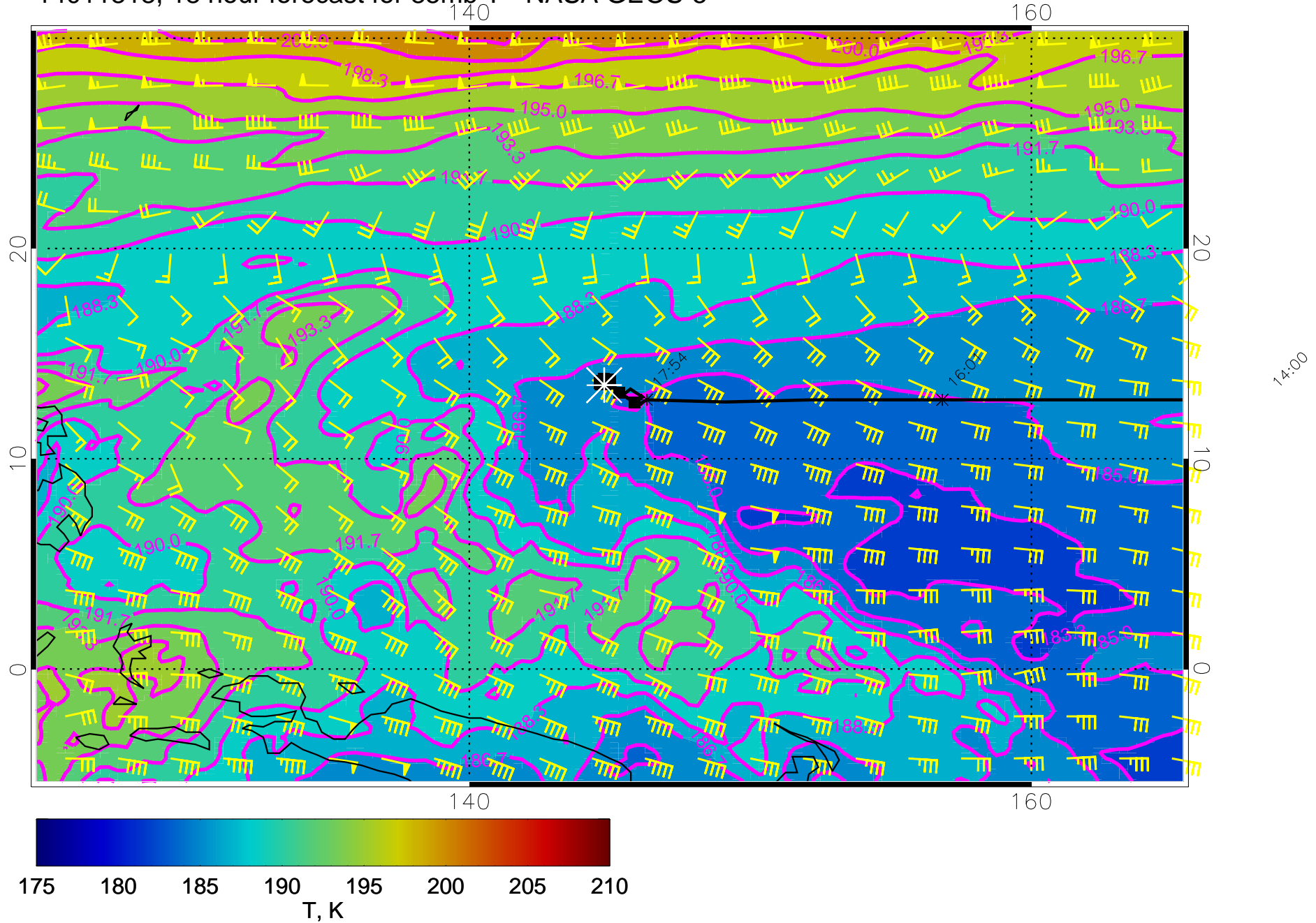
14011818, 18 hour forecast for 85mb T - NASA GEOS-5
