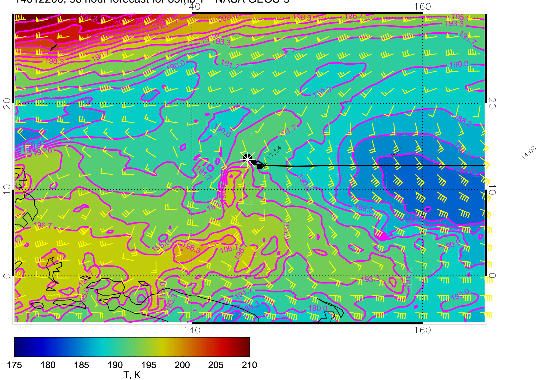
14012200, 96 hour forecast for 85mb T - NASA GEOS-5
