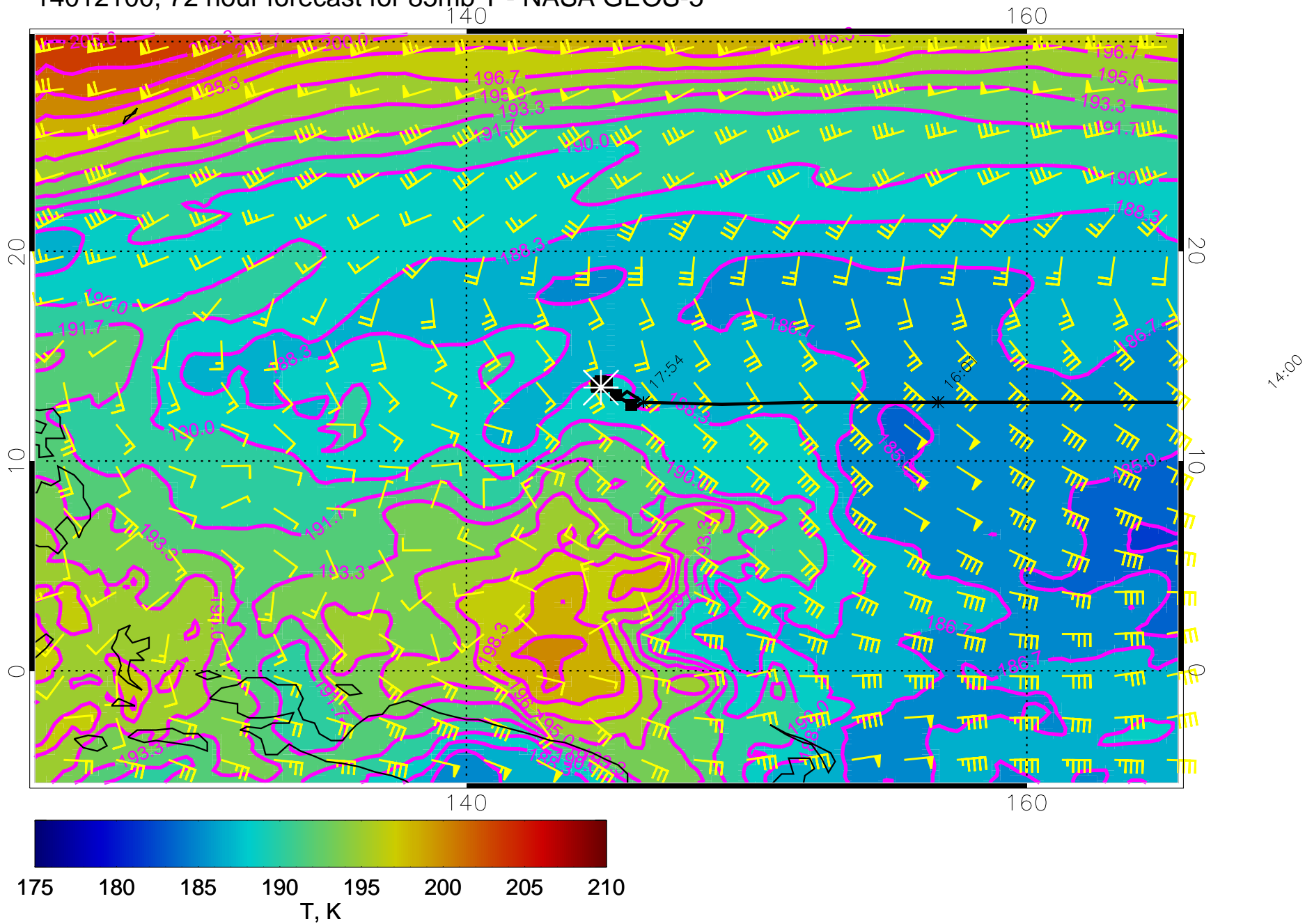
14012100, 72 hour forecast for 85mb T - NASA GEOS-5
