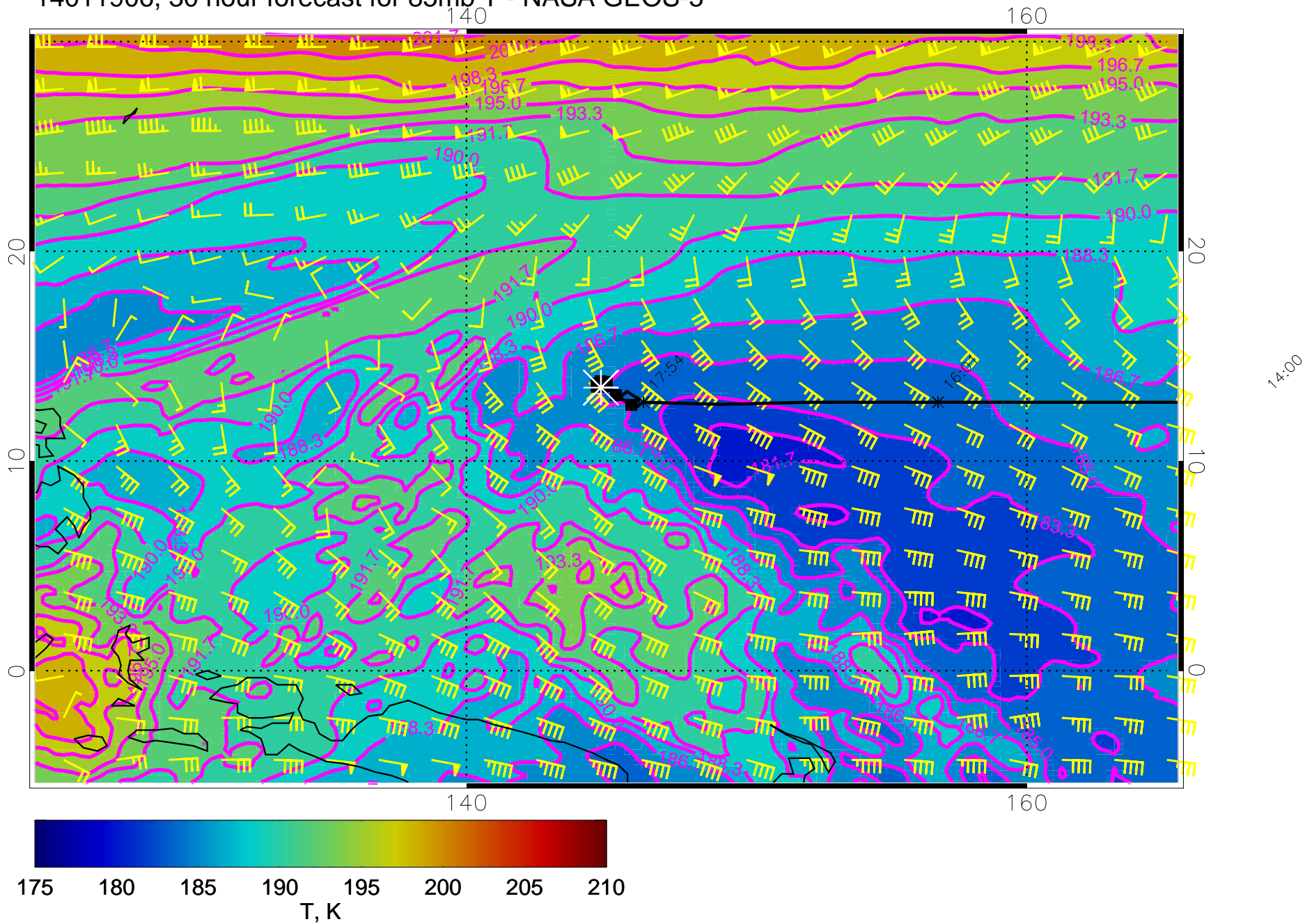
14011906, 30 hour forecast for 85mb T - NASA GEOS-5
