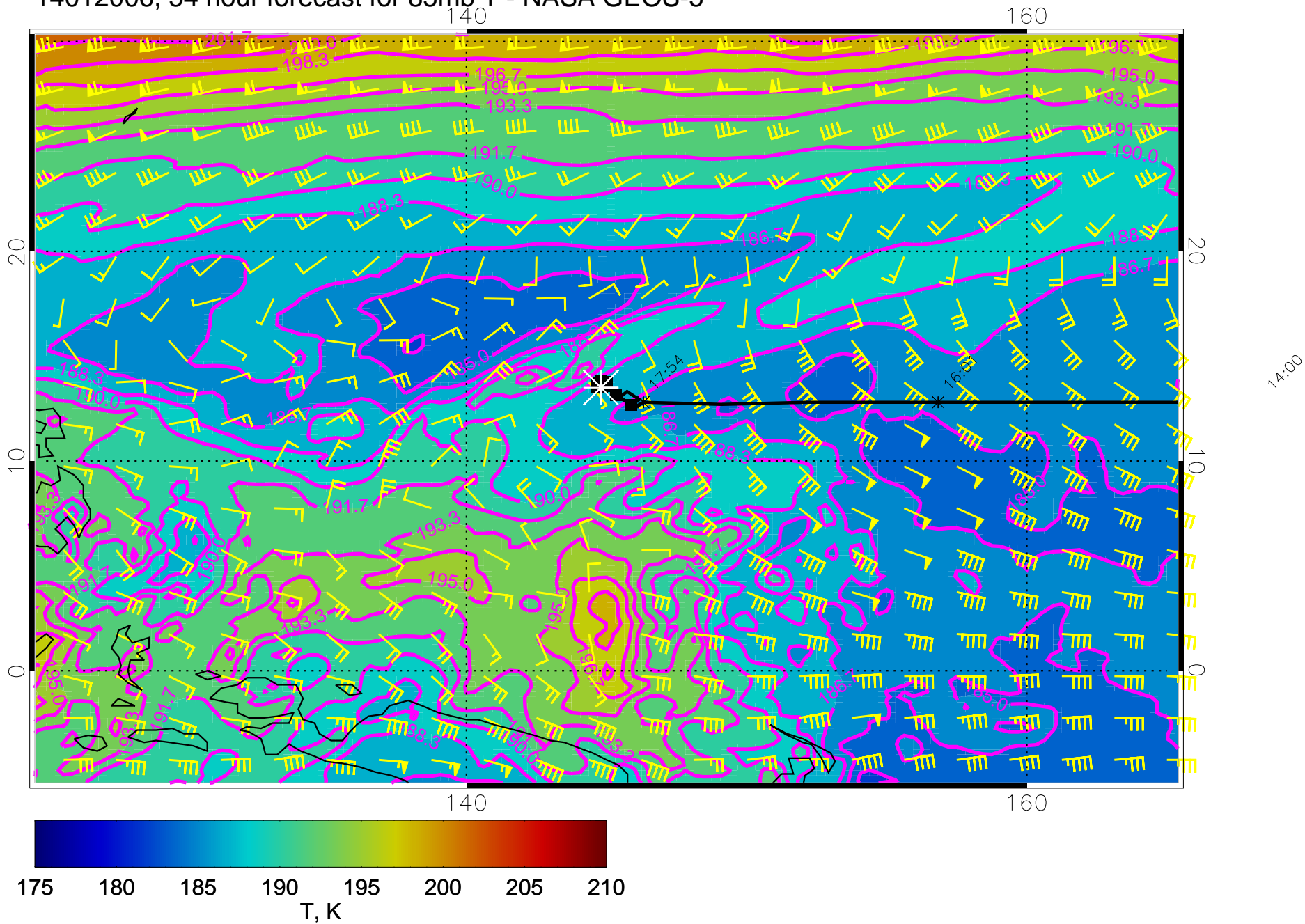
14012006, 54 hour forecast for 85mb T - NASA GEOS-5
