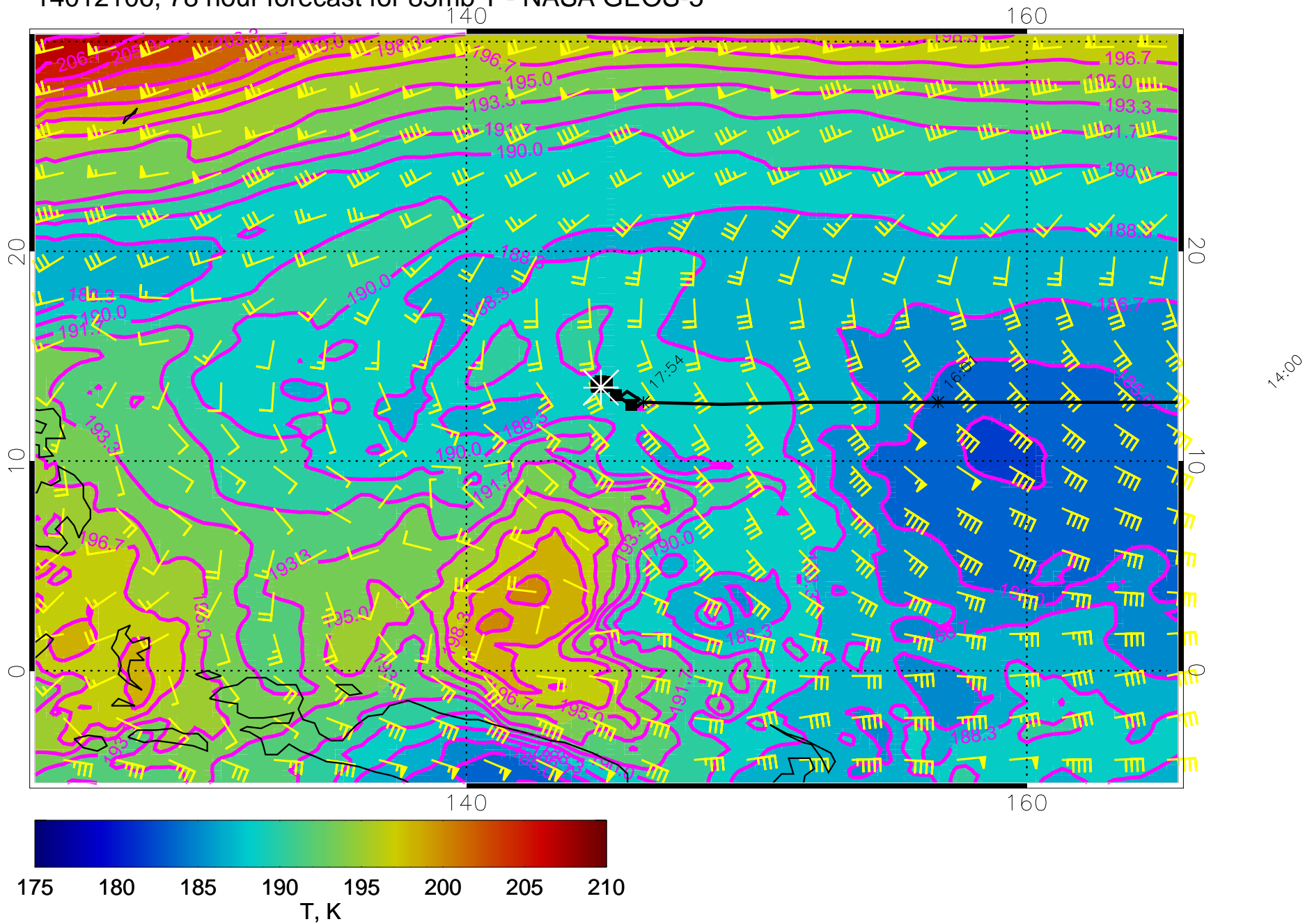
14012106, 78 hour forecast for 85mb T - NASA GEOS-5
