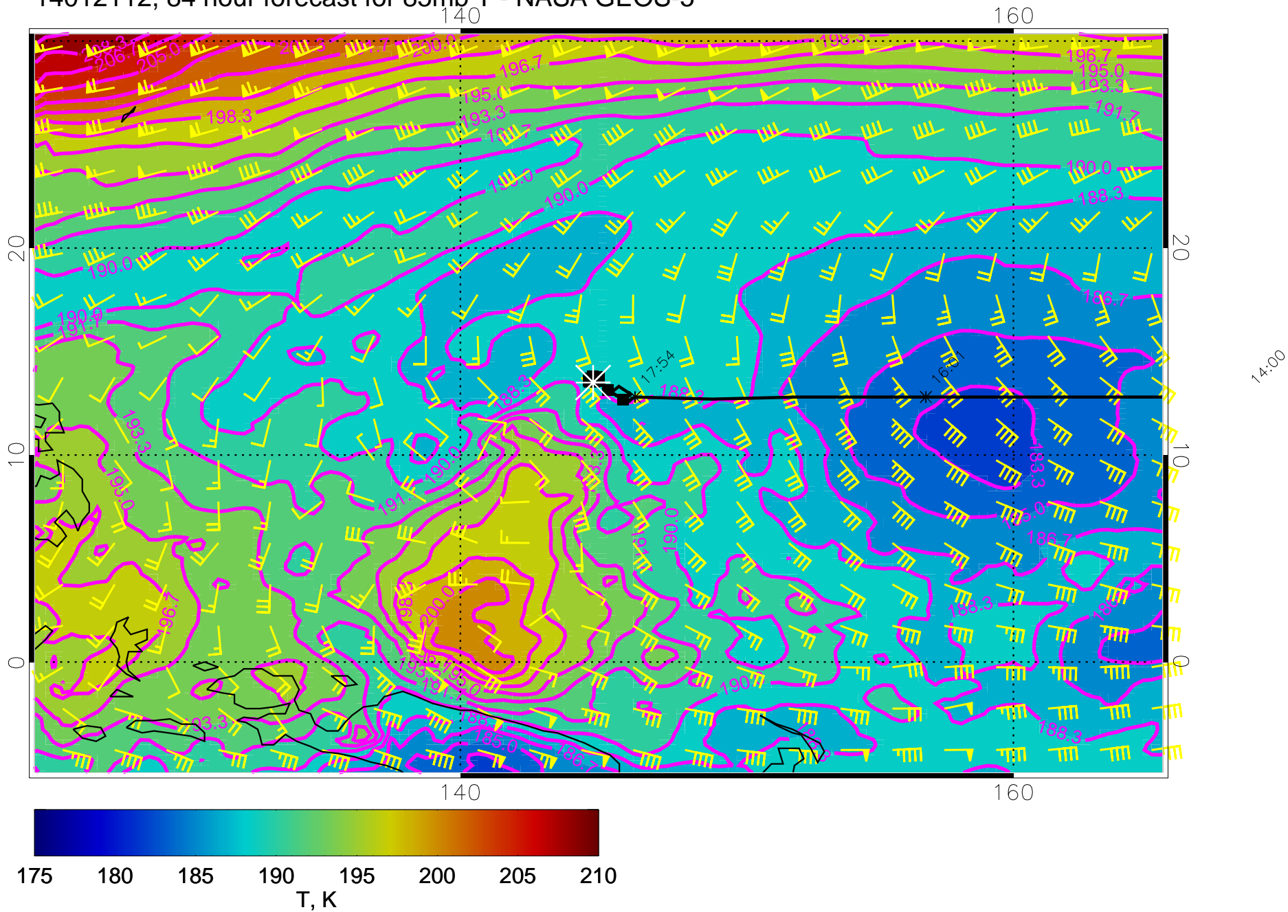
14012112, 84 hour forecast for 85mb T - NASA GEOS-5
