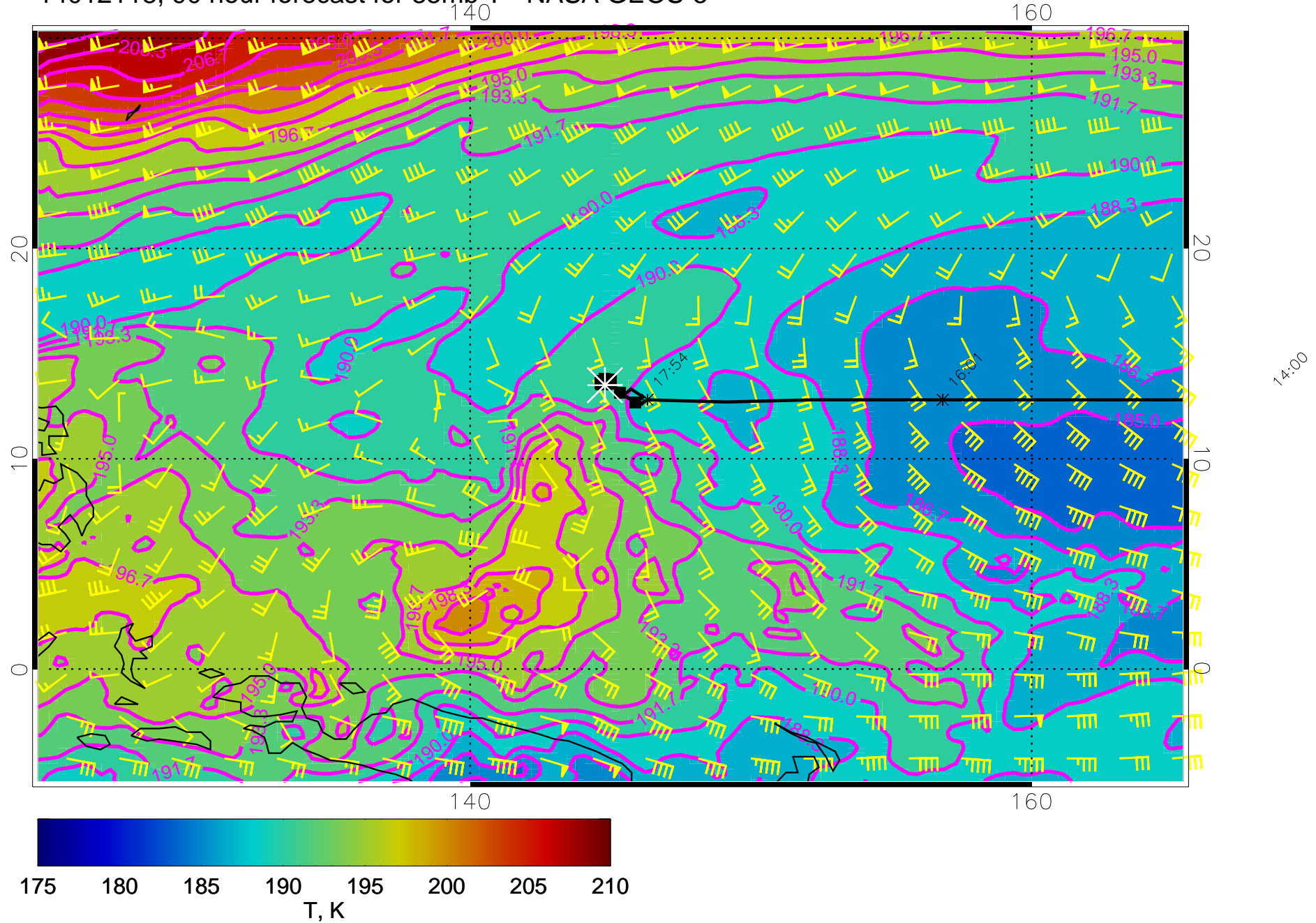
14012118, 90 hour forecast for 85mb T - NASA GEOS-5
