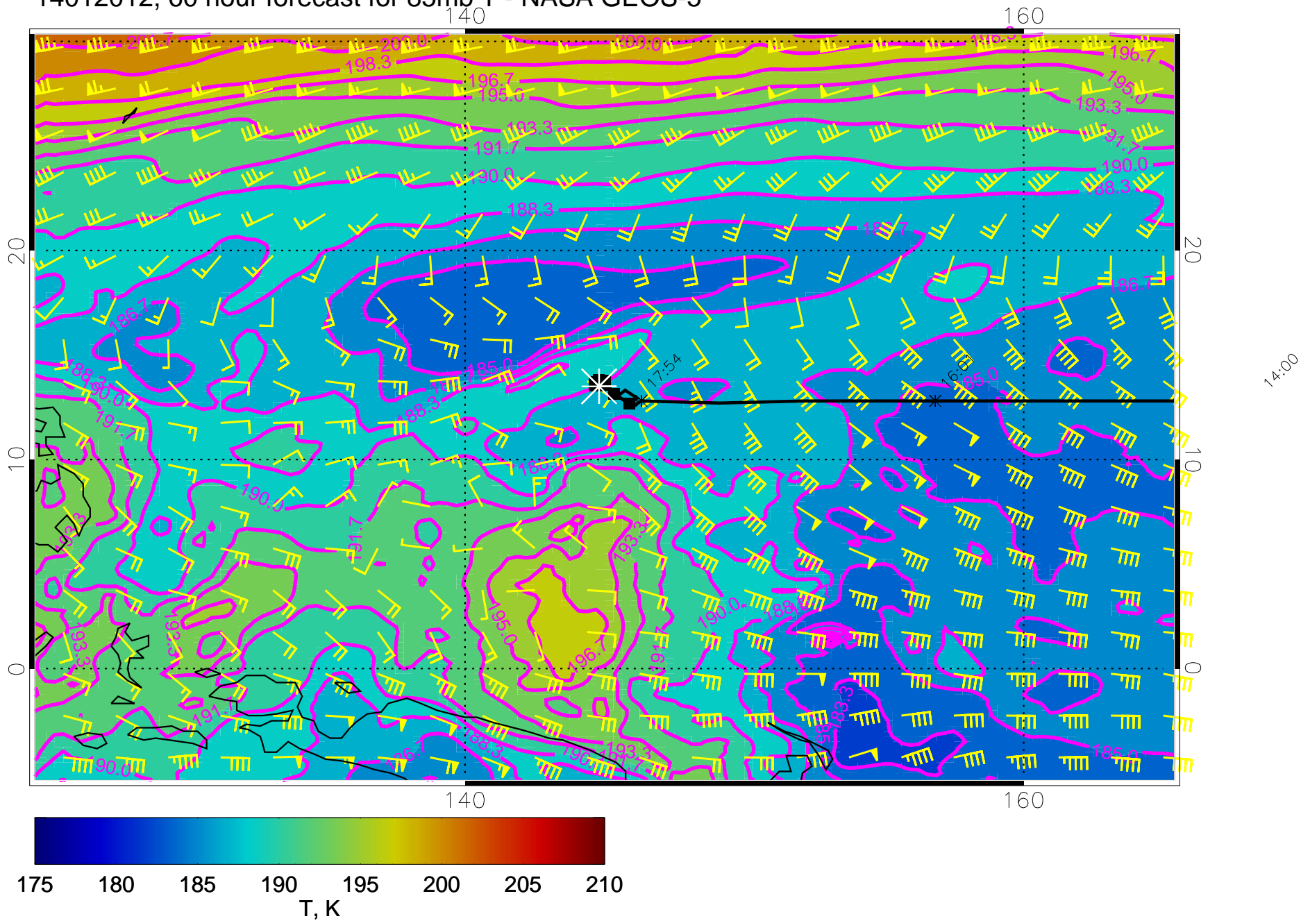
14012012, 60 hour forecast for 85mb T - NASA GEOS-5
