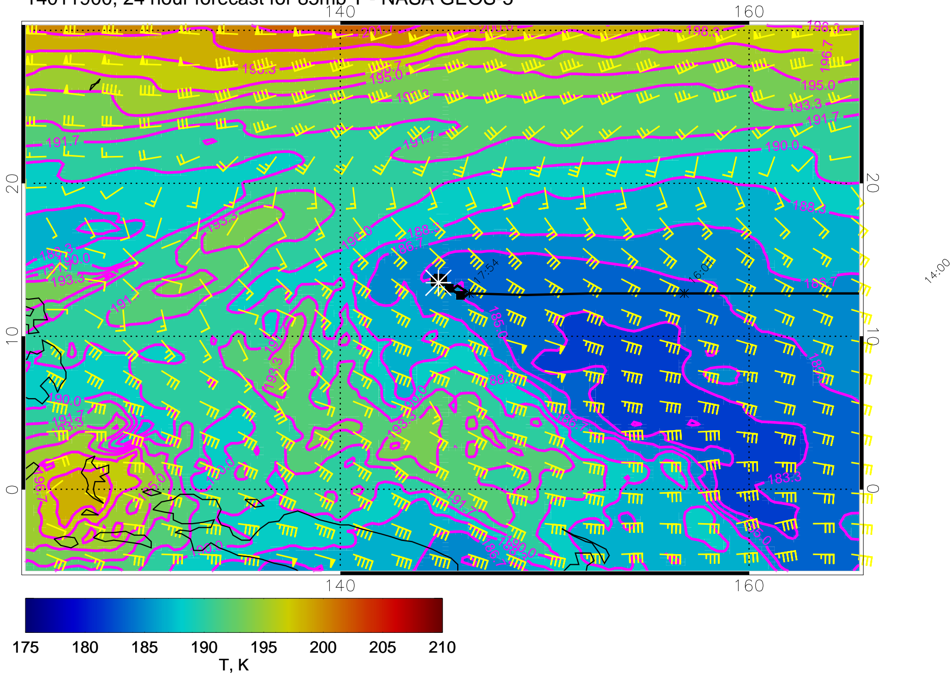
14011900, 24 hour forecast for 85mb T - NASA GEOS-5
