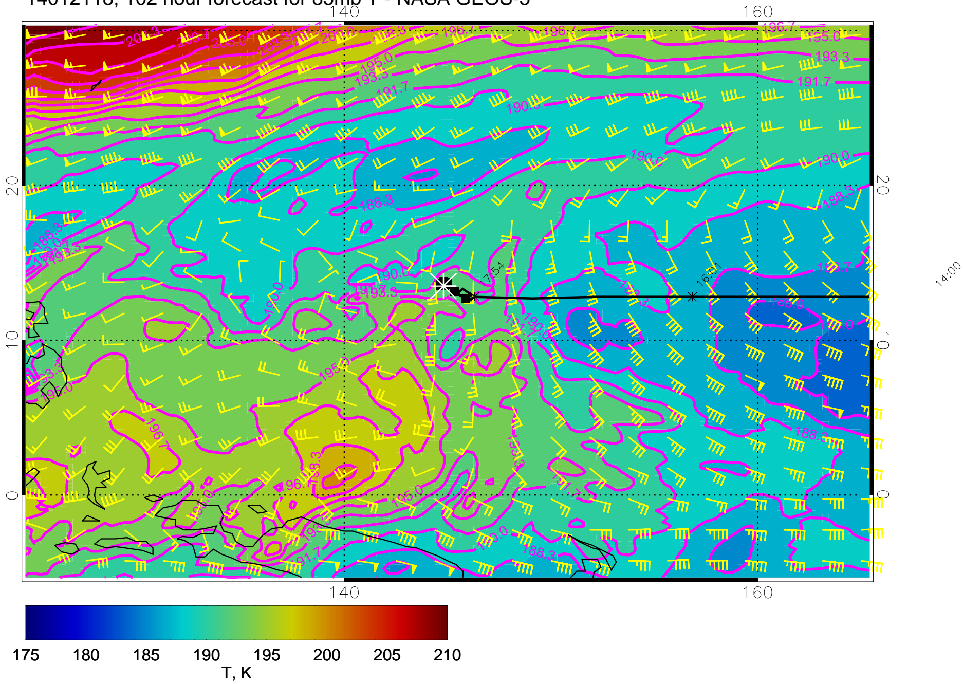
14012118, 102 hour forecast for 85mb T - NASA GEOS-5
