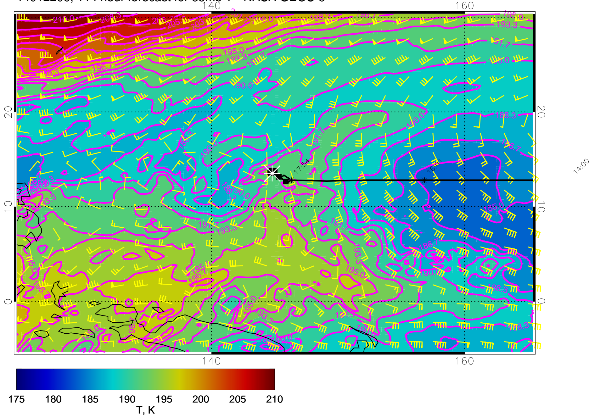
14012206, 114 hour forecast for 85mb T - NASA GEOS-5
