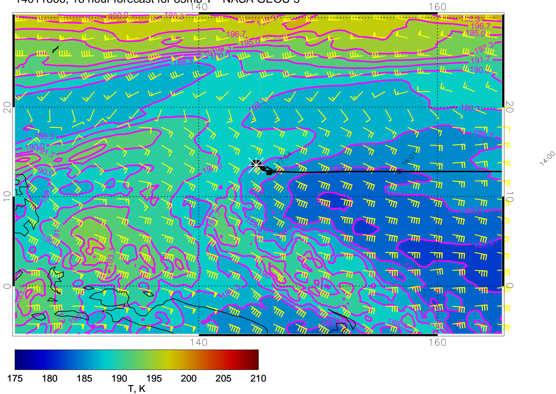
14011806, 18 hour forecast for 85mb T - NASA GEOS-5
