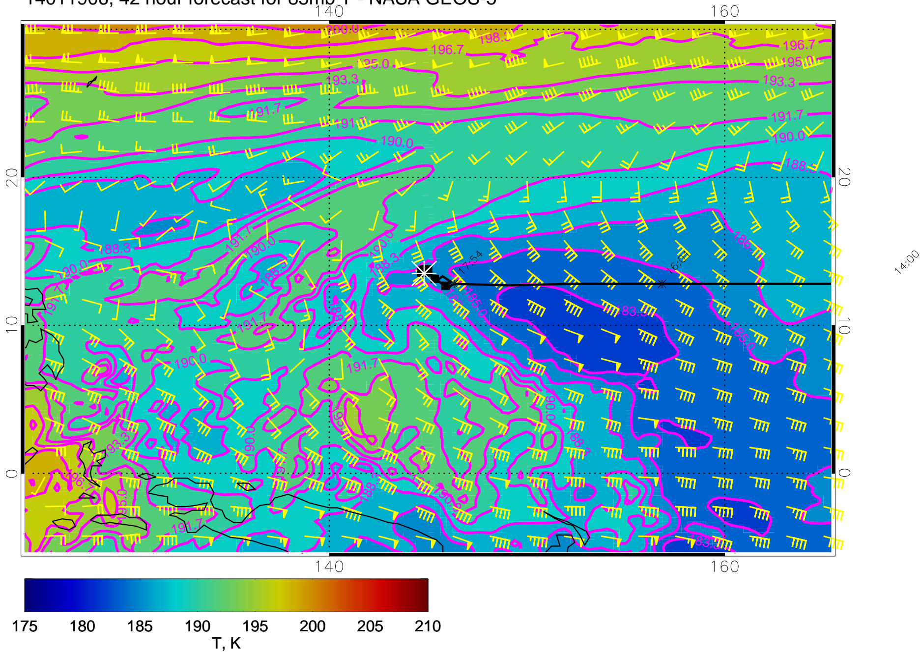
14011906, 42 hour forecast for 85mb T - NASA GEOS-5
