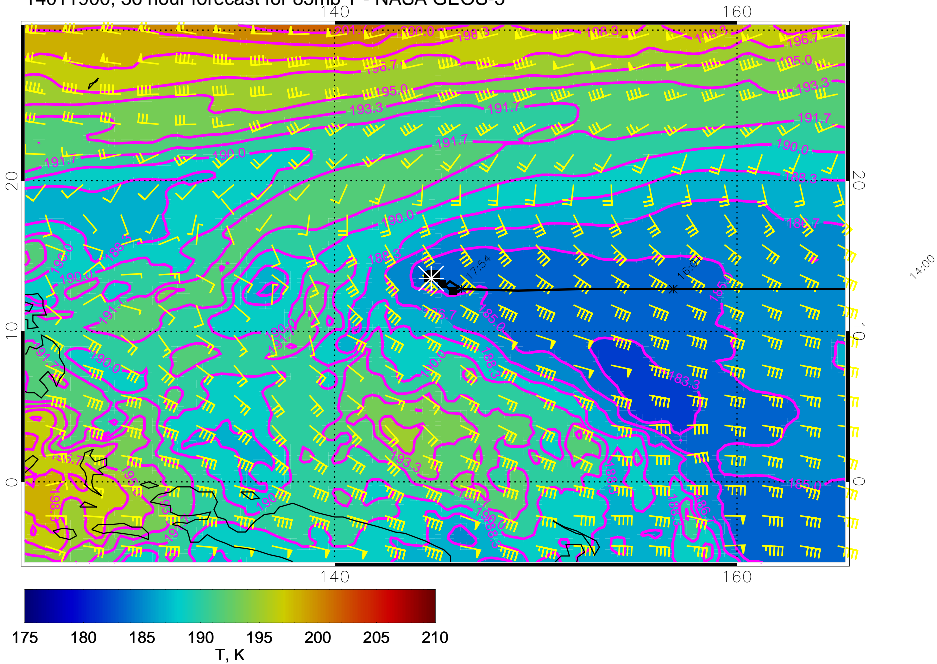
14011900, 36 hour forecast for 85mb T - NASA GEOS-5
