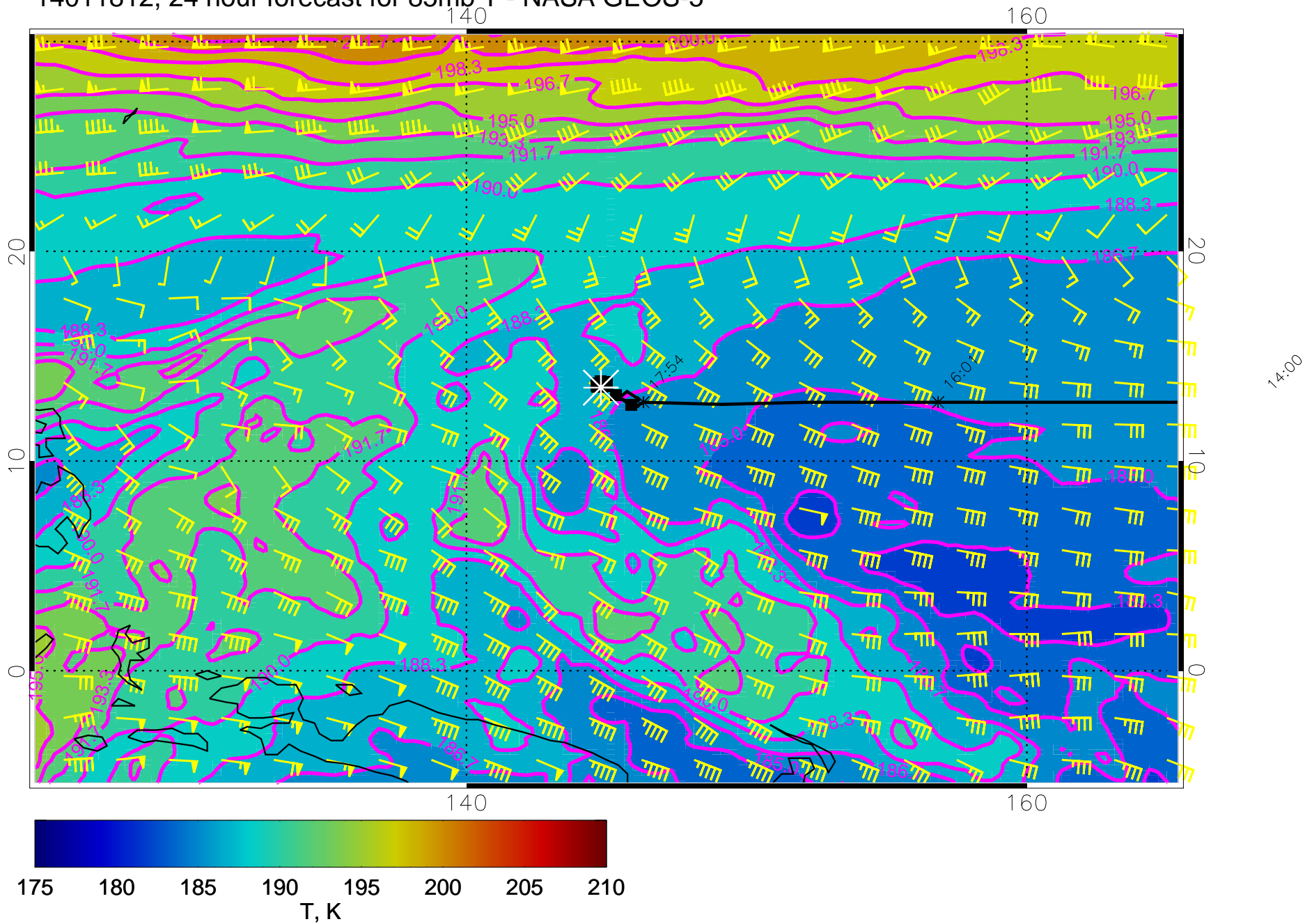
14011812, 24 hour forecast for 85mb T - NASA GEOS-5
