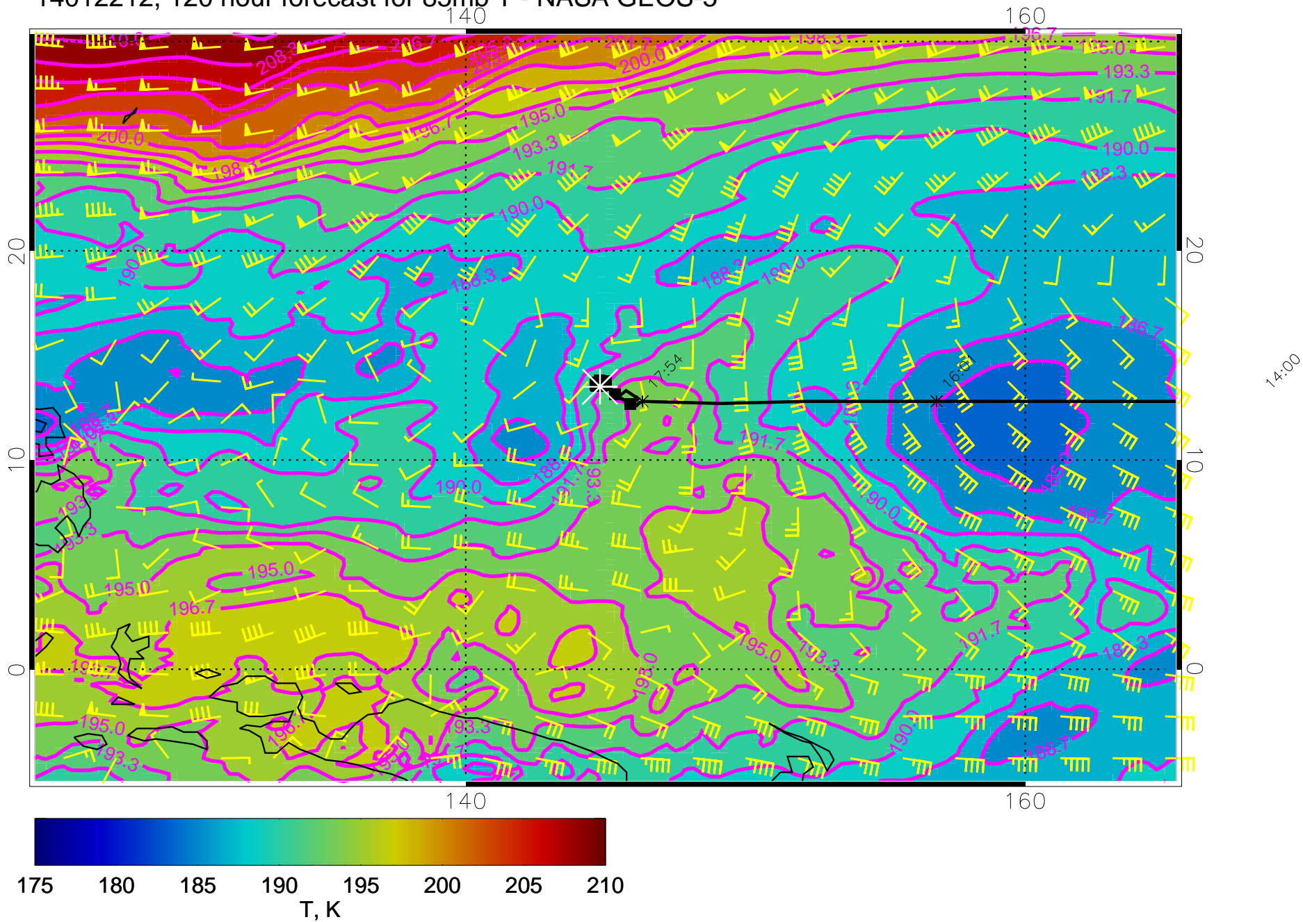
14012212, 120 hour forecast for 85mb T - NASA GEOS-5
