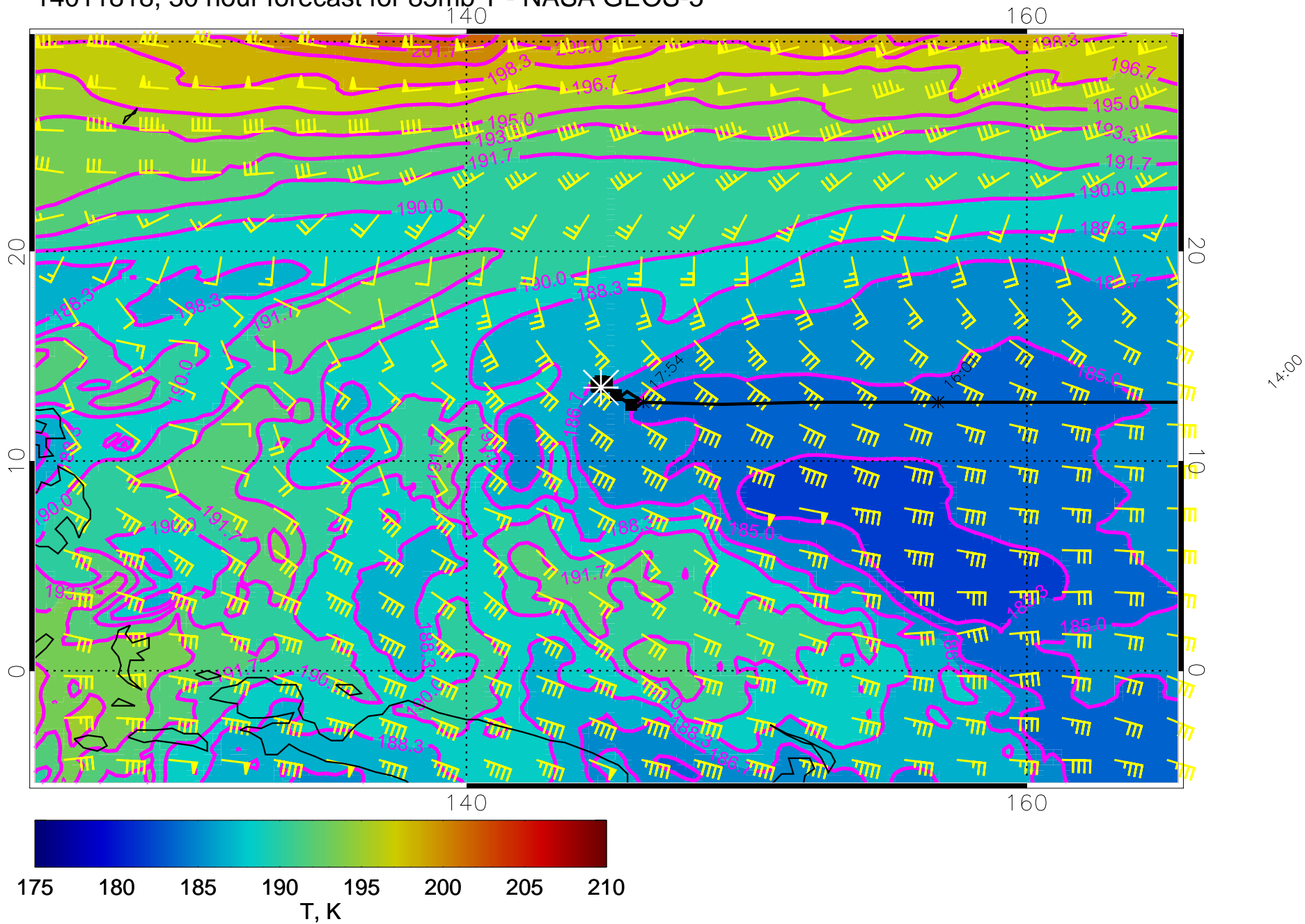
14011818, 30 hour forecast for 85mb T - NASA GEOS-5
