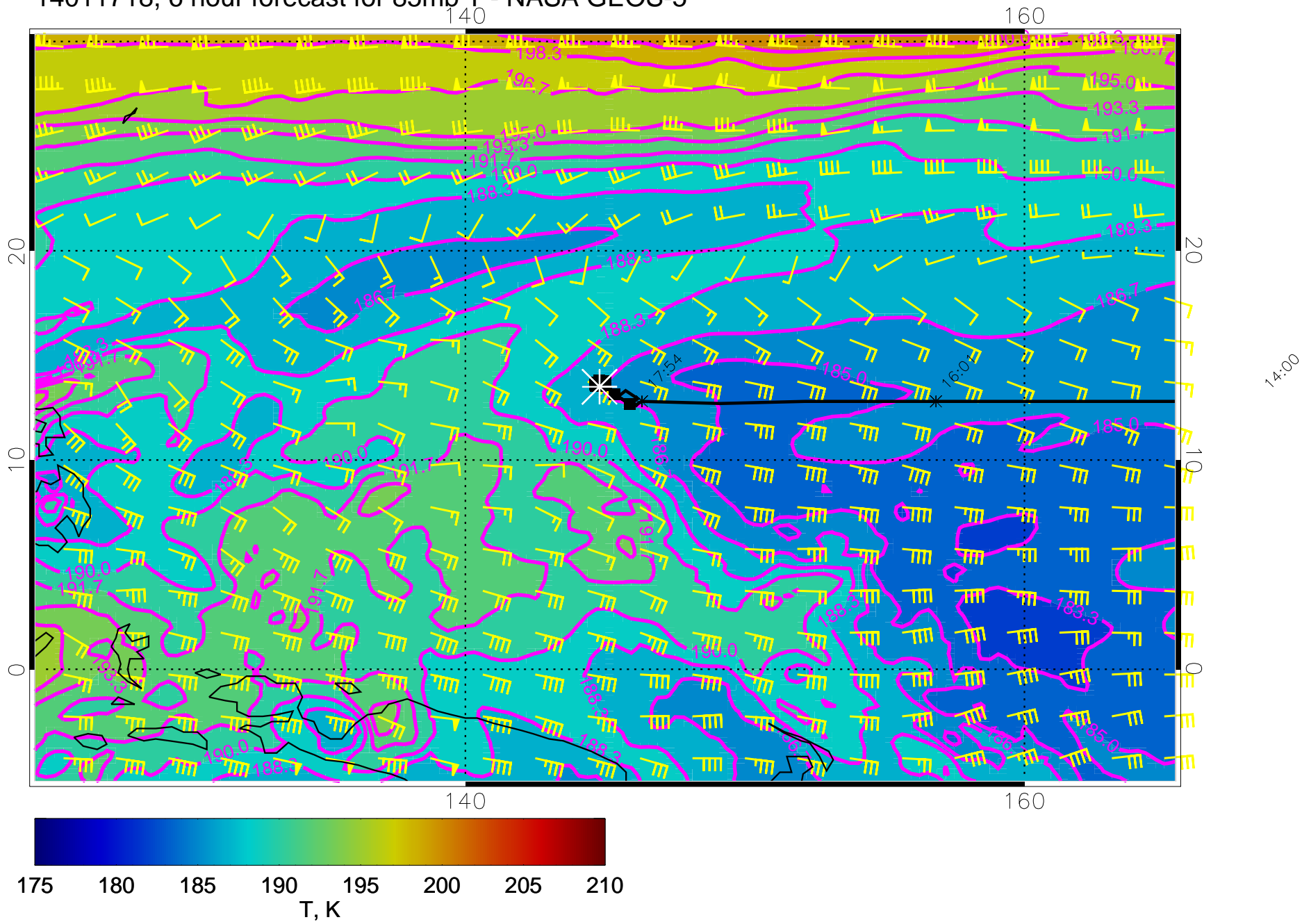
14011718, 6 hour forecast for 85mb T - NASA GEOS-5
