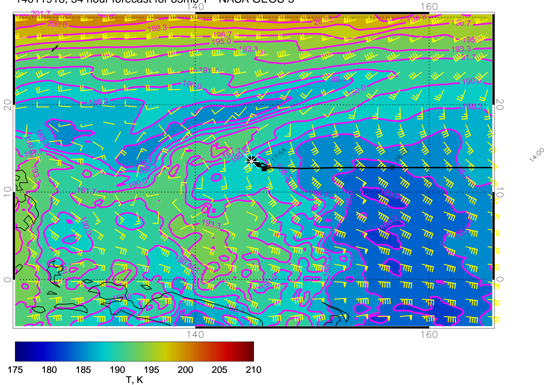
14011918, 54 hour forecast for 85mb T - NASA GEOS-5
