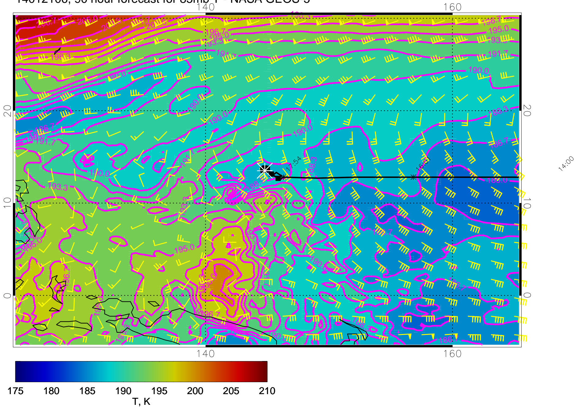
14012106, 90 hour forecast for 85mb T - NASA GEOS-5
