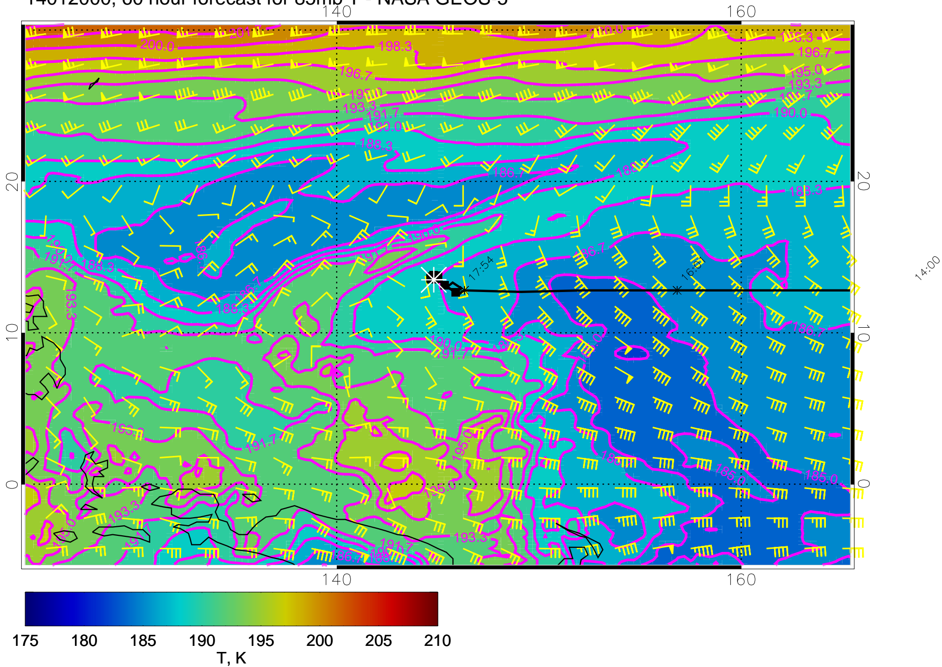
14012000, 60 hour forecast for 85mb T - NASA GEOS-5
