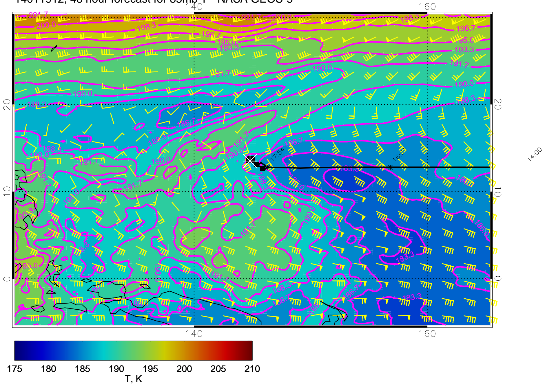
14011912, 48 hour forecast for 85mb T - NASA GEOS-5
