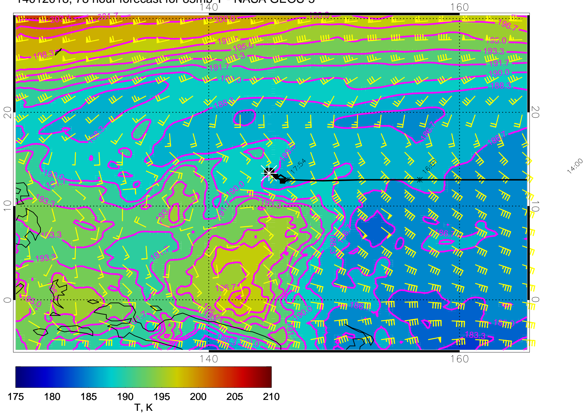
14012018, 78 hour forecast for 85mb T - NASA GEOS-5
