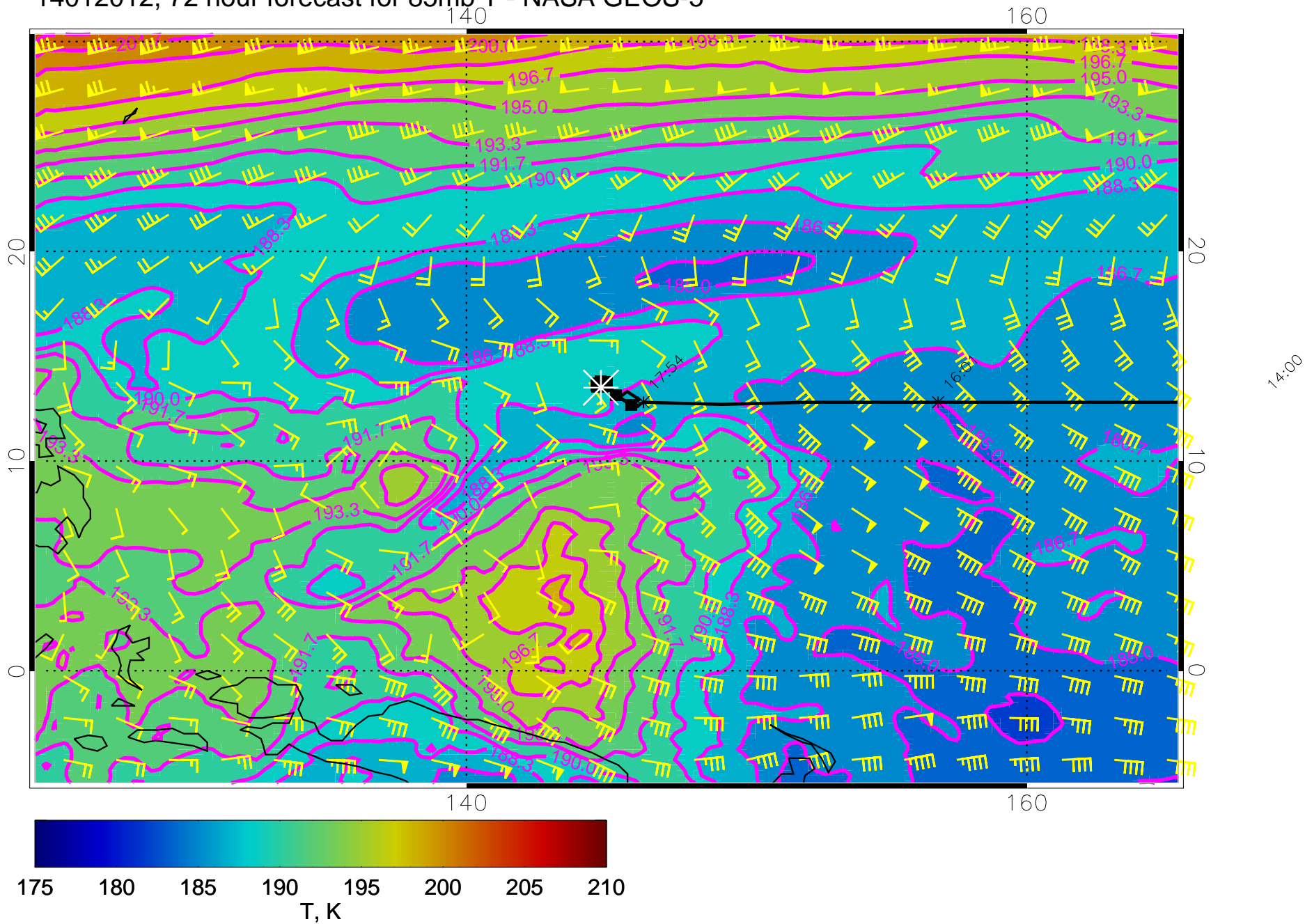
14012012, 72 hour forecast for 85mb T - NASA GEOS-5
