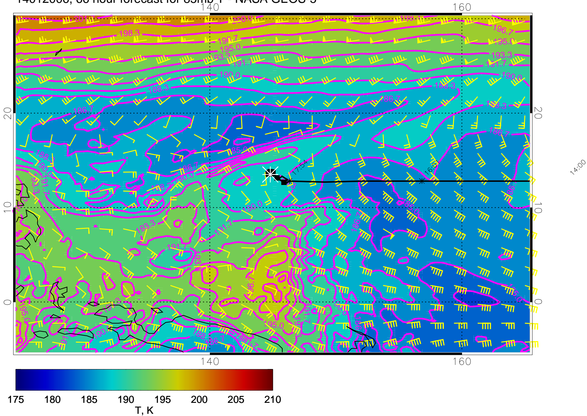
14012006, 66 hour forecast for 85mb T - NASA GEOS-5
