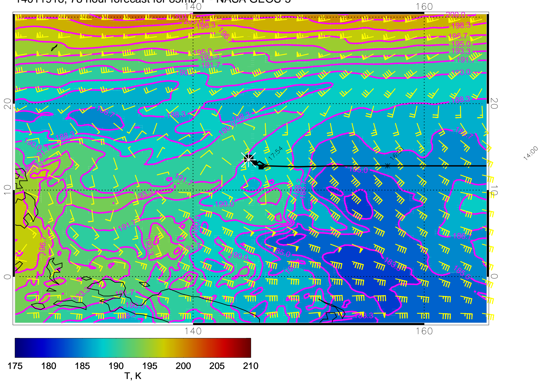
14011918, 78 hour forecast for 85mb T - NASA GEOS-5
