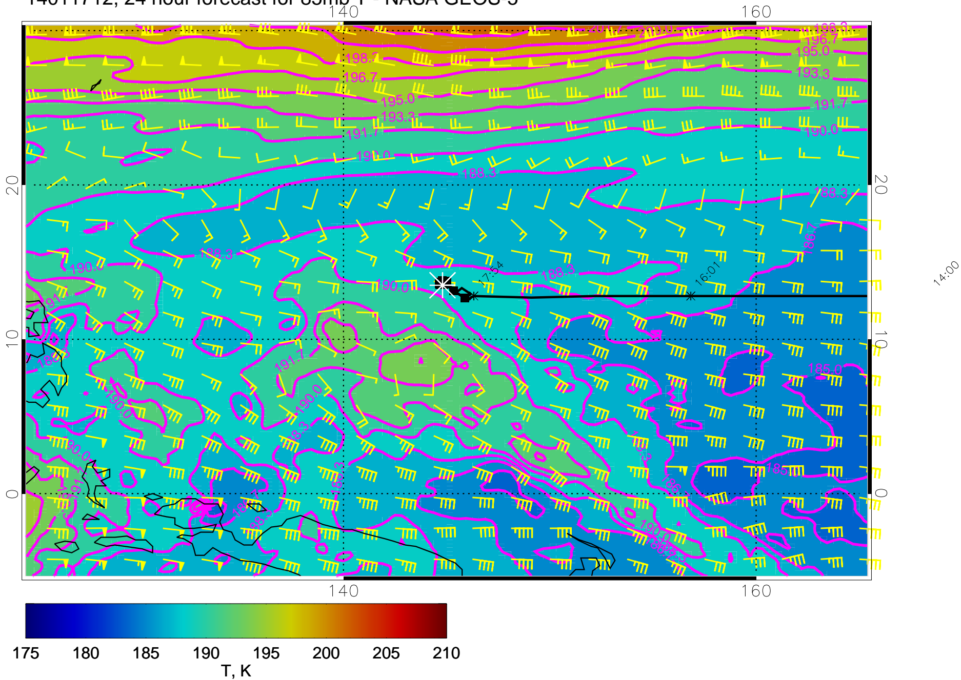
14011712, 24 hour forecast for 85mb T - NASA GEOS-5
