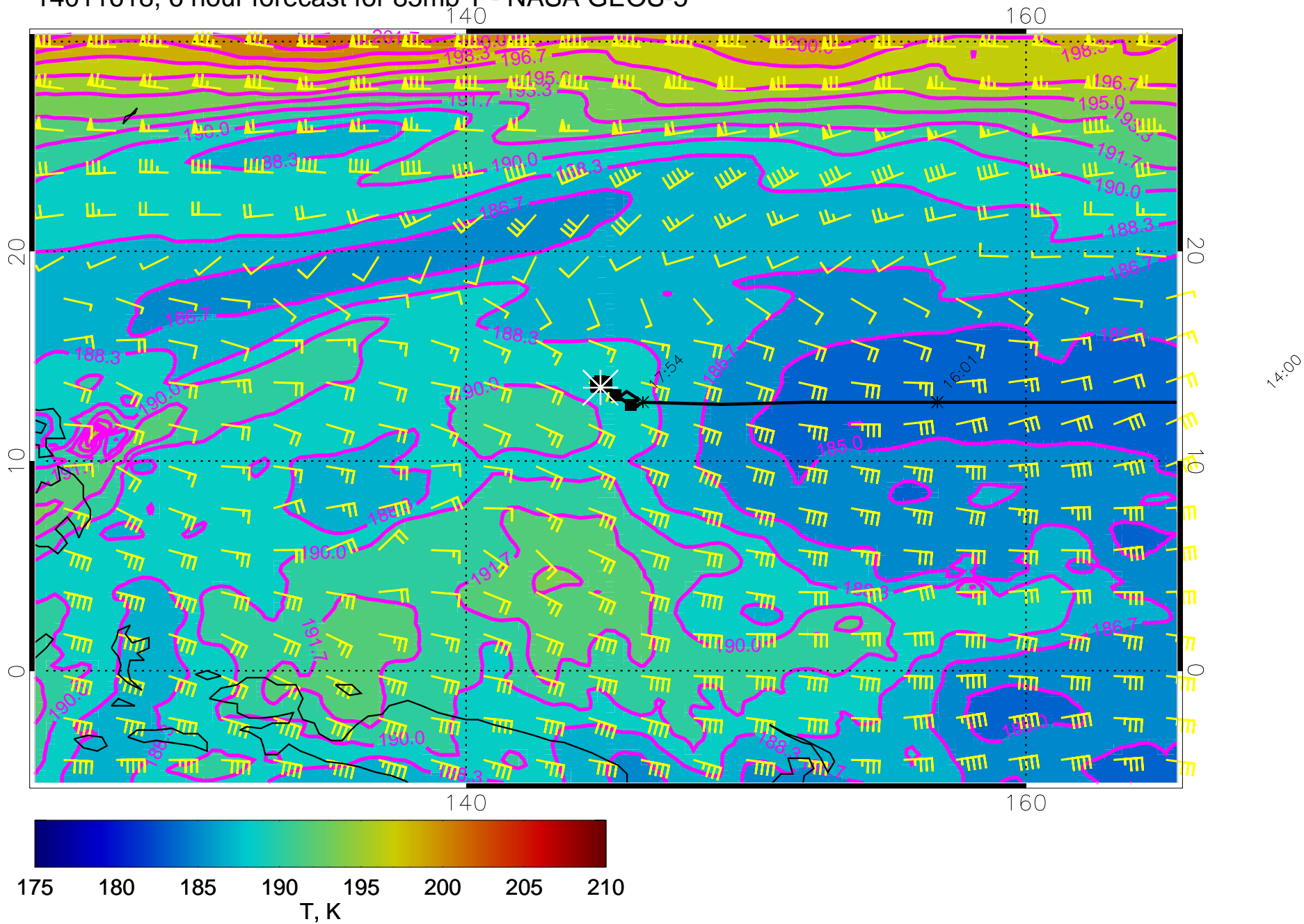
14011618, 6 hour forecast for 85mb T - NASA GEOS-5
