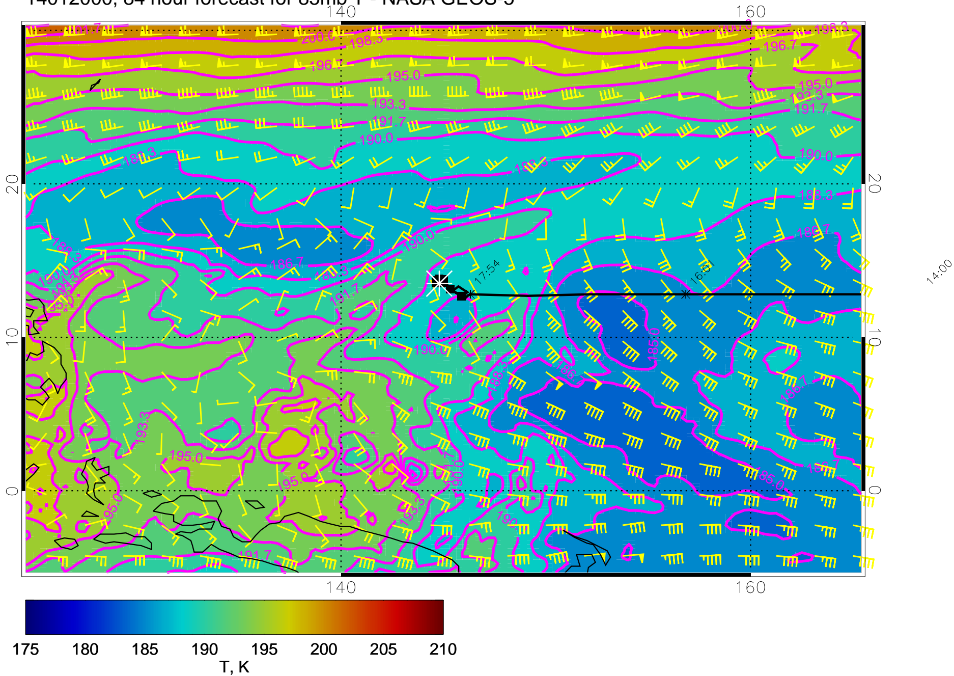
14012000, 84 hour forecast for 85mb T - NASA GEOS-5
