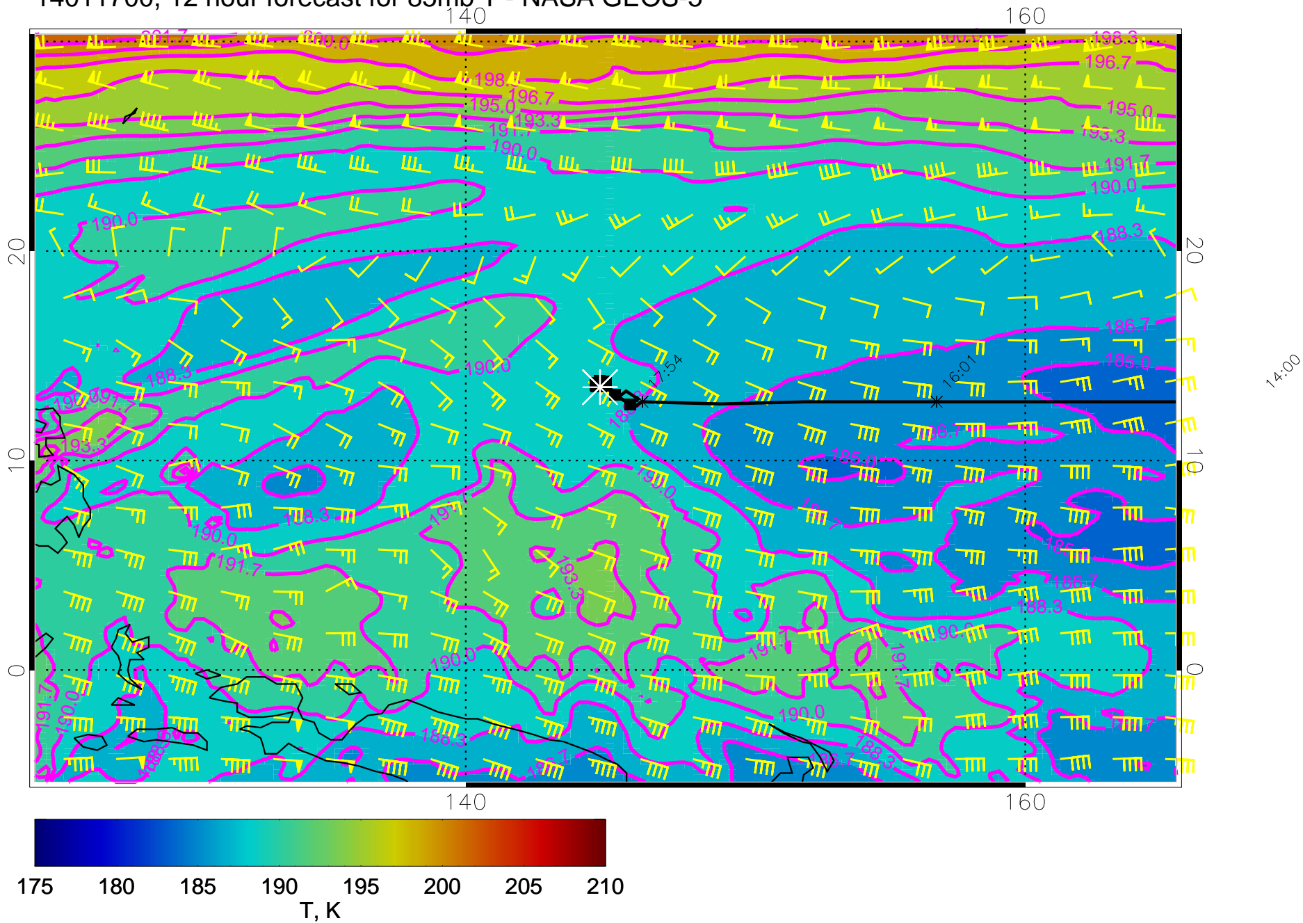
14011700, 12 hour forecast for 85mb T - NASA GEOS-5
