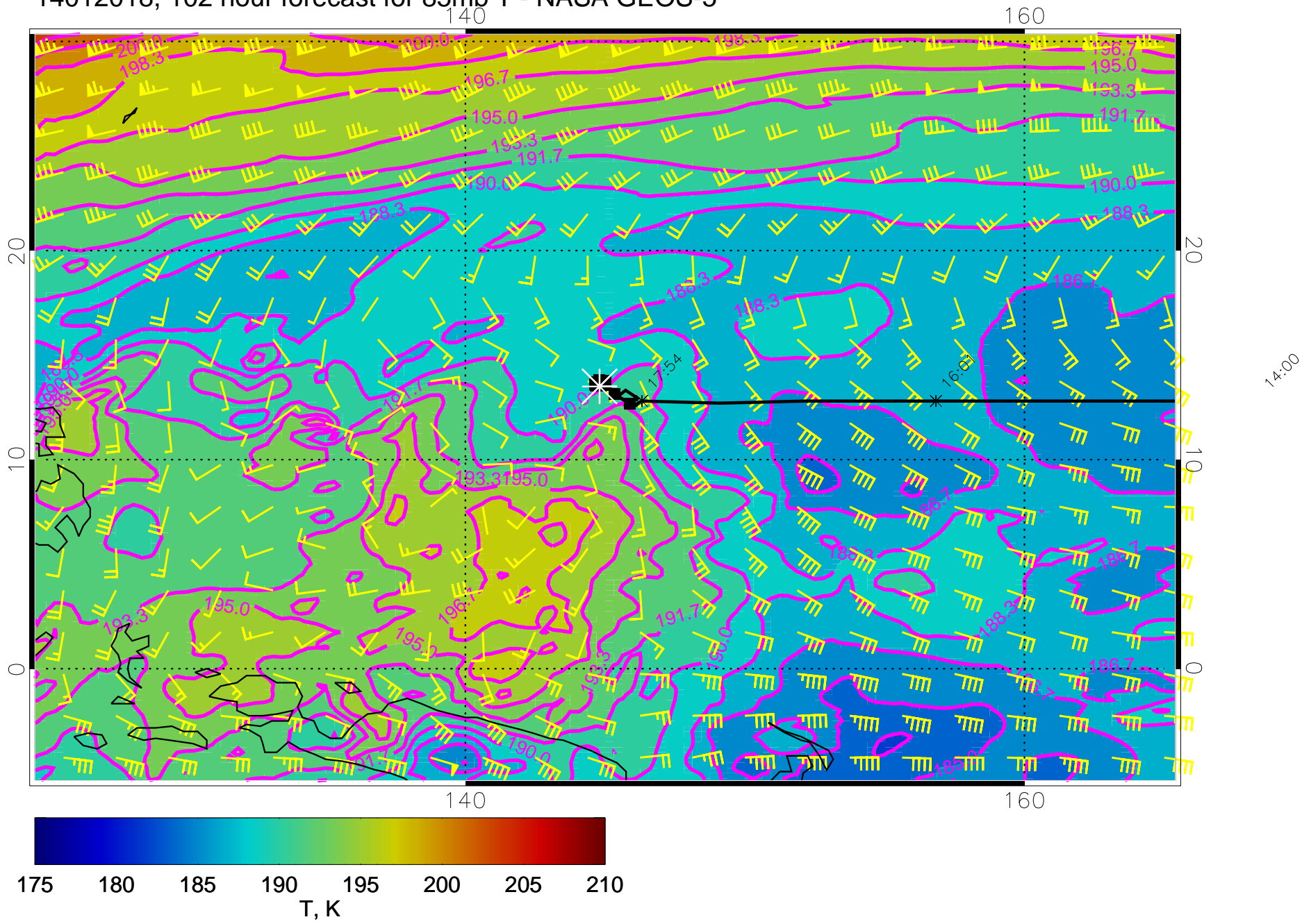
14012018, 102 hour forecast for 85mb T - NASA GEOS-5
