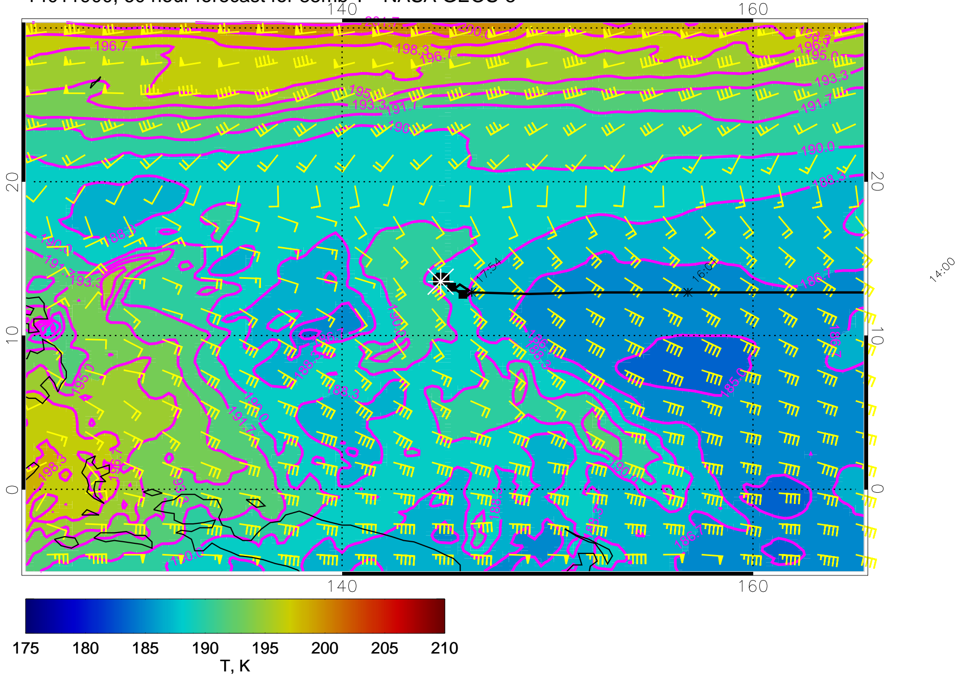
14011900, 60 hour forecast for 85mb T - NASA GEOS-5
