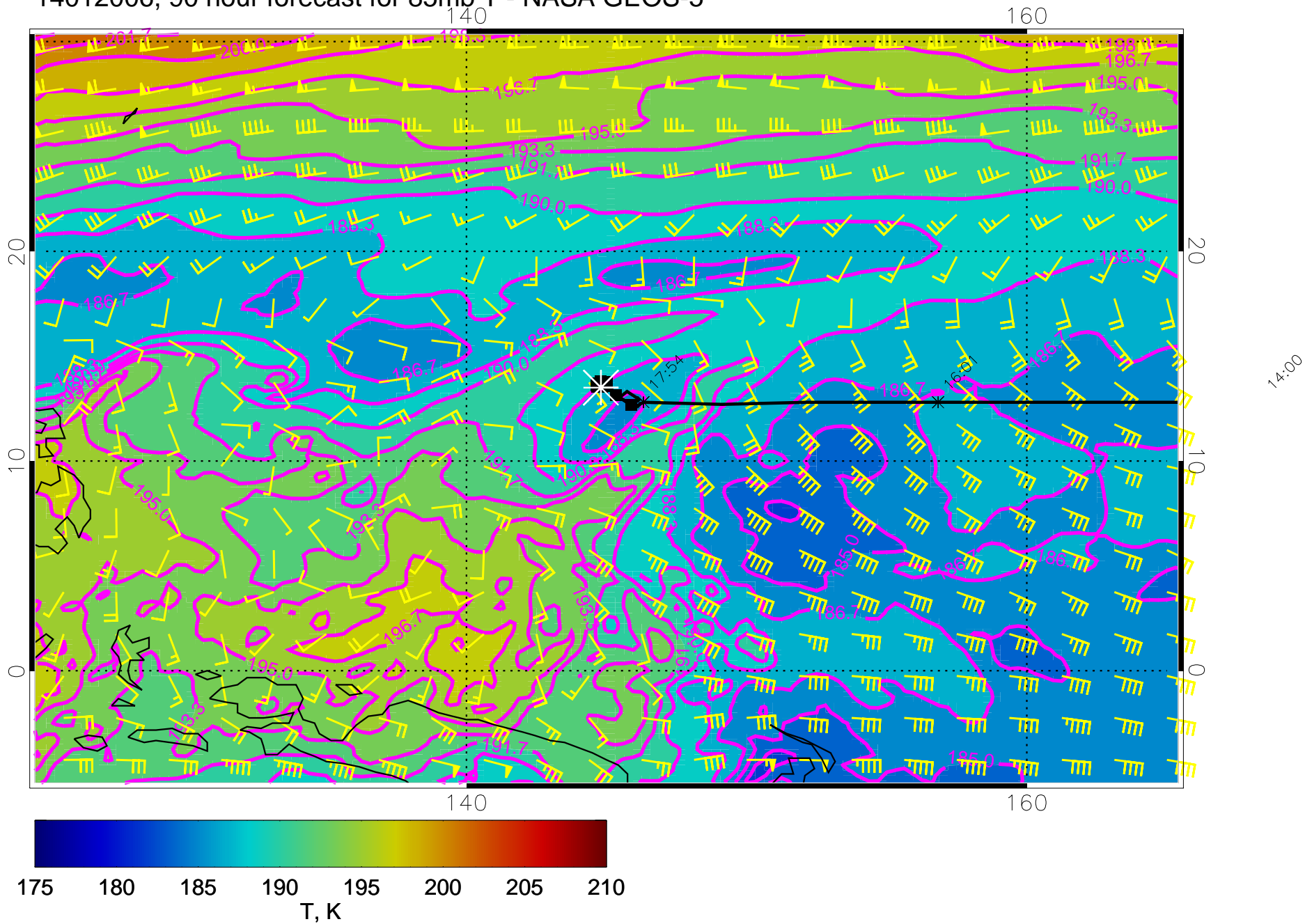
14012006, 90 hour forecast for 85mb T - NASA GEOS-5
