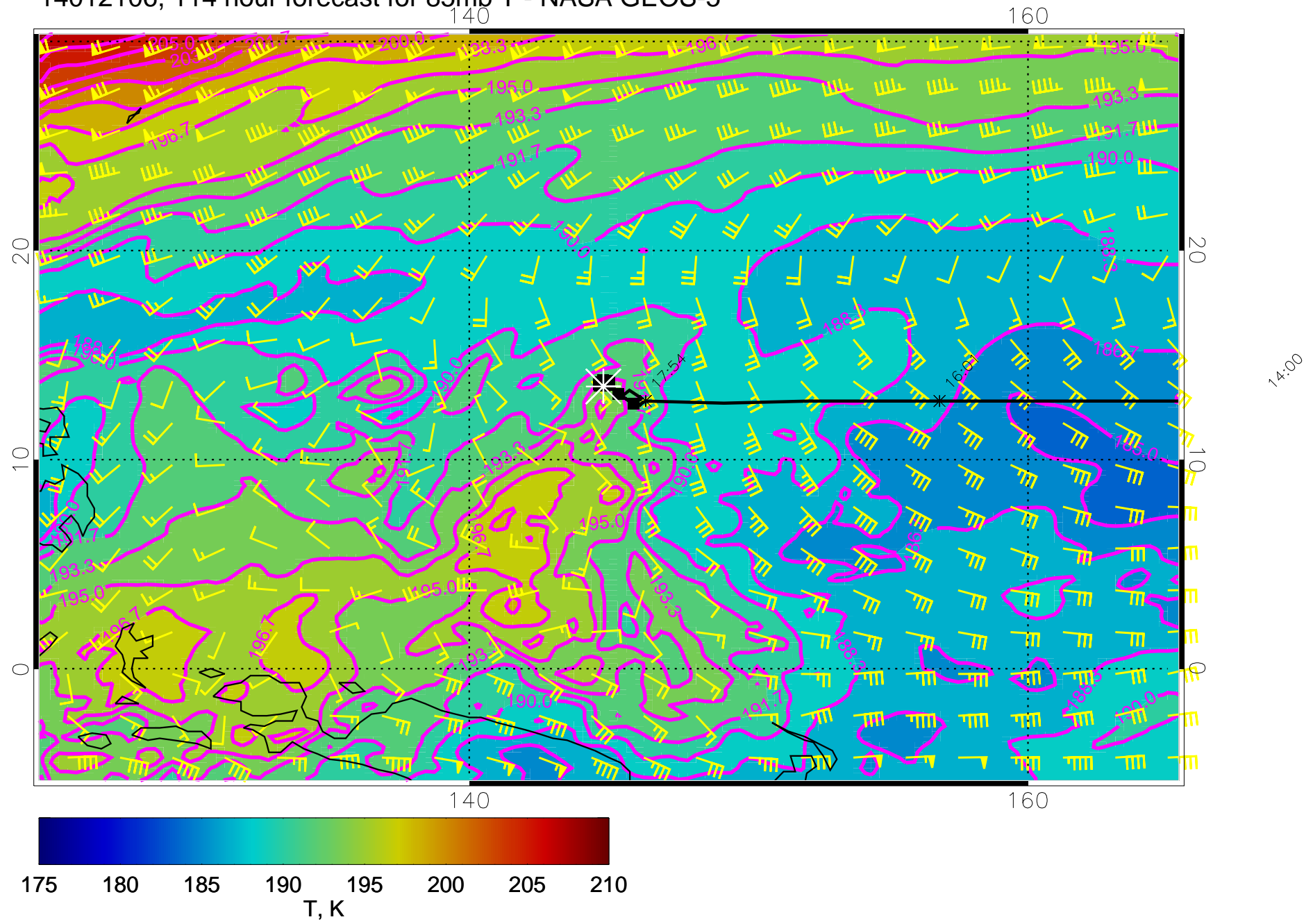
14012106, 114 hour forecast for 85mb T - NASA GEOS-5
