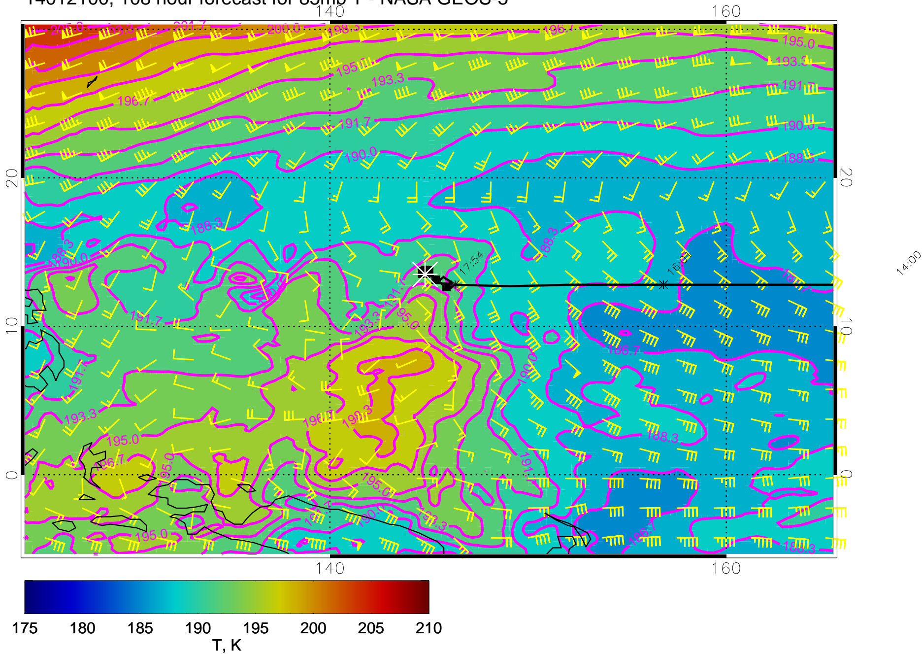
14012100, 108 hour forecast for 85mb T - NASA GEOS-5
