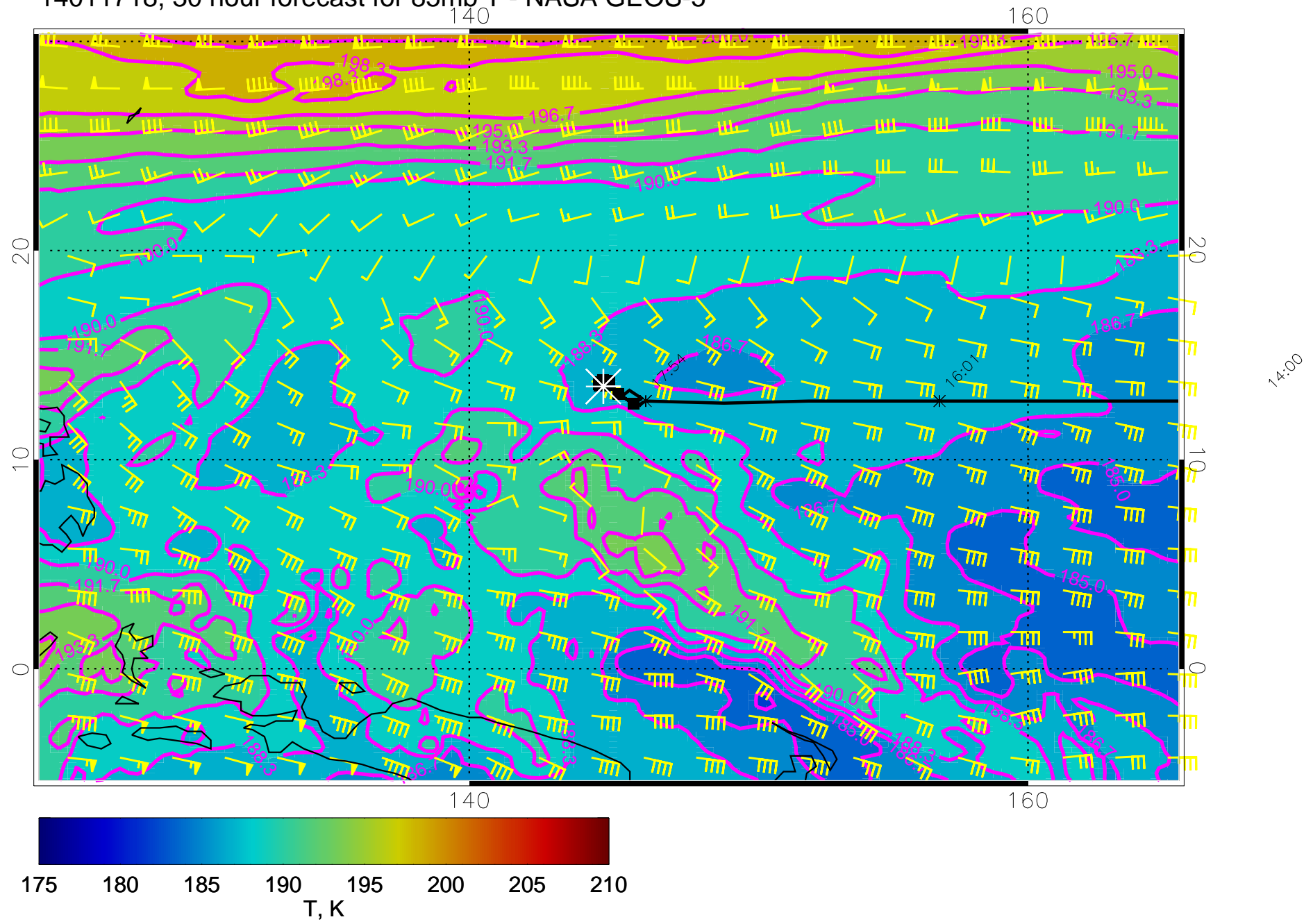
14011718, 30 hour forecast for 85mb T - NASA GEOS-5
