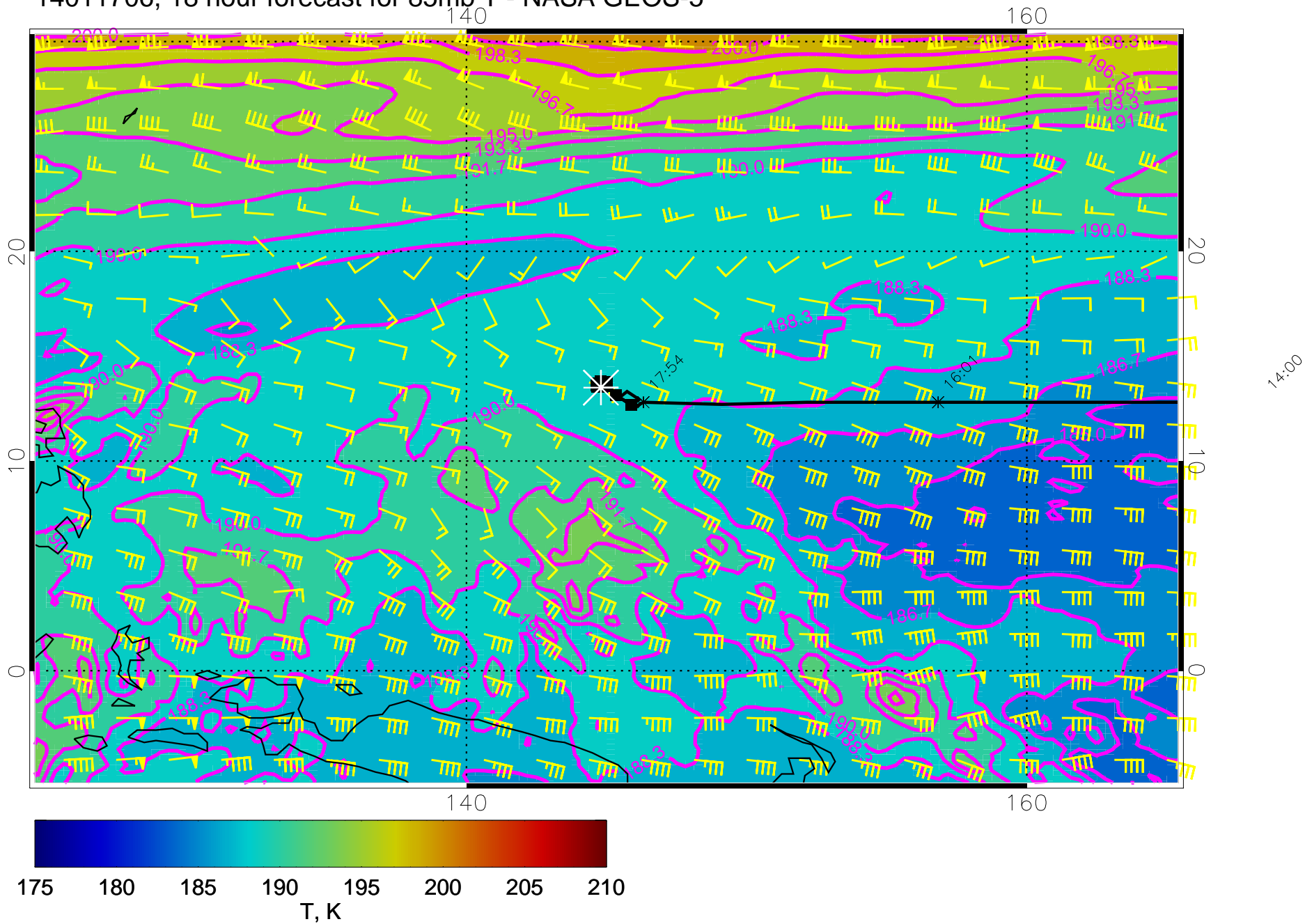
14011706, 18 hour forecast for 85mb T - NASA GEOS-5
