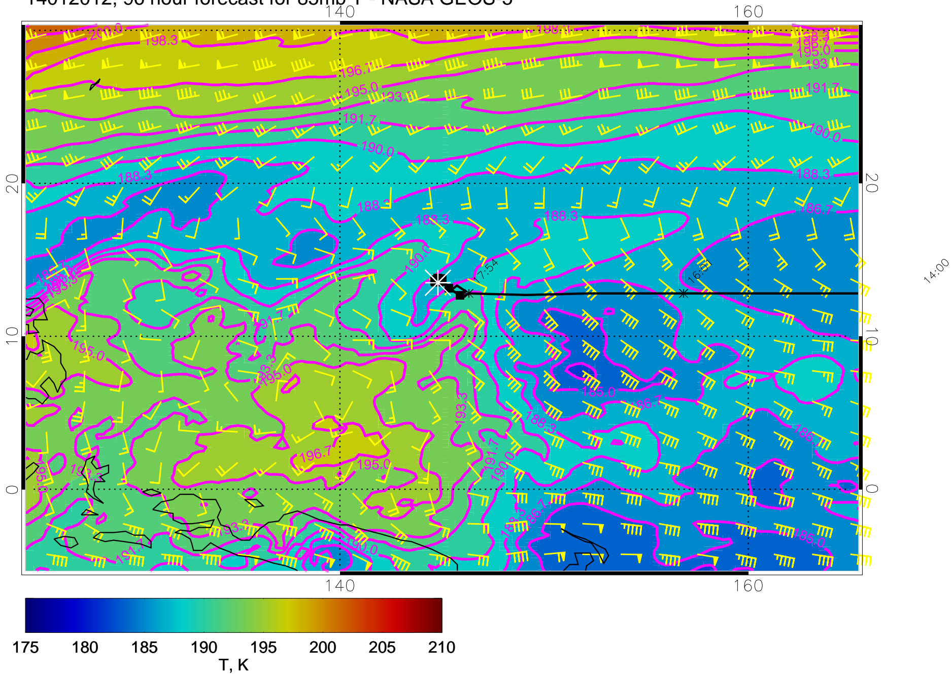
14012012, 96 hour forecast for 85mb T - NASA GEOS-5
