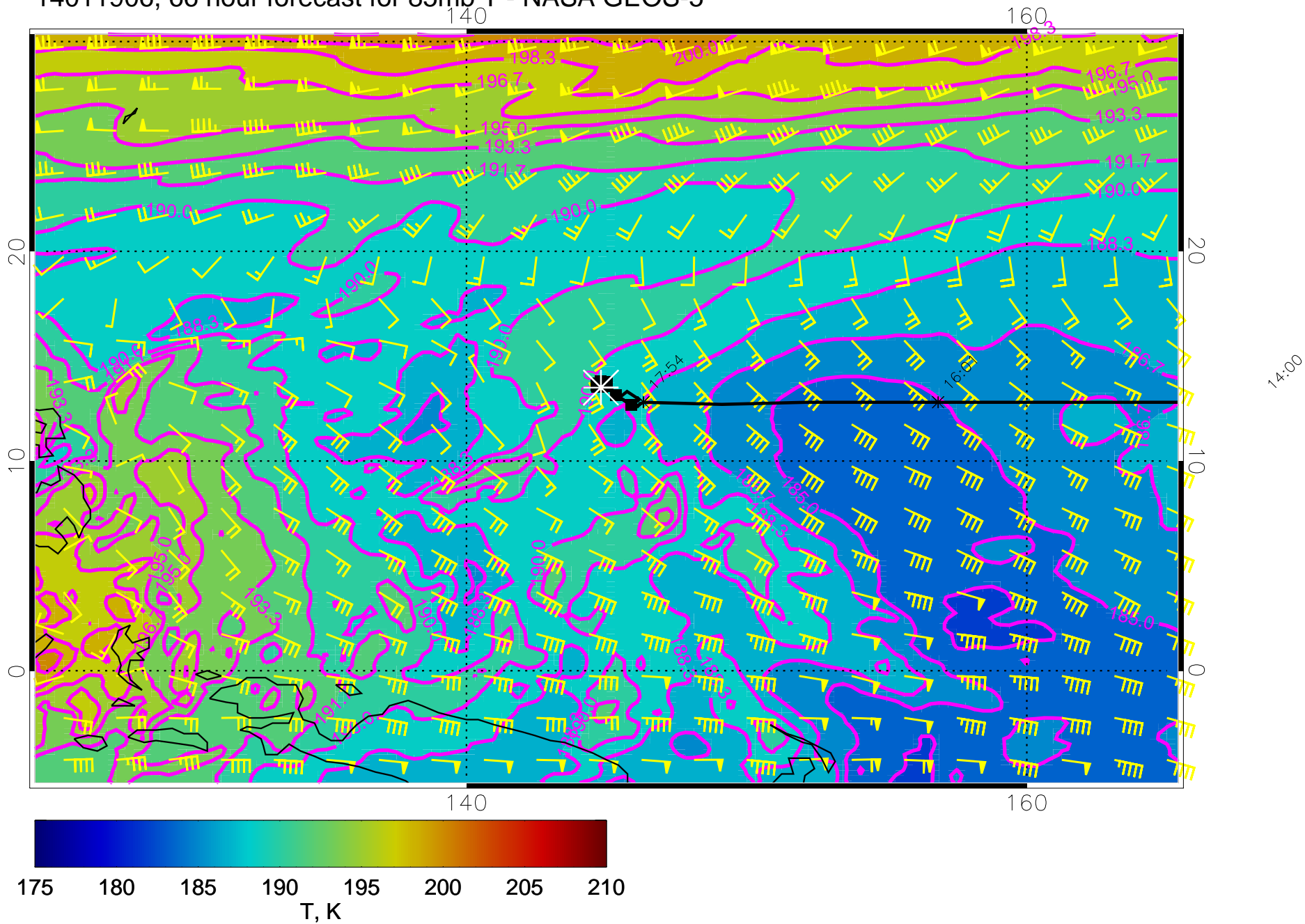
14011906, 66 hour forecast for 85mb T - NASA GEOS-5
