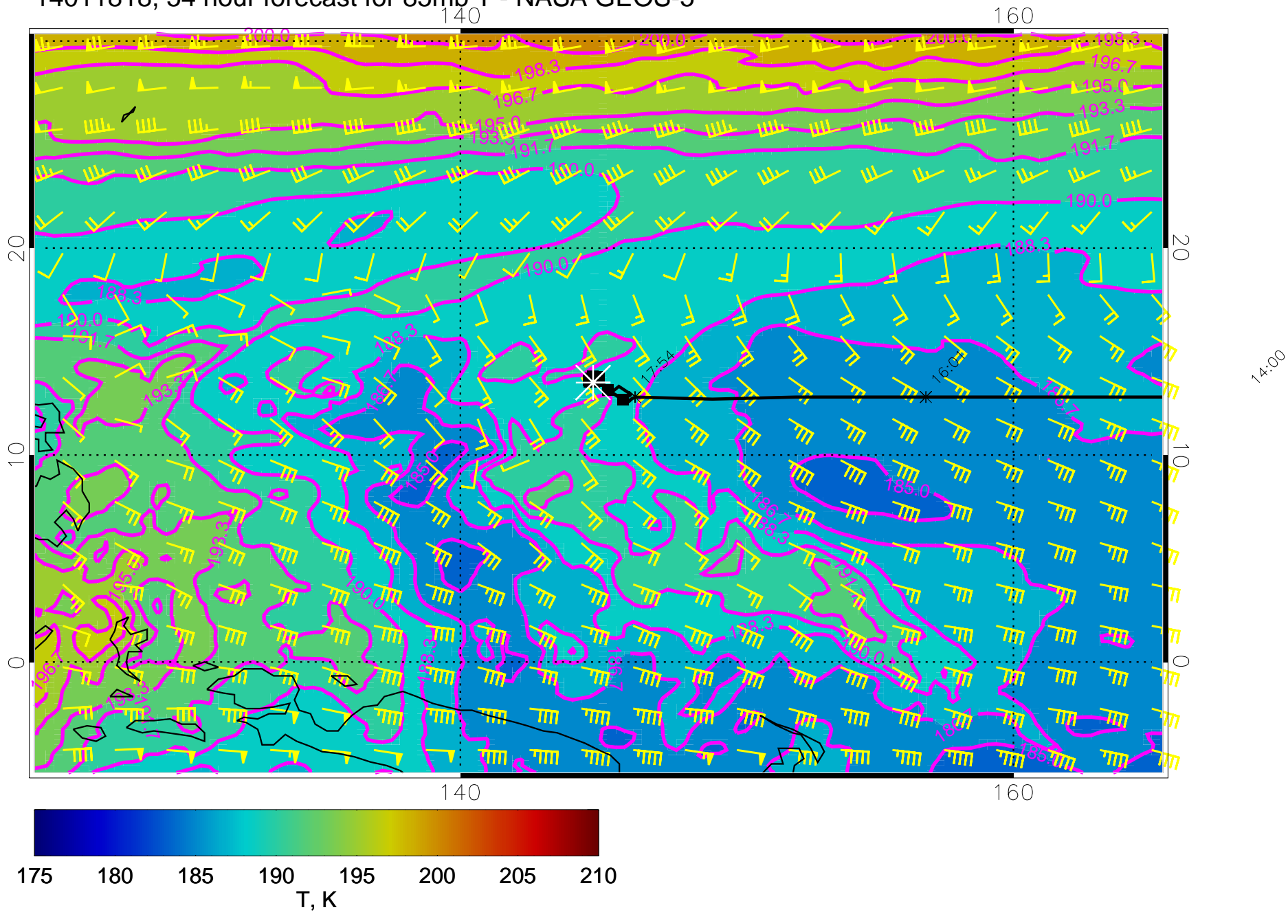
14011818, 54 hour forecast for 85mb T - NASA GEOS-5
