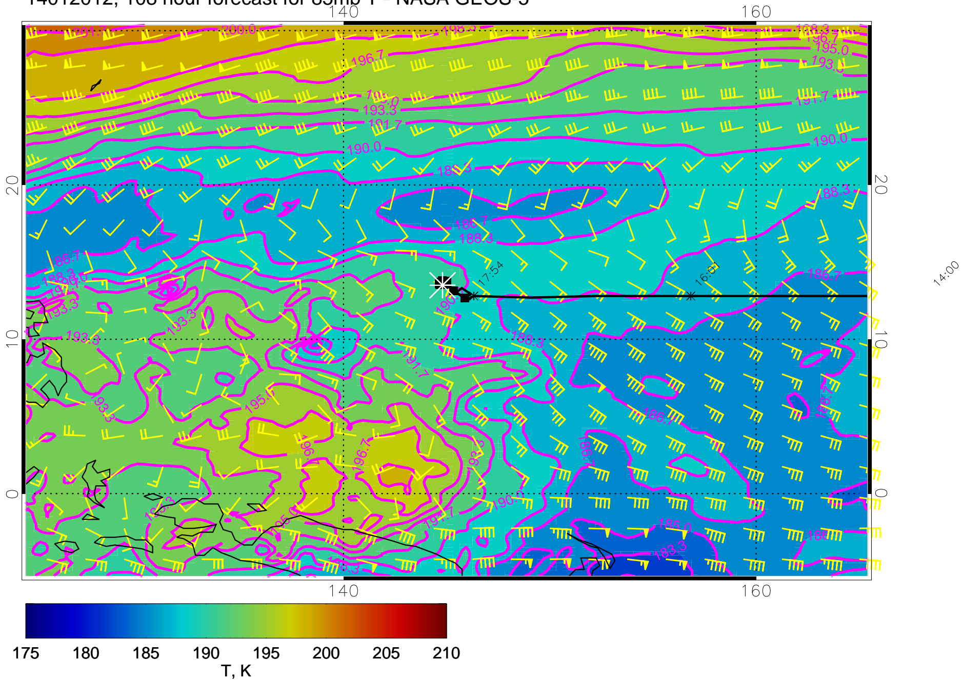
14012012, 108 hour forecast for 85mb T - NASA GEOS-5
