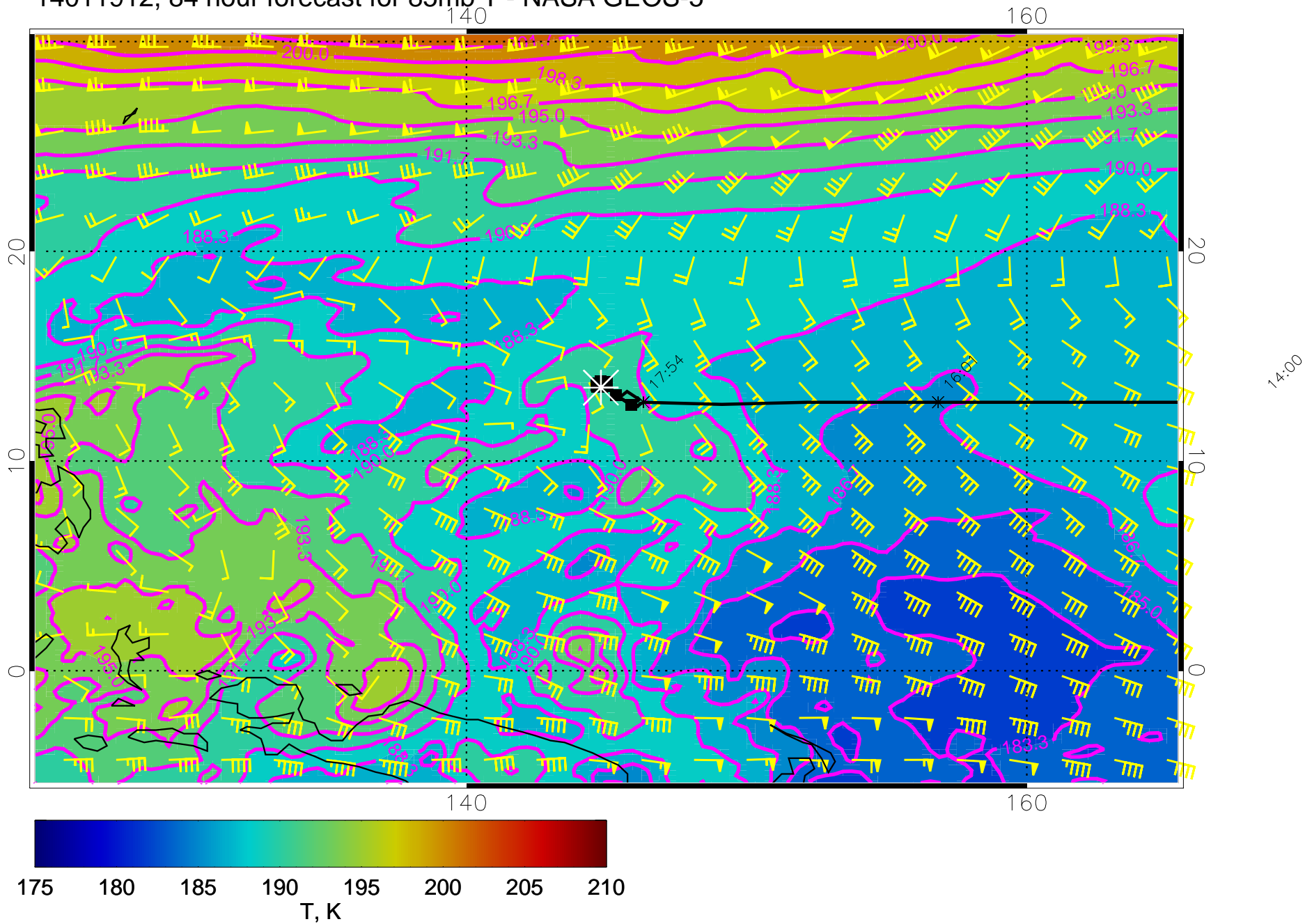
14011912, 84 hour forecast for 85mb T - NASA GEOS-5
