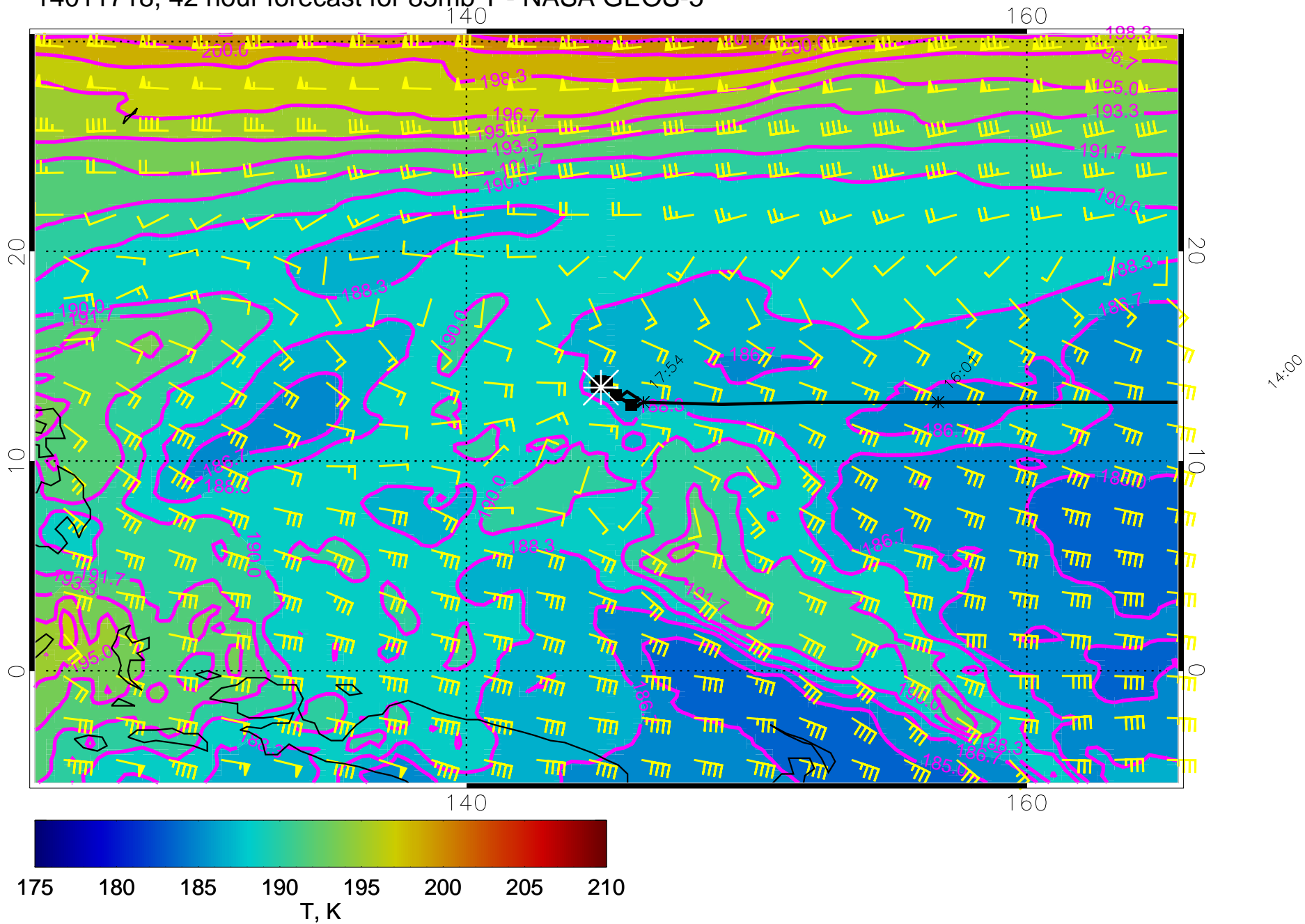
14011718, 42 hour forecast for 85mb T - NASA GEOS-5
