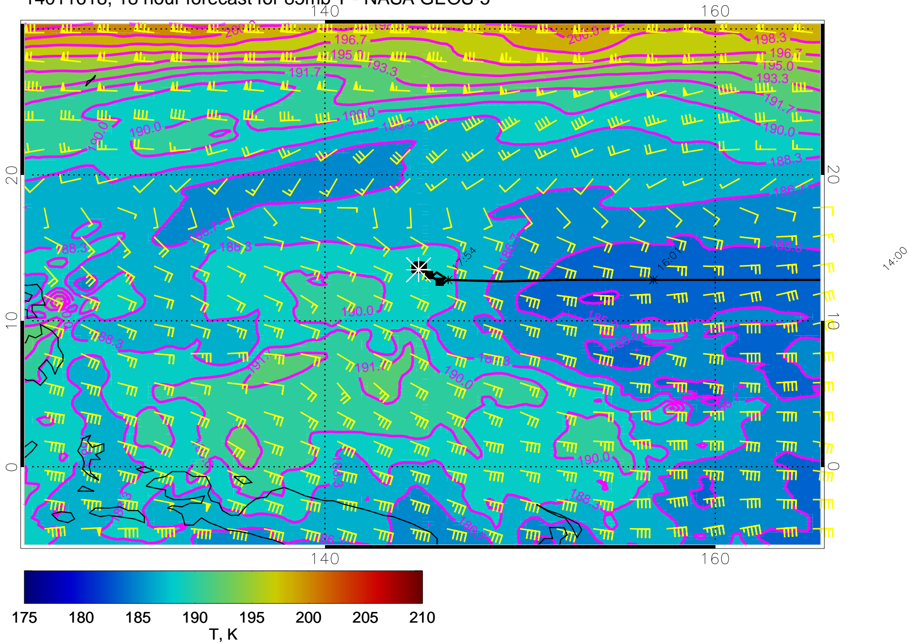
14011618, 18 hour forecast for 85mb T - NASA GEOS-5
