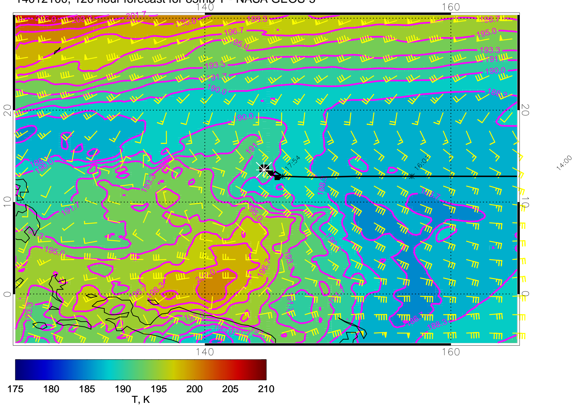
14012100, 120 hour forecast for 85mb T - NASA GEOS-5
