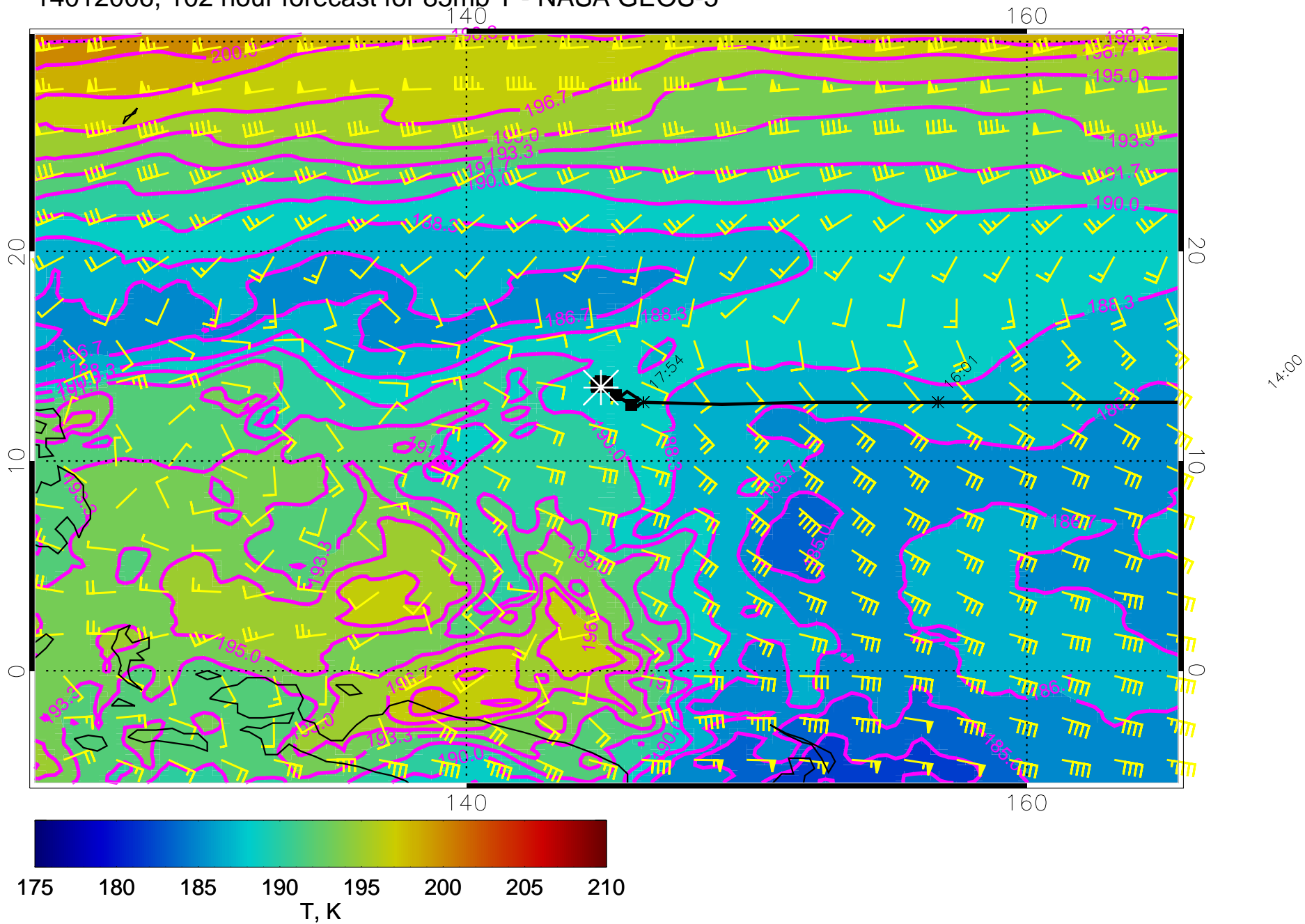
14012006, 102 hour forecast for 85mb T - NASA GEOS-5
