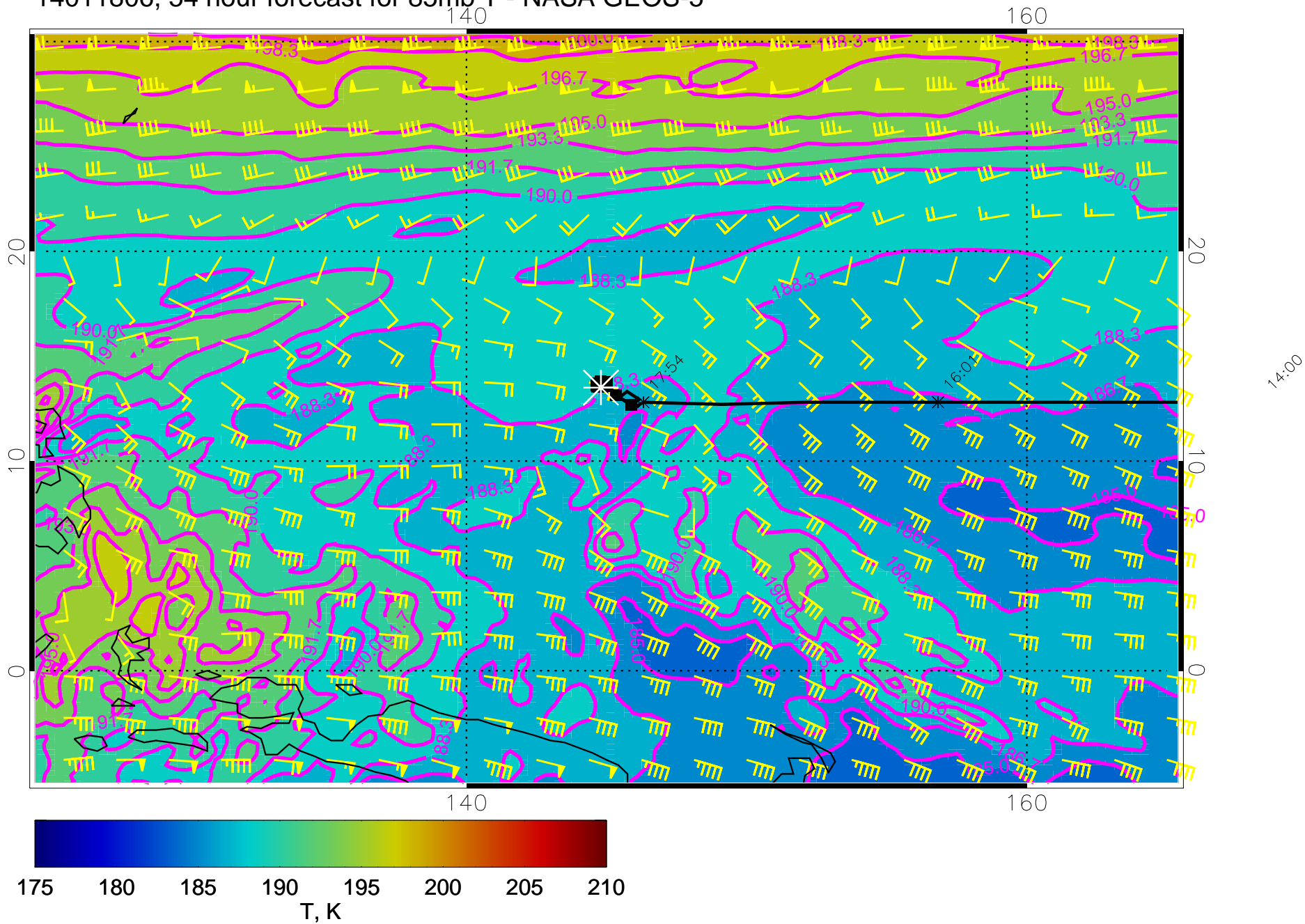
14011806, 54 hour forecast for 85mb T - NASA GEOS-5
