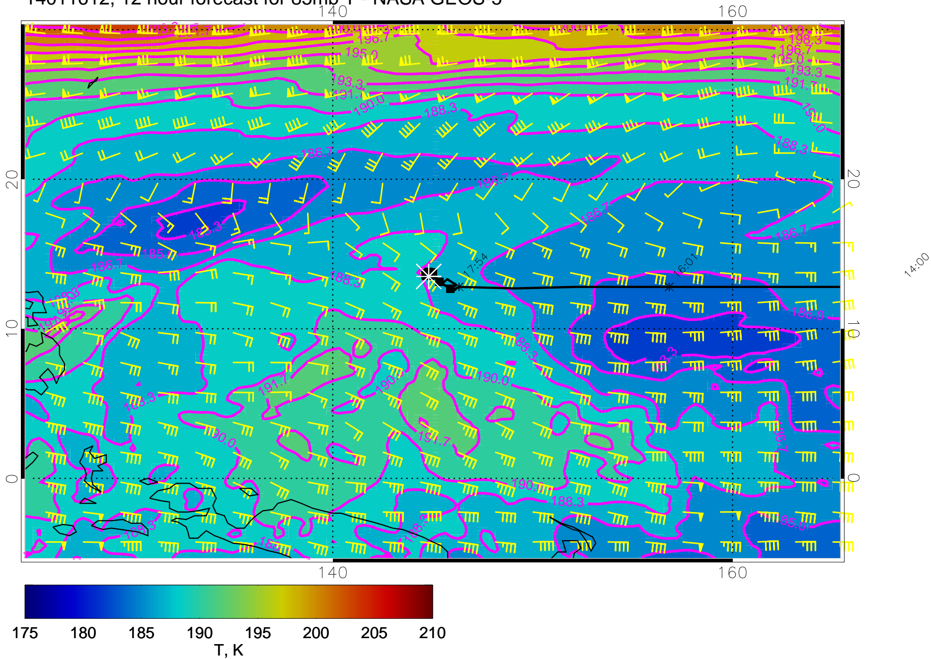
14011612, 12 hour forecast for 85mb T - NASA GEOS-5
