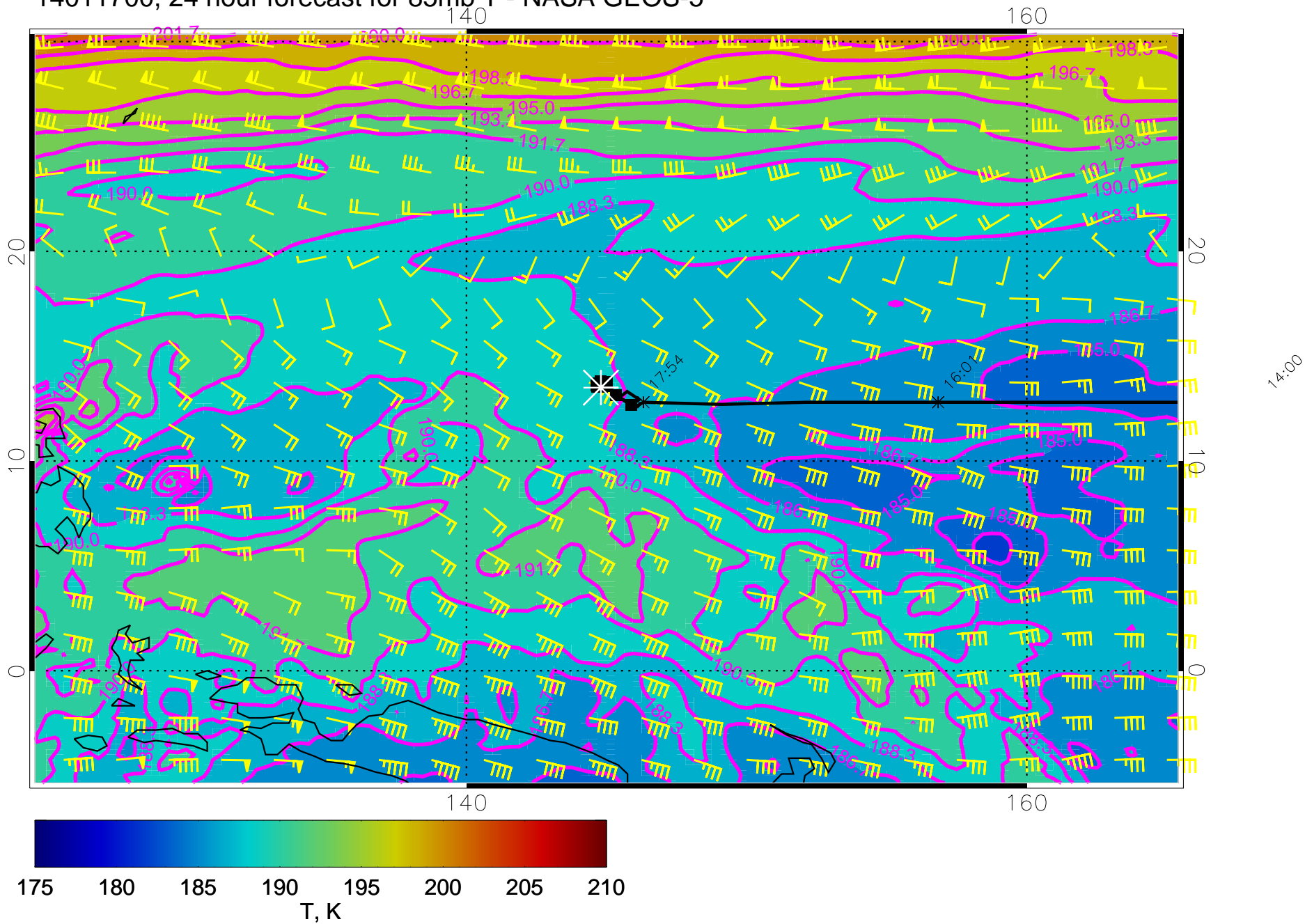
14011700, 24 hour forecast for 85mb T - NASA GEOS-5
