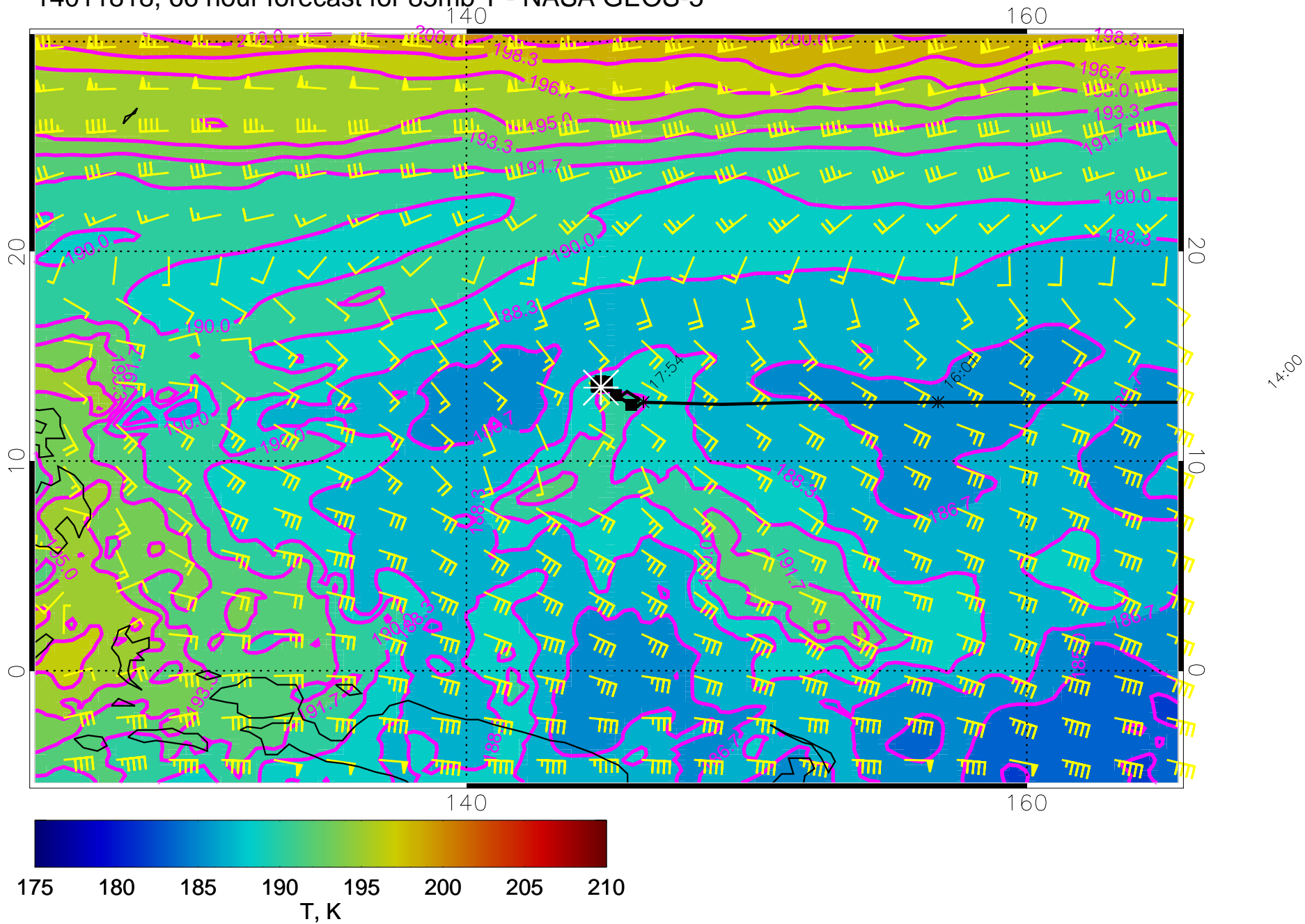
14011818, 66 hour forecast for 85mb T - NASA GEOS-5
