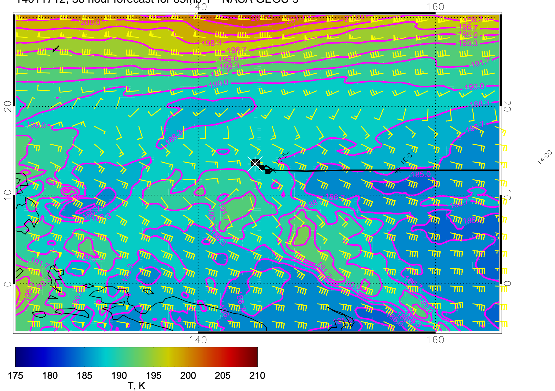
14011712, 36 hour forecast for 85mb T - NASA GEOS-5
