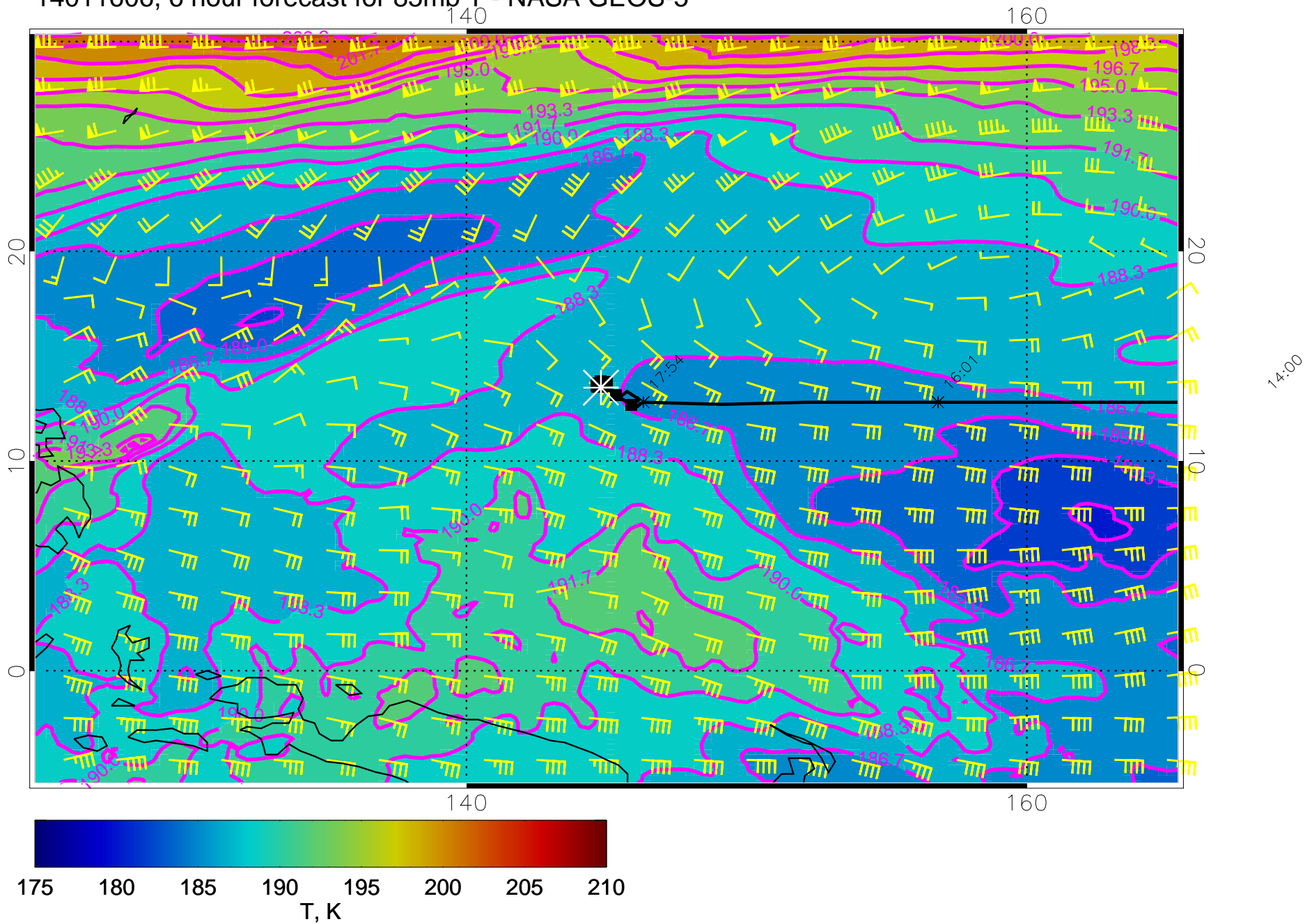
14011606, 6 hour forecast for 85mb T - NASA GEOS-5
