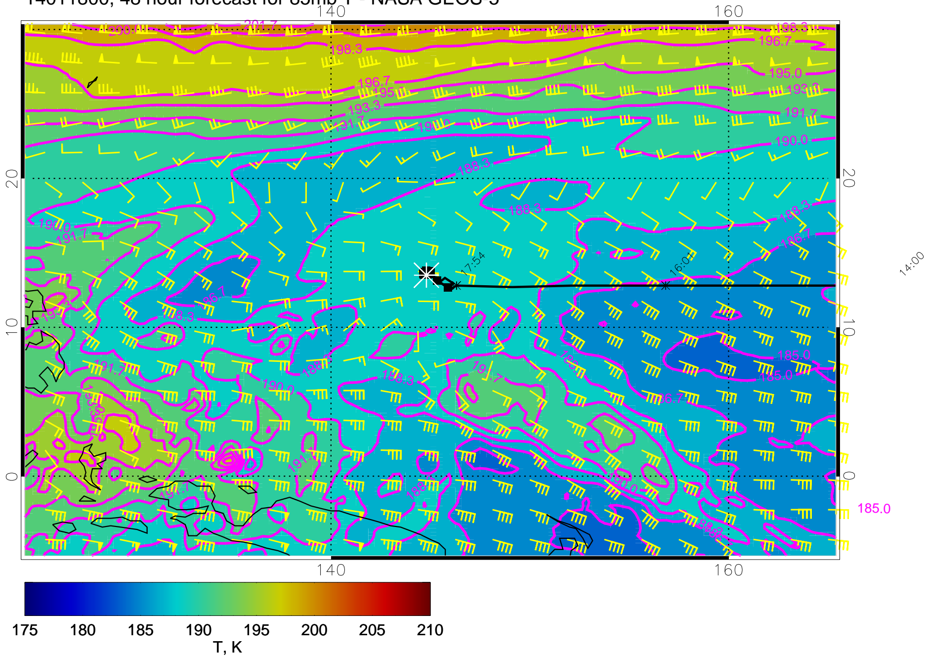
14011800, 48 hour forecast for 85mb T - NASA GEOS-5
