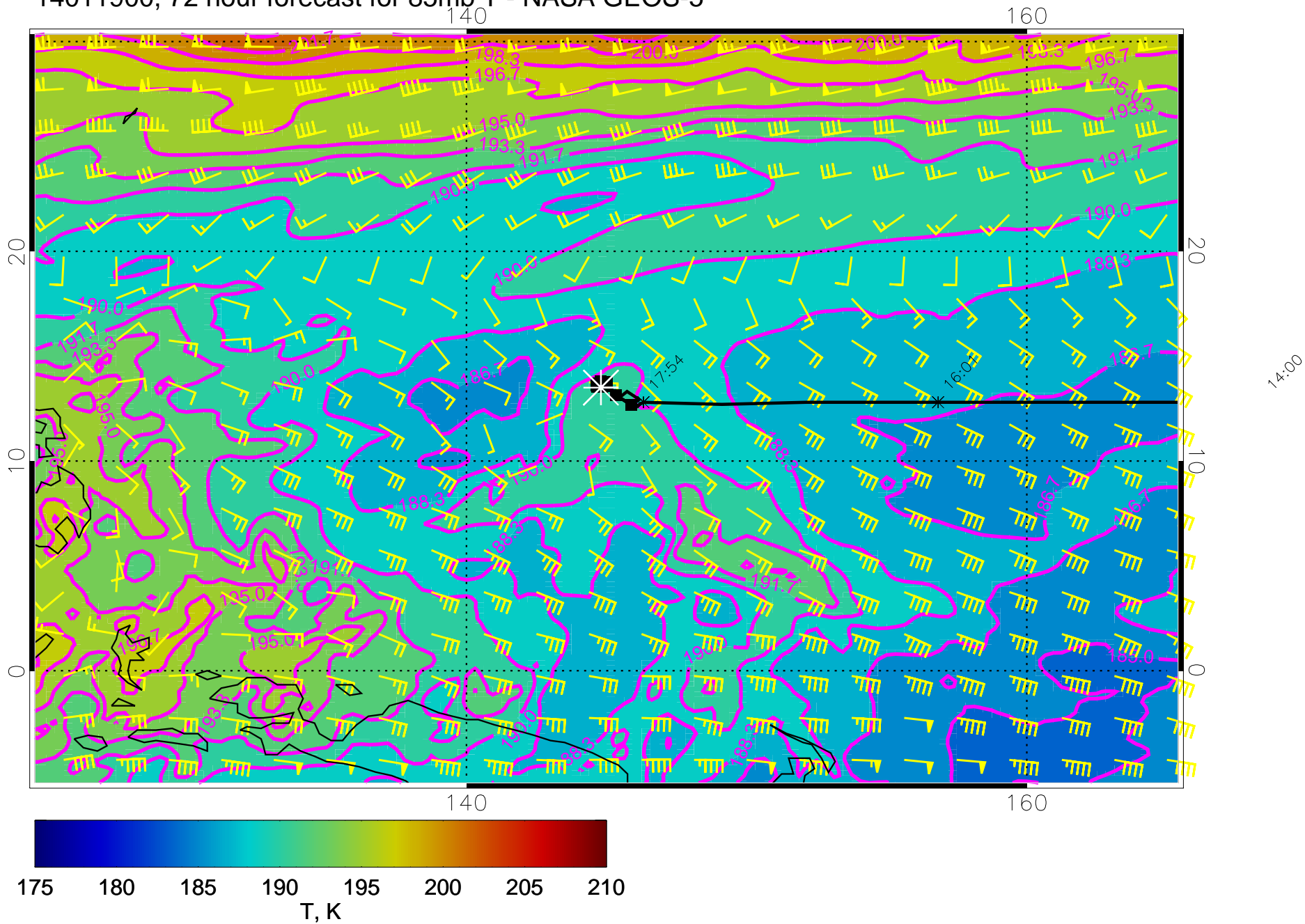
14011900, 72 hour forecast for 85mb T - NASA GEOS-5
