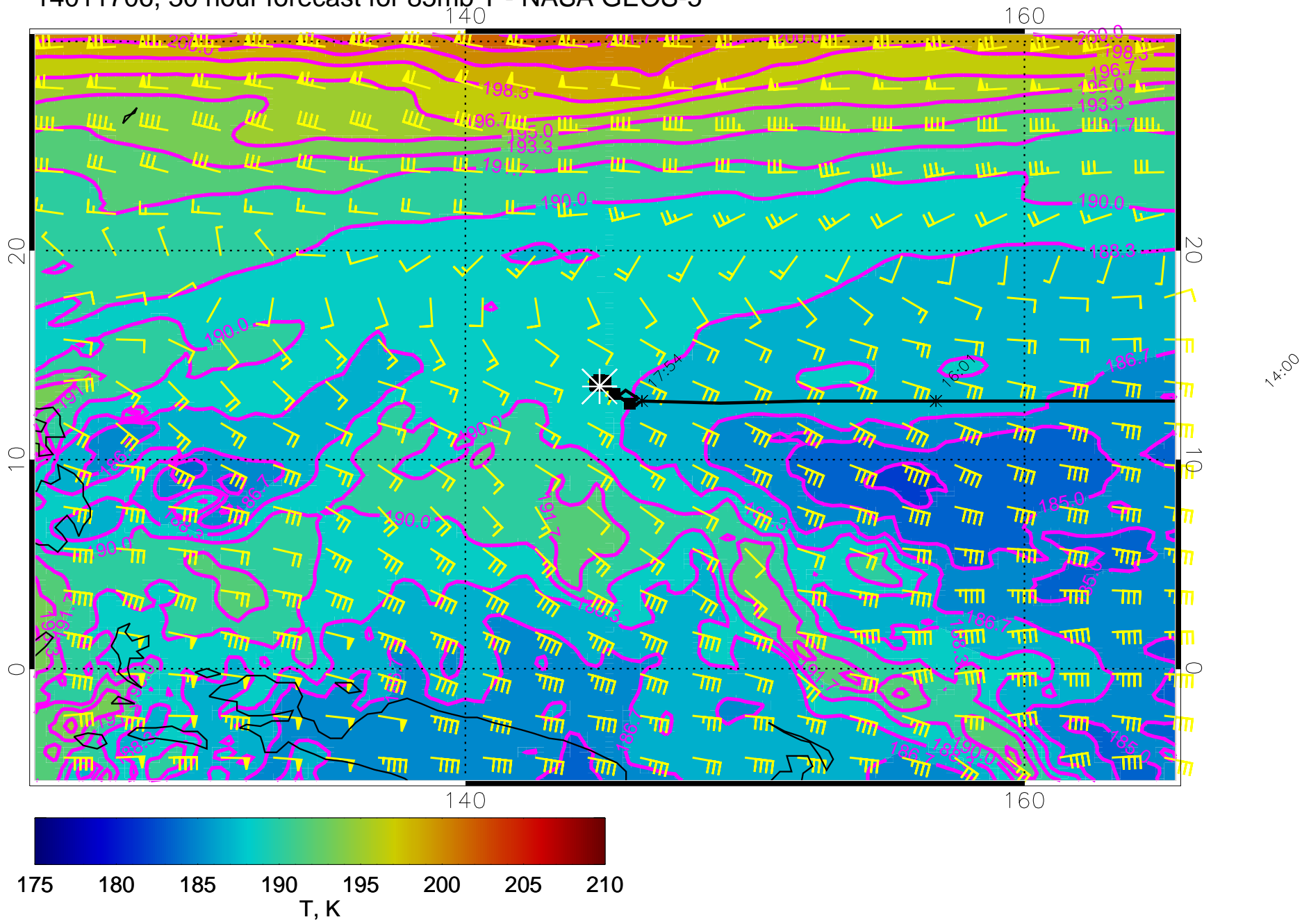
14011706, 30 hour forecast for 85mb T - NASA GEOS-5
