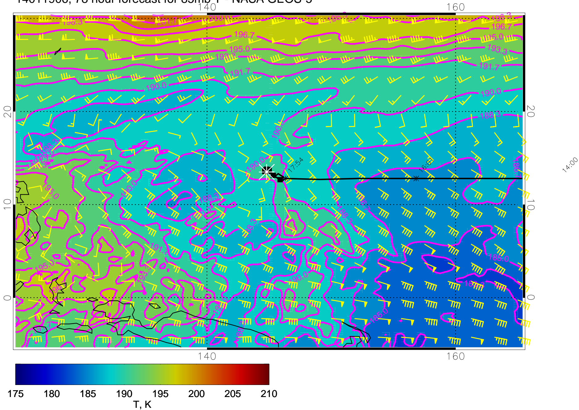
14011906, 78 hour forecast for 85mb T - NASA GEOS-5
