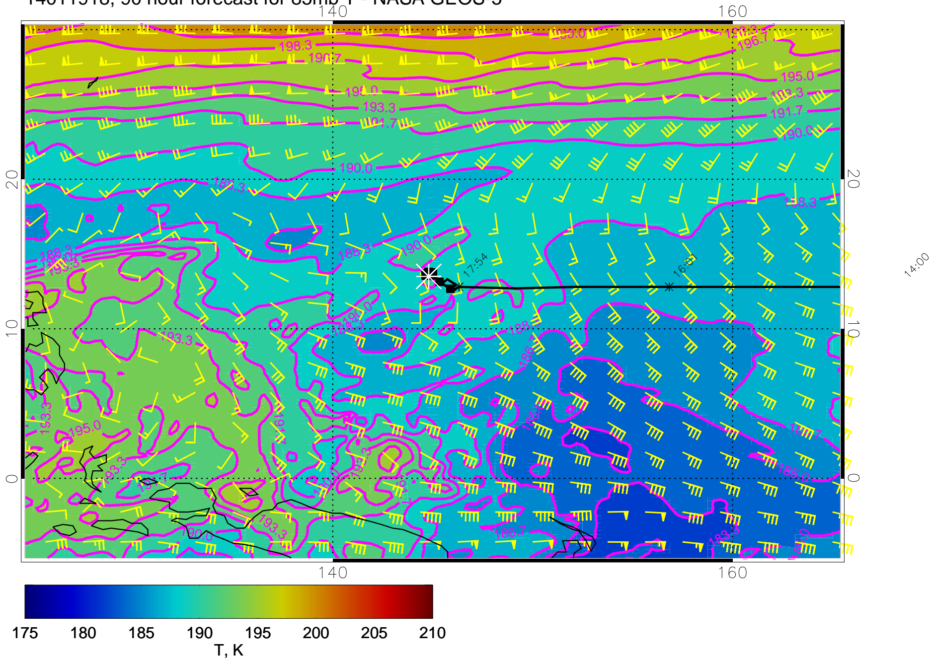
14011918, 90 hour forecast for 85mb T - NASA GEOS-5
