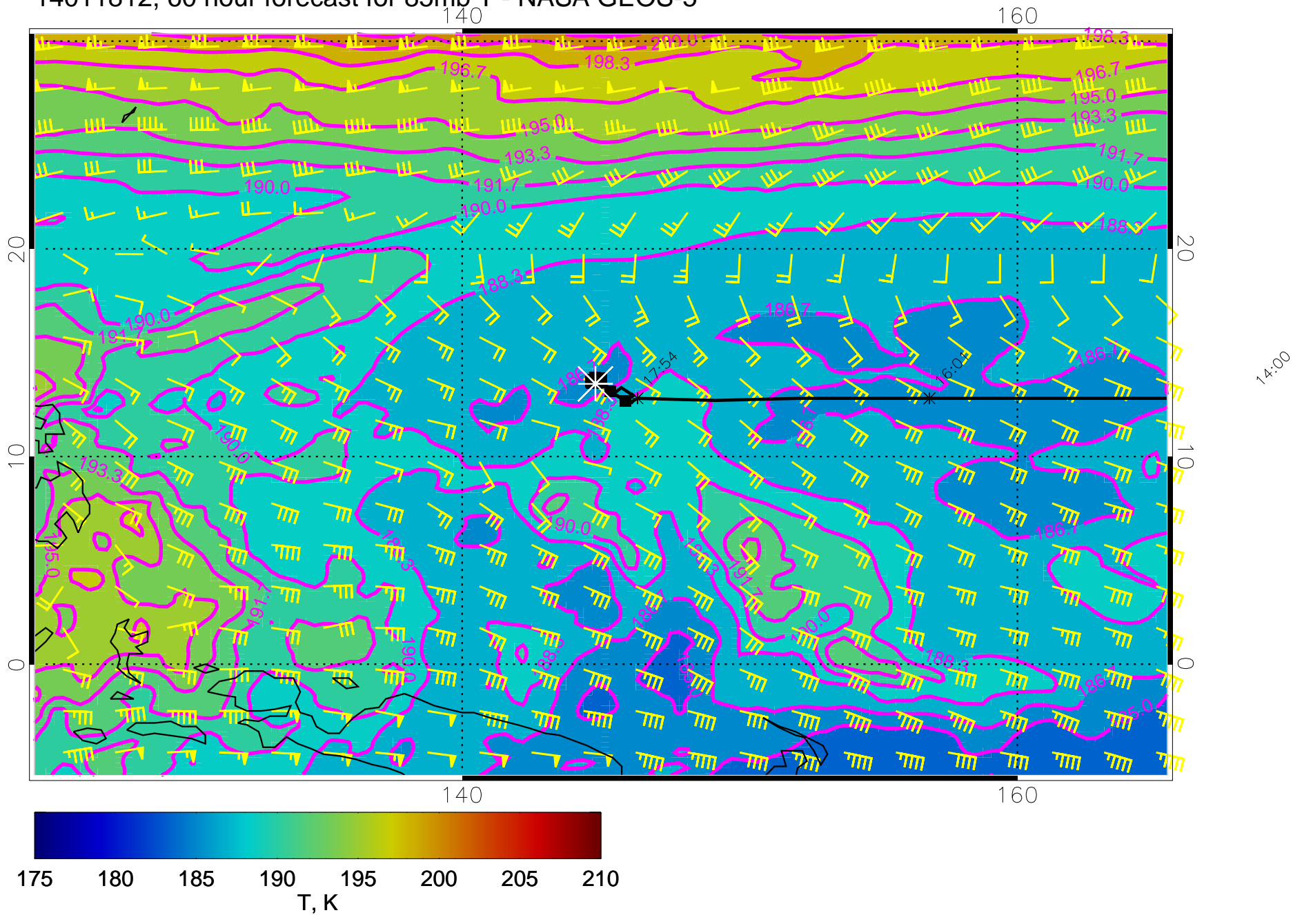
14011812, 60 hour forecast for 85mb T - NASA GEOS-5
