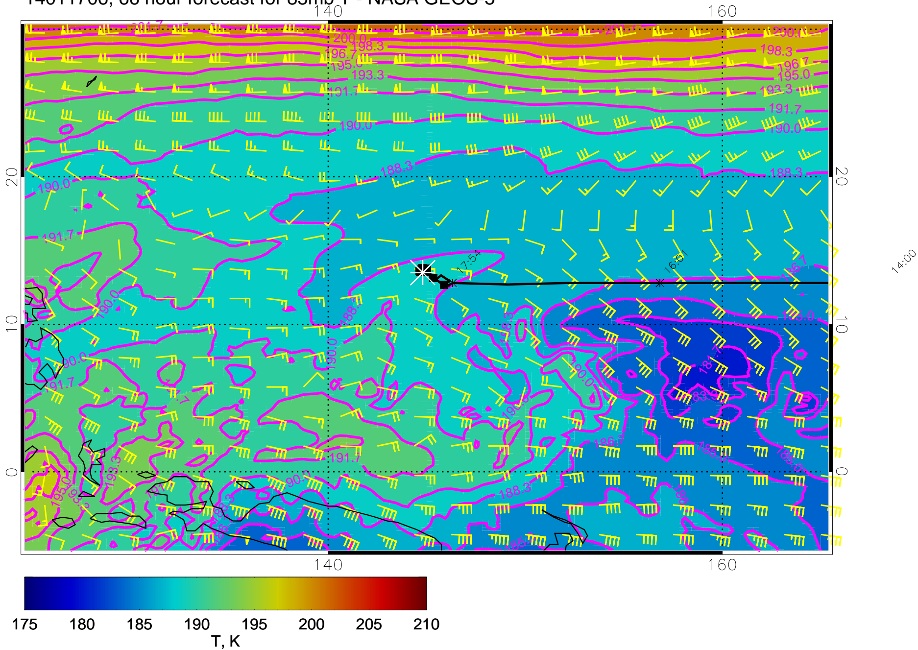
14011706, 66 hour forecast for 85mb T - NASA GEOS-5
