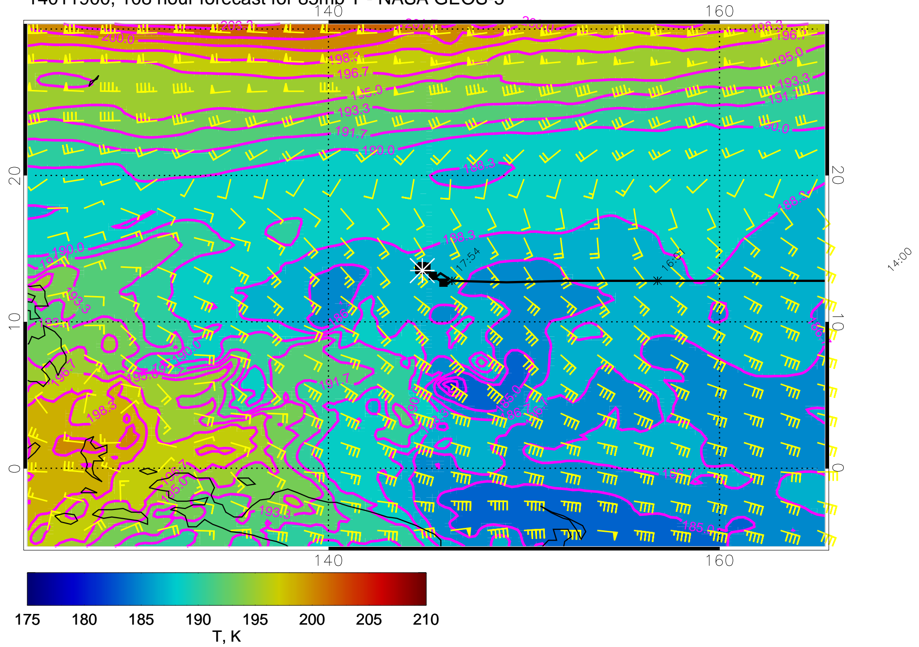
14011900, 108 hour forecast for 85mb T - NASA GEOS-5
