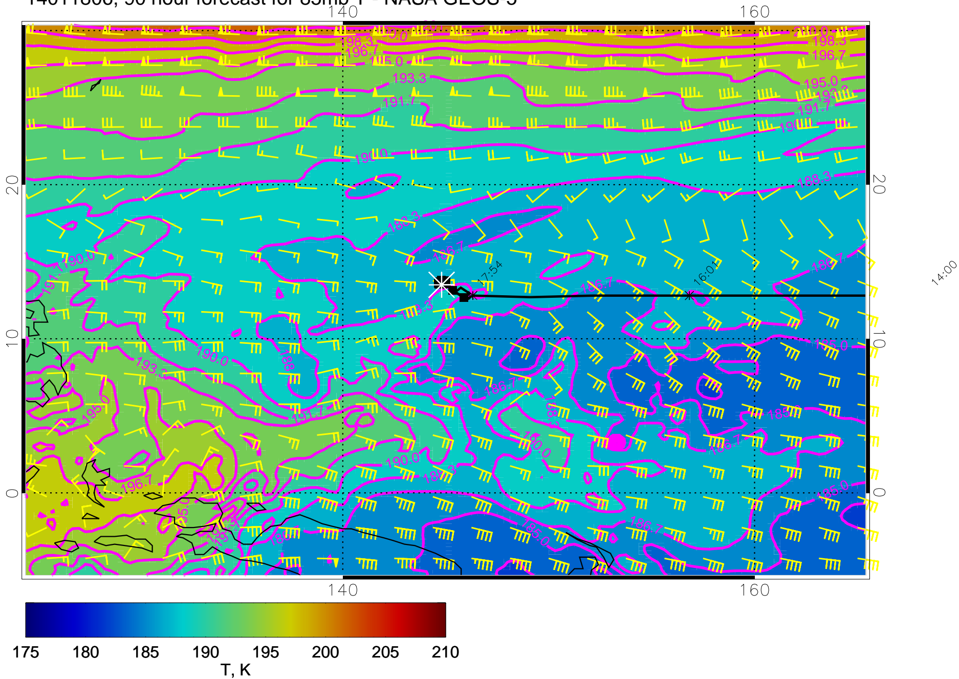
14011806, 90 hour forecast for 85mb T - NASA GEOS-5
