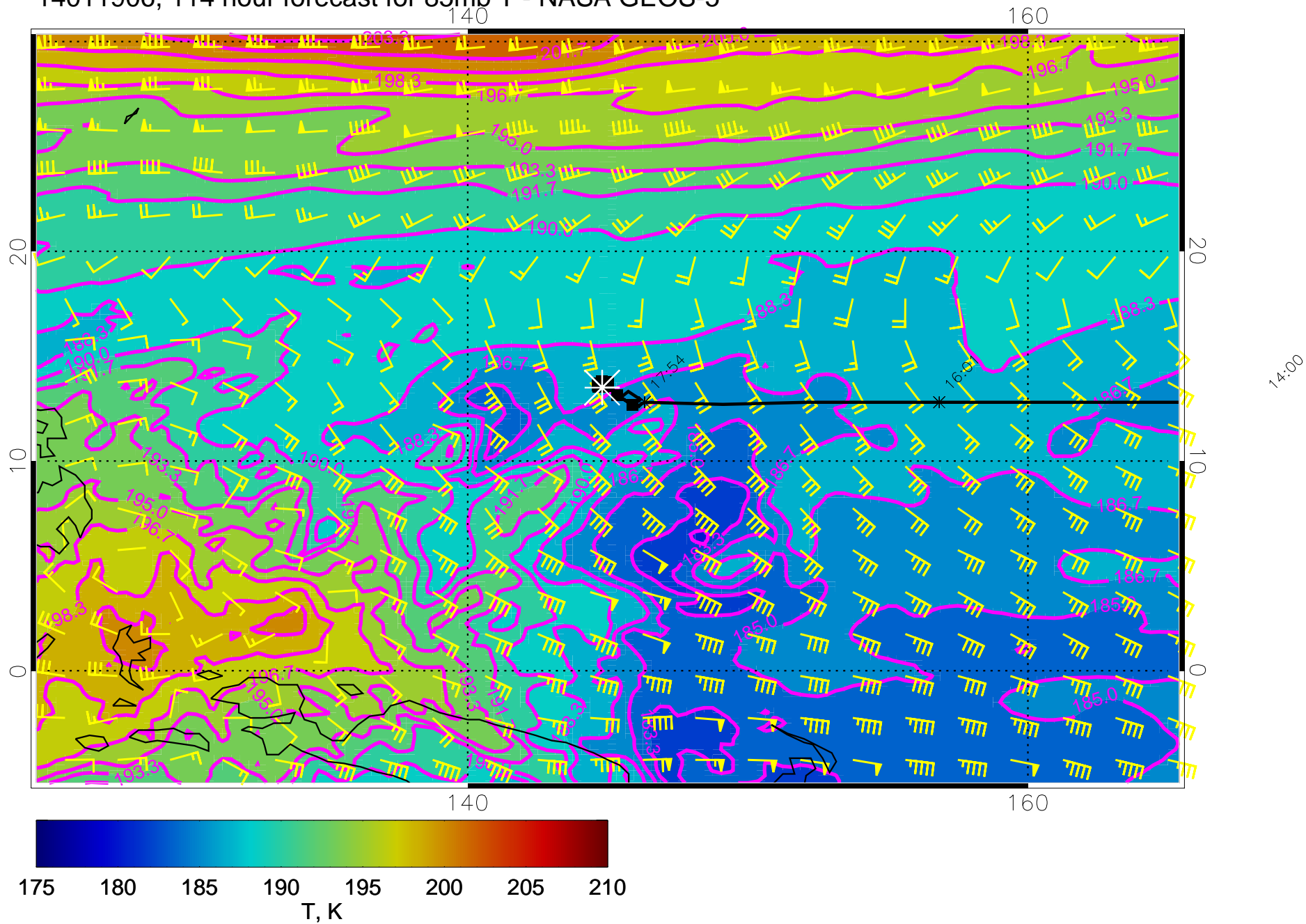
14011906, 114 hour forecast for 85mb T - NASA GEOS-5
