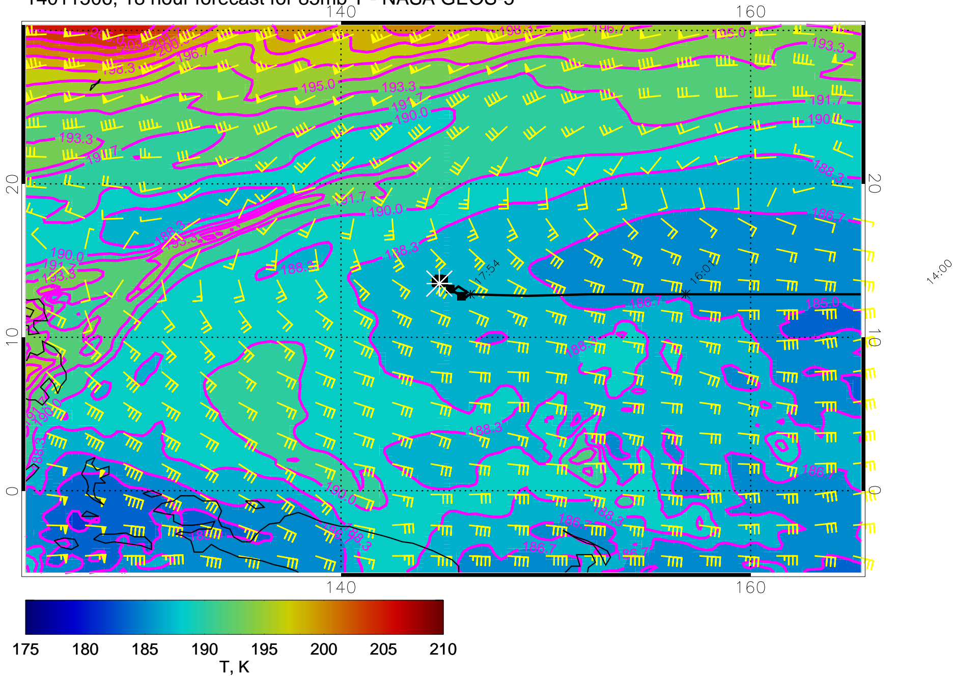
14011506, 18 hour forecast for 85mb T - NASA GEOS-5
