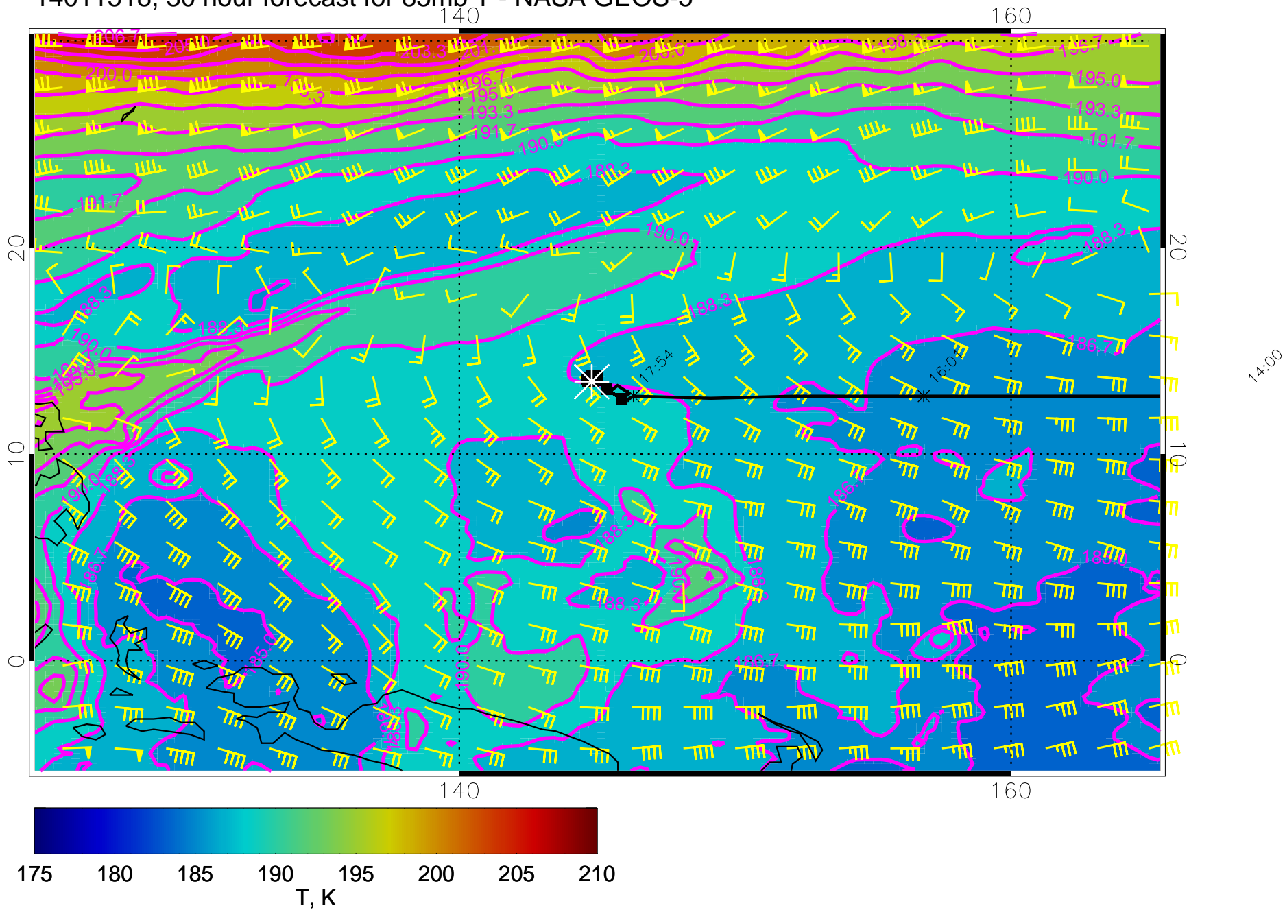
14011518, 30 hour forecast for 85mb T - NASA GEOS-5
