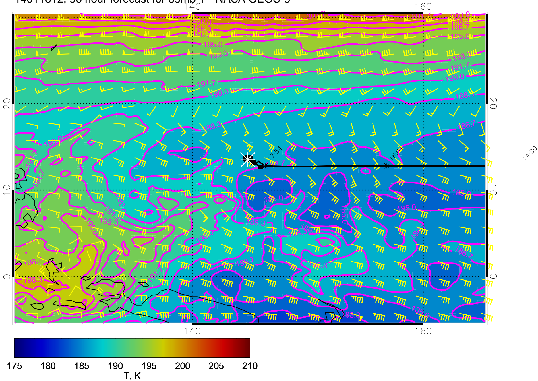
14011812, 96 hour forecast for 85mb T - NASA GEOS-5
