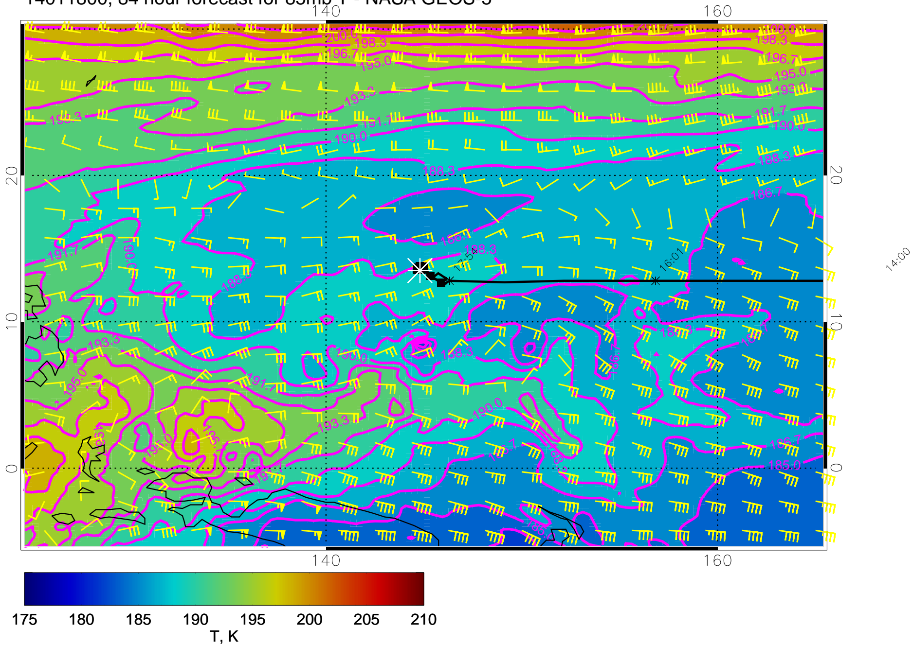
14011800, 84 hour forecast for 85mb T - NASA GEOS-5
