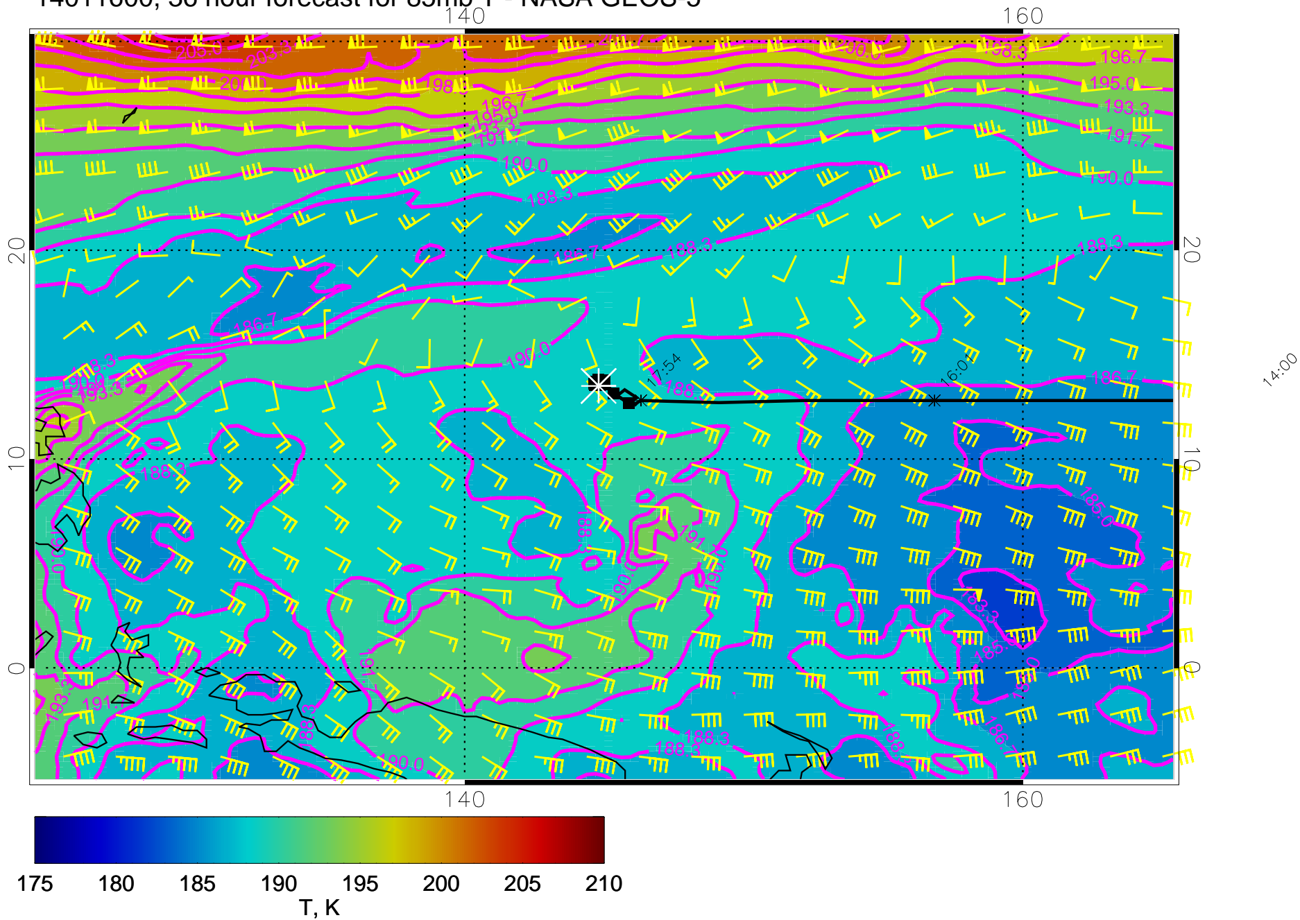
14011600, 36 hour forecast for 85mb T - NASA GEOS-5
