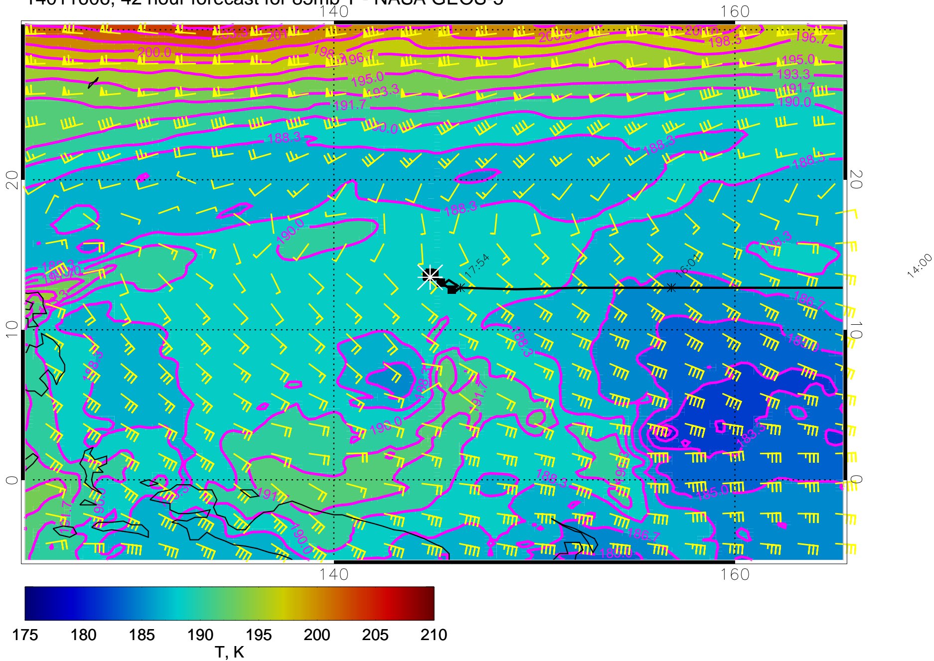
14011606, 42 hour forecast for 85mb T - NASA GEOS-5
