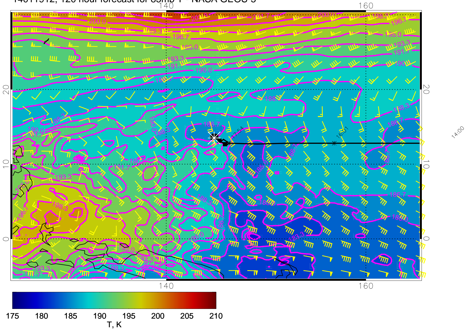
14011912, 120 hour forecast for 85mb T - NASA GEOS-5
