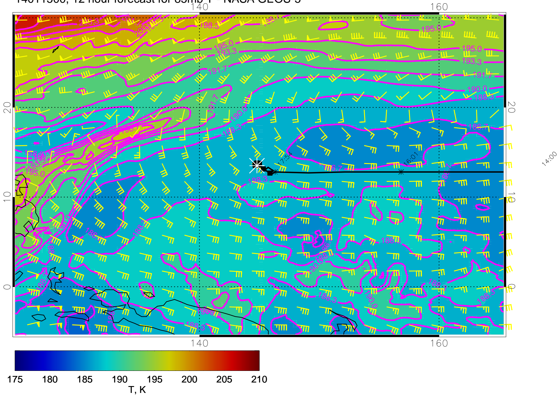
14011500, 12 hour forecast for 85mb T - NASA GEOS-5
