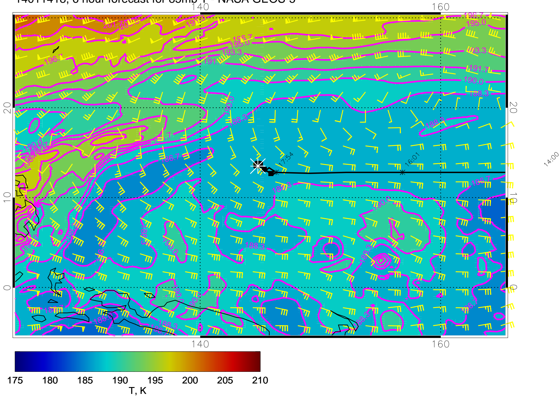
14011418, 6 hour forecast for 85mb T - NASA GEOS-5
