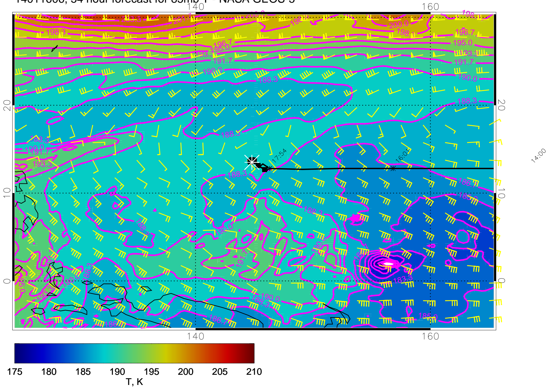
14011606, 54 hour forecast for 85mb T - NASA GEOS-5
