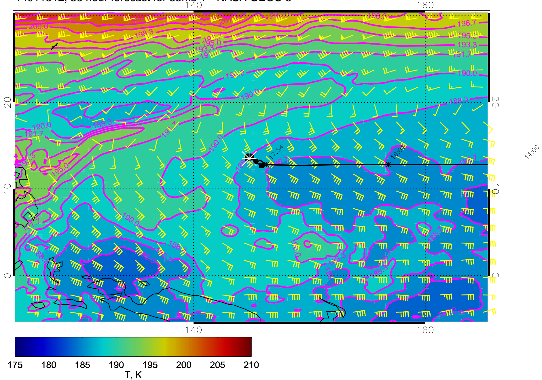
14011512, 36 hour forecast for 85mb T - NASA GEOS-5
