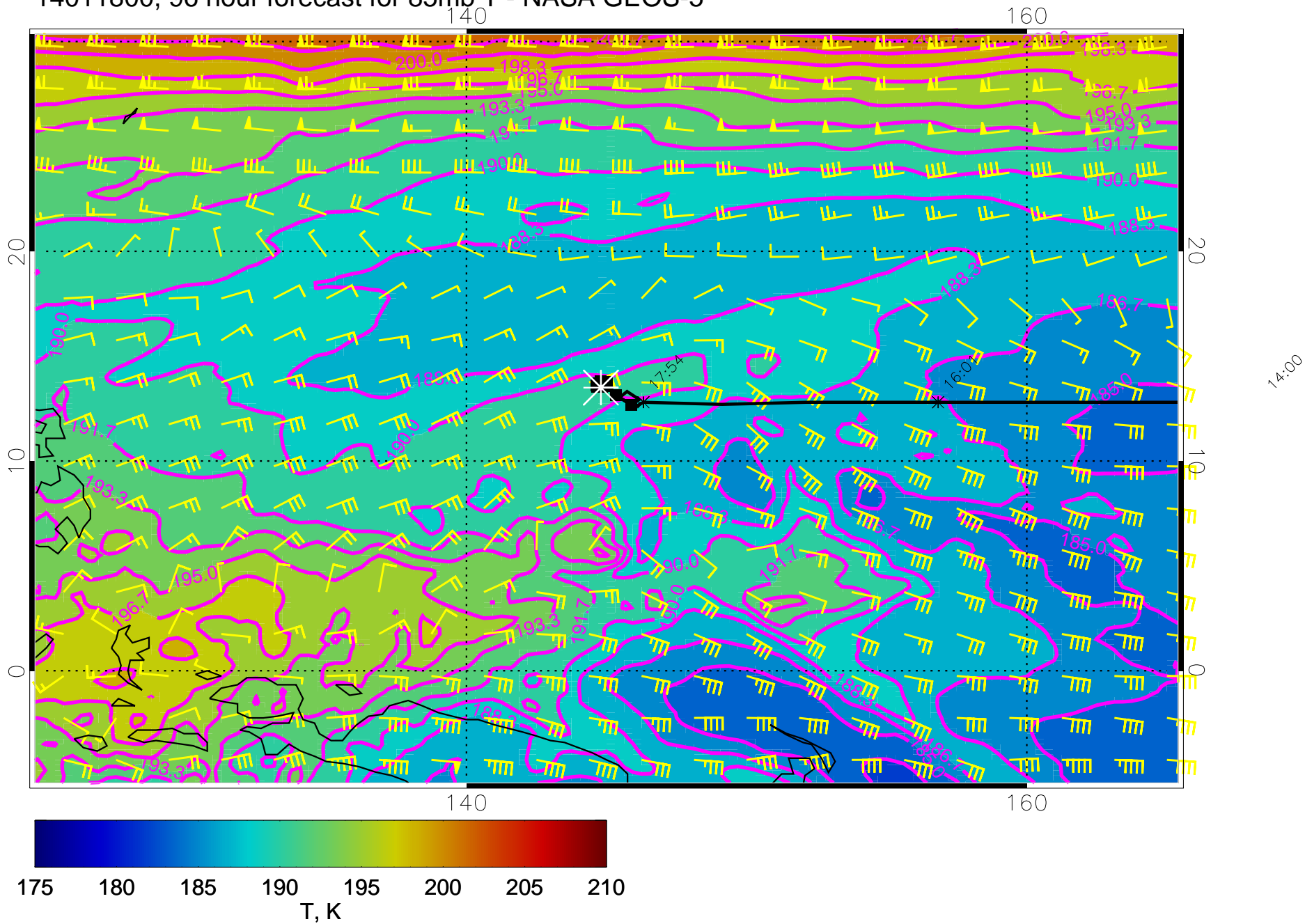
14011800, 96 hour forecast for 85mb T - NASA GEOS-5
