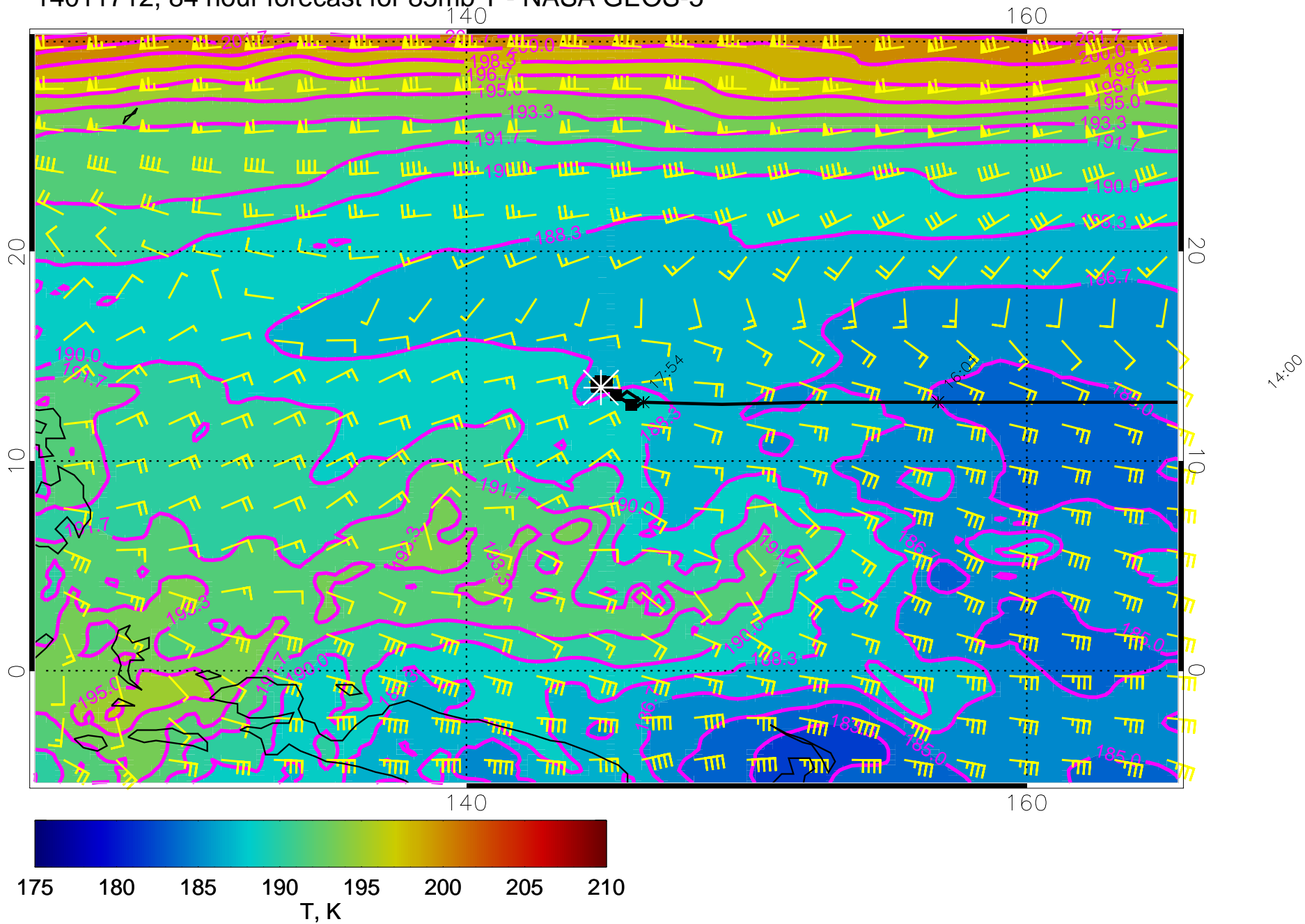
14011712, 84 hour forecast for 85mb T - NASA GEOS-5
