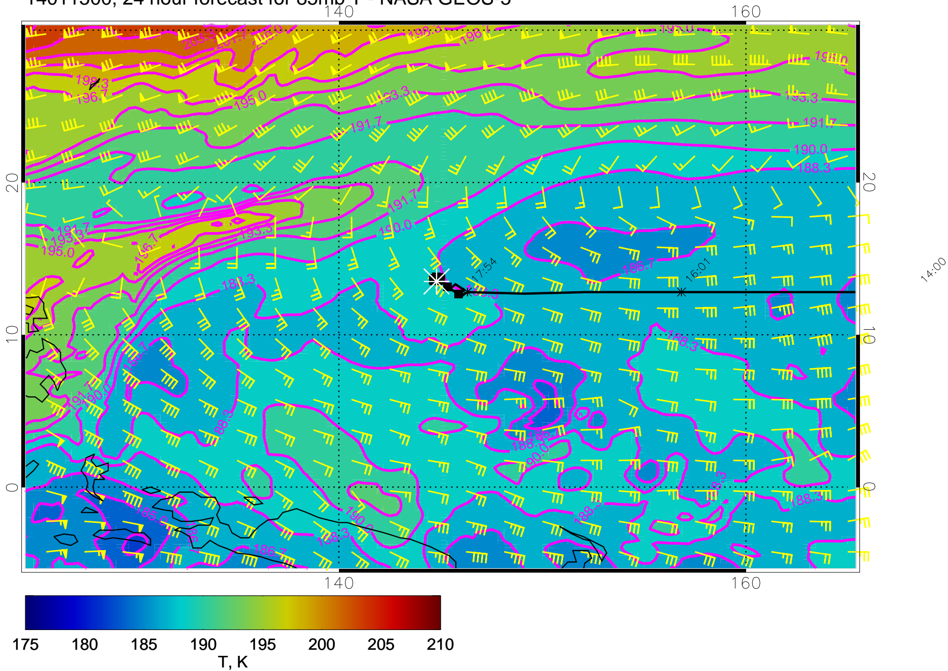
14011500, 24 hour forecast for 85mb T - NASA GEOS-5
