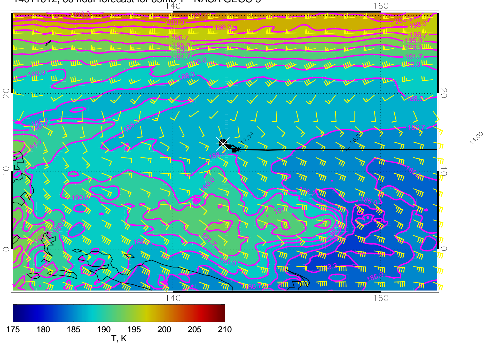
14011612, 60 hour forecast for 85mb T - NASA GEOS-5
