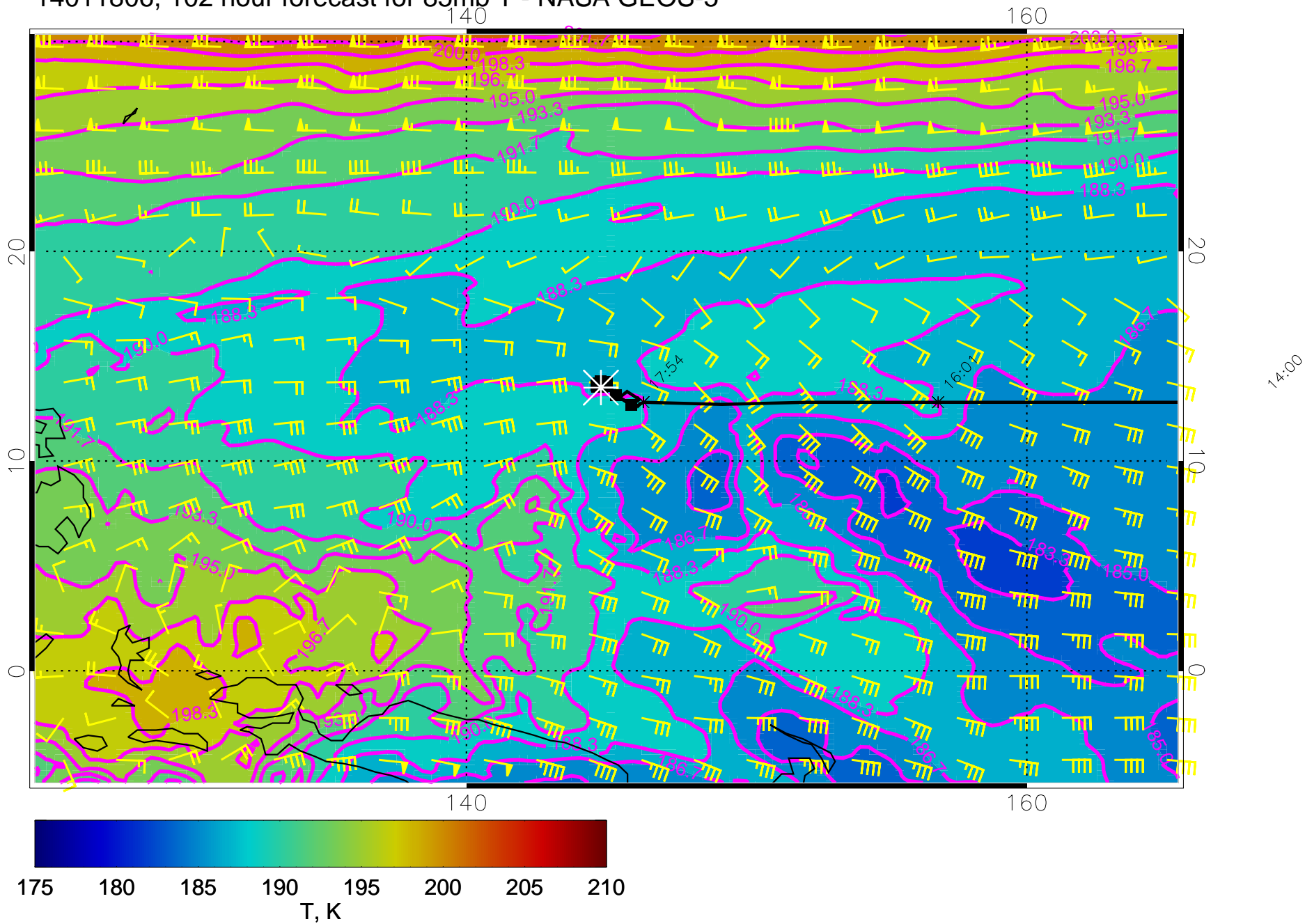
14011806, 102 hour forecast for 85mb T - NASA GEOS-5
