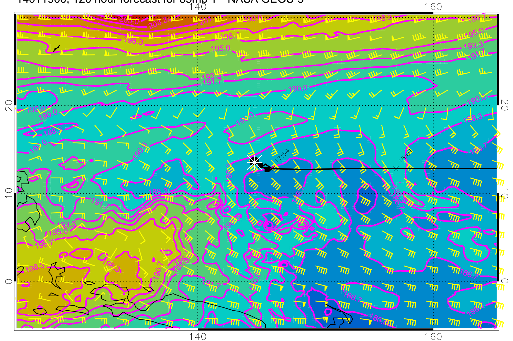
14011900, 120 hour forecast for 85mb T - NASA GEOS-5
