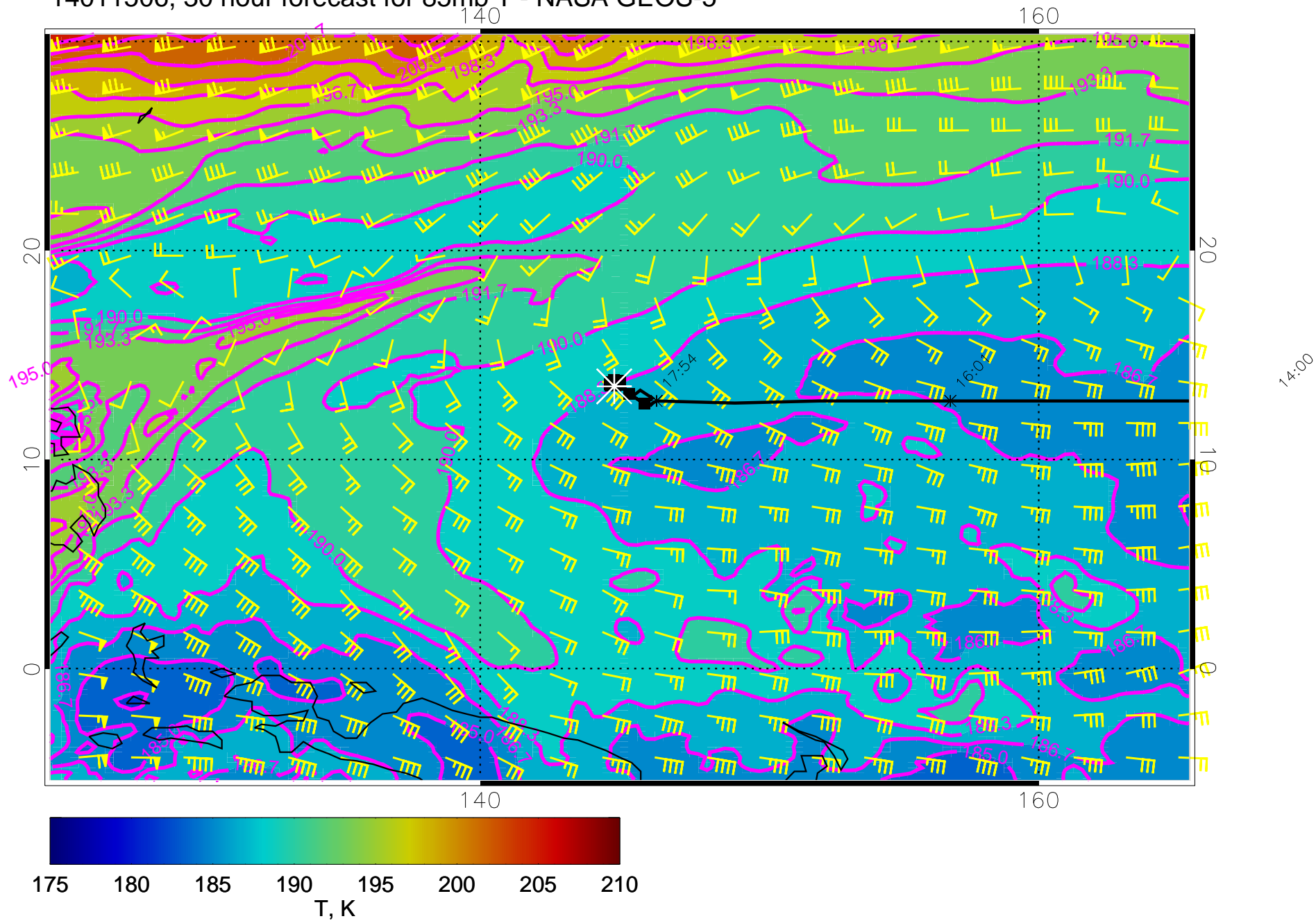
14011506, 30 hour forecast for 85mb T - NASA GEOS-5
