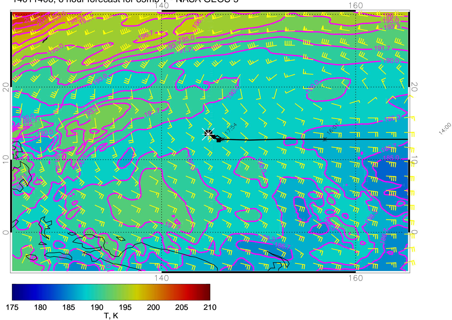
14011406, 6 hour forecast for 85mb T - NASA GEOS-5
