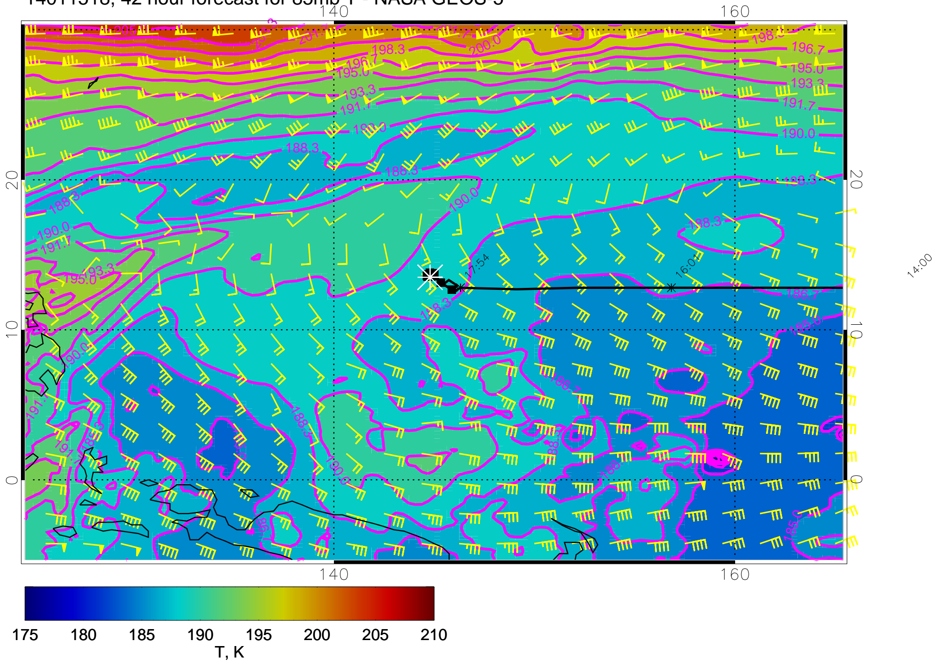
14011518, 42 hour forecast for 85mb T - NASA GEOS-5
