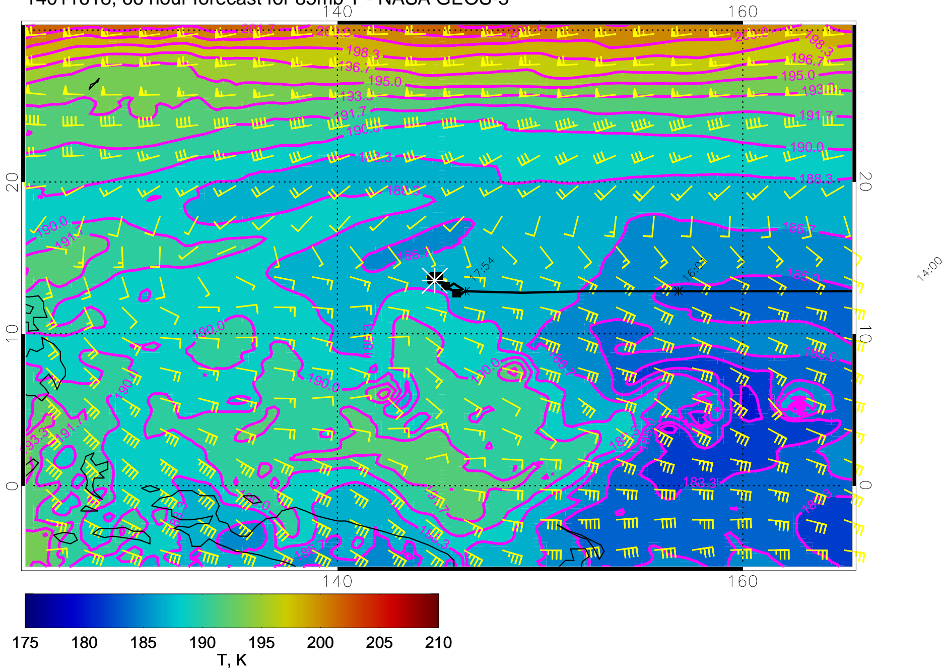
14011618, 66 hour forecast for 85mb T - NASA GEOS-5
