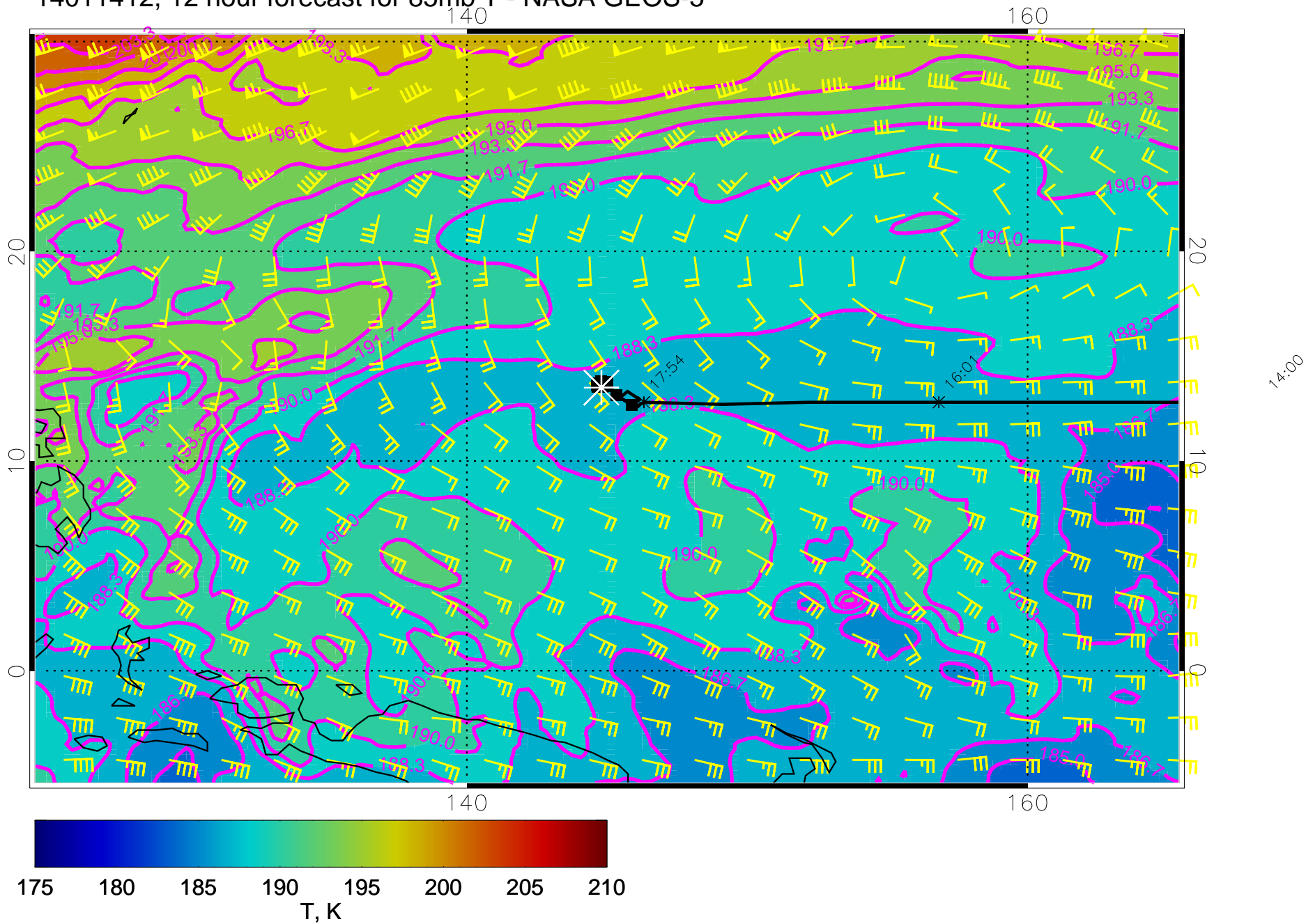
14011412, 12 hour forecast for 85mb T - NASA GEOS-5
