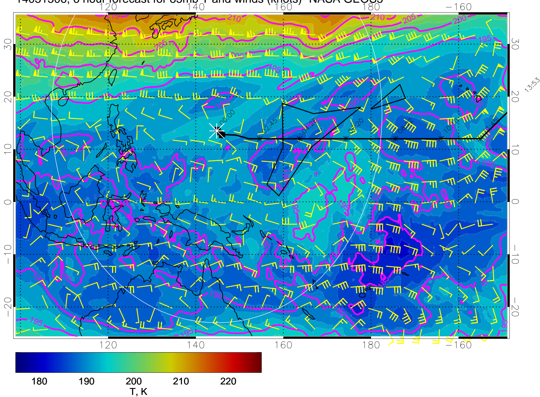
14031306, 6 hour forecast for 85mb T and winds (knots)- NASA GEOS5
