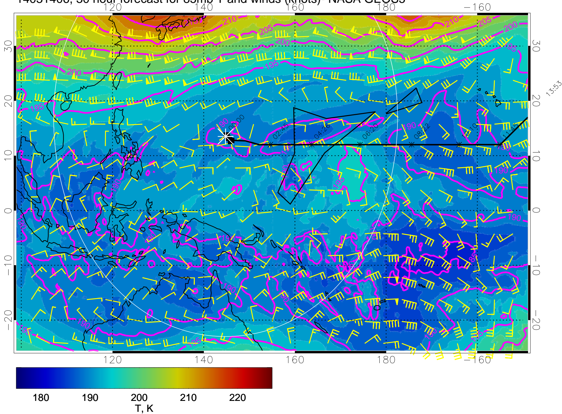
14031406, 30 hour forecast for 85mb T and winds (knots)- NASA GEOS5
