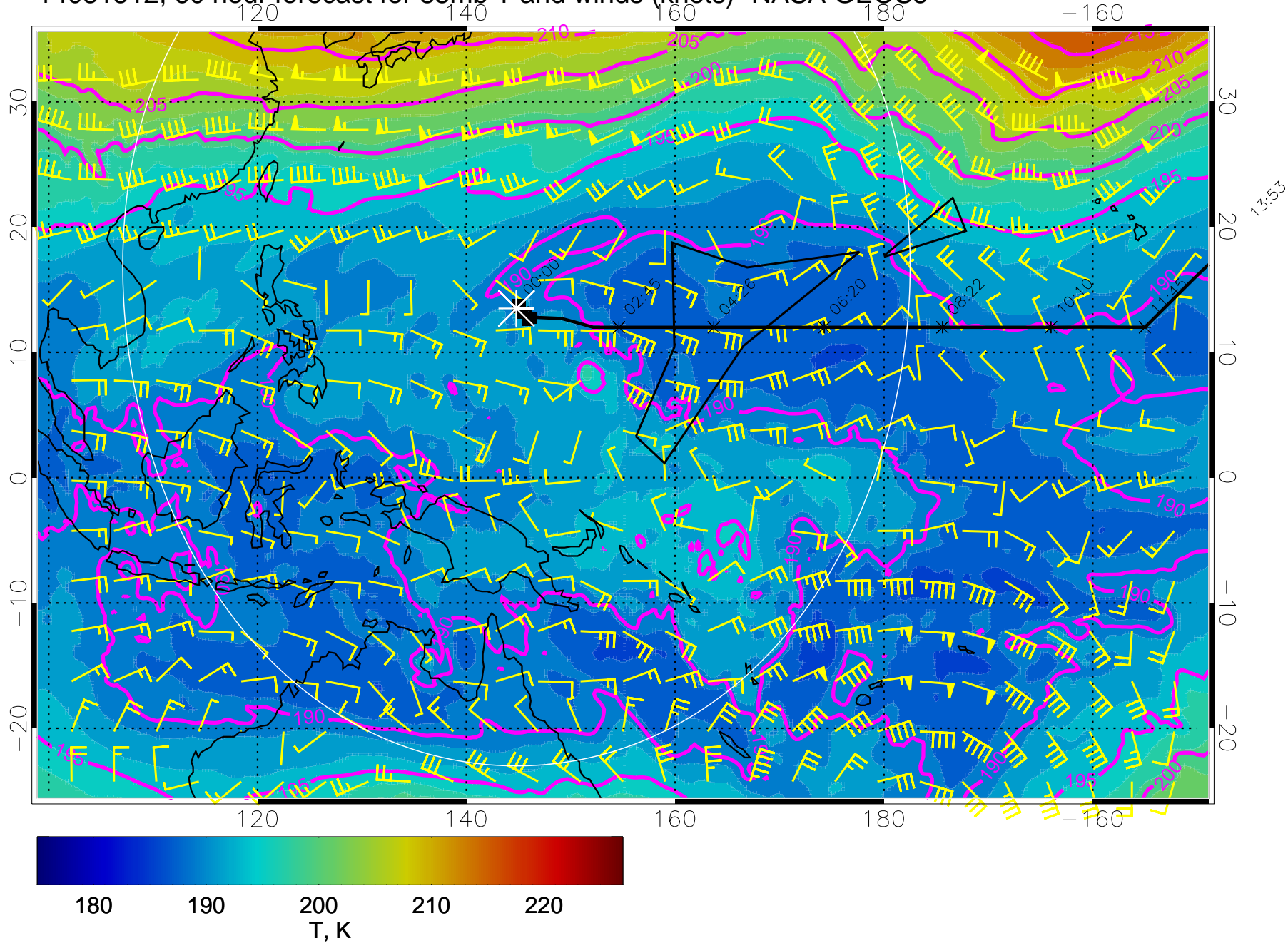
14031512, 60 hour forecast for 85mb T and winds (knots)- NASA GEOS5
