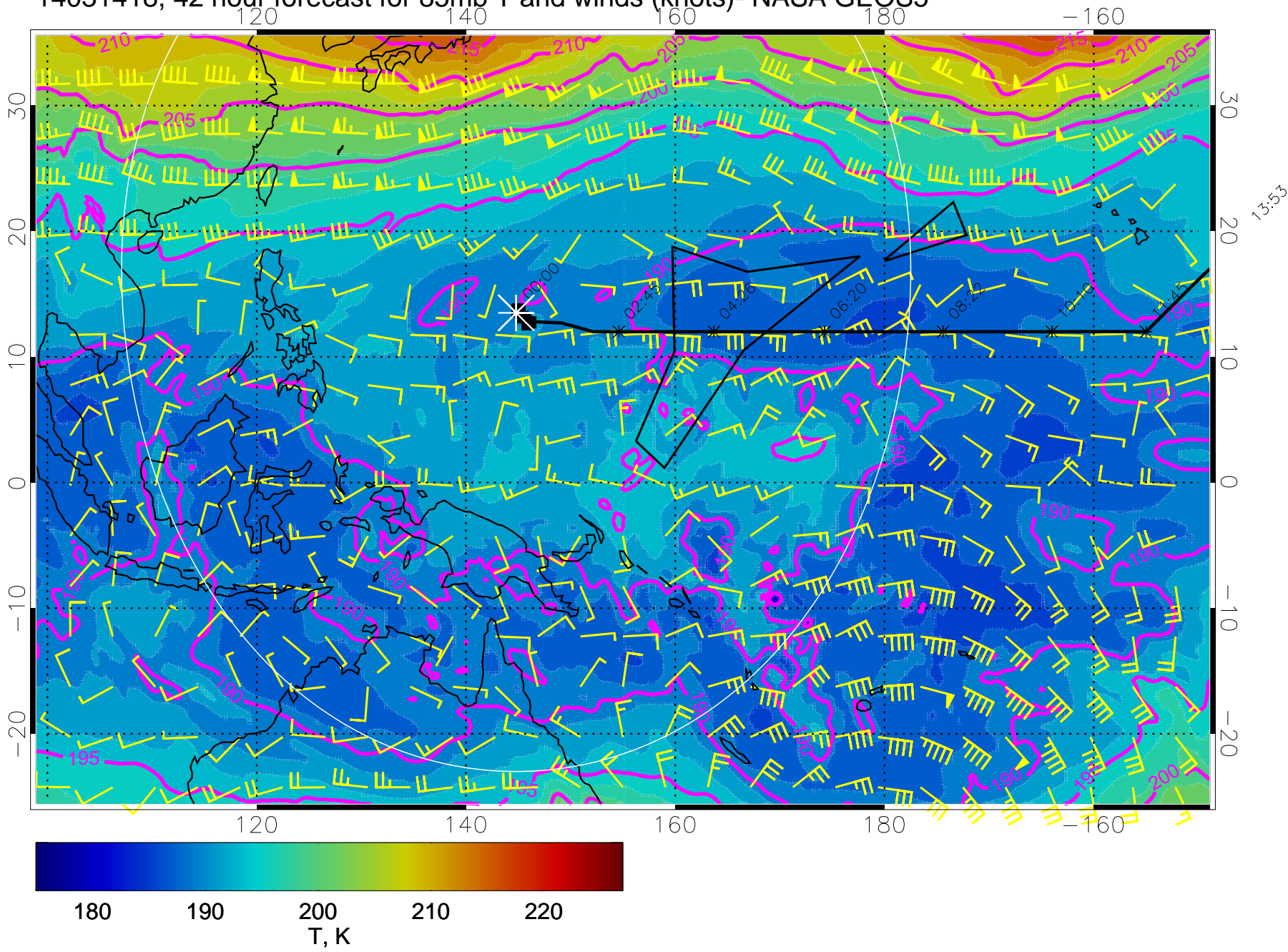
14031418, 42 hour forecast for 85mb T and winds (knots)- NASA GEOS5
