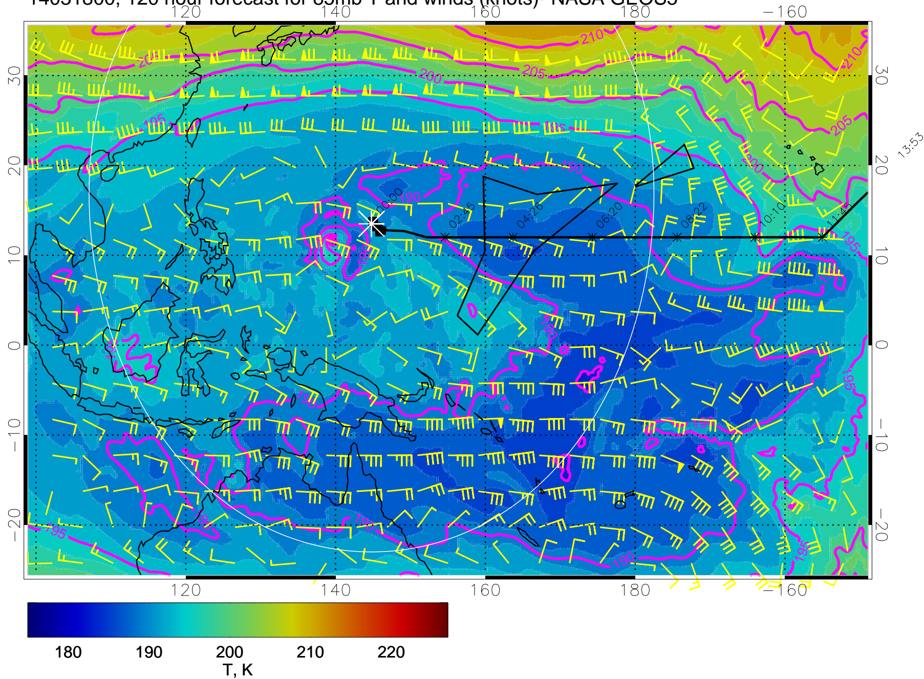
14031800, 120 hour forecast for 85mb T and winds (knots)- NASA GEOS5
