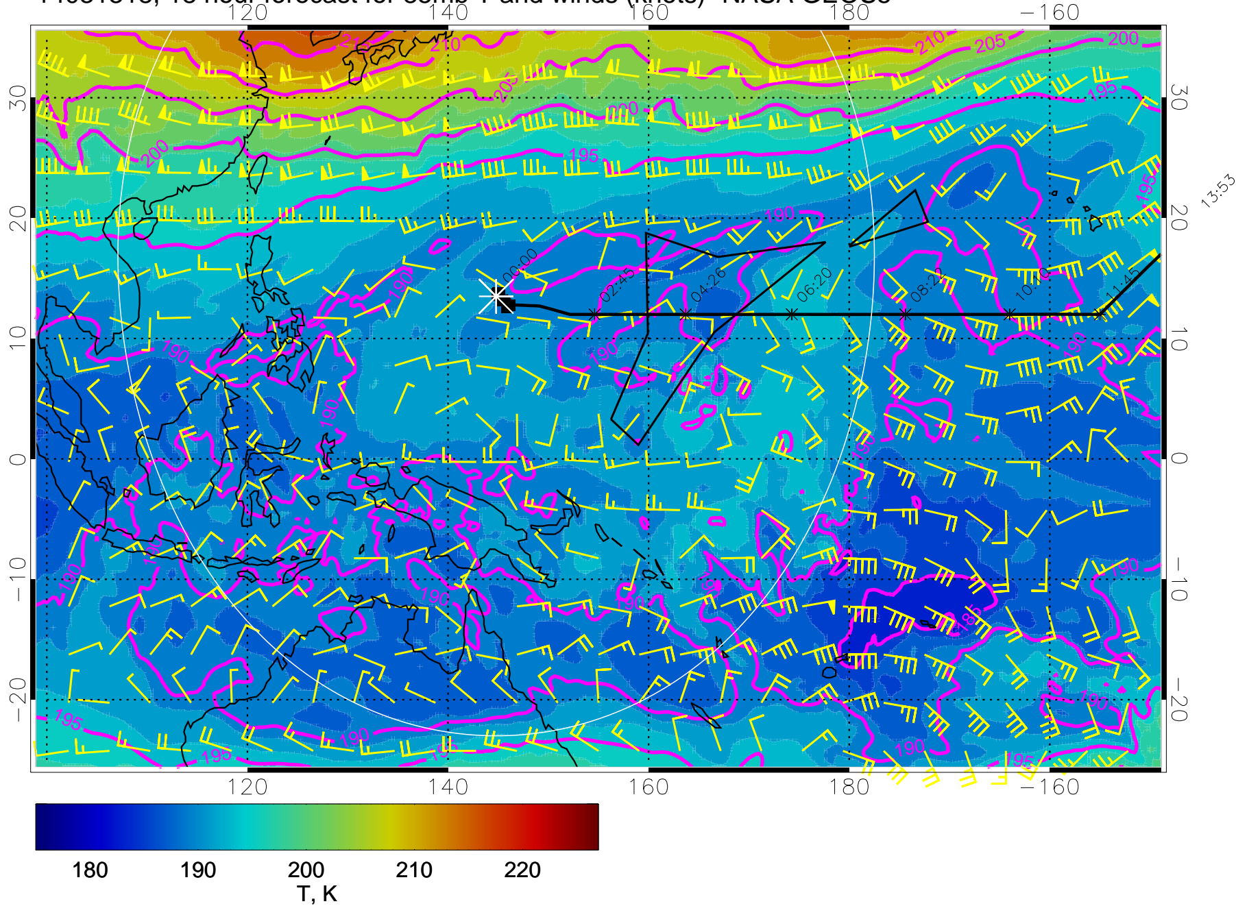
14031318, 18 hour forecast for 85mb T and winds (knots)- NASA GEOS5
