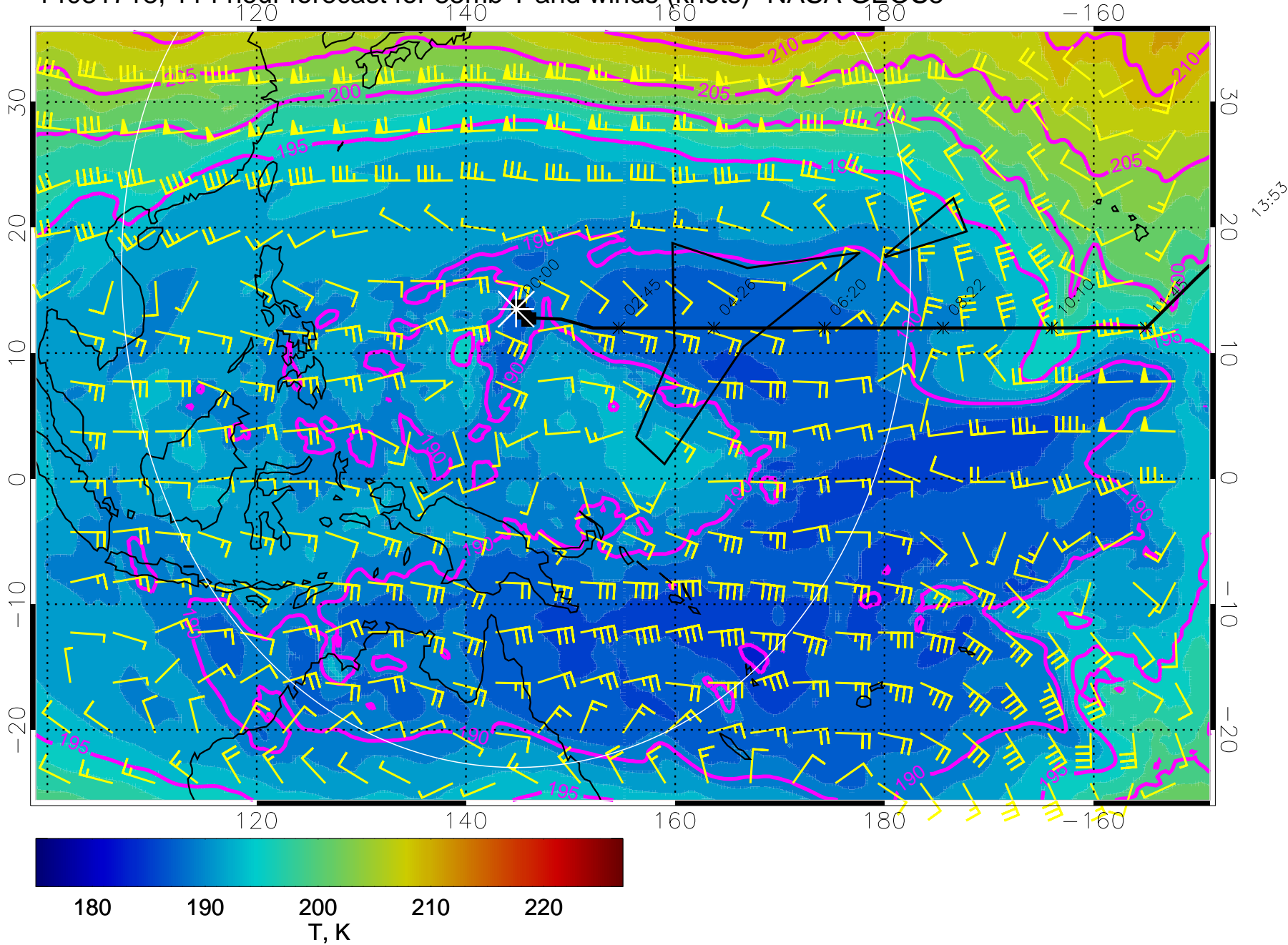
14031718, 114 hour forecast for 85mb T and winds (knots)- NASA GEOS5
