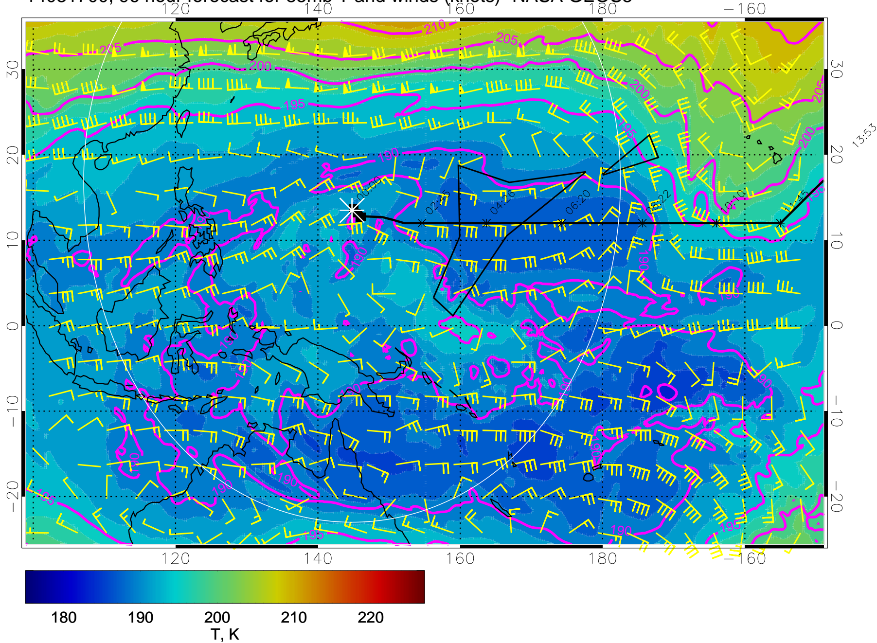
14031700, 96 hour forecast for 85mb T and winds (knots)- NASA GEOS5
