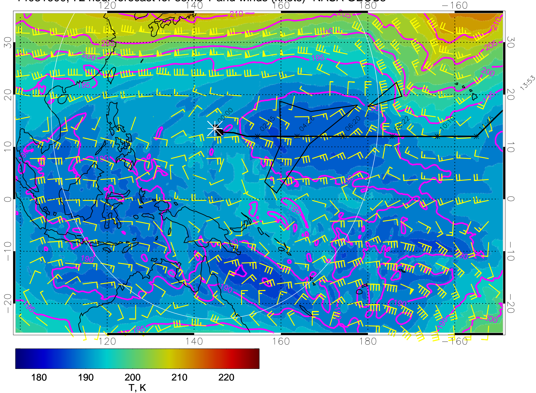
14031600, 72 hour forecast for 85mb T and winds (knots)- NASA GEOS5
