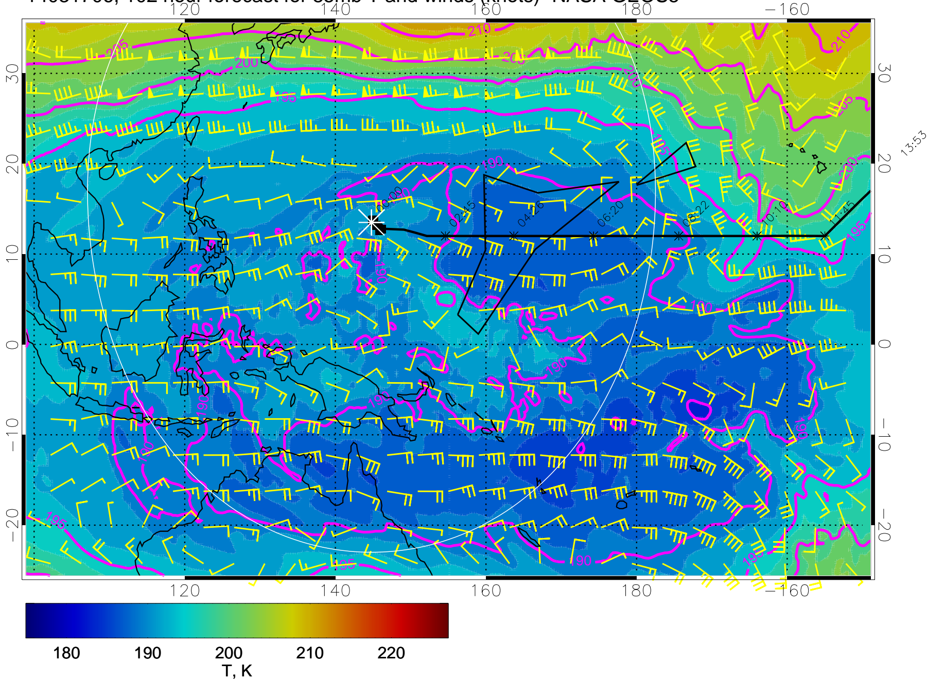
14031706, 102 hour forecast for 85mb T and winds (knots)- NASA GEOS5
