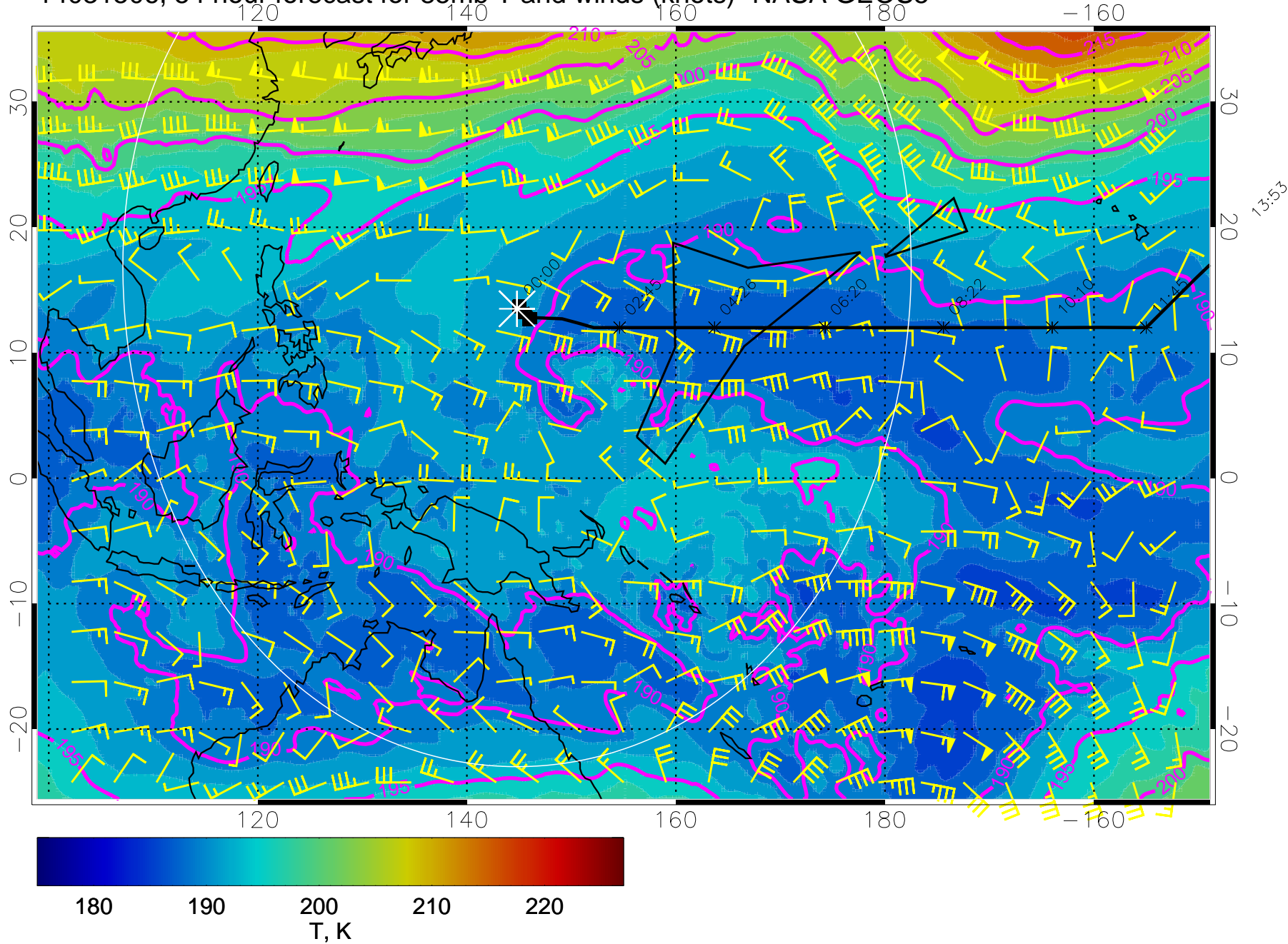
14031506, 54 hour forecast for 85mb T and winds (knots)- NASA GEOS5
