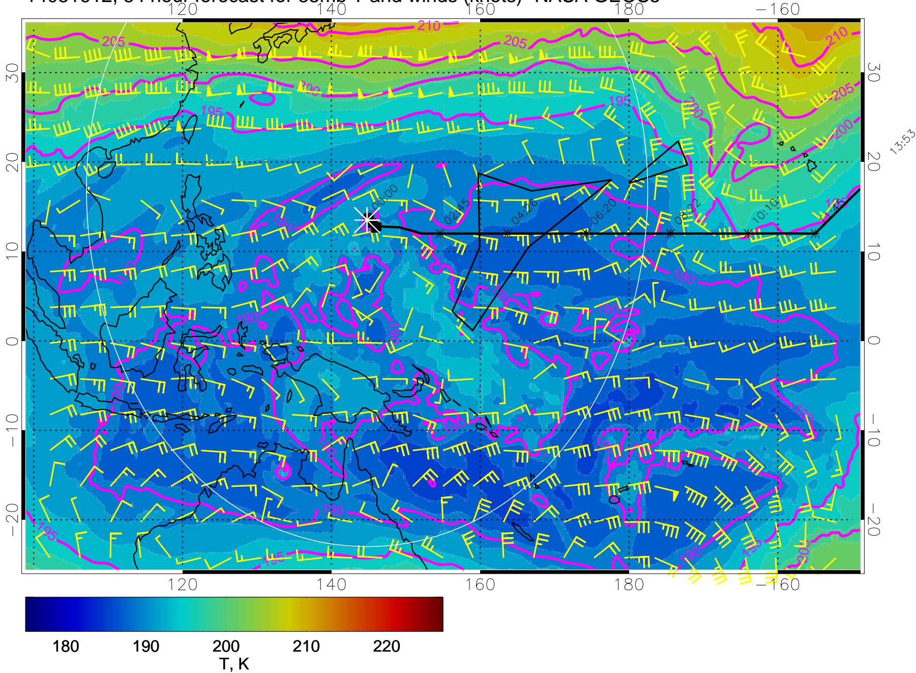
14031612, 84 hour forecast for 85mb T and winds (knots)- NASA GEOS5
