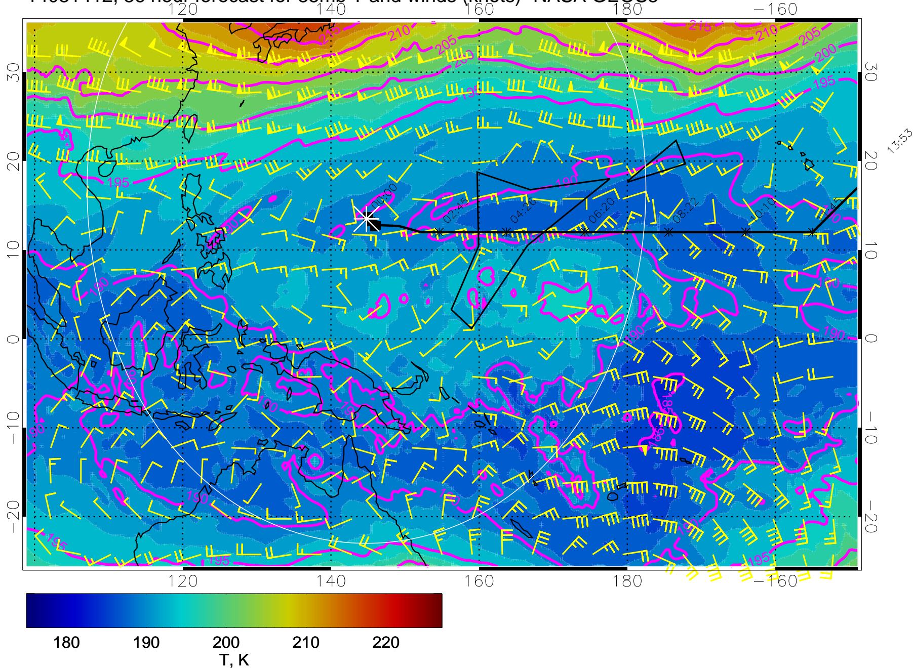
14031412, 36 hour forecast for 85mb T and winds (knots)- NASA GEOS5
