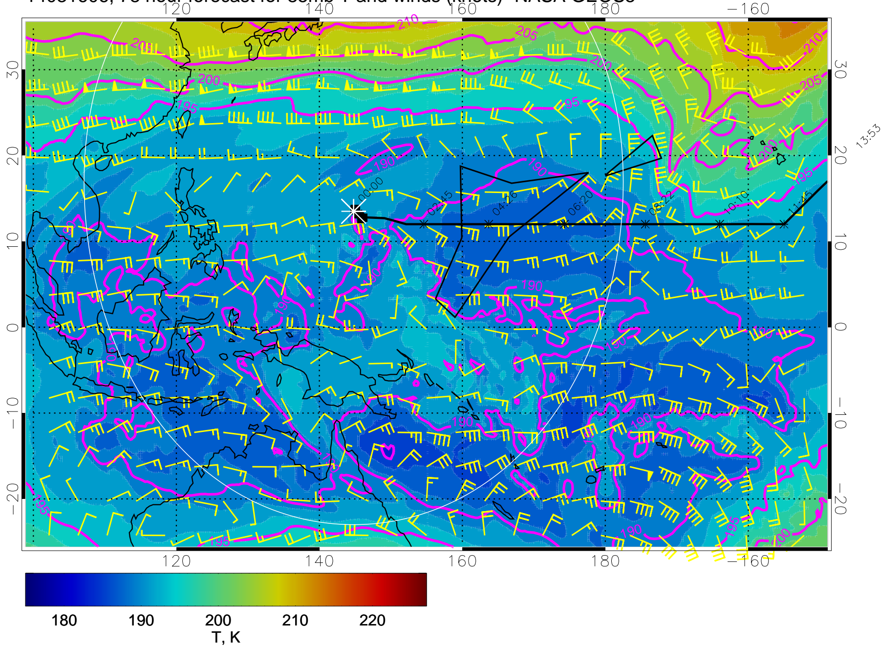
14031606, 78 hour forecast for 85mb T and winds (knots)- NASA GEOS5
