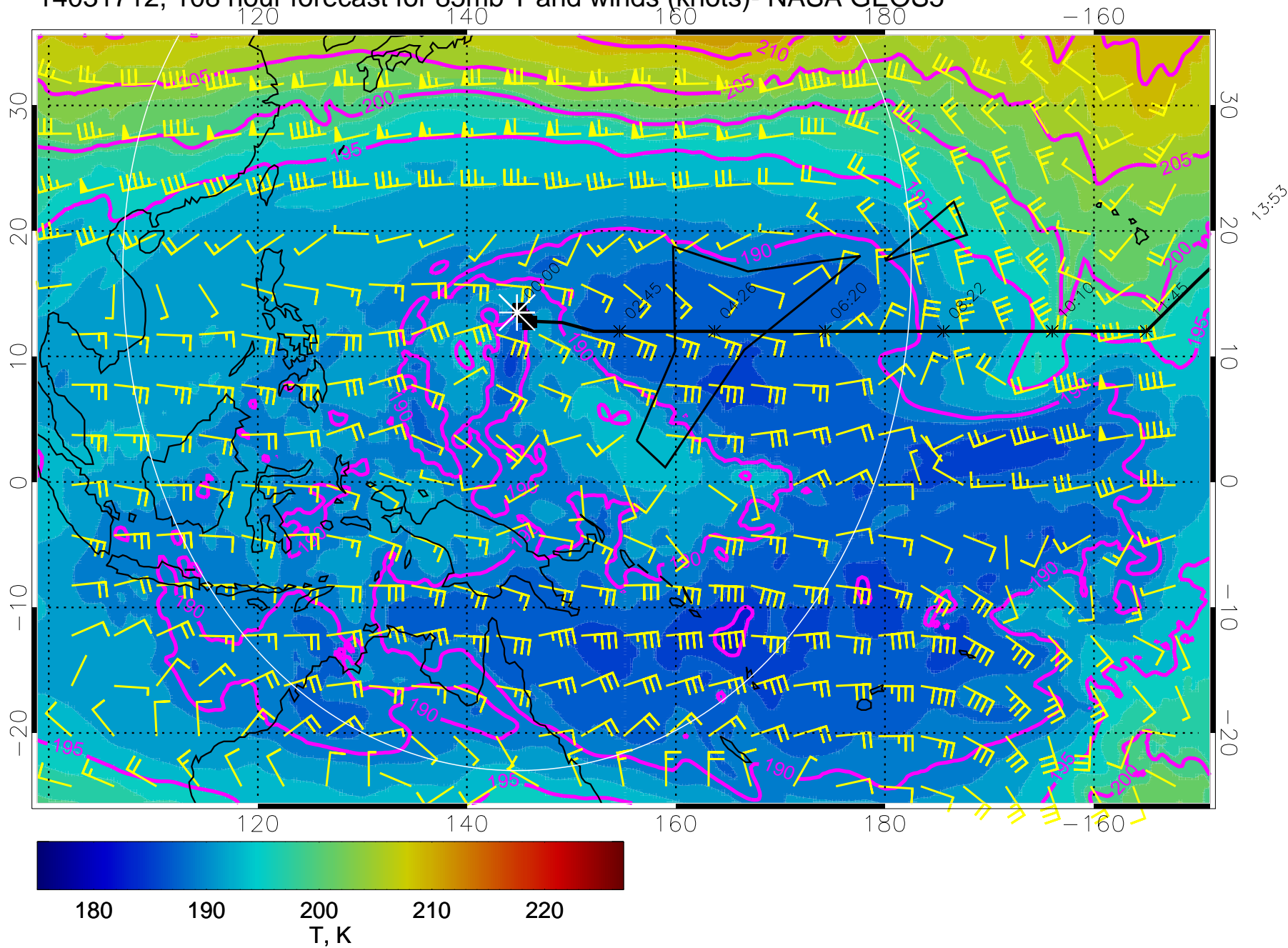
14031712, 108 hour forecast for 85mb T and winds (knots)- NASA GEOS5
