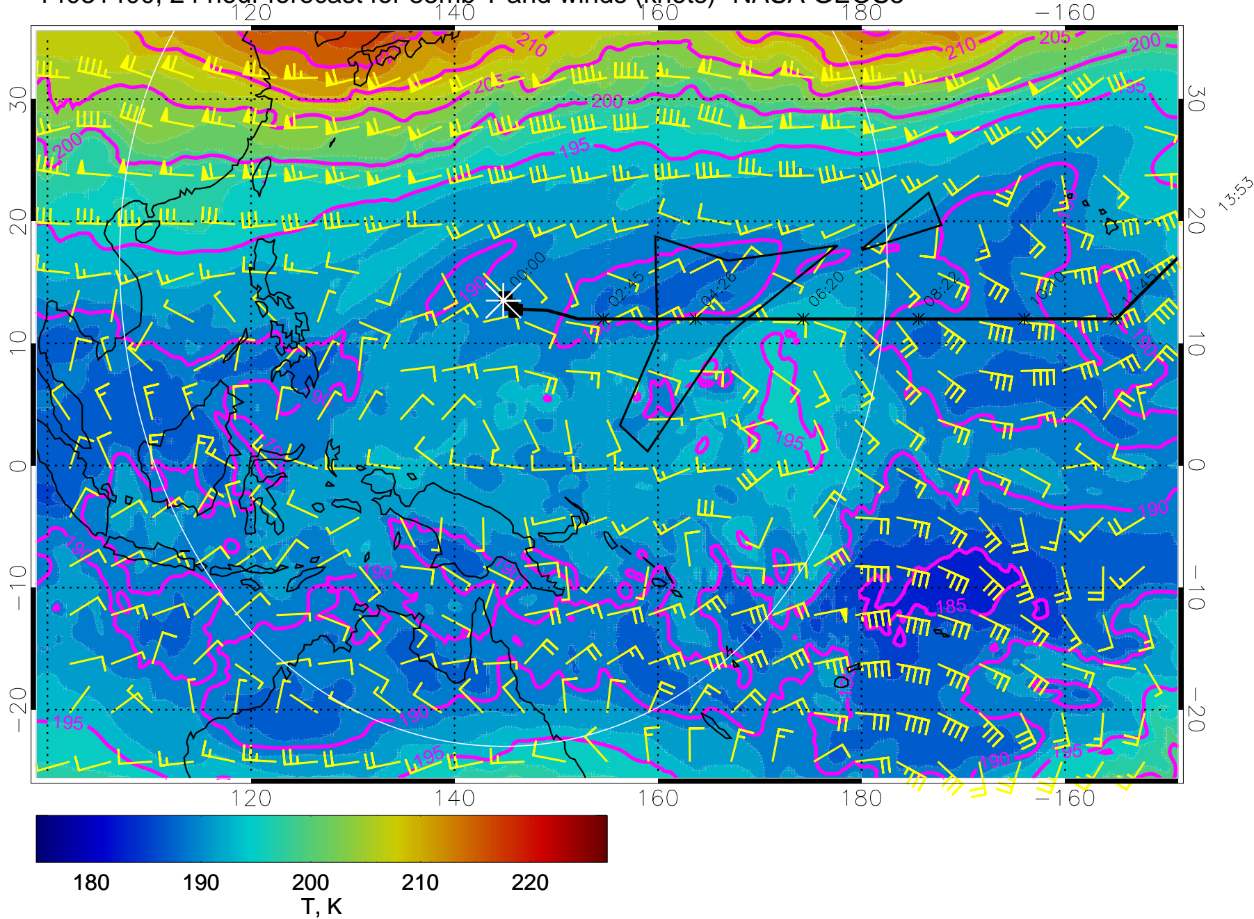
14031400, 24 hour forecast for 85mb T and winds (knots)- NASA GEOS5
