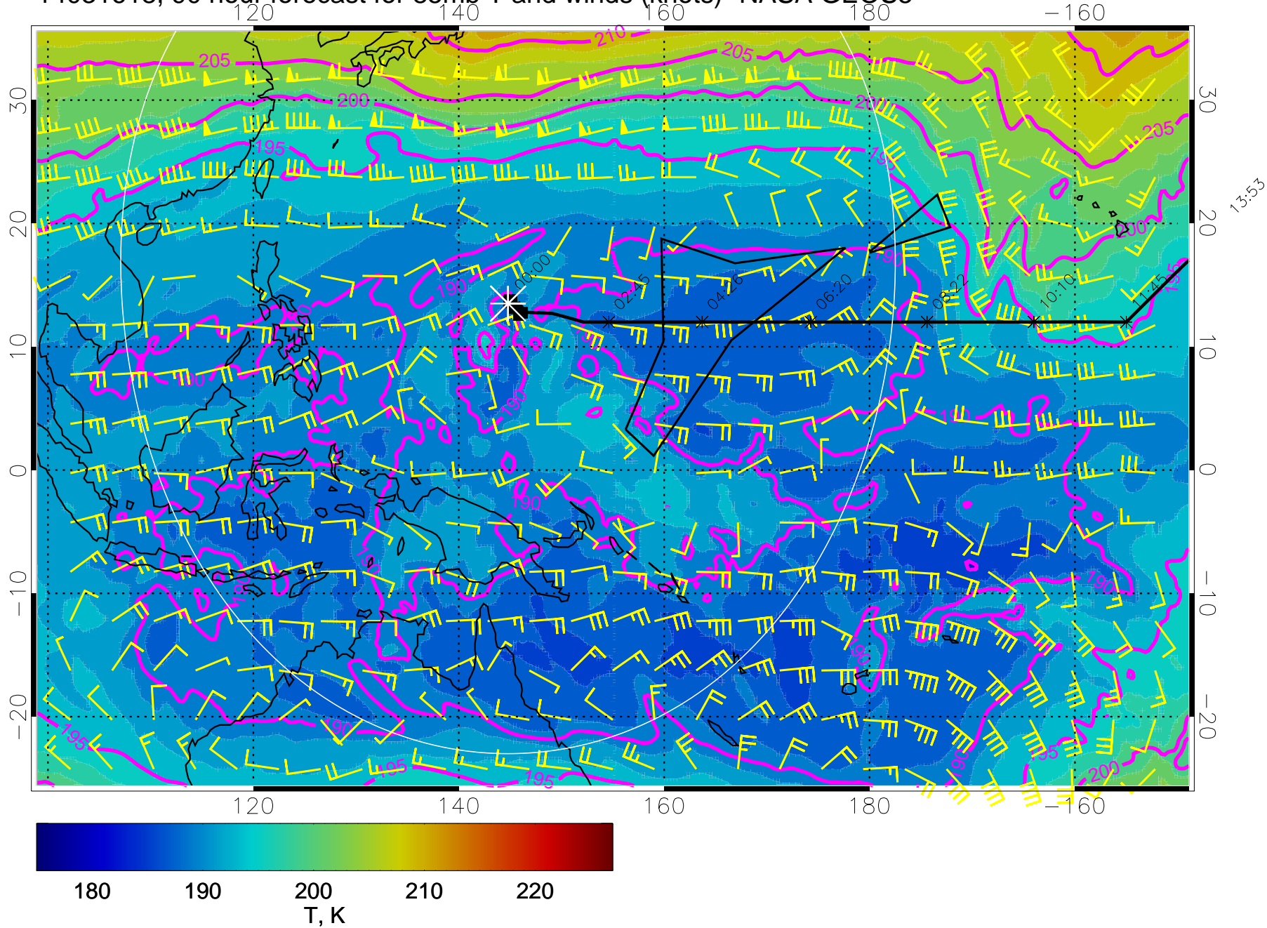
14031618, 90 hour forecast for 85mb T and winds (knots)- NASA GEOS5
