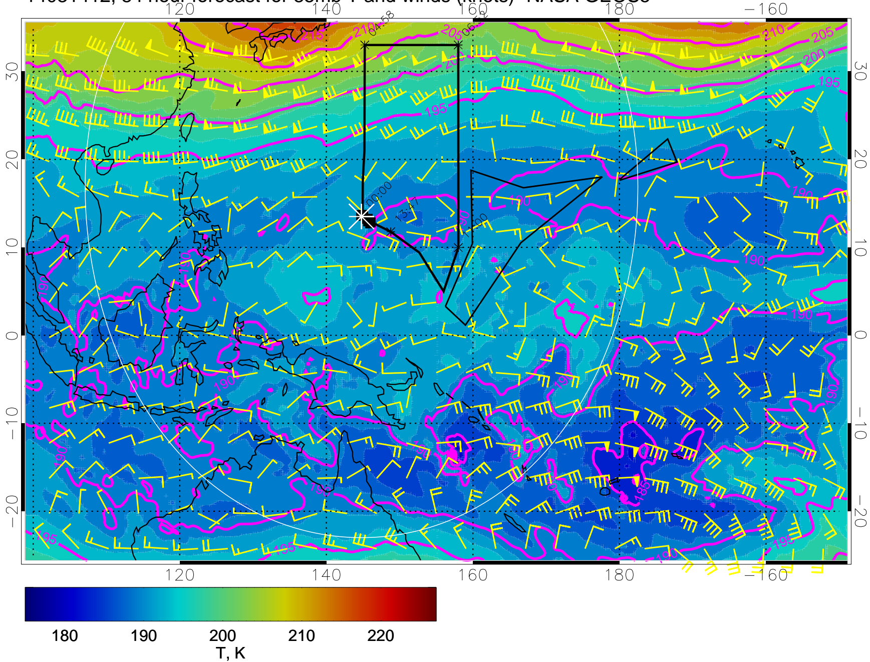
14031412, 84 hour forecast for 85mb T and winds (knots)- NASA GEOS5
