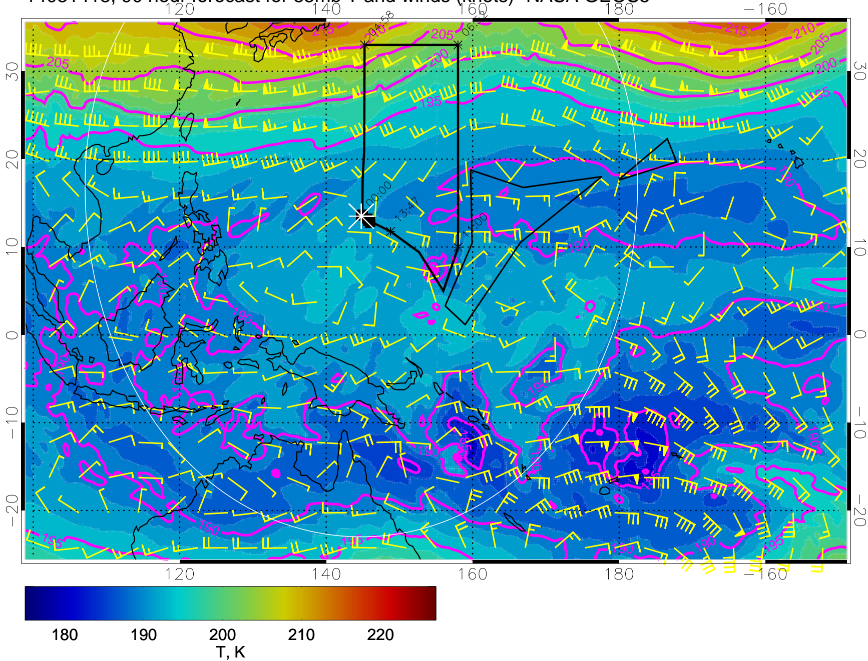
14031418, 90 hour forecast for 85mb T and winds (knots)- NASA GEOS5
