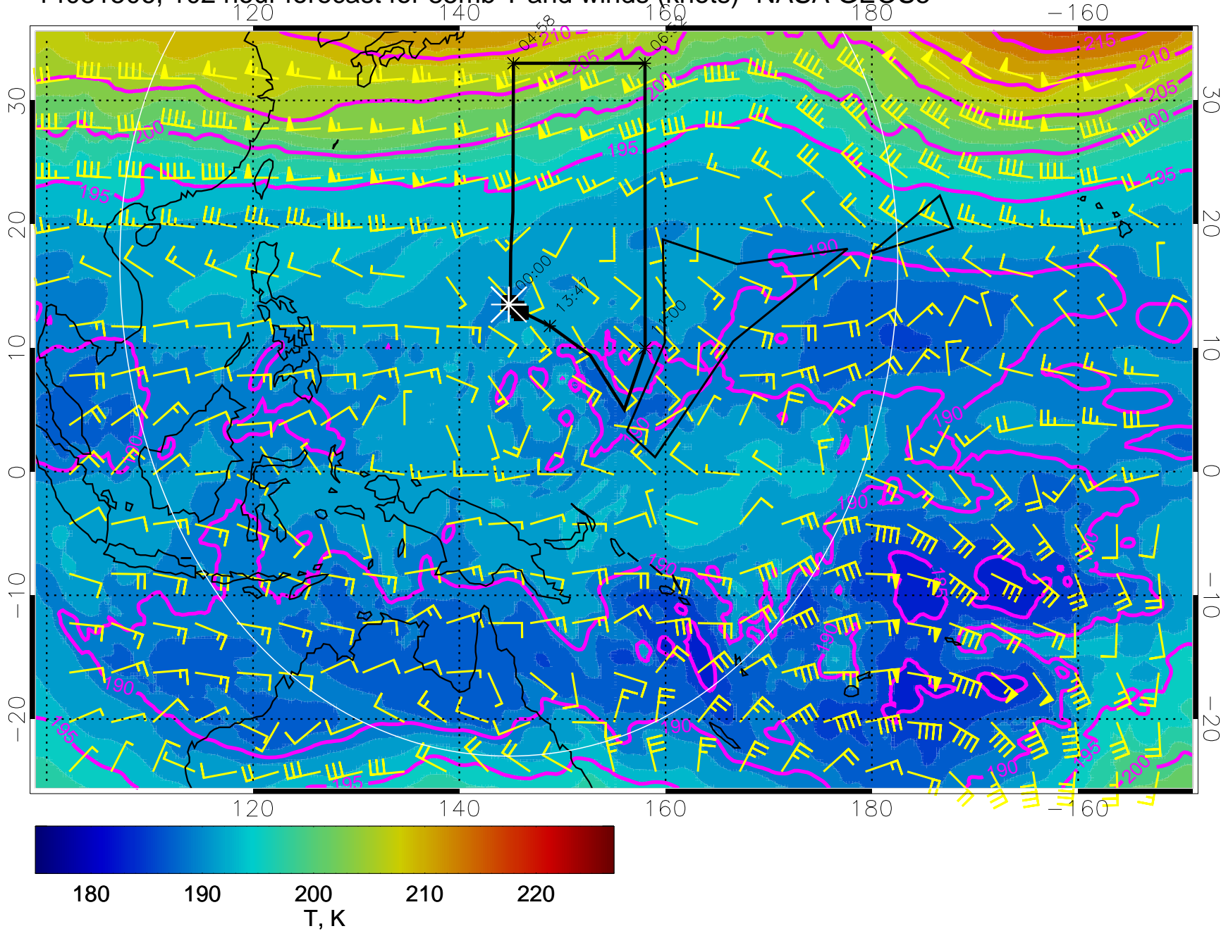
14031506, 102 hour forecast for 85mb T and winds (knots)- NASA GEOS5
