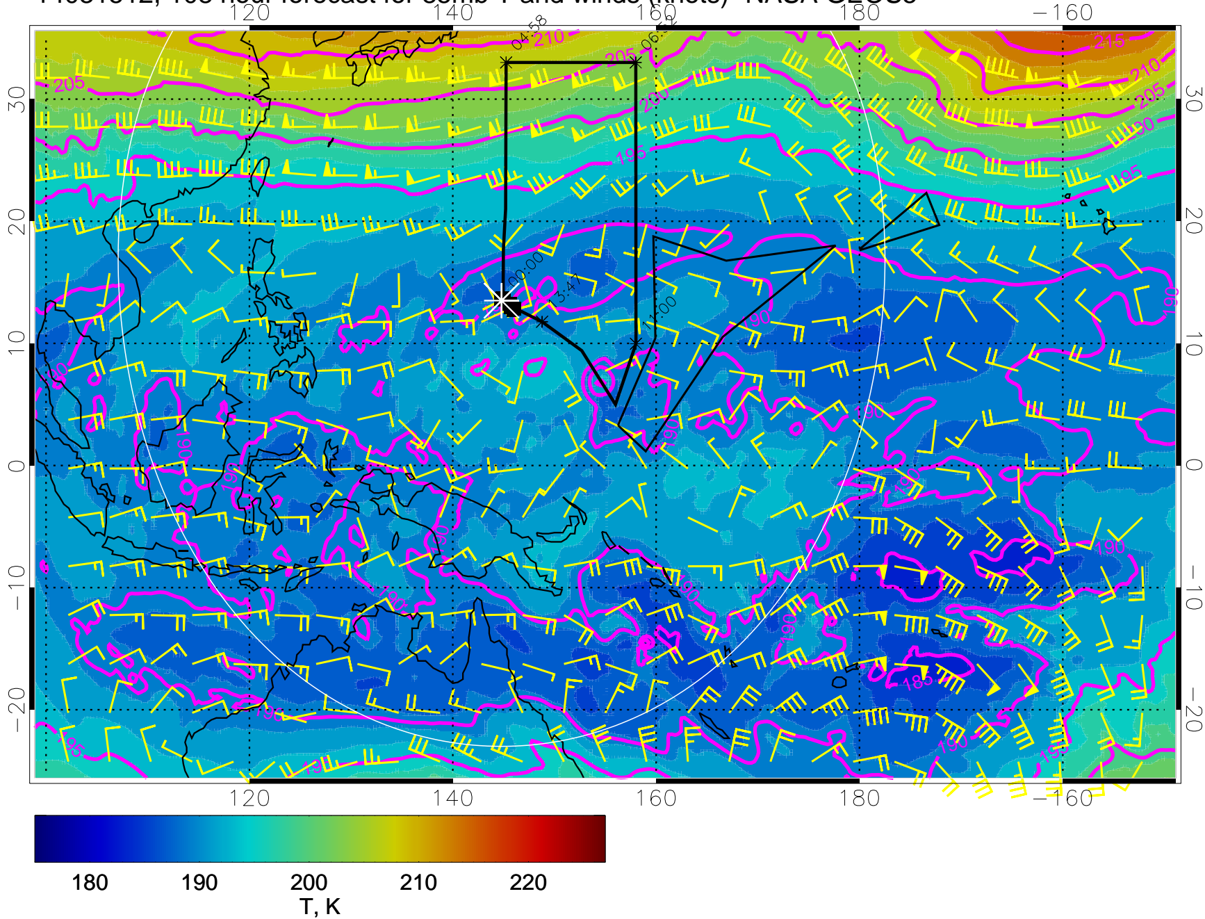
14031512, 108 hour forecast for 85mb T and winds (knots)- NASA GEOS5
