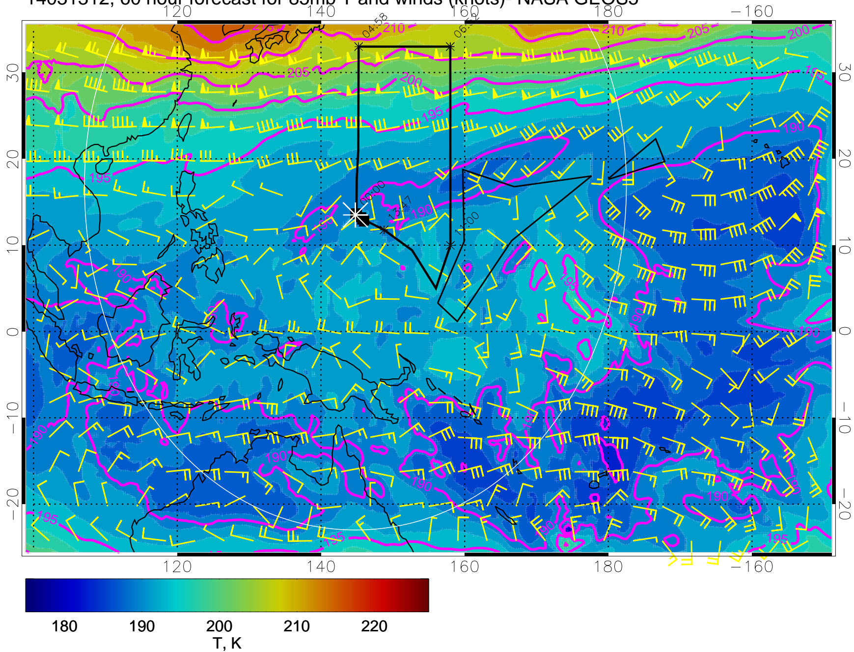
14031312, 60 hour forecast for 85mb T and winds (knots)- NASA GEOS5
