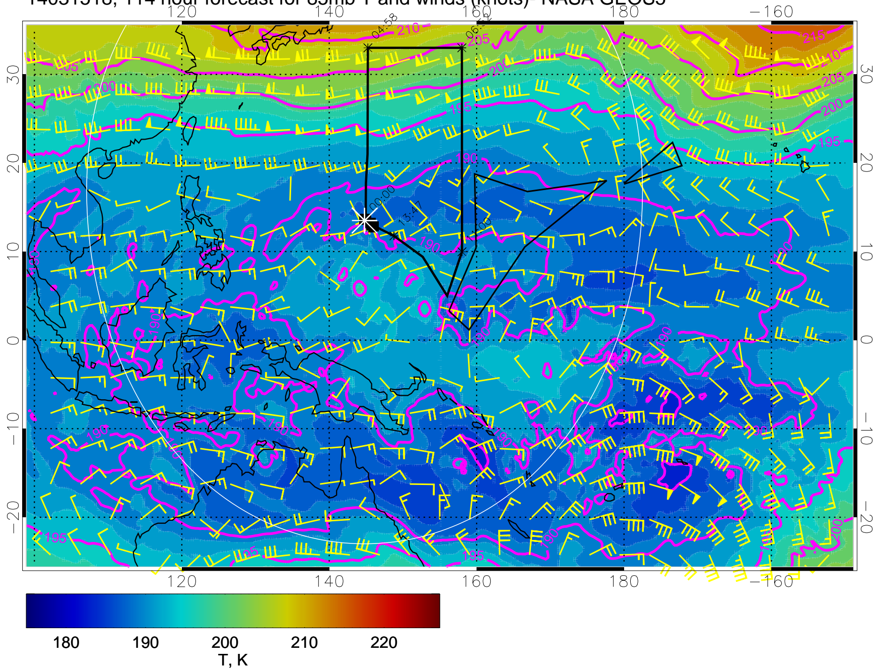
14031518, 114 hour forecast for 85mb T and winds (knots)- NASA GEOS5
