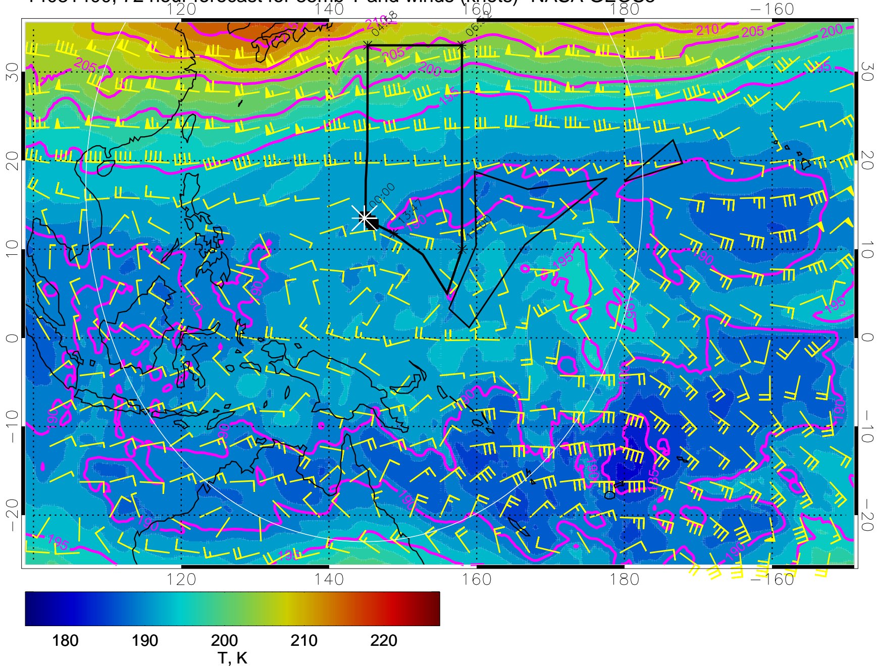
14031400, 72 hour forecast for 85mb T and winds (knots)- NASA GEOS5
