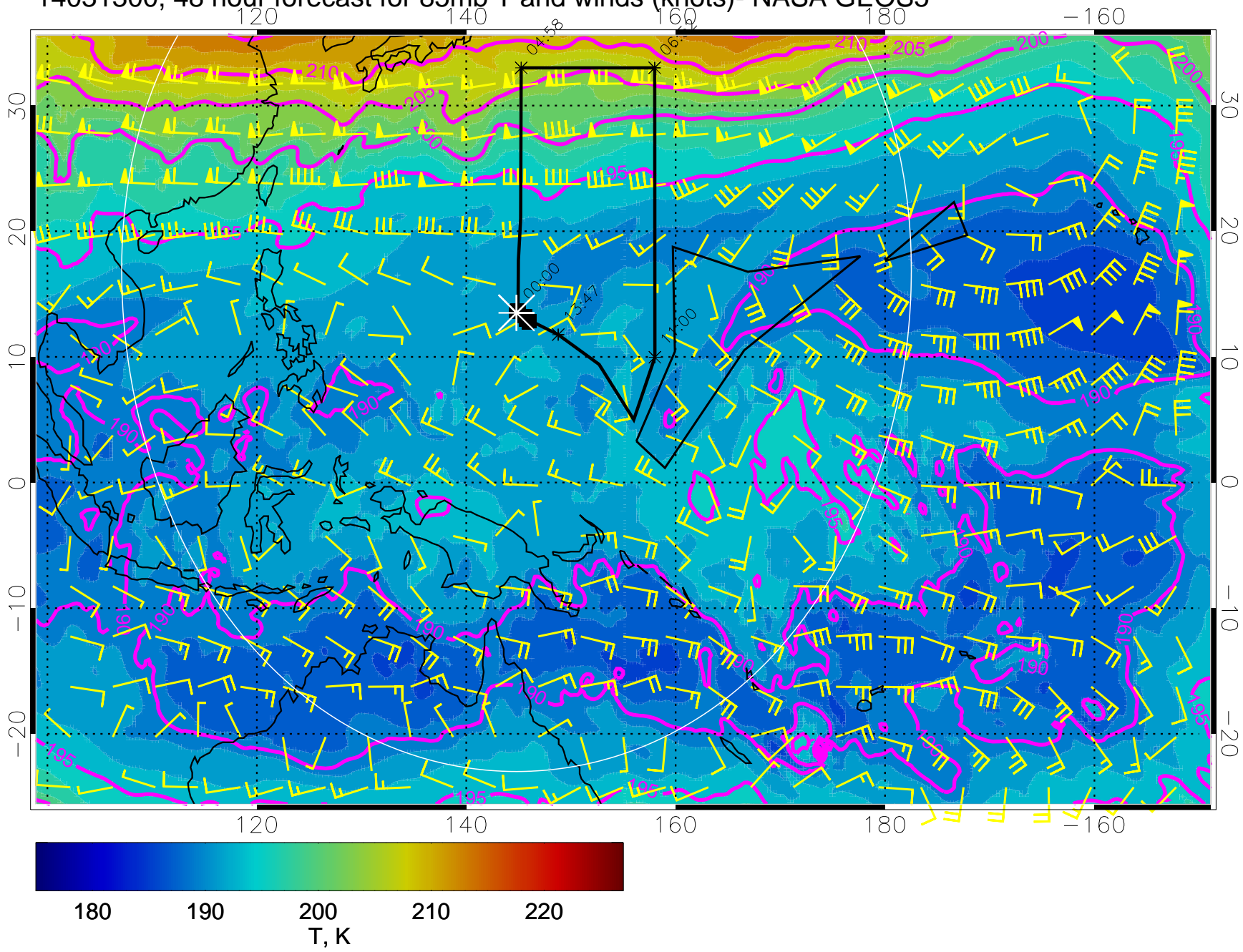
14031300, 48 hour forecast for 85mb T and winds (knots)- NASA GEOS5
