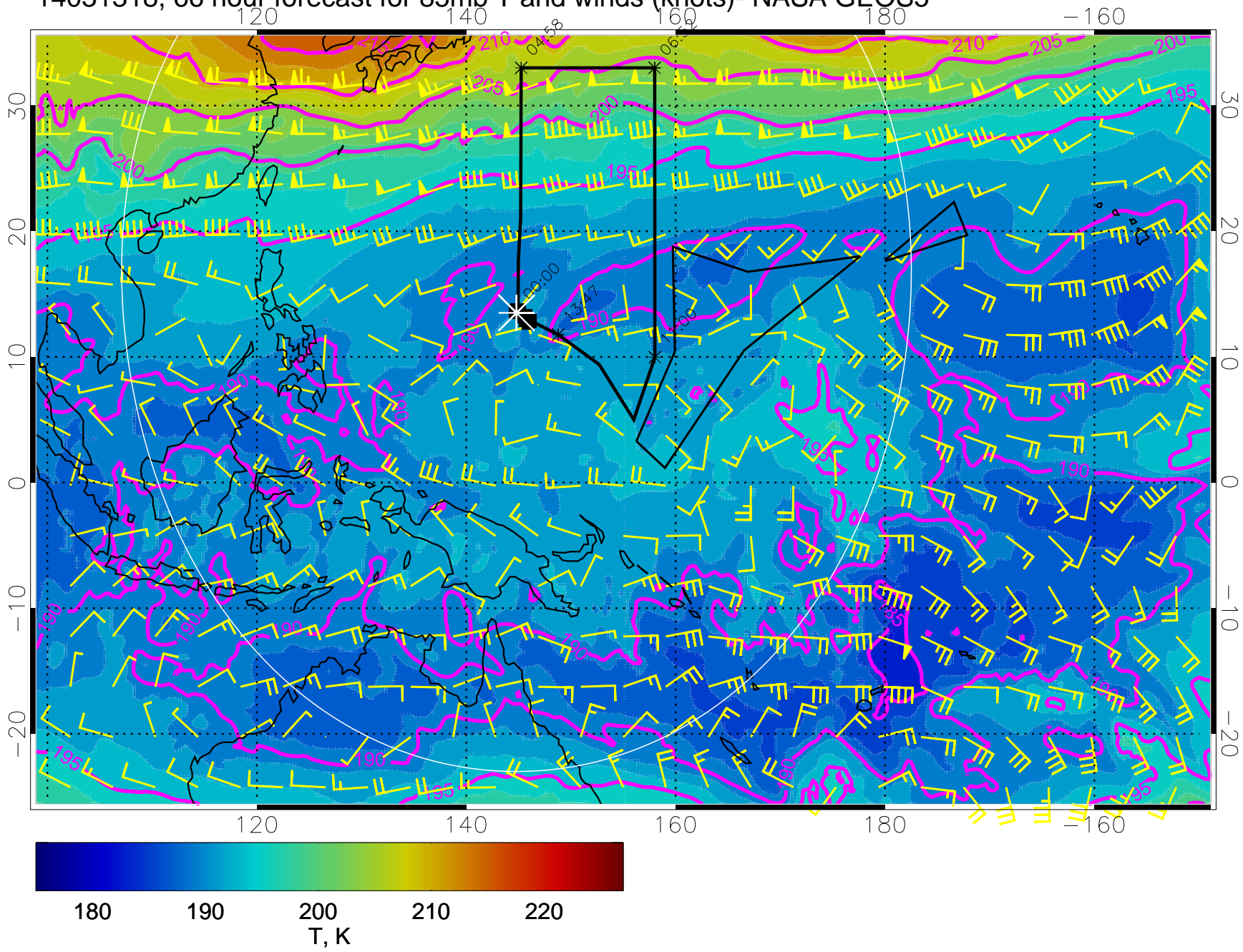
14031318, 66 hour forecast for 85mb T and winds (knots)- NASA GEOS5
