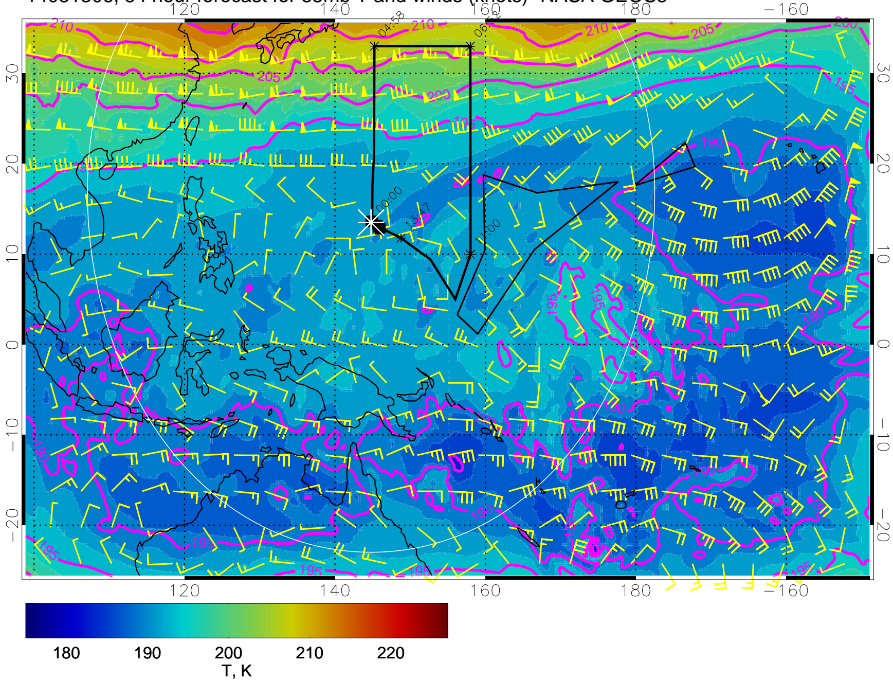
14031306, 54 hour forecast for 85mb T and winds (knots)- NASA GEOS5
