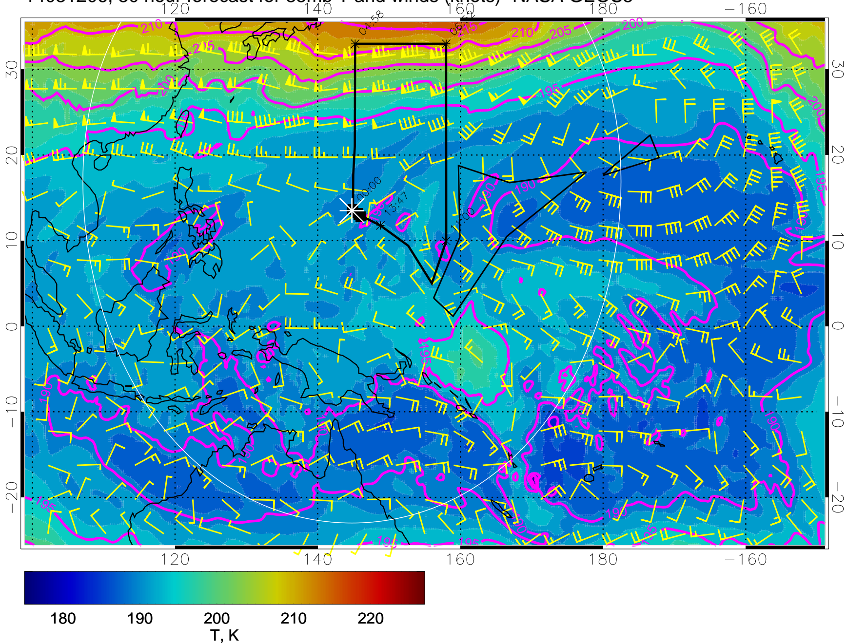
14031206, 30 hour forecast for 85mb T and winds (knots)- NASA GEOS5
