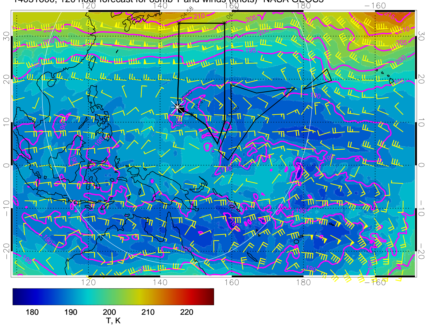
14031600, 120 hour forecast for 85mb T and winds (knots)- NASA GEOS5
