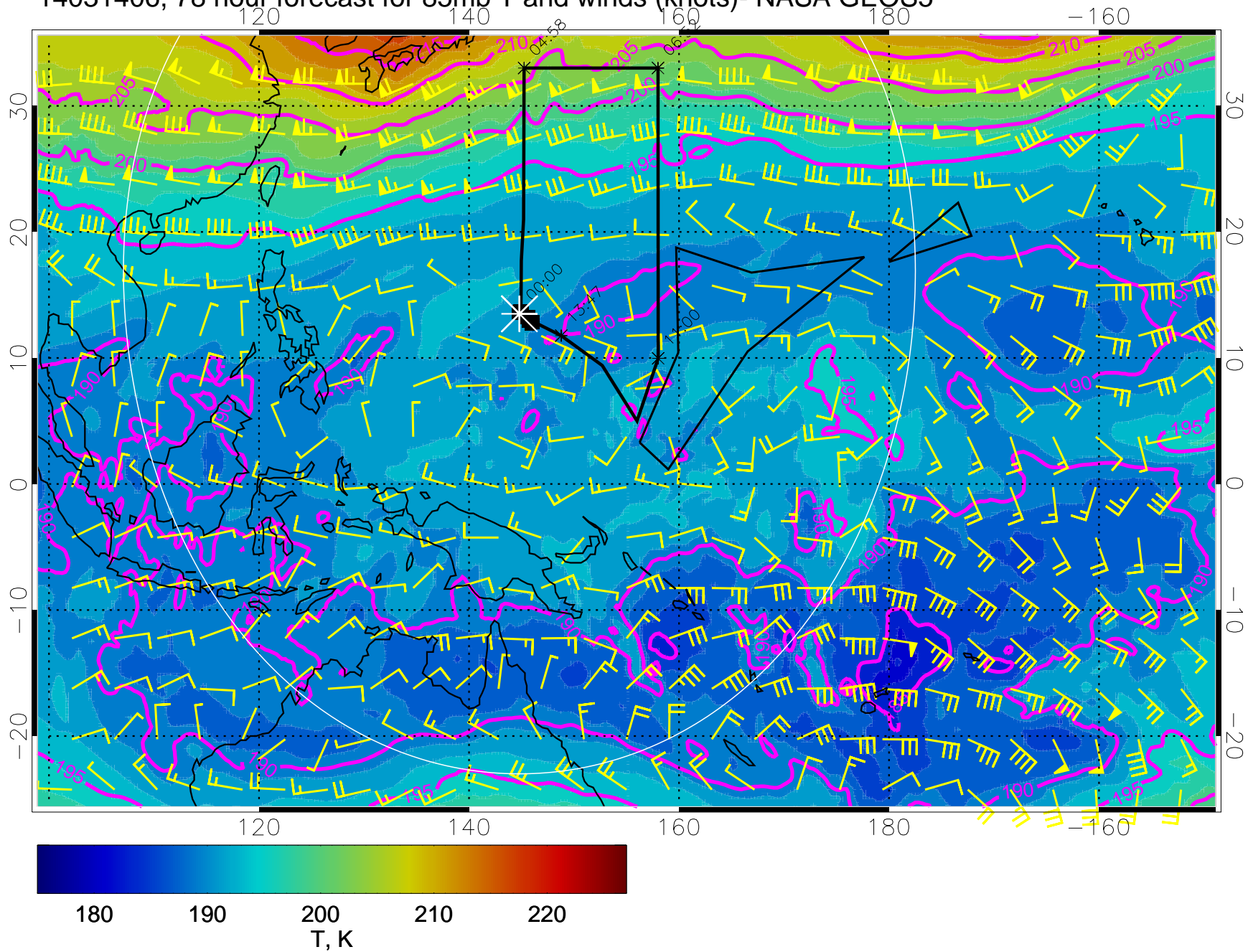
14031406, 78 hour forecast for 85mb T and winds (knots)- NASA GEOS5
