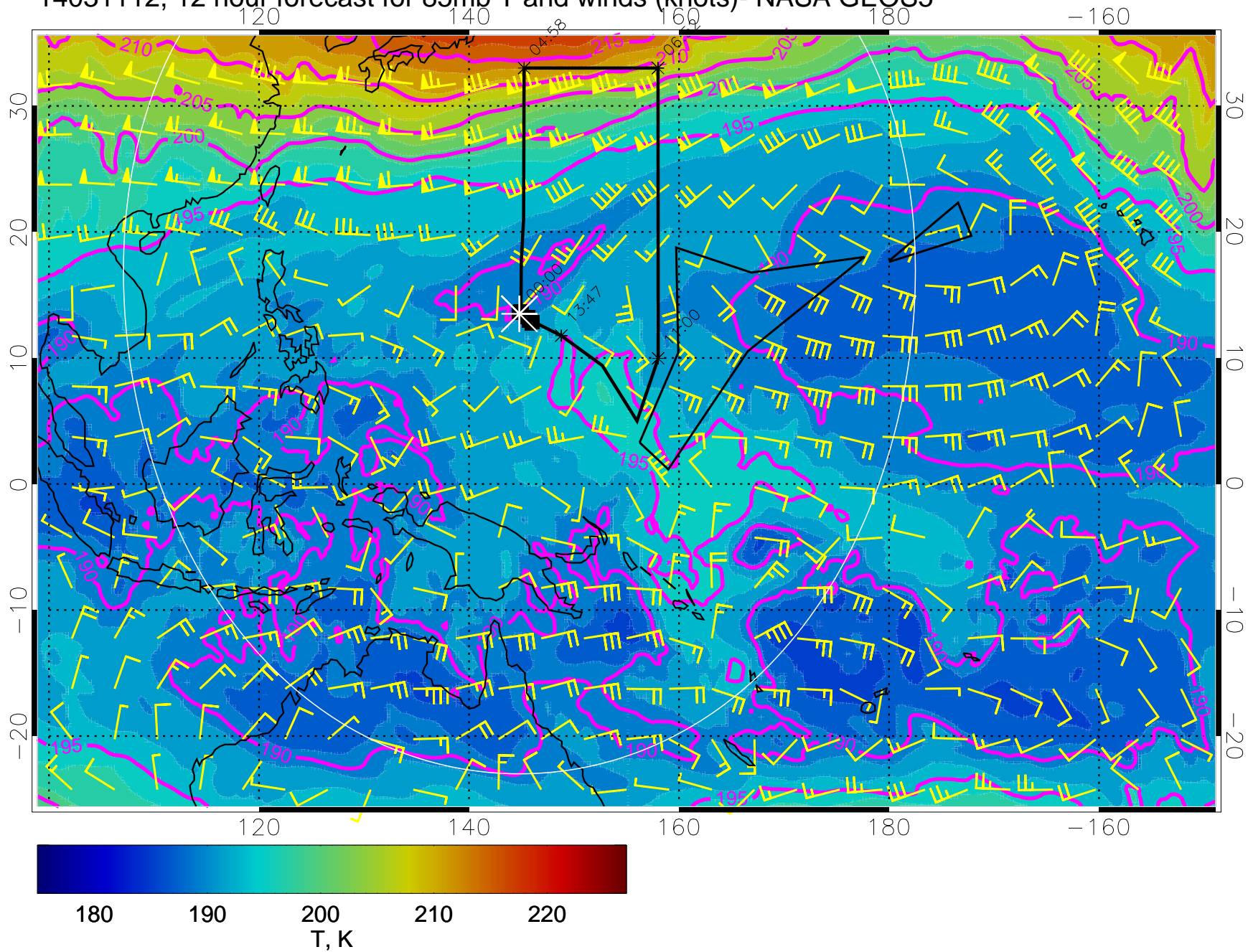
14031112, 12 hour forecast for 85mb T and winds (knots)- NASA GEOS5
