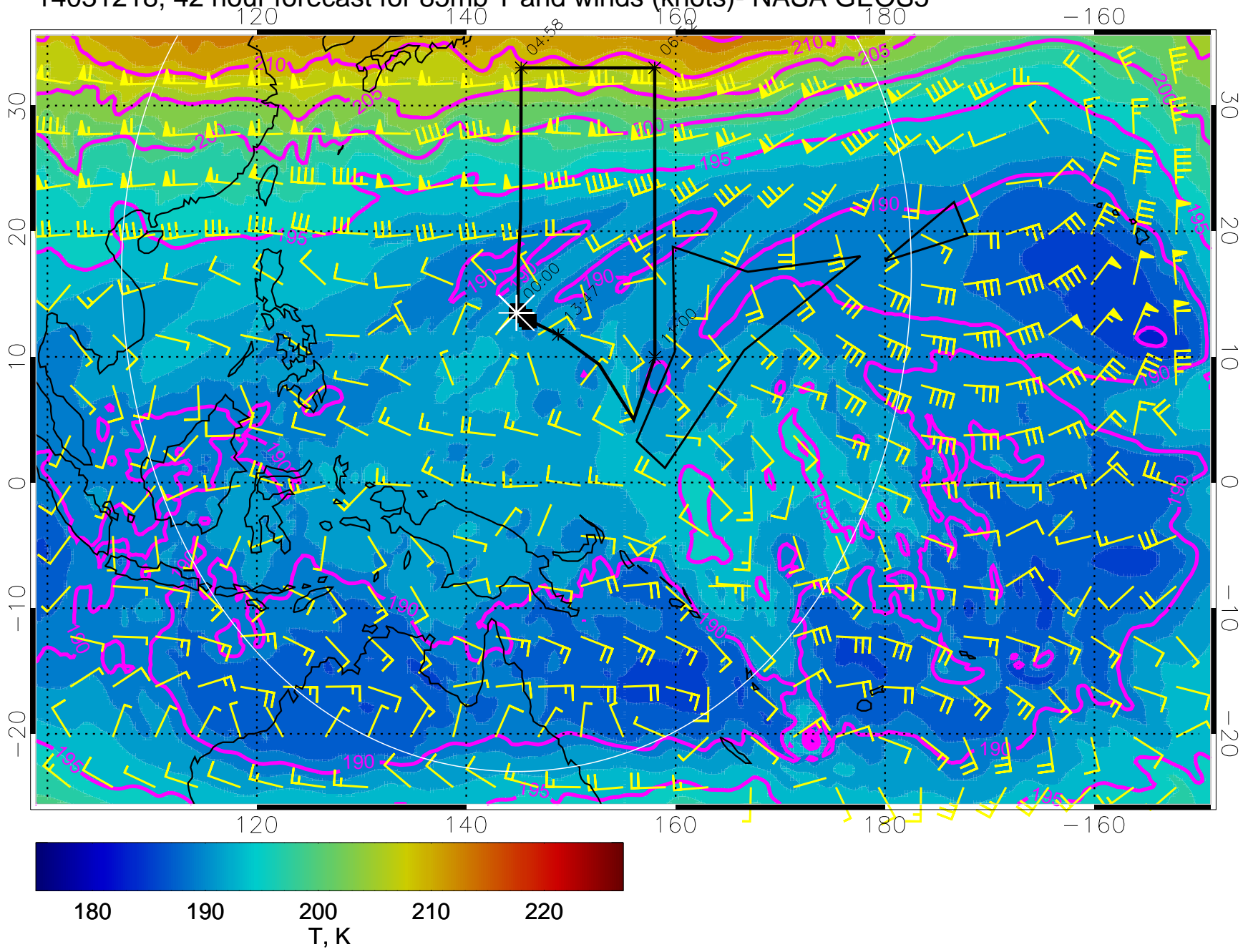
14031218, 42 hour forecast for 85mb T and winds (knots)- NASA GEOS5
