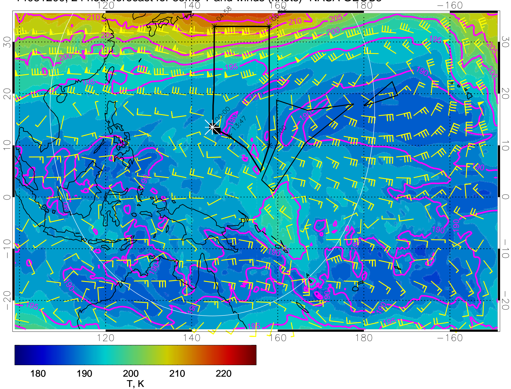
14031200, 24 hour forecast for 85mb T and winds (knots)- NASA GEOS5
