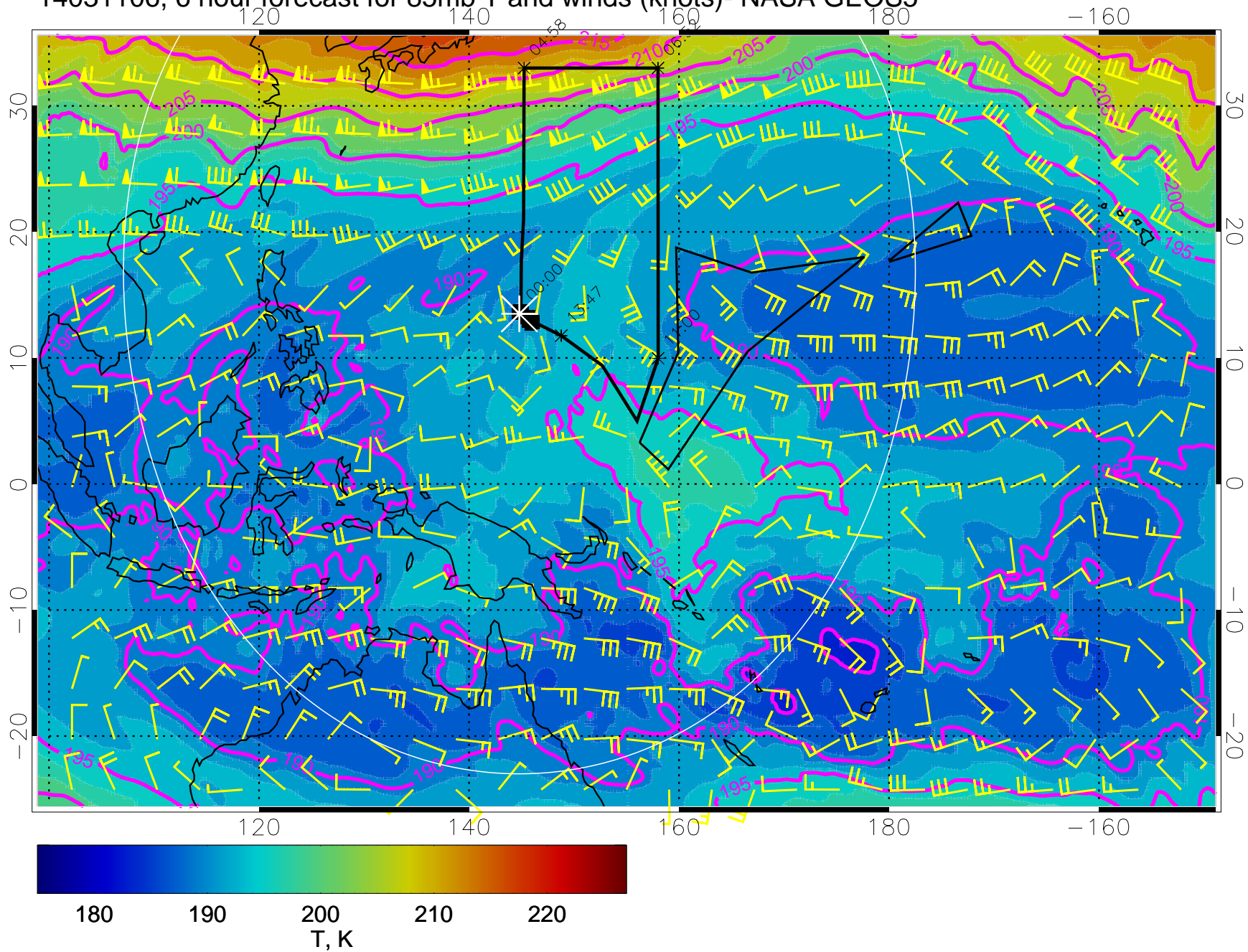
14031106, 6 hour forecast for 85mb T and winds (knots)- NASA GEOS5
