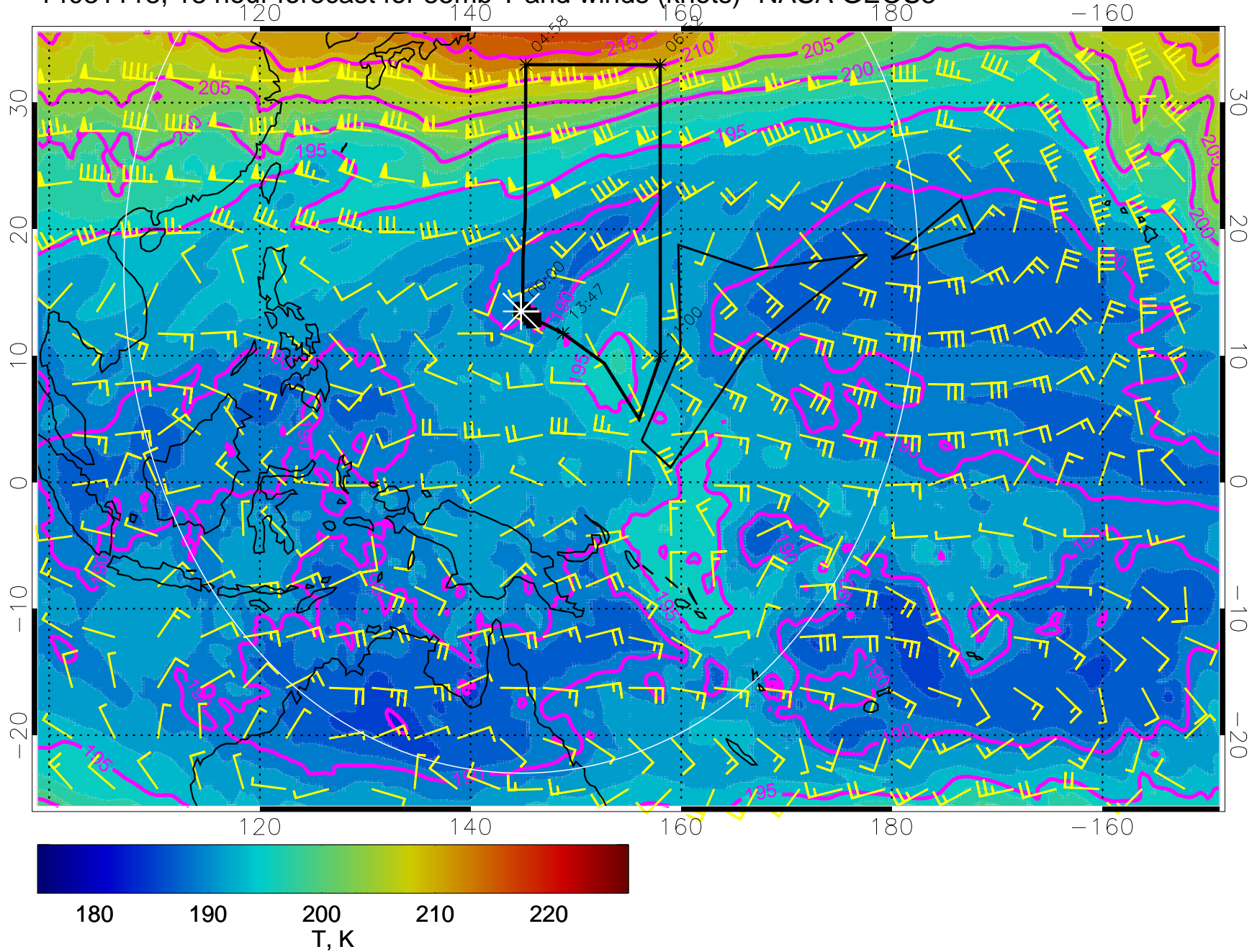
14031118, 18 hour forecast for 85mb T and winds (knots)- NASA GEOS5
