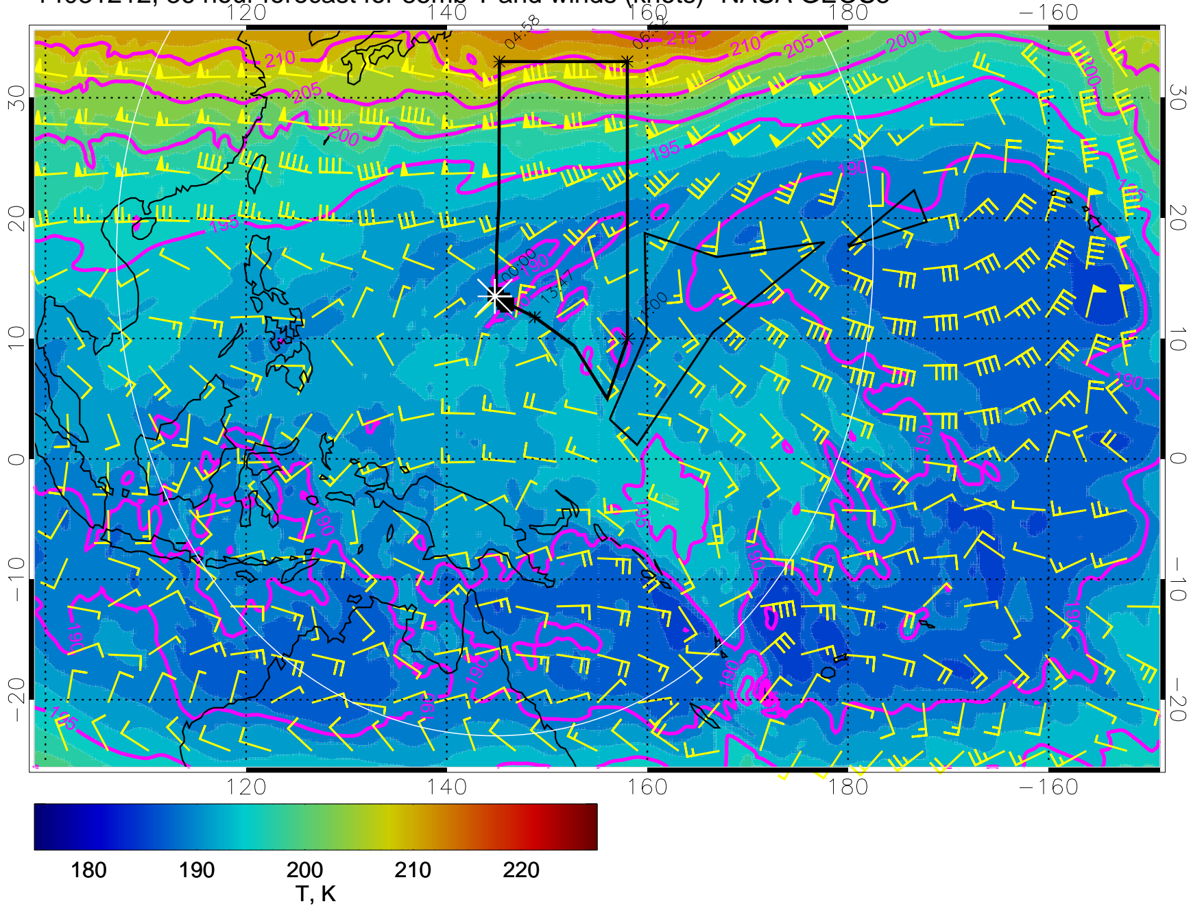
14031212, 36 hour forecast for 85mb T and winds (knots)- NASA GEOS5
