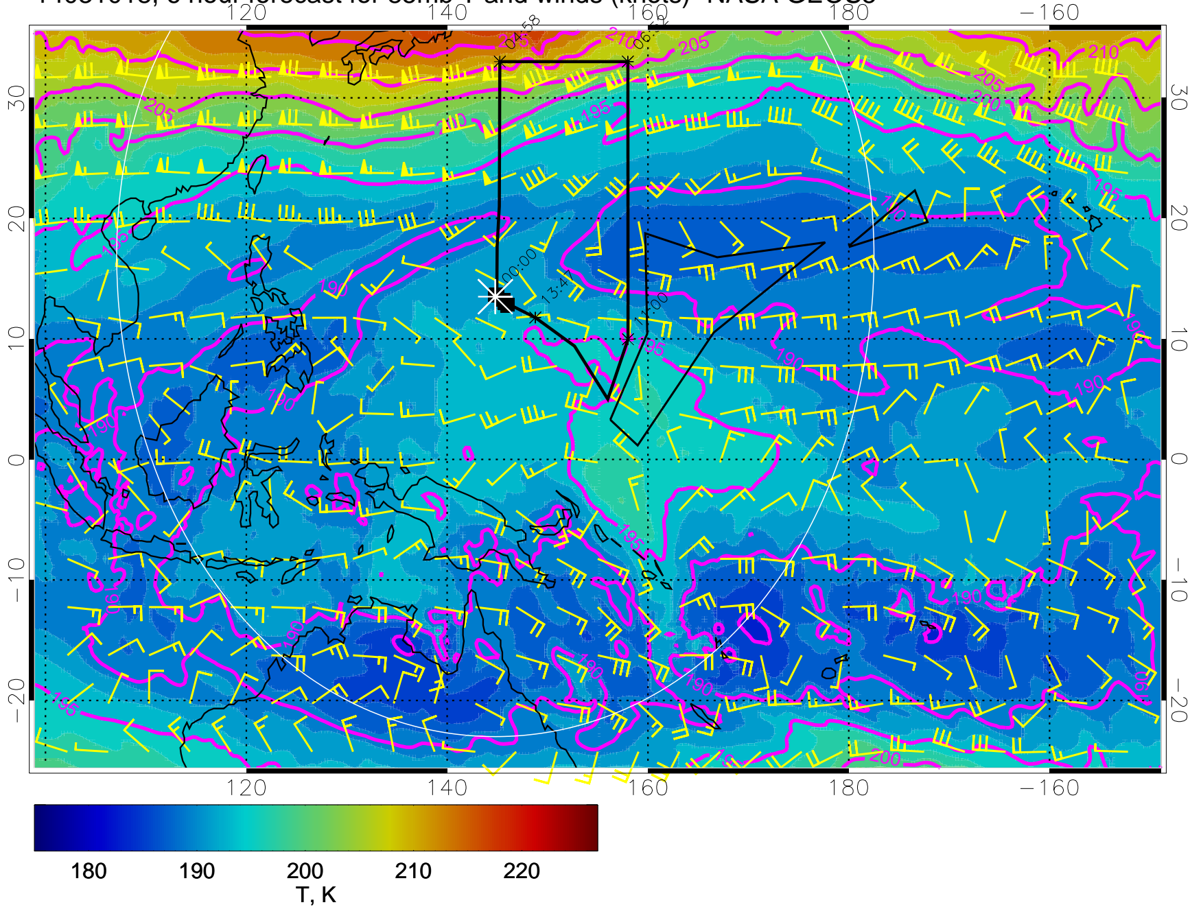
14031018, 6 hour forecast for 85mb T and winds (knots)- NASA GEOS5
