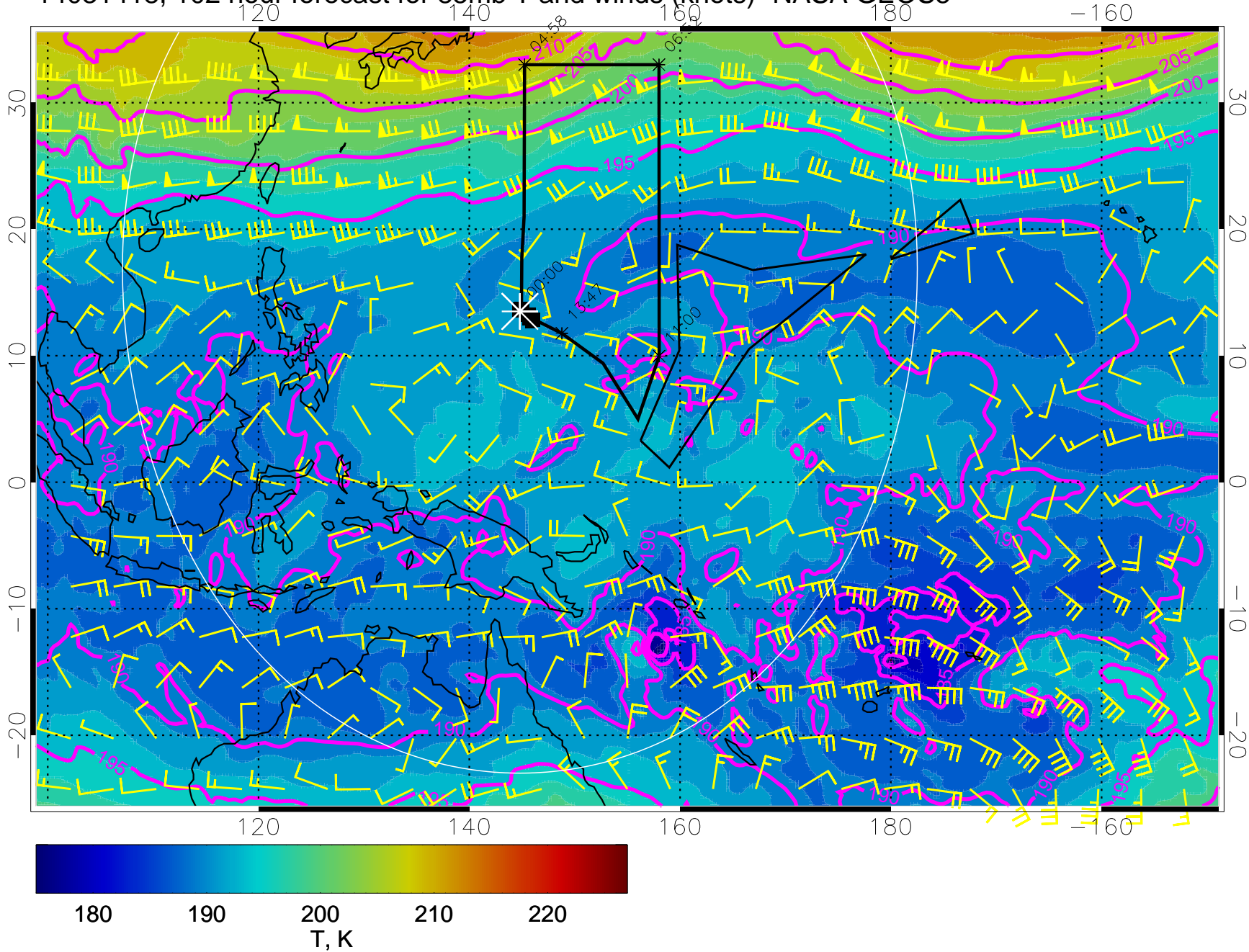
14031418, 102 hour forecast for 85mb T and winds (knots)- NASA GEOS5
