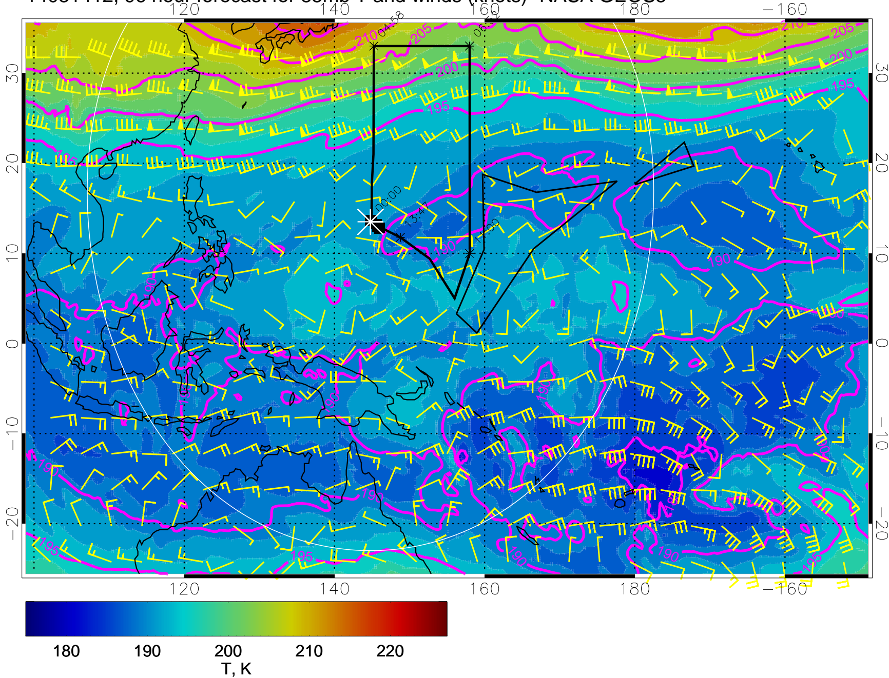
14031412, 96 hour forecast for 85mb T and winds (knots)- NASA GEOS5
