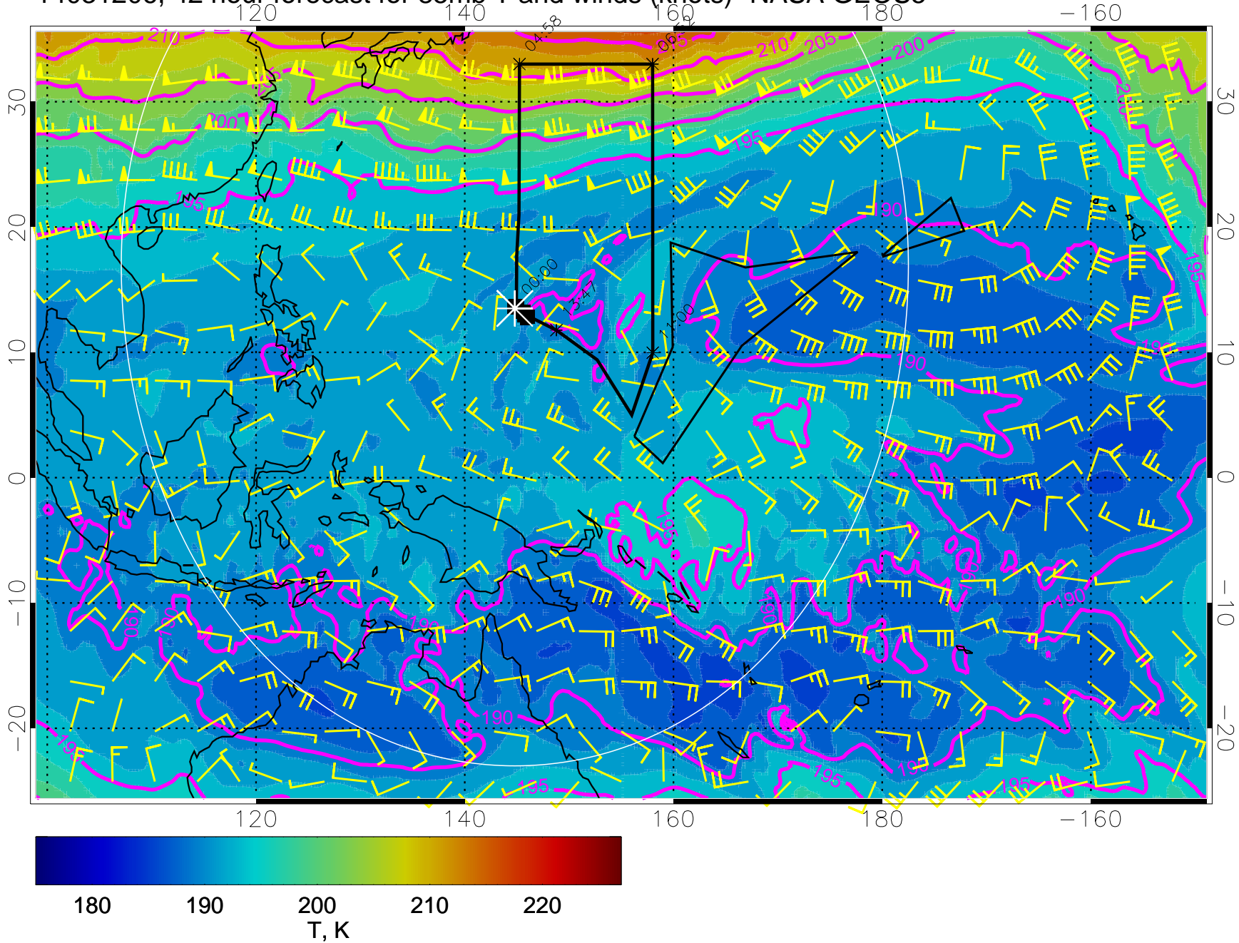
14031206, 42 hour forecast for 85mb T and winds (knots)- NASA GEOS5
