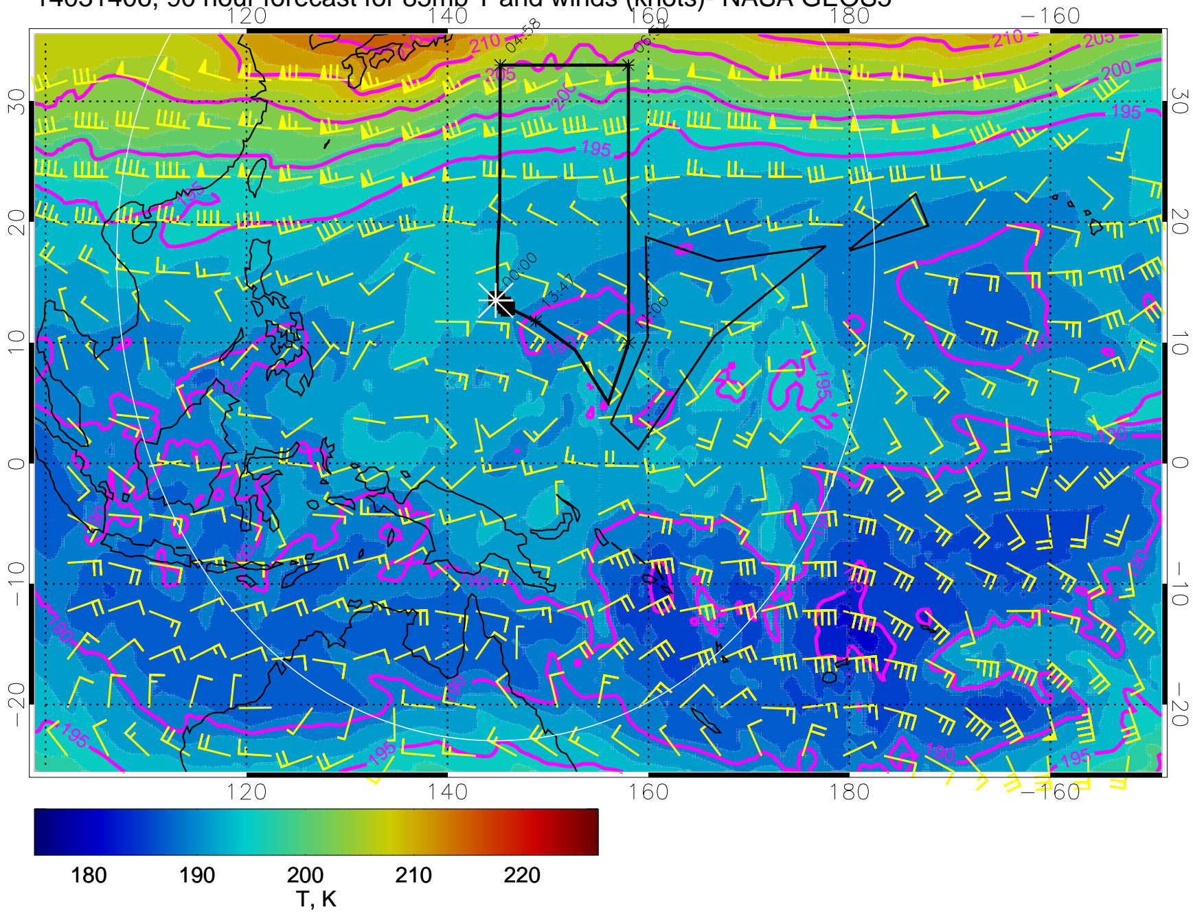
14031406, 90 hour forecast for 85mb T and winds (knots)- NASA GEOS5
