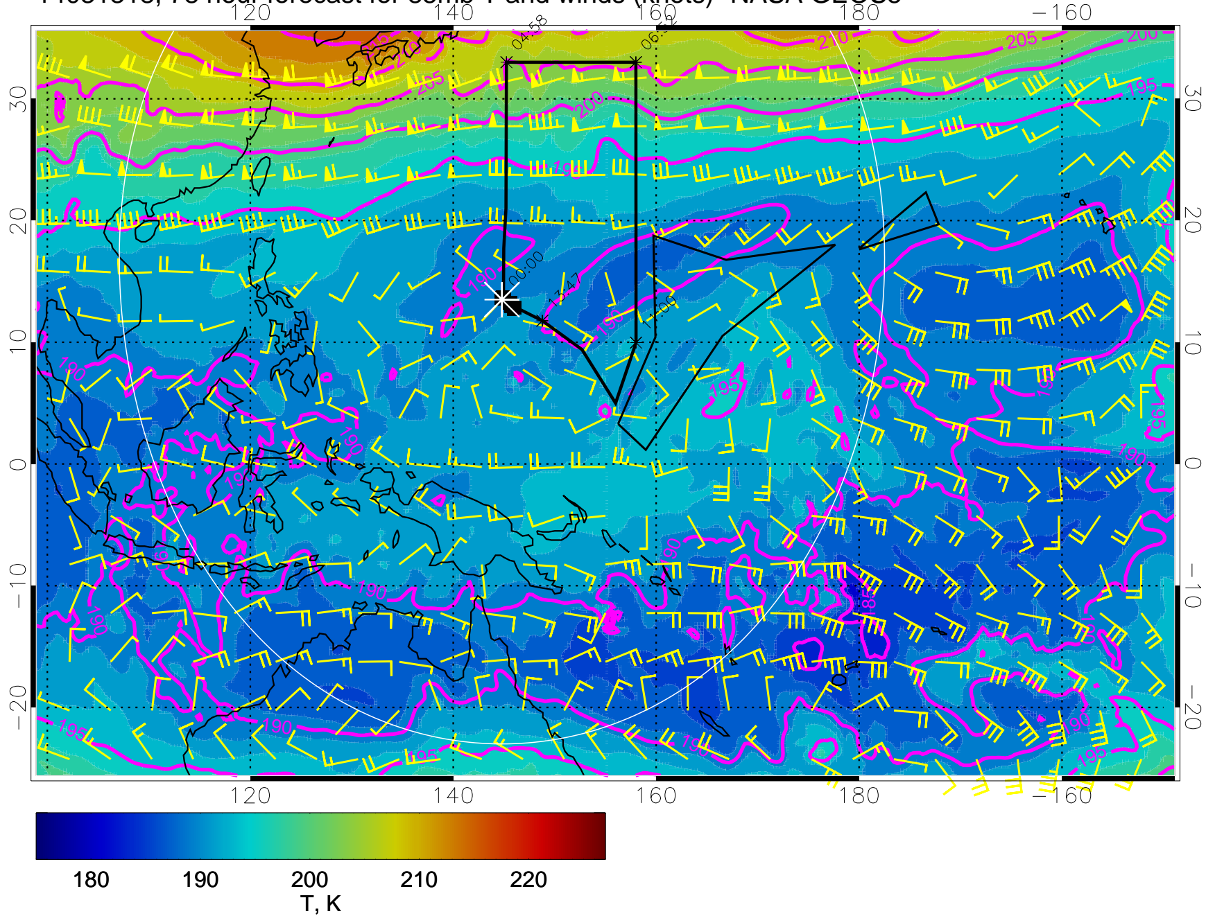
14031318, 78 hour forecast for 85mb T and winds (knots)- NASA GEOS5
