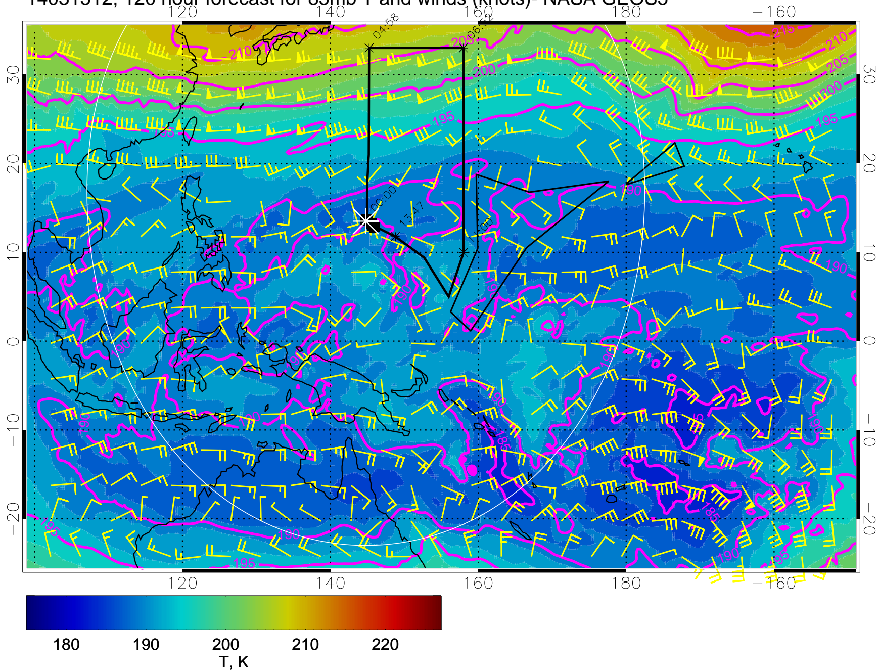
14031512, 120 hour forecast for 85mb T and winds (knots)- NASA GEOS5
