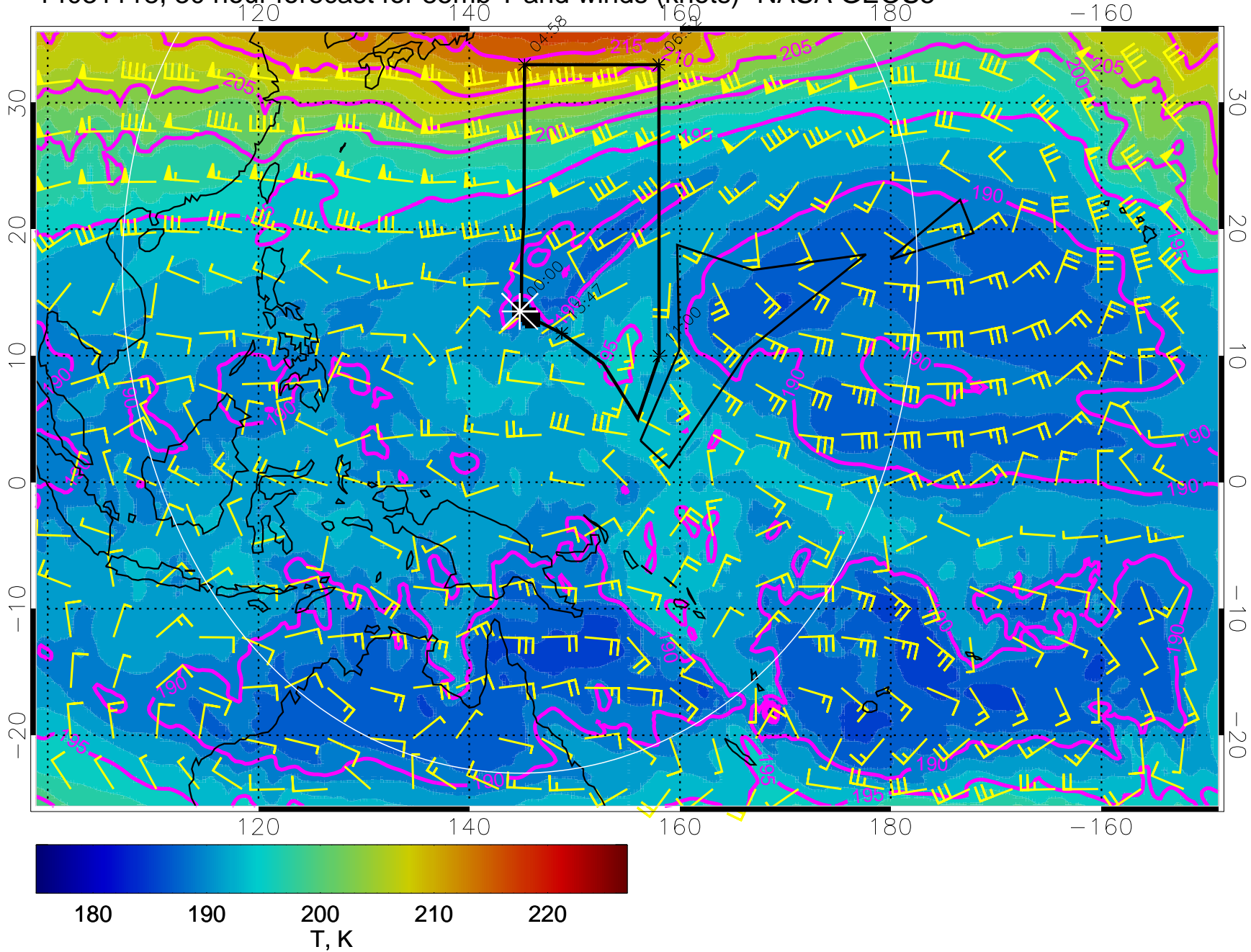
14031118, 30 hour forecast for 85mb T and winds (knots)- NASA GEOS5
