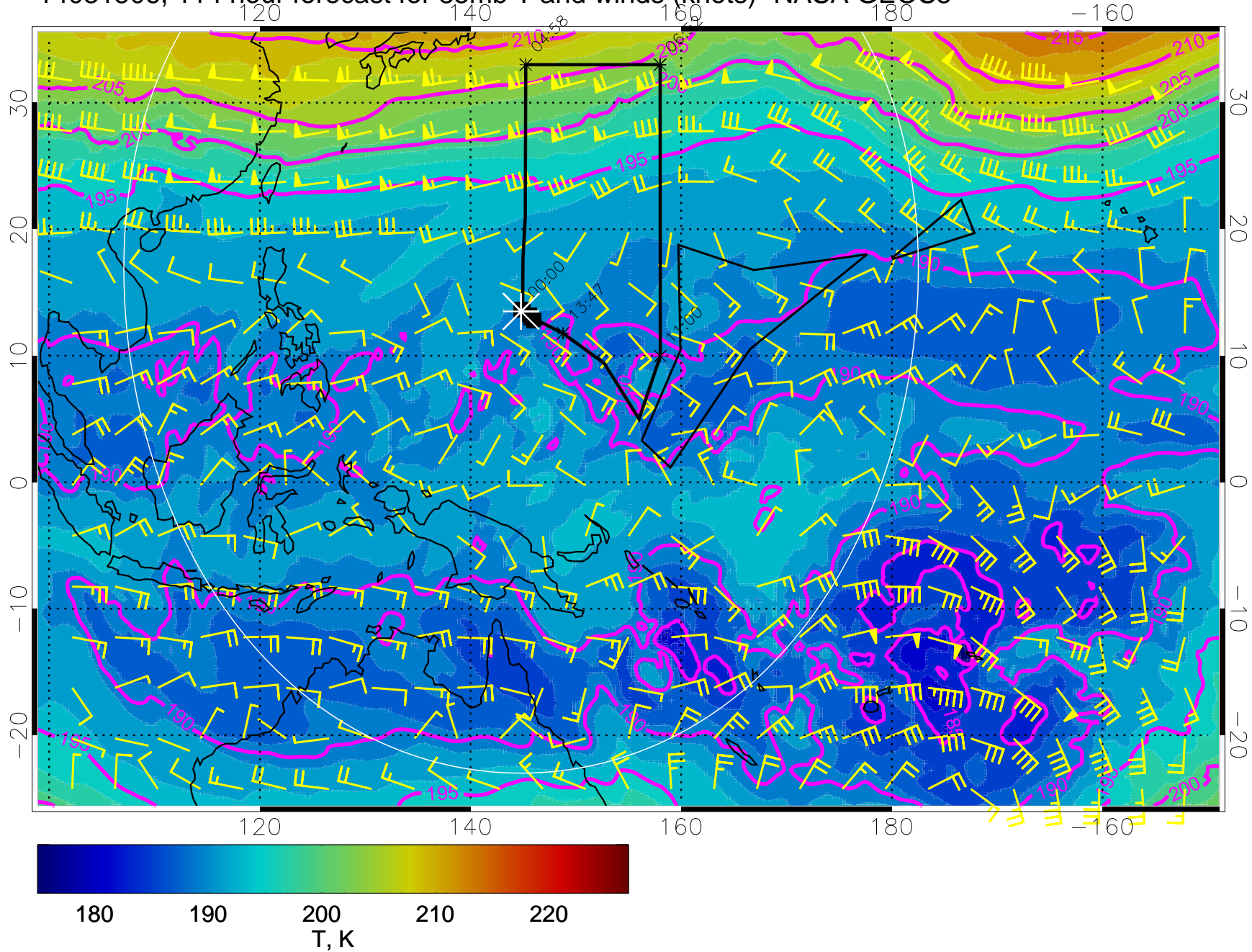
14031506, 114 hour forecast for 85mb T and winds (knots)- NASA GEOS5
