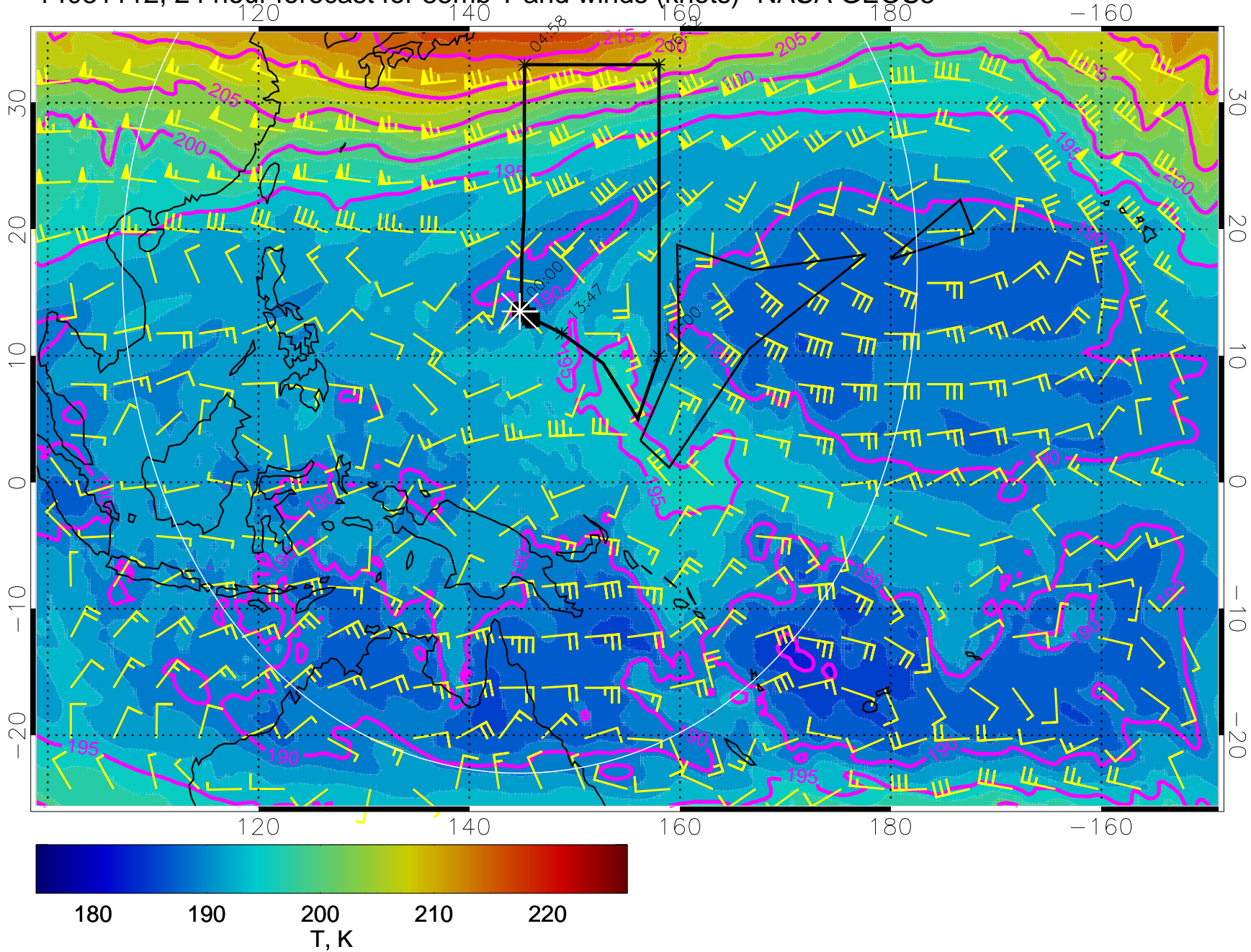
14031112, 24 hour forecast for 85mb T and winds (knots)- NASA GEOS5
