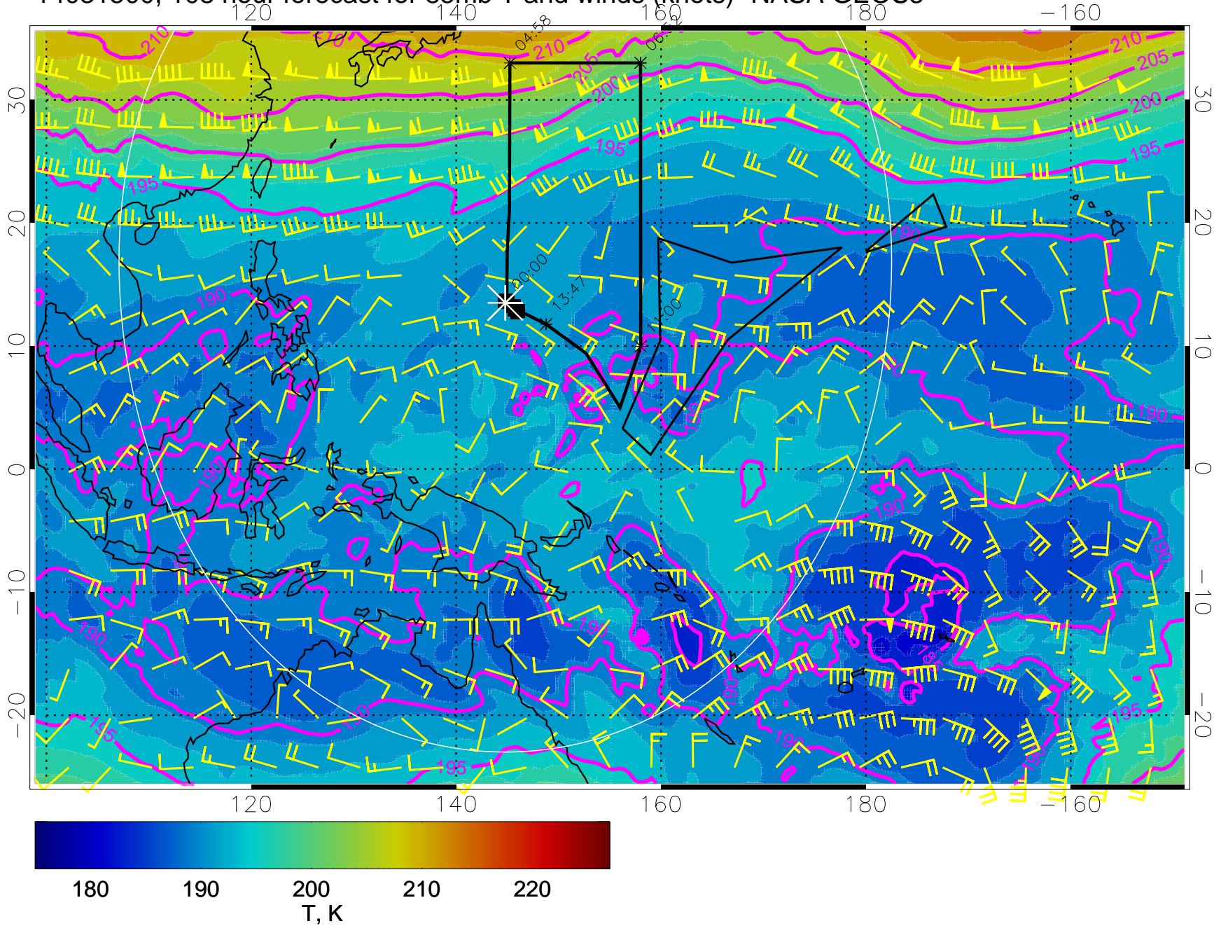
14031500, 108 hour forecast for 85mb T and winds (knots)- NASA GEOS5
