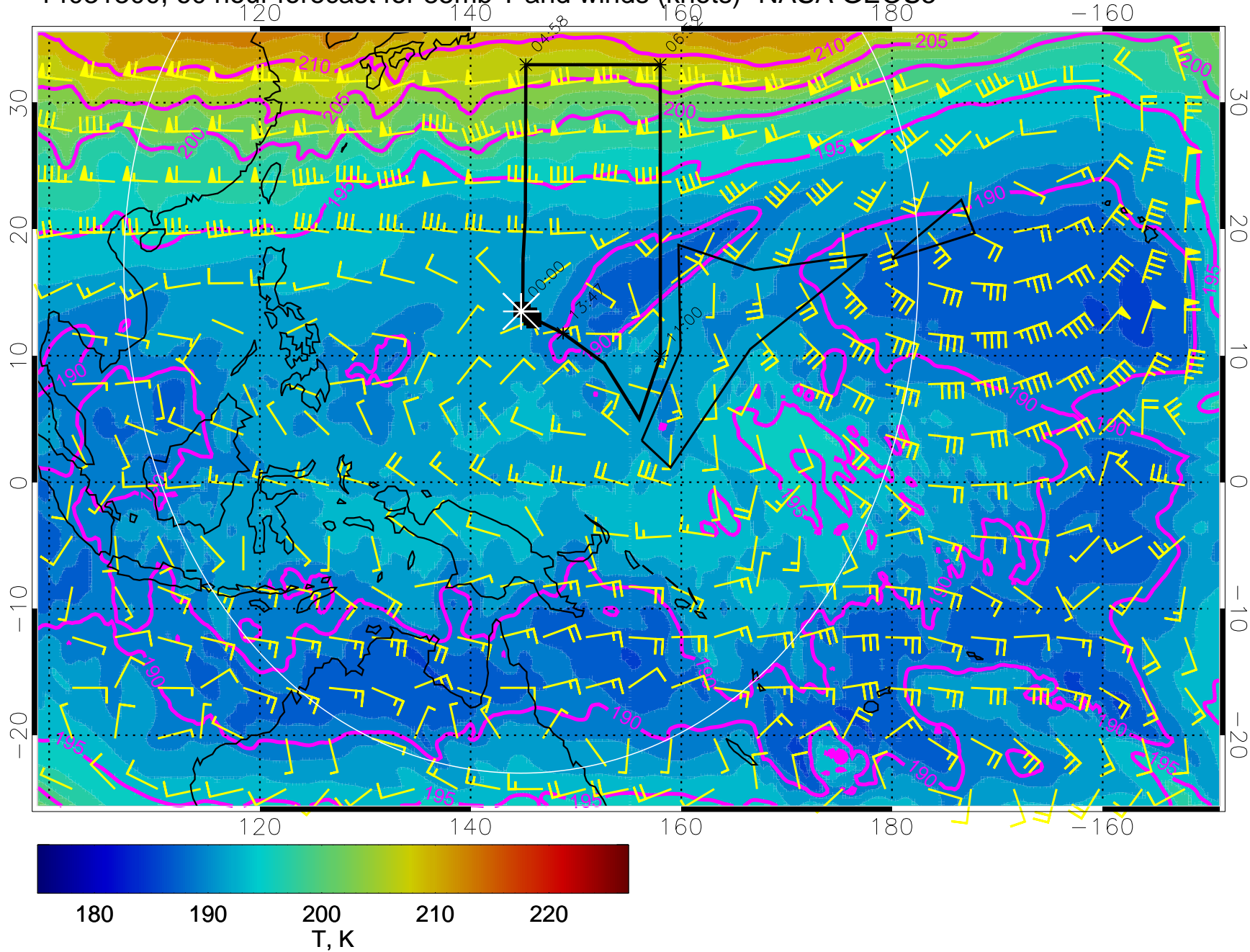
14031300, 60 hour forecast for 85mb T and winds (knots)- NASA GEOS5
