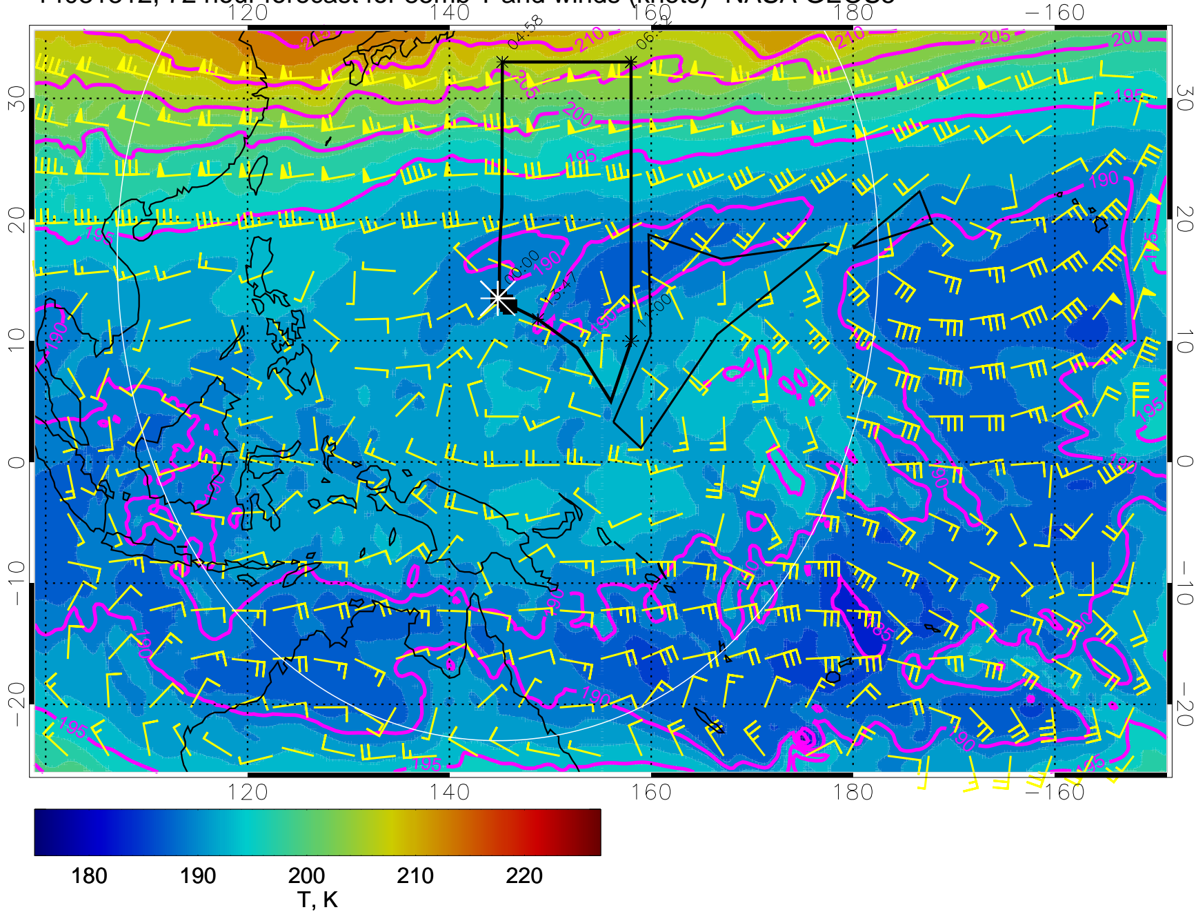
14031312, 72 hour forecast for 85mb T and winds (knots)- NASA GEOS5
