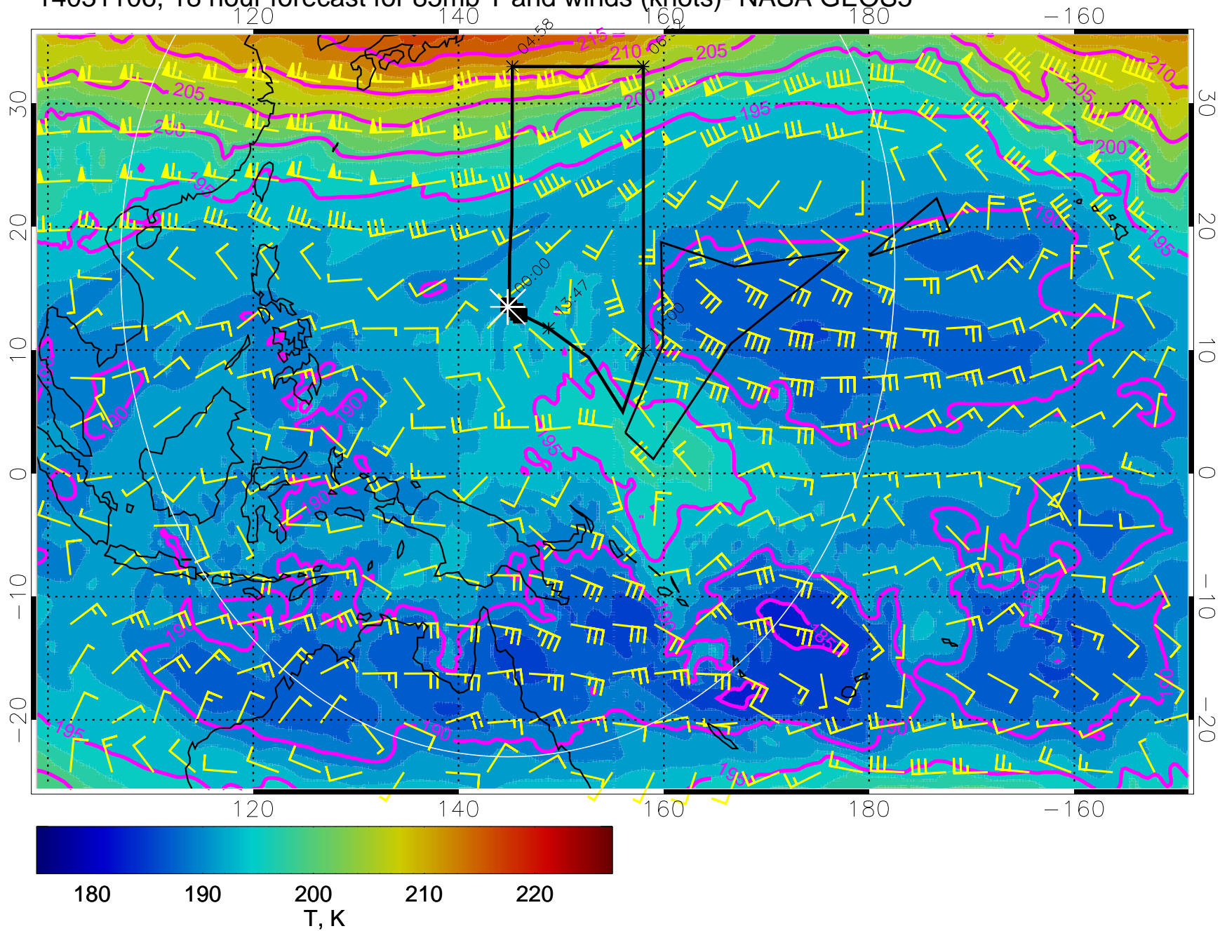
14031106, 18 hour forecast for 85mb T and winds (knots)- NASA GEOS5
