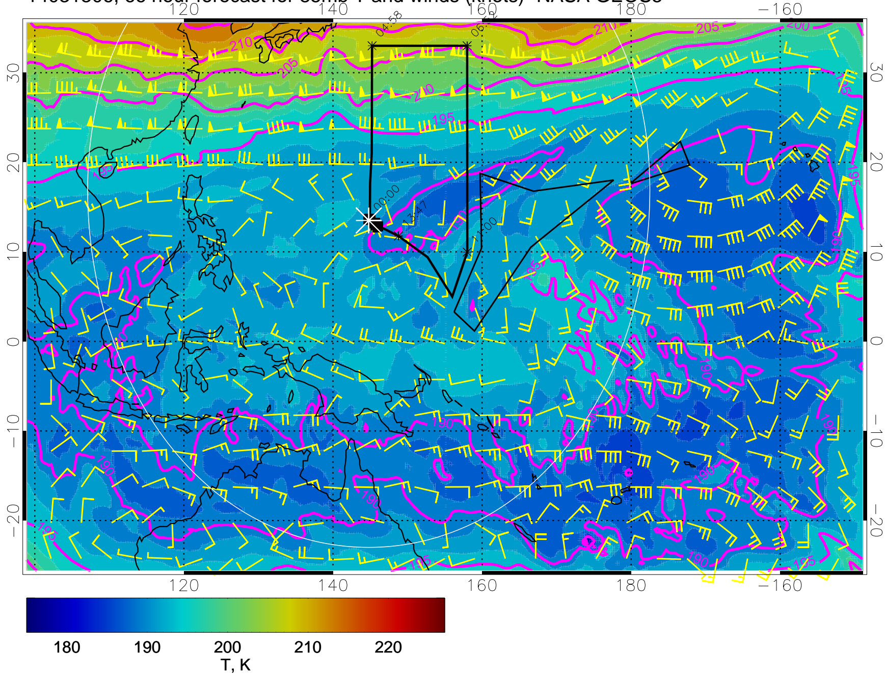
14031306, 66 hour forecast for 85mb T and winds (knots)- NASA GEOS5
