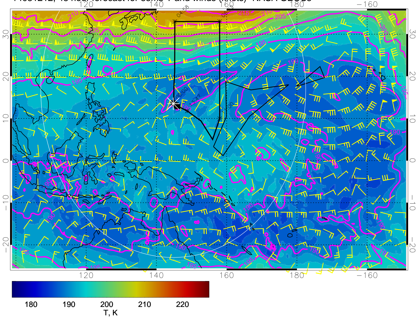
14031212, 48 hour forecast for 85mb T and winds (knots)- NASA GEOS5
