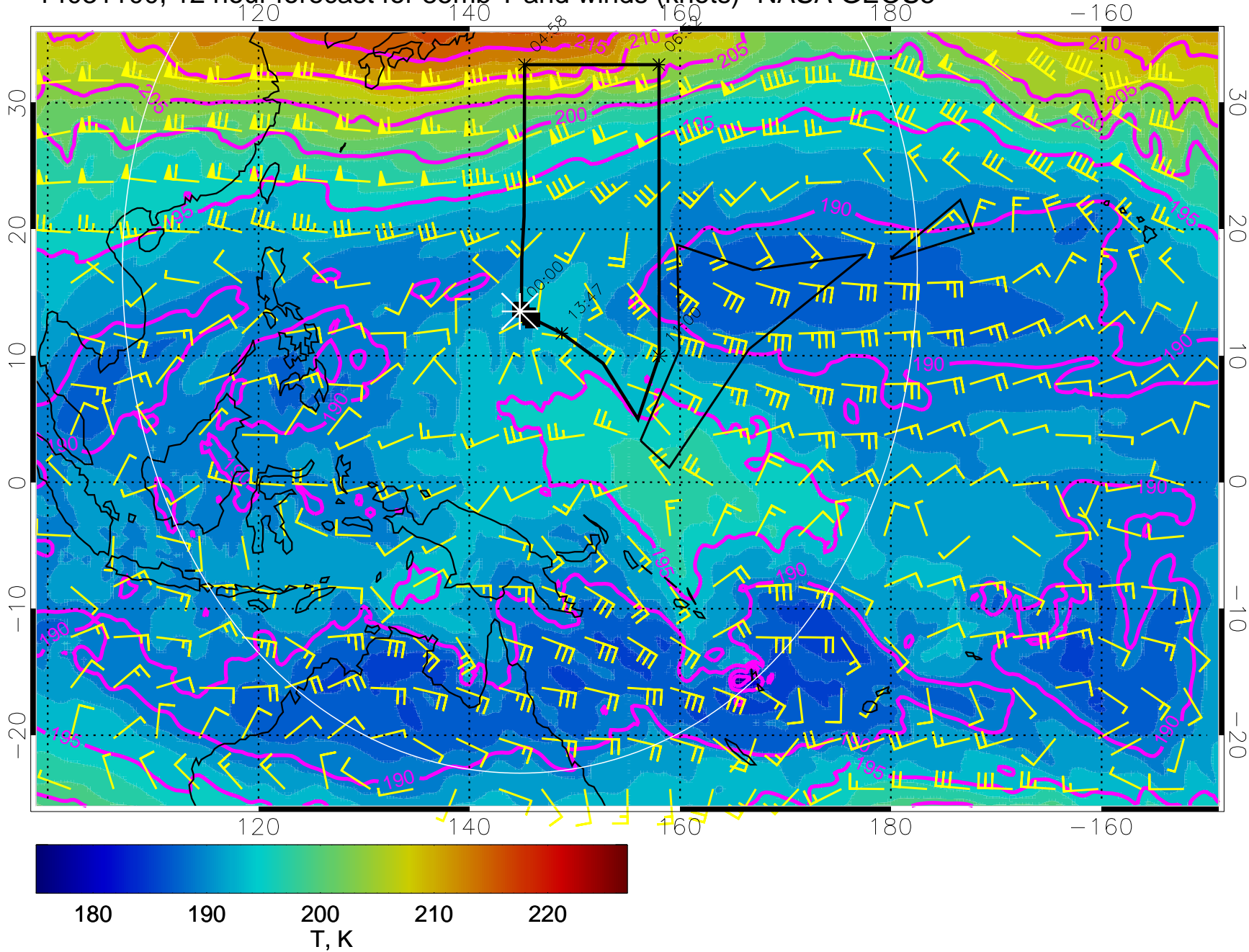
14031100, 12 hour forecast for 85mb T and winds (knots)- NASA GEOS5
