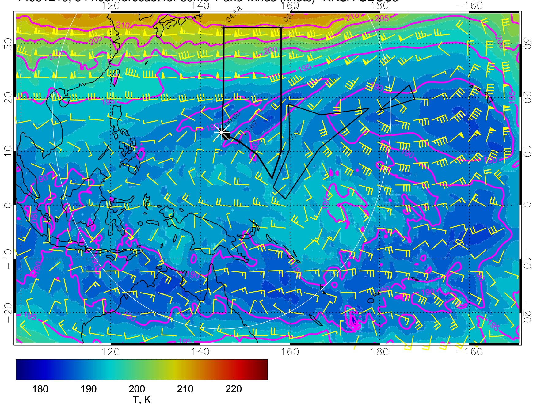
14031218, 54 hour forecast for 85mb T and winds (knots)- NASA GEOS5
