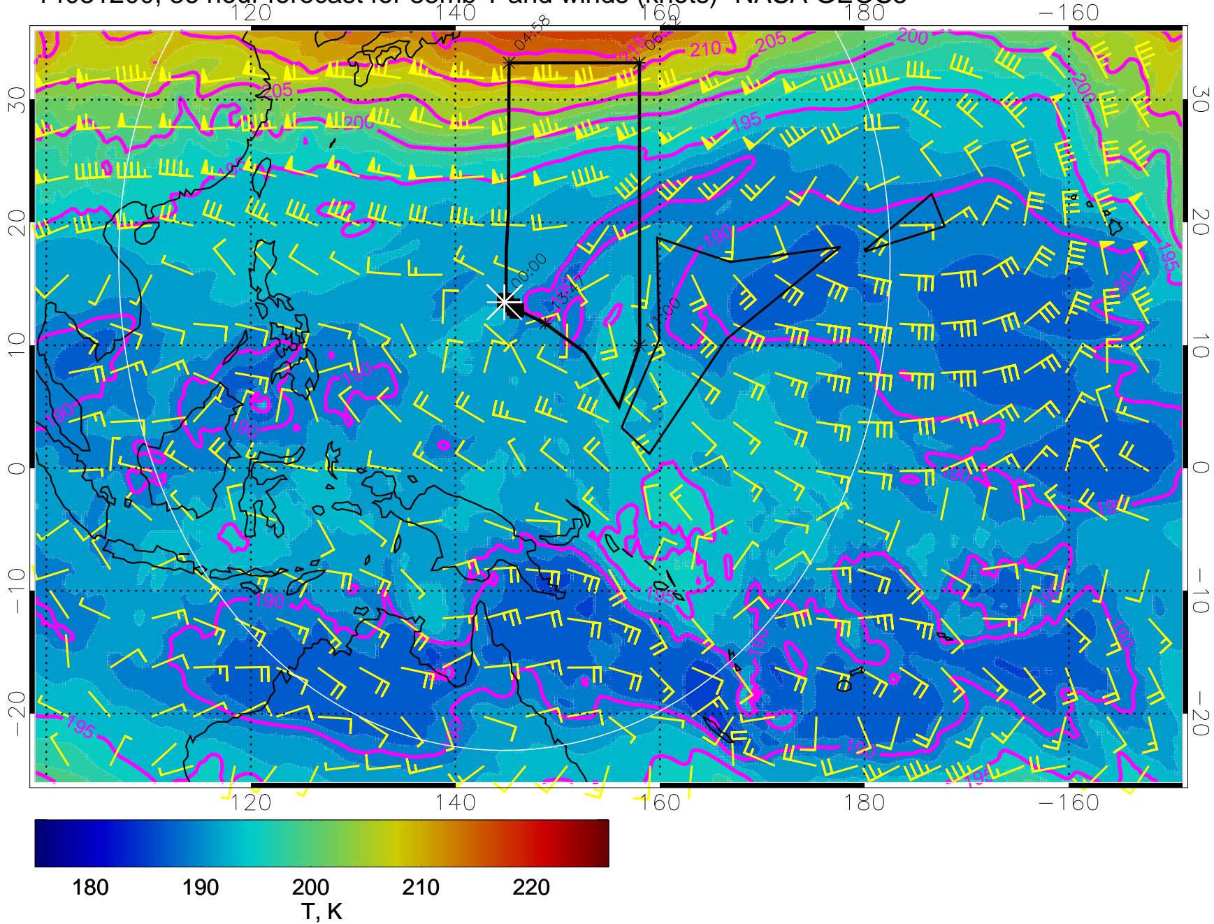
14031200, 36 hour forecast for 85mb T and winds (knots)- NASA GEOS5
