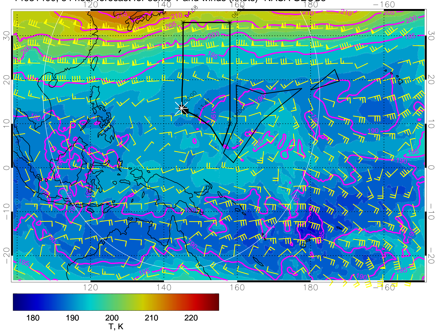
14031400, 84 hour forecast for 85mb T and winds (knots)- NASA GEOS5
