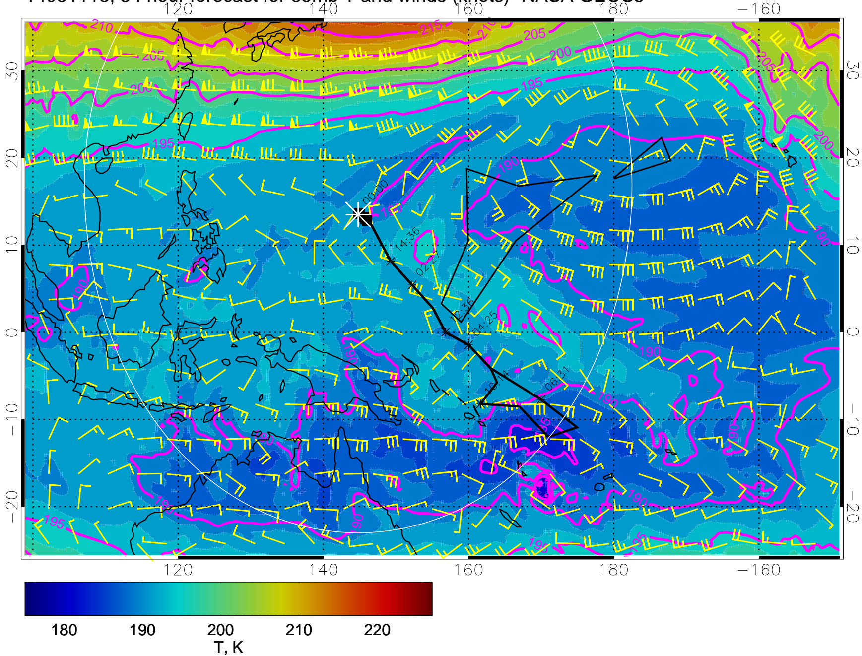
14031118, 54 hour forecast for 85mb T and winds (knots)- NASA GEOS5
