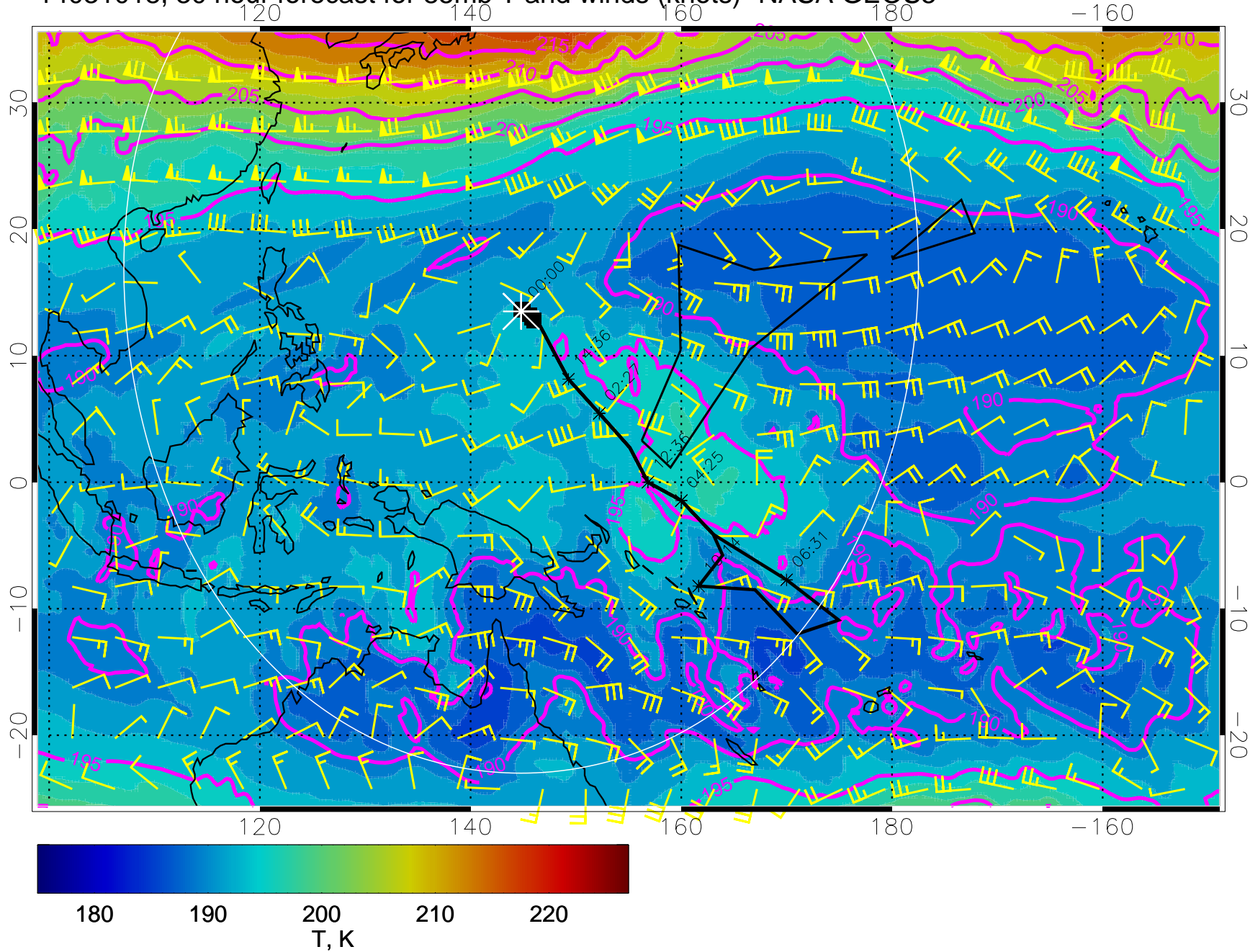
14031018, 30 hour forecast for 85mb T and winds (knots)- NASA GEOS5
