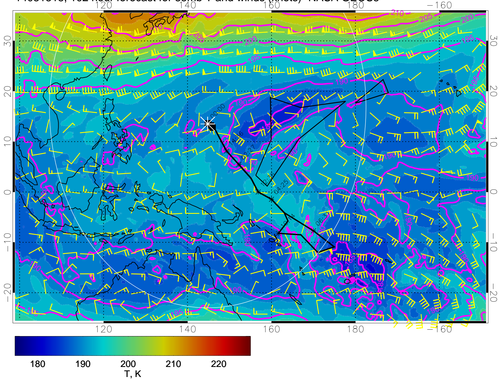
14031318, 102 hour forecast for 85mb T and winds (knots)- NASA GEOS5
