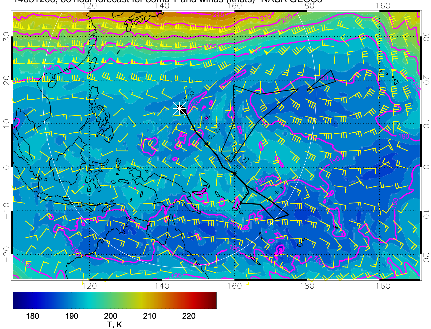
14031206, 66 hour forecast for 85mb T and winds (knots)- NASA GEOS5
