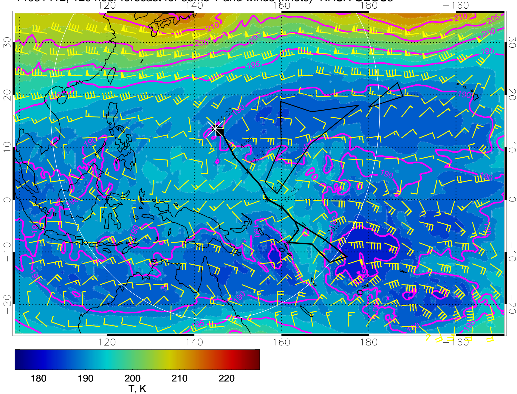
14031412, 120 hour forecast for 85mb T and winds (knots)- NASA GEOS5
