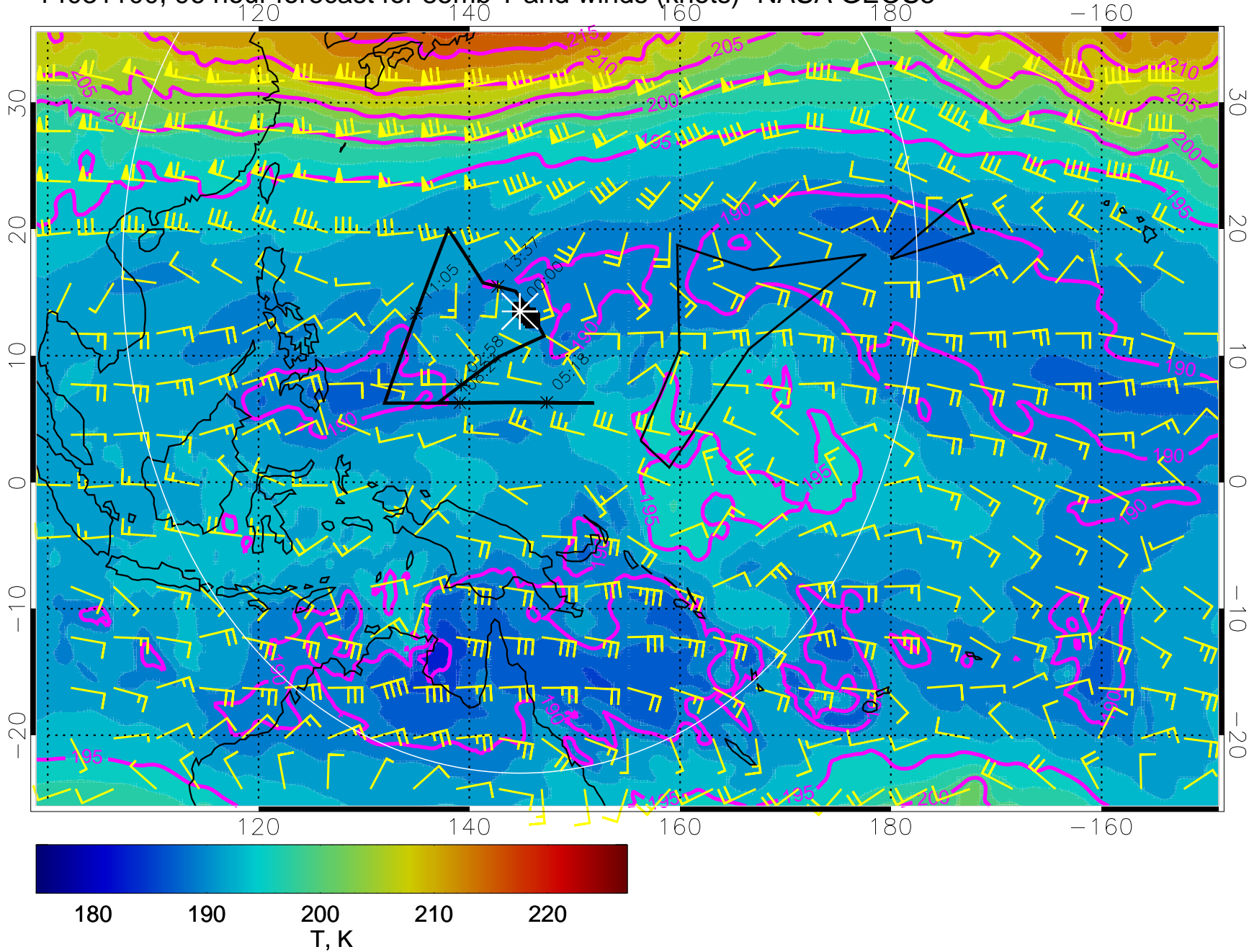
14031100, 96 hour forecast for 85mb T and winds (knots)- NASA GEOS5
