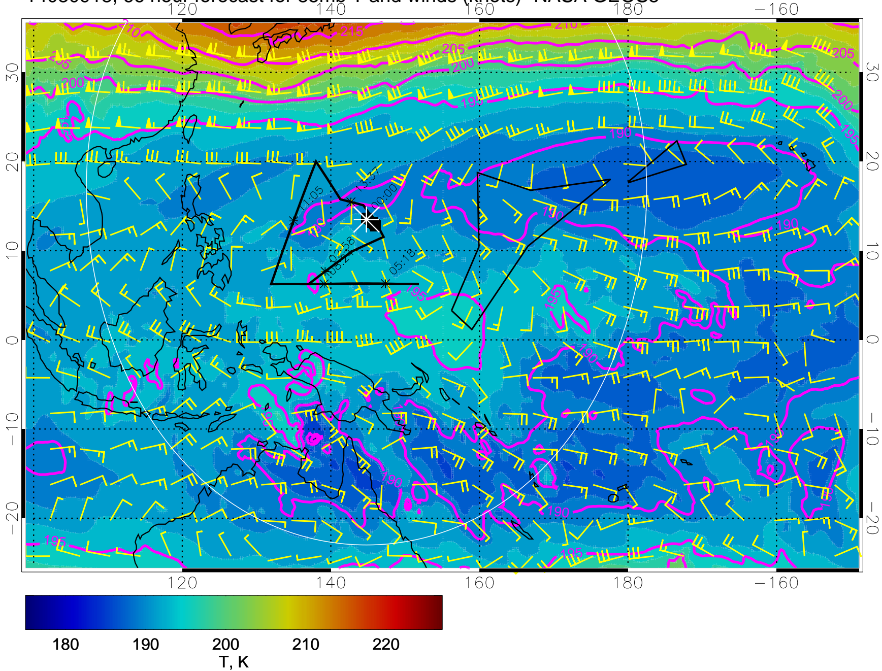
14030918, 66 hour forecast for 85mb T and winds (knots)- NASA GEOS5
