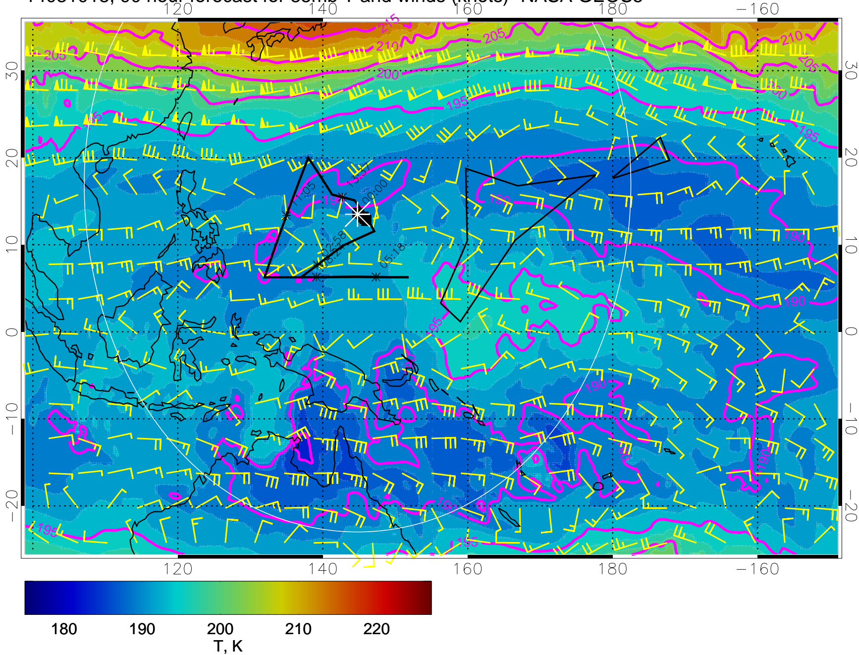
14031018, 90 hour forecast for 85mb T and winds (knots)- NASA GEOS5
