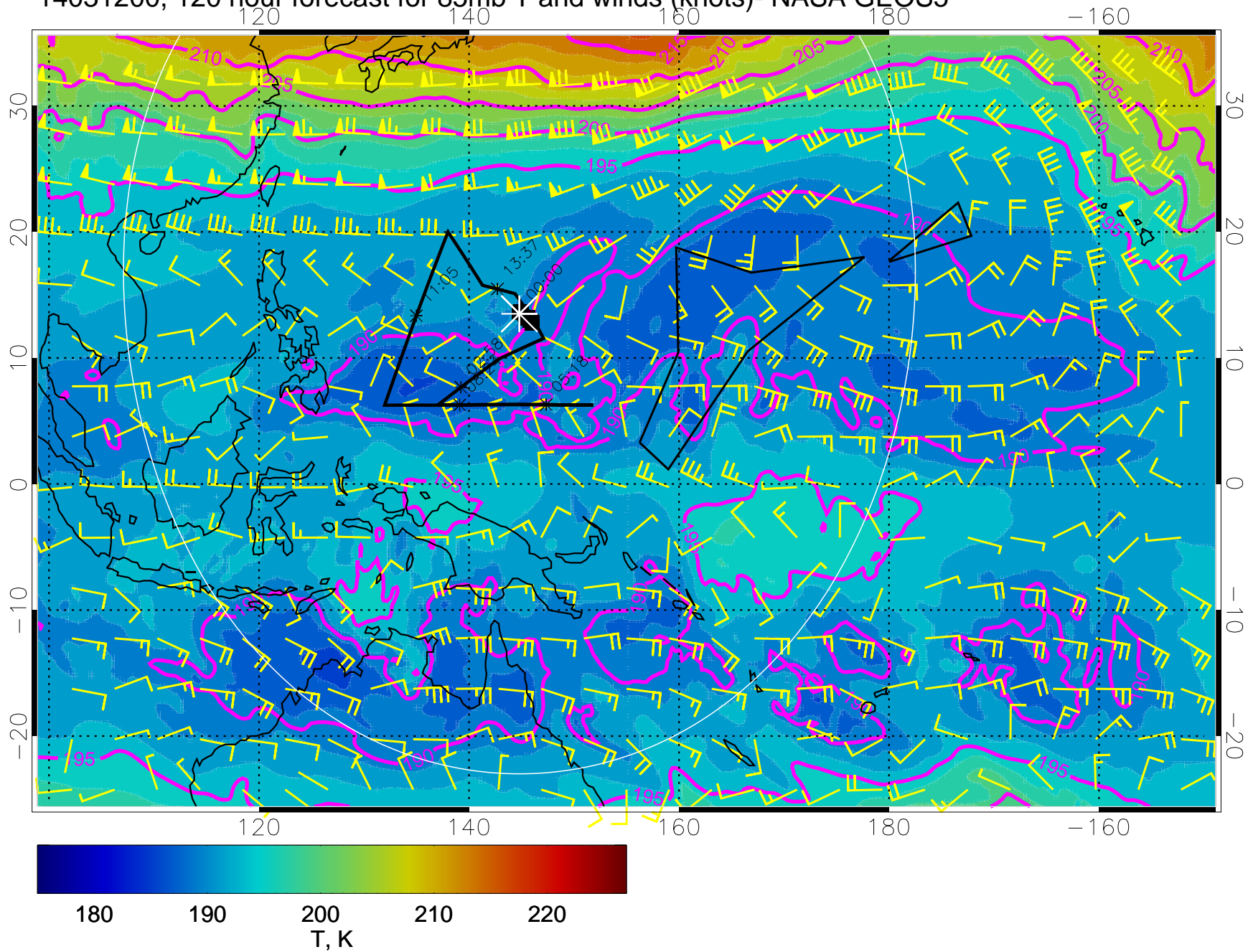
14031200, 120 hour forecast for 85mb T and winds (knots)- NASA GEOS5
