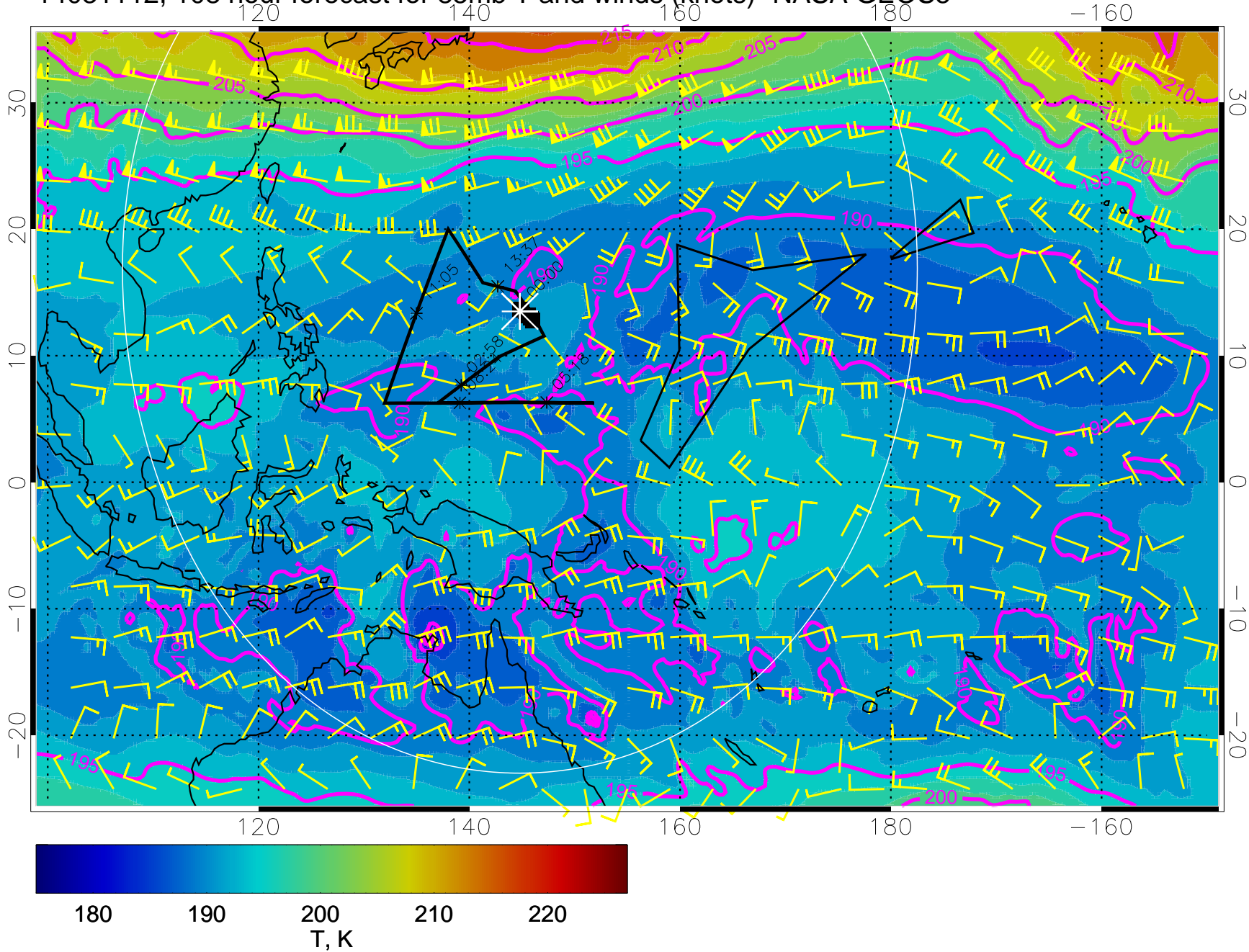
14031112, 108 hour forecast for 85mb T and winds (knots)- NASA GEOS5
