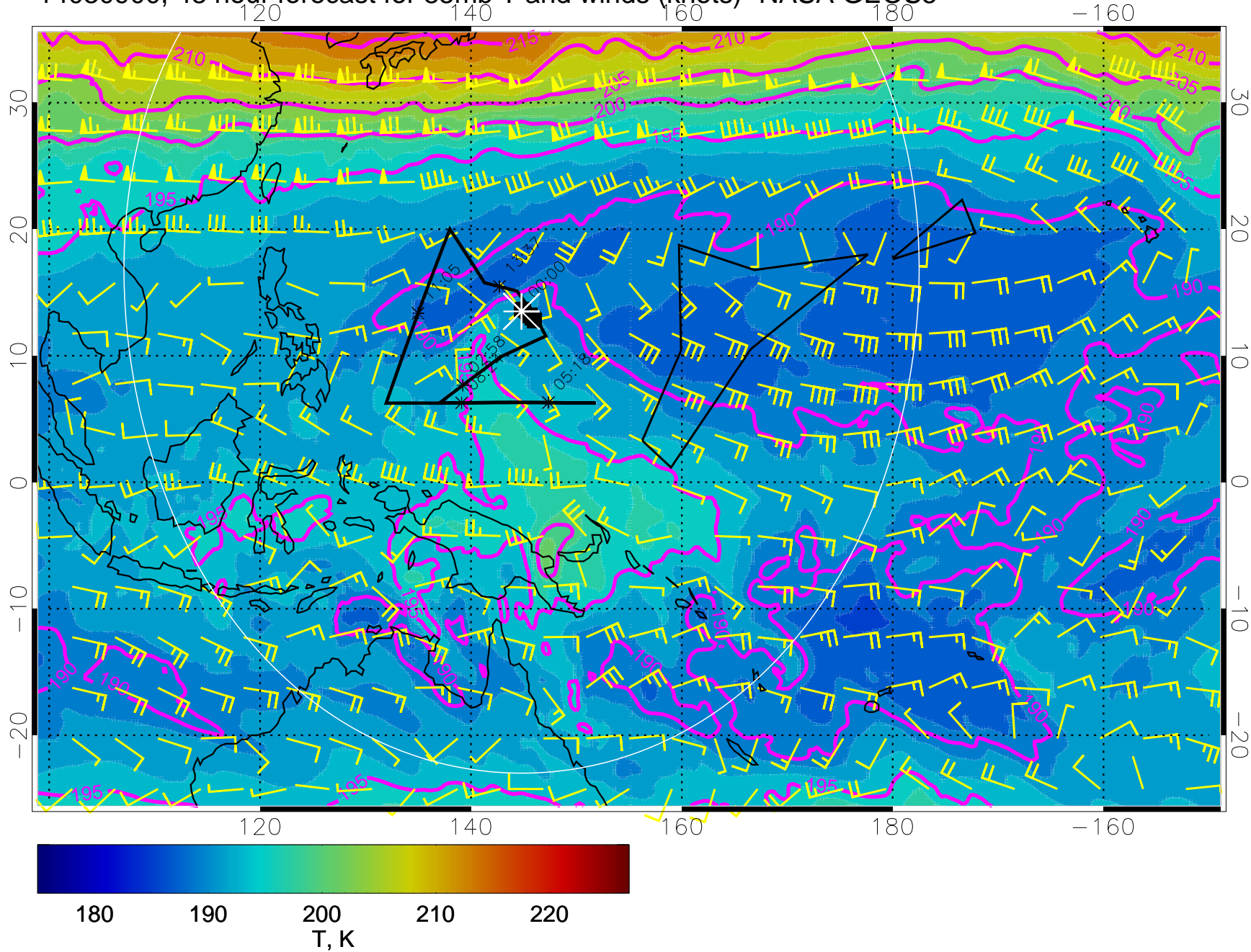
14030900, 48 hour forecast for 85mb T and winds (knots)- NASA GEOS5
