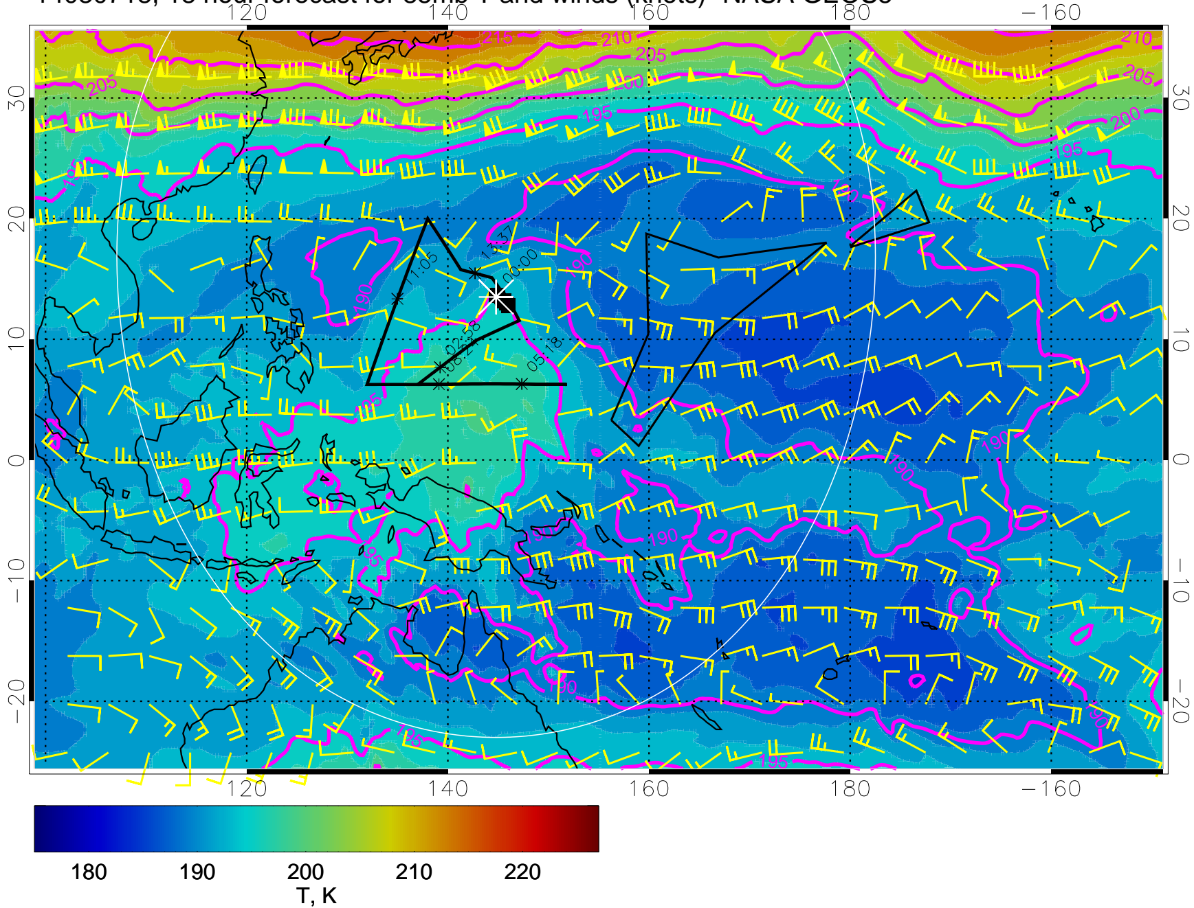
14030718, 18 hour forecast for 85mb T and winds (knots)- NASA GEOS5
