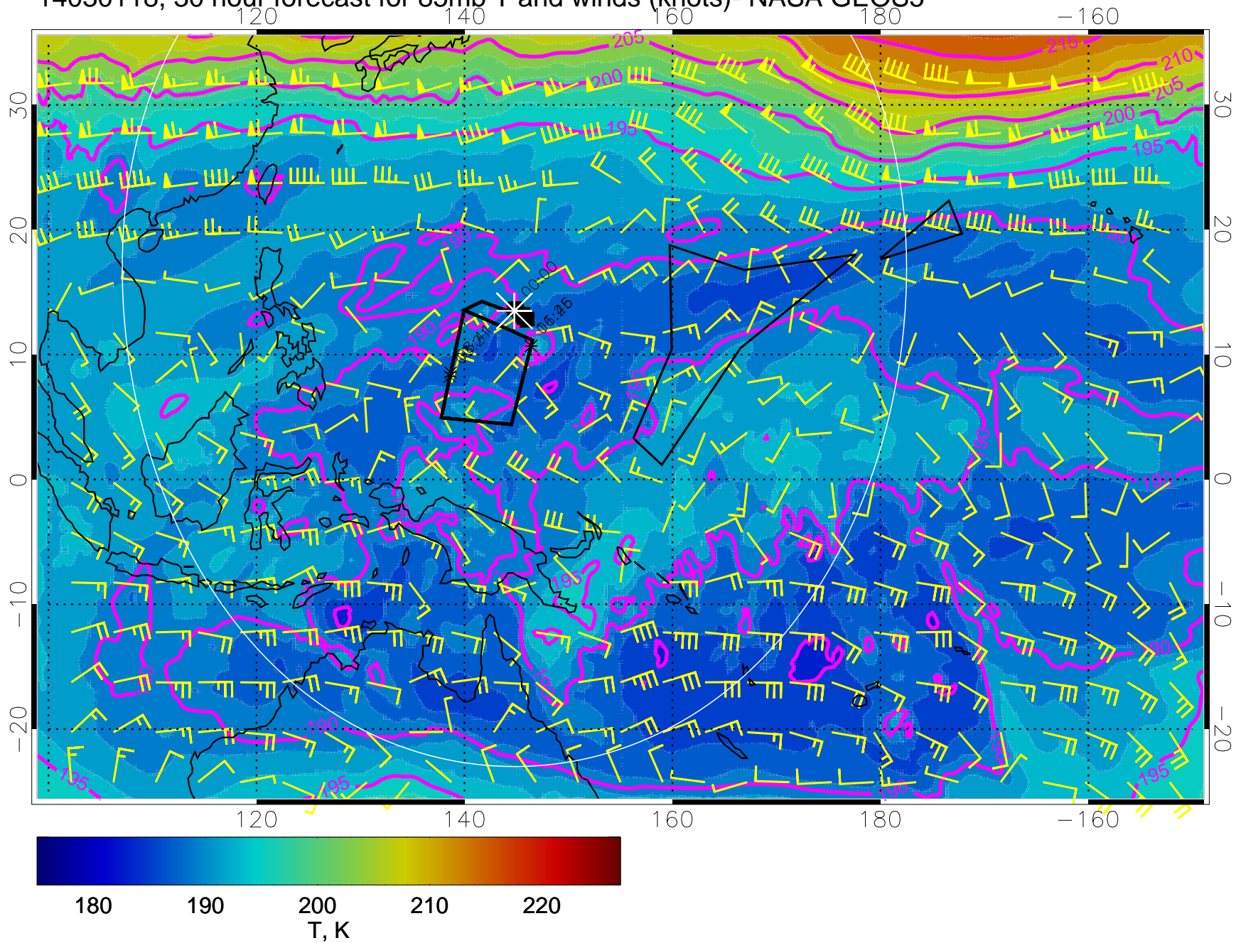
14030118, 30 hour forecast for 85mb T and winds (knots)- NASA GEOS5
