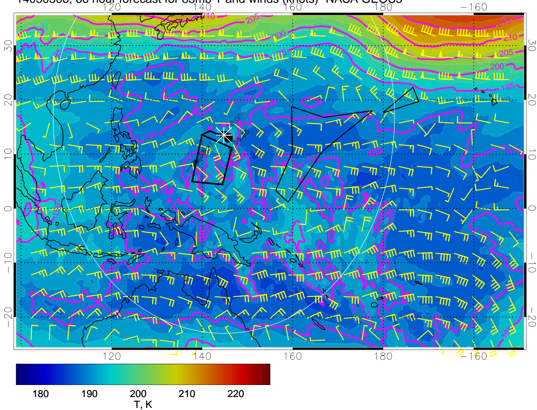
14030306, 66 hour forecast for 85mb T and winds (knots)- NASA GEOS5
