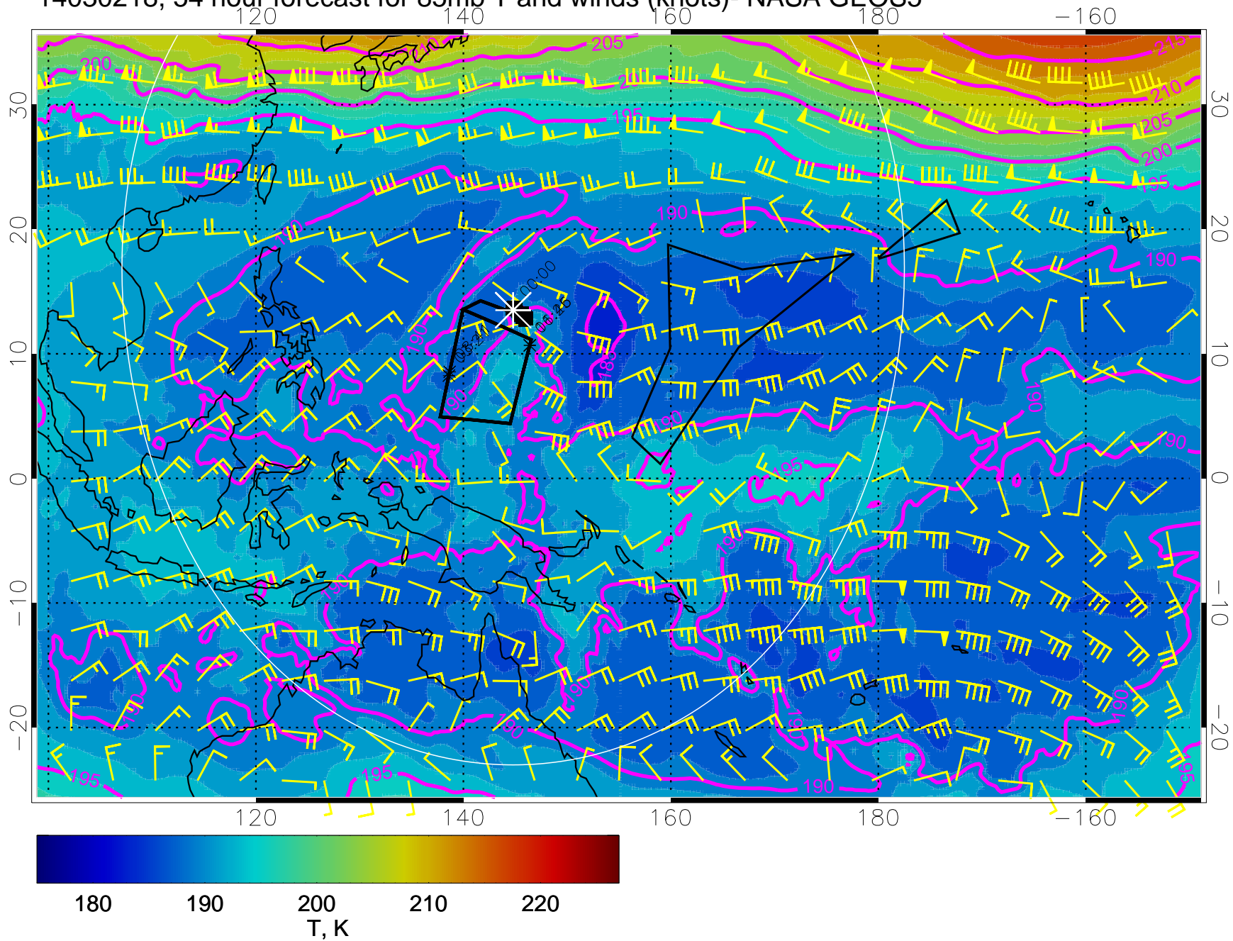
14030218, 54 hour forecast for 85mb T and winds (knots)- NASA GEOS5
