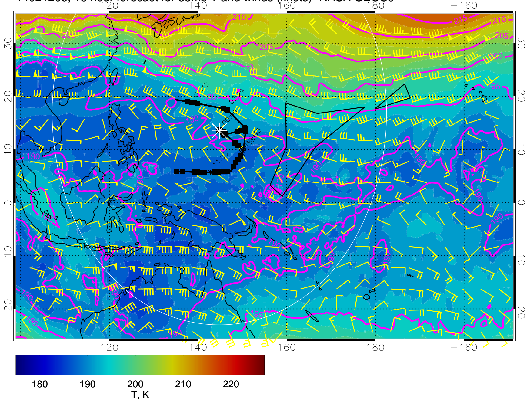
14021206, 18 hour forecast for 85mb T and winds (knots)- NASA GEOS5
