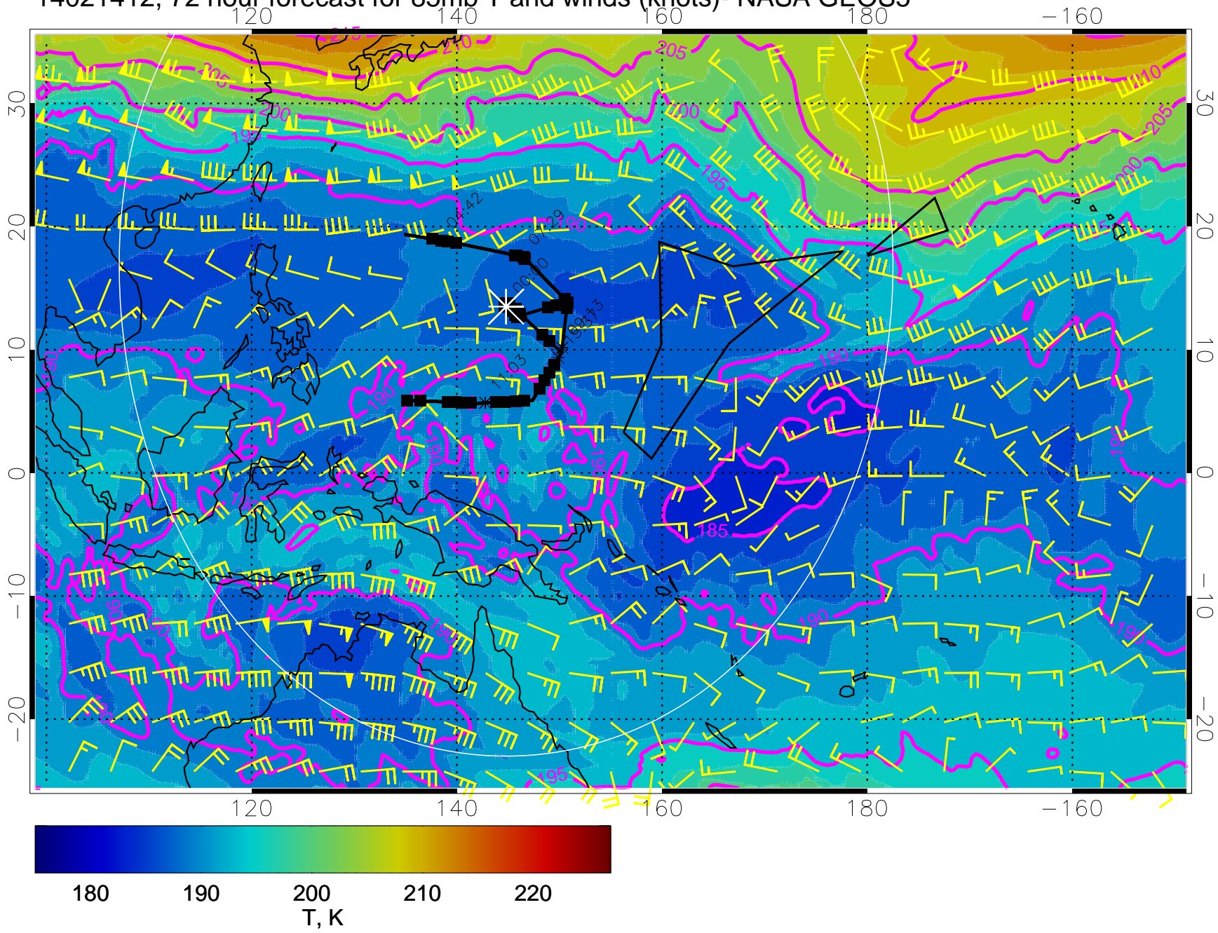
14021412, 72 hour forecast for 85mb T and winds (knots)- NASA GEOS5
