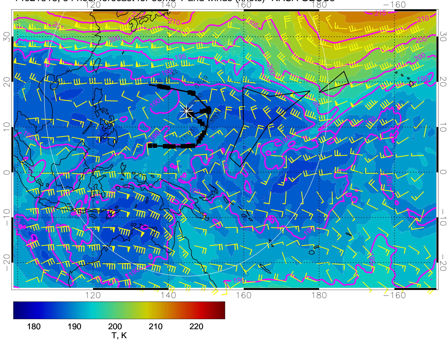
14021318, 54 hour forecast for 85mb T and winds (knots)- NASA GEOS5
