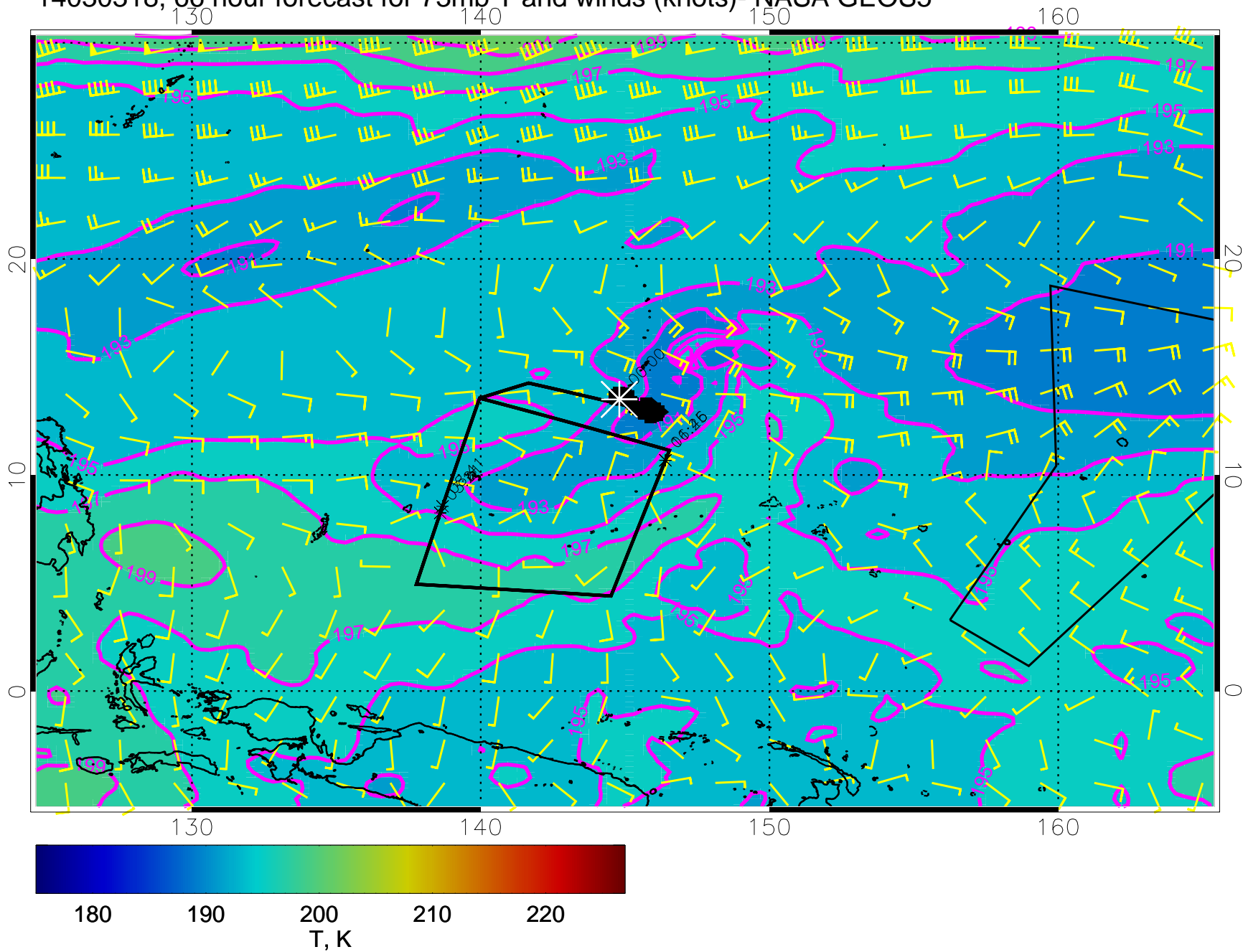
14030318, 66 hour forecast for 73mb T and winds (knots)- NASA GEOS5
