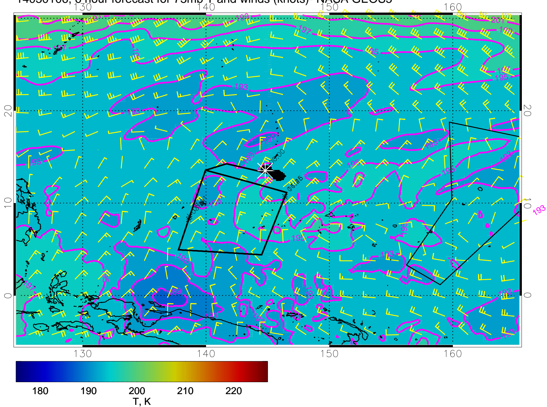
14030106, 6 hour forecast for 73mb T and winds (knots)- NASA GEOS5
