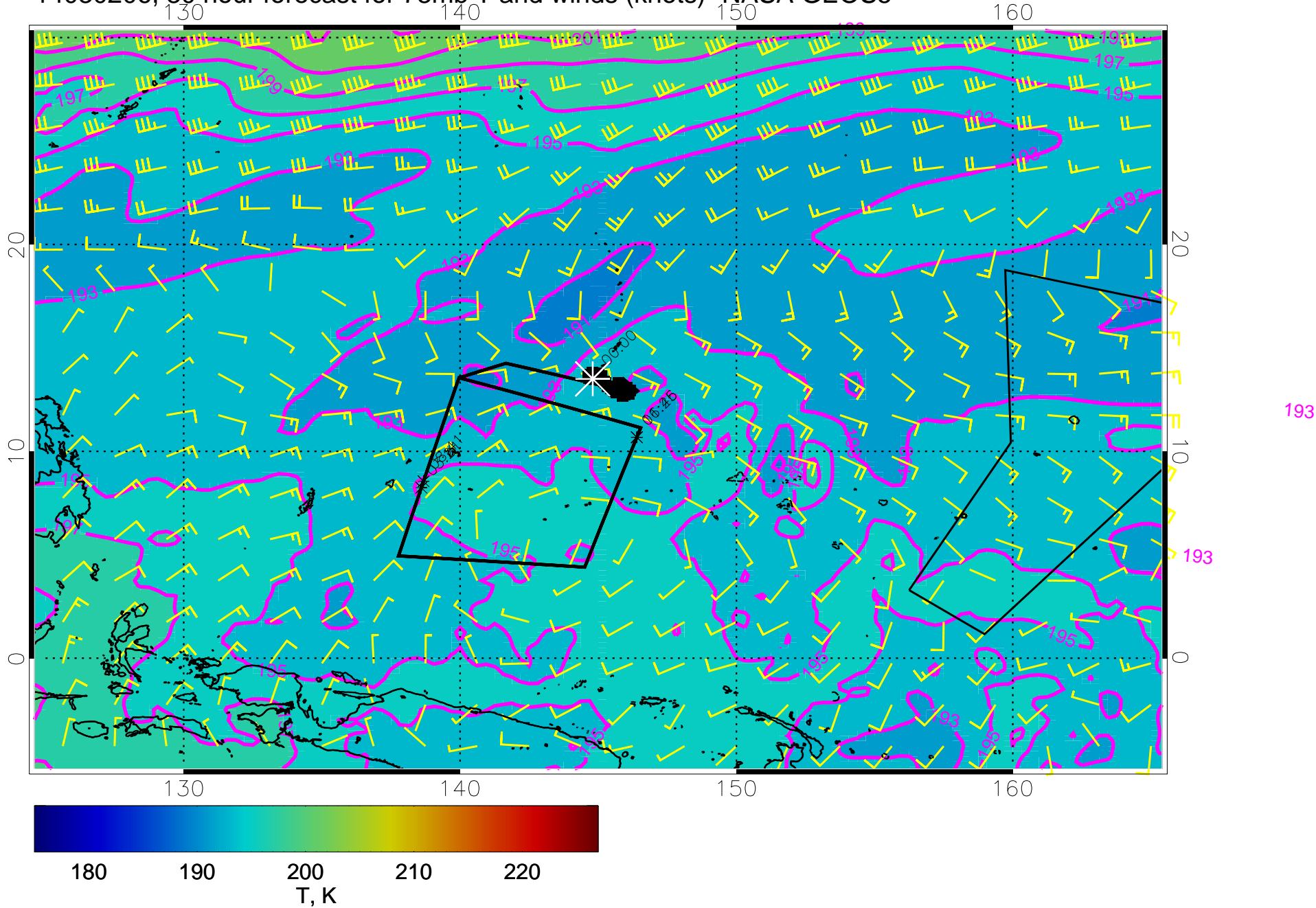
14030206, 30 hour forecast for 73mb T and winds (knots)- NASA GEOS5
