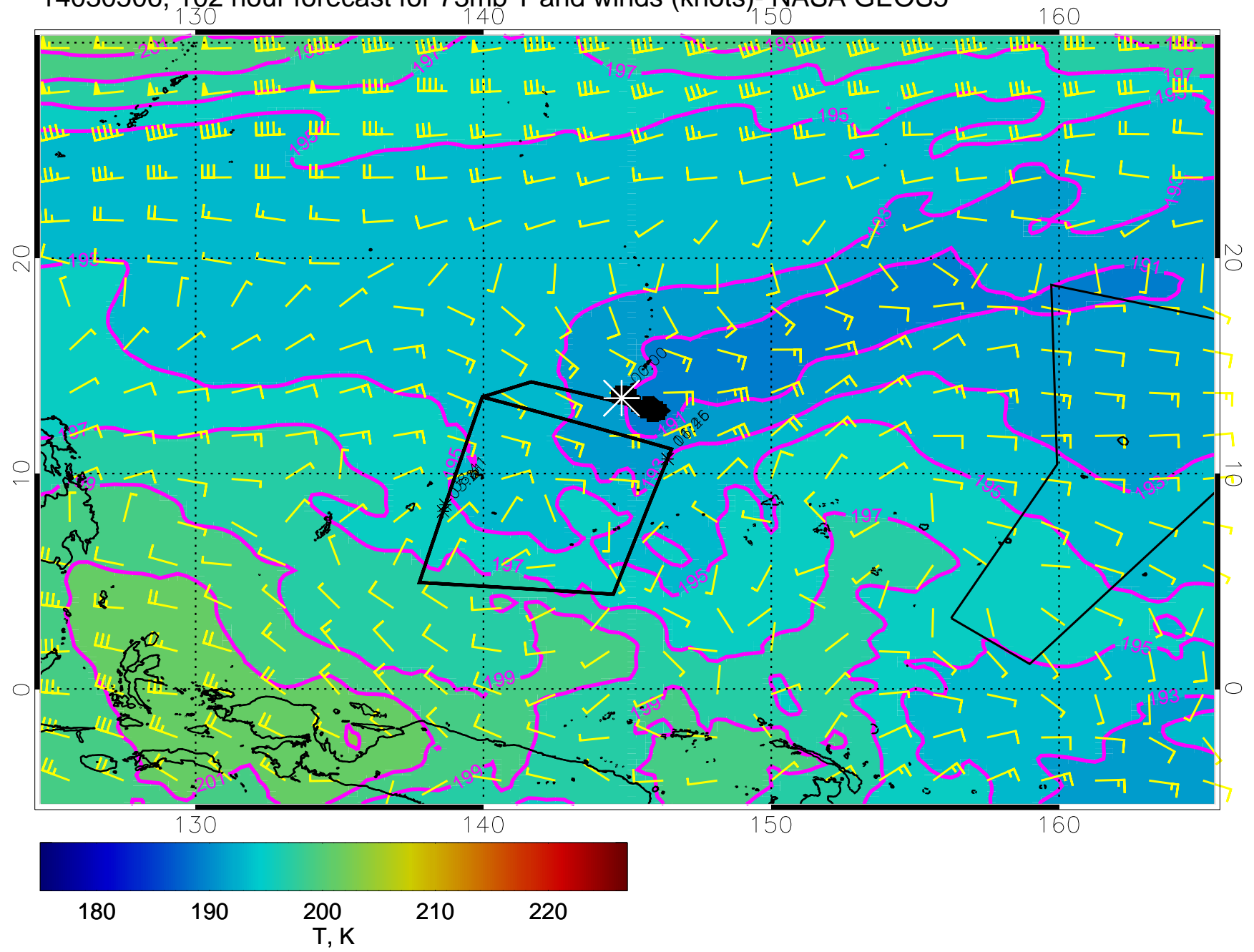
14030506, 102 hour forecast for 73mb T and winds (knots)- NASA GEOS5
