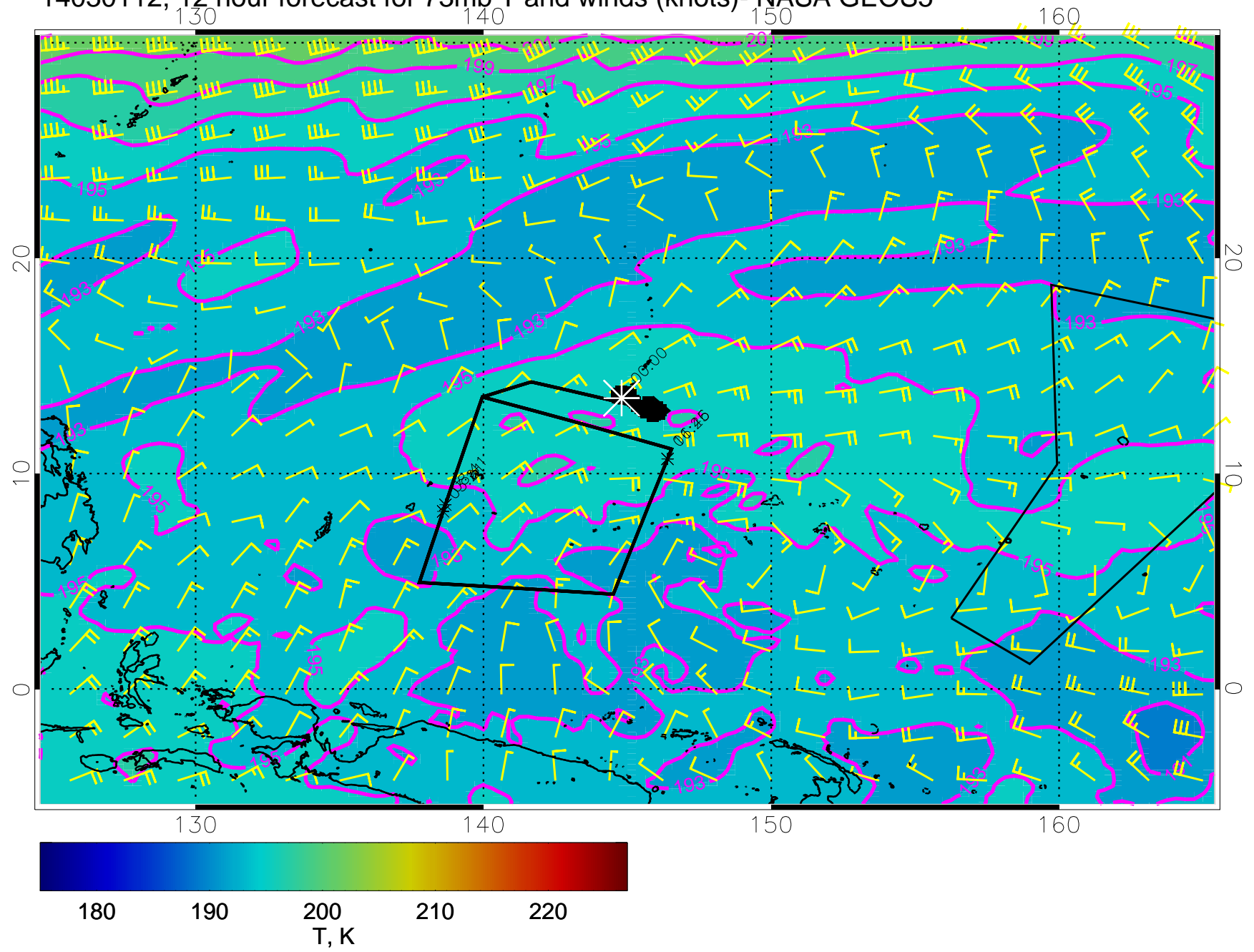
14030112, 12 hour forecast for 73mb T and winds (knots)- NASA GEOS5
