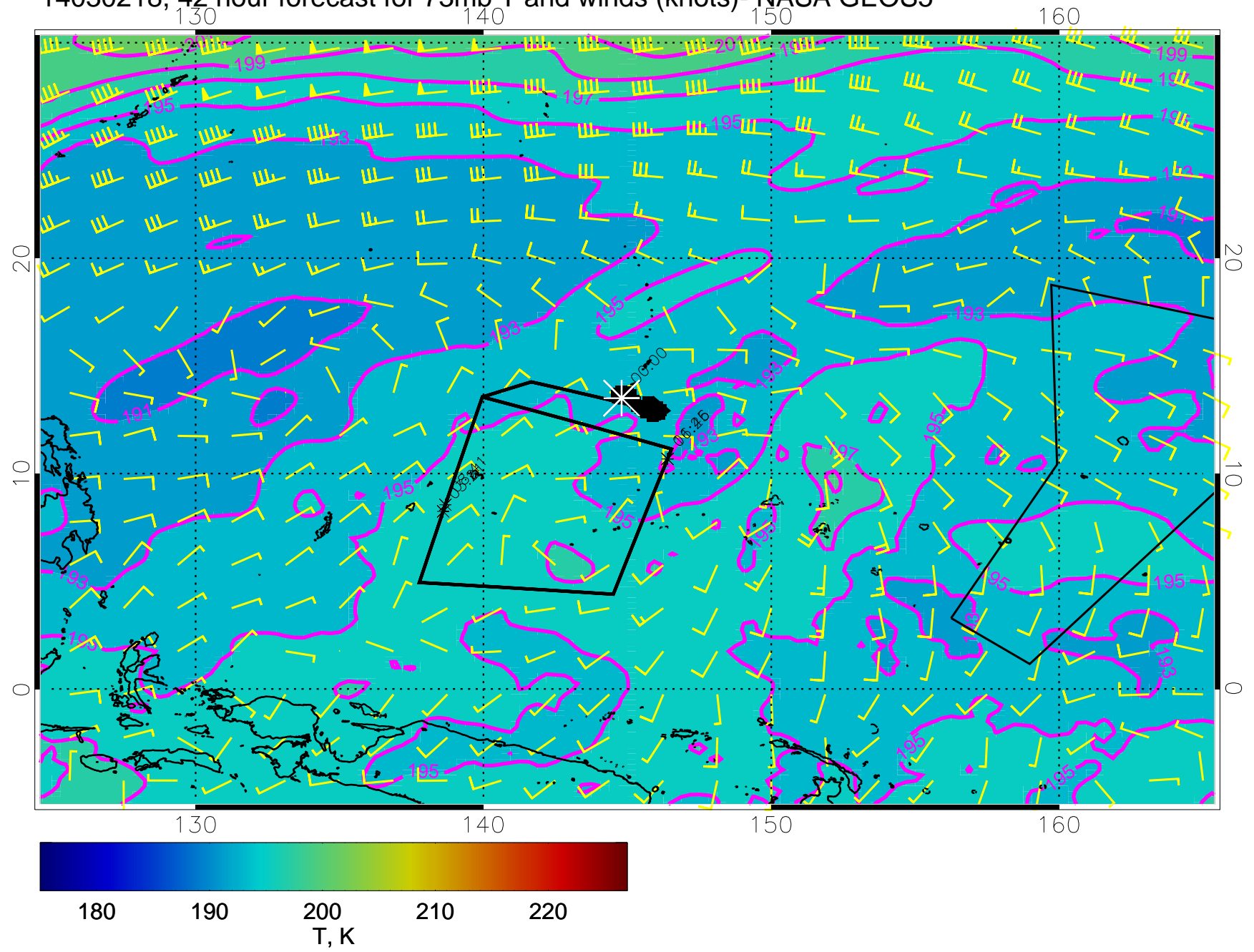
14030218, 42 hour forecast for 73mb T and winds (knots)- NASA GEOS5
