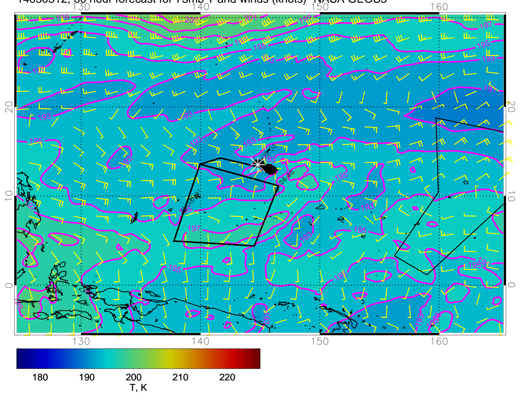
14030312, 60 hour forecast for 73mb T and winds (knots)- NASA GEOS5
