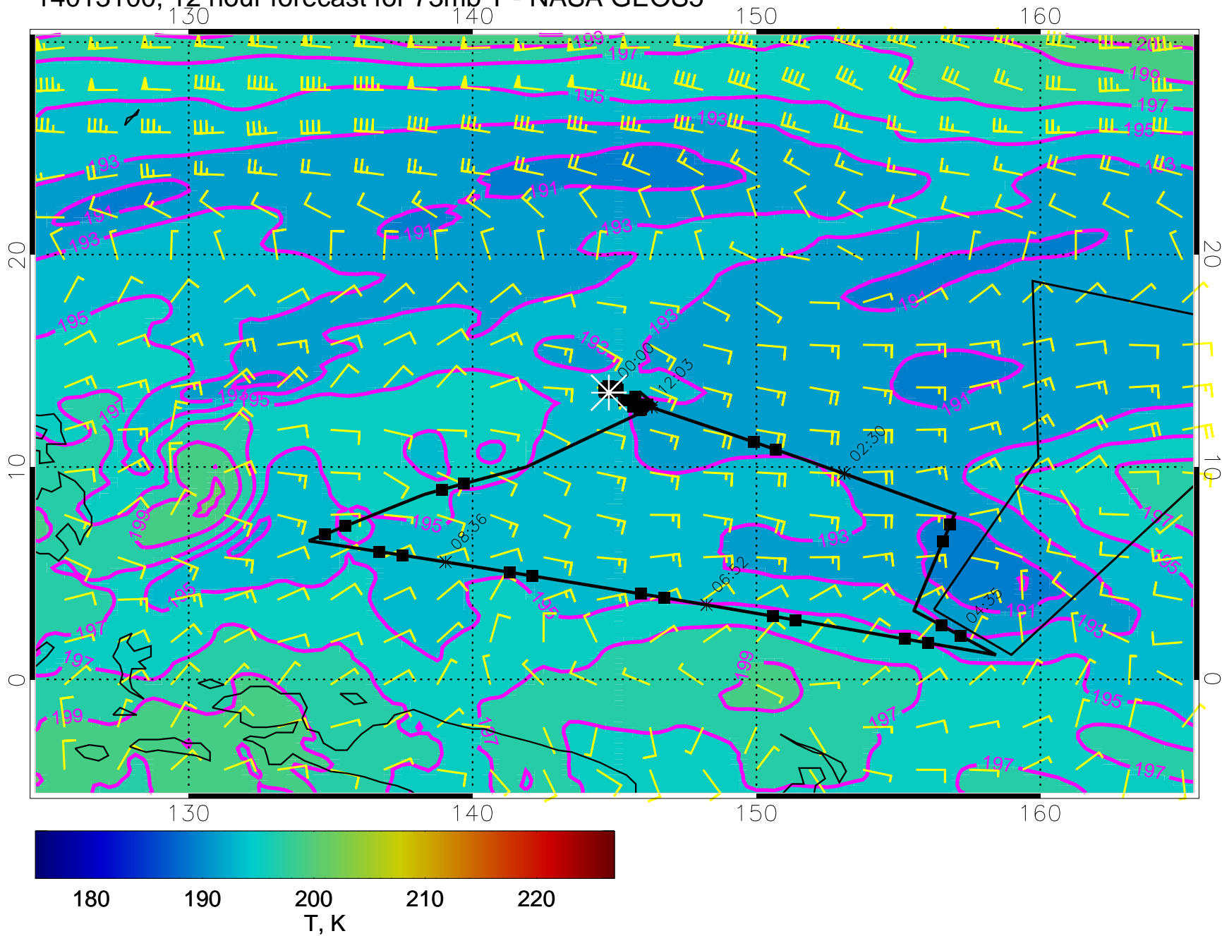
14013100, 12 hour forecast for 73mb T - NASA GEOS5
