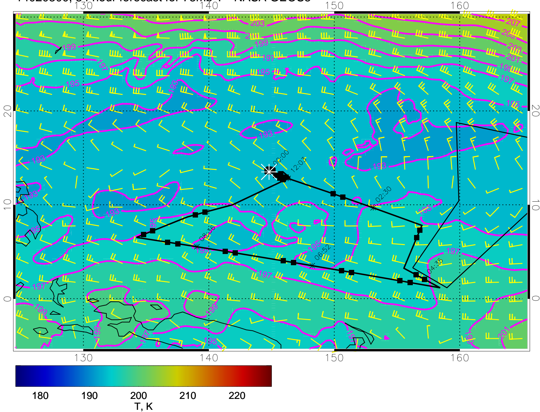
14020300, 84 hour forecast for 73mb T - NASA GEOS5
