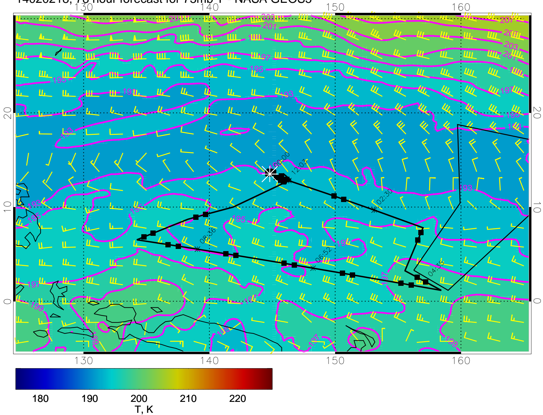
14020218, 78 hour forecast for 73mb T - NASA GEOS5
