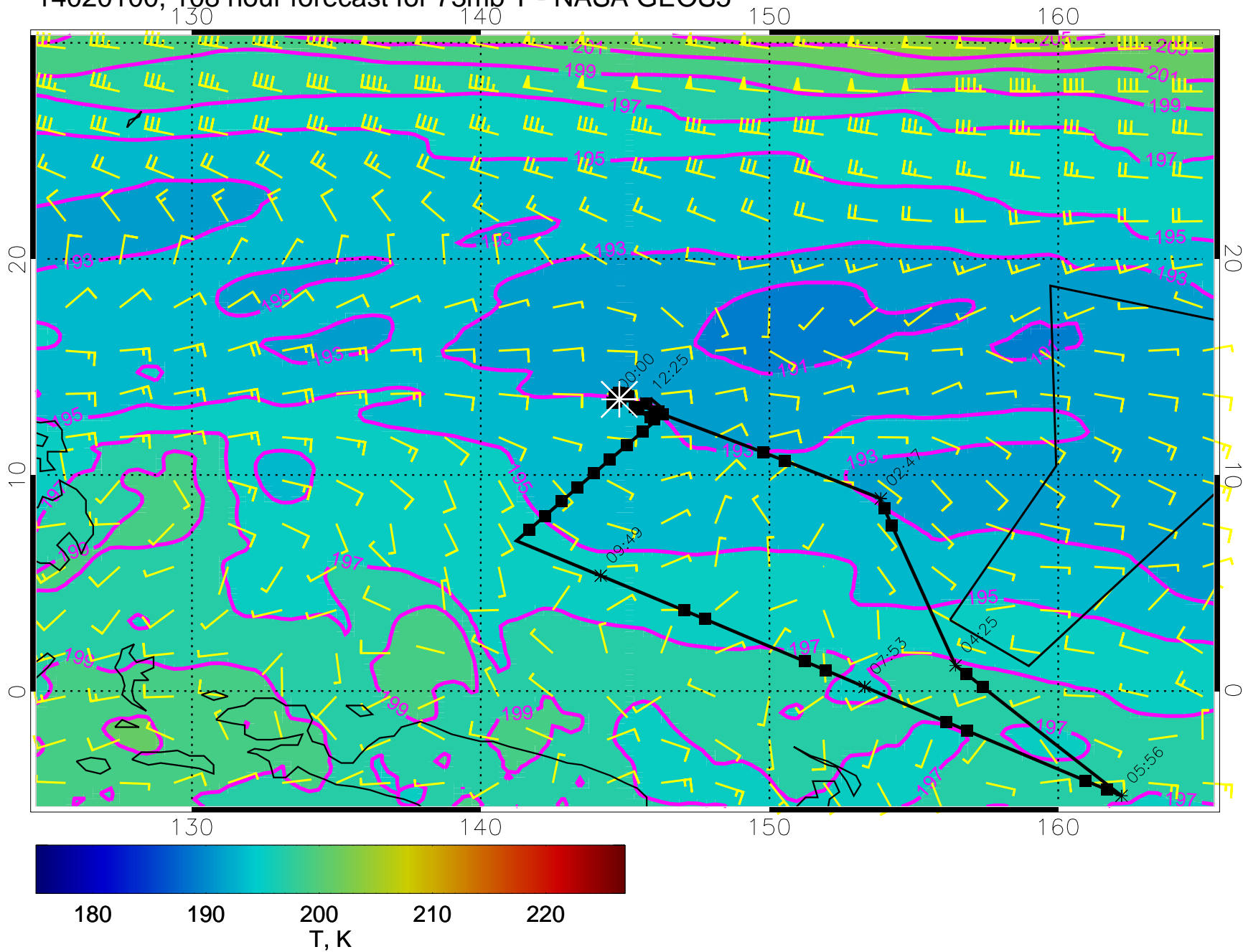
14020100, 108 hour forecast for 73mb T - NASA GEOS5
