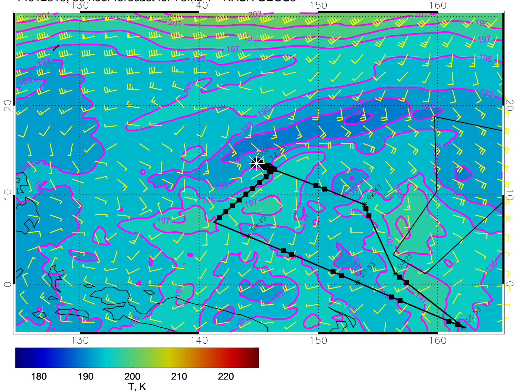
14012818, 30 hour forecast for 73mb T - NASA GEOS5
