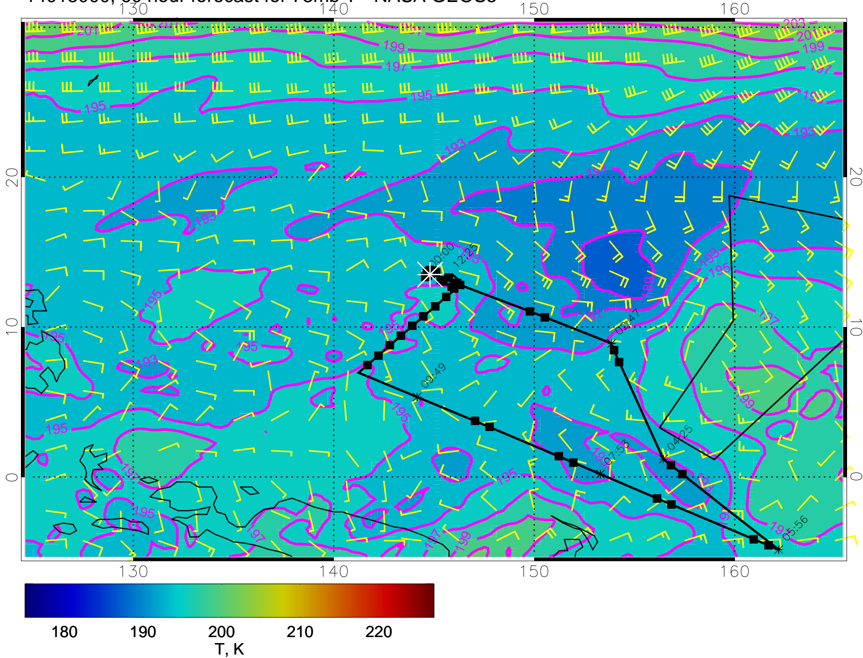
14013000, 60 hour forecast for 73mb T - NASA GEOS5
