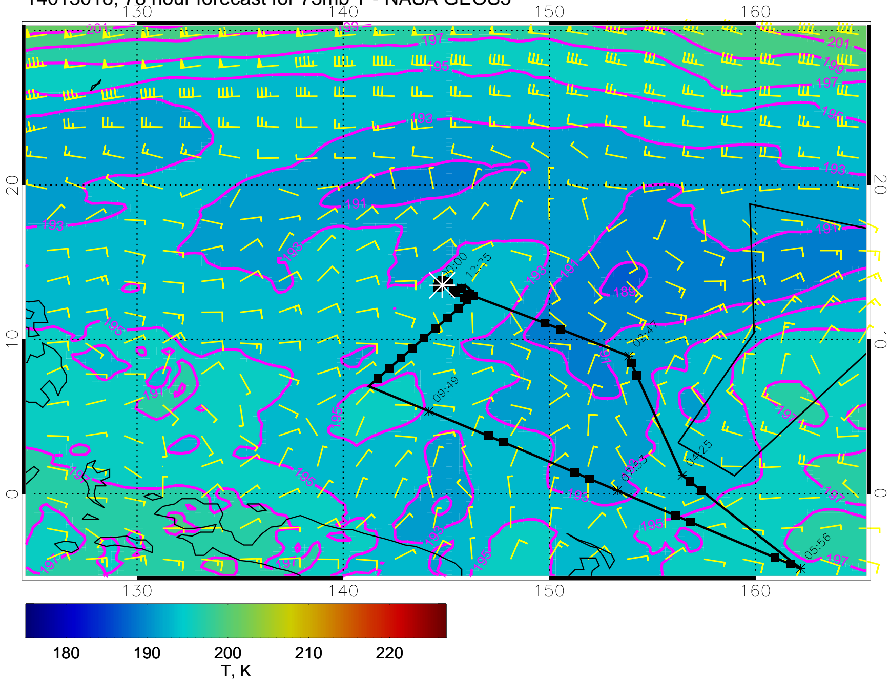
14013018, 78 hour forecast for 73mb T - NASA GEOS5
