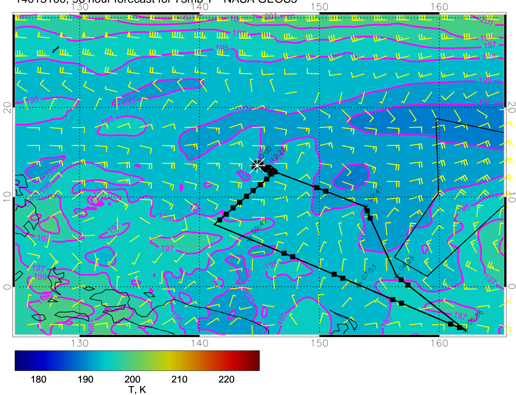
14013100, 96 hour forecast for 73mb T - NASA GEOS5
