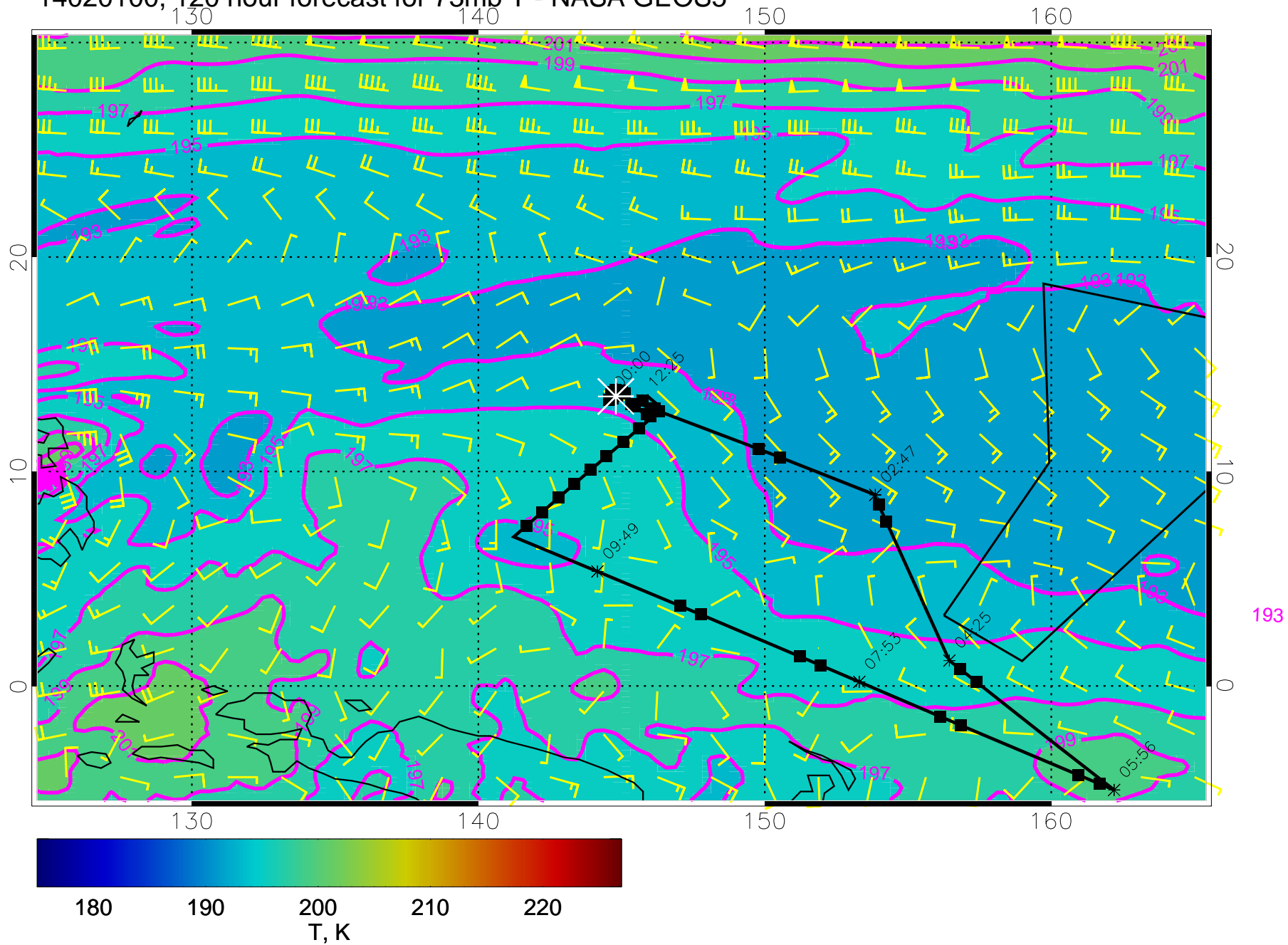
14020100, 120 hour forecast for 73mb T - NASA GEOS5
