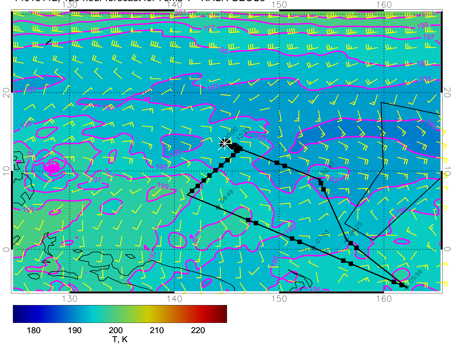
14013112, 120 hour forecast for 73mb T - NASA GEOS5
