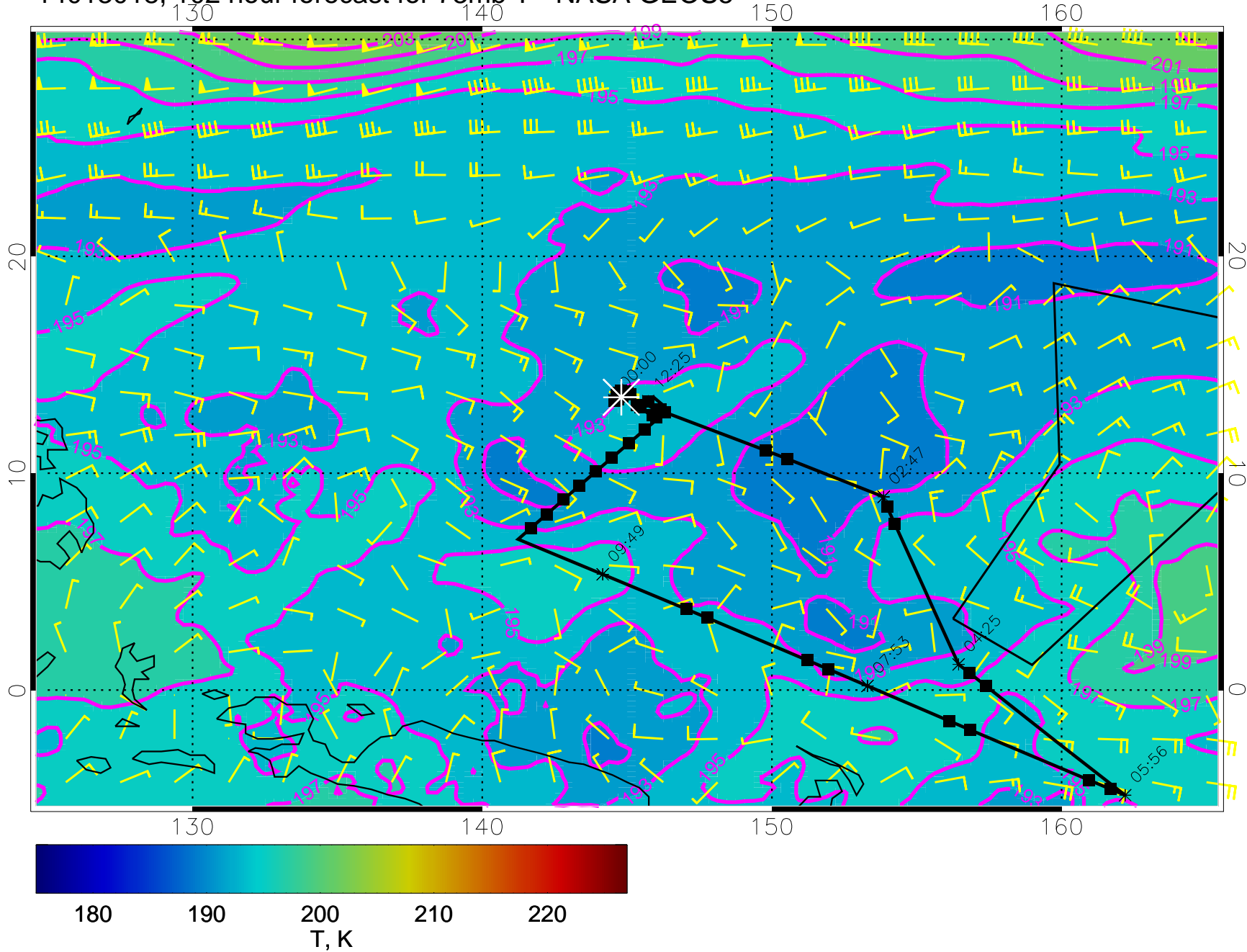
14013018, 102 hour forecast for 73mb T - NASA GEOS5
