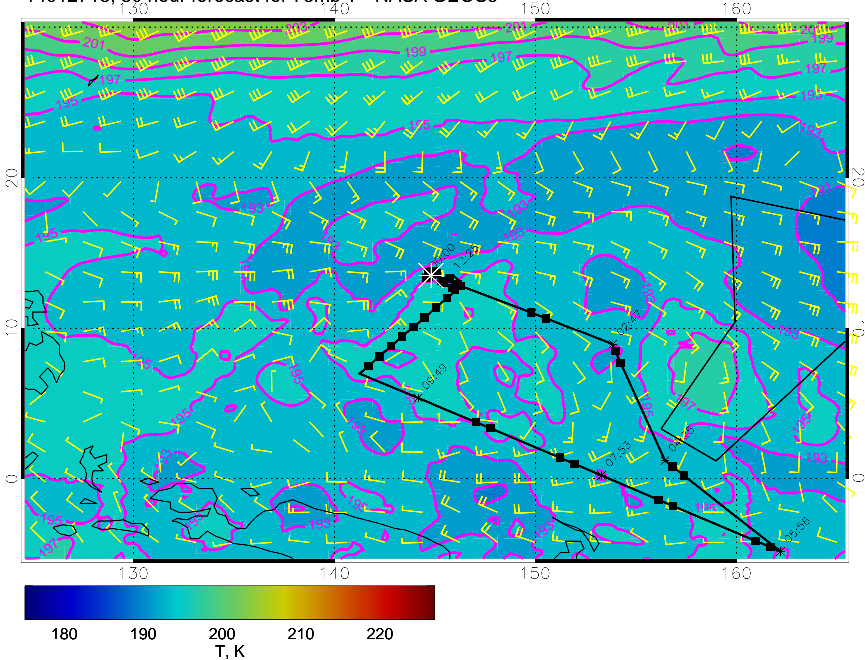
14012718, 30 hour forecast for 73mb T - NASA GEOS5
