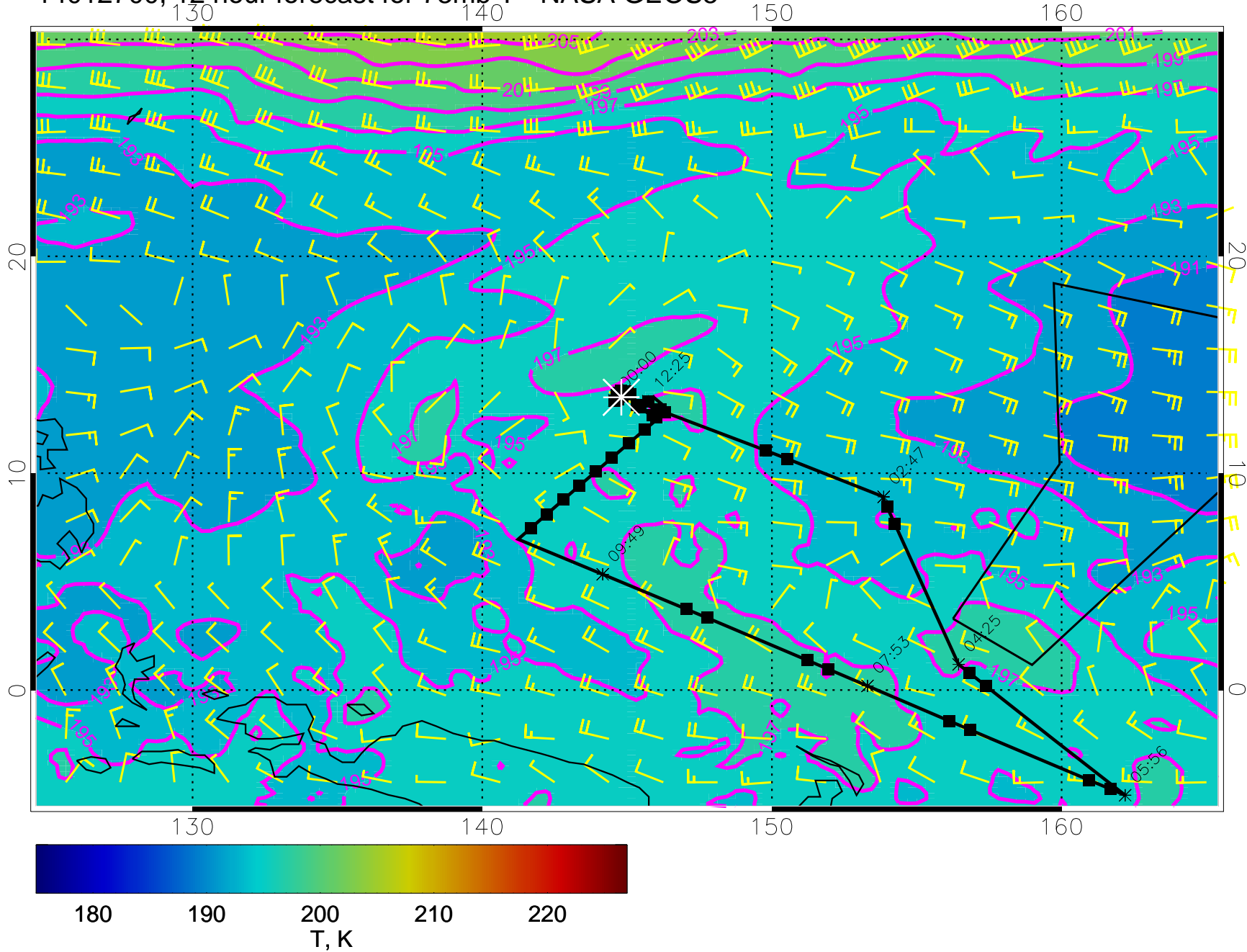
14012700, 12 hour forecast for 73mb T - NASA GEOS5
