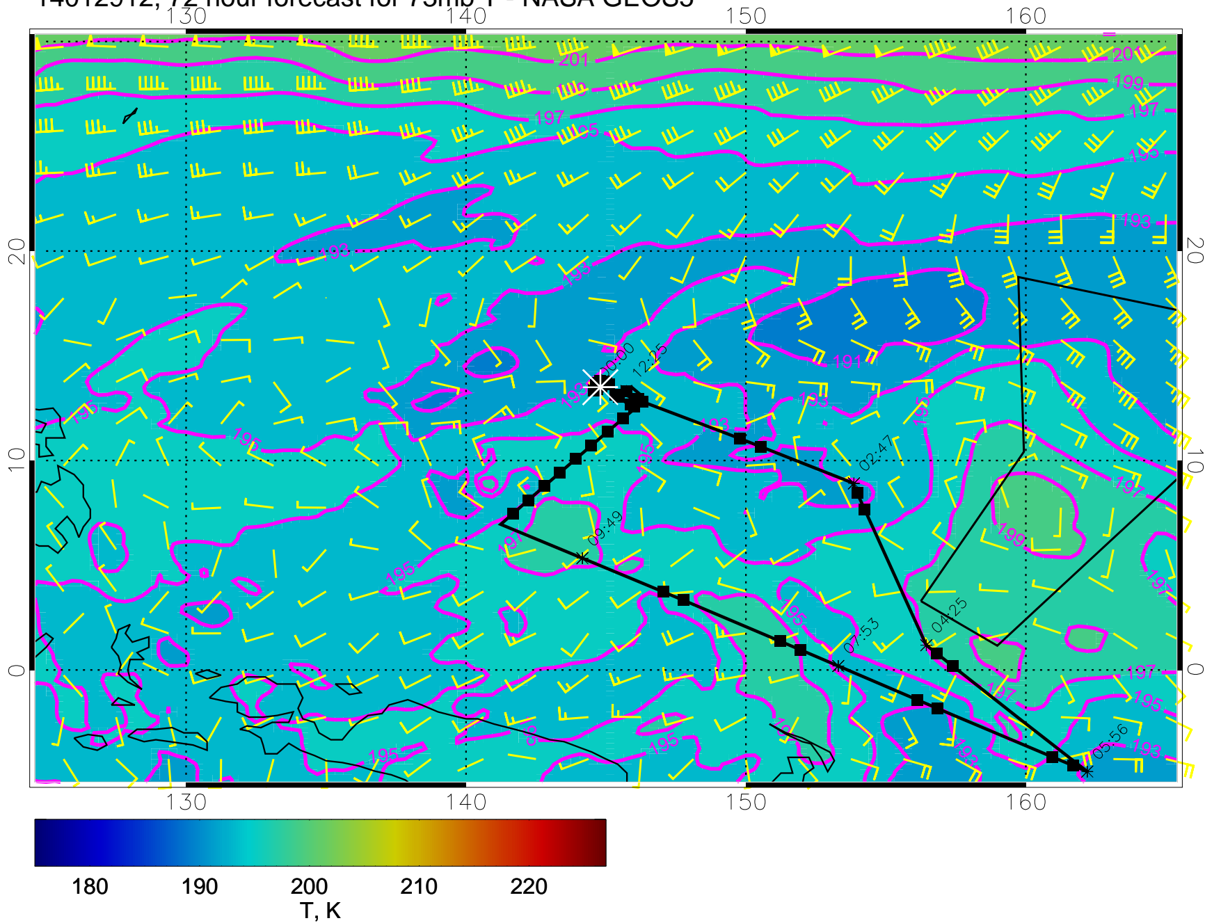
14012912, 72 hour forecast for 73mb T - NASA GEOS5
