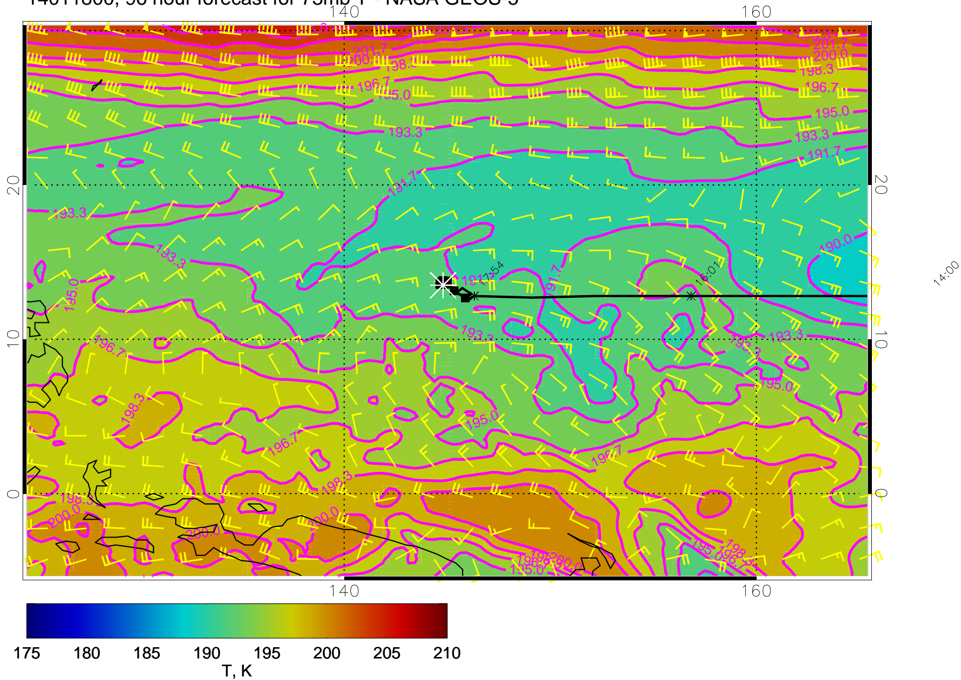
14011800, 96 hour forecast for 73mb T - NASA GEOS-5
