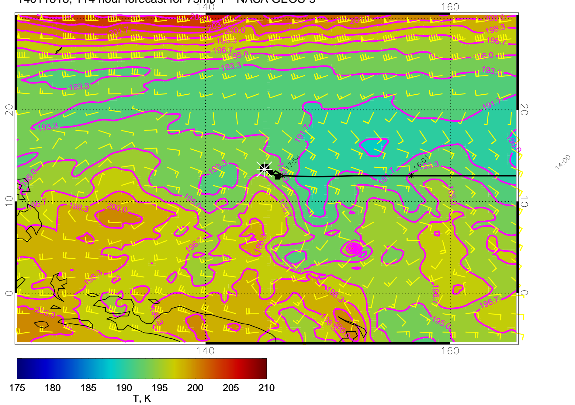
14011818, 114 hour forecast for 73mb T - NASA GEOS-5
