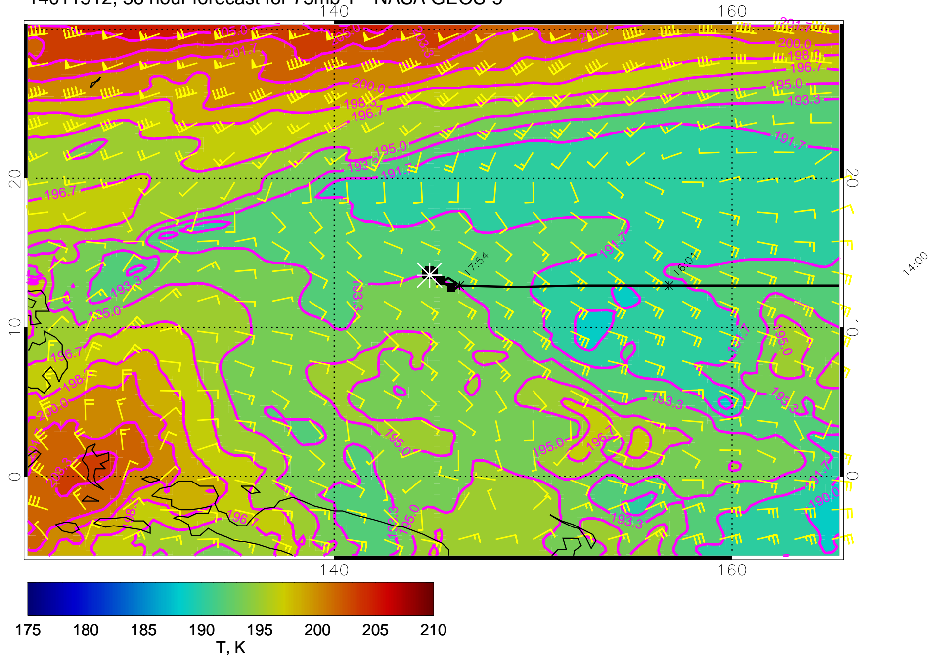
14011512, 36 hour forecast for 73mb T - NASA GEOS-5
