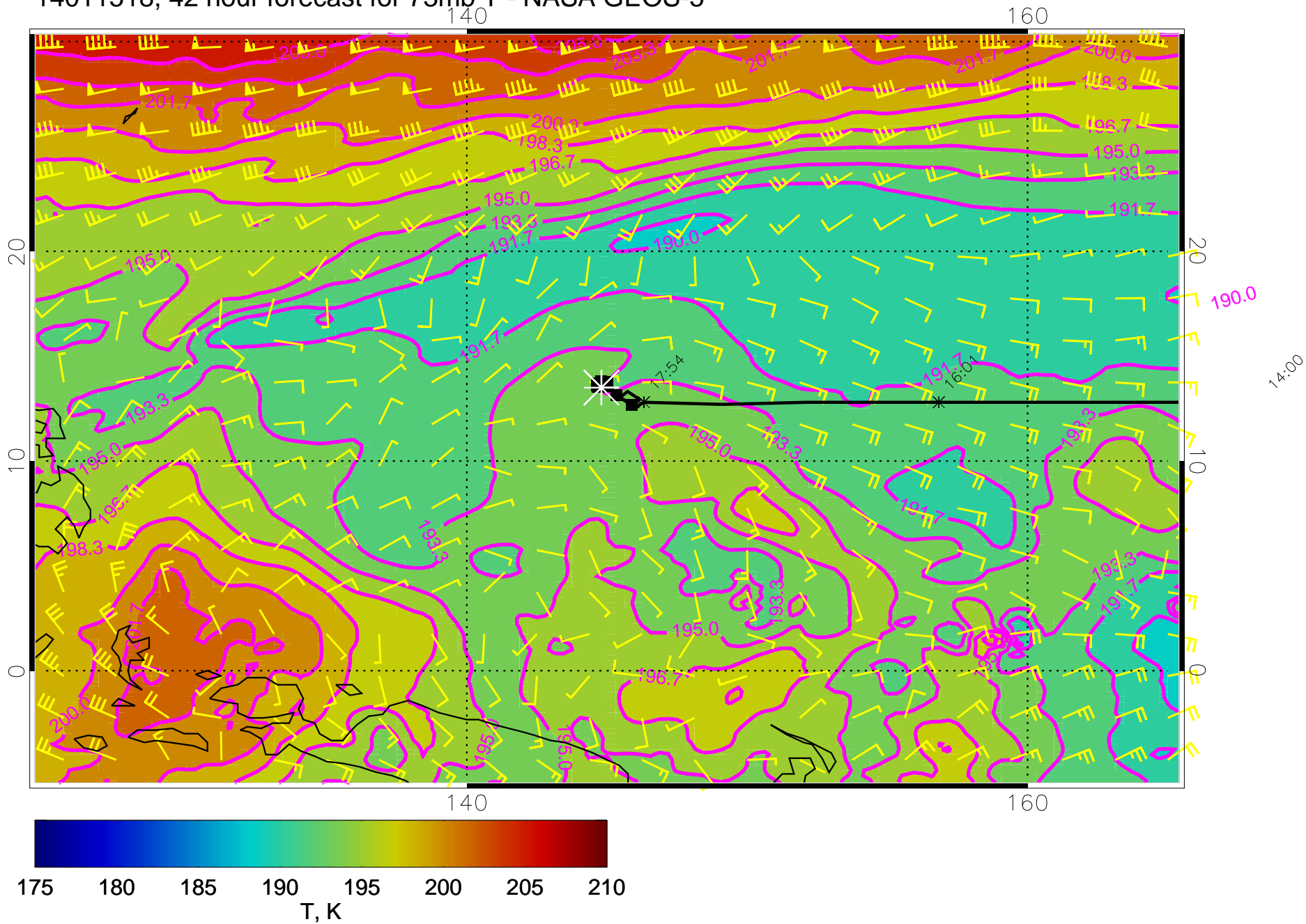
14011518, 42 hour forecast for 73mb T - NASA GEOS-5
