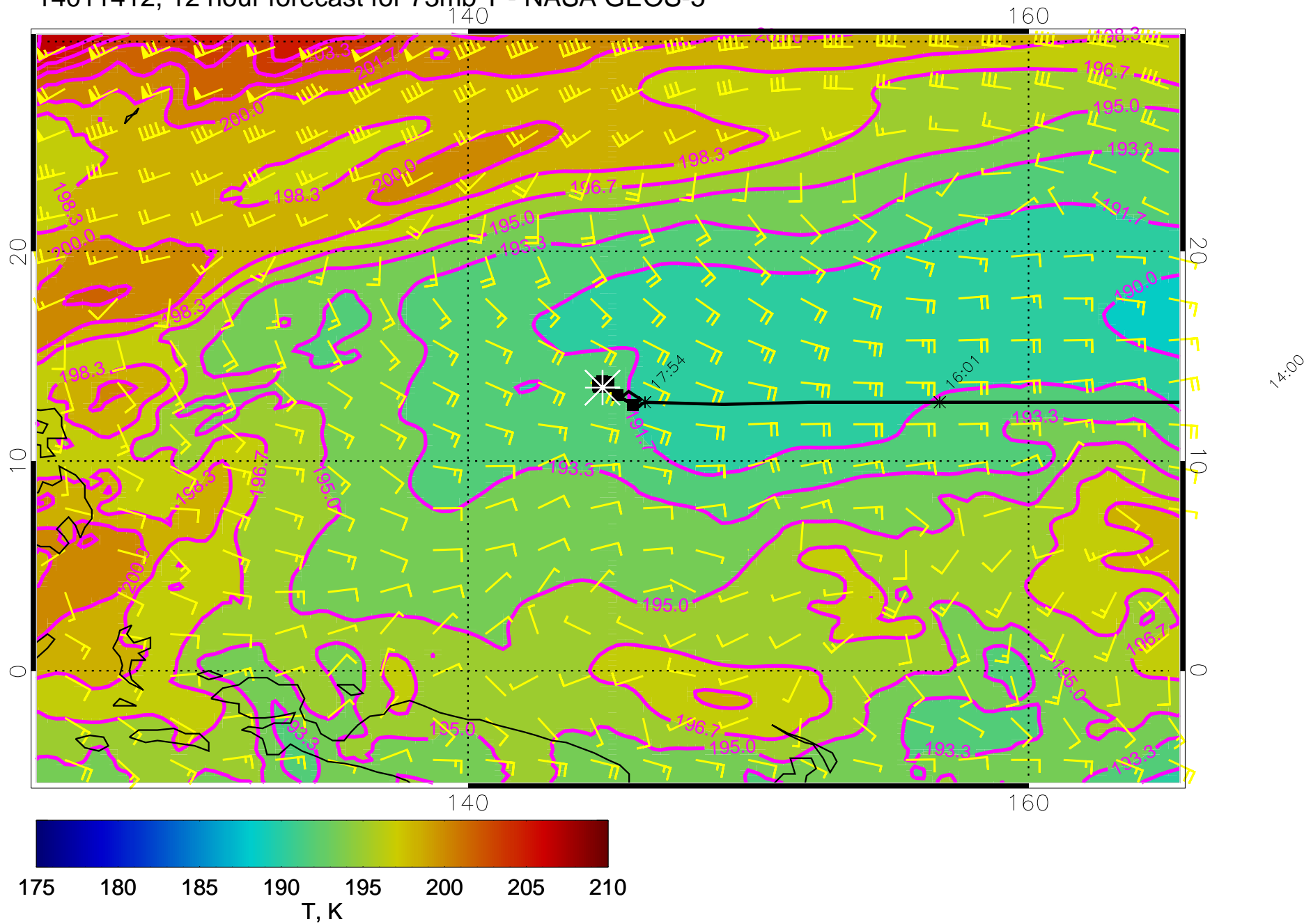
14011412, 12 hour forecast for 73mb T - NASA GEOS-5
