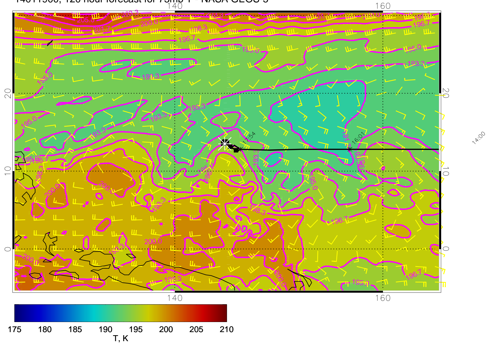
14011900, 120 hour forecast for 73mb T - NASA GEOS-5
