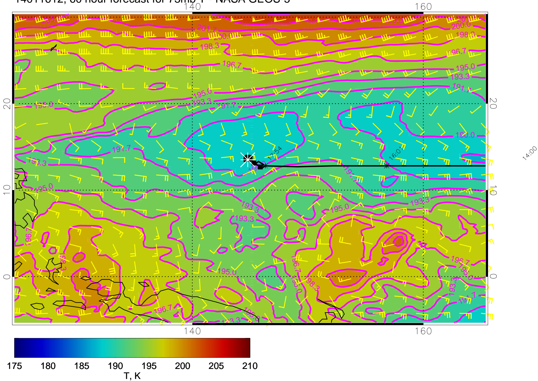
14011612, 60 hour forecast for 73mb T - NASA GEOS-5
