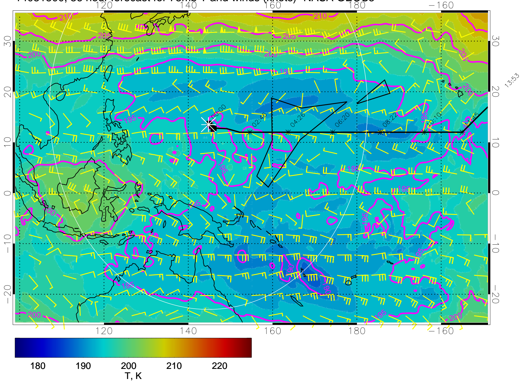
14031800, 36 hour forecast for 73mb T and winds (knots)- NASA GEOS5
