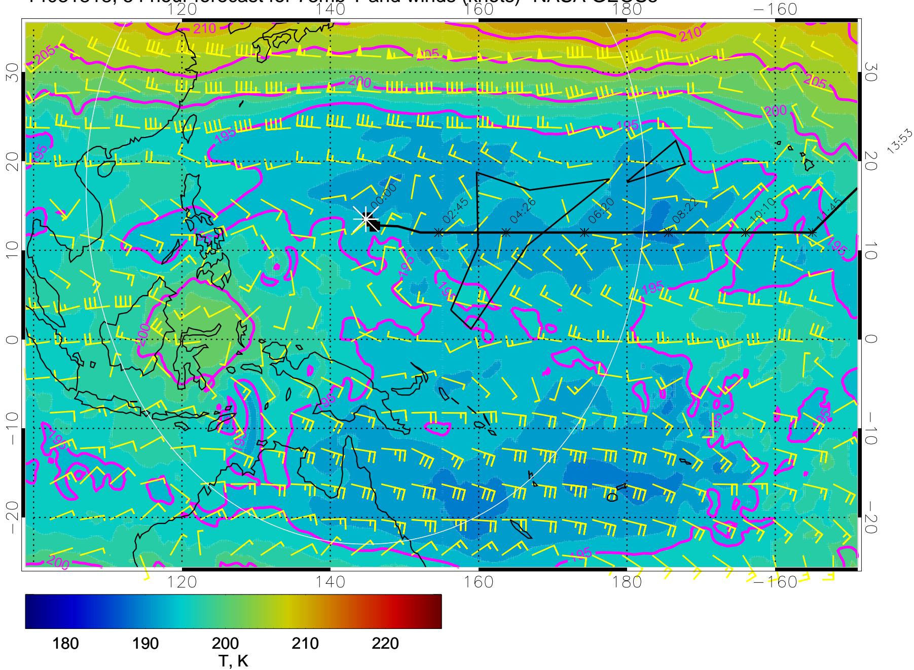
14031818, 54 hour forecast for 73mb T and winds (knots)- NASA GEOS5
