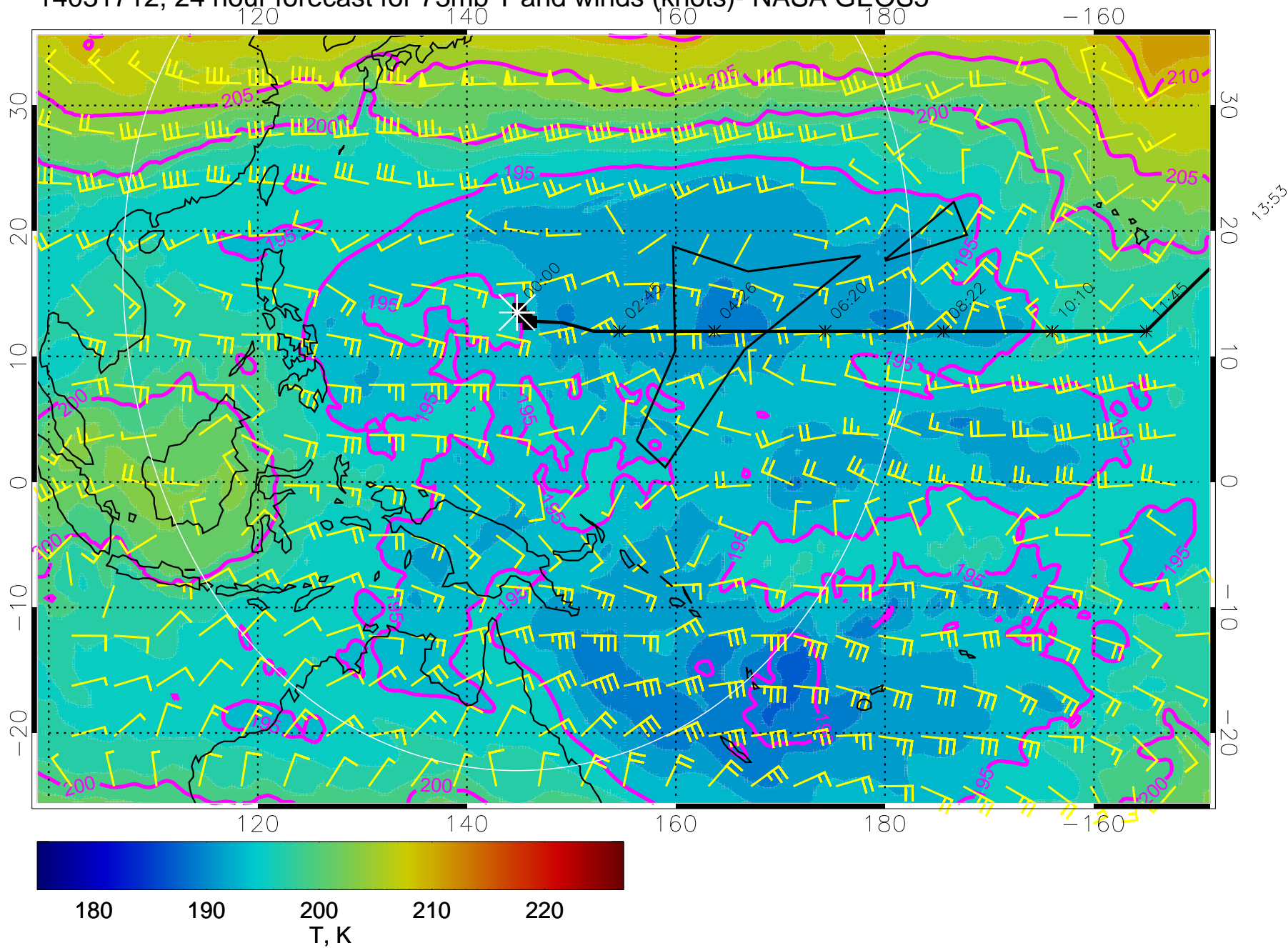
14031712, 24 hour forecast for 73mb T and winds (knots)- NASA GEOS5
