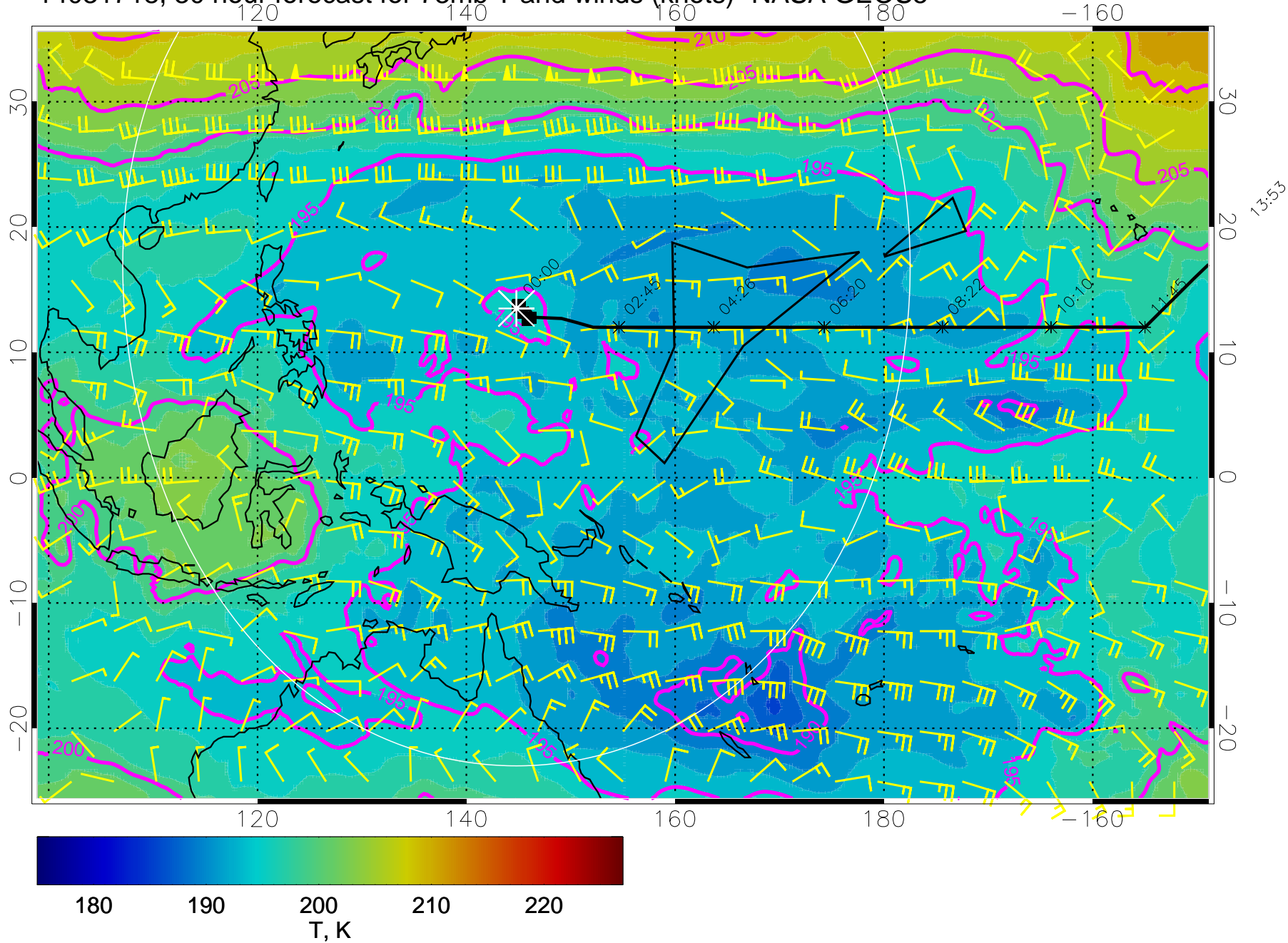
14031718, 30 hour forecast for 73mb T and winds (knots)- NASA GEOS5
