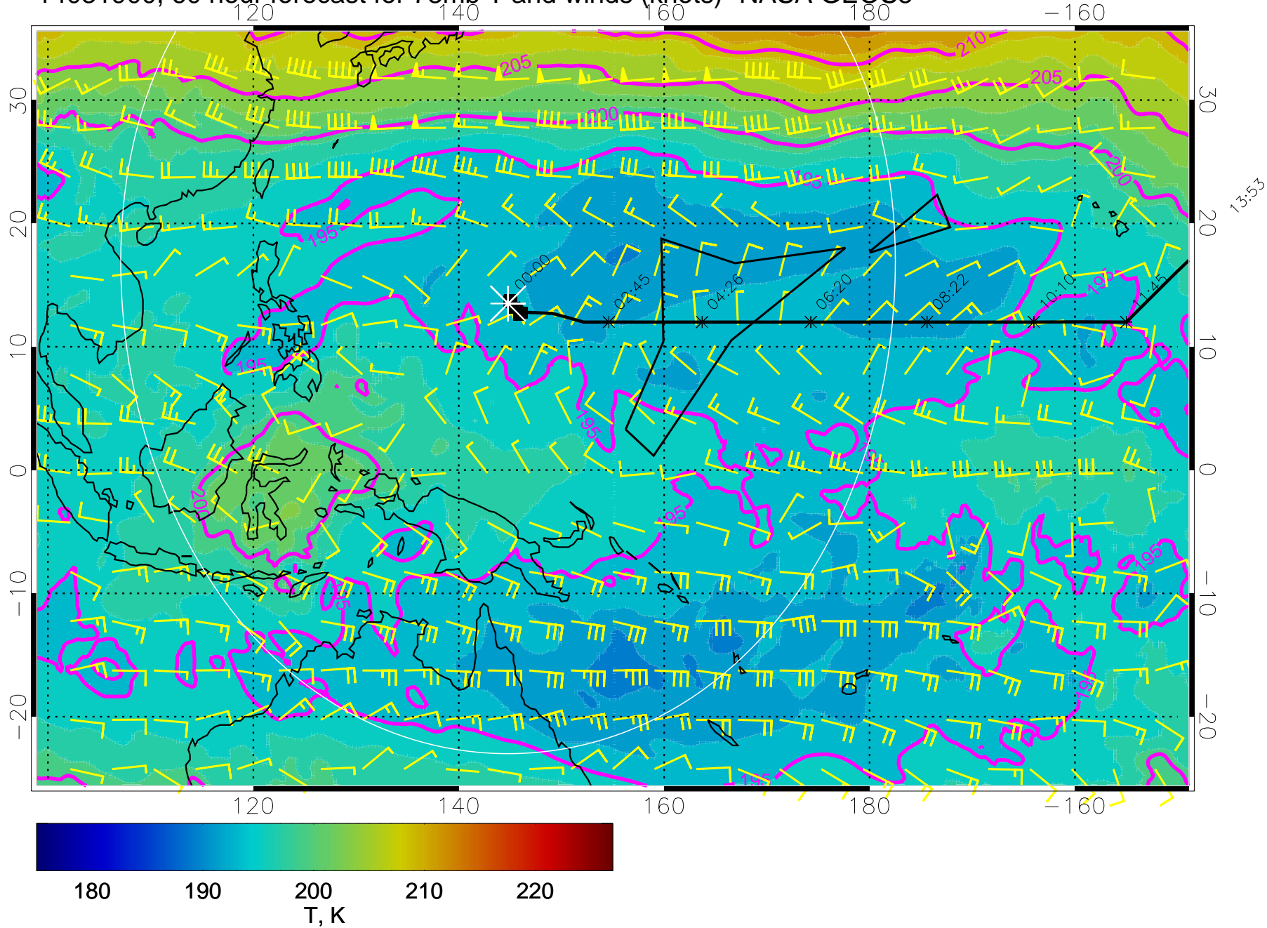
14031900, 60 hour forecast for 73mb T and winds (knots)- NASA GEOS5
