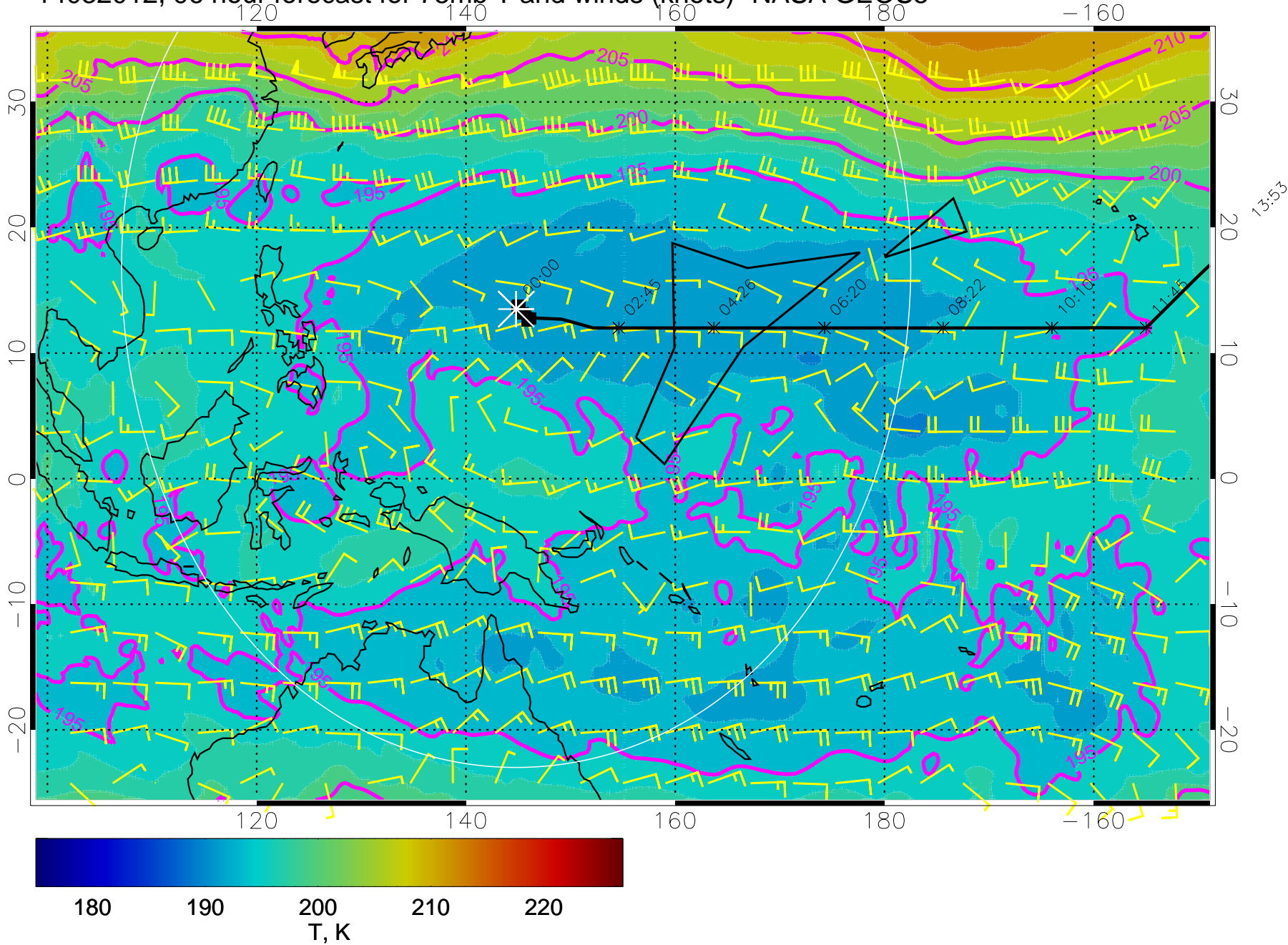
14032012, 96 hour forecast for 73mb T and winds (knots)- NASA GEOS5
