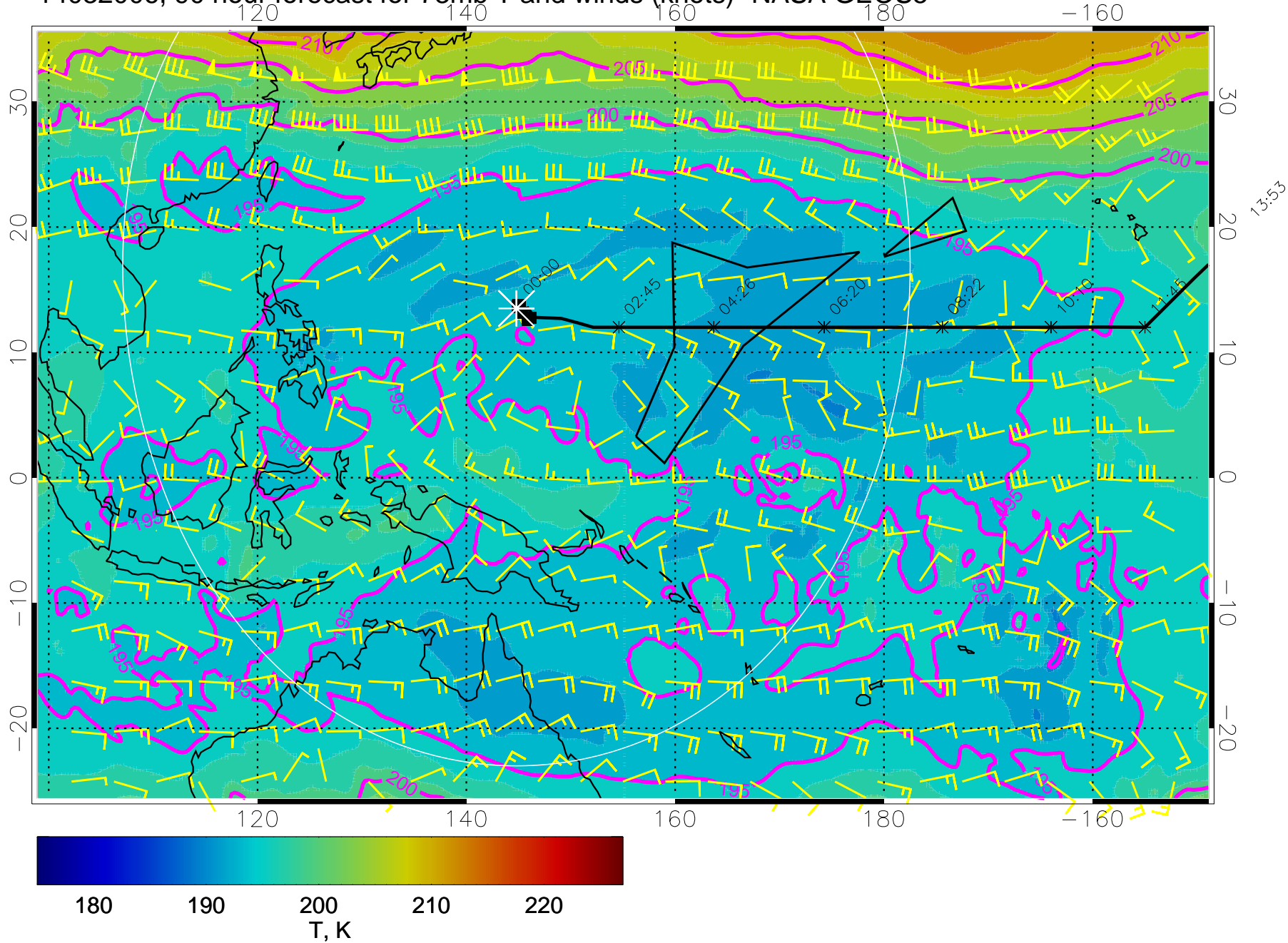
14032006, 90 hour forecast for 73mb T and winds (knots)- NASA GEOS5
