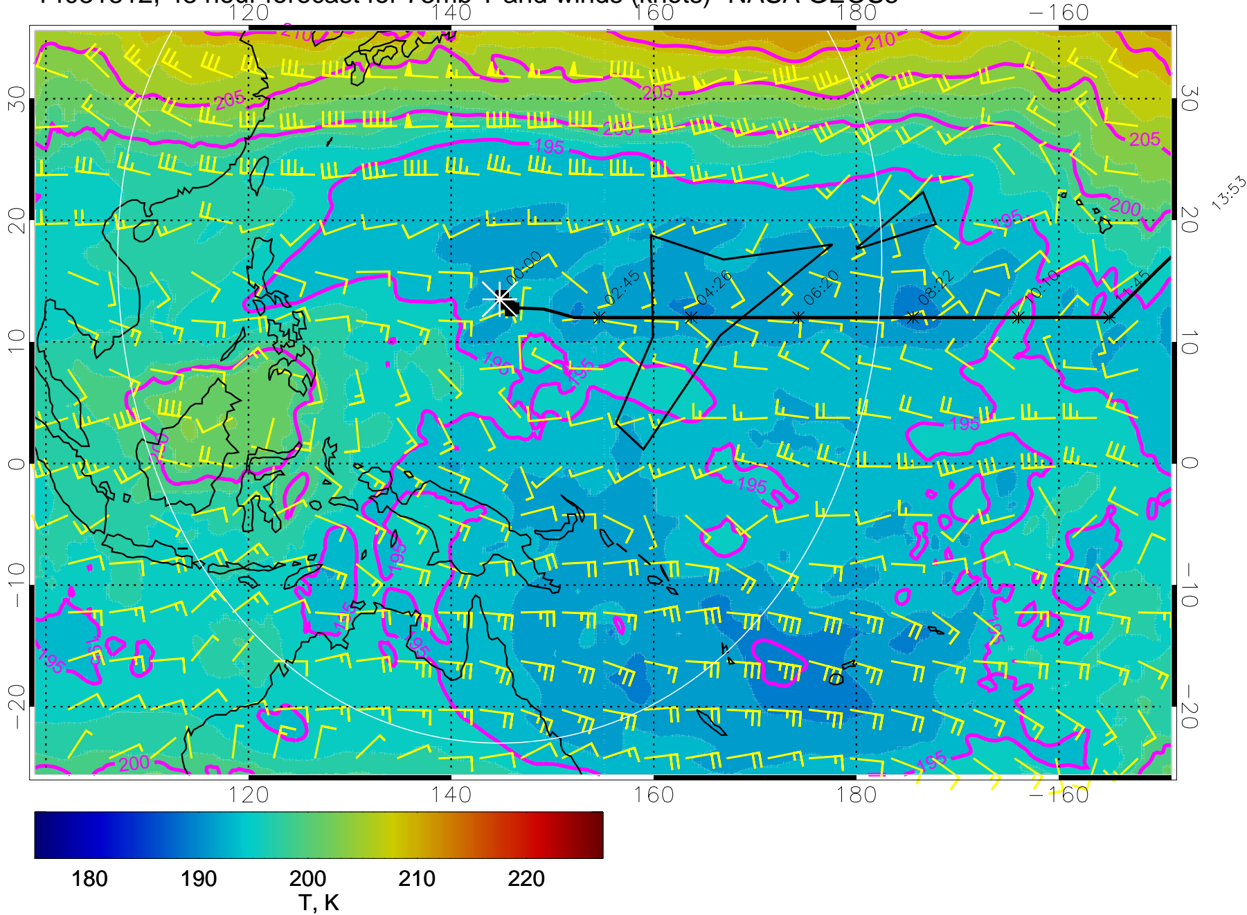
14031812, 48 hour forecast for 73mb T and winds (knots)- NASA GEOS5
