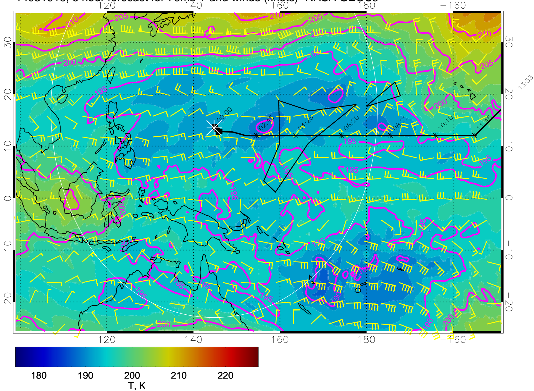
14031618, 6 hour forecast for 73mb T and winds (knots)- NASA GEOS5
