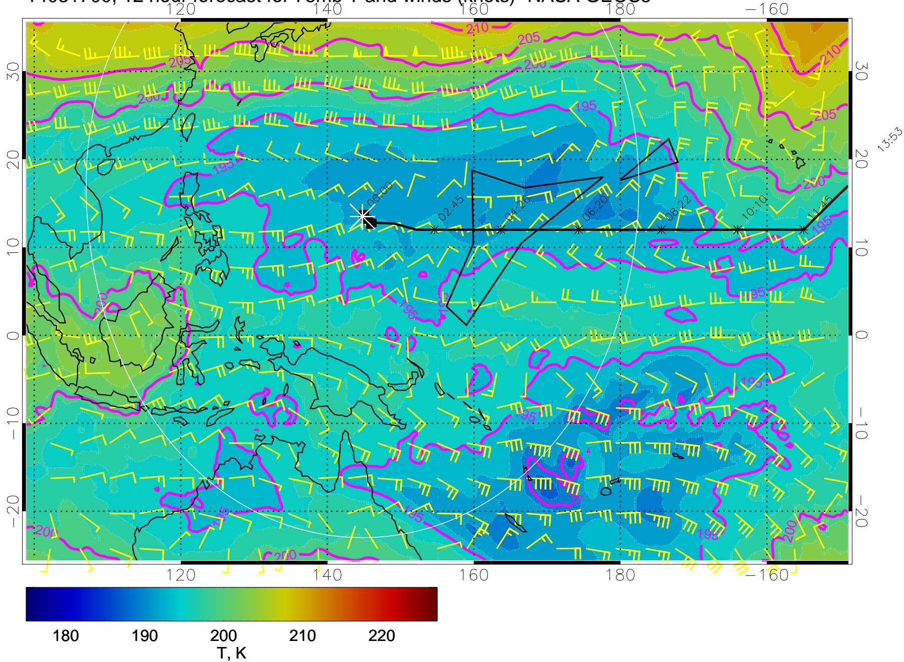
14031700, 12 hour forecast for 73mb T and winds (knots)- NASA GEOS5
