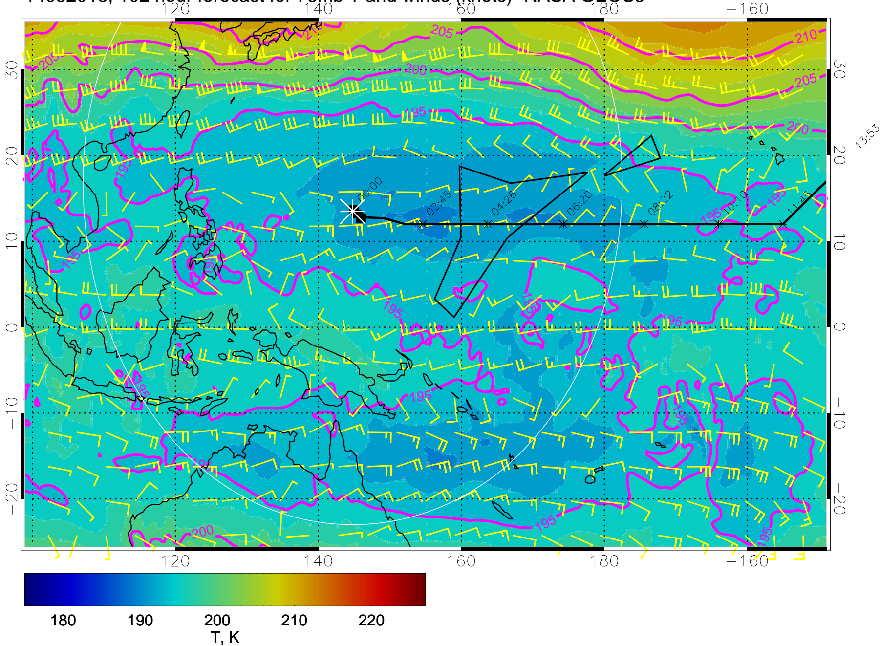
14032018, 102 hour forecast for 73mb T and winds (knots)- NASA GEOS5
