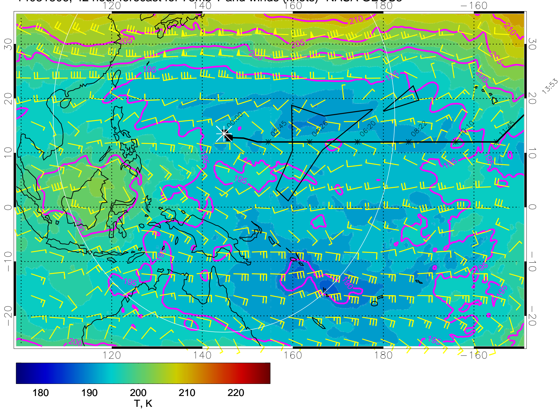
14031806, 42 hour forecast for 73mb T and winds (knots)- NASA GEOS5
