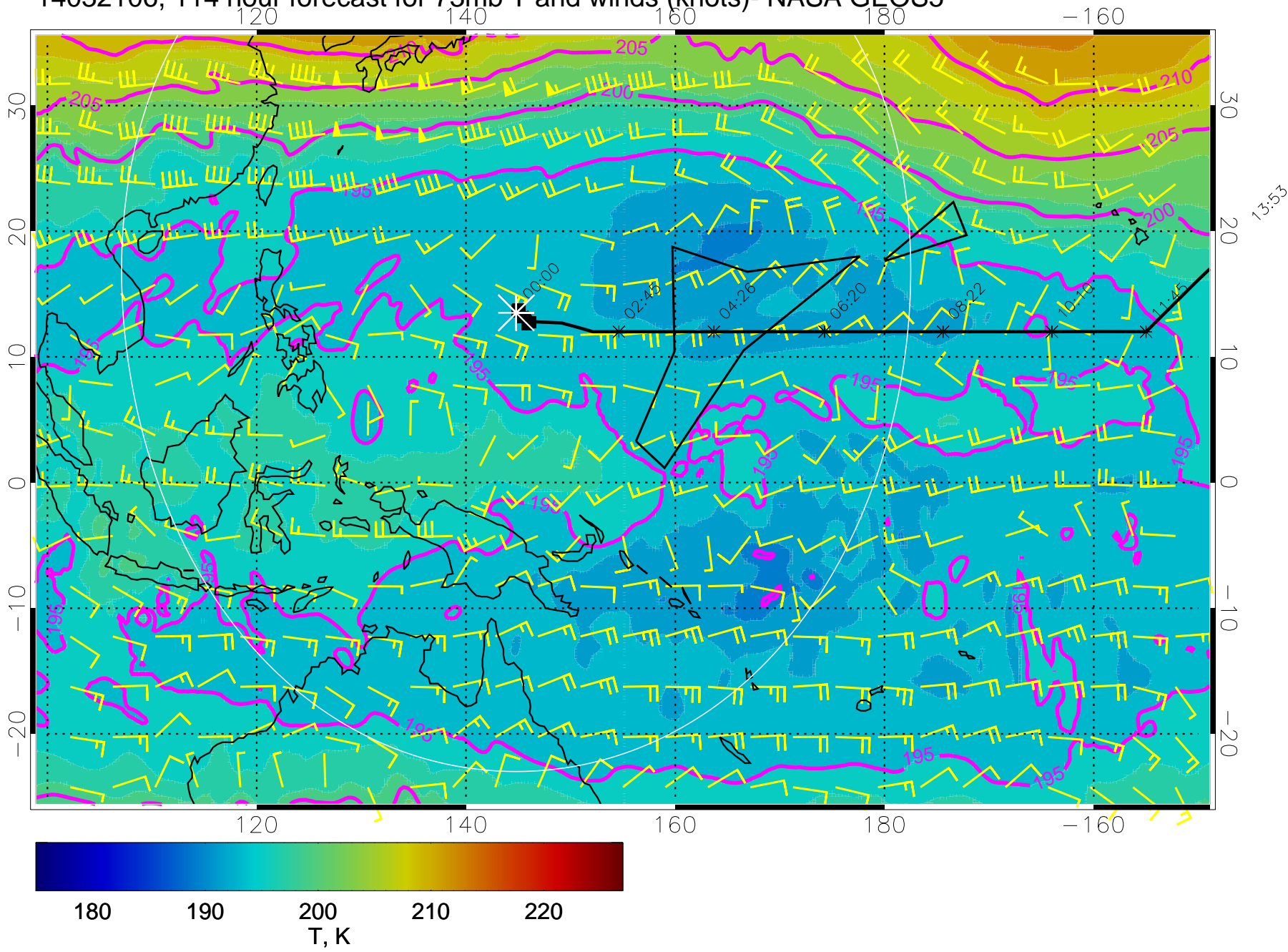
14032106, 114 hour forecast for 73mb T and winds (knots)- NASA GEOS5
