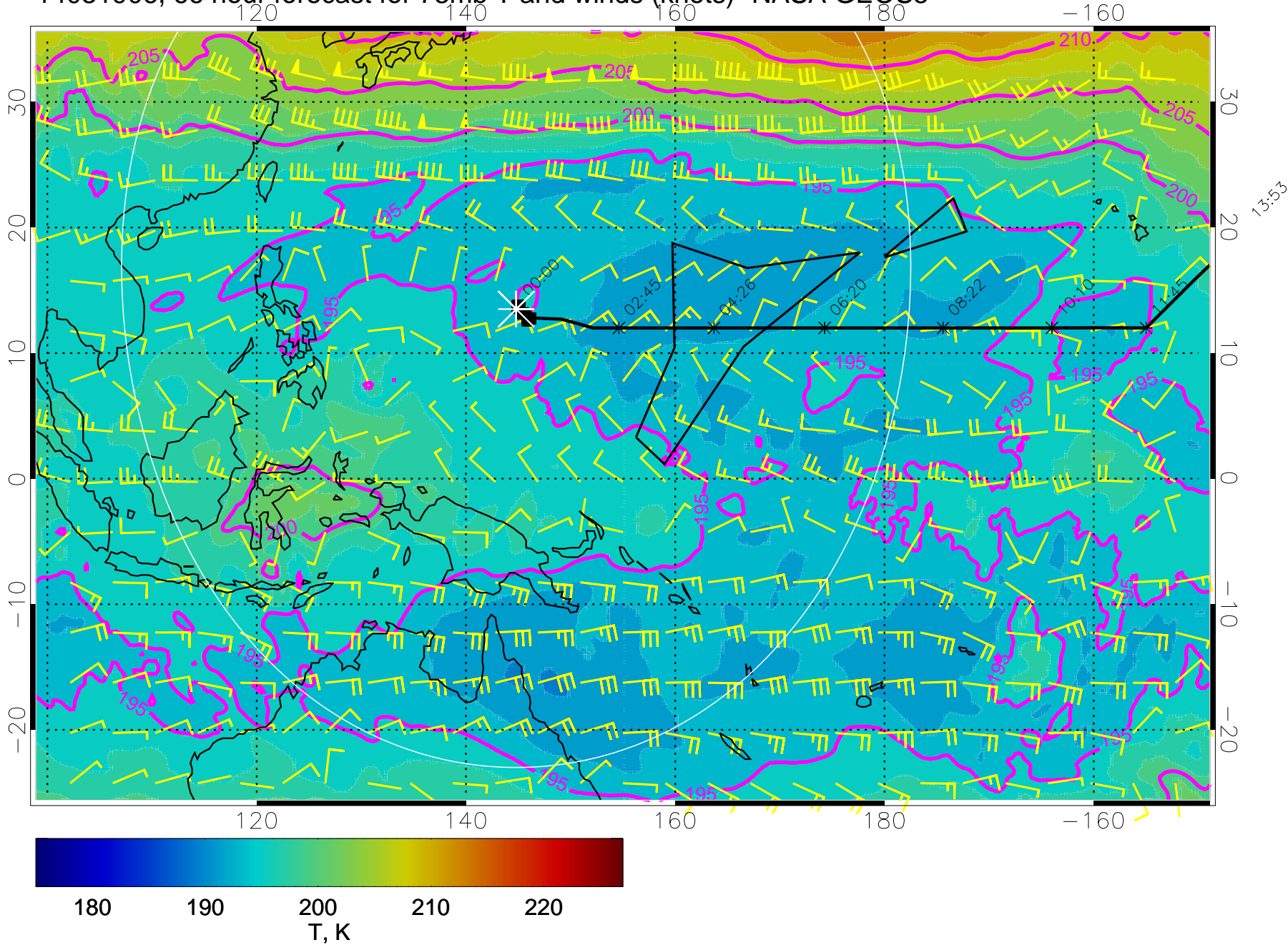
14031906, 66 hour forecast for 73mb T and winds (knots)- NASA GEOS5
