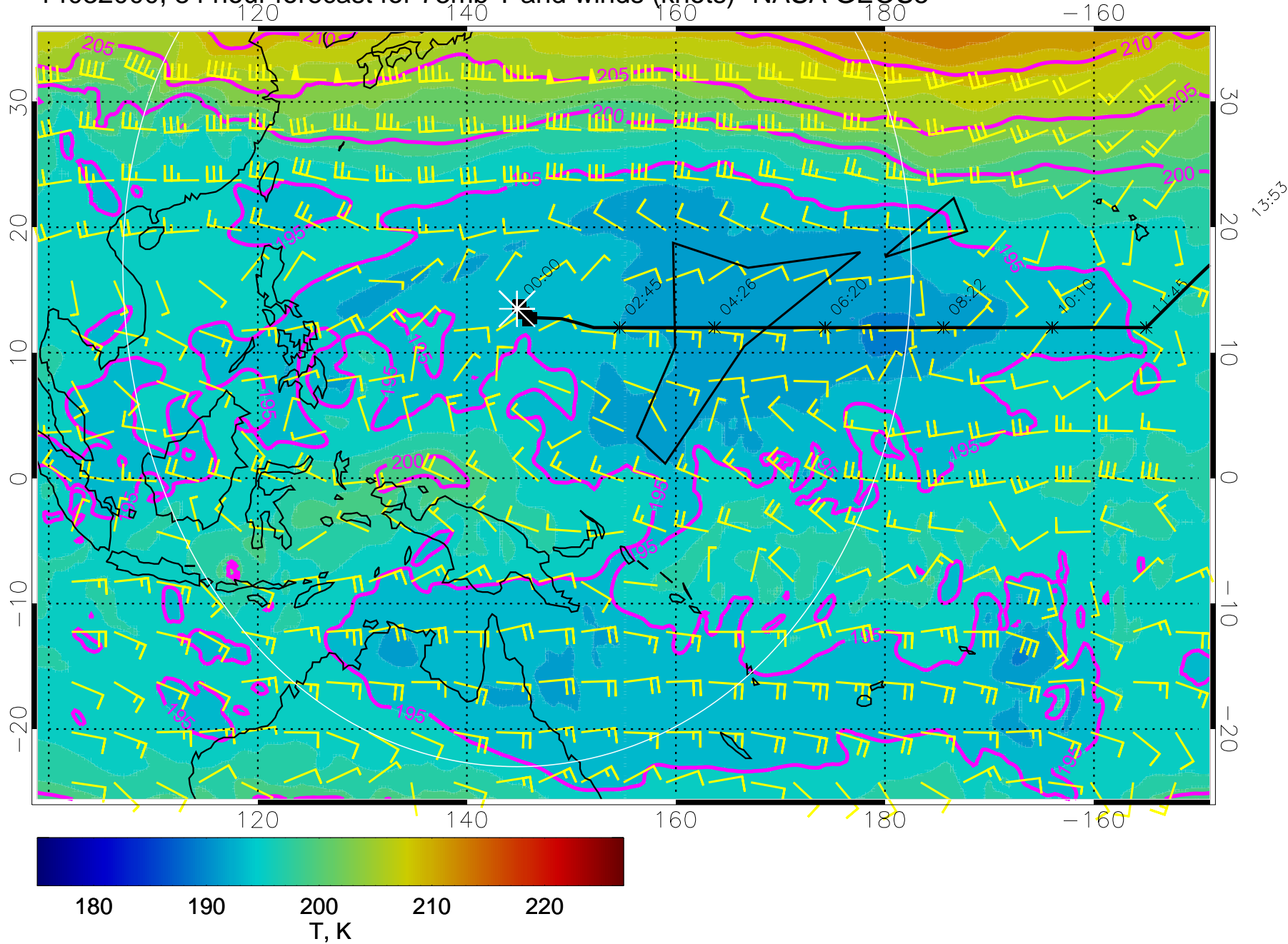
14032000, 84 hour forecast for 73mb T and winds (knots)- NASA GEOS5
