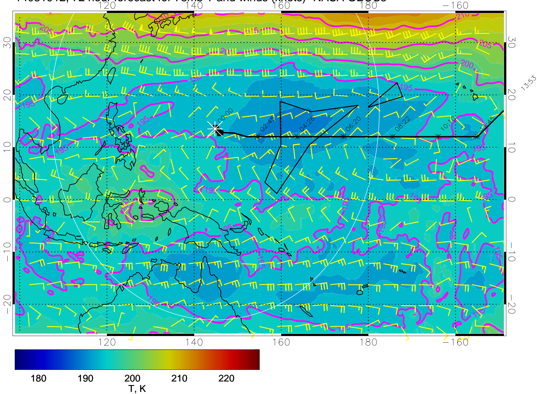
14031912, 72 hour forecast for 73mb T and winds (knots)- NASA GEOS5
