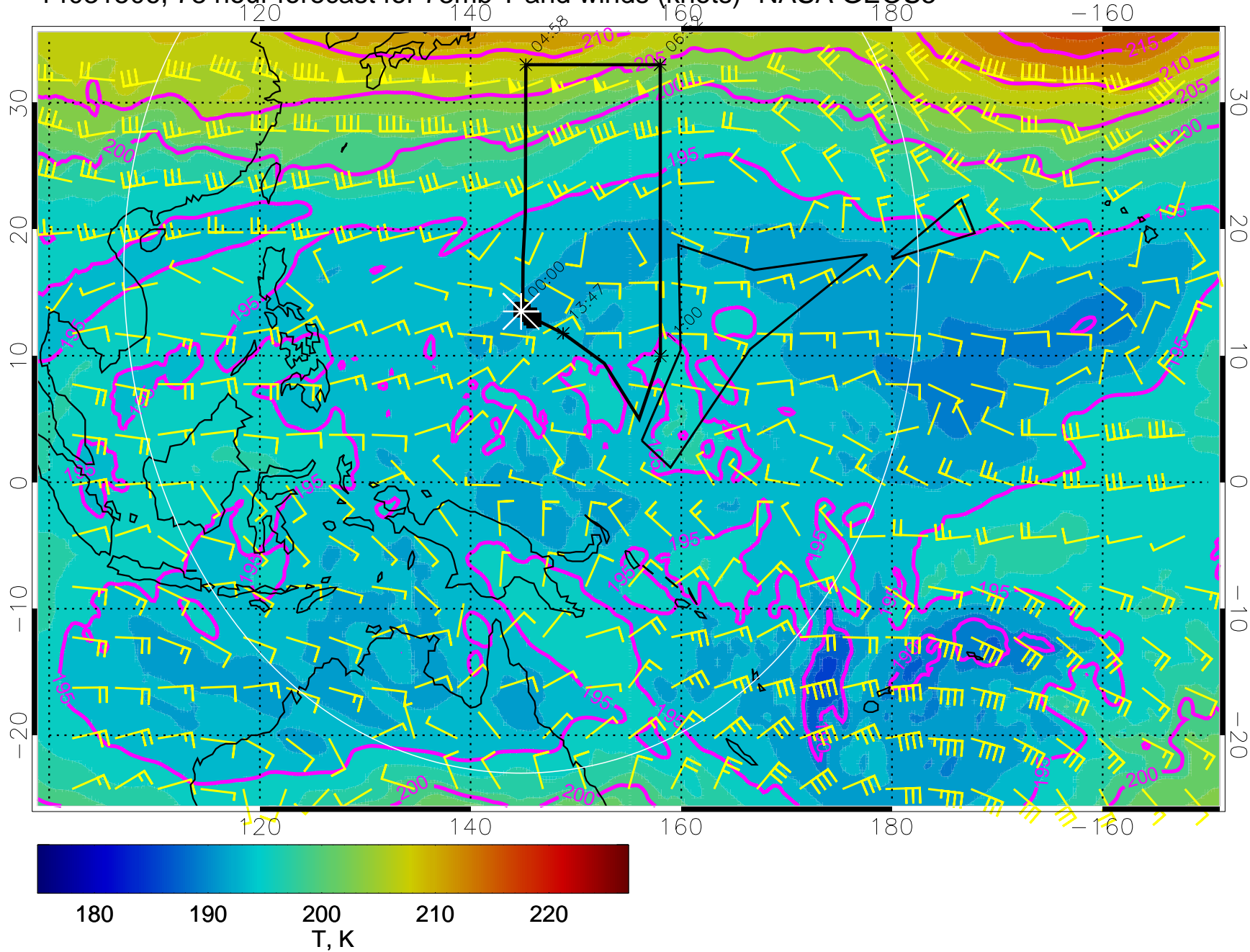
14031506, 78 hour forecast for 73mb T and winds (knots)- NASA GEOS5
