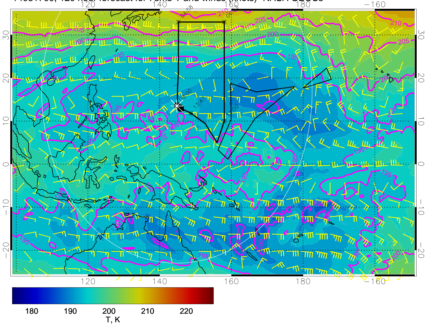
14031700, 120 hour forecast for 73mb T and winds (knots)- NASA GEOS5
