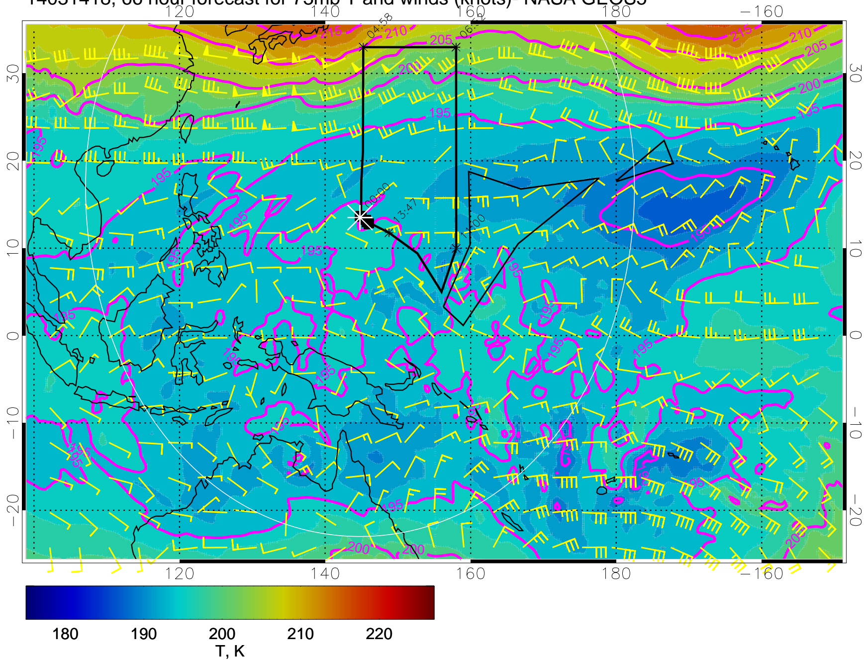
14031418, 66 hour forecast for 73mb T and winds (knots)- NASA GEOS5
