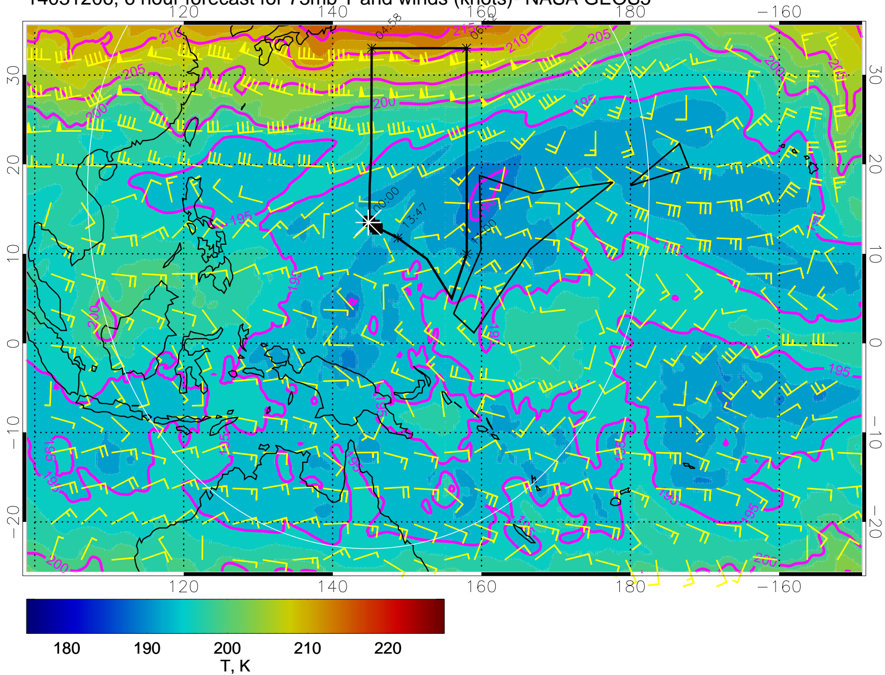
14031206, 6 hour forecast for 73mb T and winds (knots)- NASA GEOS5
