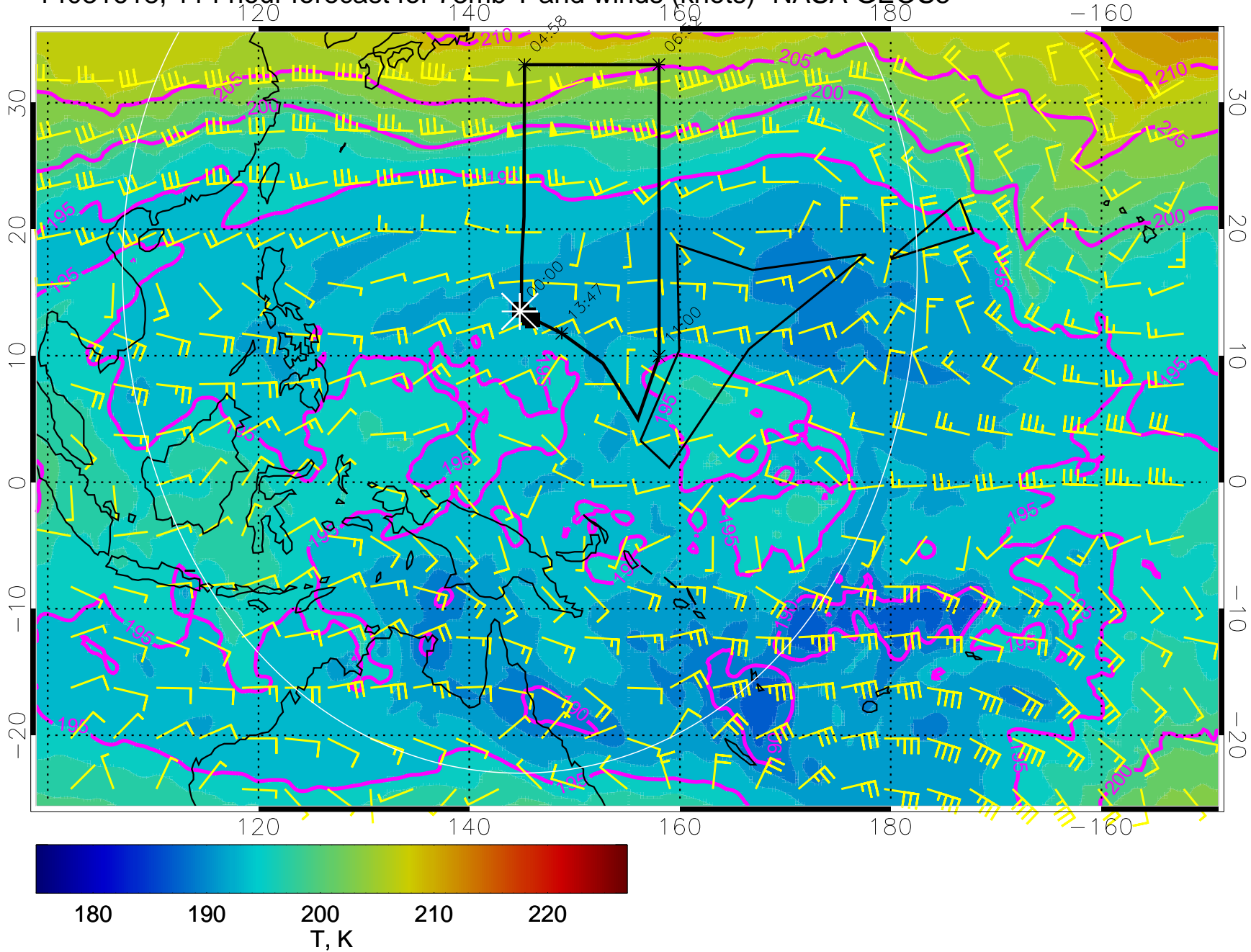
14031618, 114 hour forecast for 73mb T and winds (knots)- NASA GEOS5
