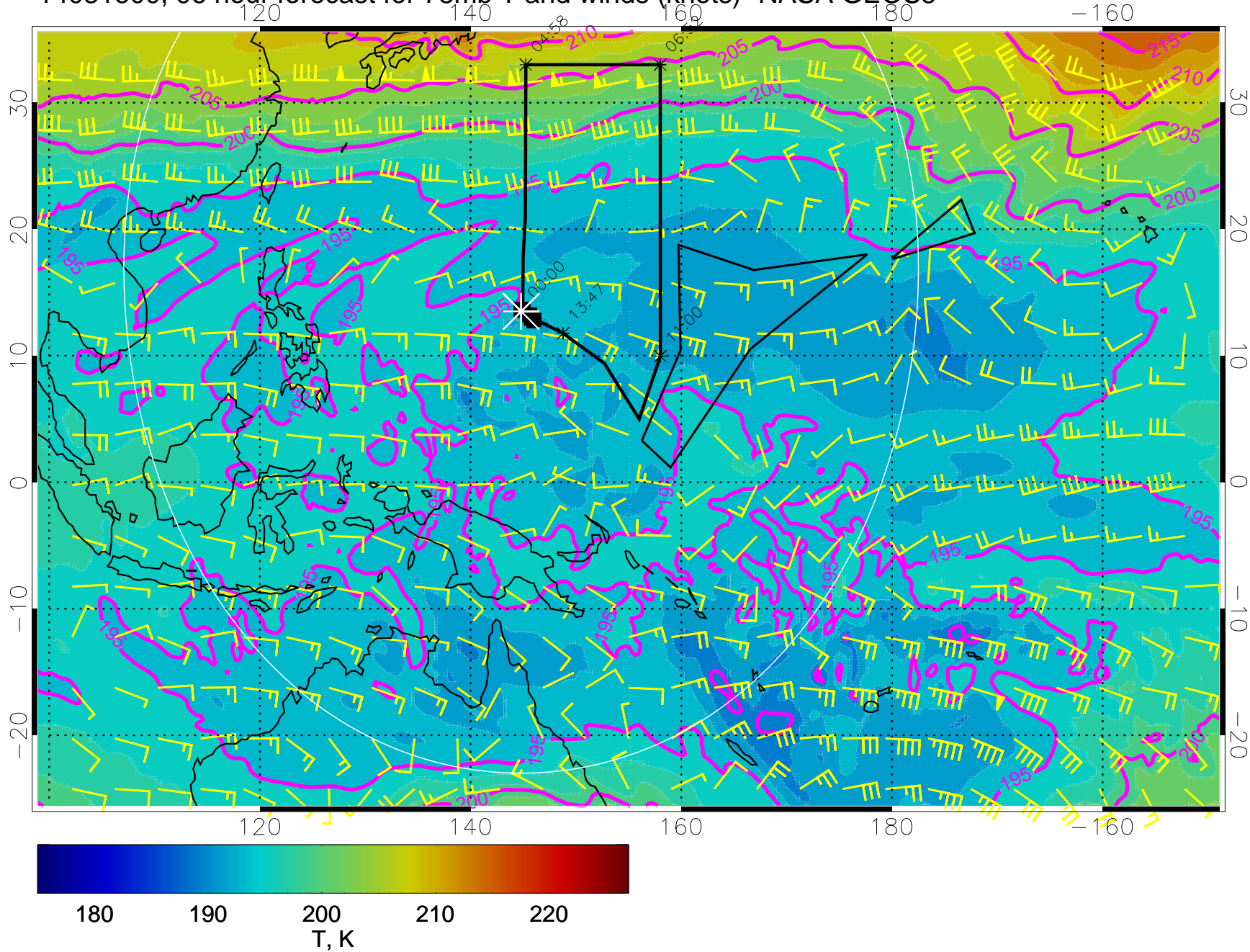
14031600, 96 hour forecast for 73mb T and winds (knots)- NASA GEOS5
