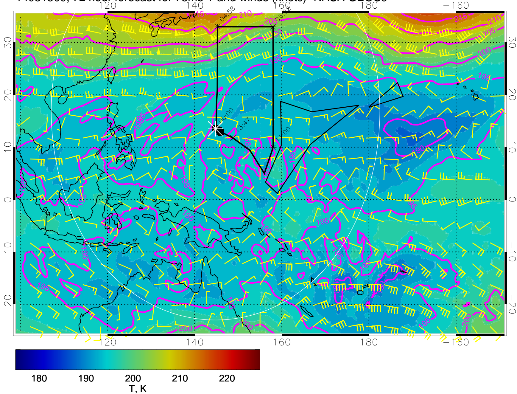
14031500, 72 hour forecast for 73mb T and winds (knots)- NASA GEOS5
