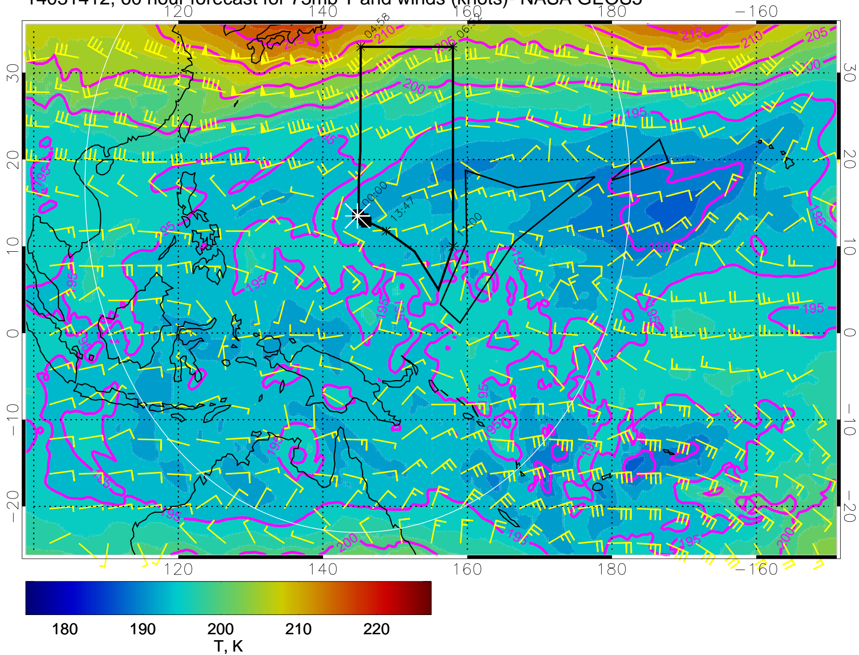
14031412, 60 hour forecast for 73mb T and winds (knots)- NASA GEOS5
