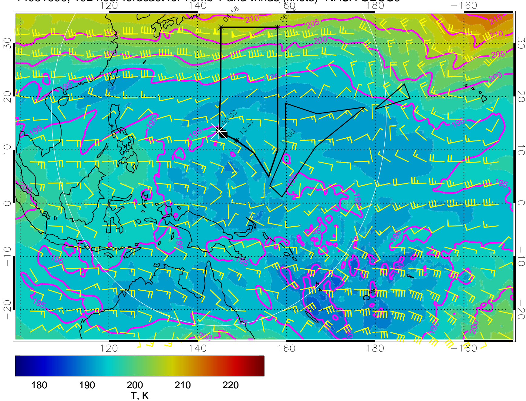
14031606, 102 hour forecast for 73mb T and winds (knots)- NASA GEOS5
