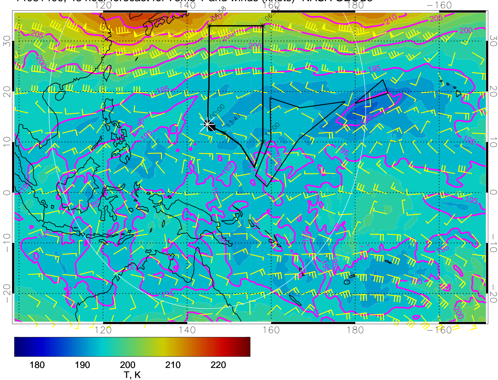
14031400, 48 hour forecast for 73mb T and winds (knots)- NASA GEOS5
