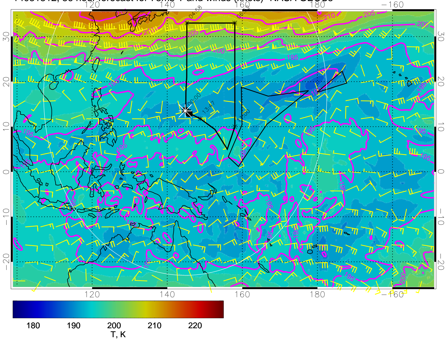
14031312, 36 hour forecast for 73mb T and winds (knots)- NASA GEOS5
