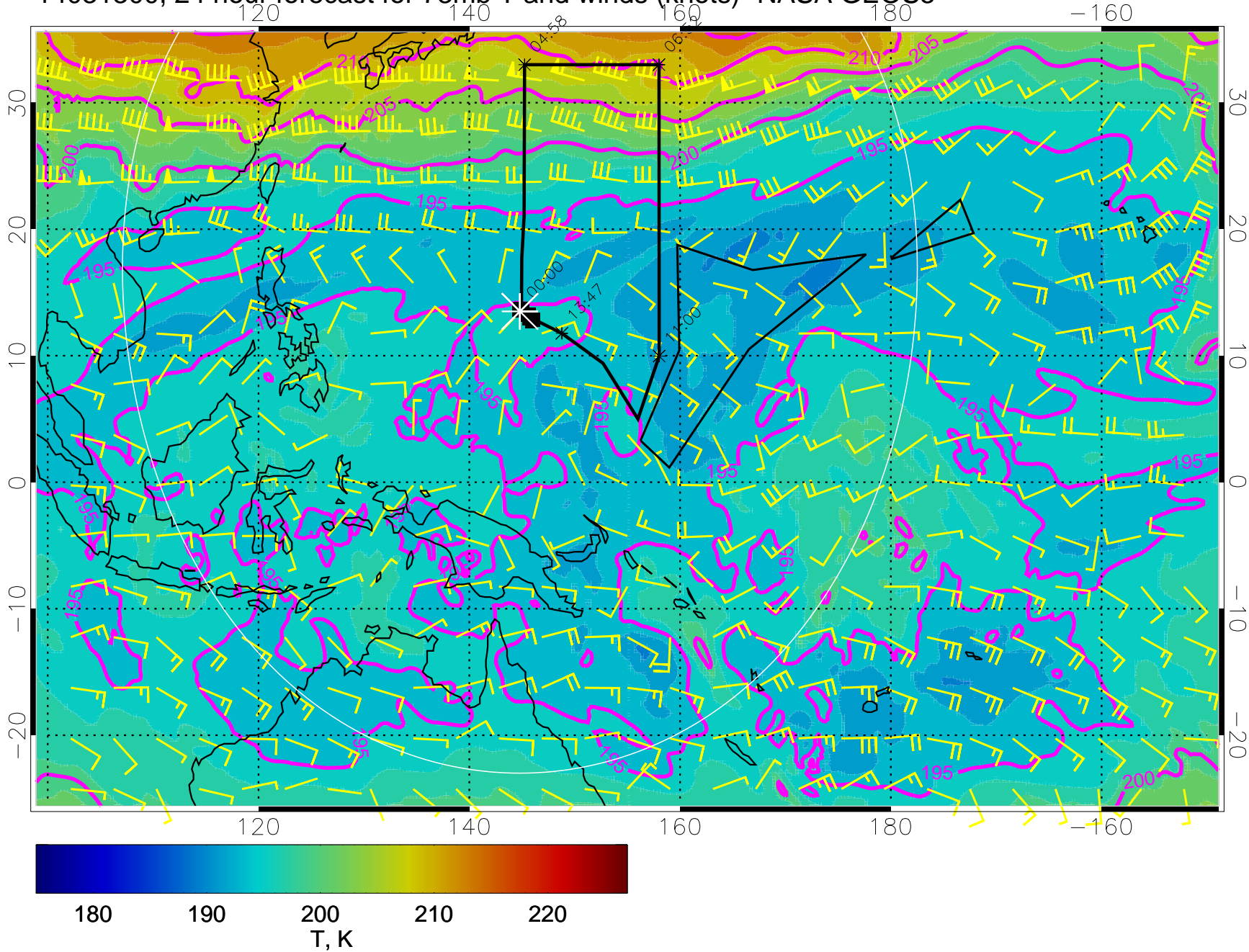
14031300, 24 hour forecast for 73mb T and winds (knots)- NASA GEOS5
