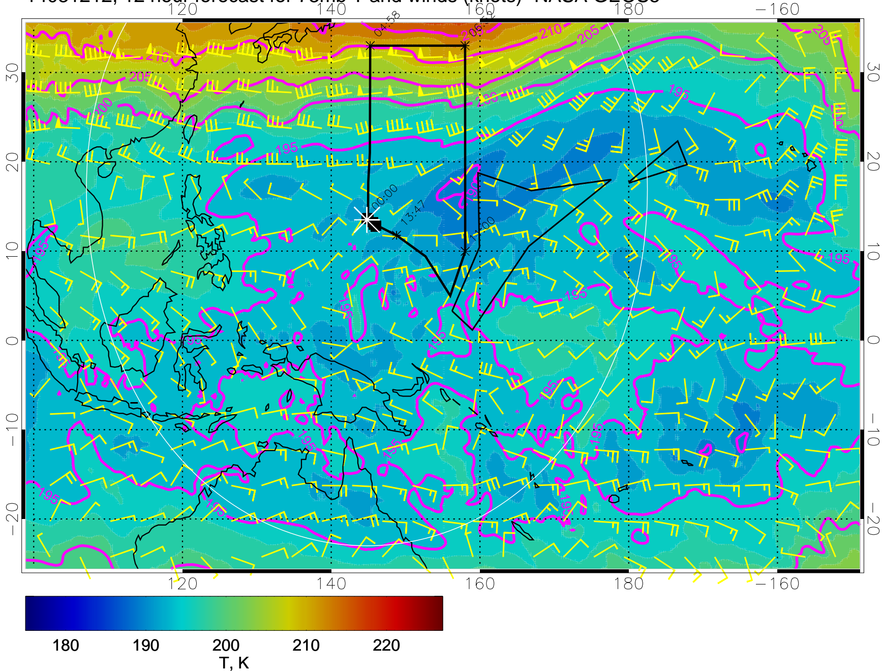
14031212, 12 hour forecast for 73mb T and winds (knots)- NASA GEOS5
