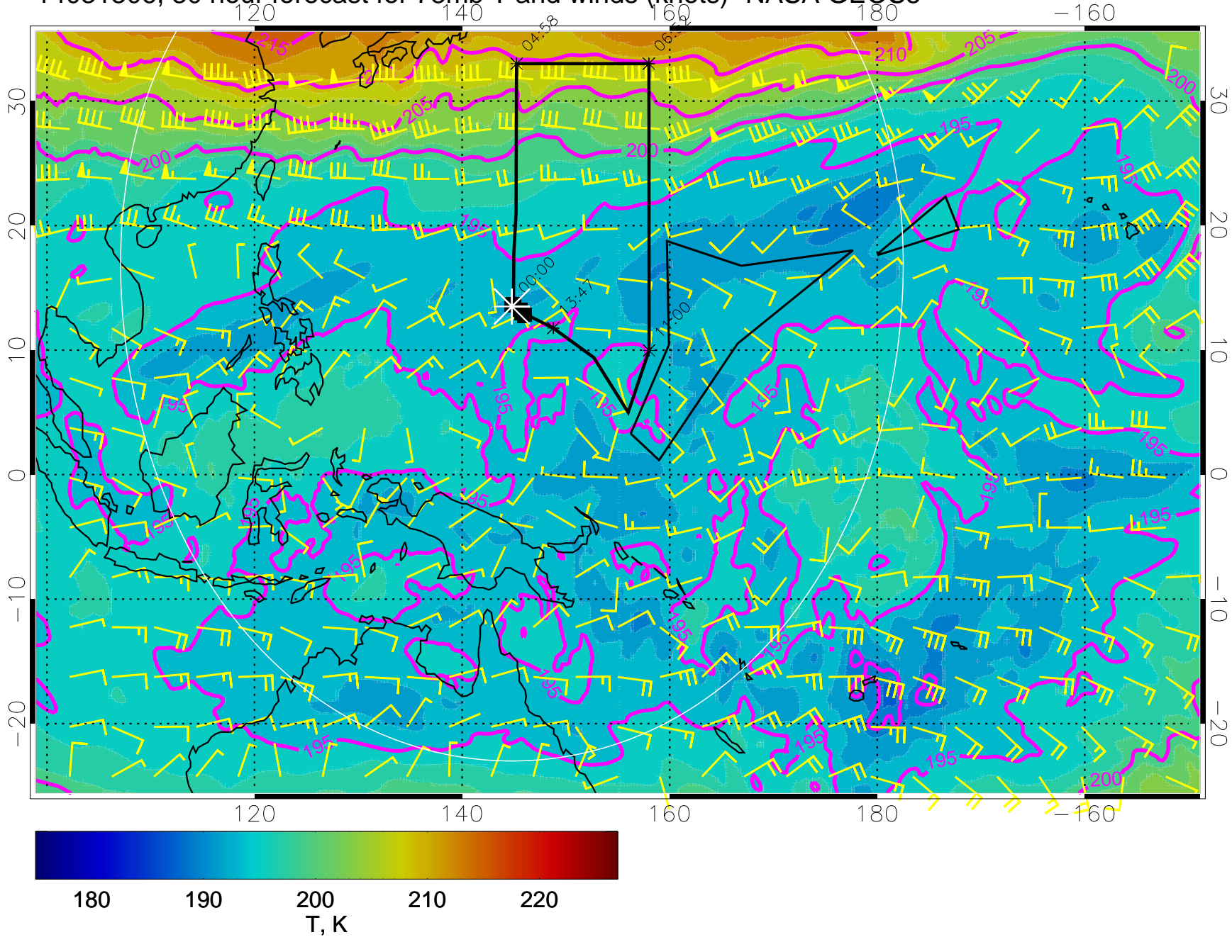
14031306, 30 hour forecast for 73mb T and winds (knots)- NASA GEOS5
