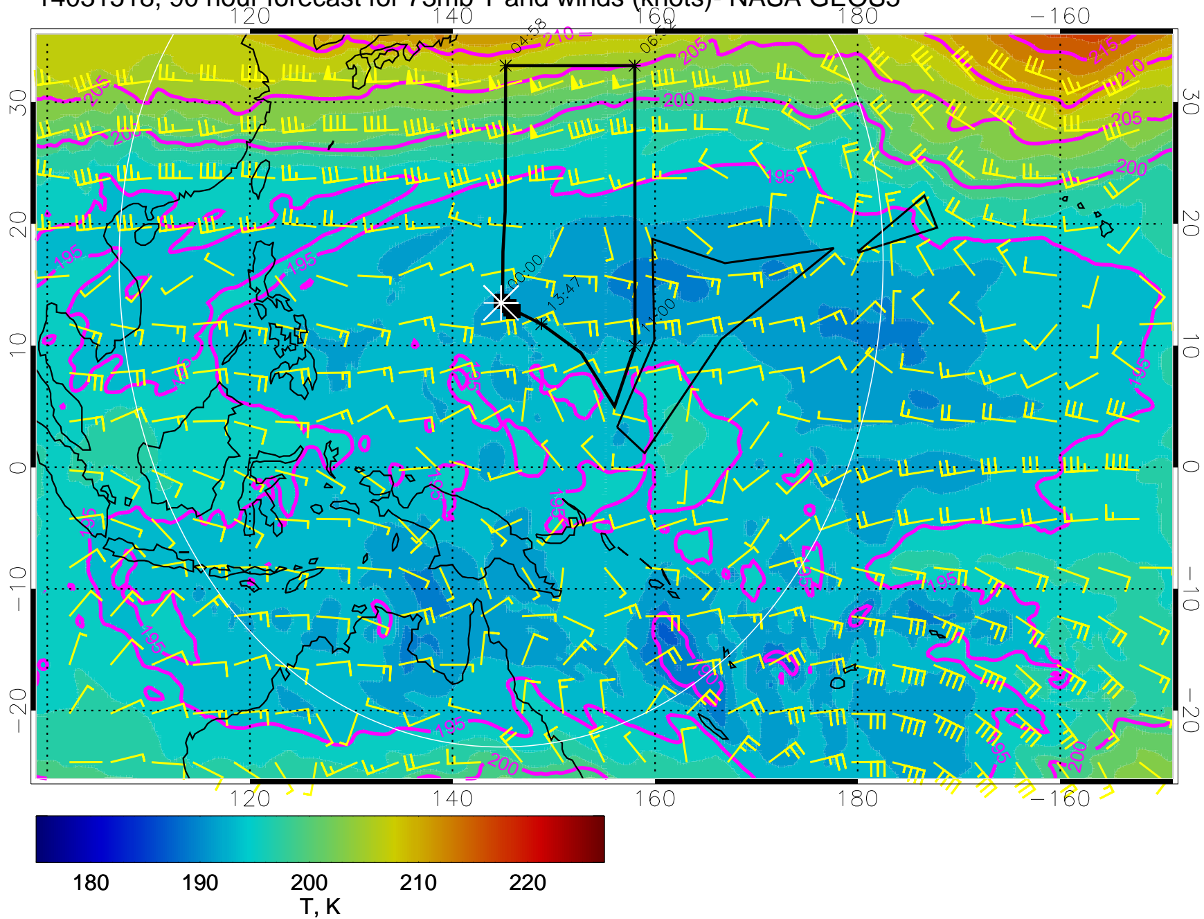
14031518, 90 hour forecast for 73mb T and winds (knots)- NASA GEOS5
