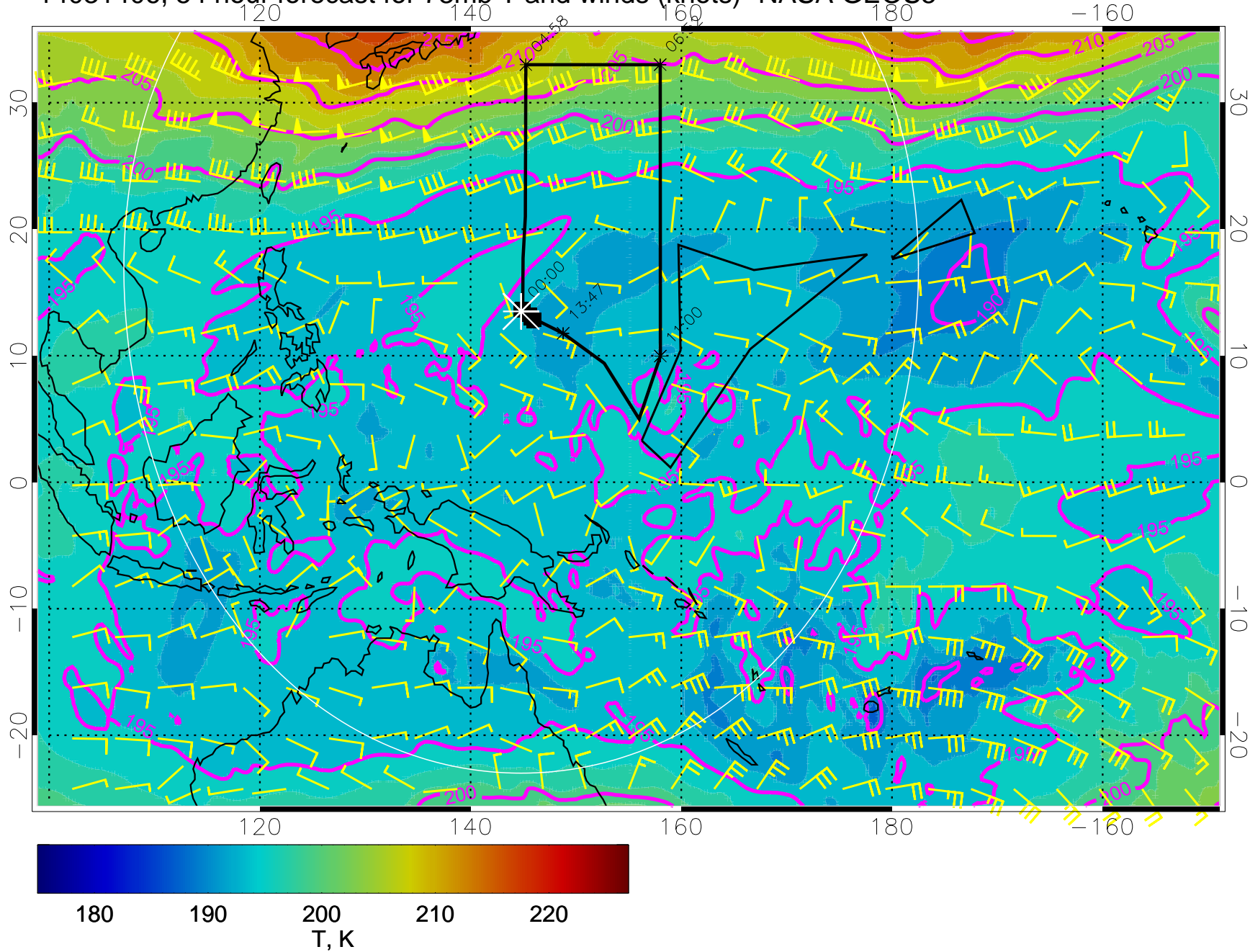
14031406, 54 hour forecast for 73mb T and winds (knots)- NASA GEOS5
