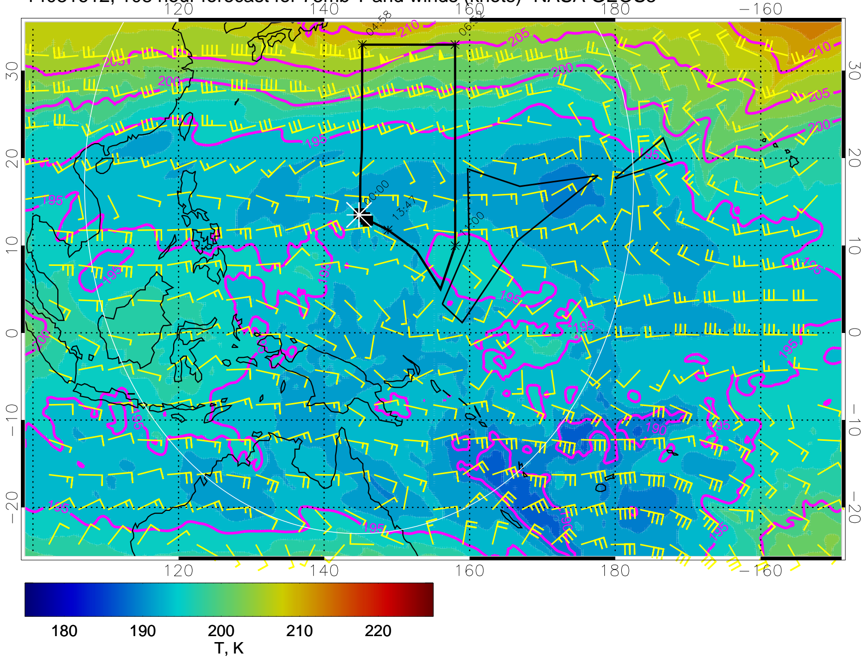
14031612, 108 hour forecast for 73mb T and winds (knots)- NASA GEOS5
