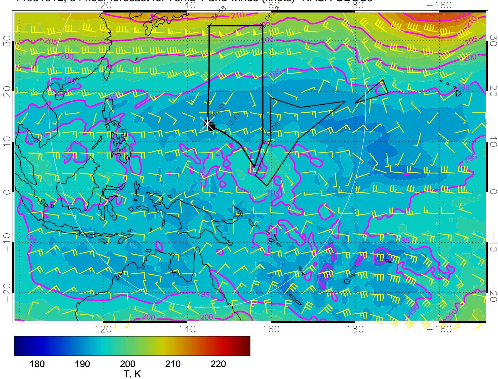
14031512, 84 hour forecast for 73mb T and winds (knots)- NASA GEOS5
