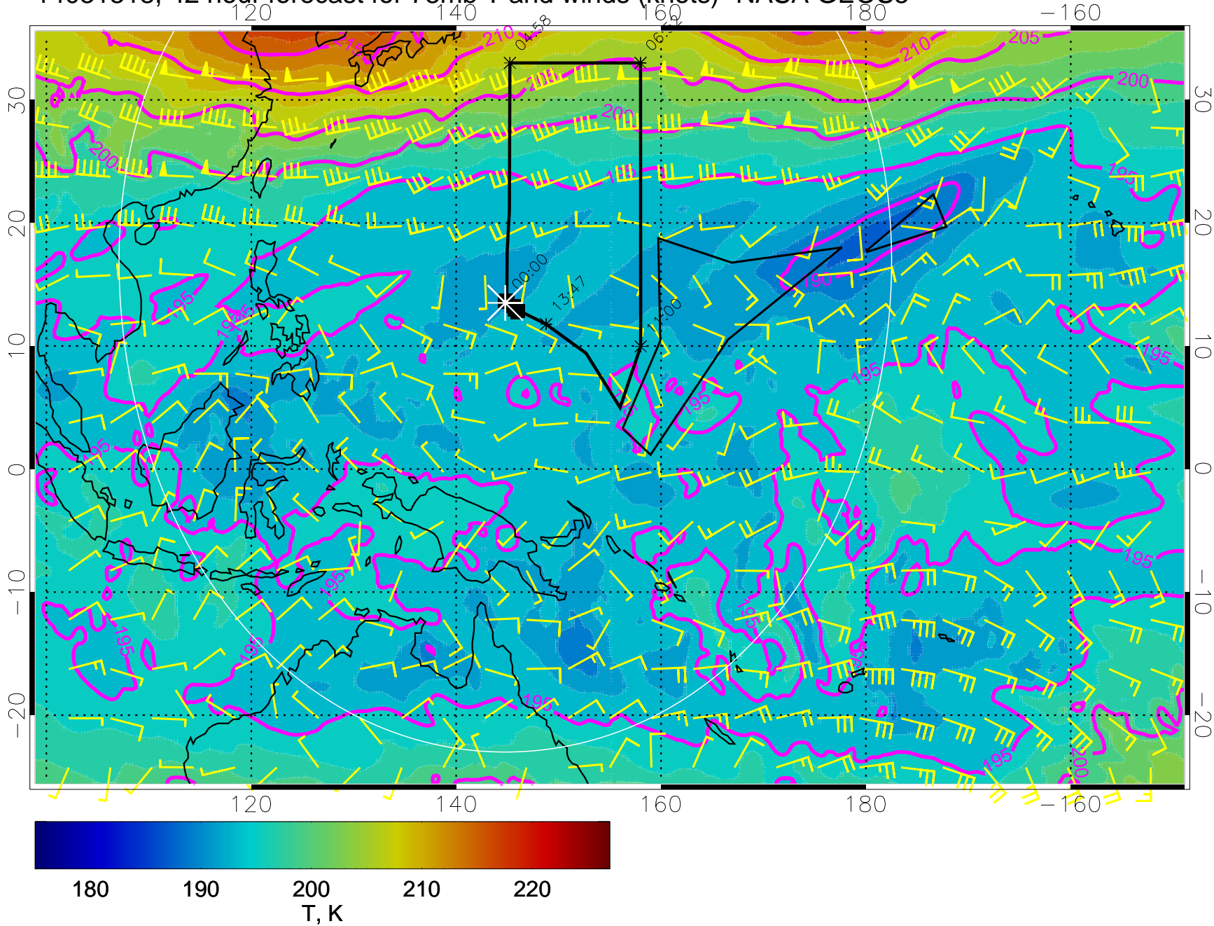
14031318, 42 hour forecast for 73mb T and winds (knots)- NASA GEOS5
