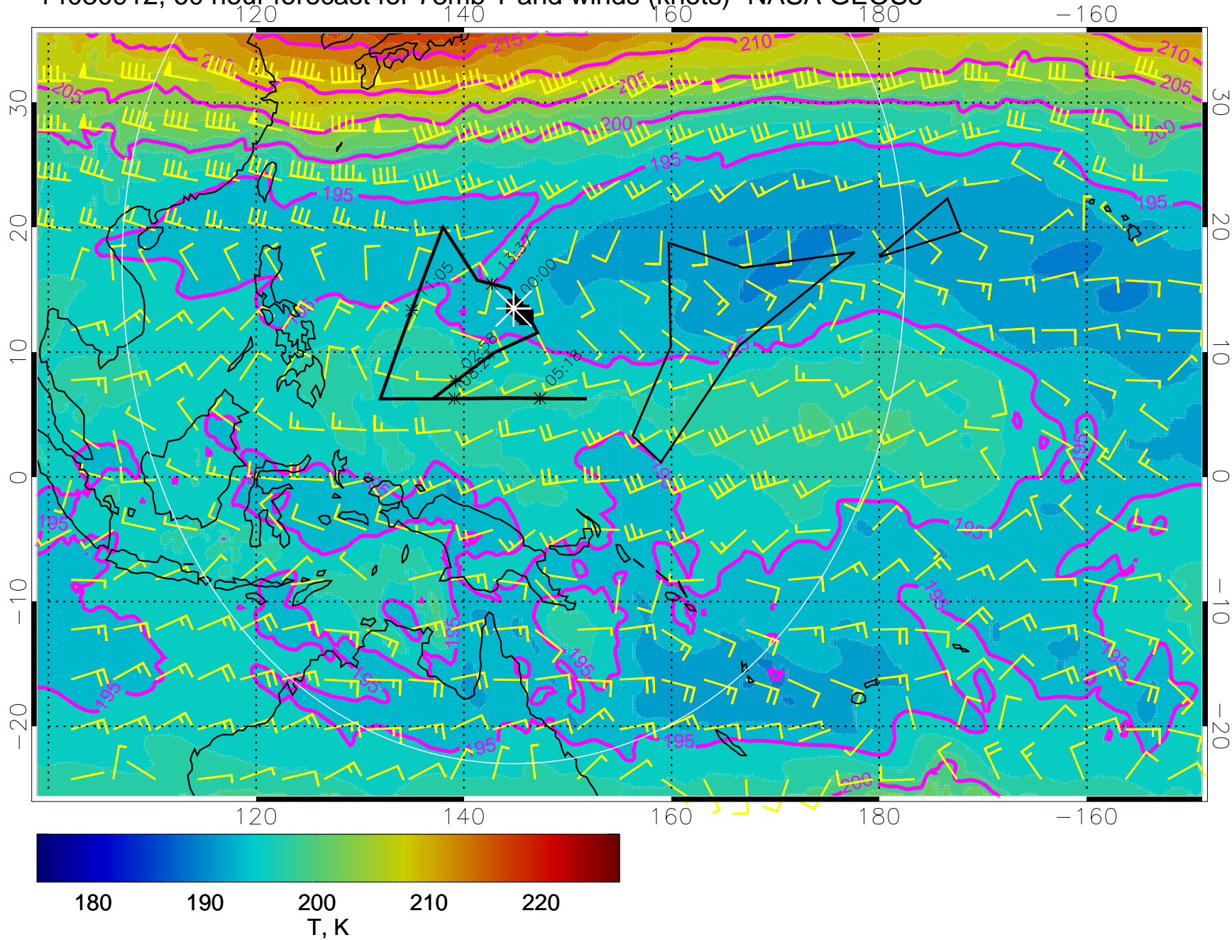
14030912, 60 hour forecast for 73mb T and winds (knots)- NASA GEOS5
