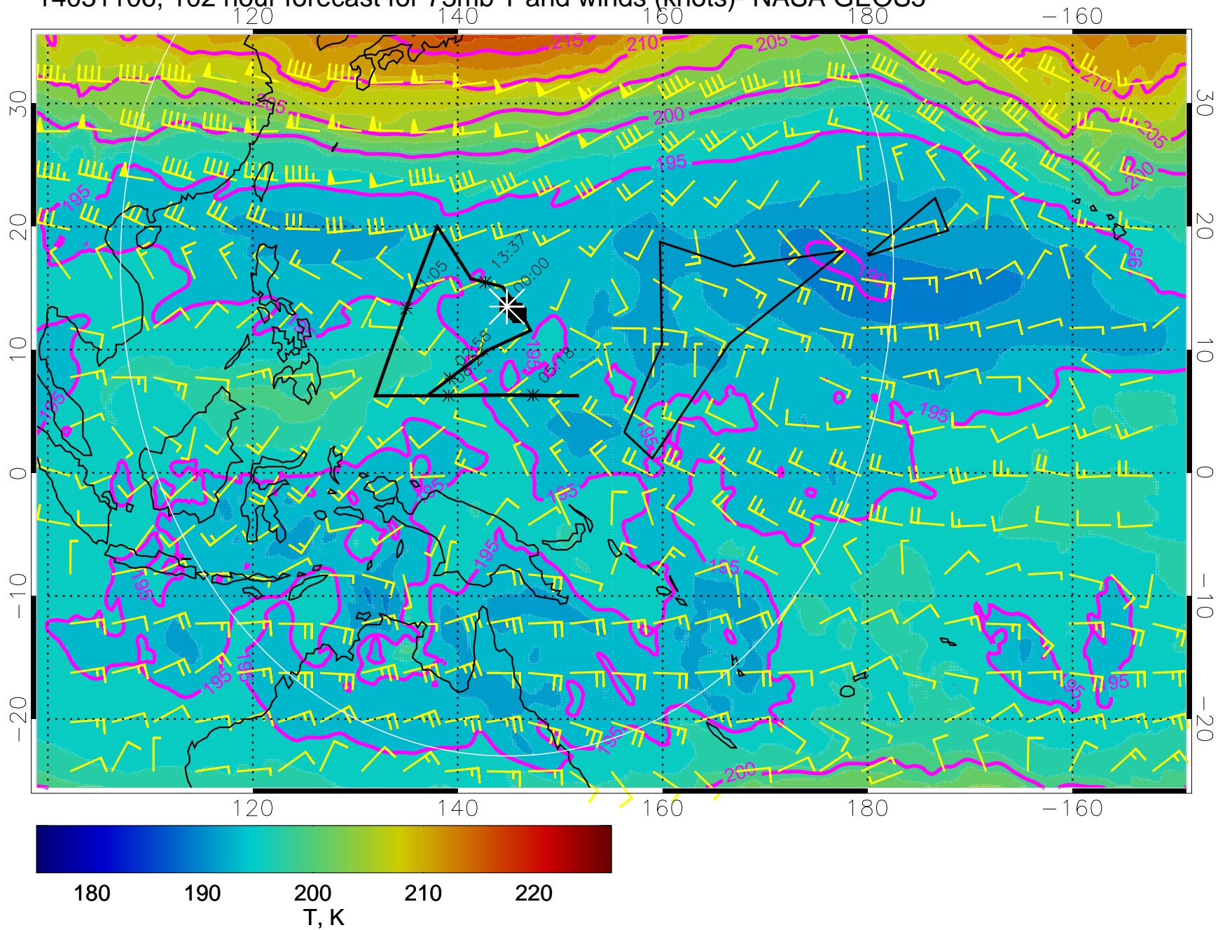
14031106, 102 hour forecast for 73mb T and winds (knots)- NASA GEOS5
