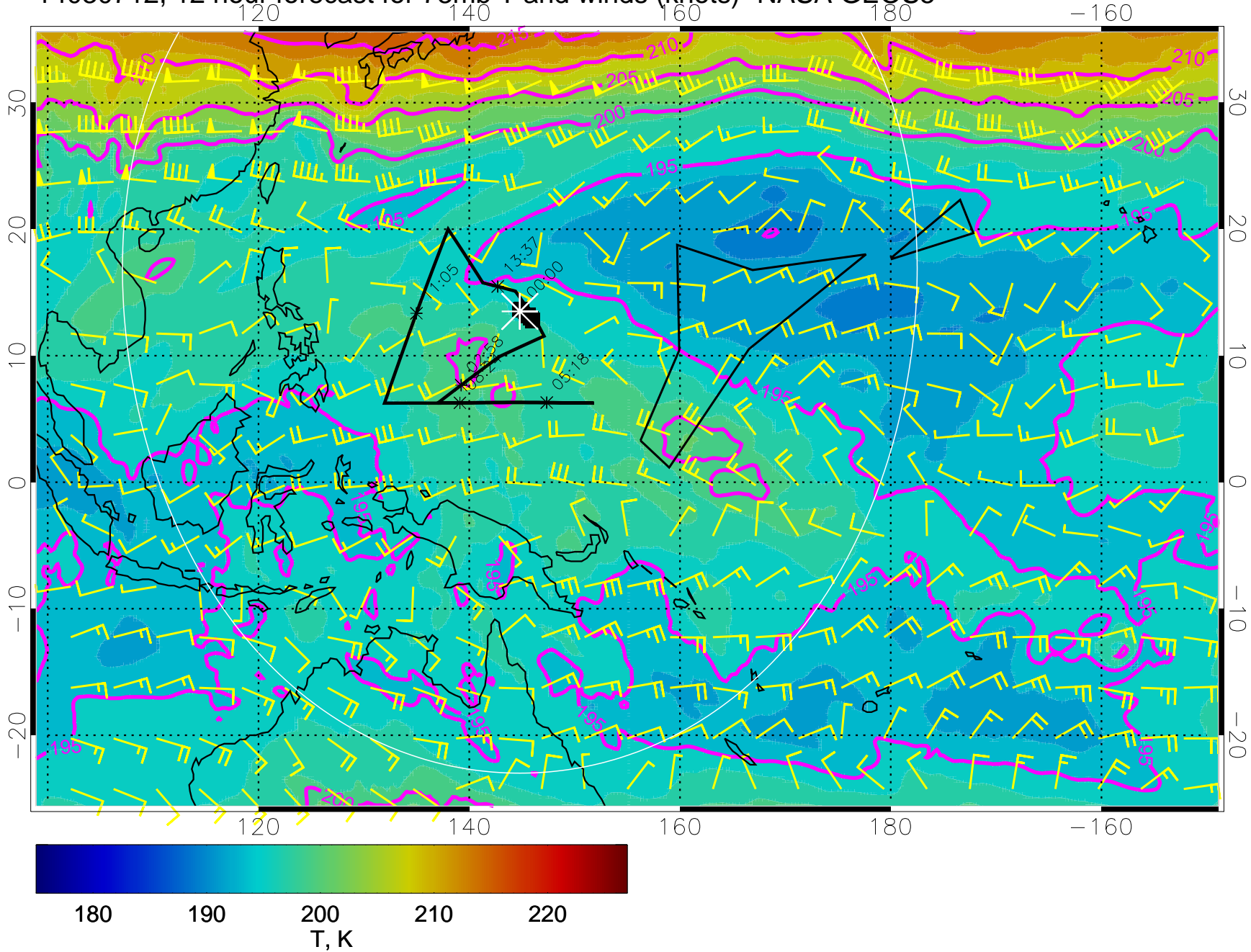
14030712, 12 hour forecast for 73mb T and winds (knots)- NASA GEOS5
