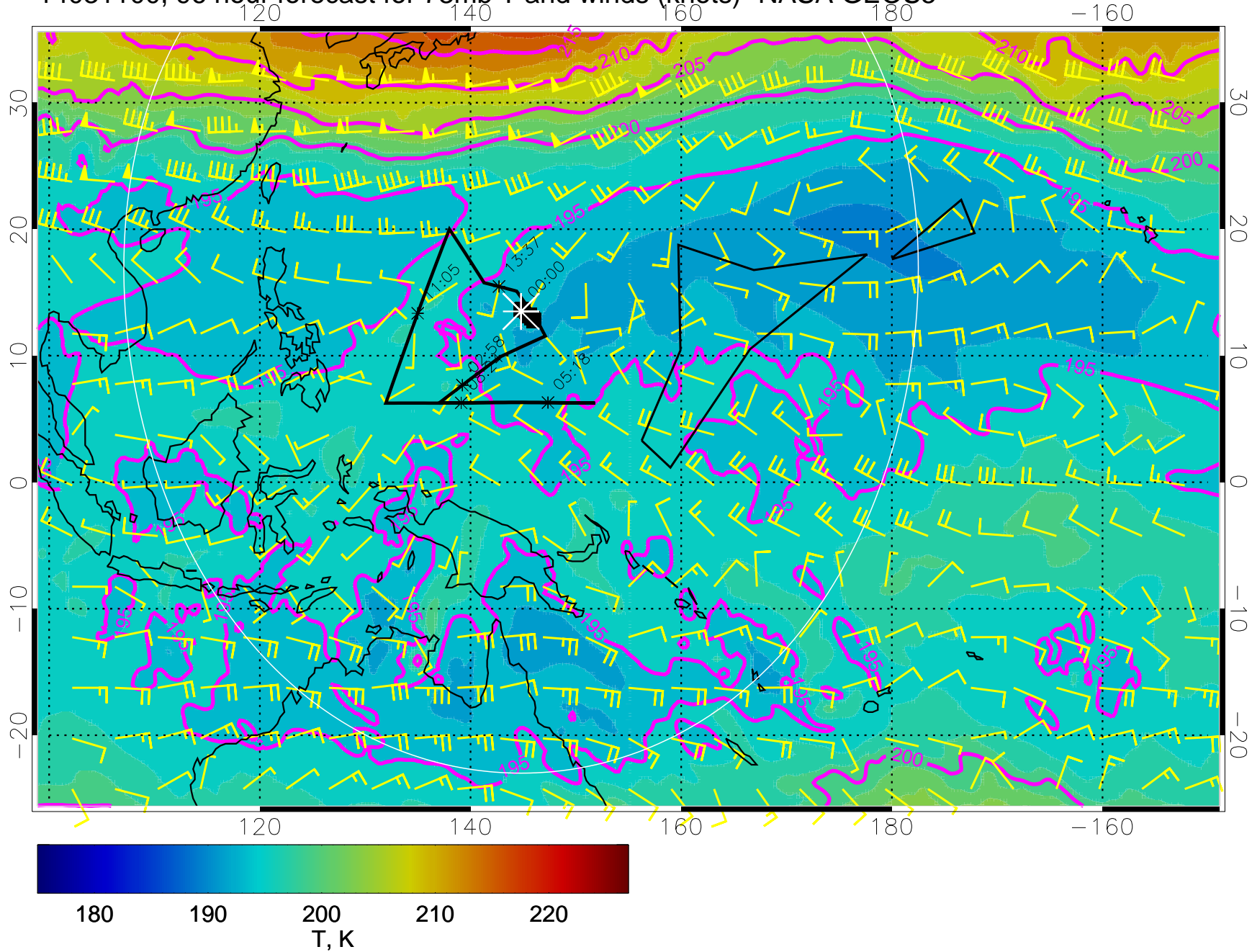
14031100, 96 hour forecast for 73mb T and winds (knots)- NASA GEOS5
