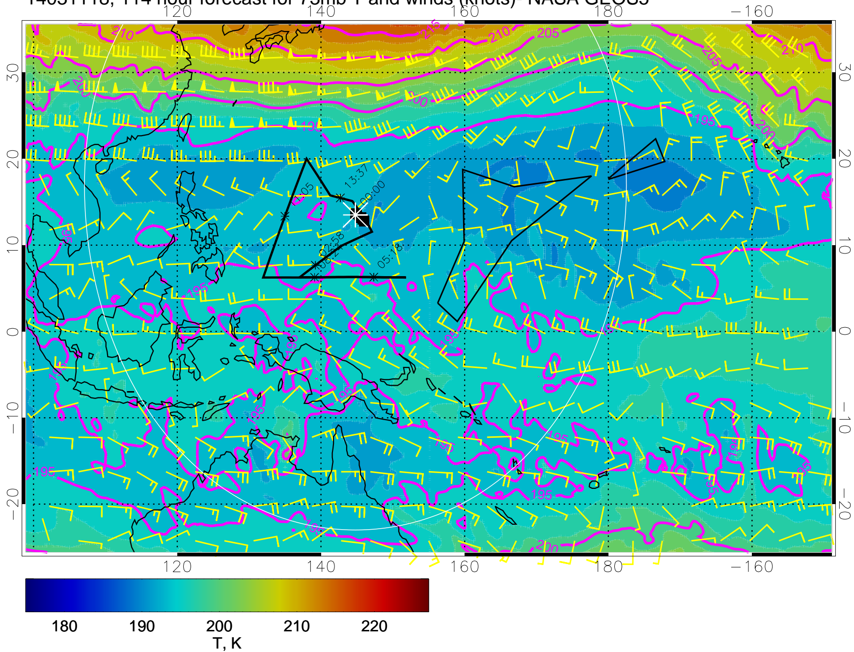
14031118, 114 hour forecast for 73mb T and winds (knots)- NASA GEOS5
