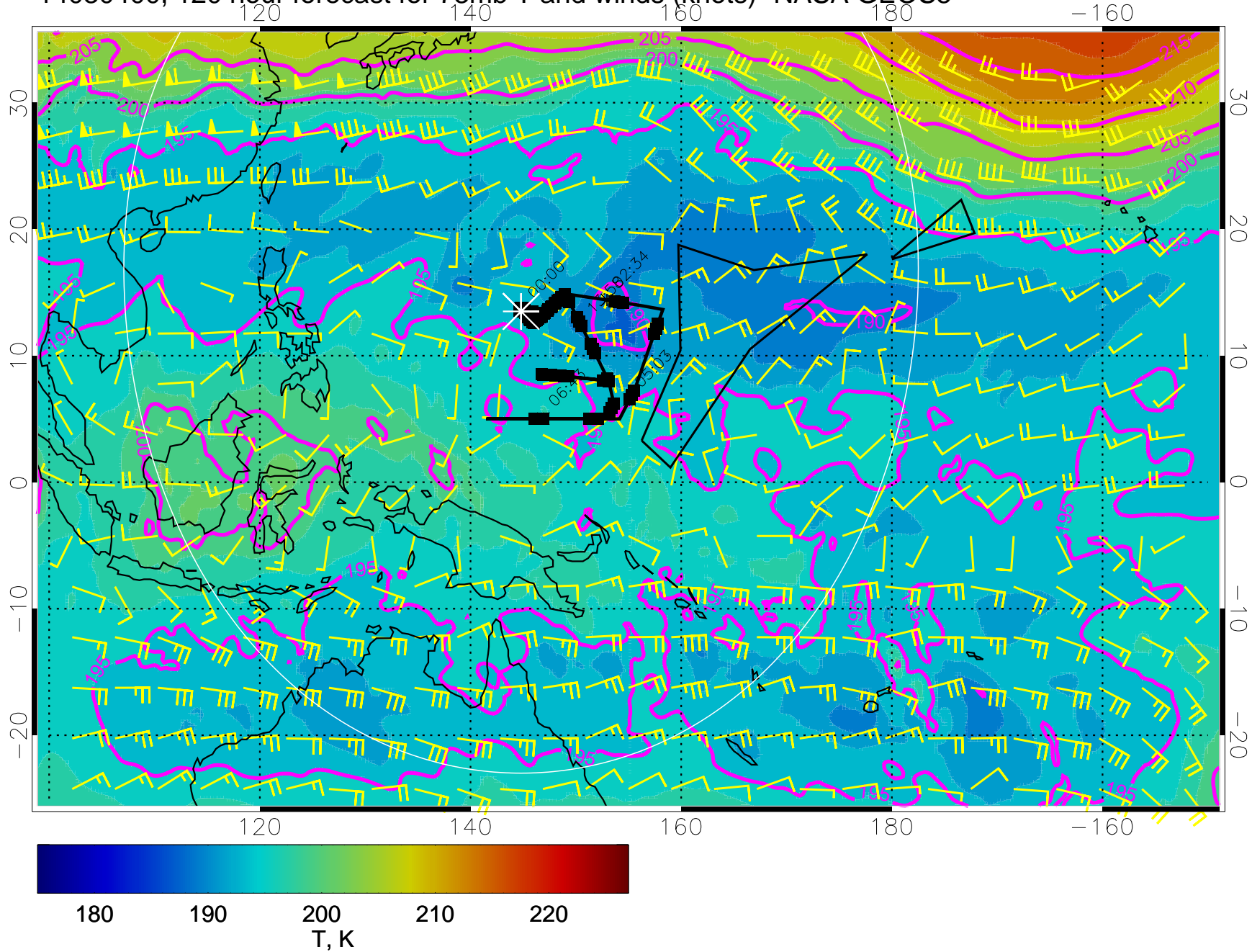
14030400, 120 hour forecast for 73mb T and winds (knots)- NASA GEOS5
