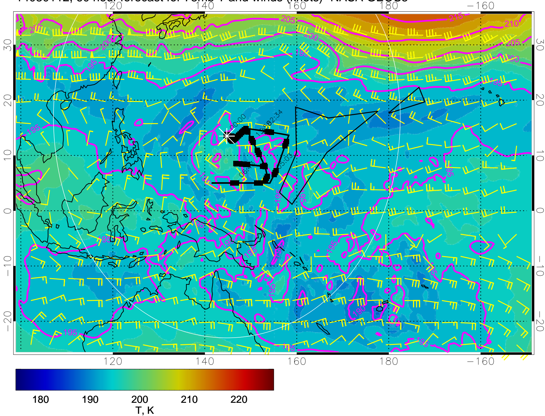
14030112, 60 hour forecast for 73mb T and winds (knots)- NASA GEOS5
