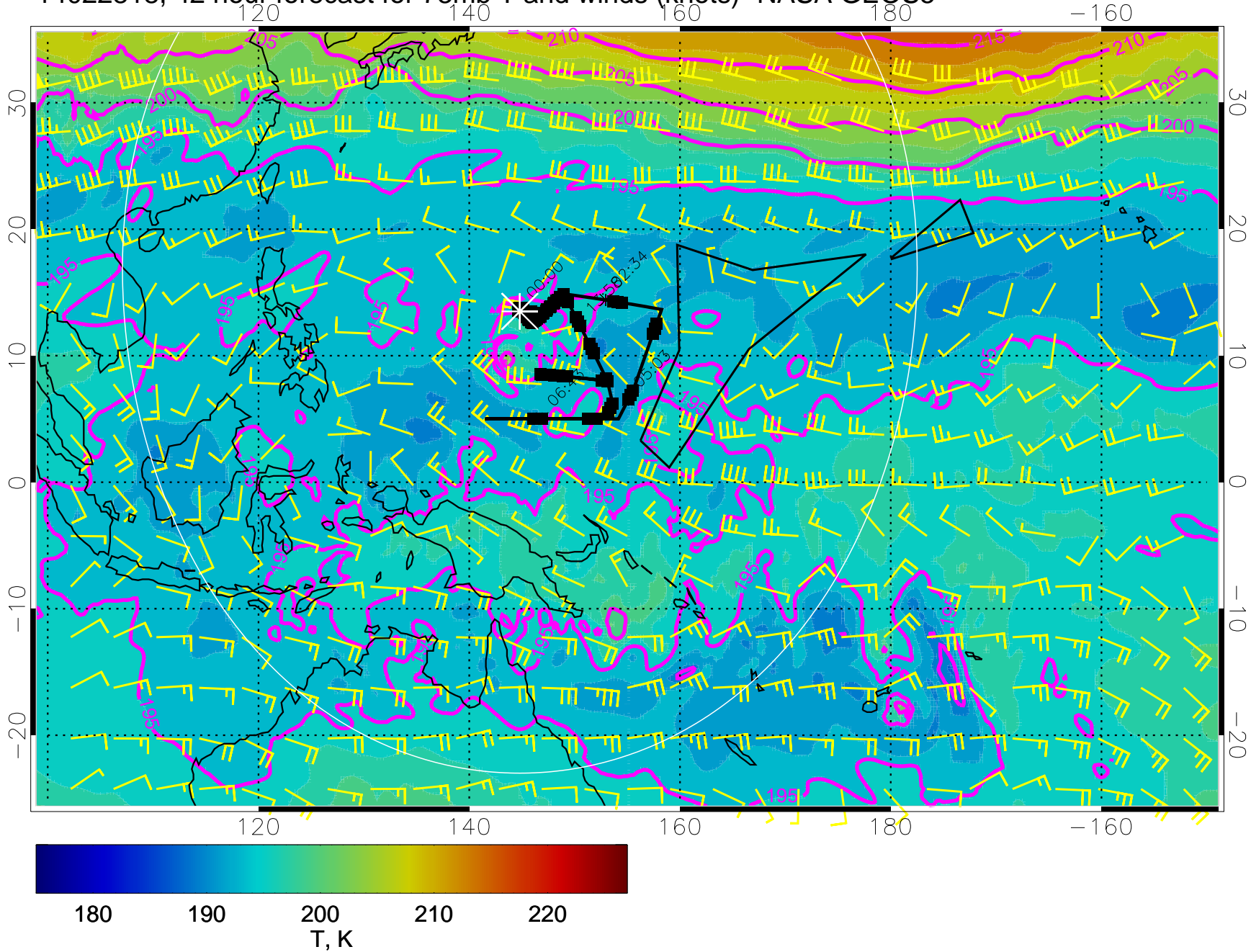
14022818, 42 hour forecast for 73mb T and winds (knots)- NASA GEOS5
