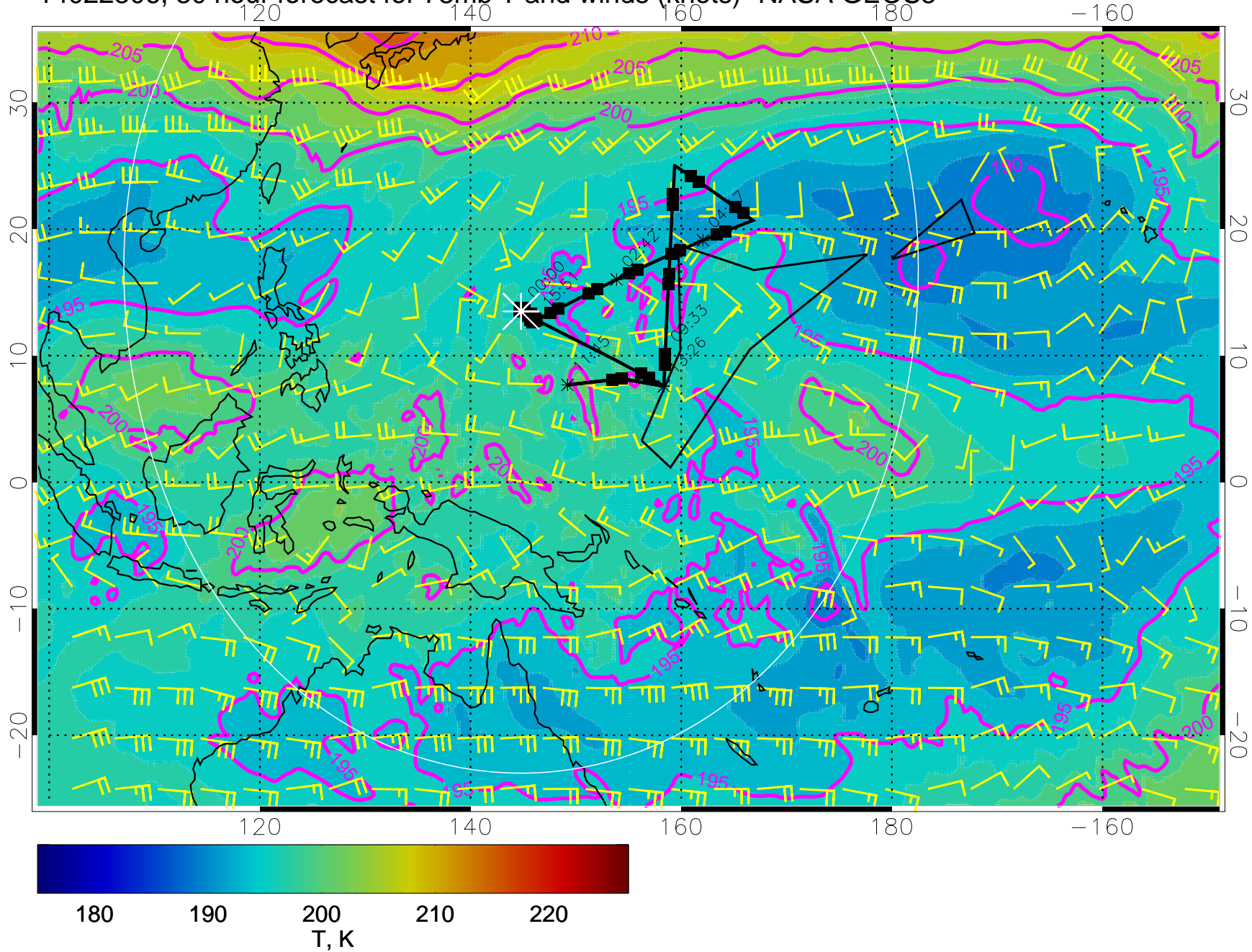
14022306, 30 hour forecast for 73mb T and winds (knots)- NASA GEOS5
