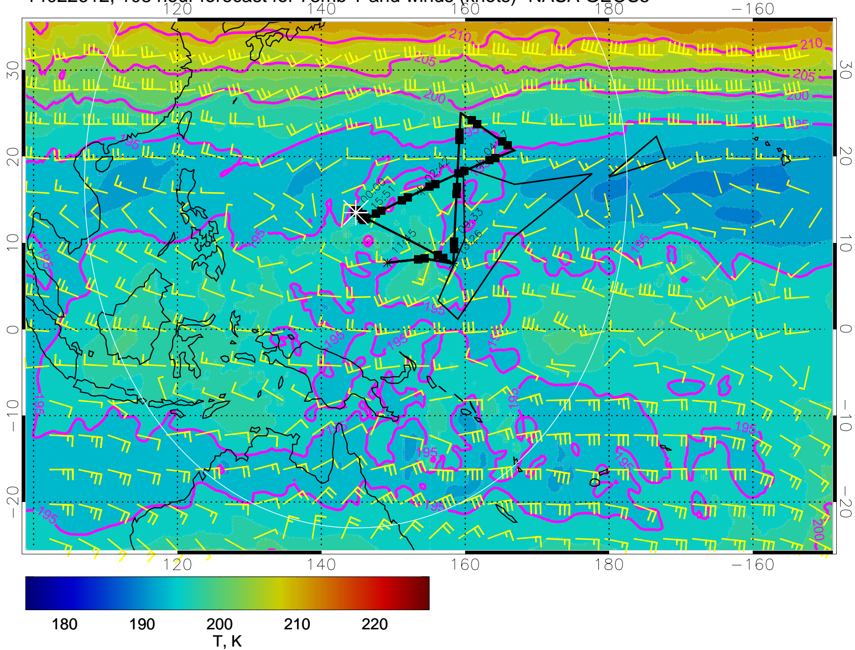
14022612, 108 hour forecast for 73mb T and winds (knots)- NASA GEOS5
