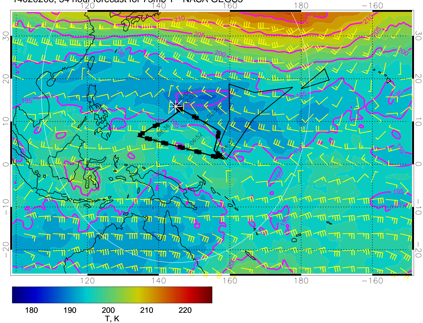
14020206, 54 hour forecast for 73mb T - NASA GEOS5
