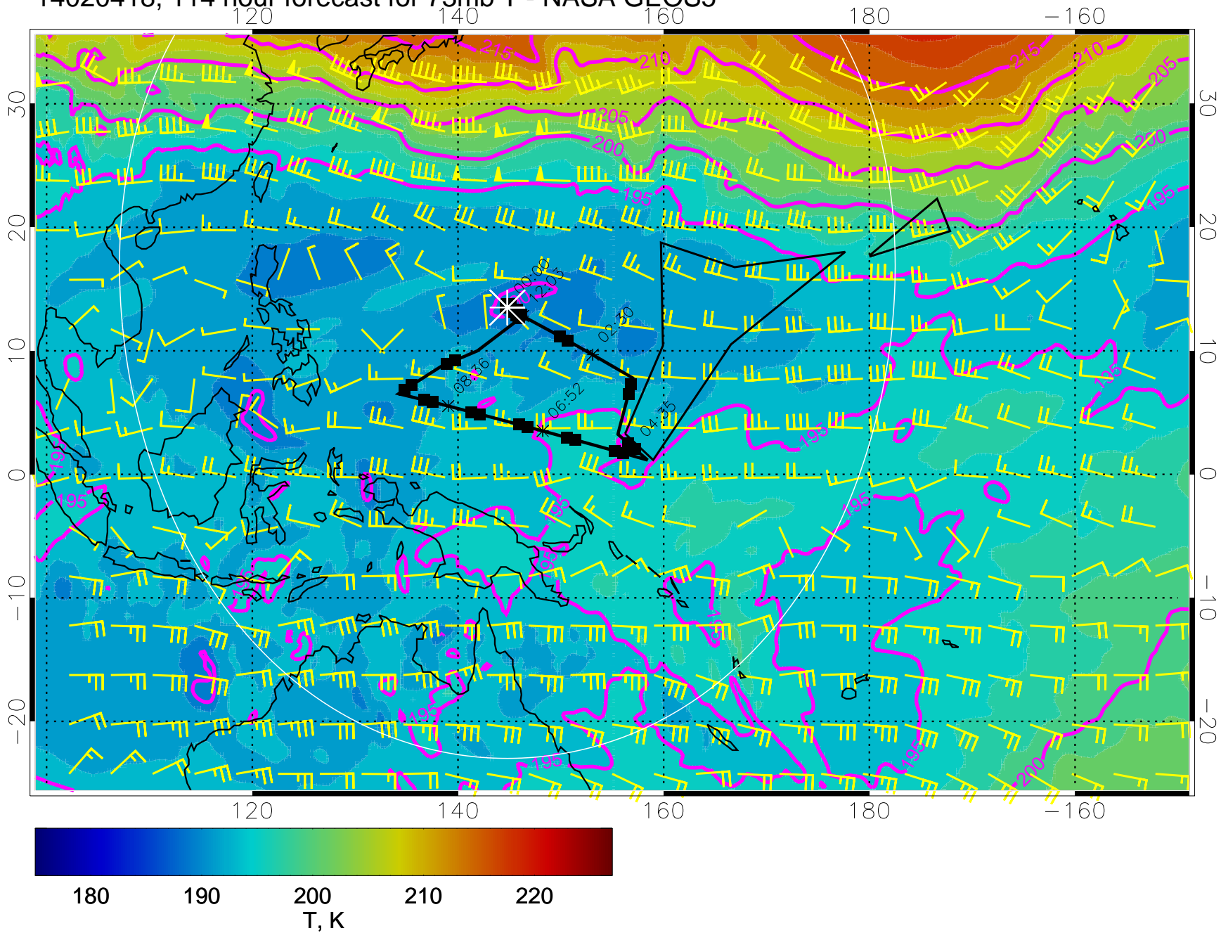
14020418, 114 hour forecast for 73mb T - NASA GEOS5
