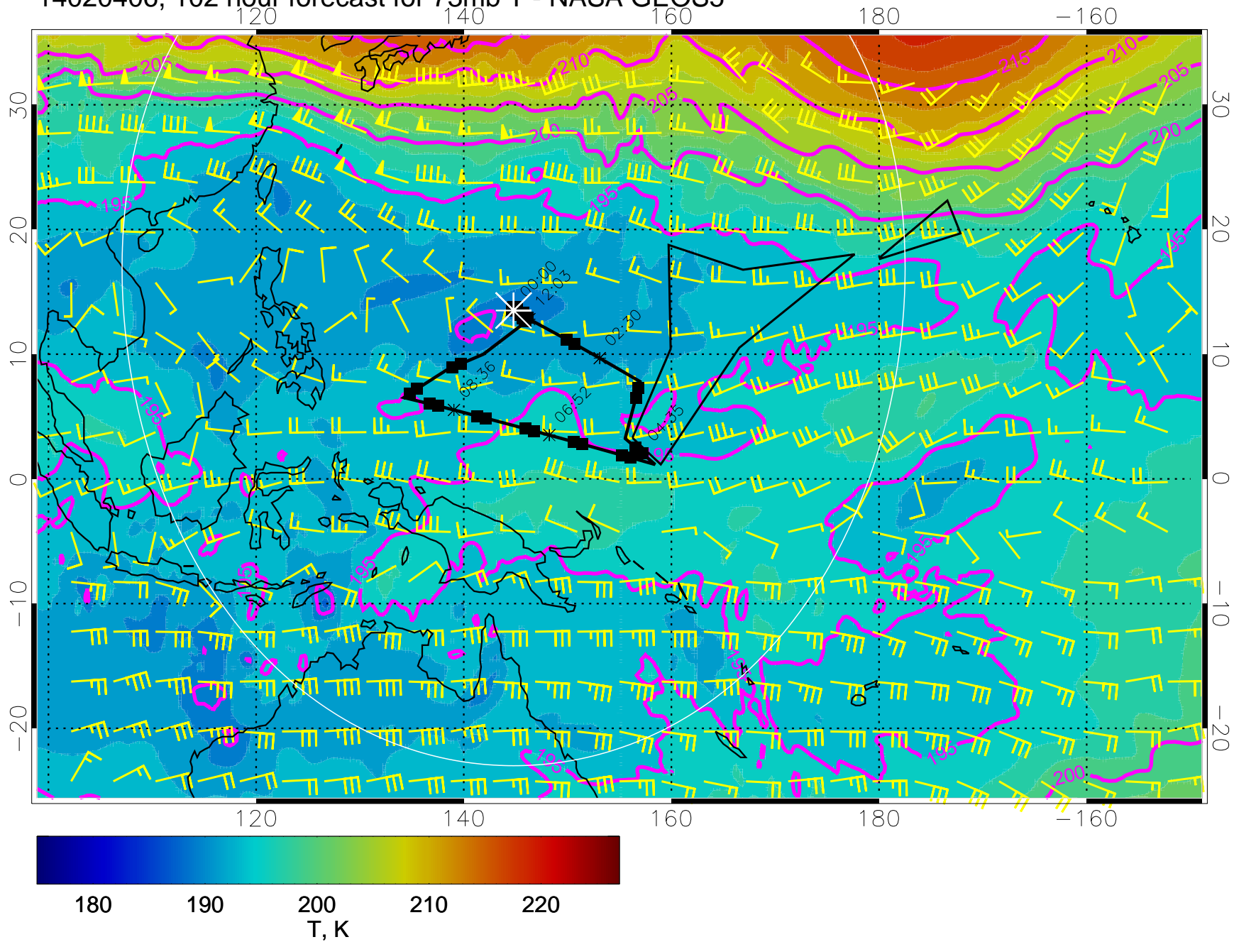
14020406, 102 hour forecast for 73mb T - NASA GEOS5
