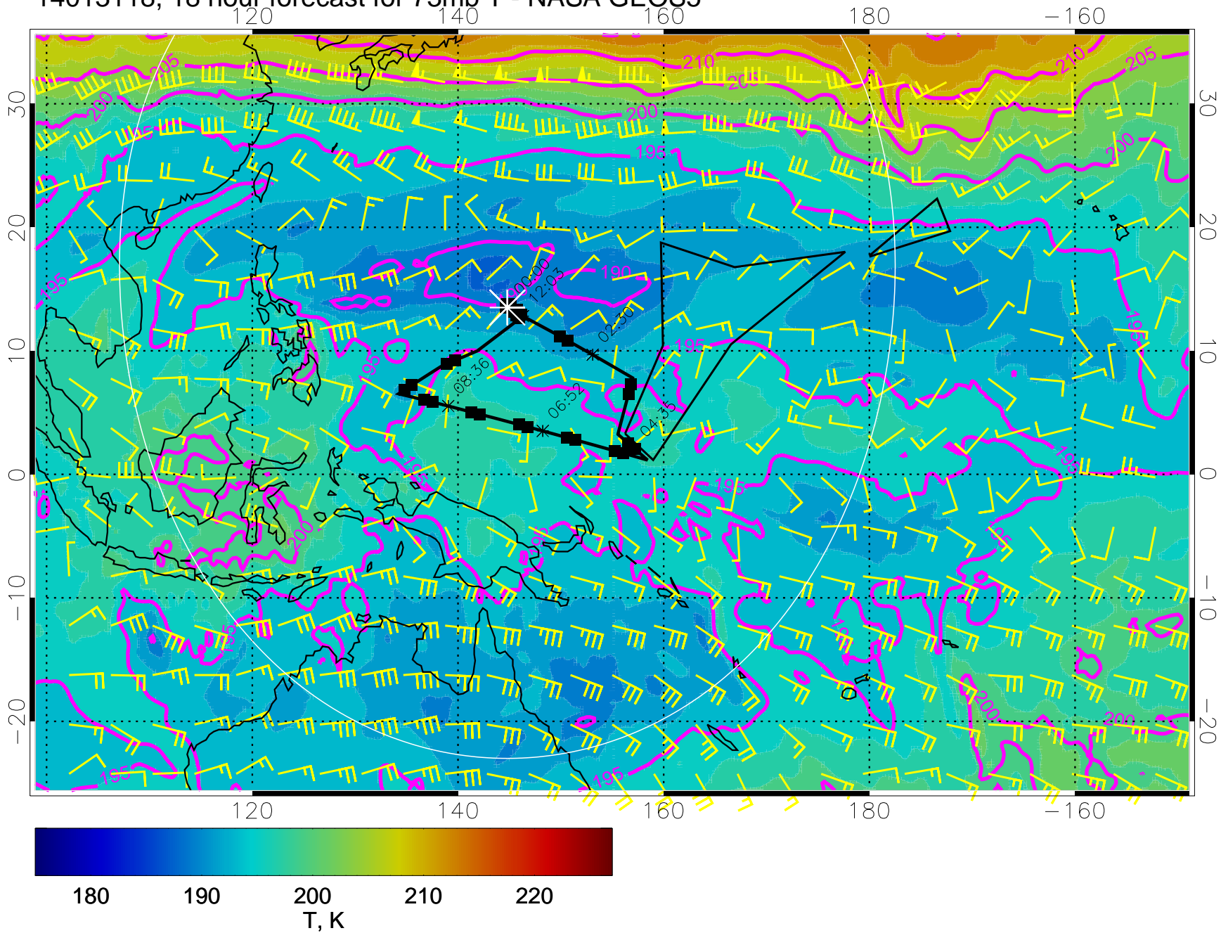
14013118, 18 hour forecast for 73mb T - NASA GEOS5
