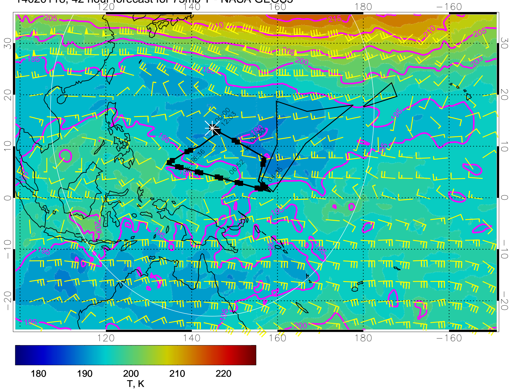
14020118, 42 hour forecast for 73mb T - NASA GEOS5
