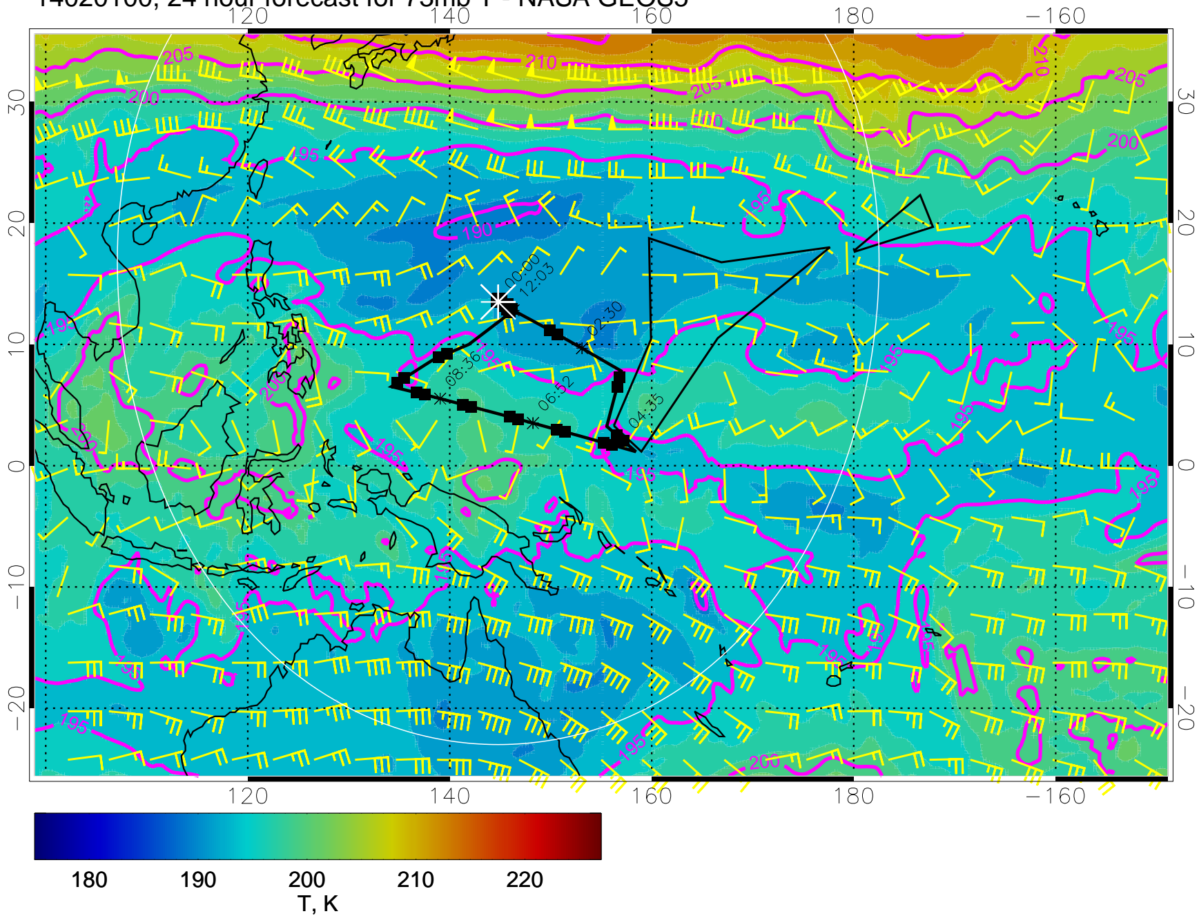
14020100, 24 hour forecast for 73mb T - NASA GEOS5
