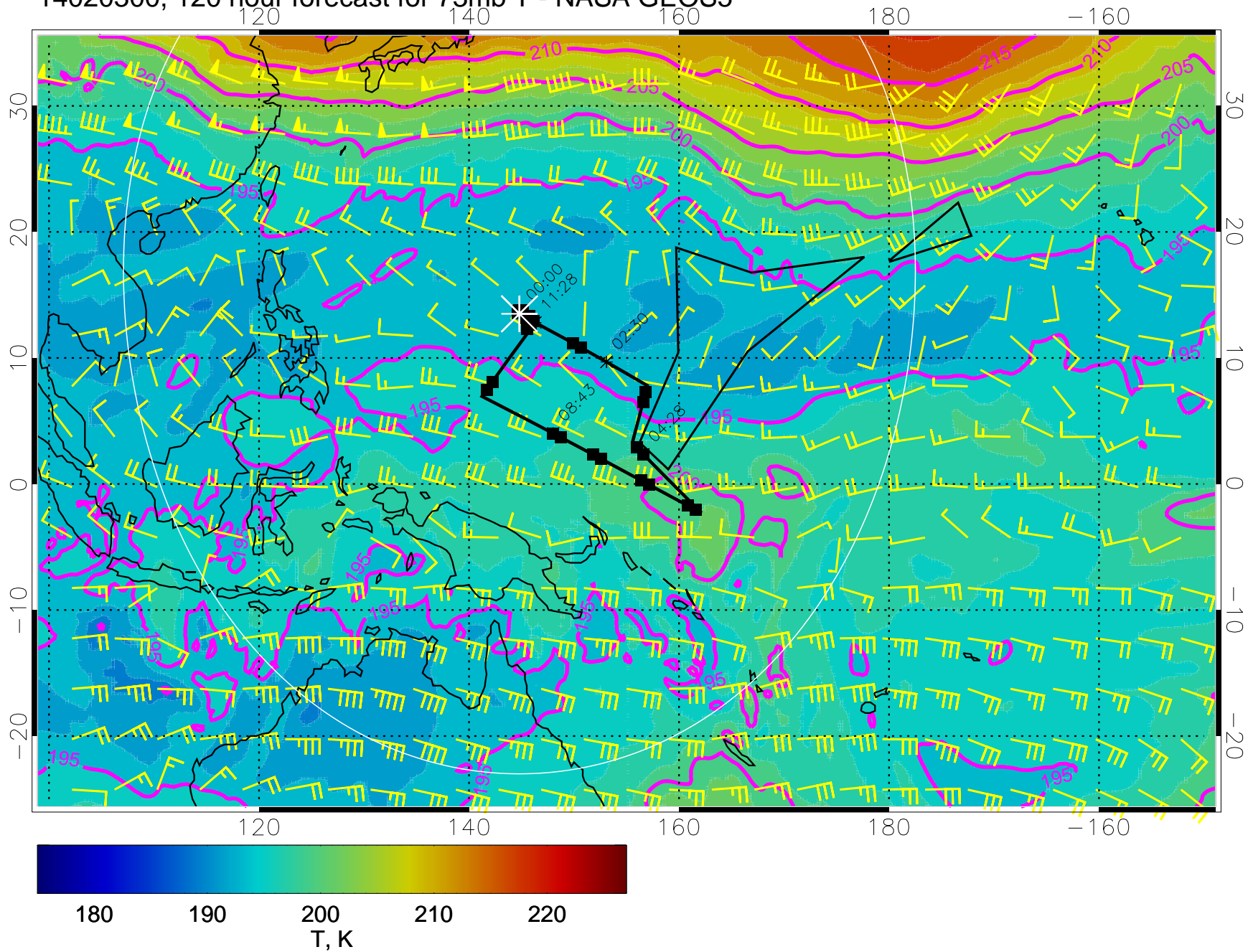
14020300, 120 hour forecast for 73mb T - NASA GEOS5
