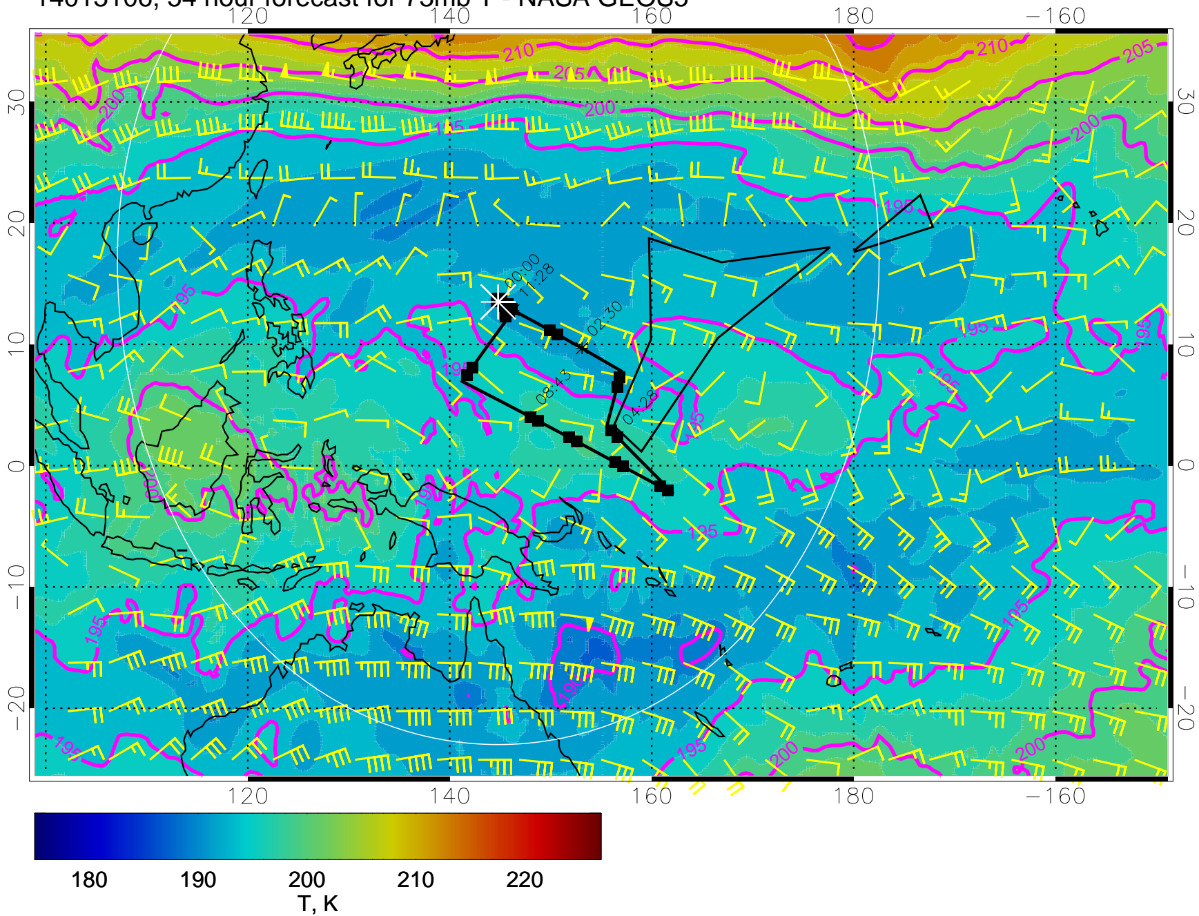
14013106, 54 hour forecast for 73mb T - NASA GEOS5
