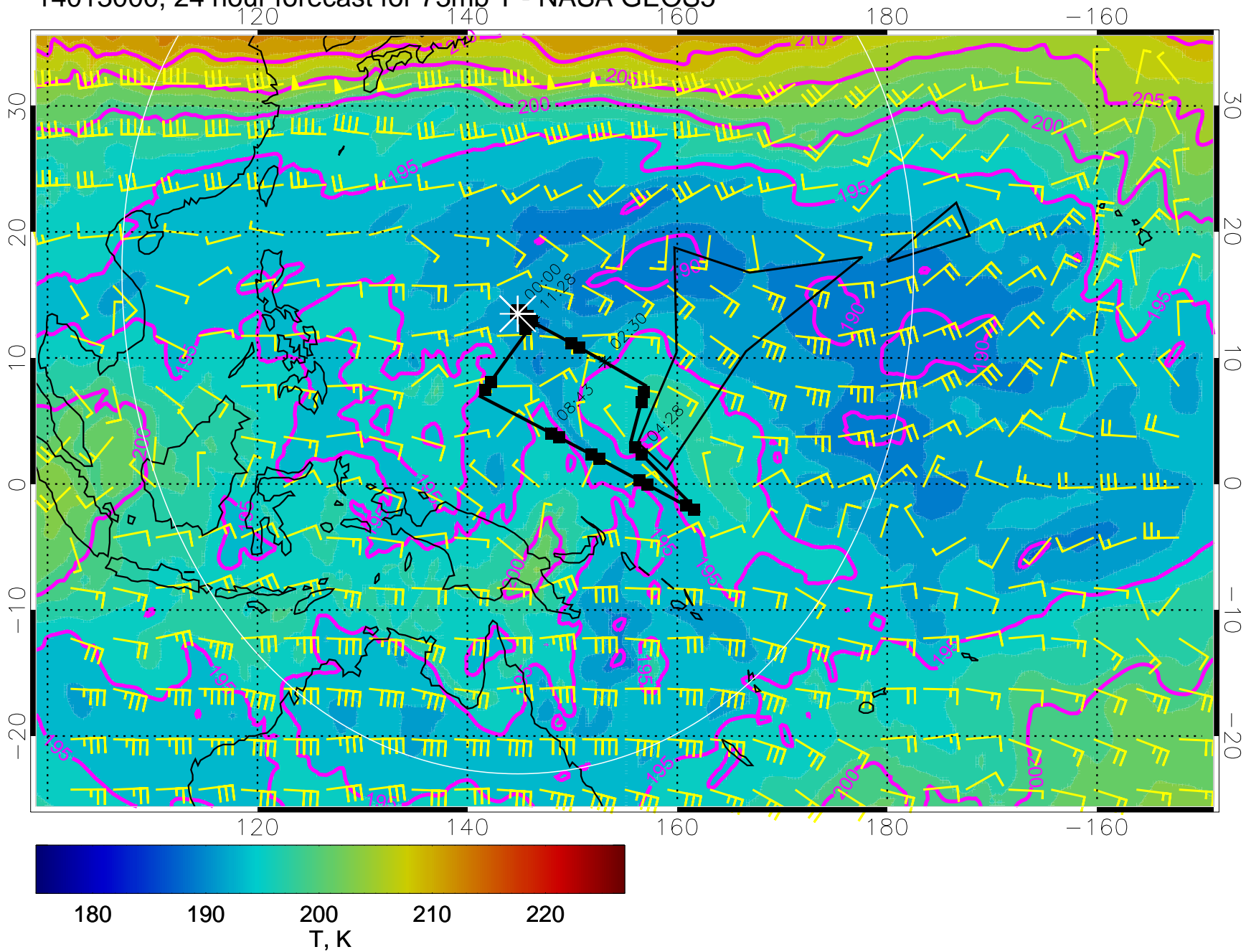
14013000, 24 hour forecast for 73mb T - NASA GEOS5
