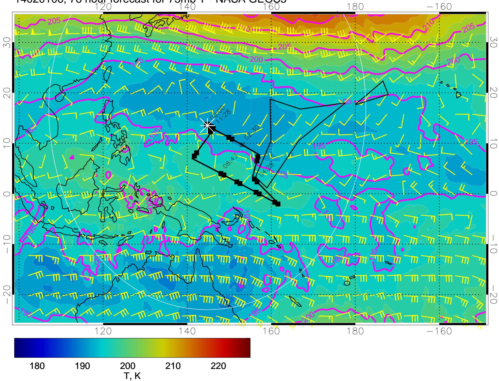
14020106, 78 hour forecast for 73mb T - NASA GEOS5
