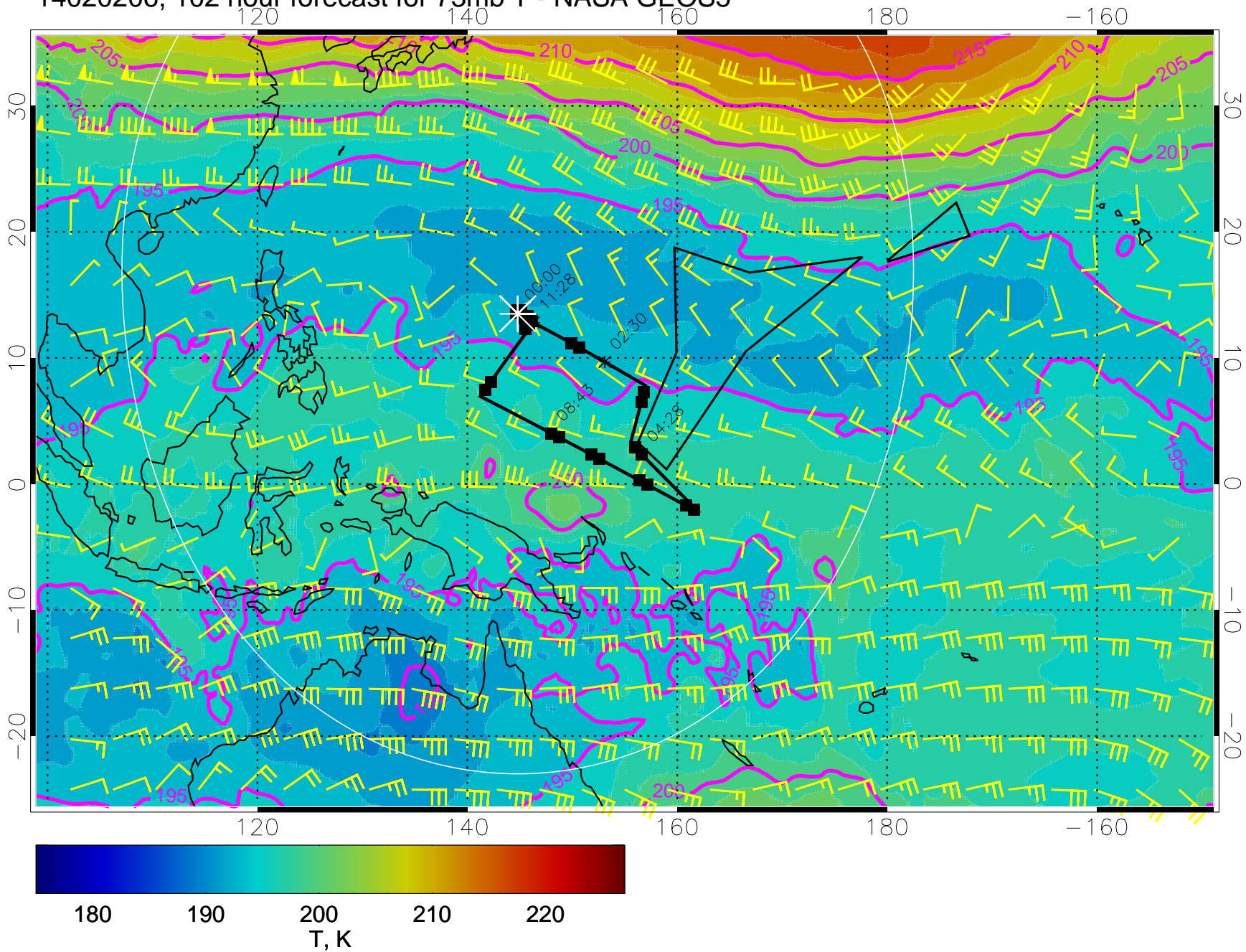
14020206, 102 hour forecast for 73mb T - NASA GEOS5
