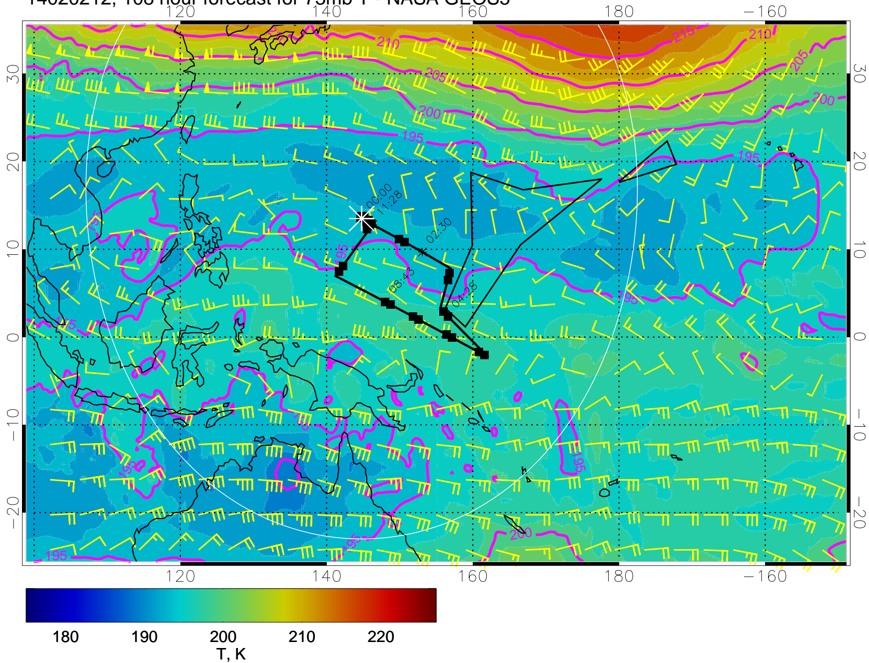
14020212, 108 hour forecast for 73mb T - NASA GEOS5
