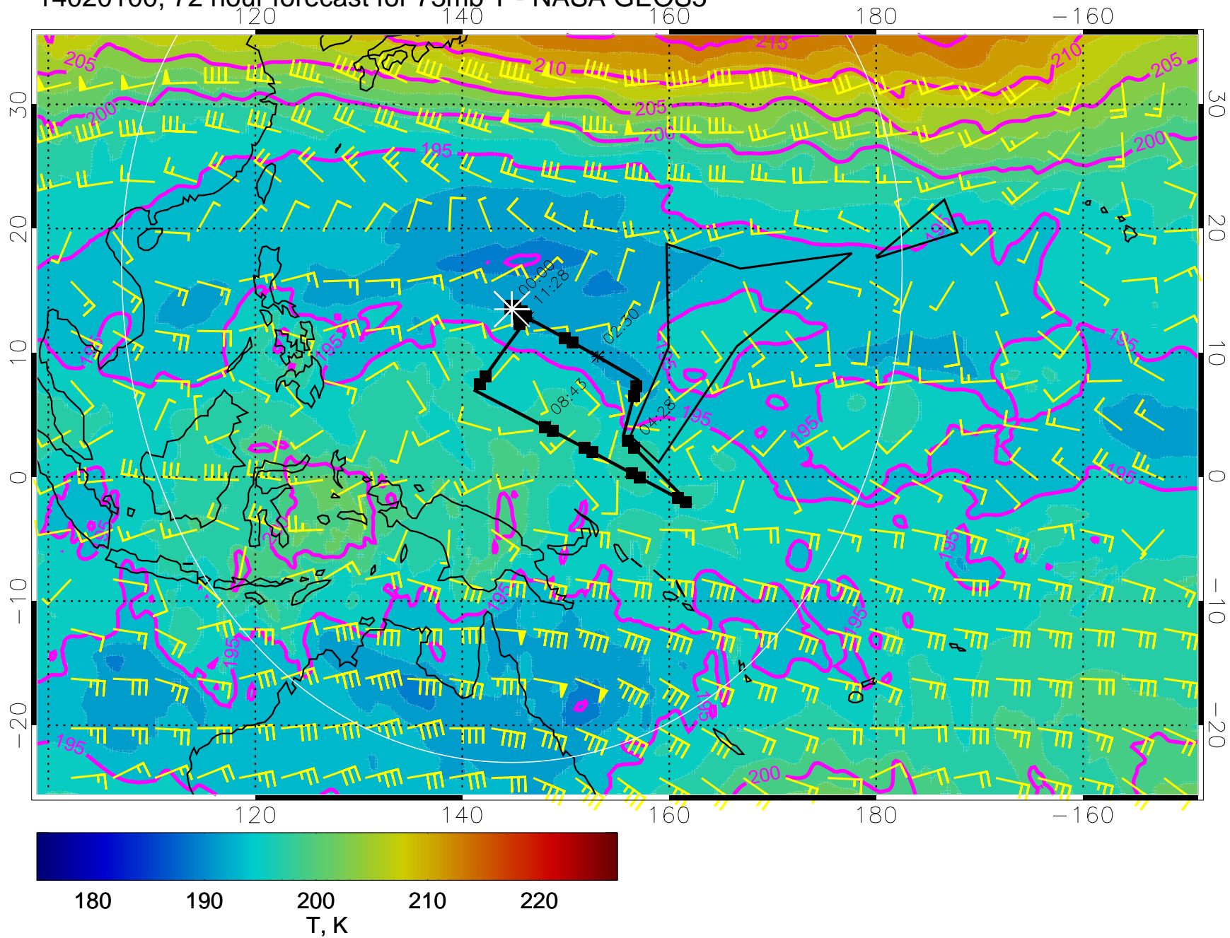
14020100, 72 hour forecast for 73mb T - NASA GEOS5
