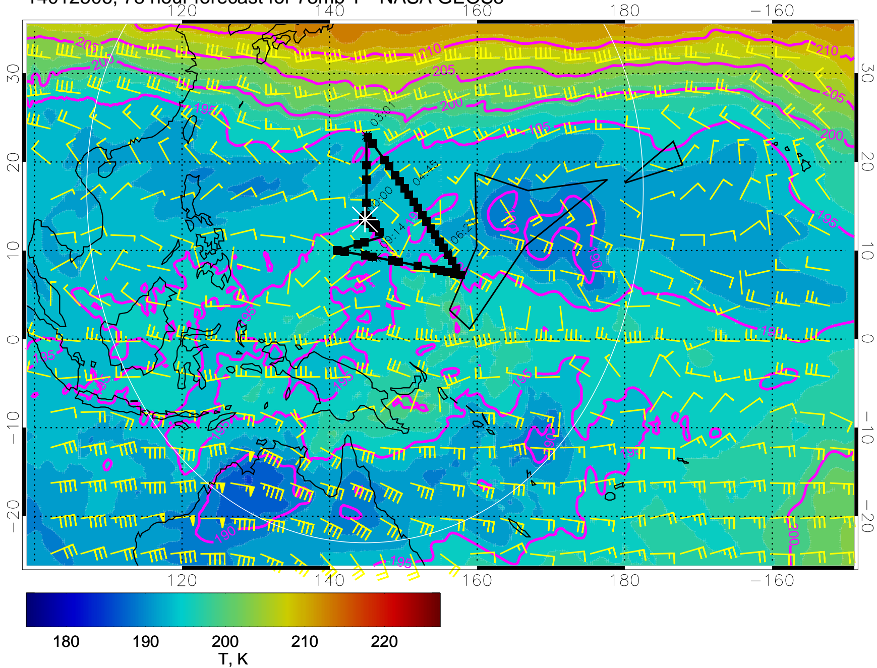
14012506, 78 hour forecast for 73mb T - NASA GEOS5
