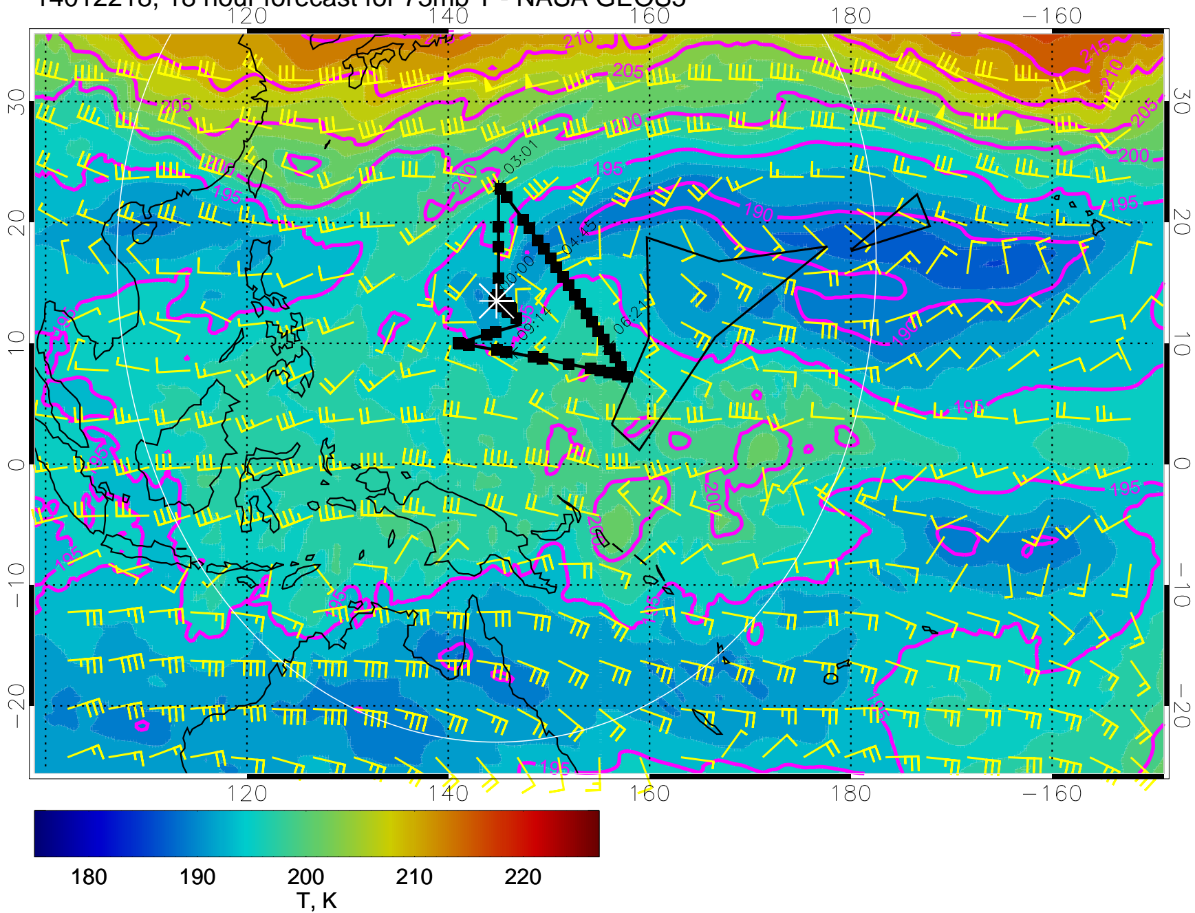
14012218, 18 hour forecast for 73mb T - NASA GEOS5
