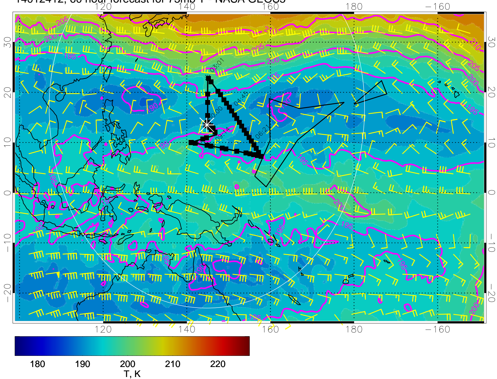
14012412, 60 hour forecast for 73mb T - NASA GEOS5
