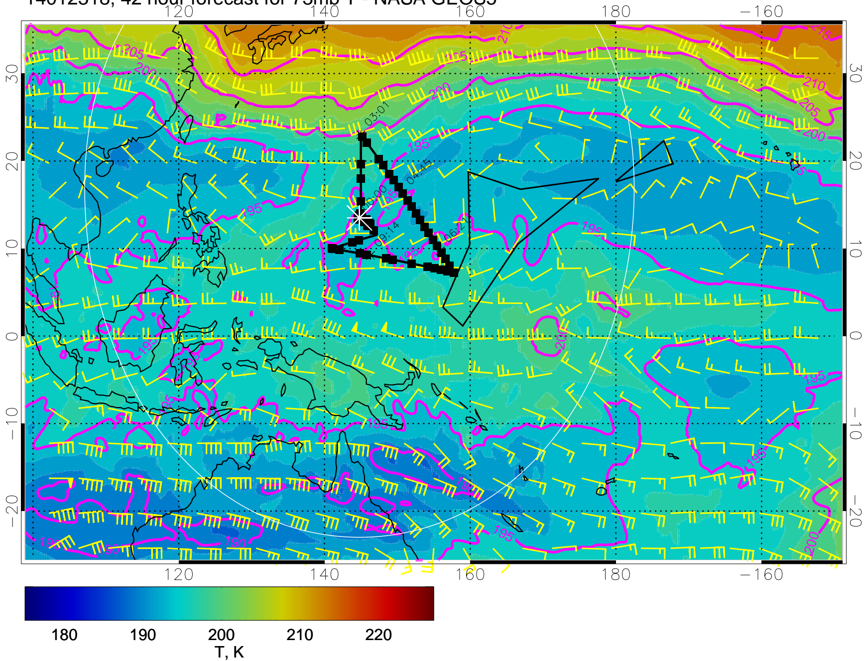
14012318, 42 hour forecast for 73mb T - NASA GEOS5
