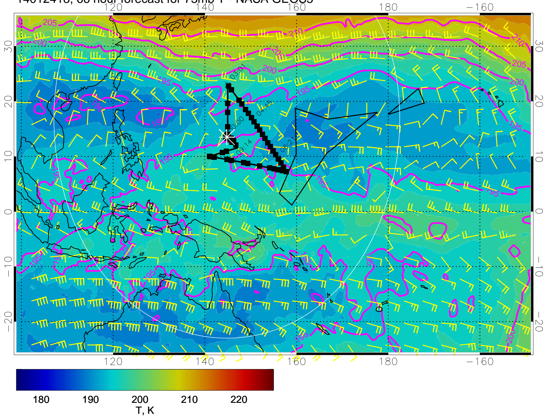
14012418, 66 hour forecast for 73mb T - NASA GEOS5
