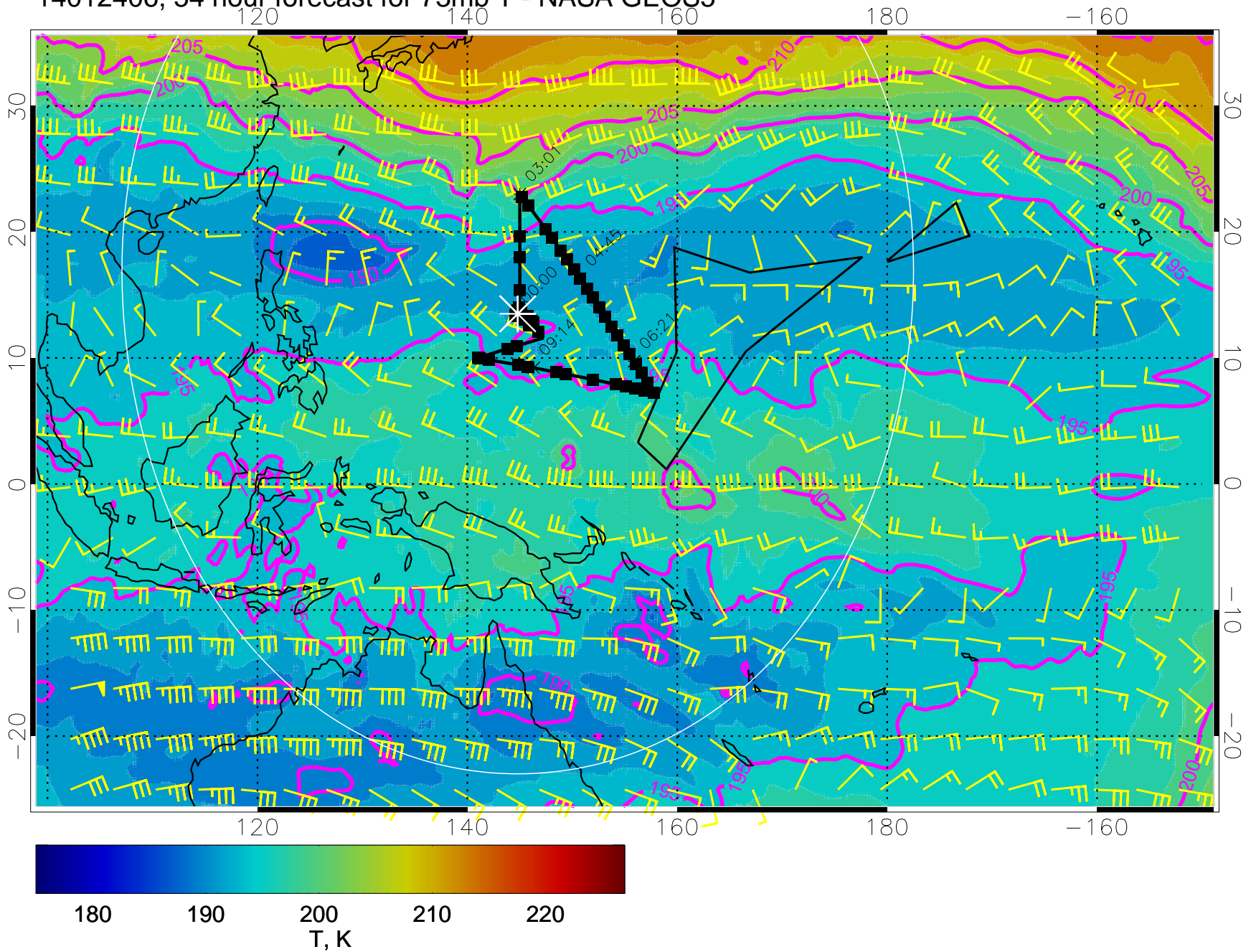
14012406, 54 hour forecast for 73mb T - NASA GEOS5
