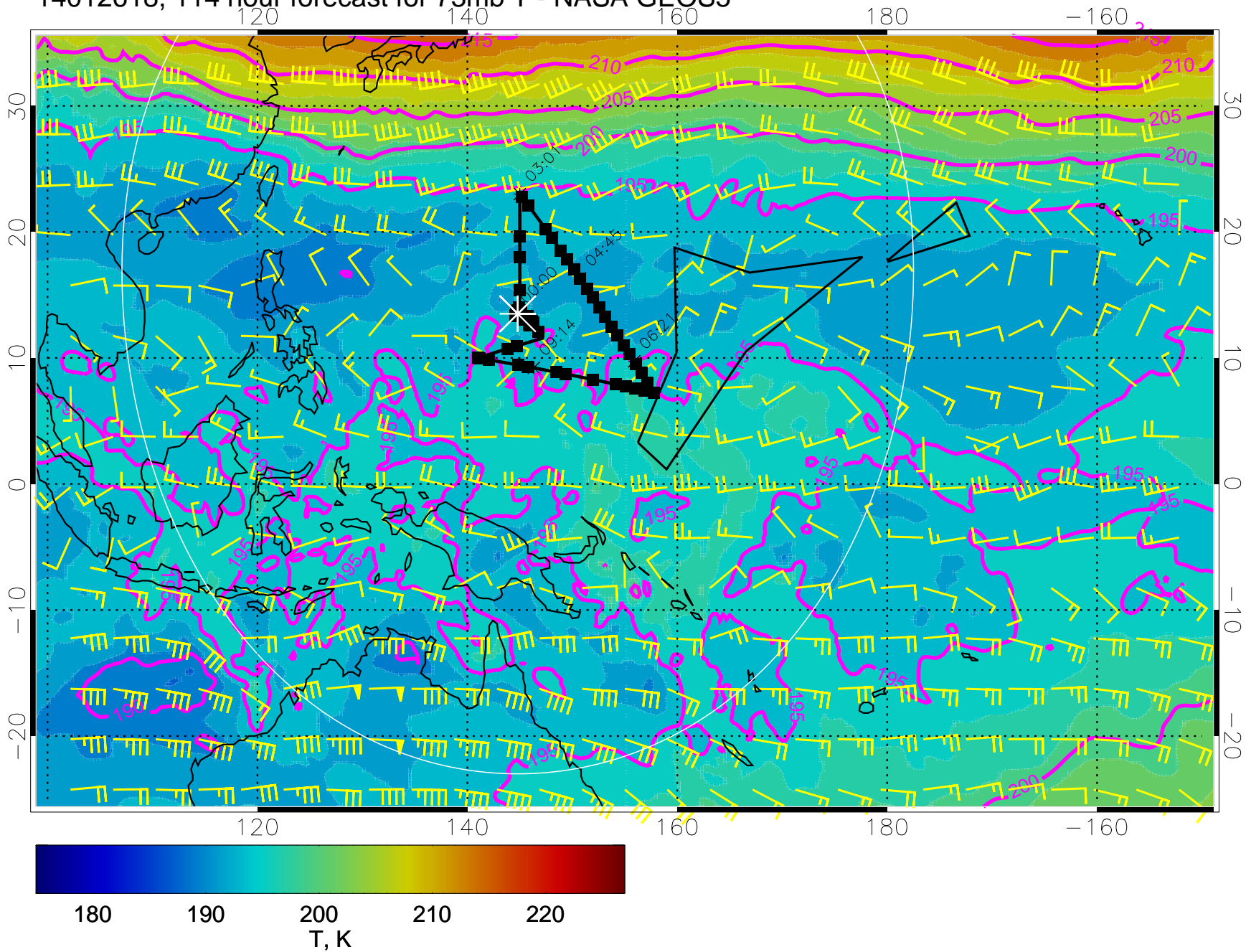
14012618, 114 hour forecast for 73mb T - NASA GEOS5
