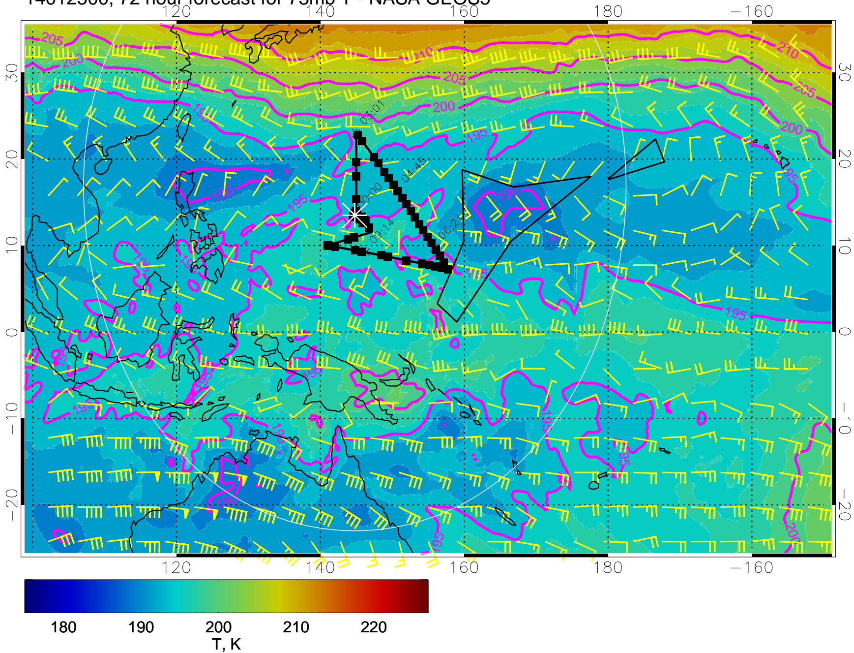
14012500, 72 hour forecast for 73mb T - NASA GEOS5
