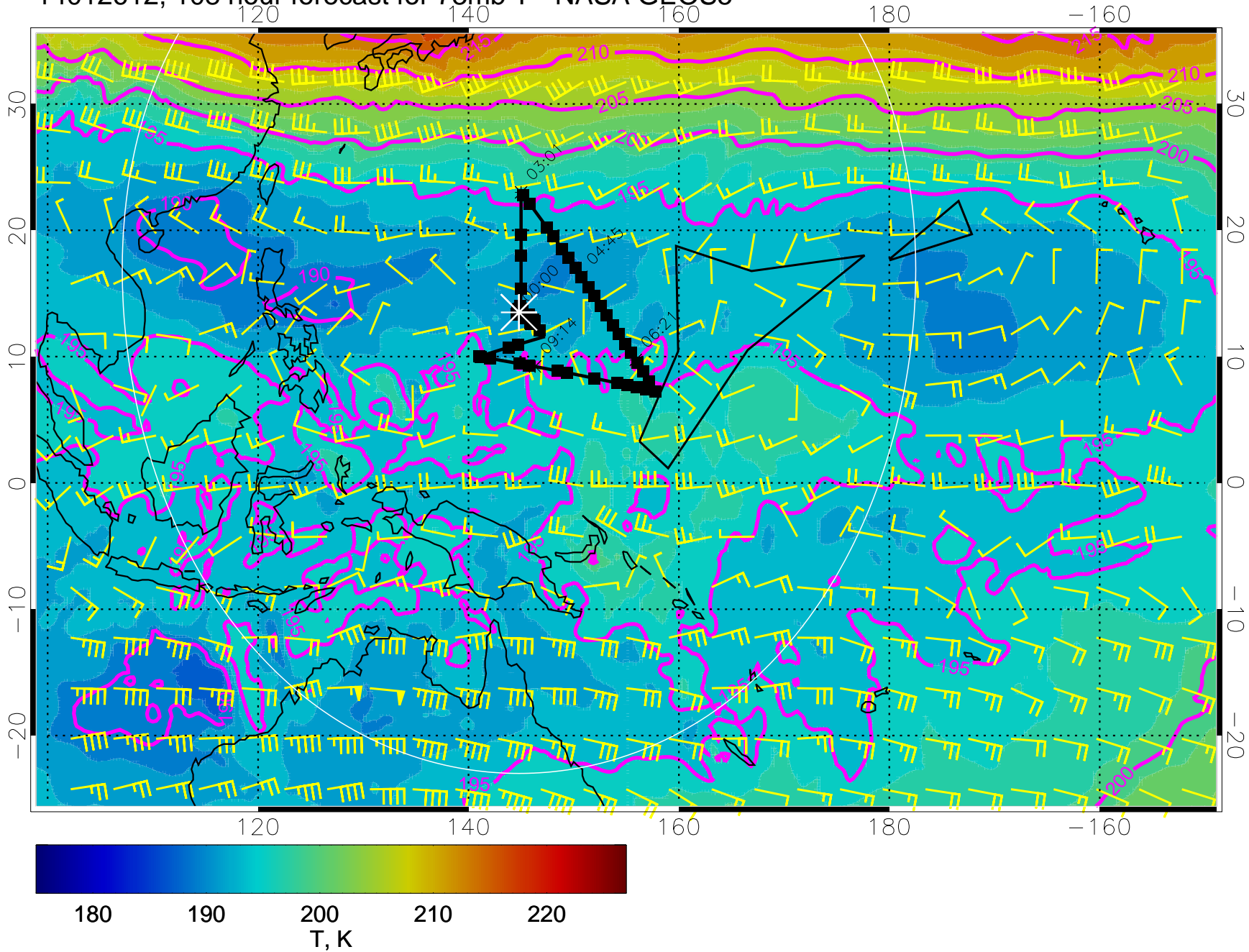
14012612, 108 hour forecast for 73mb T - NASA GEOS5
