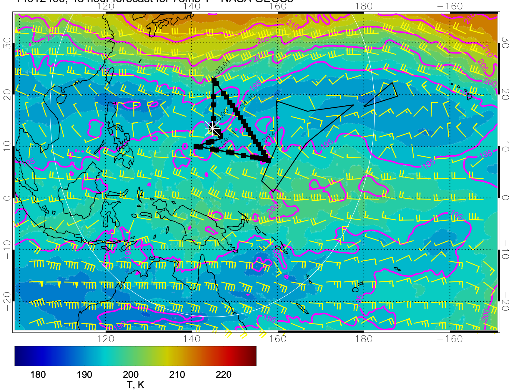
14012400, 48 hour forecast for 73mb T - NASA GEOS5
