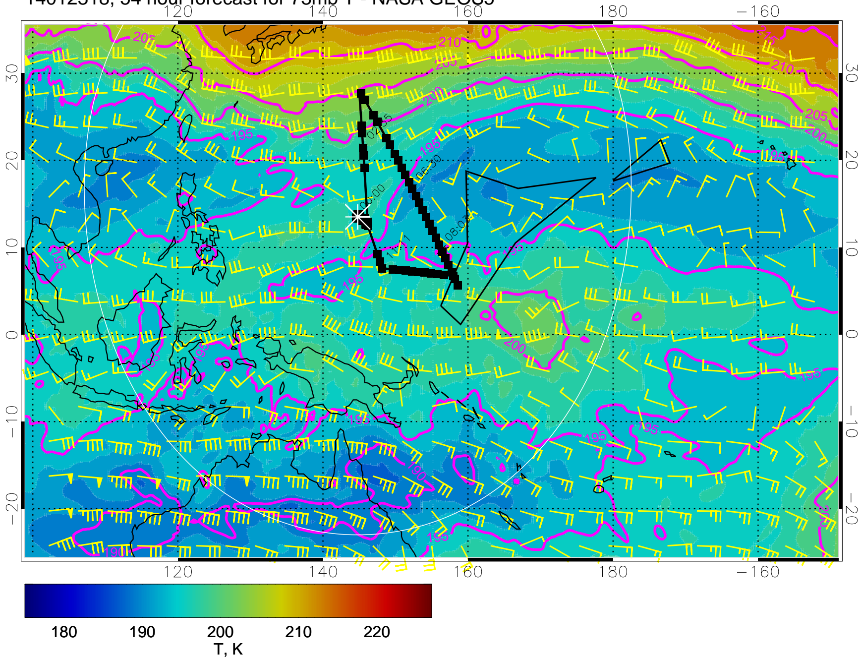
14012318, 54 hour forecast for 73mb T - NASA GEOS5
