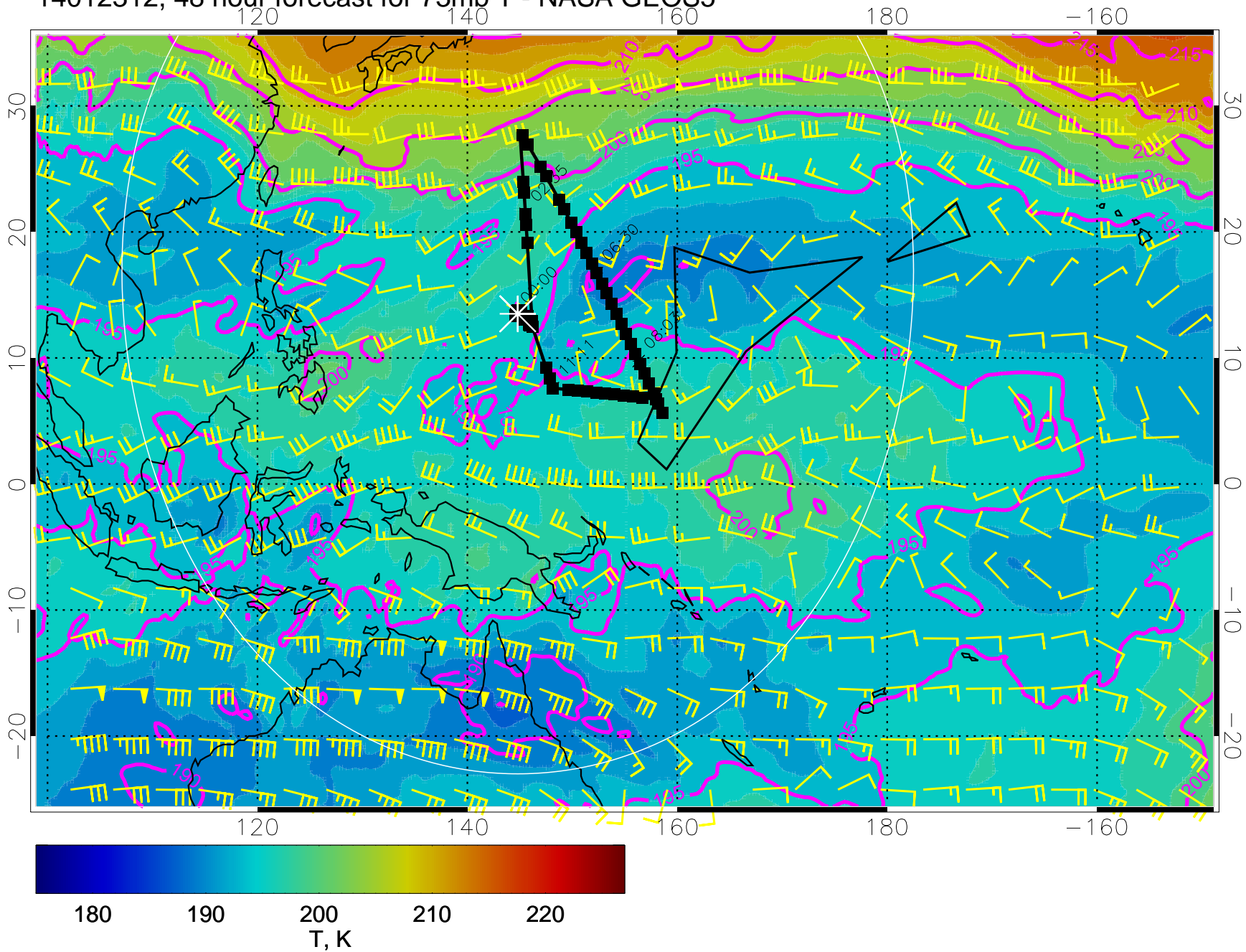
14012312, 48 hour forecast for 73mb T - NASA GEOS5
