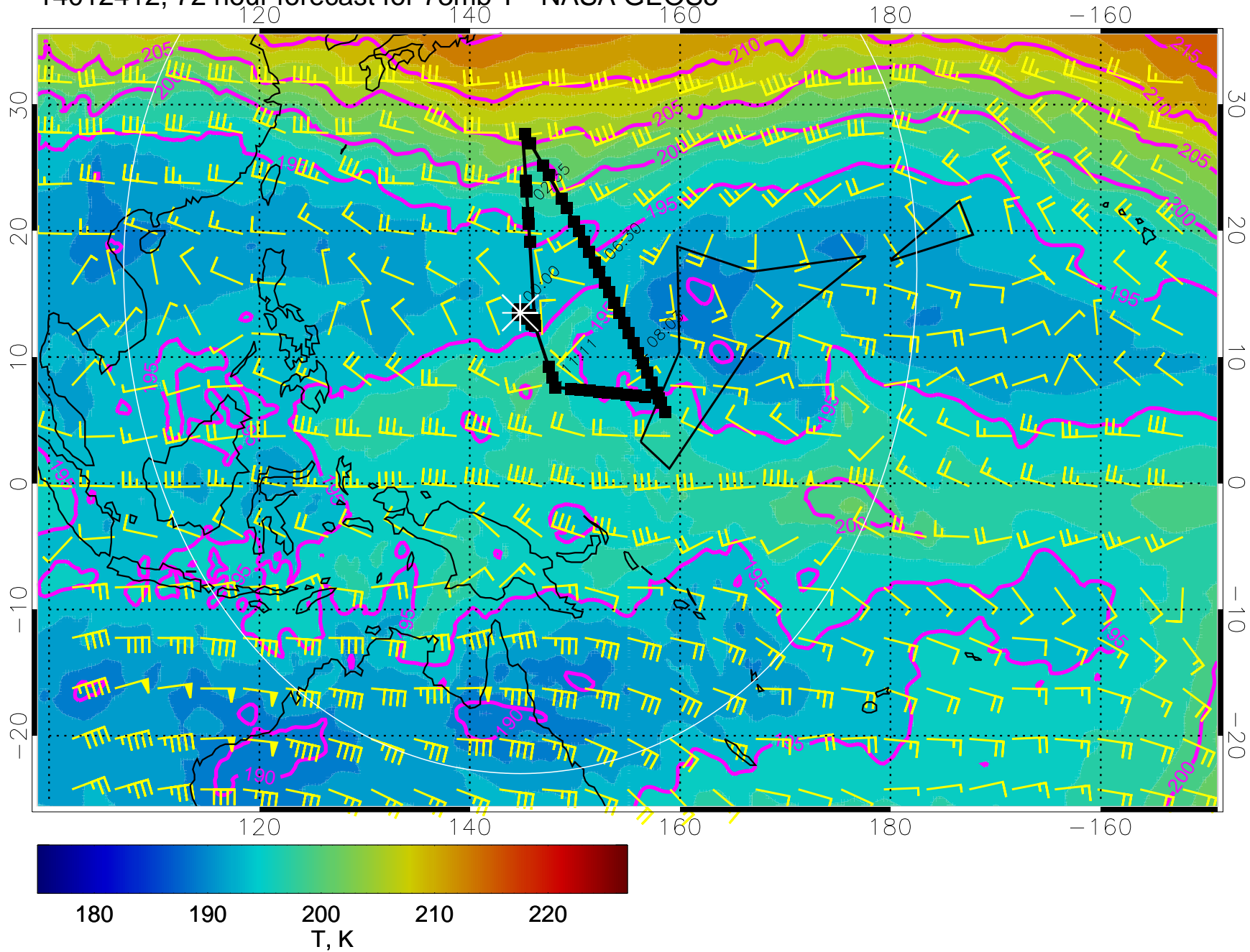
14012412, 72 hour forecast for 73mb T - NASA GEOS5
