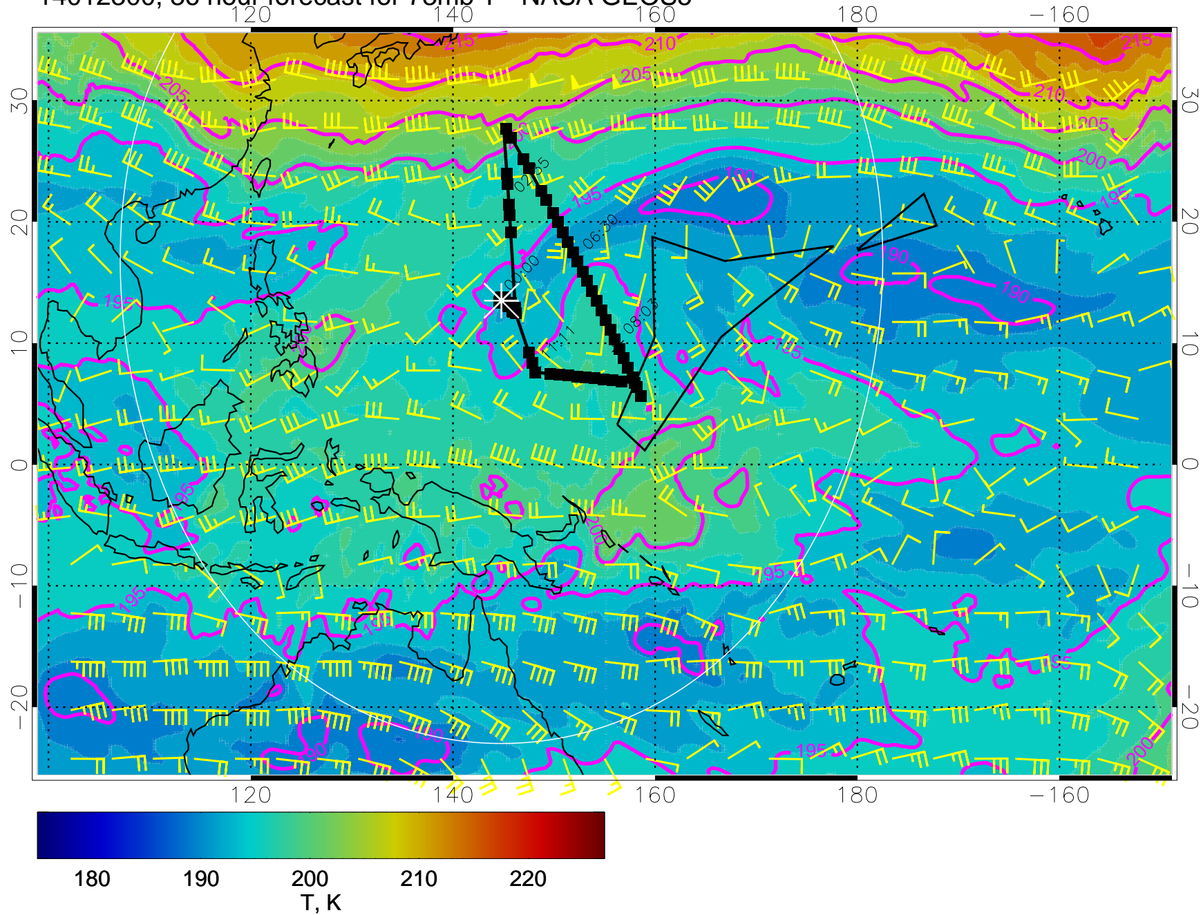
14012300, 36 hour forecast for 73mb T - NASA GEOS5
