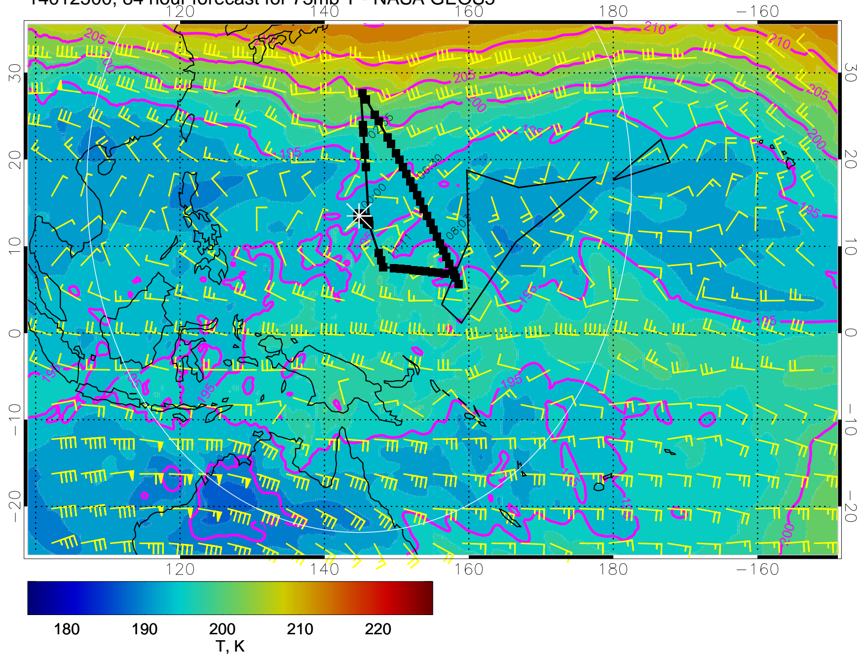
14012500, 84 hour forecast for 73mb T - NASA GEOS5
