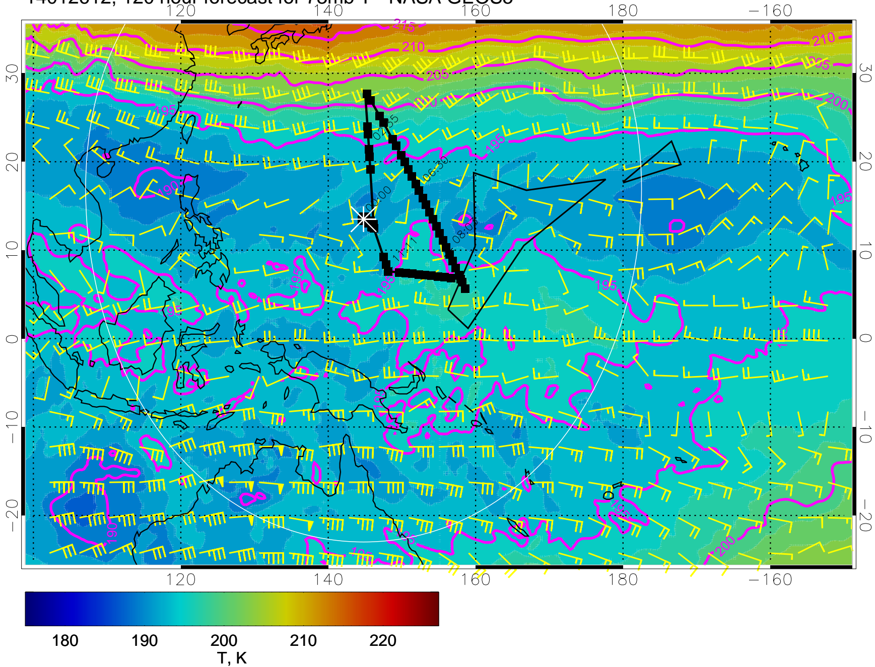
14012612, 120 hour forecast for 73mb T - NASA GEOS5
