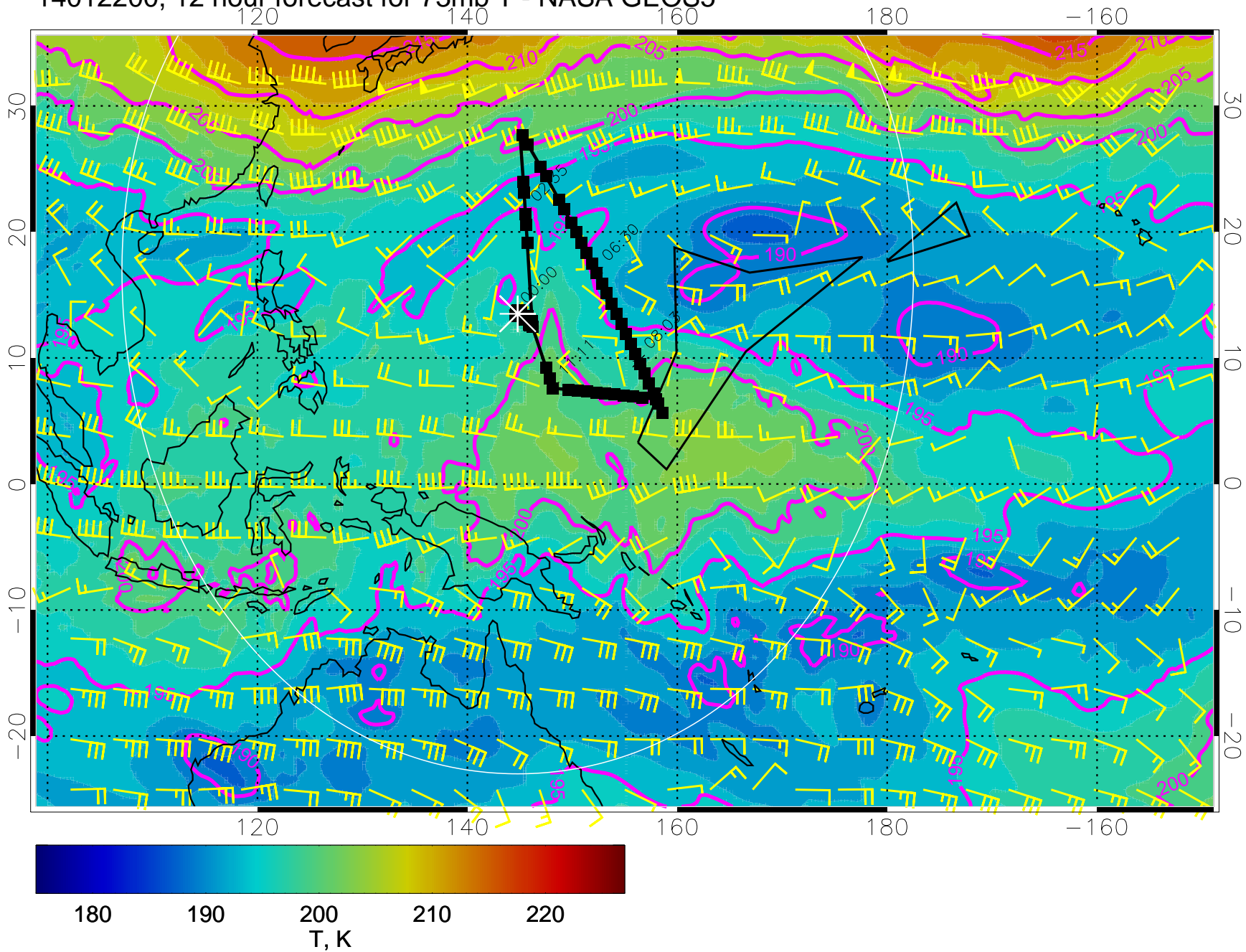
14012200, 12 hour forecast for 73mb T - NASA GEOS5
