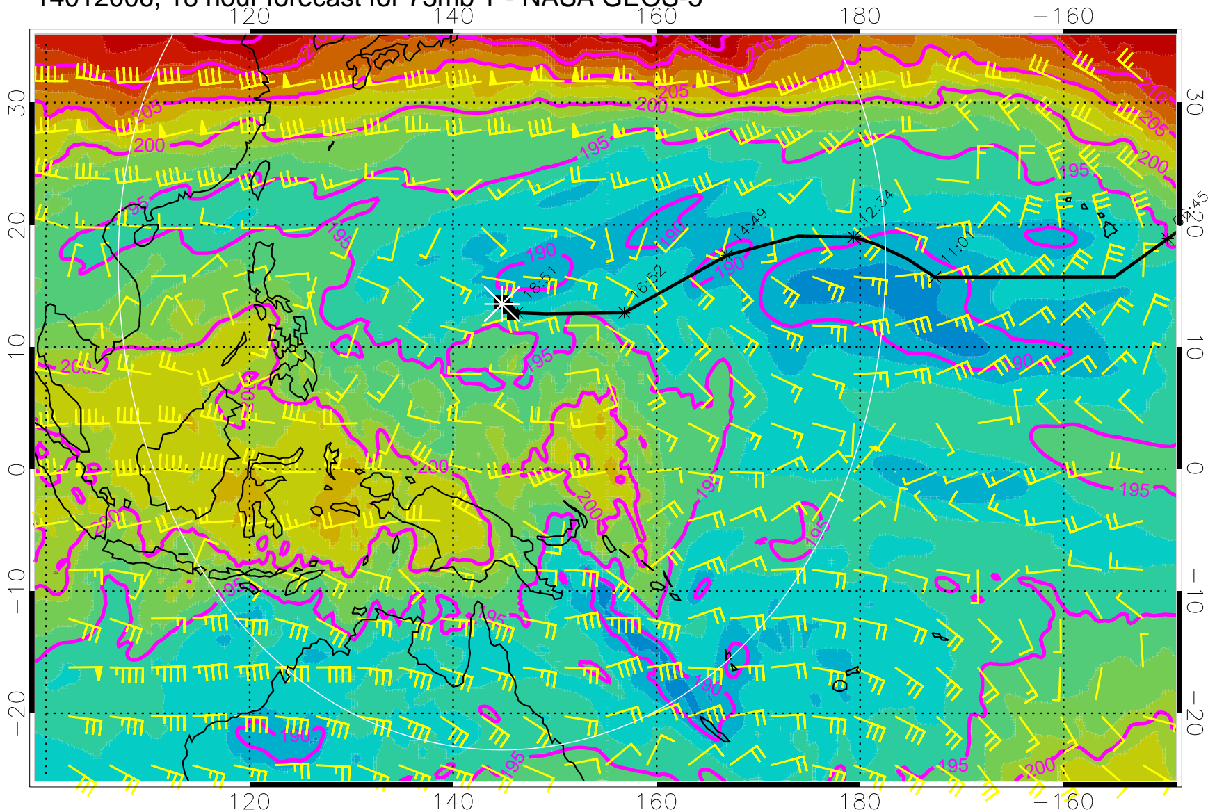
14012006, 18 hour forecast for 73mb T - NASA GEOS-5
