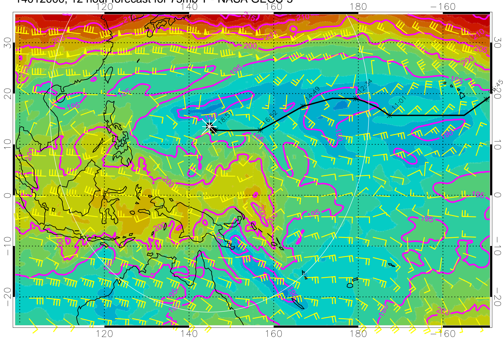
14012000, 12 hour forecast for 73mb T - NASA GEOS-5
