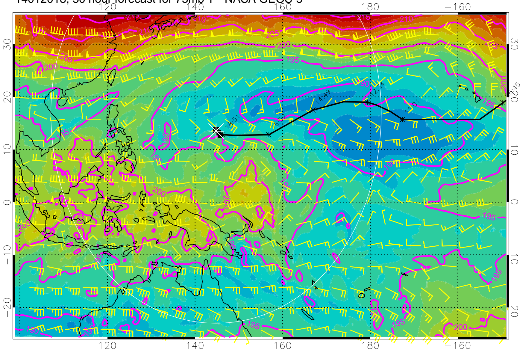
14012018, 30 hour forecast for 73mb T - NASA GEOS-5
