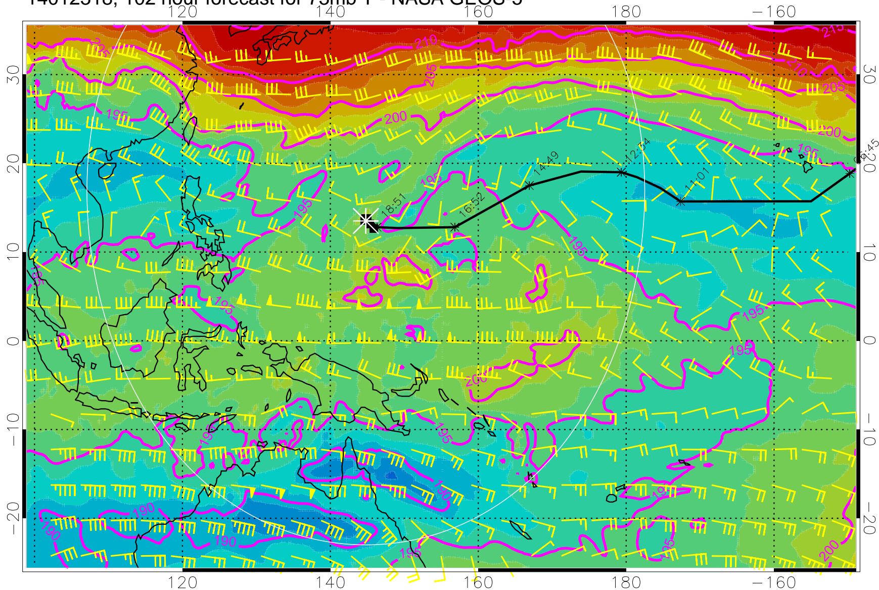
14012318, 102 hour forecast for 73mb T - NASA GEOS-5
