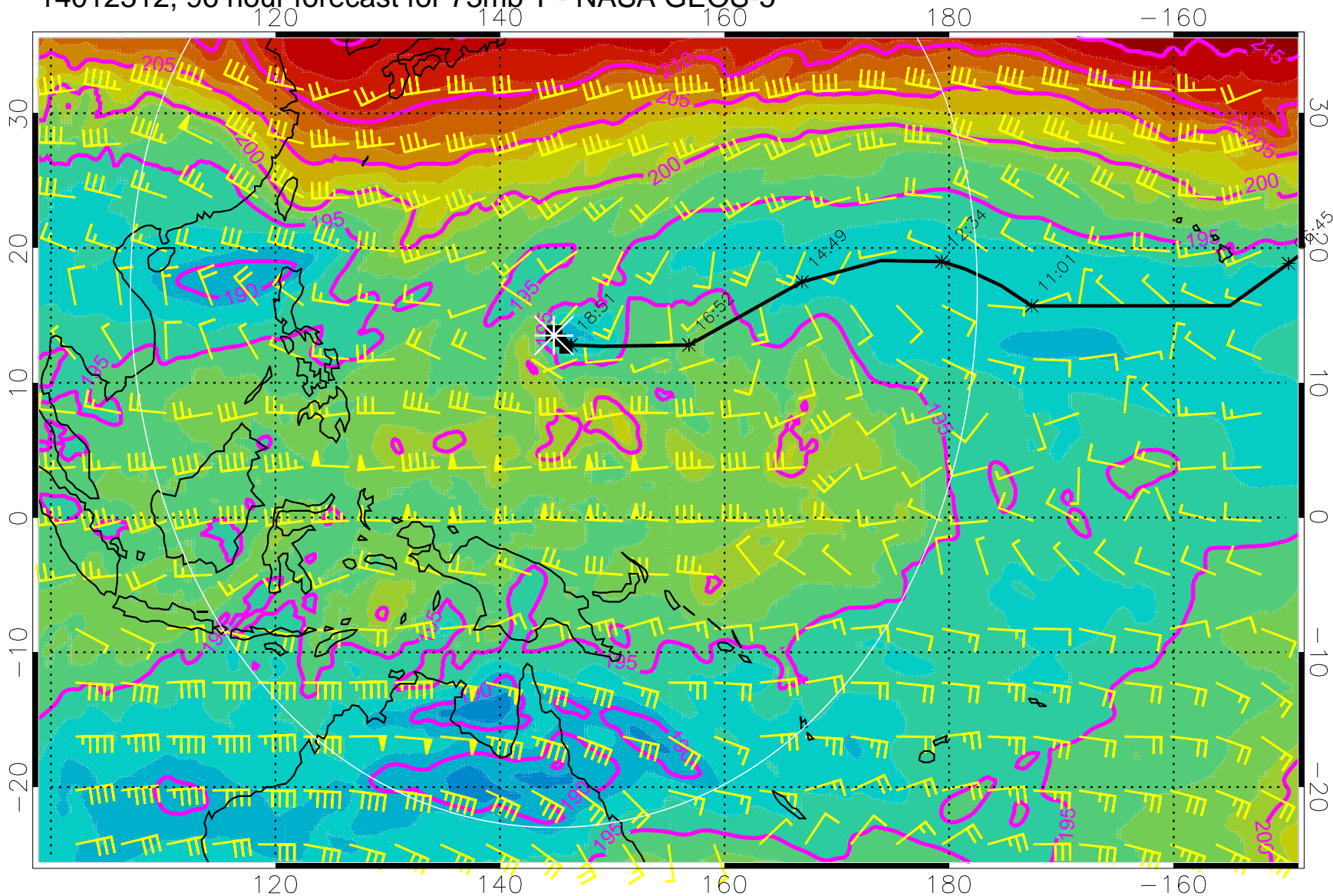
14012312, 96 hour forecast for 73mb T - NASA GEOS-5
