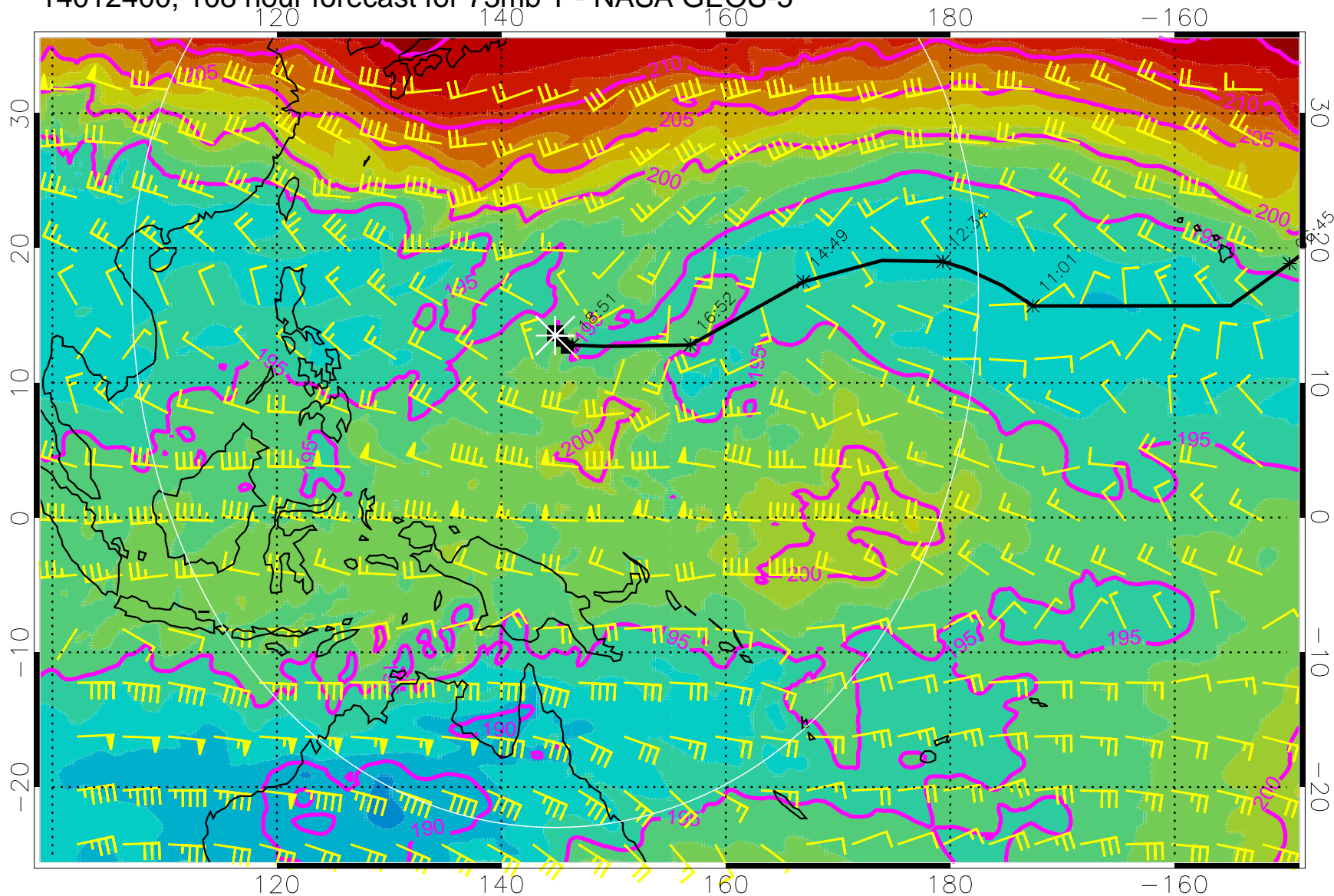
14012400, 108 hour forecast for 73mb T - NASA GEOS-5
