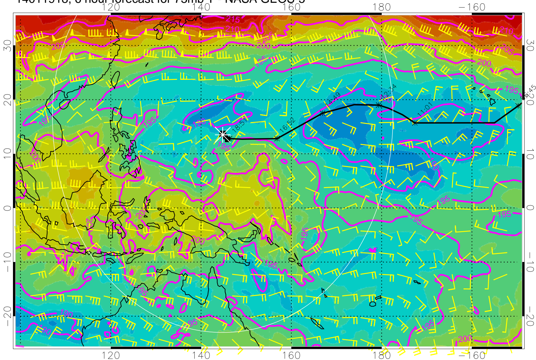
14011918, 6 hour forecast for 73mb T - NASA GEOS-5
