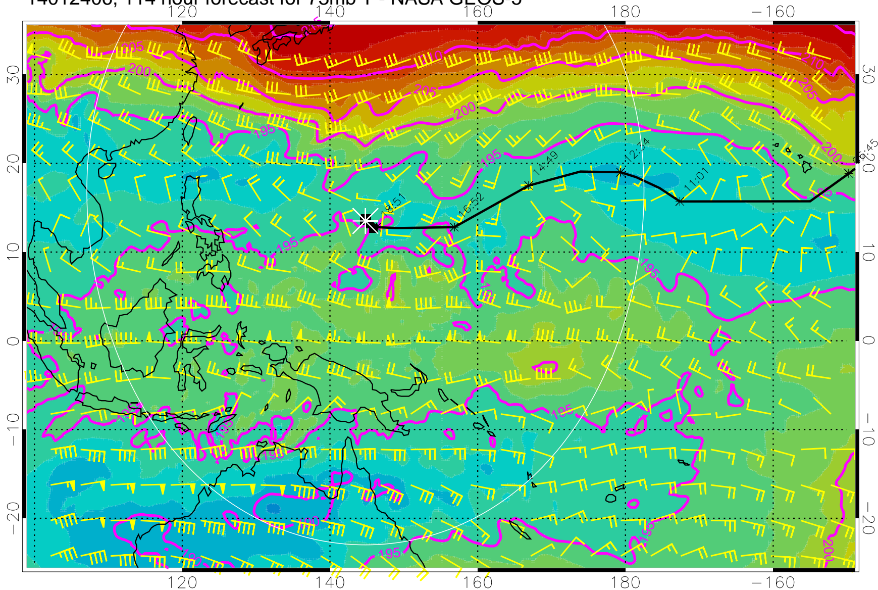
14012406, 114 hour forecast for 73mb T - NASA GEOS-5
