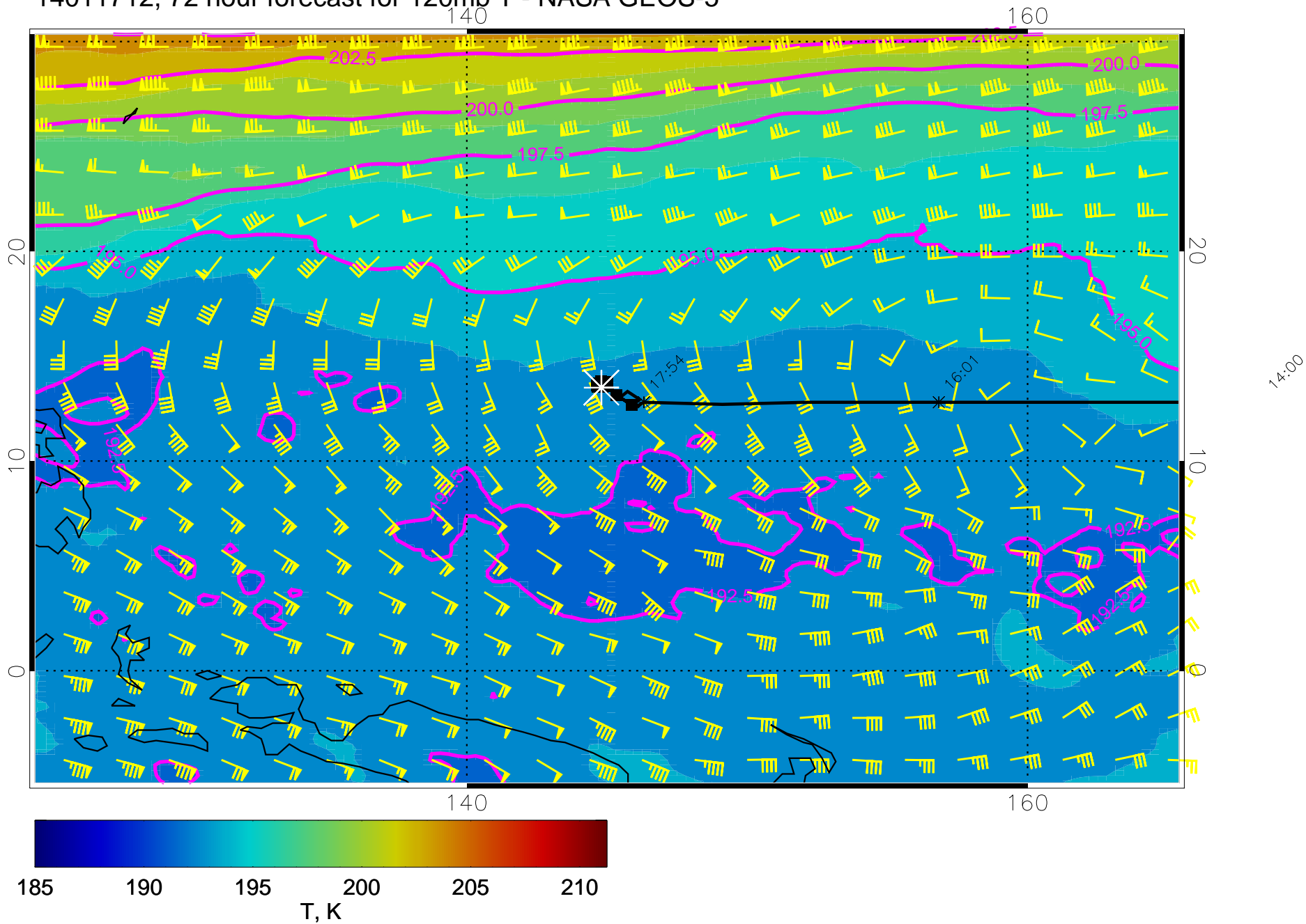
14011712, 72 hour forecast for 120mb T - NASA GEOS-5
