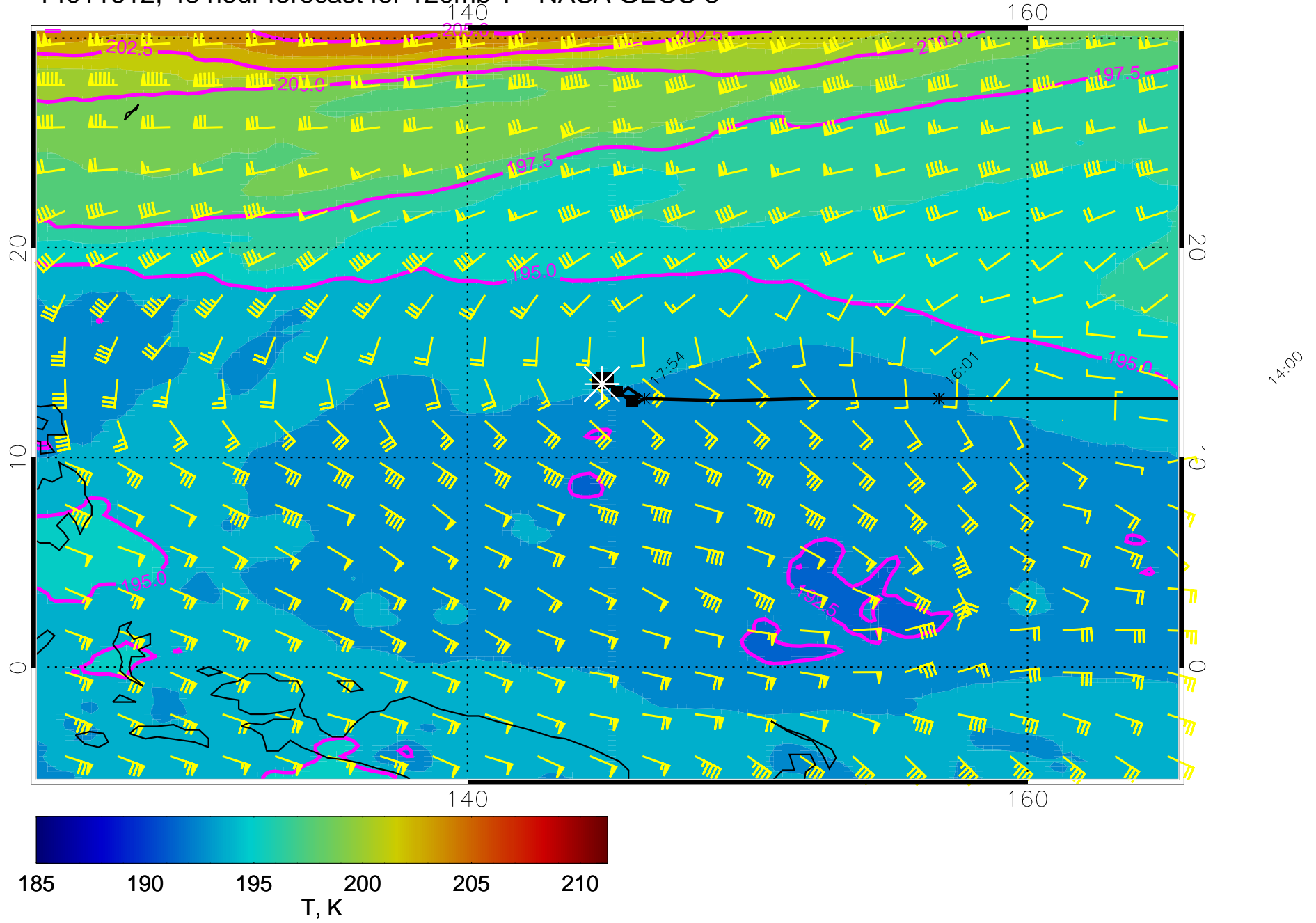
14011612, 48 hour forecast for 120mb T - NASA GEOS-5
