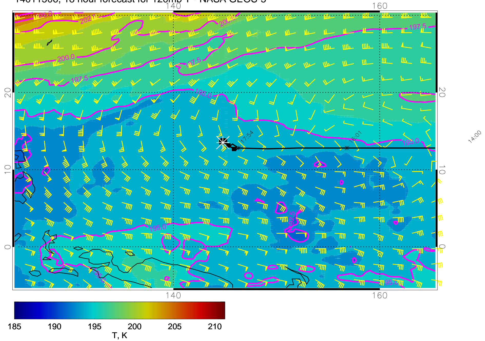
14011506, 18 hour forecast for 120mb T - NASA GEOS-5
