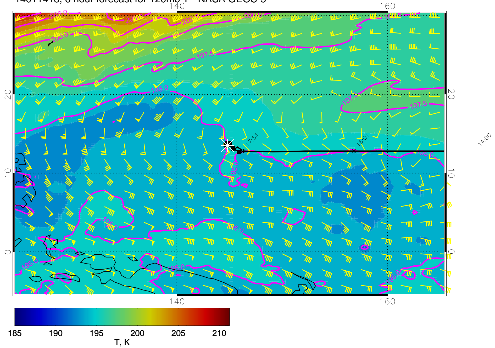
14011418, 6 hour forecast for 120mb T - NASA GEOS-5
