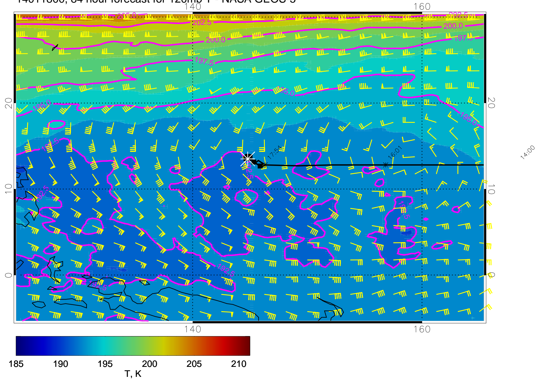
14011800, 84 hour forecast for 120mb T - NASA GEOS-5
