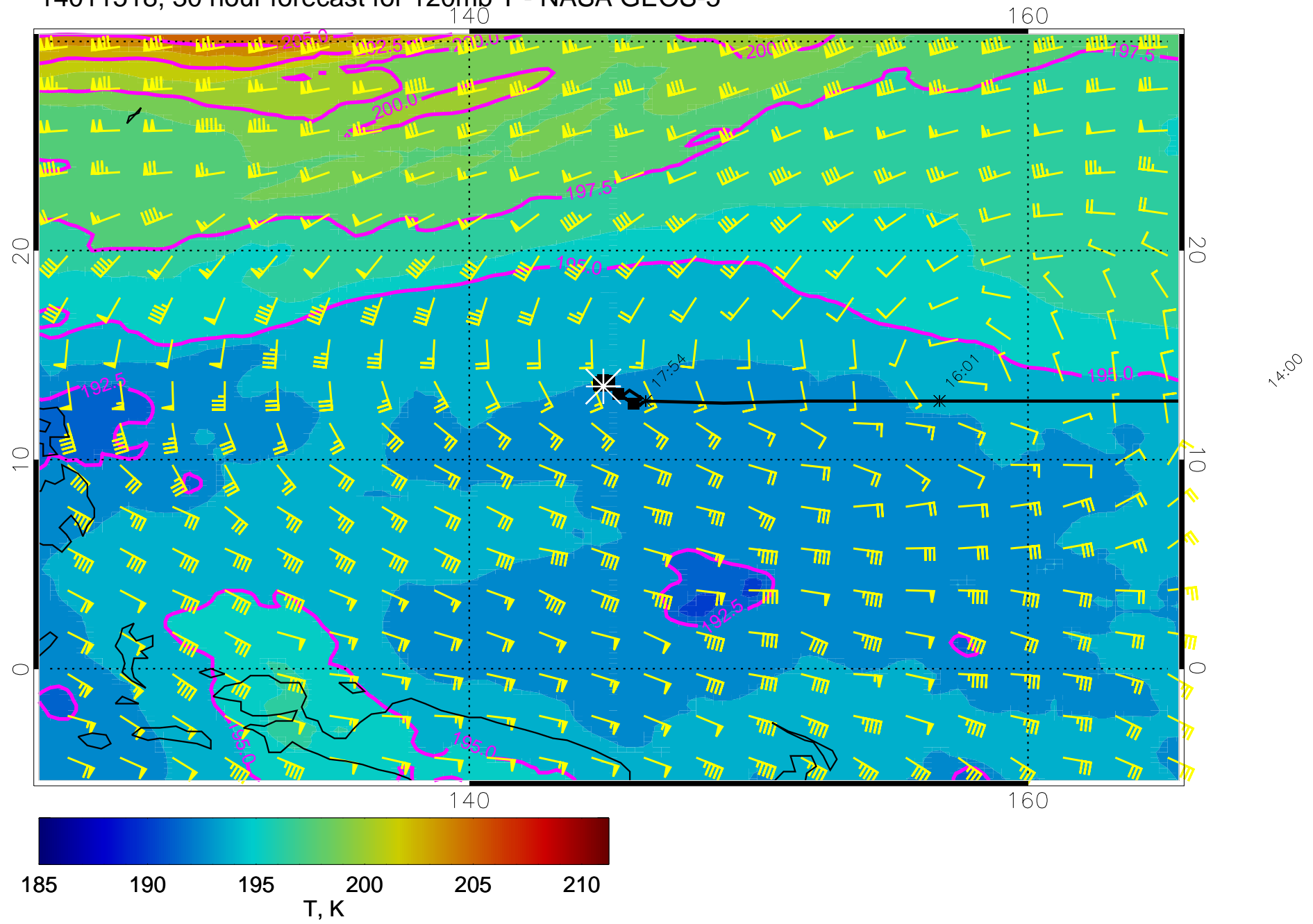
14011518, 30 hour forecast for 120mb T - NASA GEOS-5
