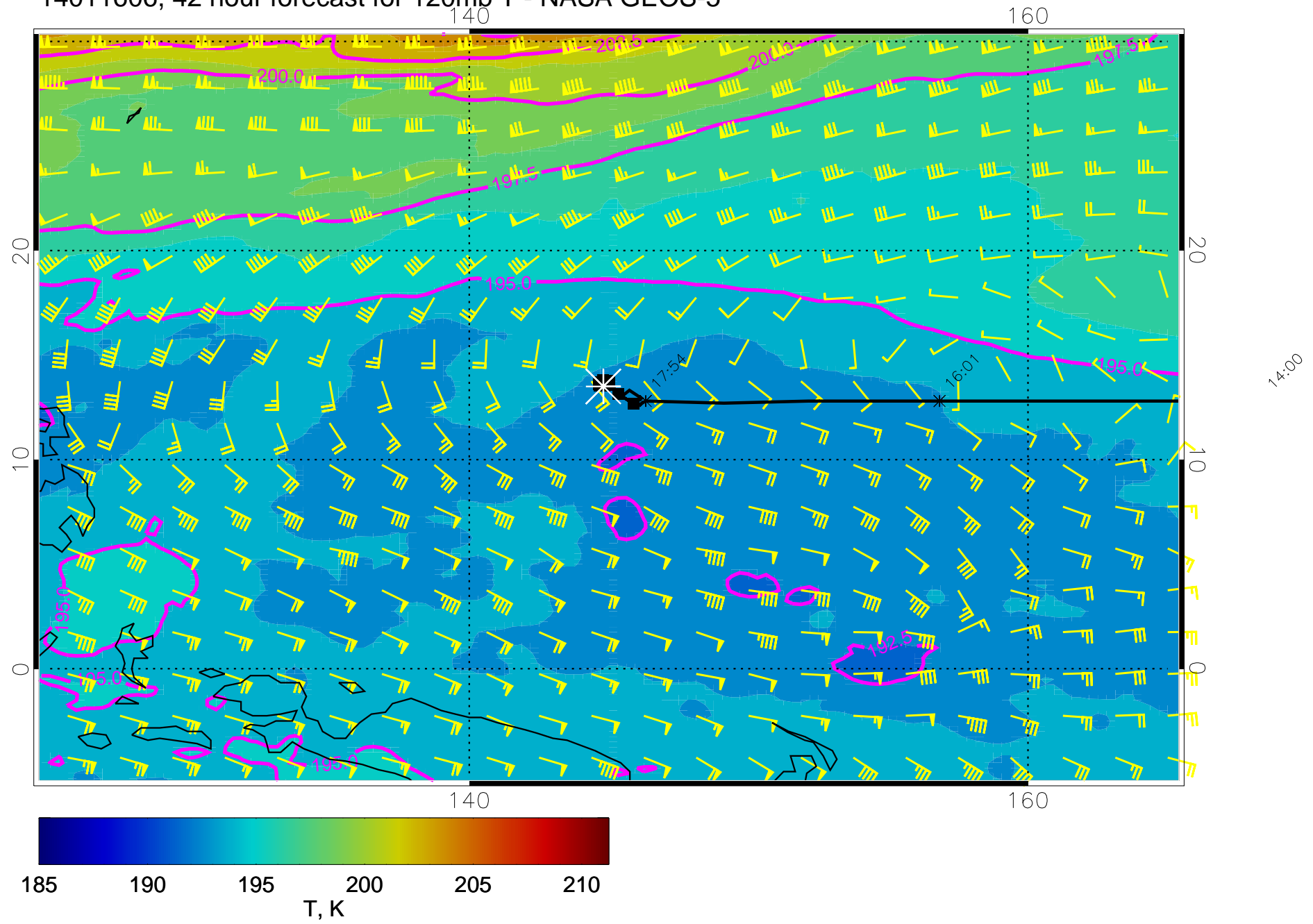
14011606, 42 hour forecast for 120mb T - NASA GEOS-5
