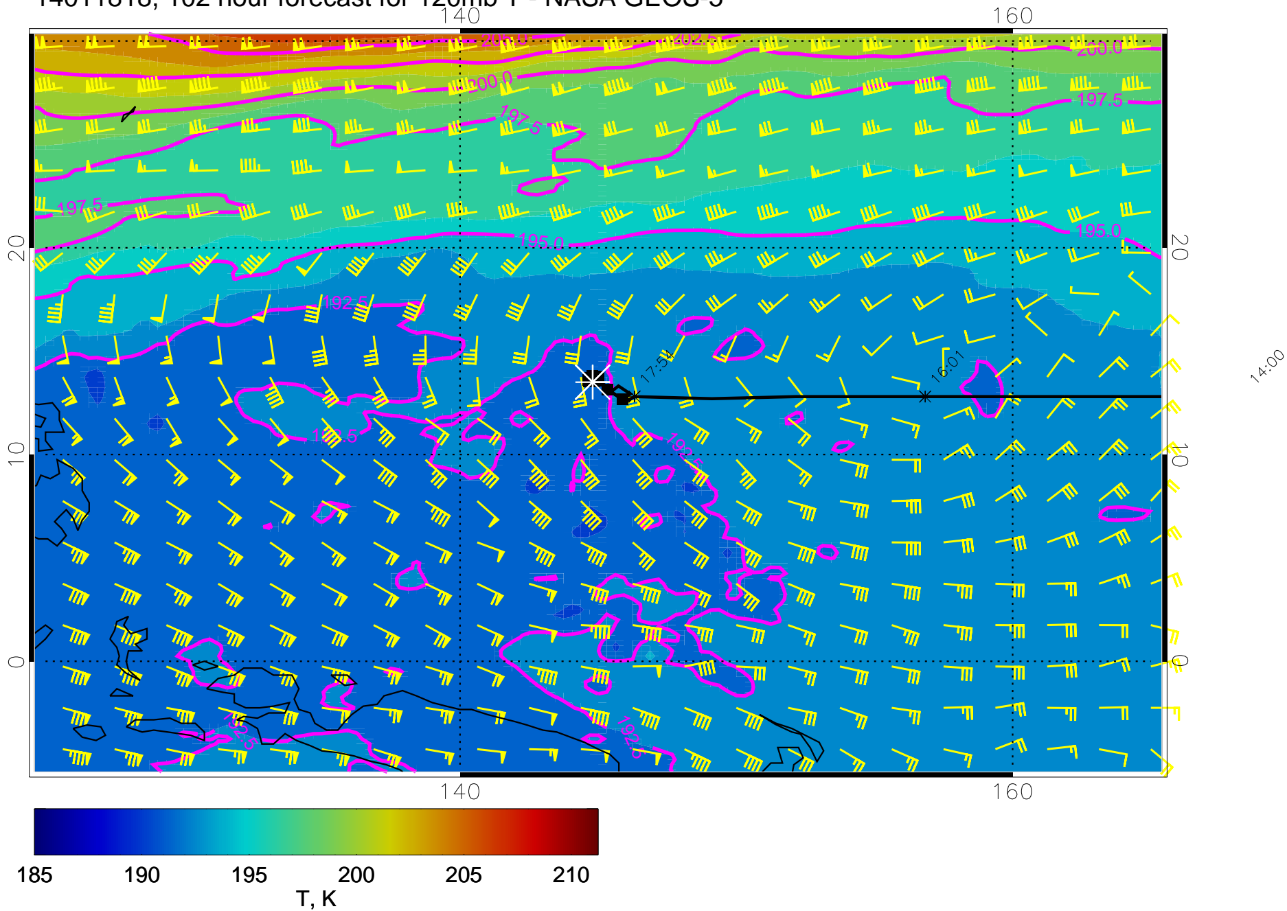
14011818, 102 hour forecast for 120mb T - NASA GEOS-5
