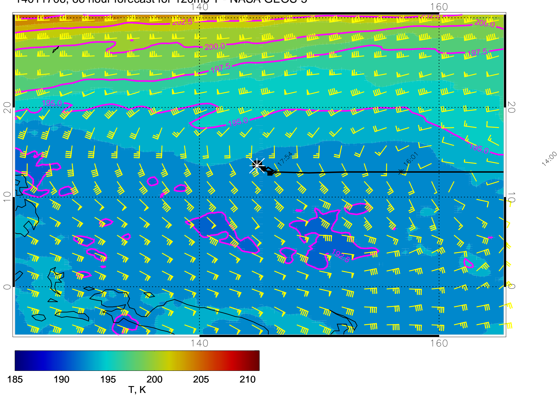
14011706, 66 hour forecast for 120mb T - NASA GEOS-5
