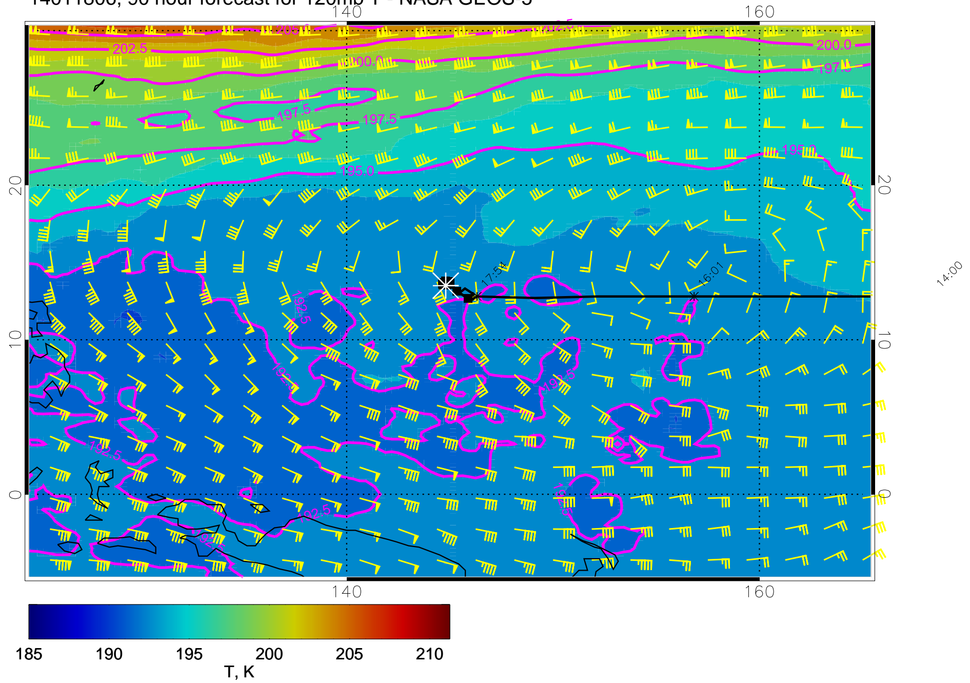
14011806, 90 hour forecast for 120mb T - NASA GEOS-5
