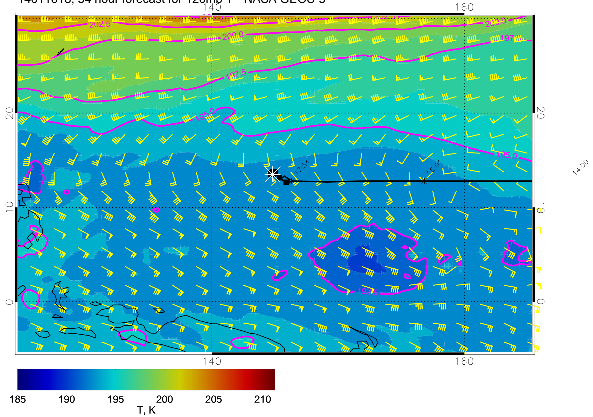
14011618, 54 hour forecast for 120mb T - NASA GEOS-5
