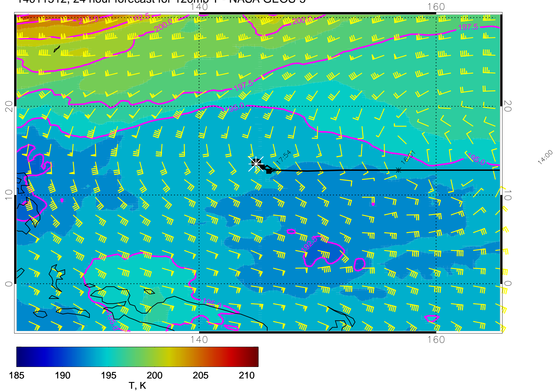
14011512, 24 hour forecast for 120mb T - NASA GEOS-5
