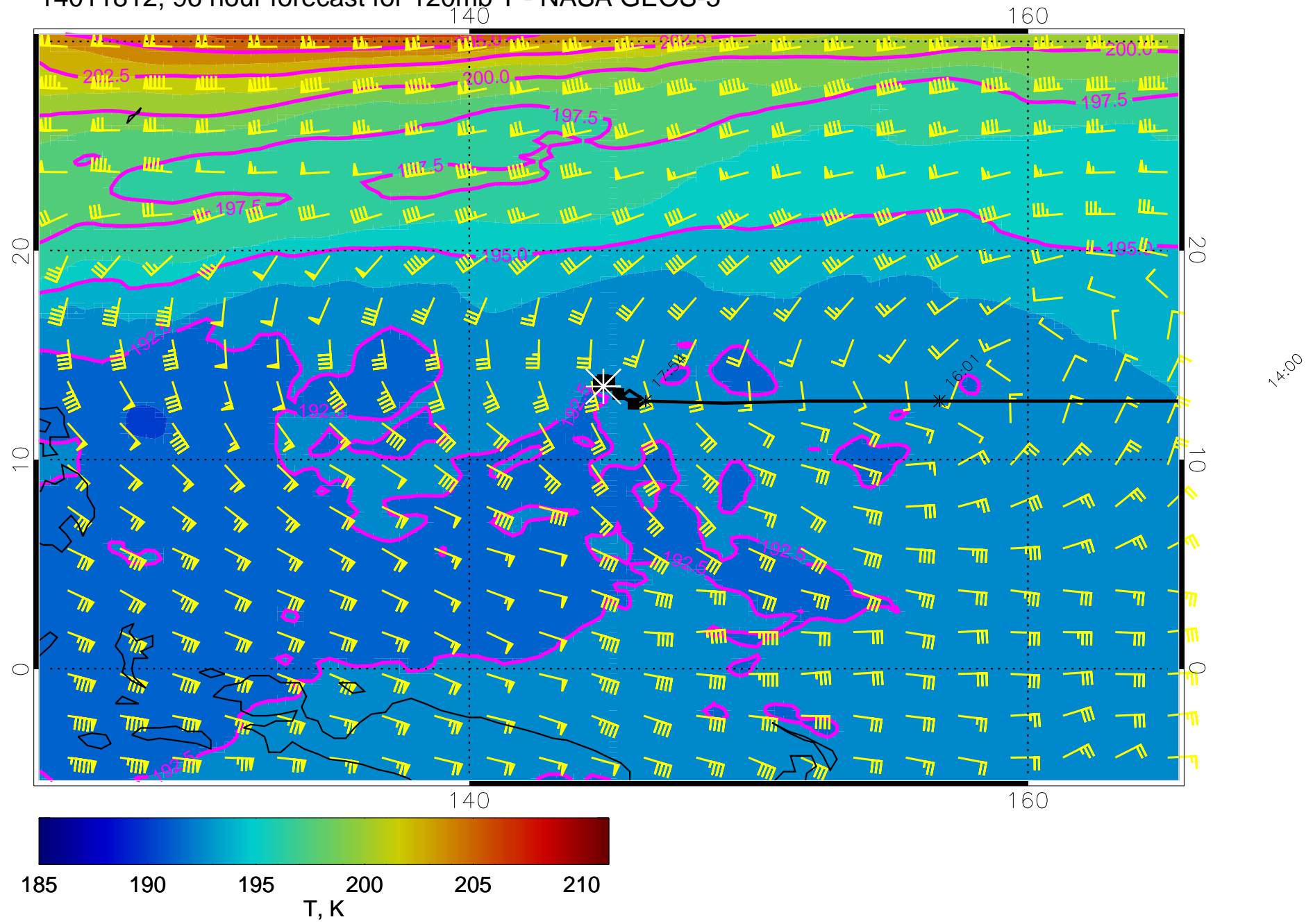
14011812, 96 hour forecast for 120mb T - NASA GEOS-5
