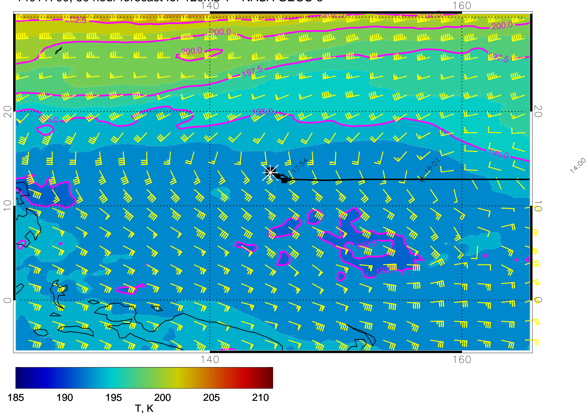
14011700, 60 hour forecast for 120mb T - NASA GEOS-5
