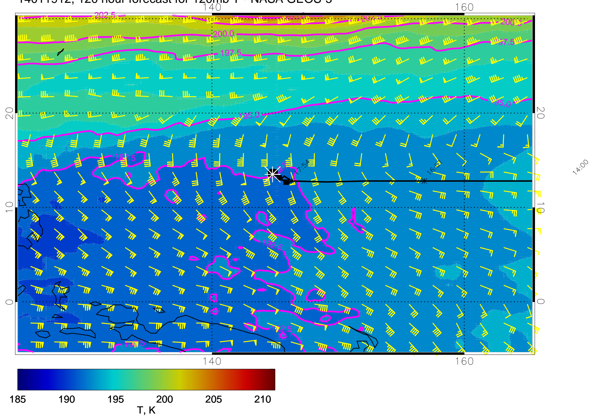
14011912, 120 hour forecast for 120mb T - NASA GEOS-5
