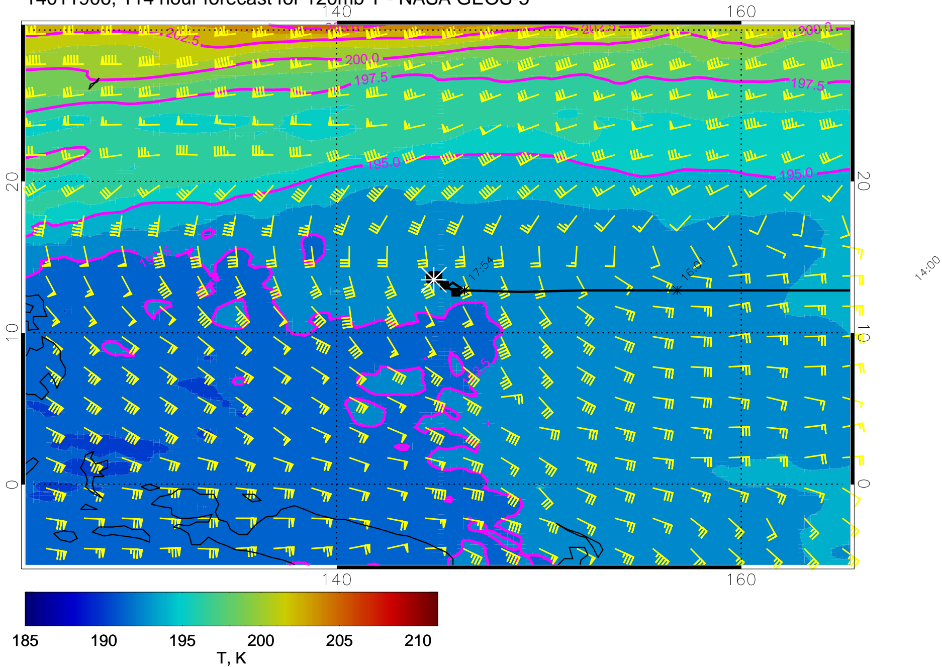
14011906, 114 hour forecast for 120mb T - NASA GEOS-5
