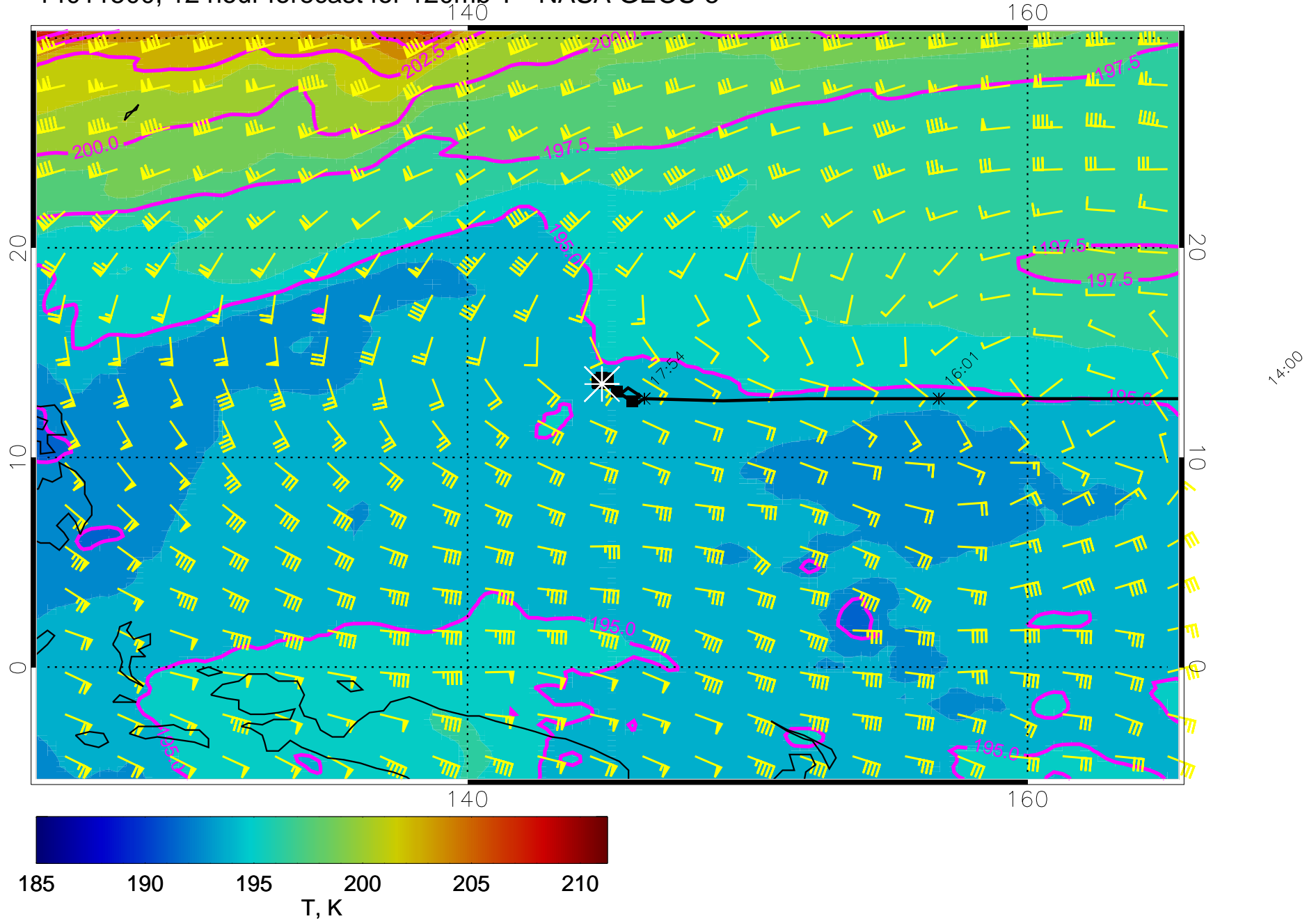
14011500, 12 hour forecast for 120mb T - NASA GEOS-5
