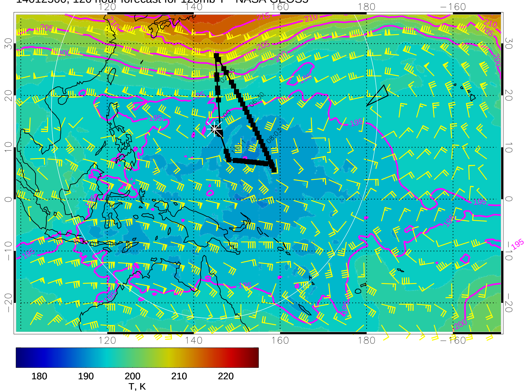
14012500, 120 hour forecast for 120mb T - NASA GEOS5
