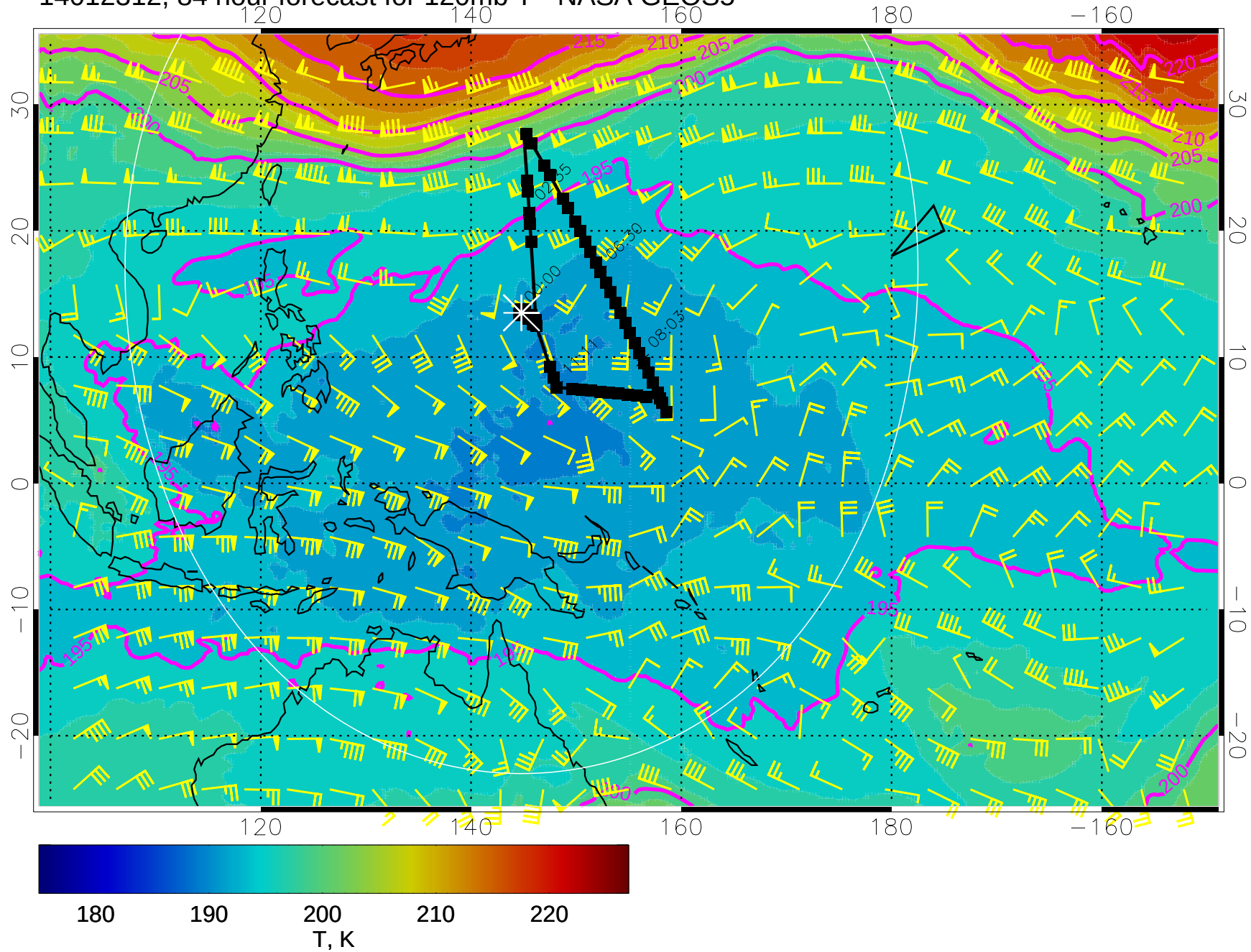
14012312, 84 hour forecast for 120mb T - NASA GEOS5
