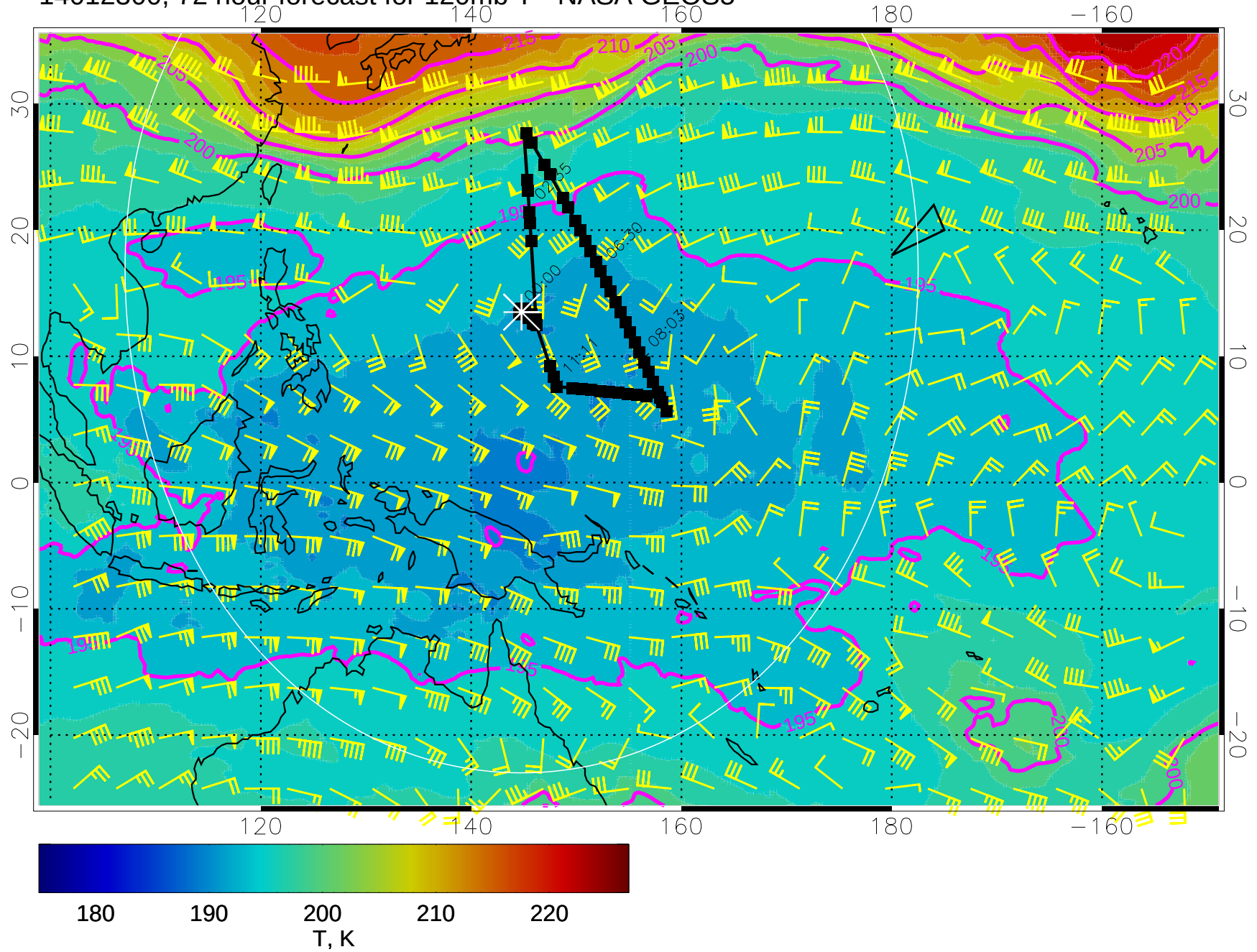
14012300, 72 hour forecast for 120mb T - NASA GEOS5
