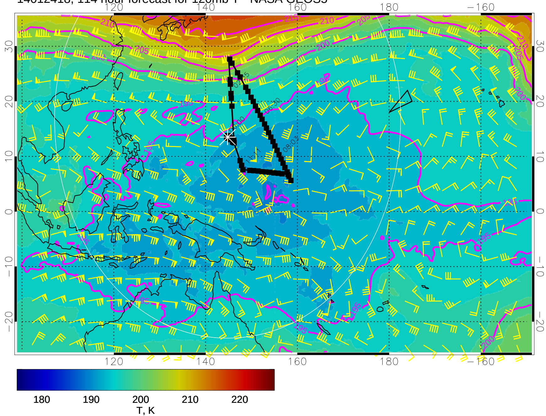
14012418, 114 hour forecast for 120mb T - NASA GEOS5
