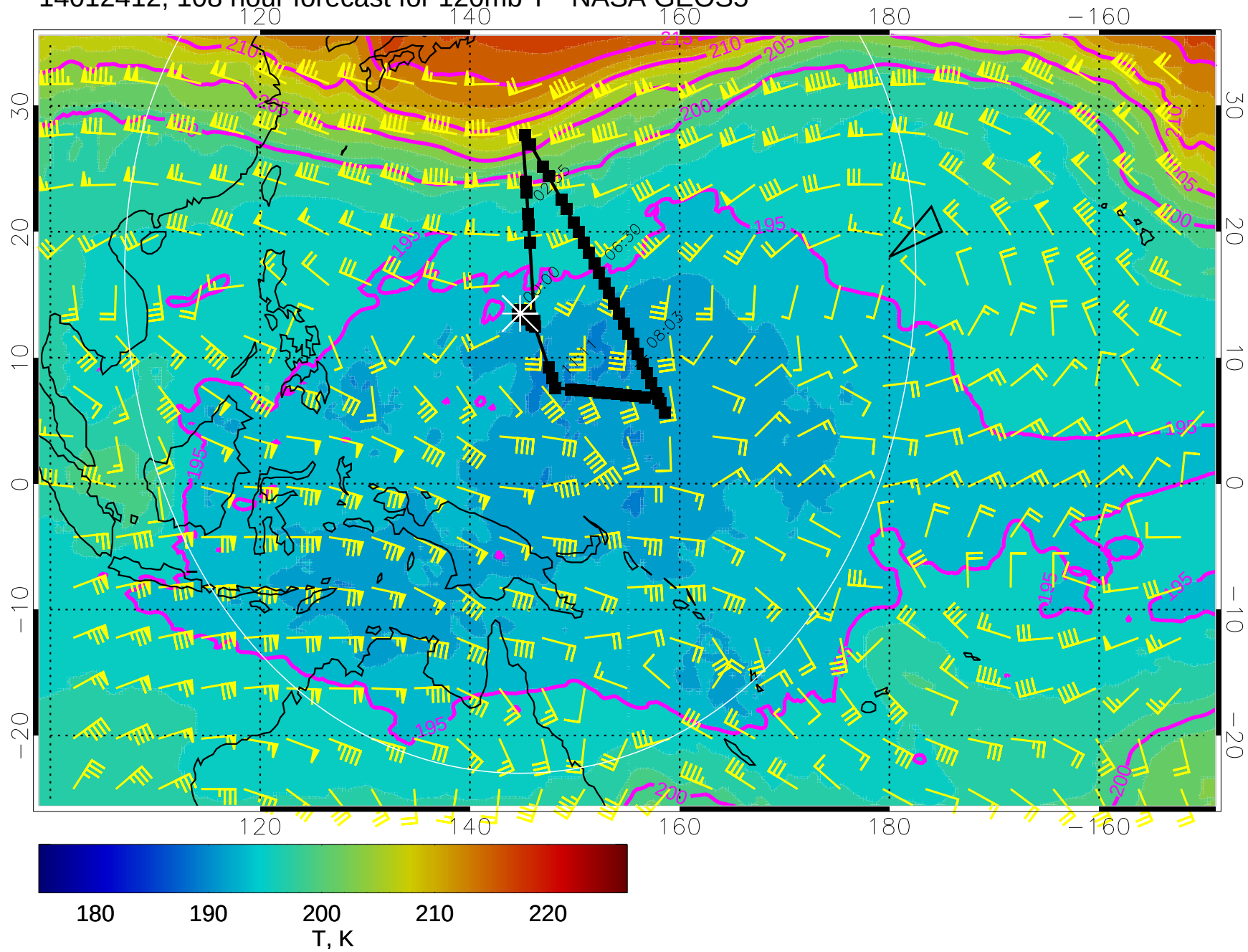
14012412, 108 hour forecast for 120mb T - NASA GEOS5
