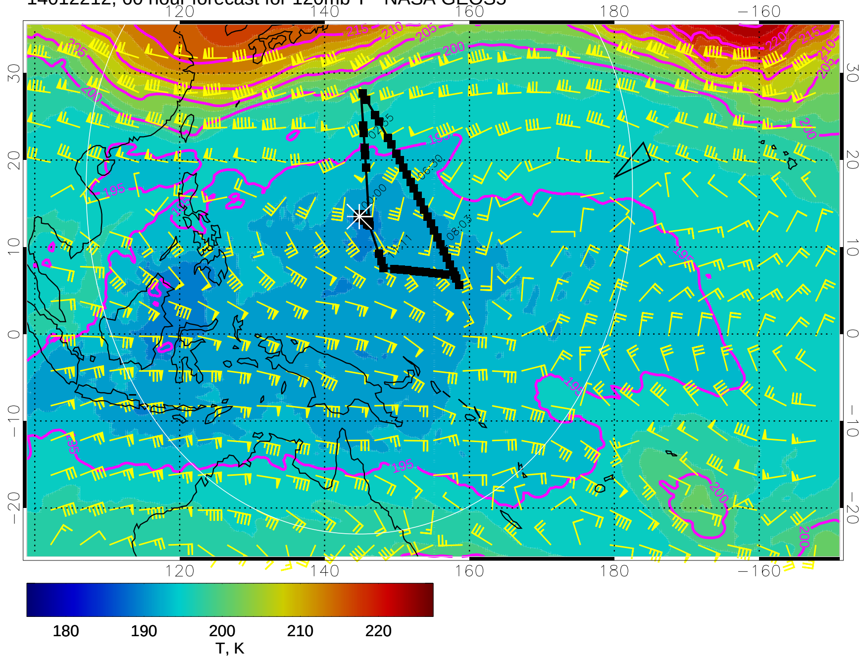
14012212, 60 hour forecast for 120mb T - NASA GEOS5
