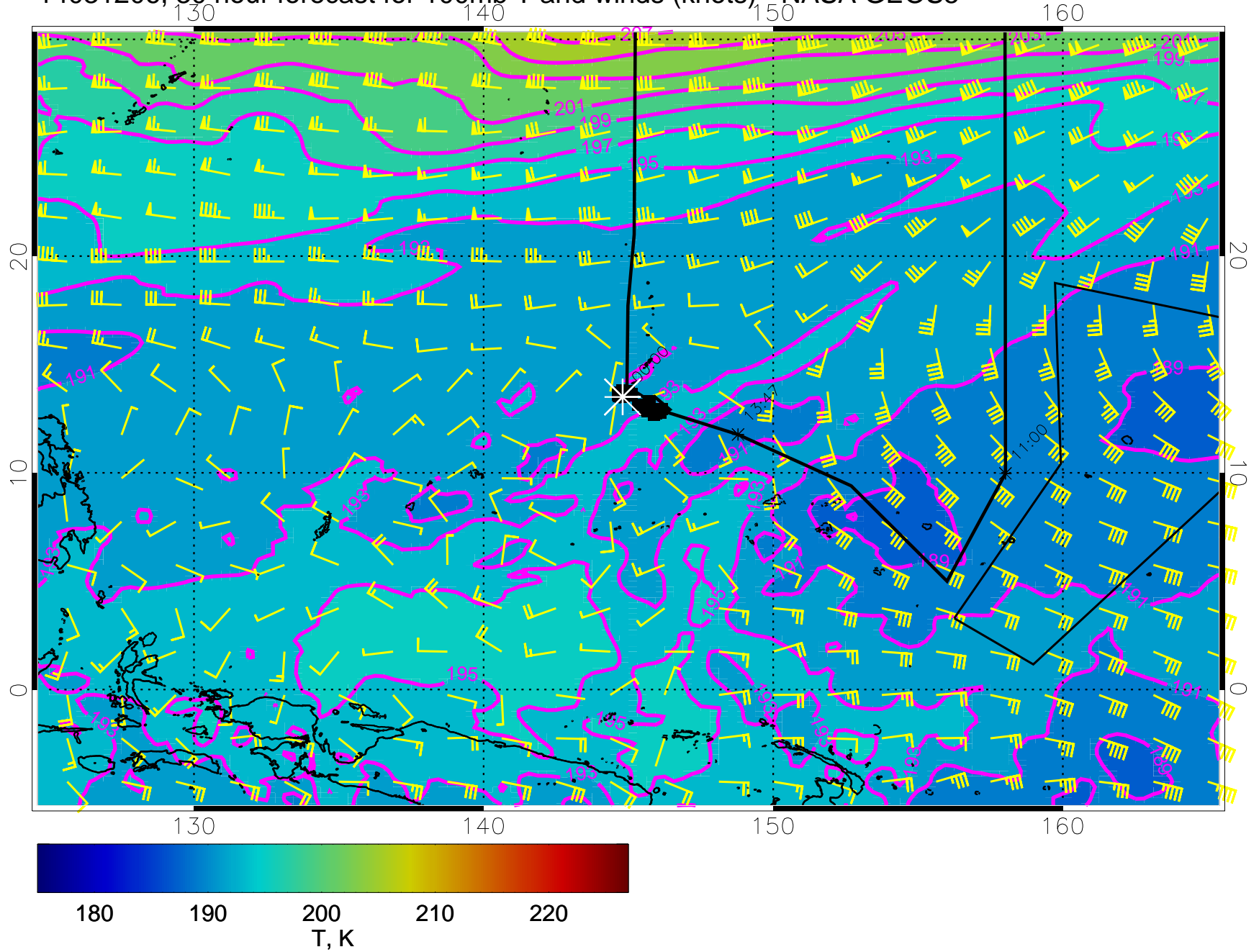
14031206, 30 hour forecast for 100mb T and winds (knots) - NASA GEOS5
