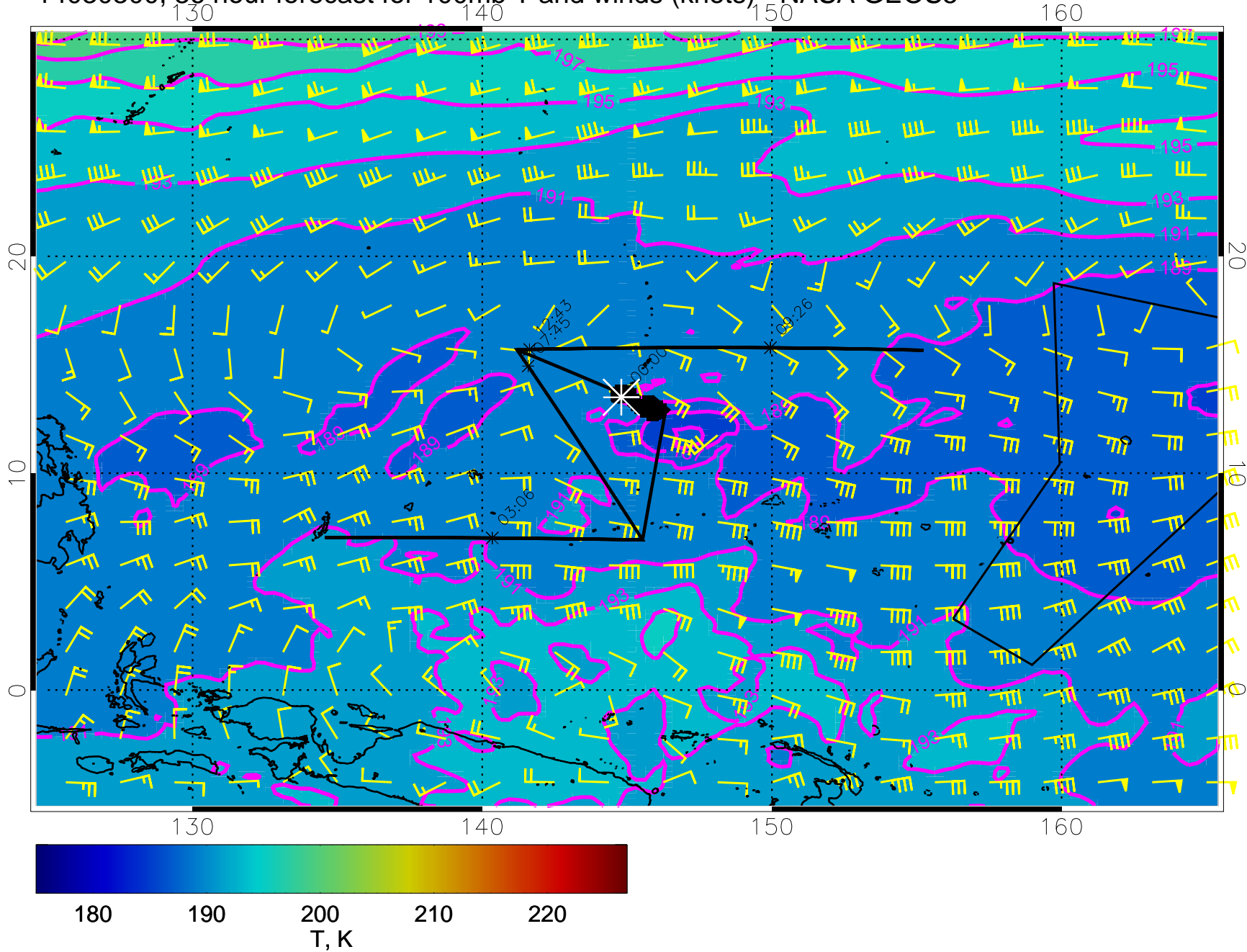
14030300, 36 hour forecast for 100mb T and winds (knots) - NASA GEOS5
