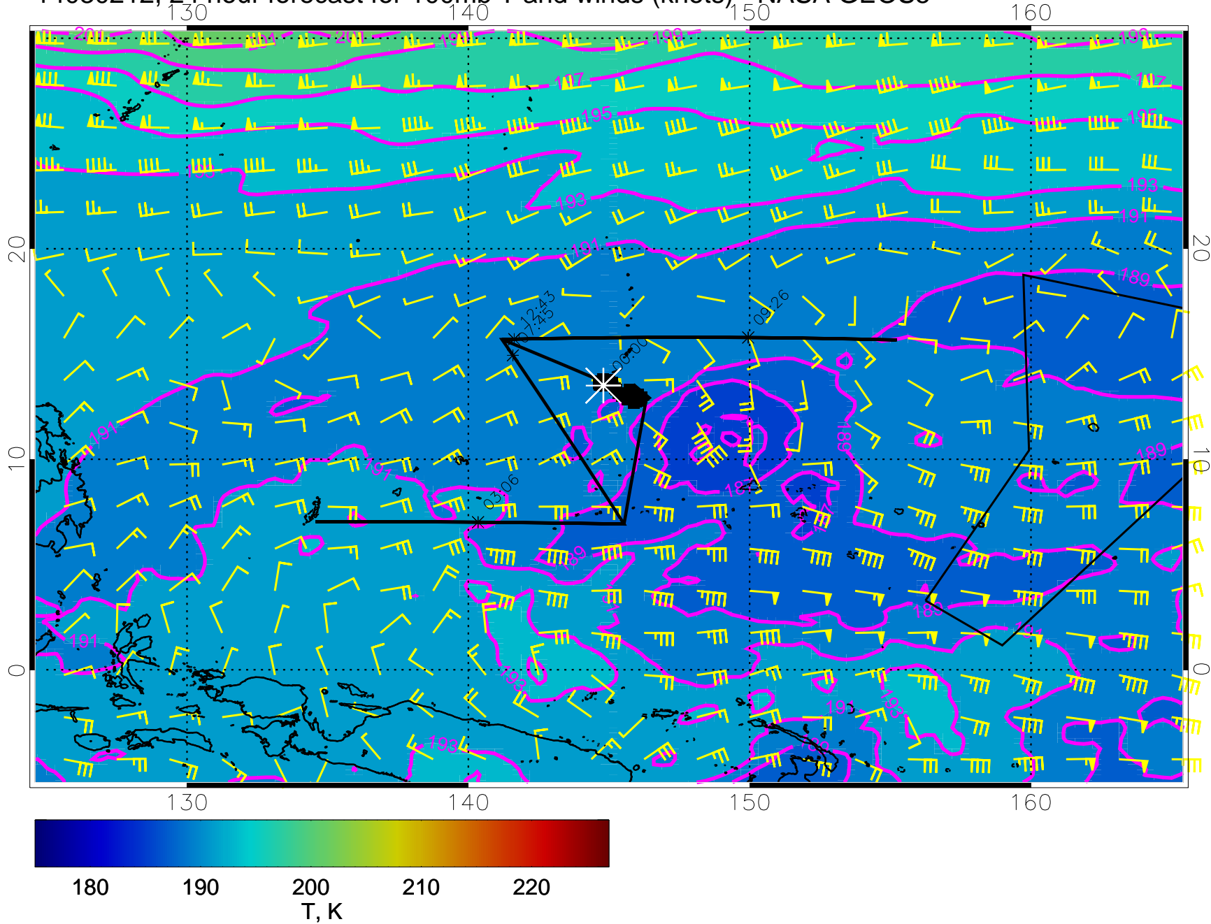
14030212, 24 hour forecast for 100mb T and winds (knots) - NASA GEOS5
