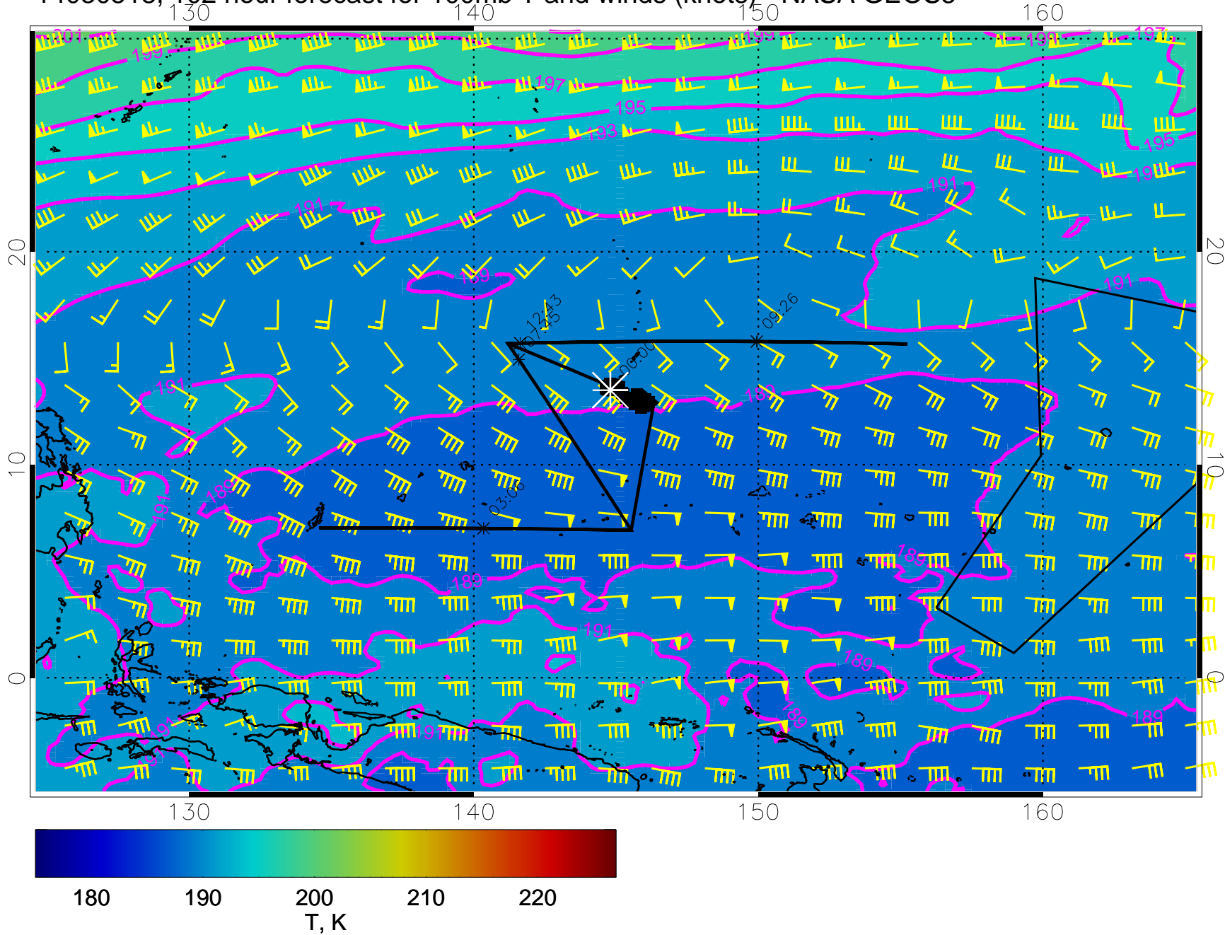
14030518, 102 hour forecast for 100mb T and winds (knots) - NASA GEOS5
