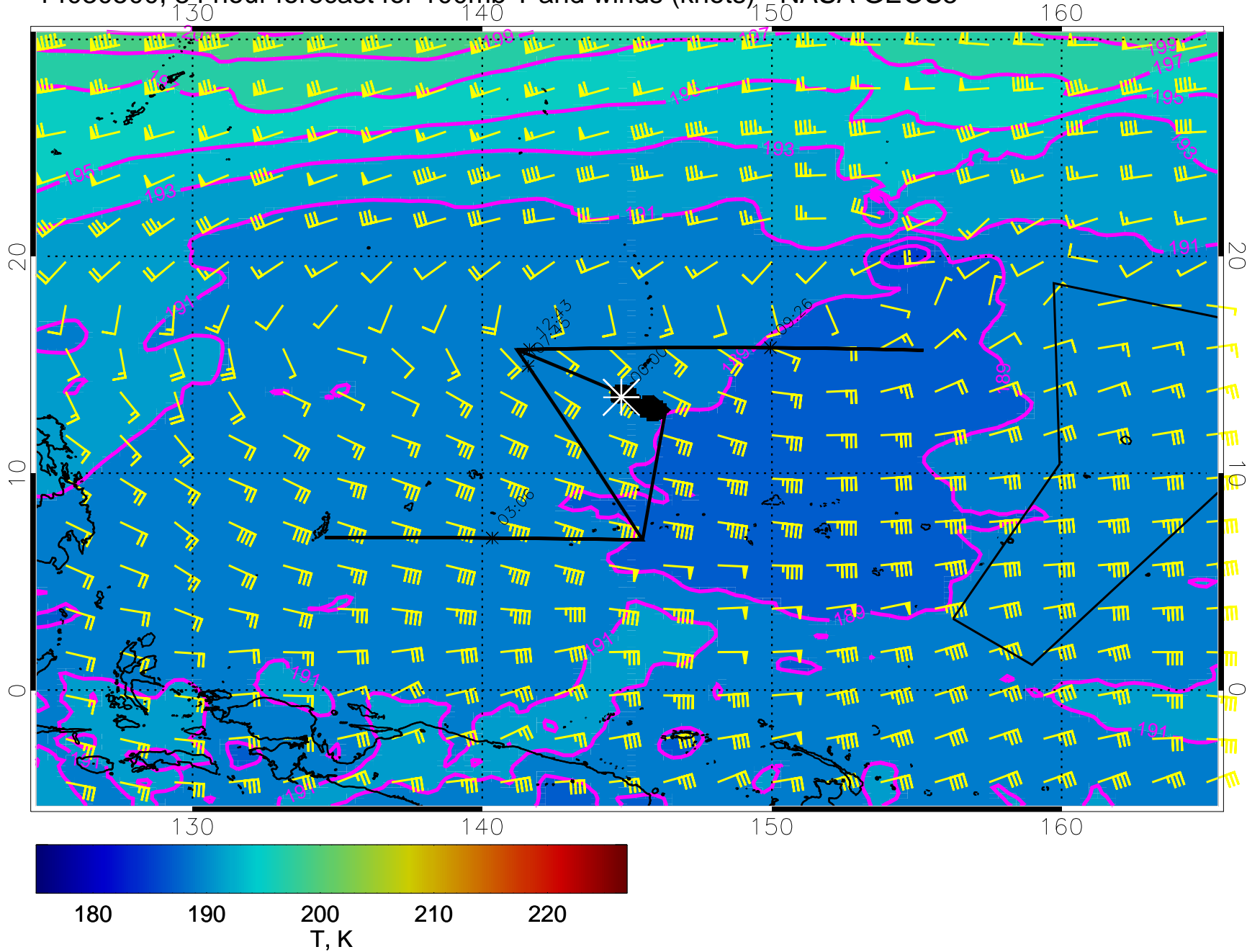
14030500, 84 hour forecast for 100mb T and winds (knots) - NASA GEOS5
