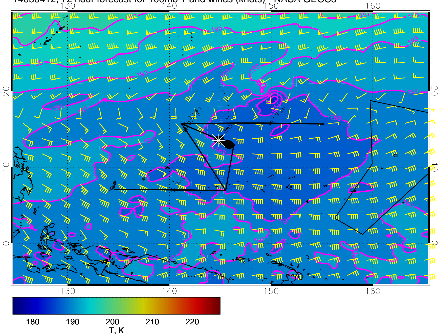
14030412, 72 hour forecast for 100mb T and winds (knots) - NASA GEOS5
