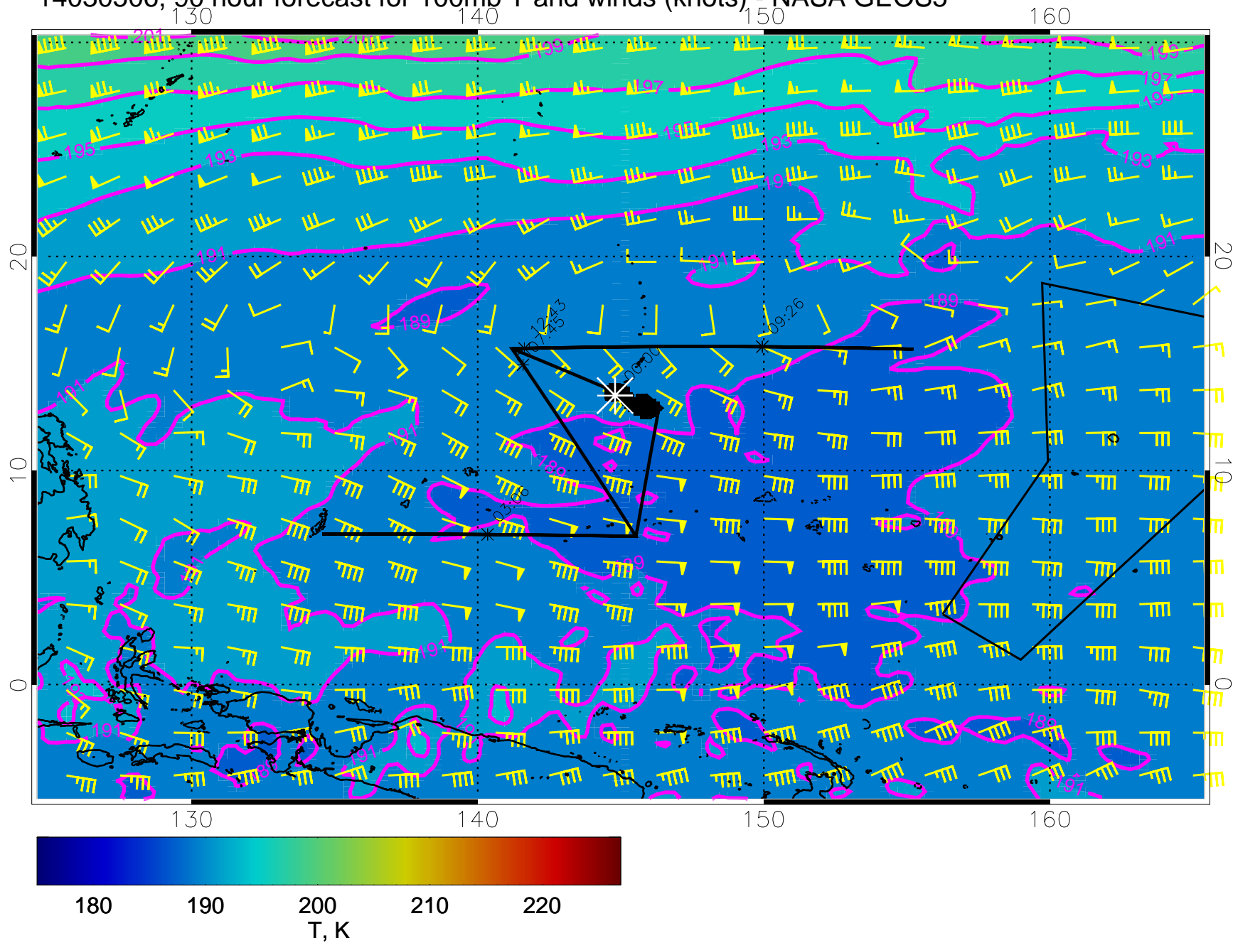
14030506, 90 hour forecast for 100mb T and winds (knots) - NASA GEOS5
