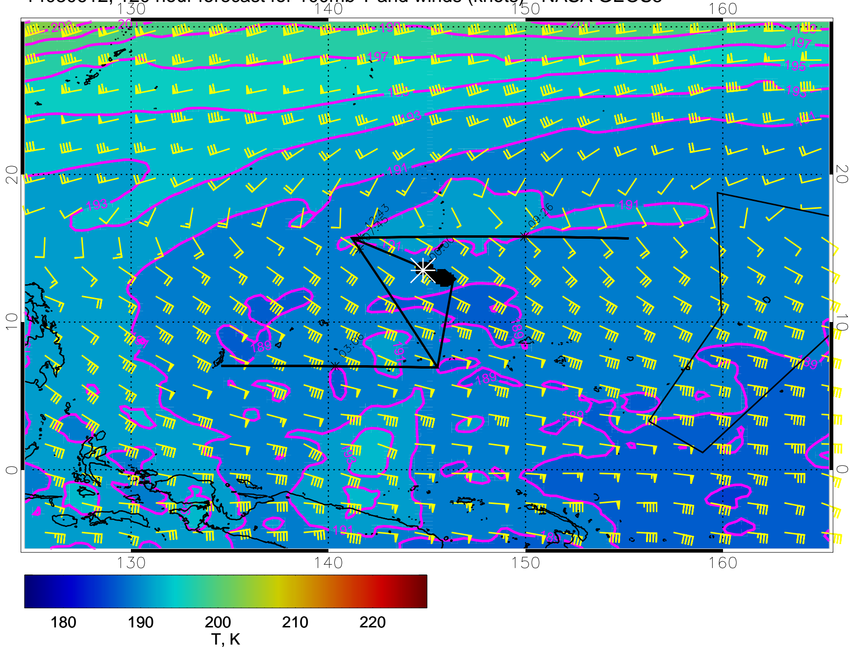
14030612, 120 hour forecast for 100mb T and winds (knots) - NASA GEOS5
