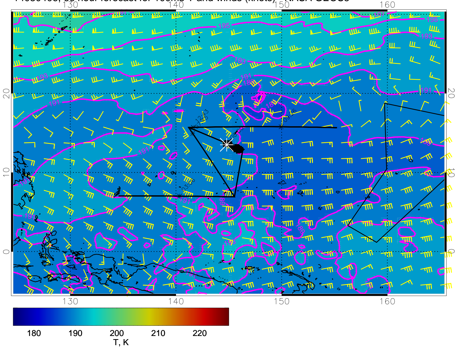
14030406, 66 hour forecast for 100mb T and winds (knots) - NASA GEOS5
