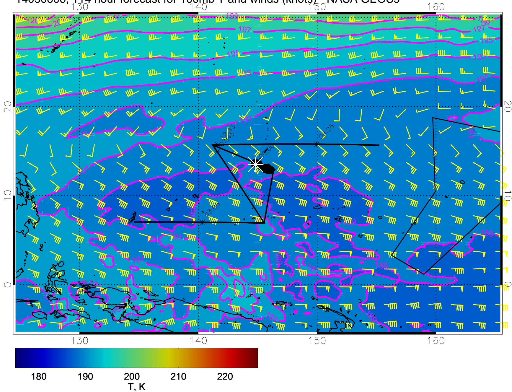
14030606, 114 hour forecast for 100mb T and winds (knots) - NASA GEOS5
