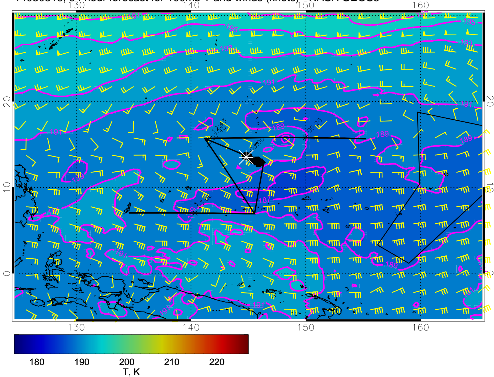
14030318, 54 hour forecast for 100mb T and winds (knots) - NASA GEOS5
