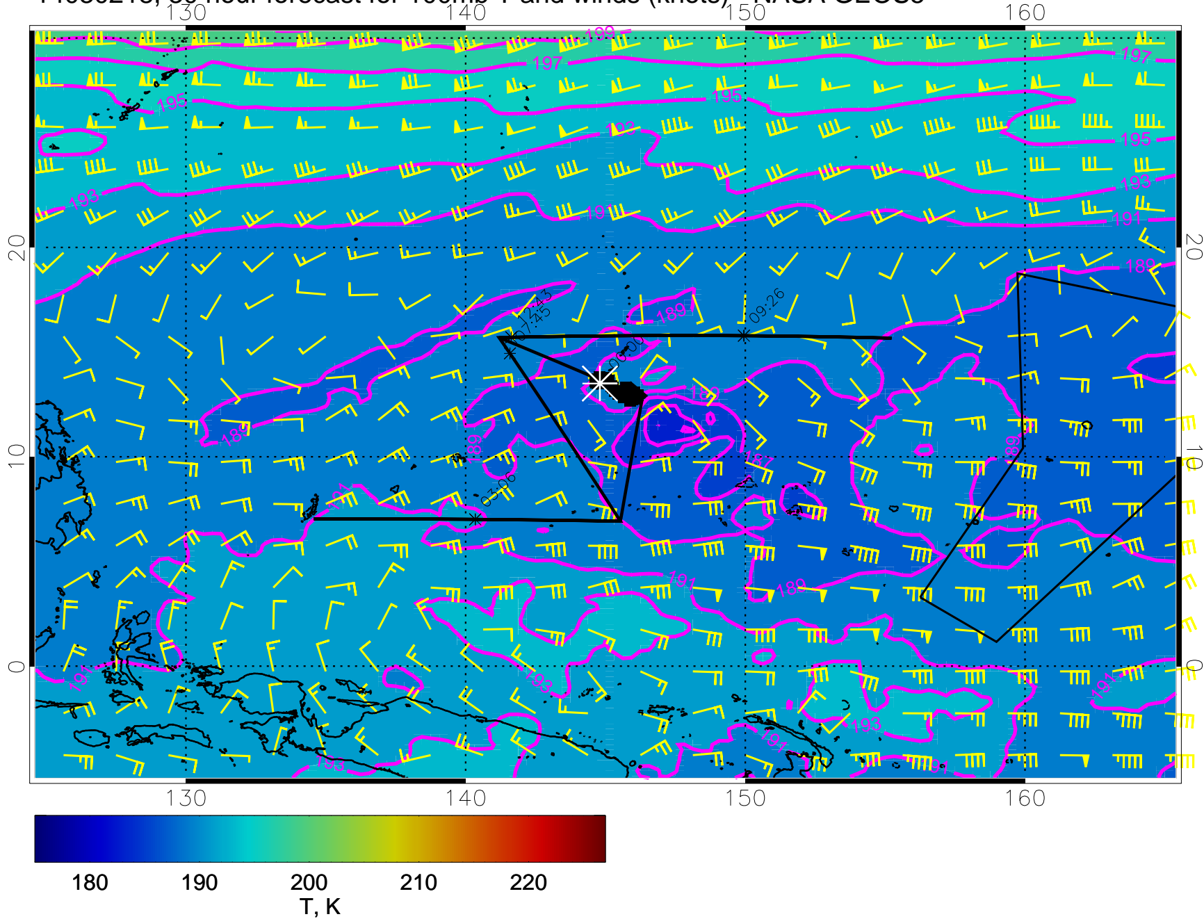
14030218, 30 hour forecast for 100mb T and winds (knots) - NASA GEOS5
