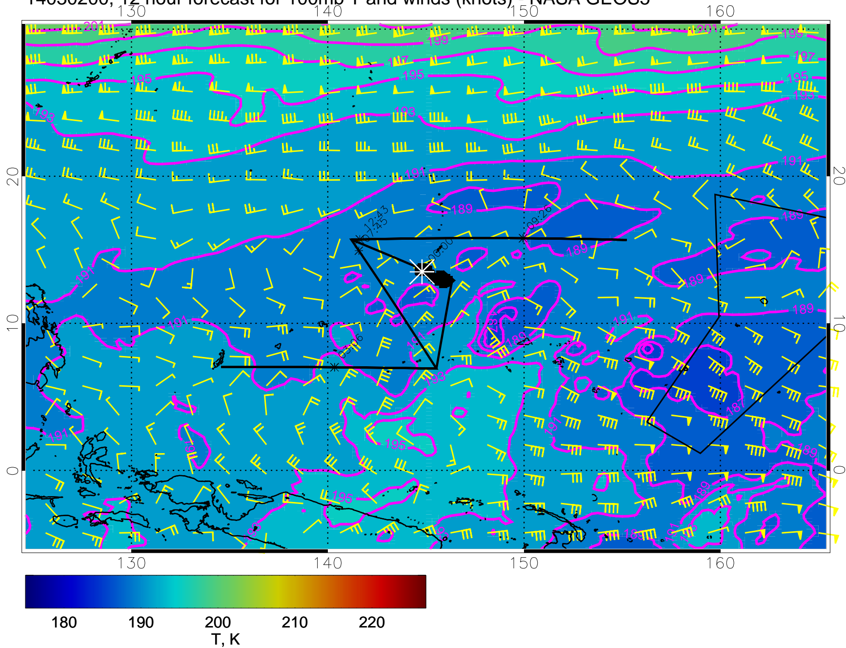
14030200, 12 hour forecast for 100mb T and winds (knots) - NASA GEOS5
