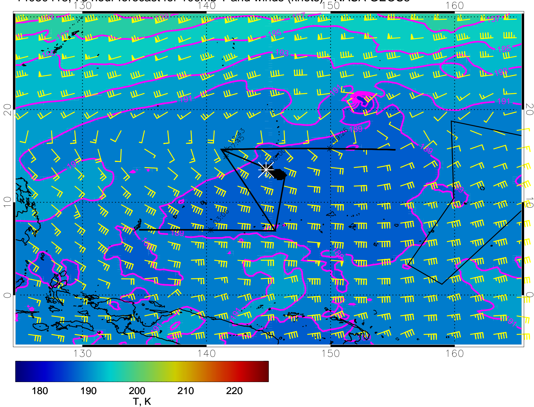
14030418, 78 hour forecast for 100mb T and winds (knots) - NASA GEOS5
