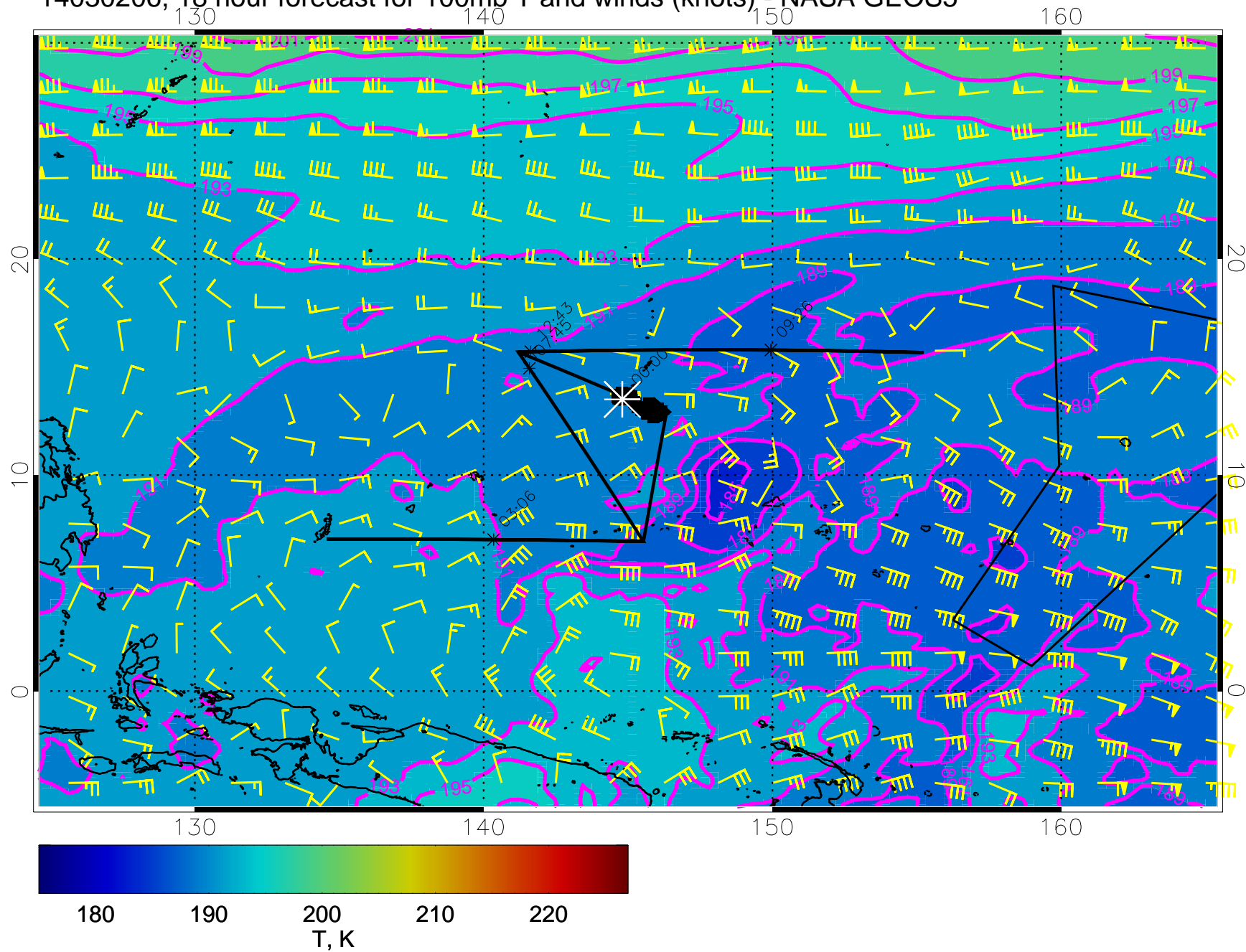
14030206, 18 hour forecast for 100mb T and winds (knots) - NASA GEOS5
