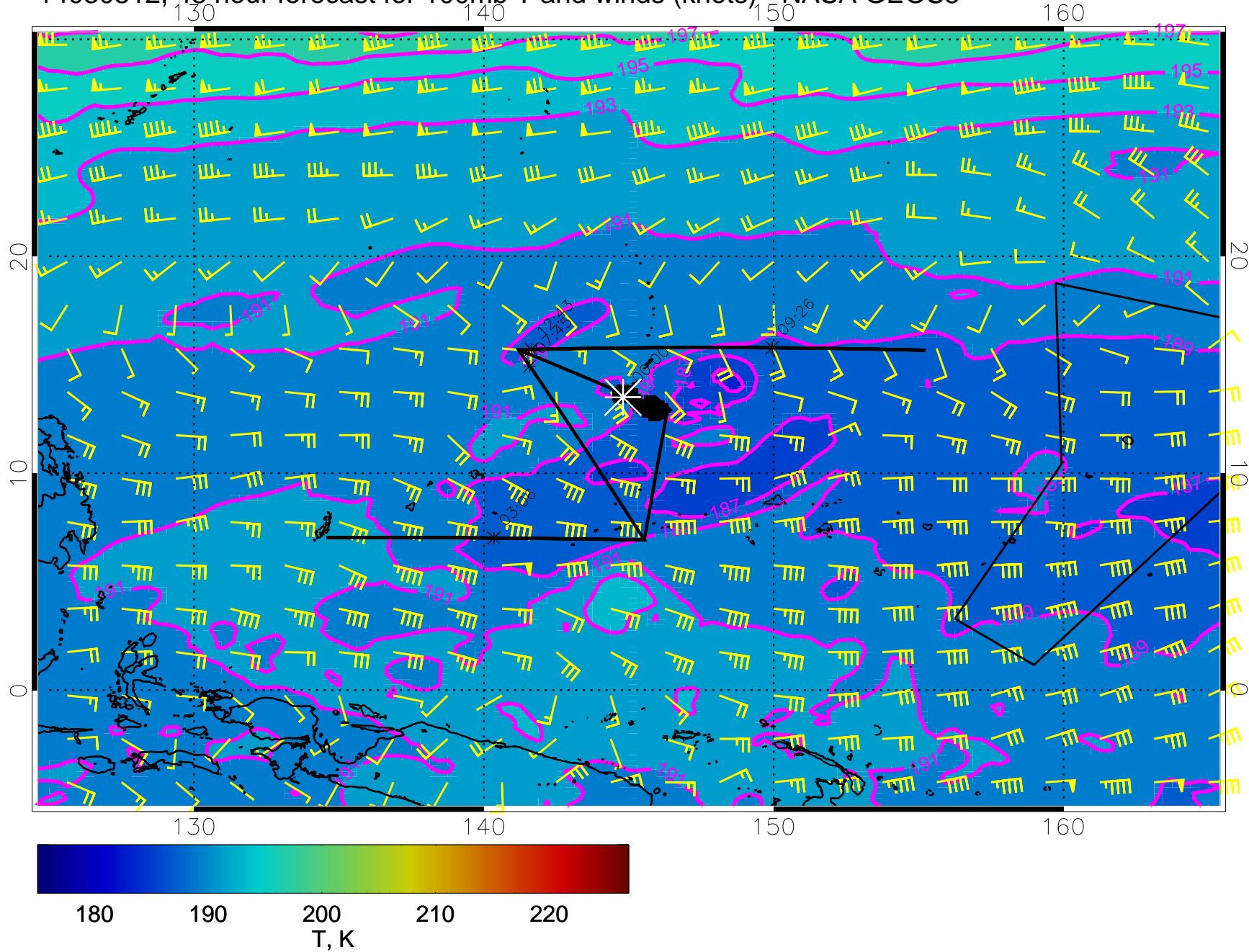
14030312, 48 hour forecast for 100mb T and winds (knots) - NASA GEOS5
