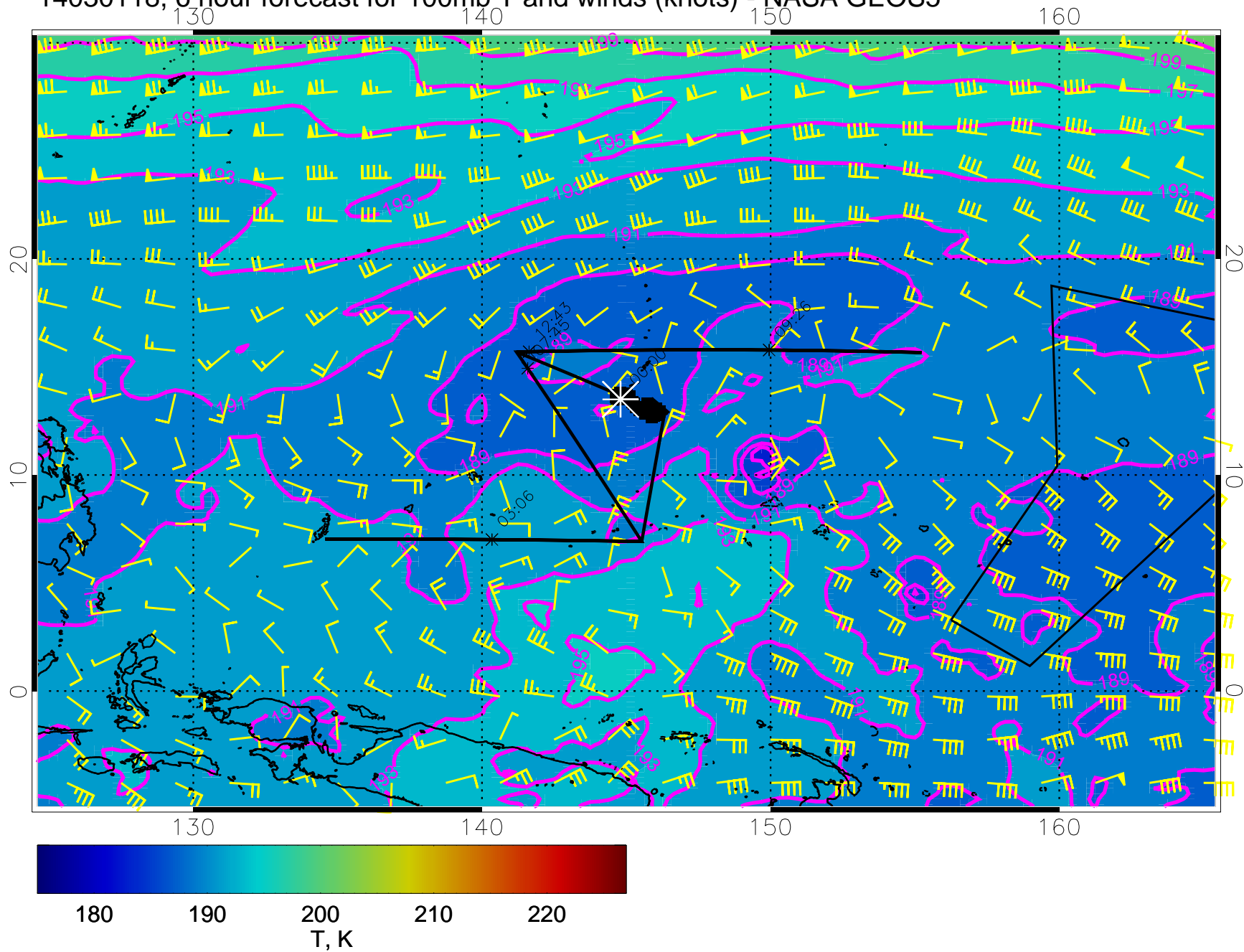
14030118, 6 hour forecast for 100mb T and winds (knots) - NASA GEOS5
