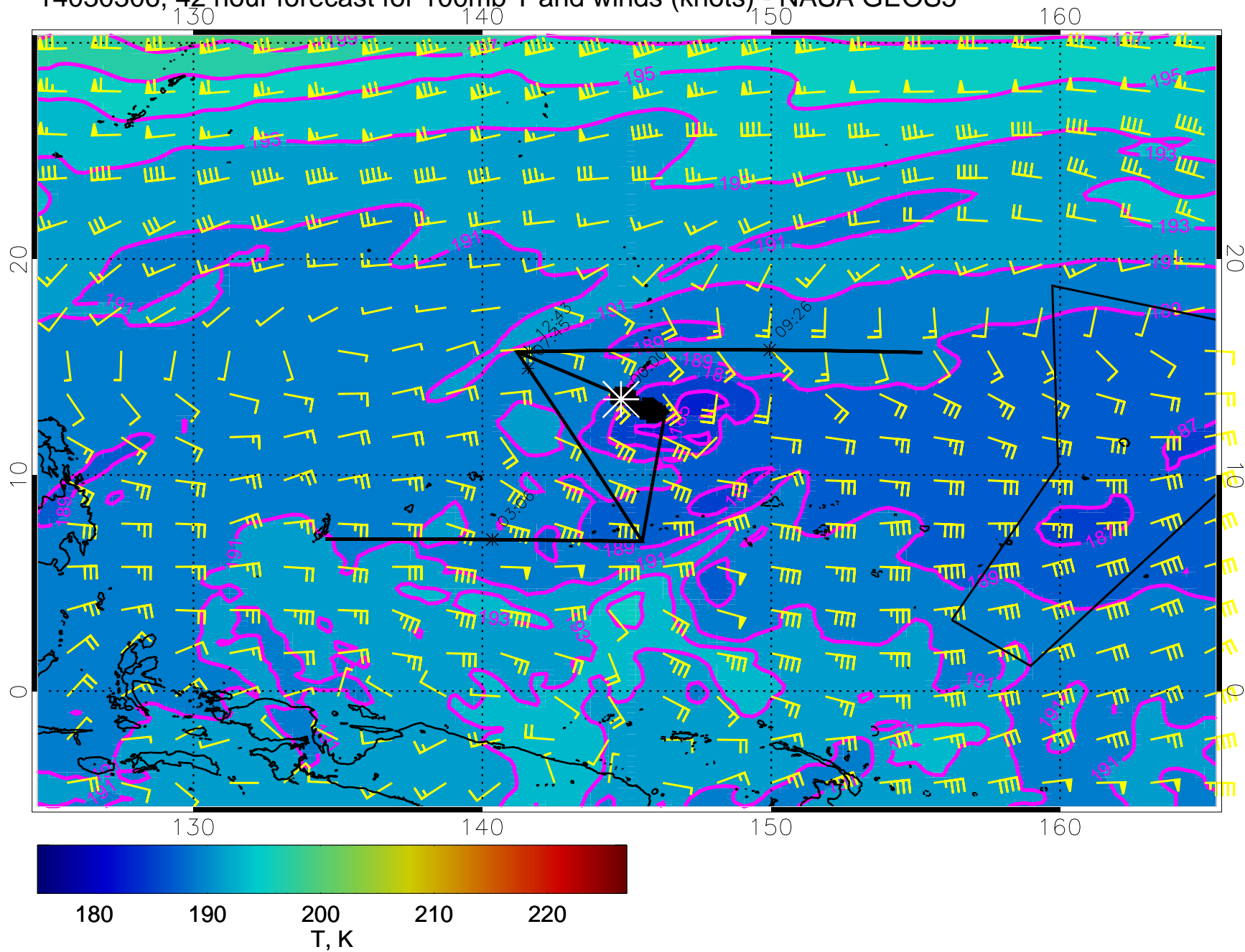
14030306, 42 hour forecast for 100mb T and winds (knots) - NASA GEOS5
