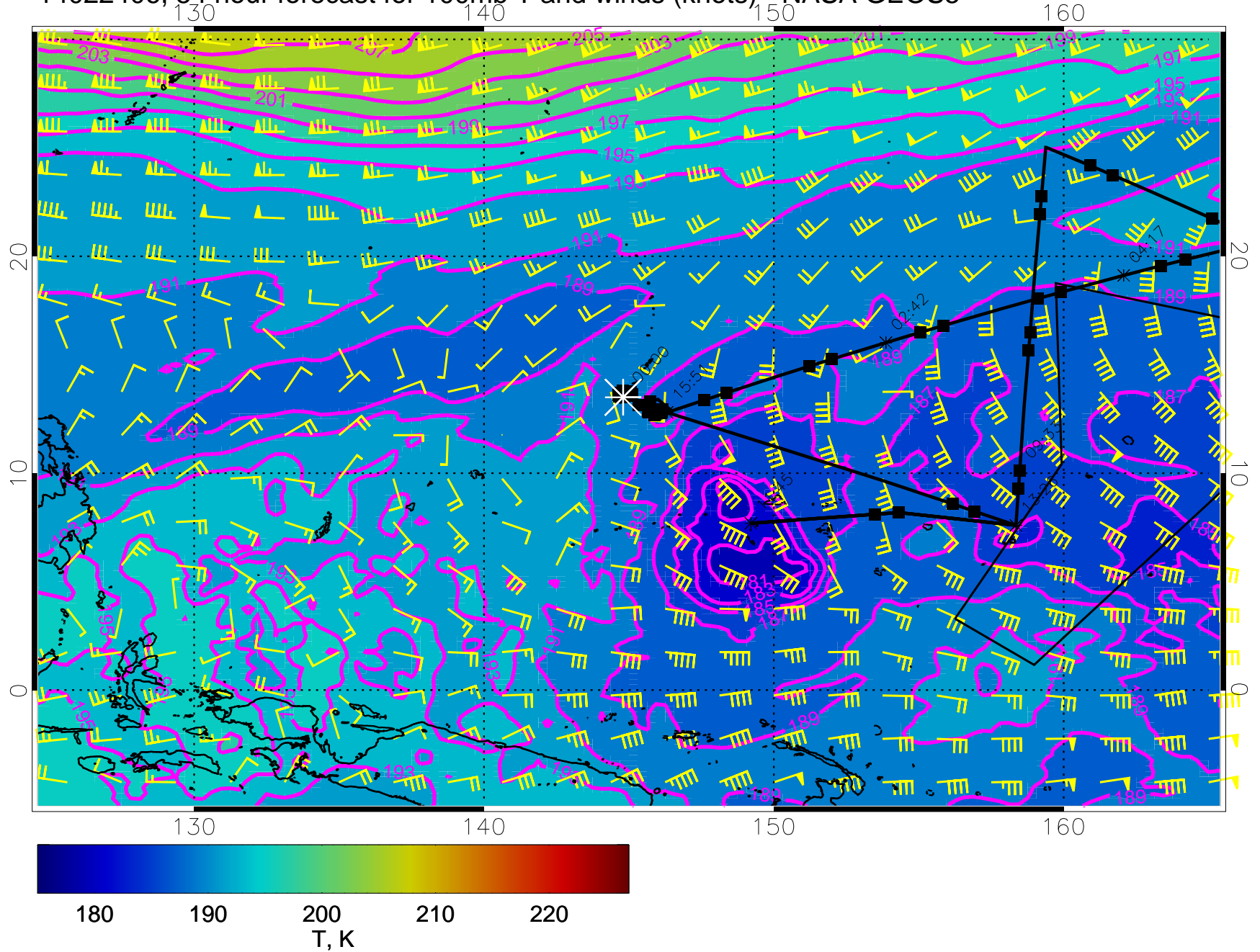
14022406, 54 hour forecast for 100mb T and winds (knots) - NASA GEOS5
