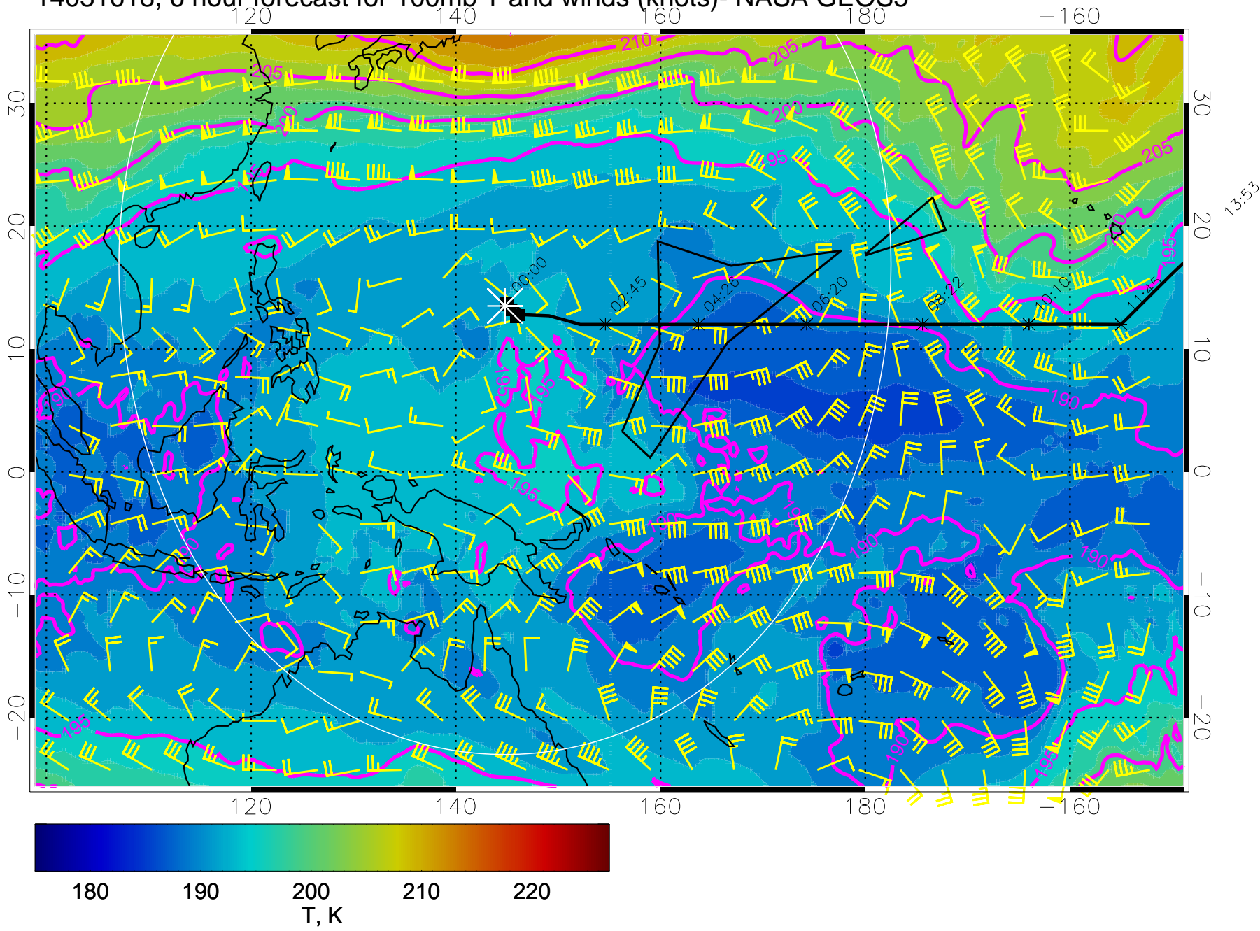
14031618, 6 hour forecast for 100mb T and winds (knots)- NASA GEOS5
