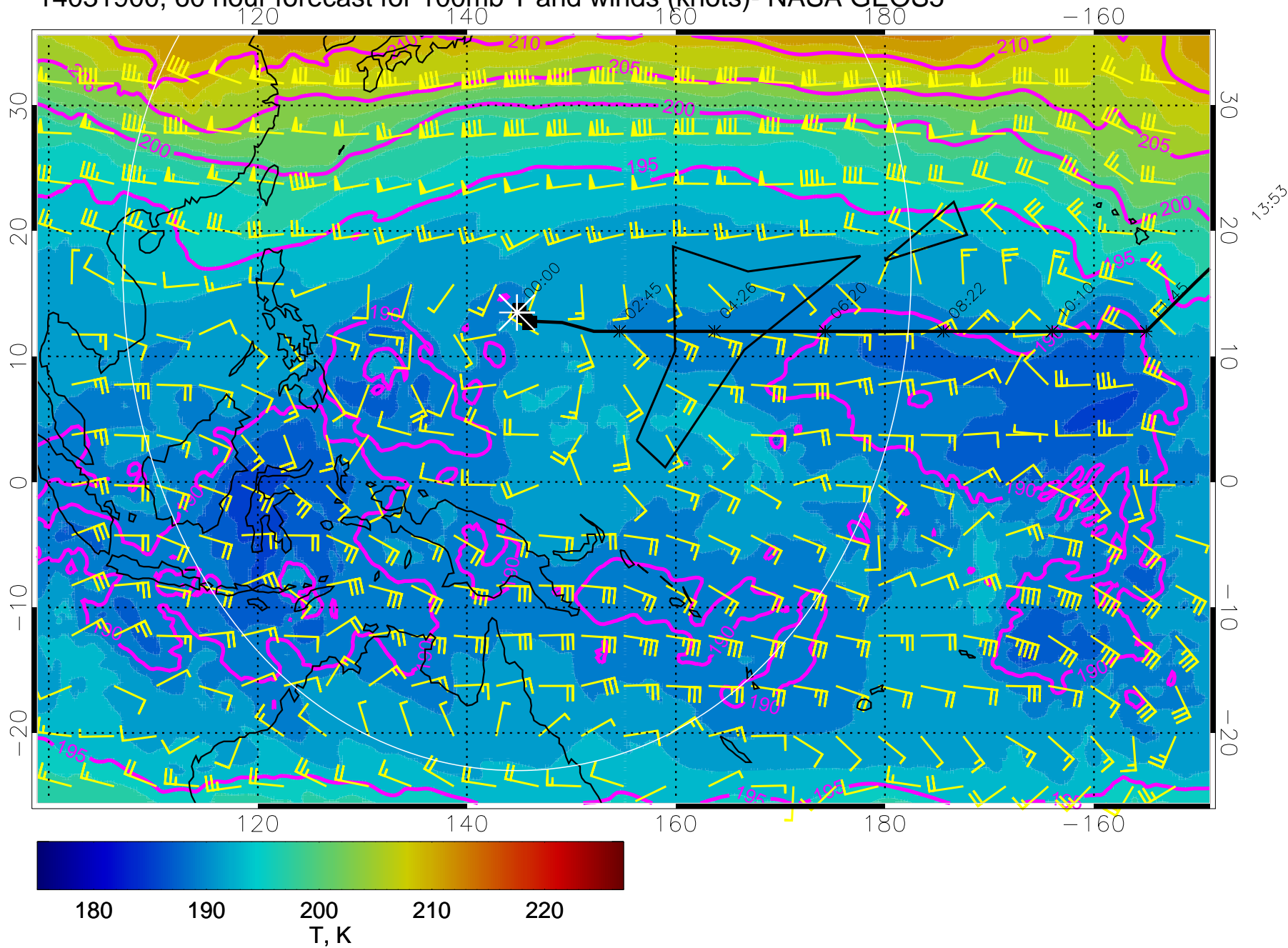
14031900, 60 hour forecast for 100mb T and winds (knots)- NASA GEOS5
