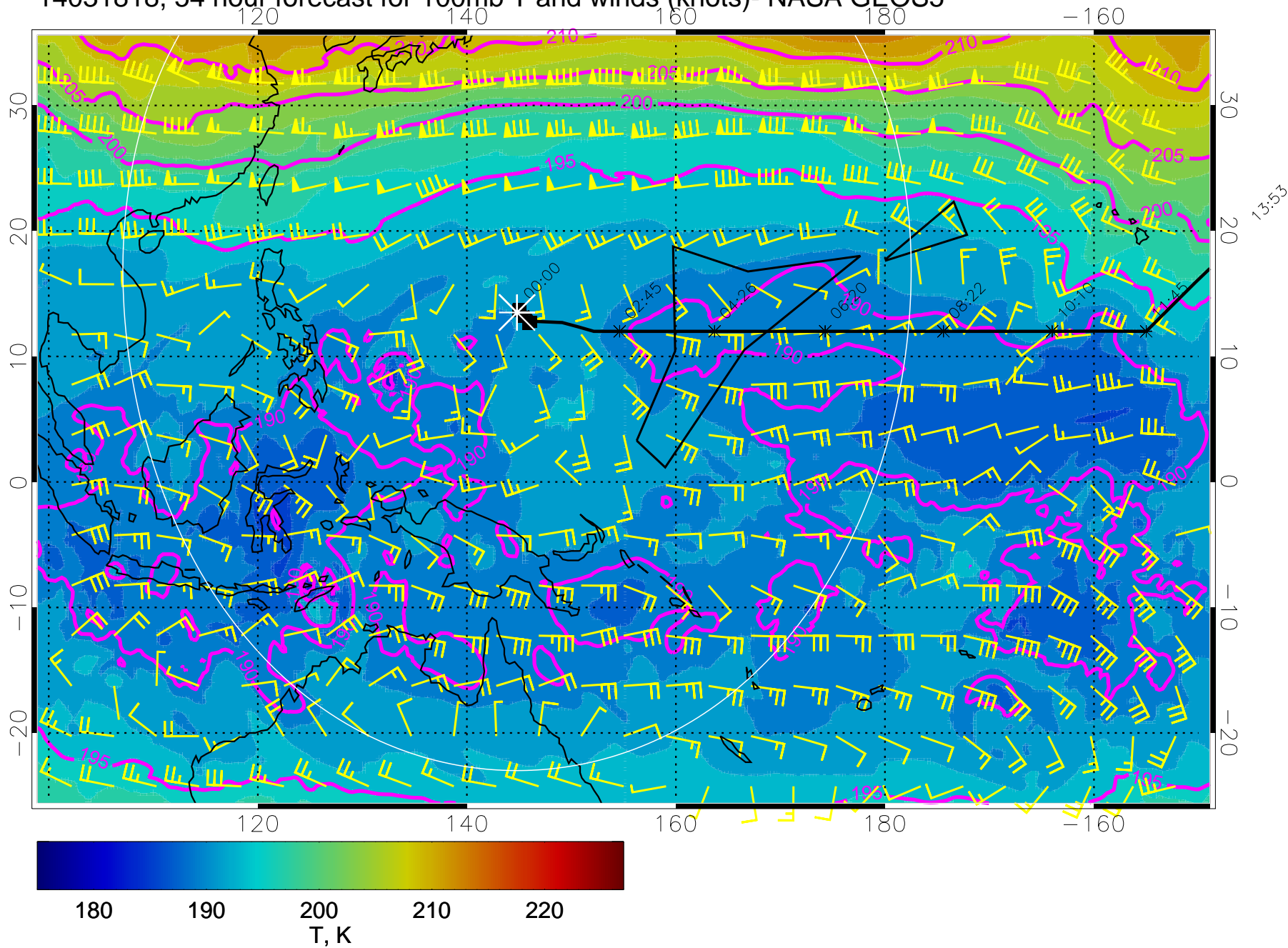
14031818, 54 hour forecast for 100mb T and winds (knots)- NASA GEOS5
