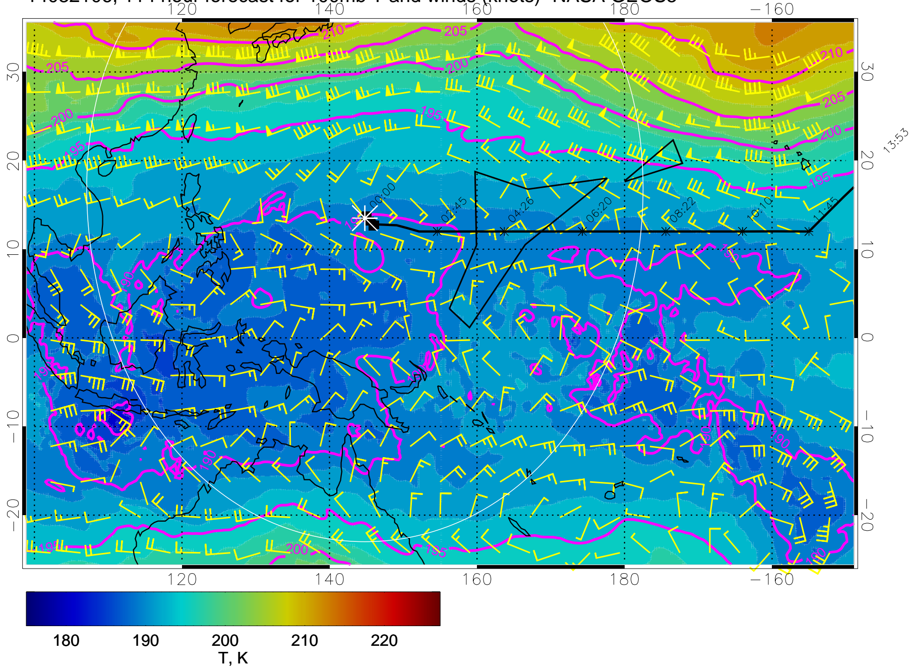
14032106, 114 hour forecast for 100mb T and winds (knots)- NASA GEOS5
