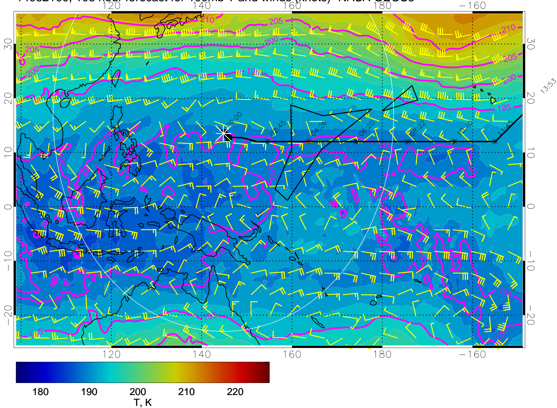
14032100, 108 hour forecast for 100mb T and winds (knots)- NASA GEOS5
