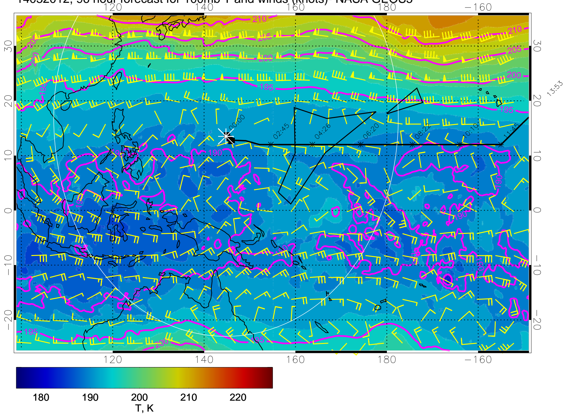
14032012, 96 hour forecast for 100mb T and winds (knots)- NASA GEOS5
