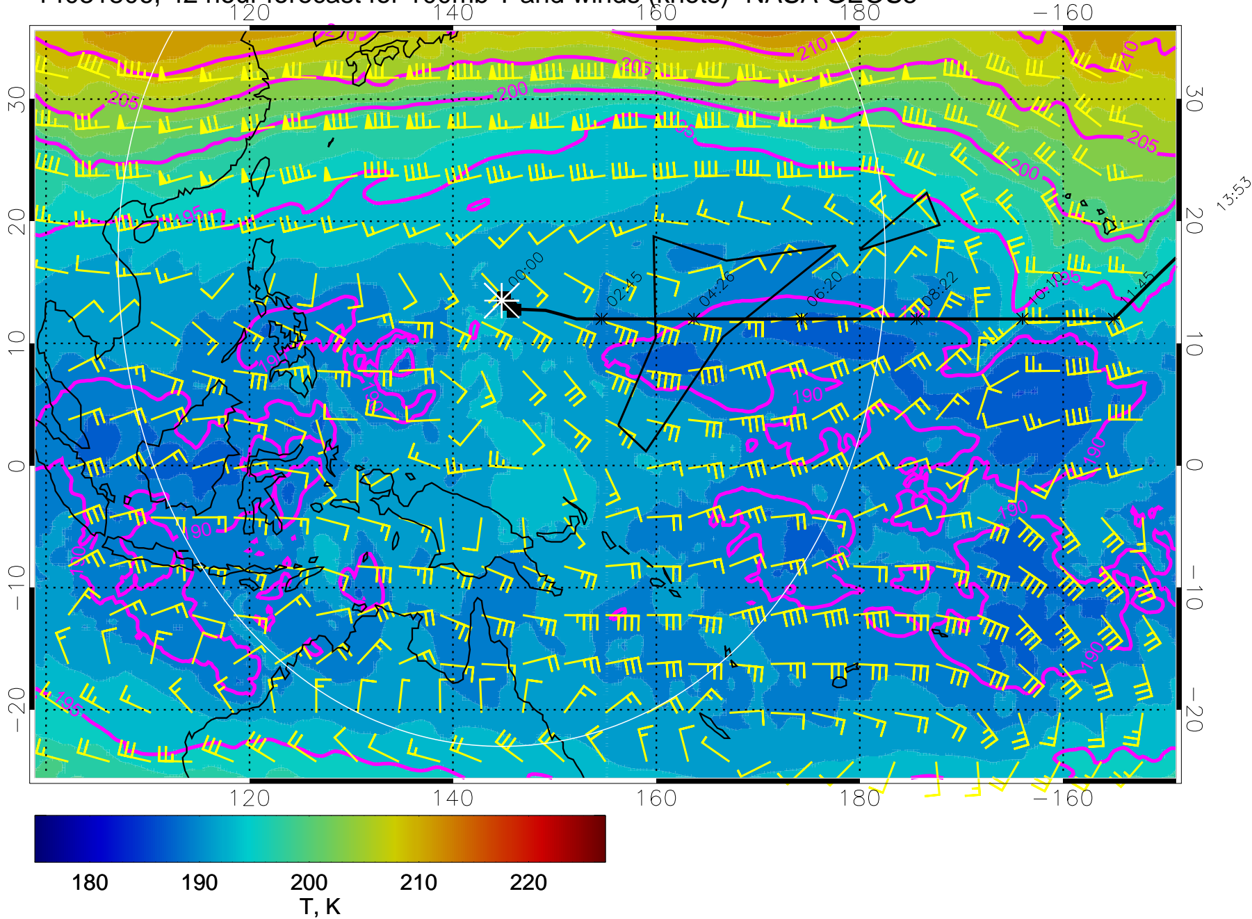
14031806, 42 hour forecast for 100mb T and winds (knots)- NASA GEOS5
