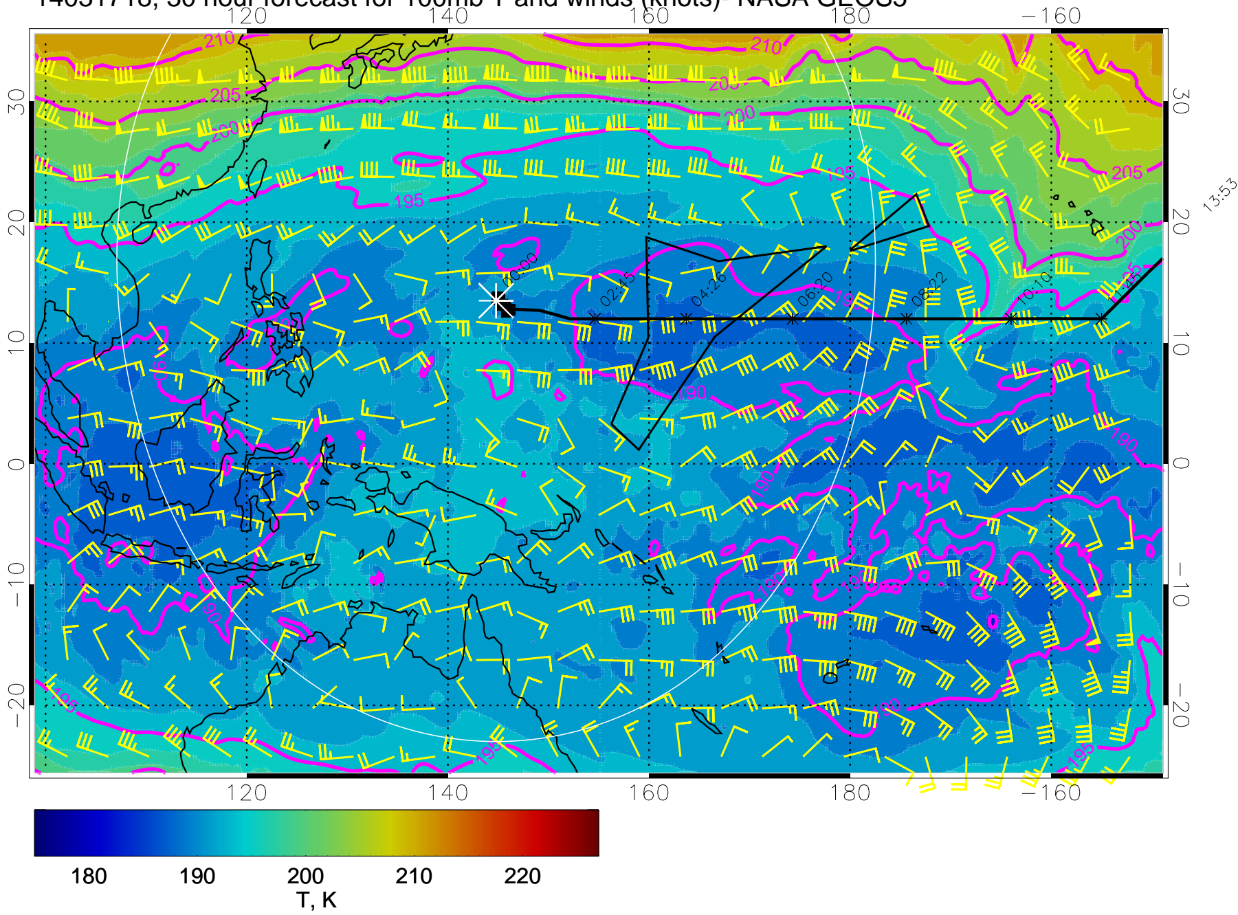
14031718, 30 hour forecast for 100mb T and winds (knots)- NASA GEOS5
