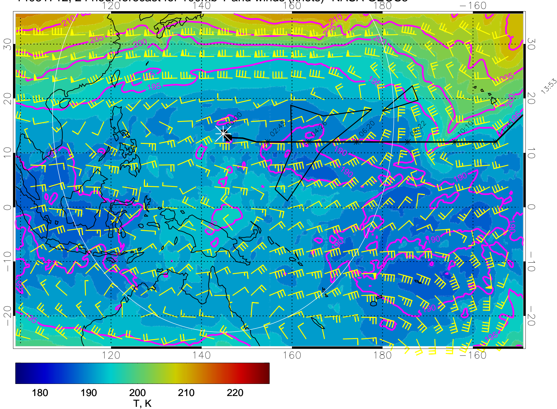
14031712, 24 hour forecast for 100mb T and winds (knots)- NASA GEOS5
