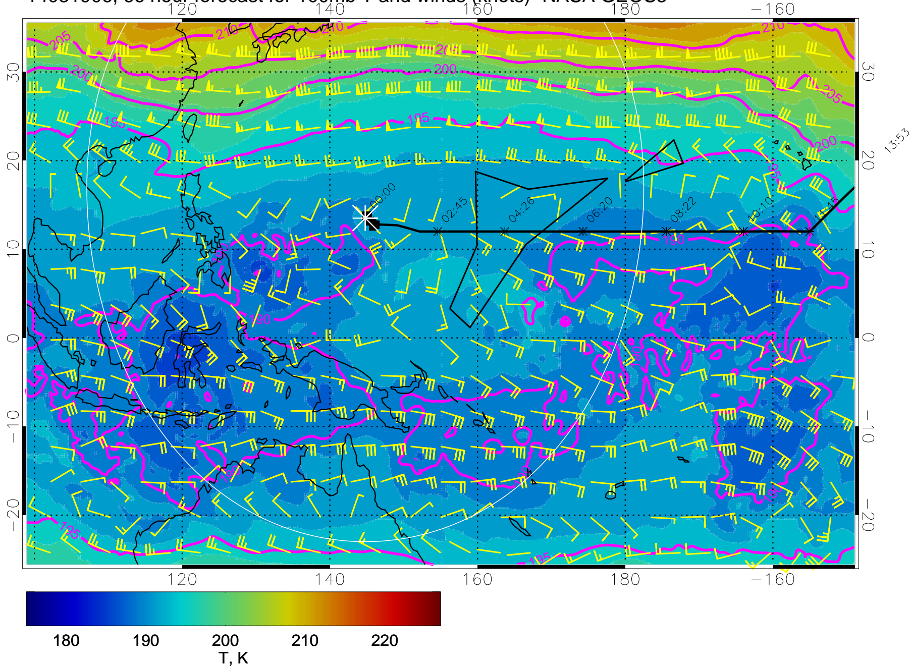
14031906, 66 hour forecast for 100mb T and winds (knots)- NASA GEOS5
