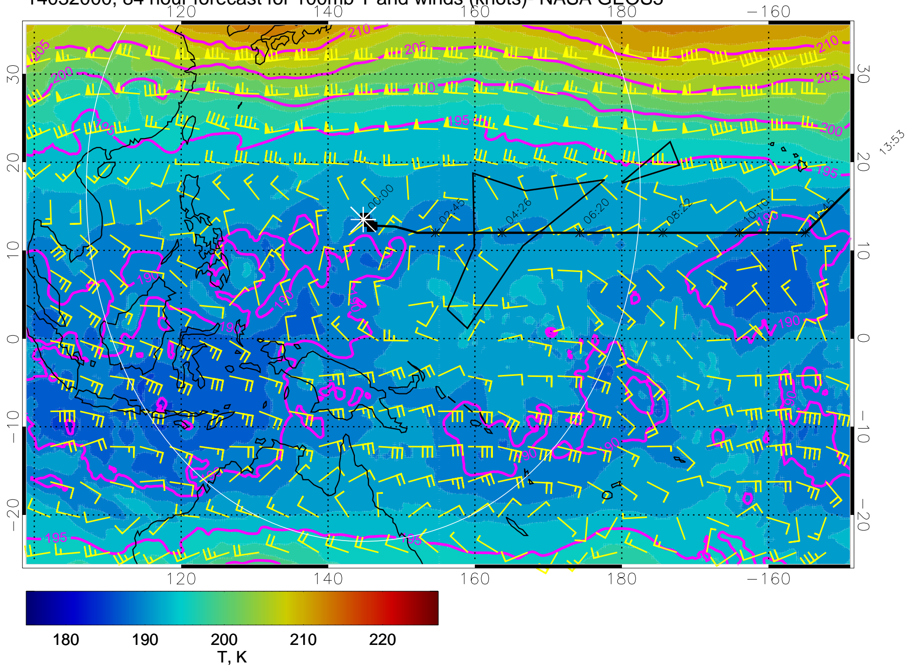
14032000, 84 hour forecast for 100mb T and winds (knots)- NASA GEOS5
