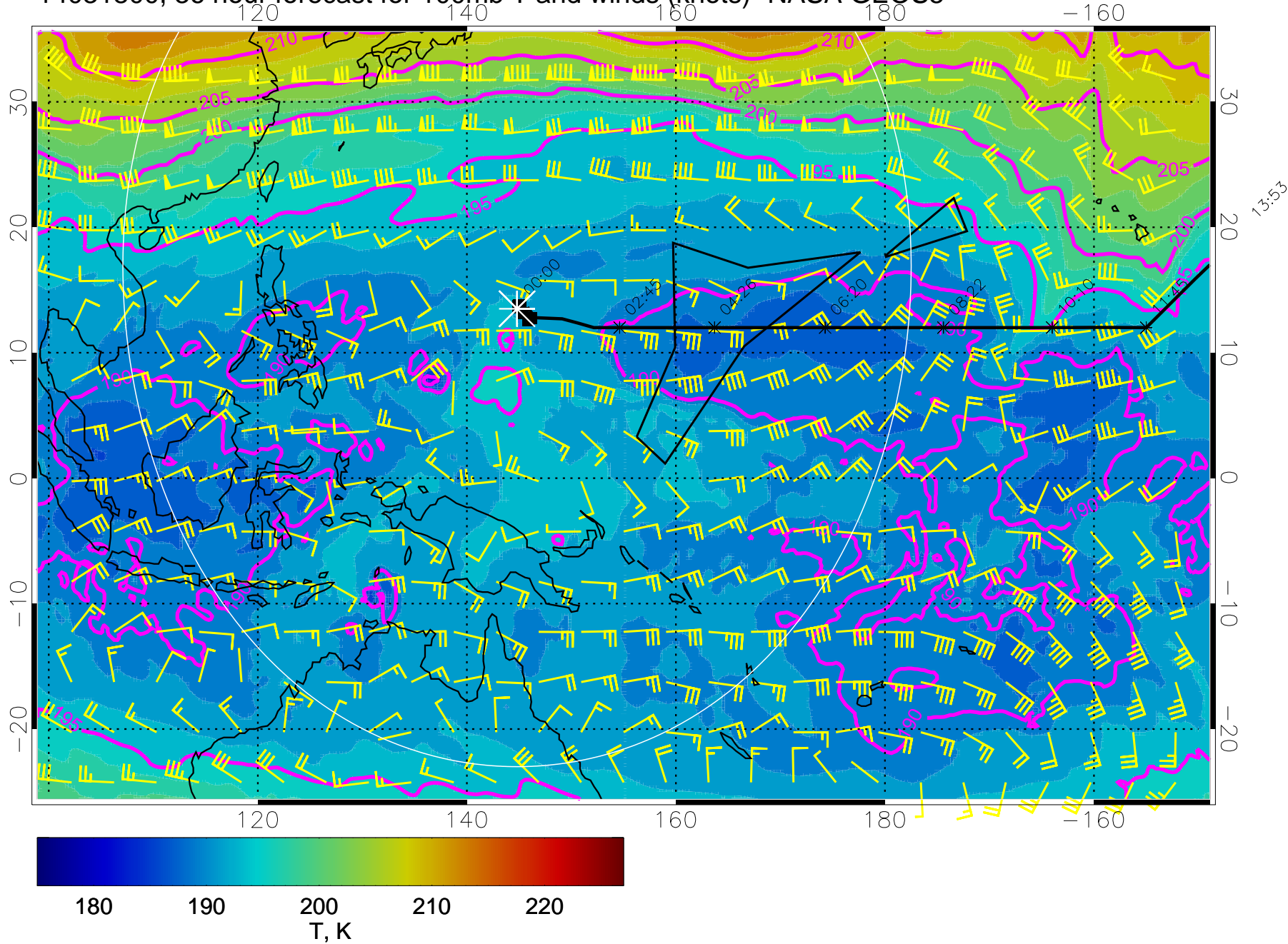
14031800, 36 hour forecast for 100mb T and winds (knots)- NASA GEOS5
