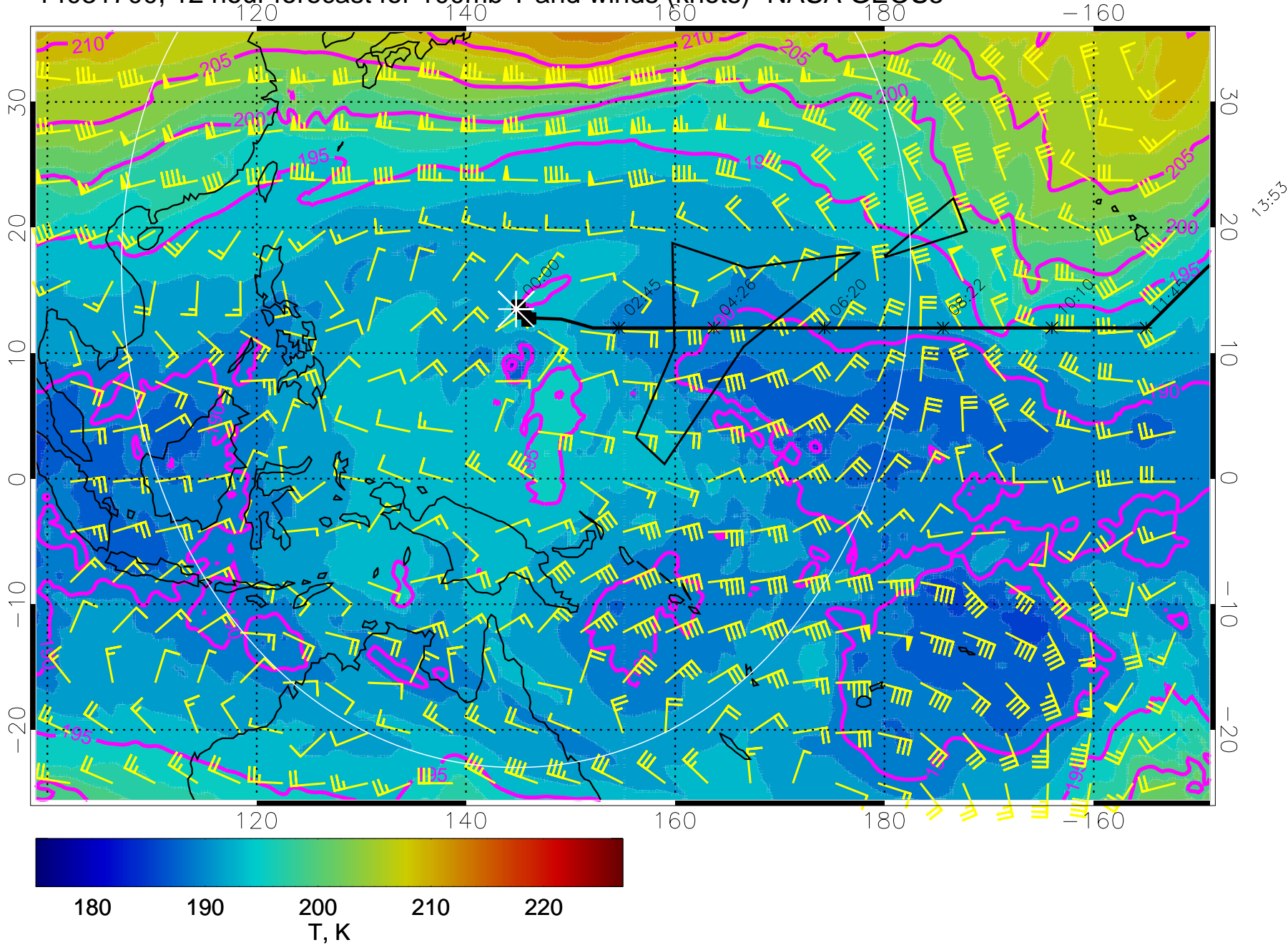
14031700, 12 hour forecast for 100mb T and winds (knots)- NASA GEOS5
