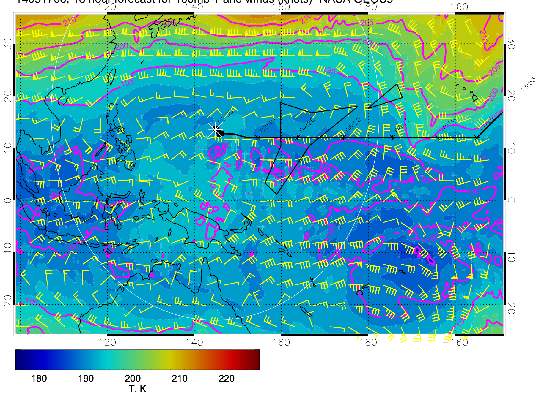
14031706, 18 hour forecast for 100mb T and winds (knots)- NASA GEOS5
