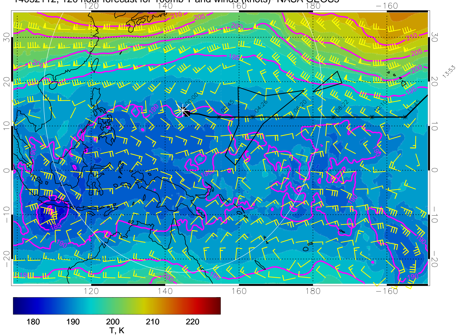
14032112, 120 hour forecast for 100mb T and winds (knots)- NASA GEOS5
