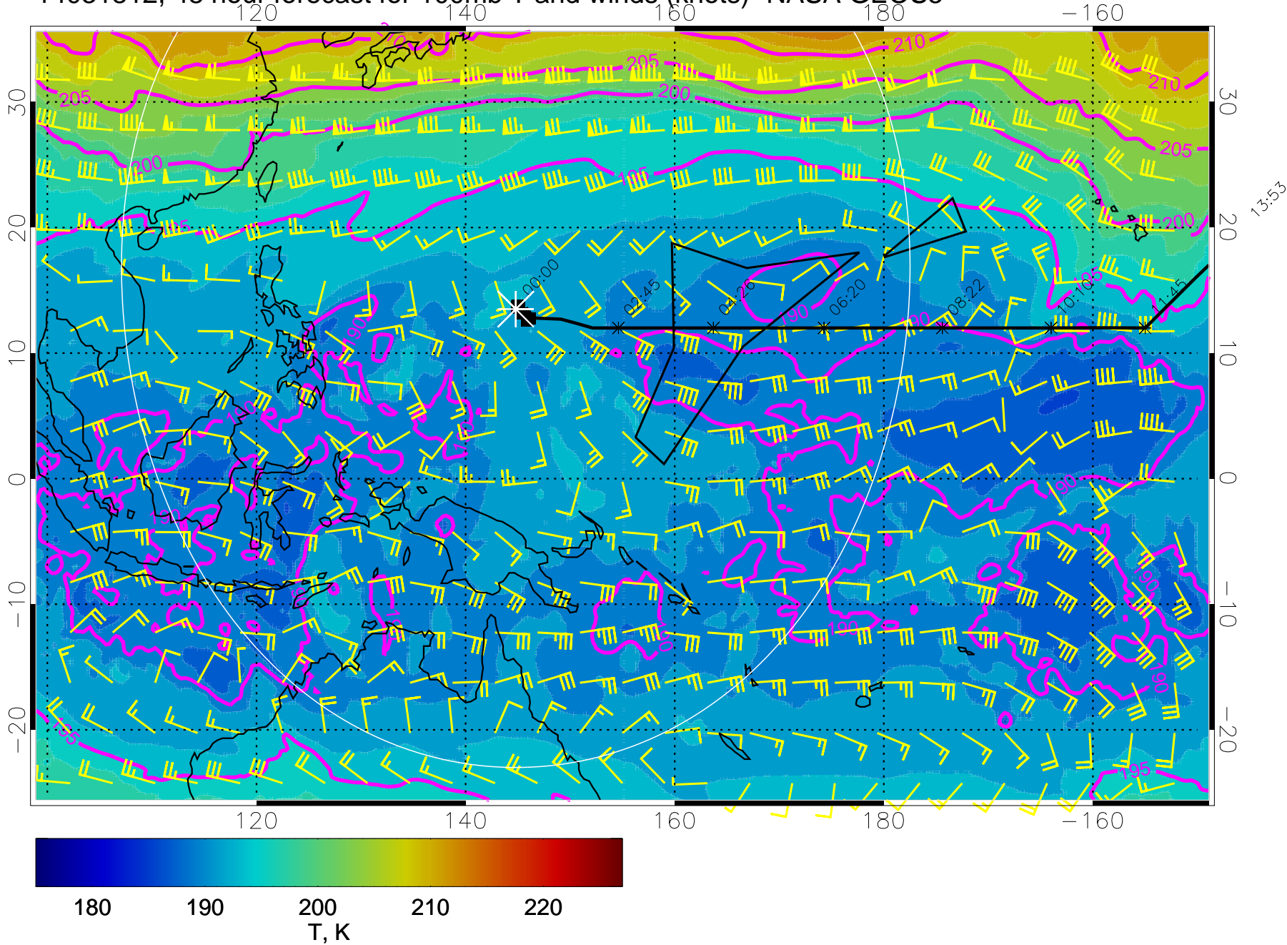
14031812, 48 hour forecast for 100mb T and winds (knots)- NASA GEOS5
