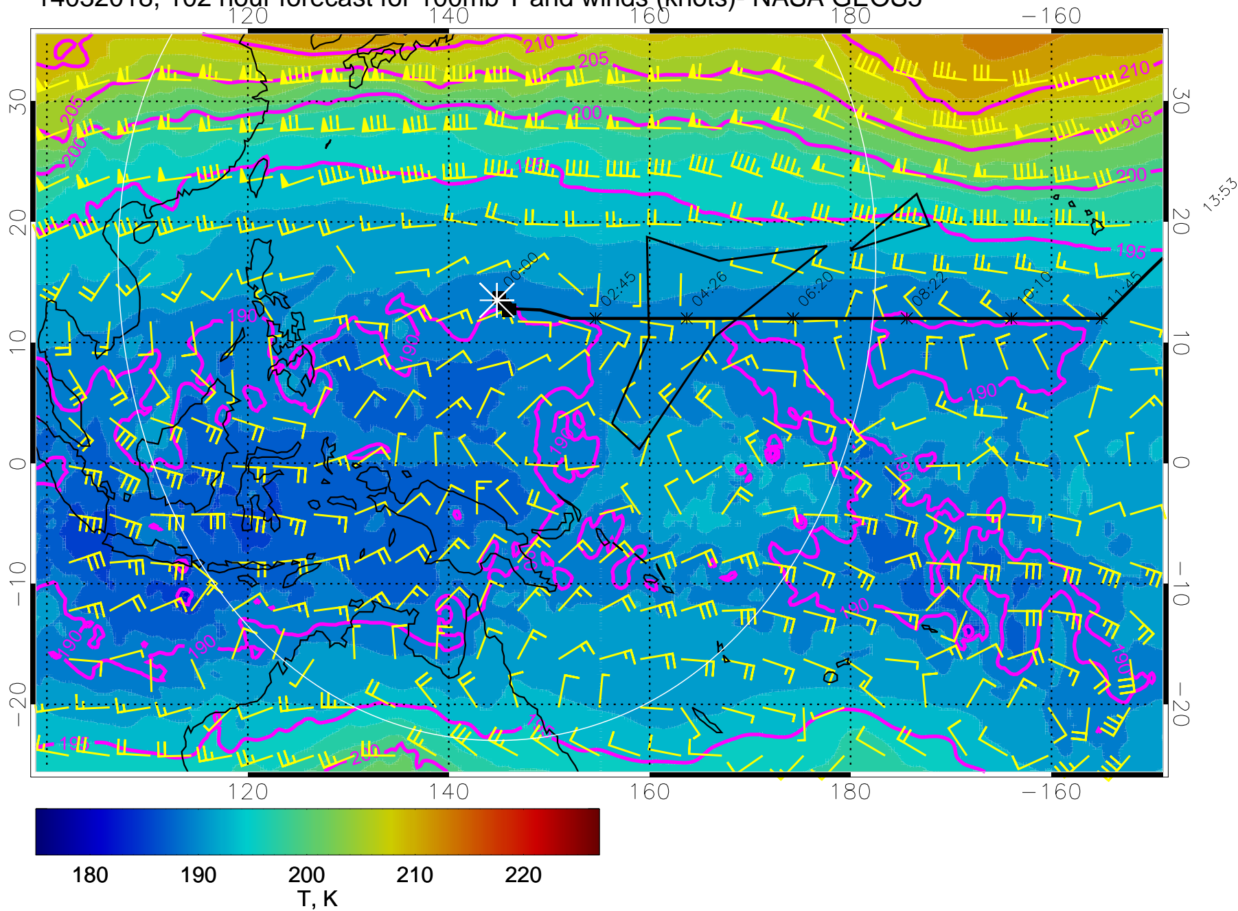
14032018, 102 hour forecast for 100mb T and winds (knots)- NASA GEOS5
