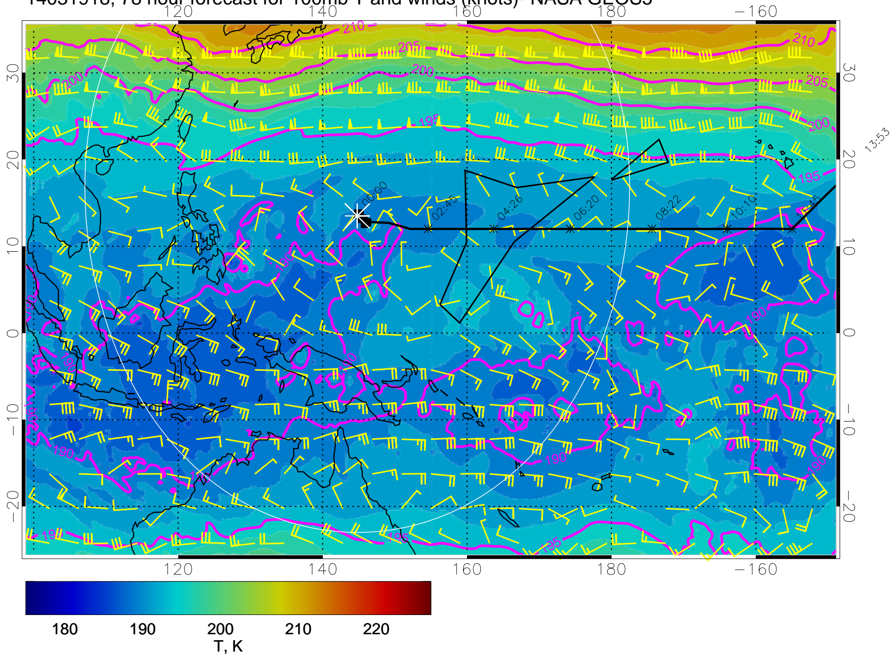
14031918, 78 hour forecast for 100mb T and winds (knots)- NASA GEOS5
