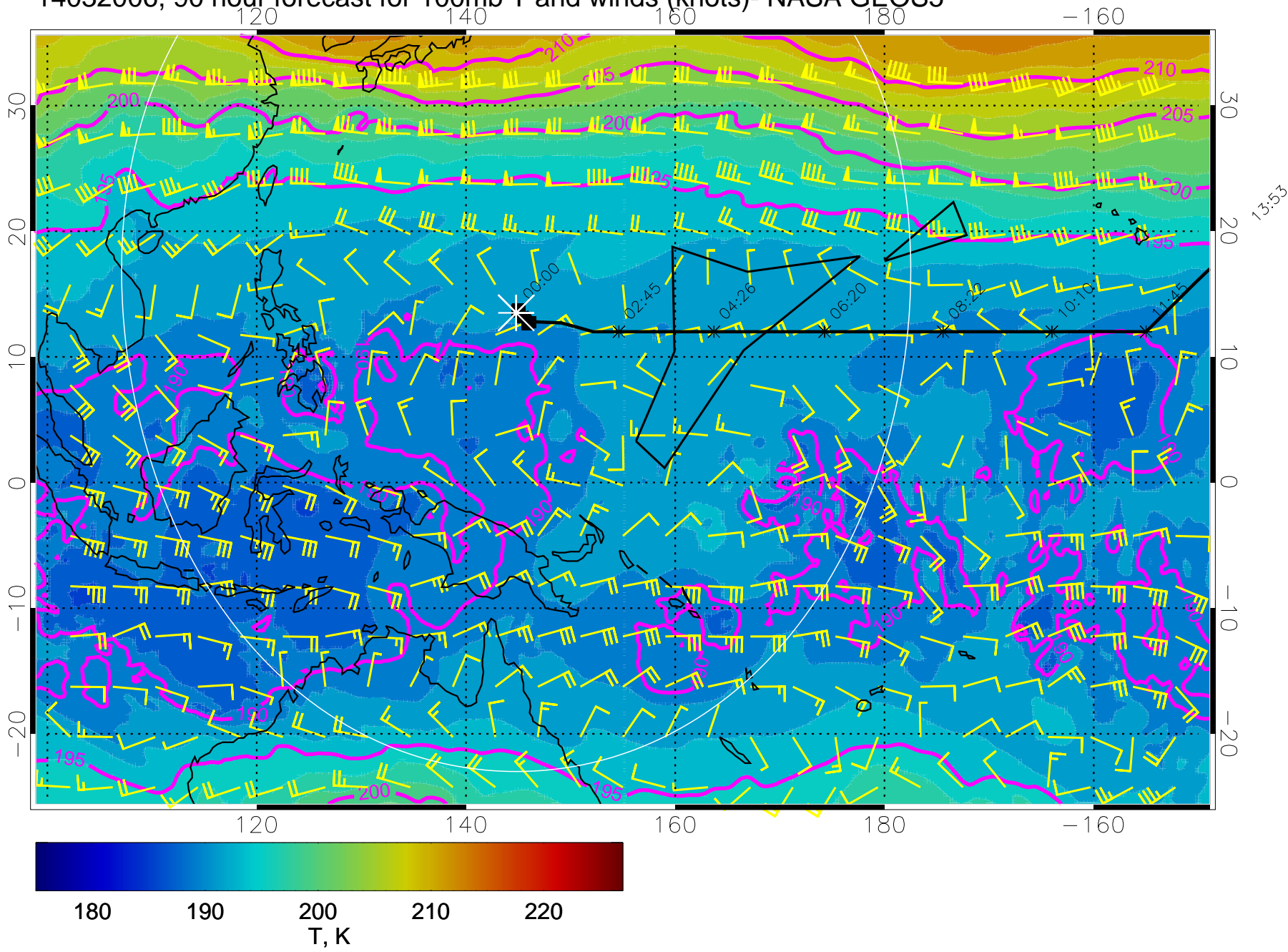
14032006, 90 hour forecast for 100mb T and winds (knots)- NASA GEOS5
