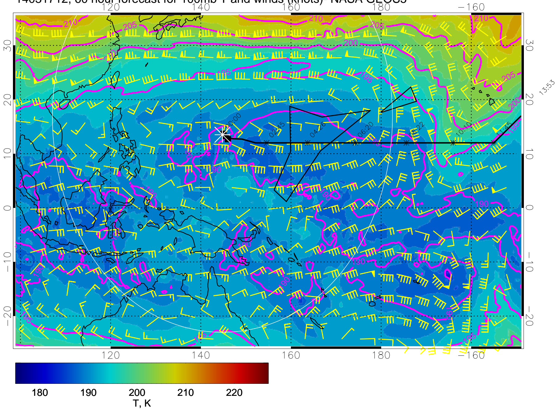
14031712, 60 hour forecast for 100mb T and winds (knots)- NASA GEOS5
