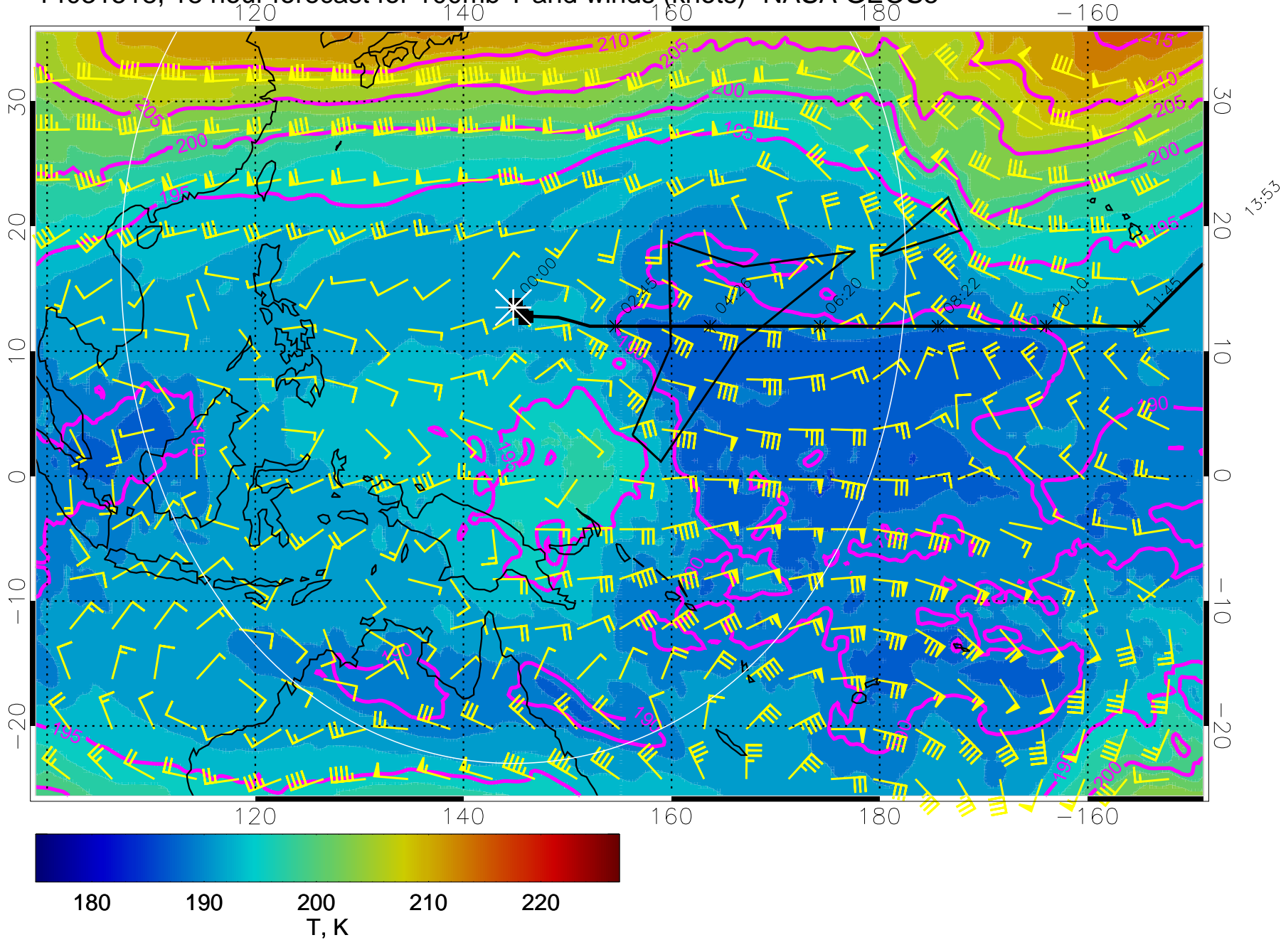
14031518, 18 hour forecast for 100mb T and winds (knots)- NASA GEOS5
