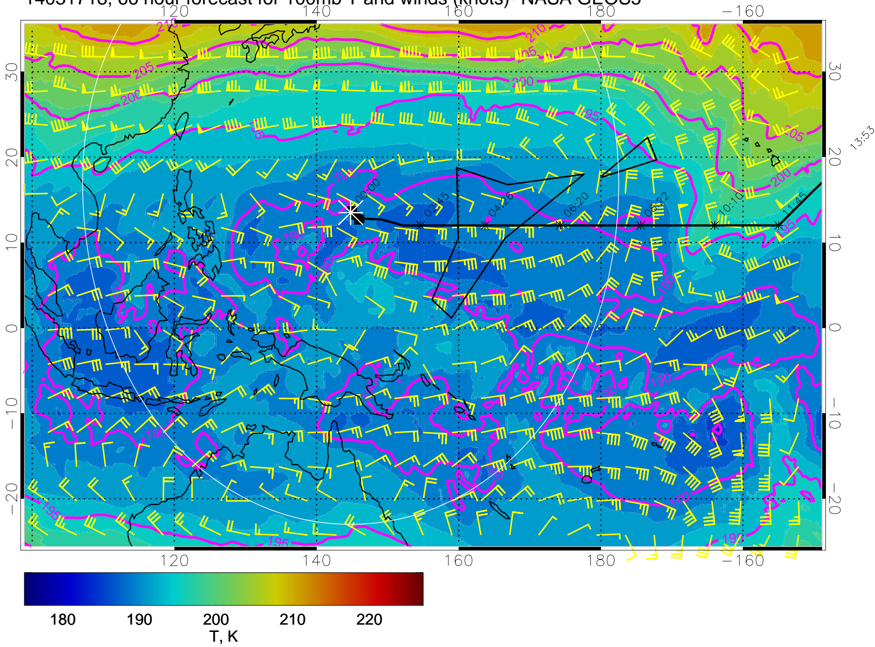
14031718, 66 hour forecast for 100mb T and winds (knots)- NASA GEOS5
