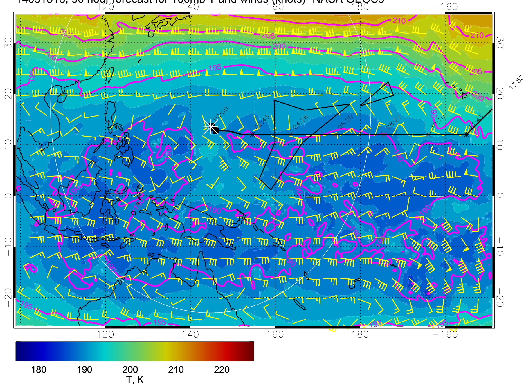
14031818, 90 hour forecast for 100mb T and winds (knots)- NASA GEOS5
