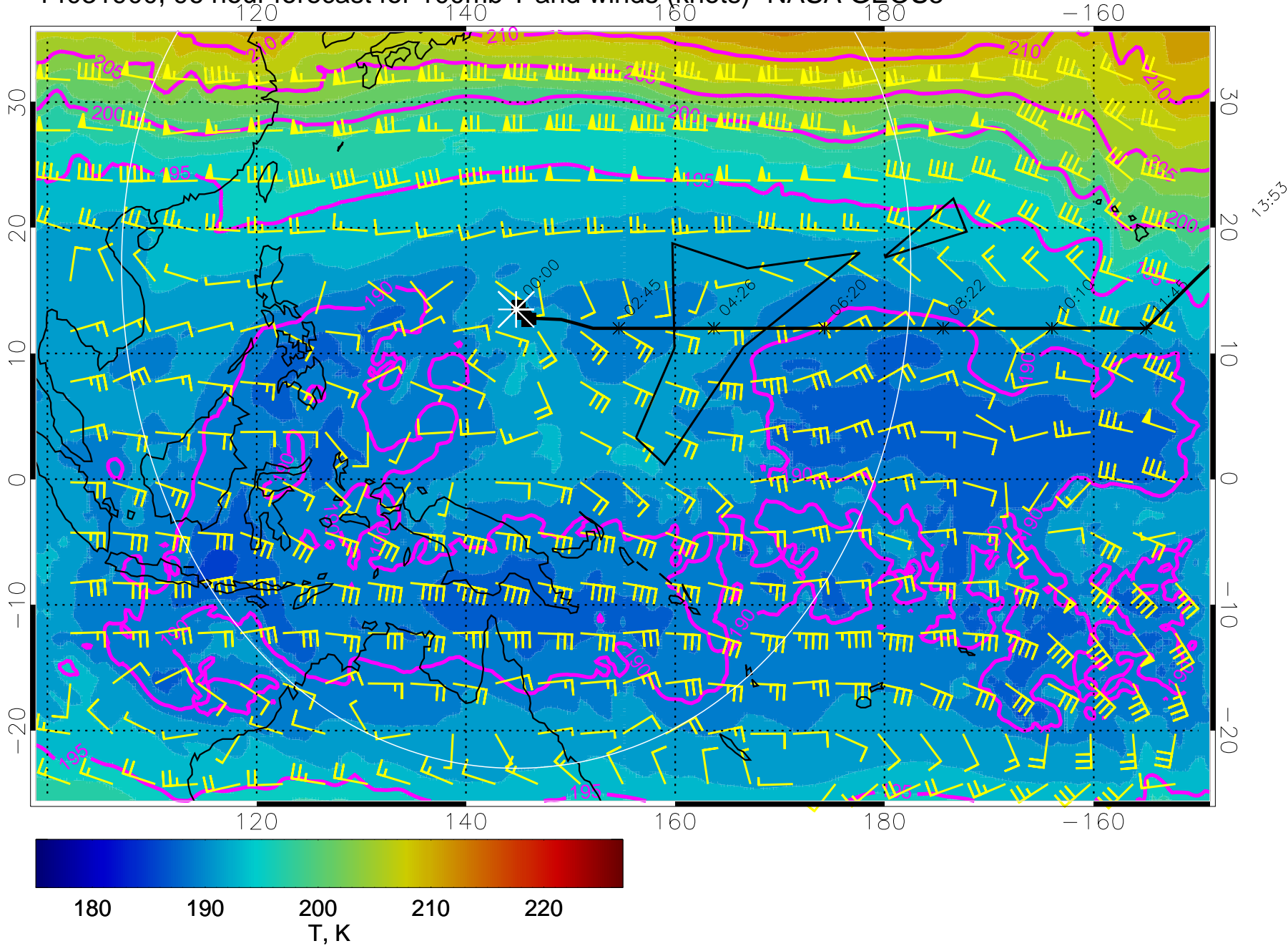
14031900, 96 hour forecast for 100mb T and winds (knots)- NASA GEOS5
