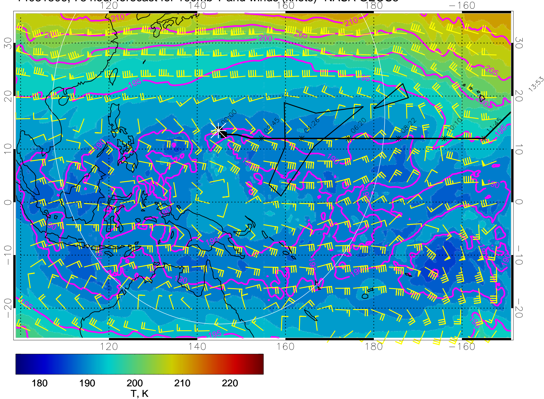
14031806, 78 hour forecast for 100mb T and winds (knots)- NASA GEOS5
