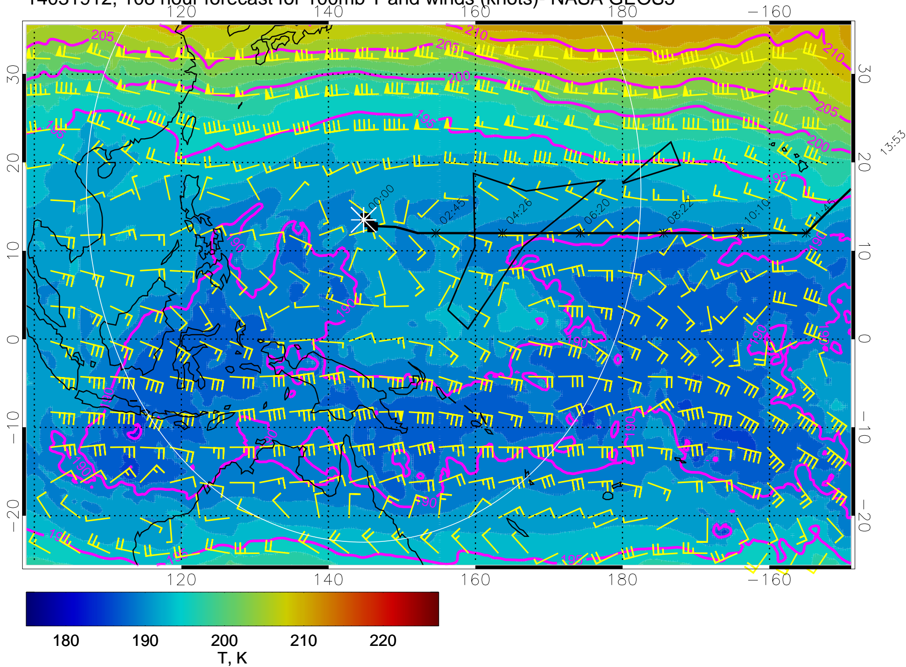
14031912, 108 hour forecast for 100mb T and winds (knots)- NASA GEOS5
