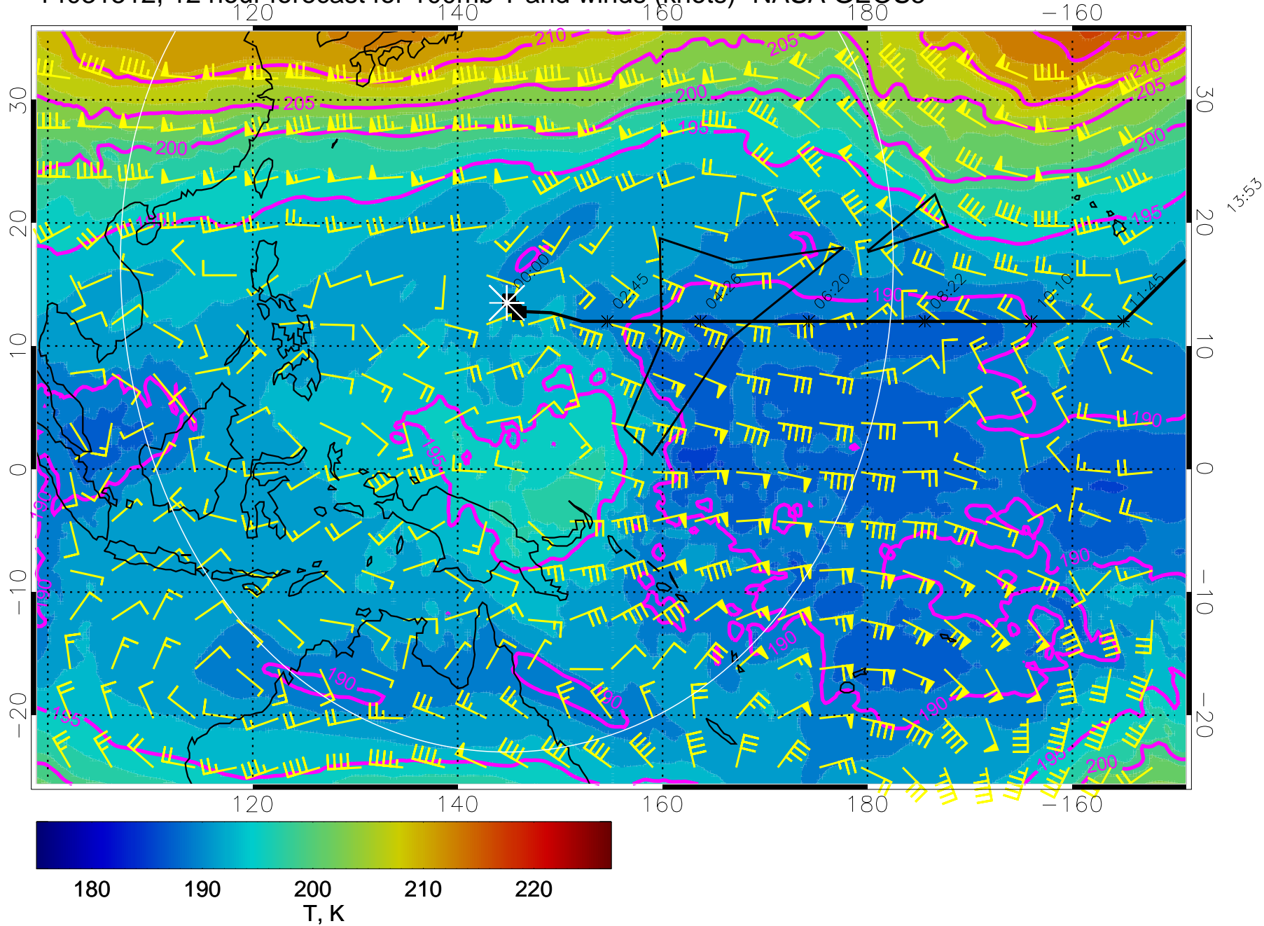
14031512, 12 hour forecast for 100mb T and winds (knots)- NASA GEOS5
