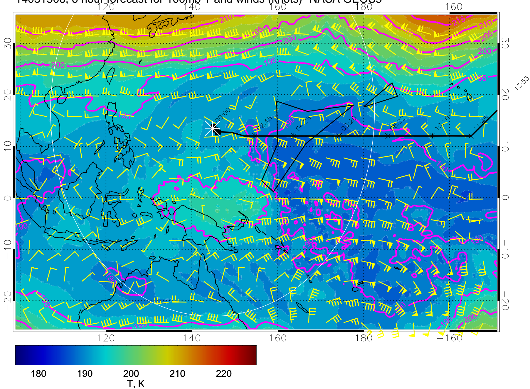
14031506, 6 hour forecast for 100mb T and winds (knots)- NASA GEOS5
