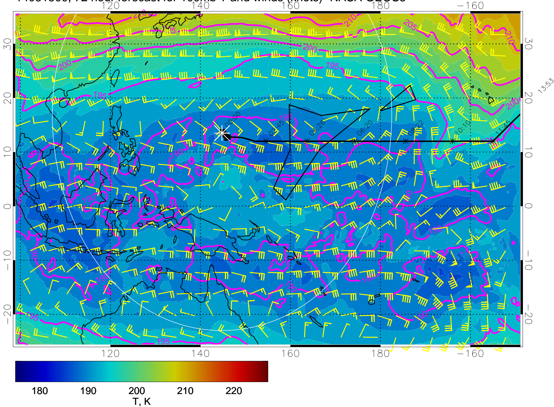
14031800, 72 hour forecast for 100mb T and winds (knots)- NASA GEOS5
