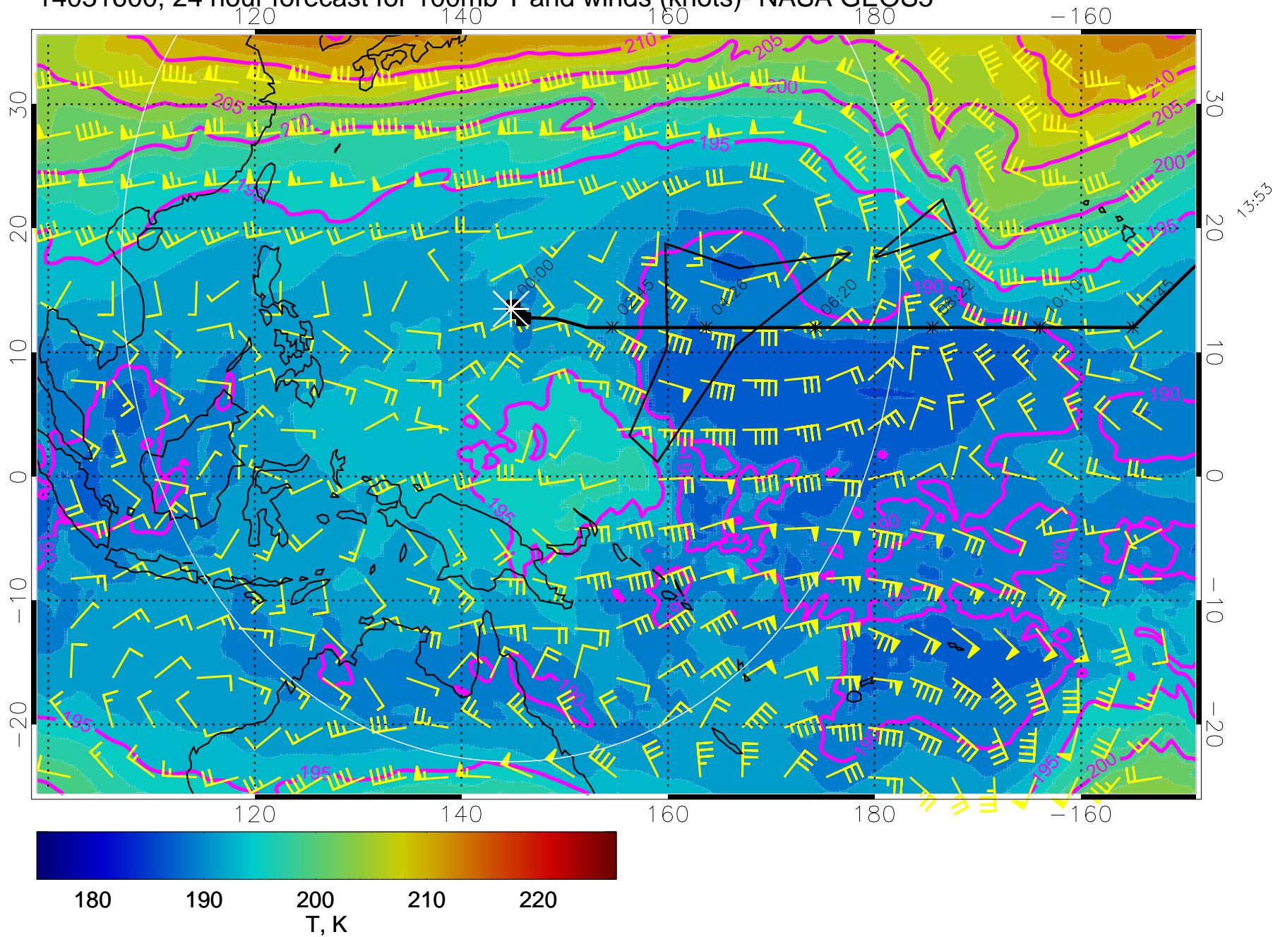
14031600, 24 hour forecast for 100mb T and winds (knots)- NASA GEOS5
