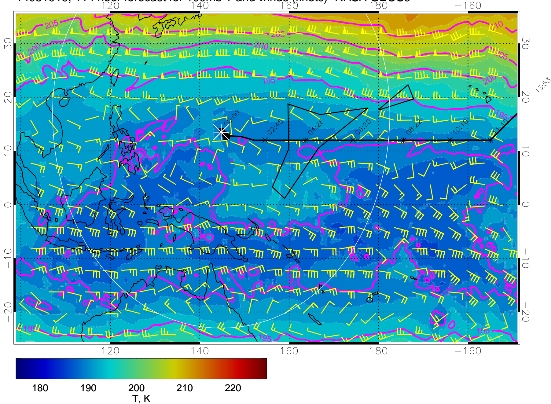
14031918, 114 hour forecast for 100mb T and winds (knots)- NASA GEOS5
