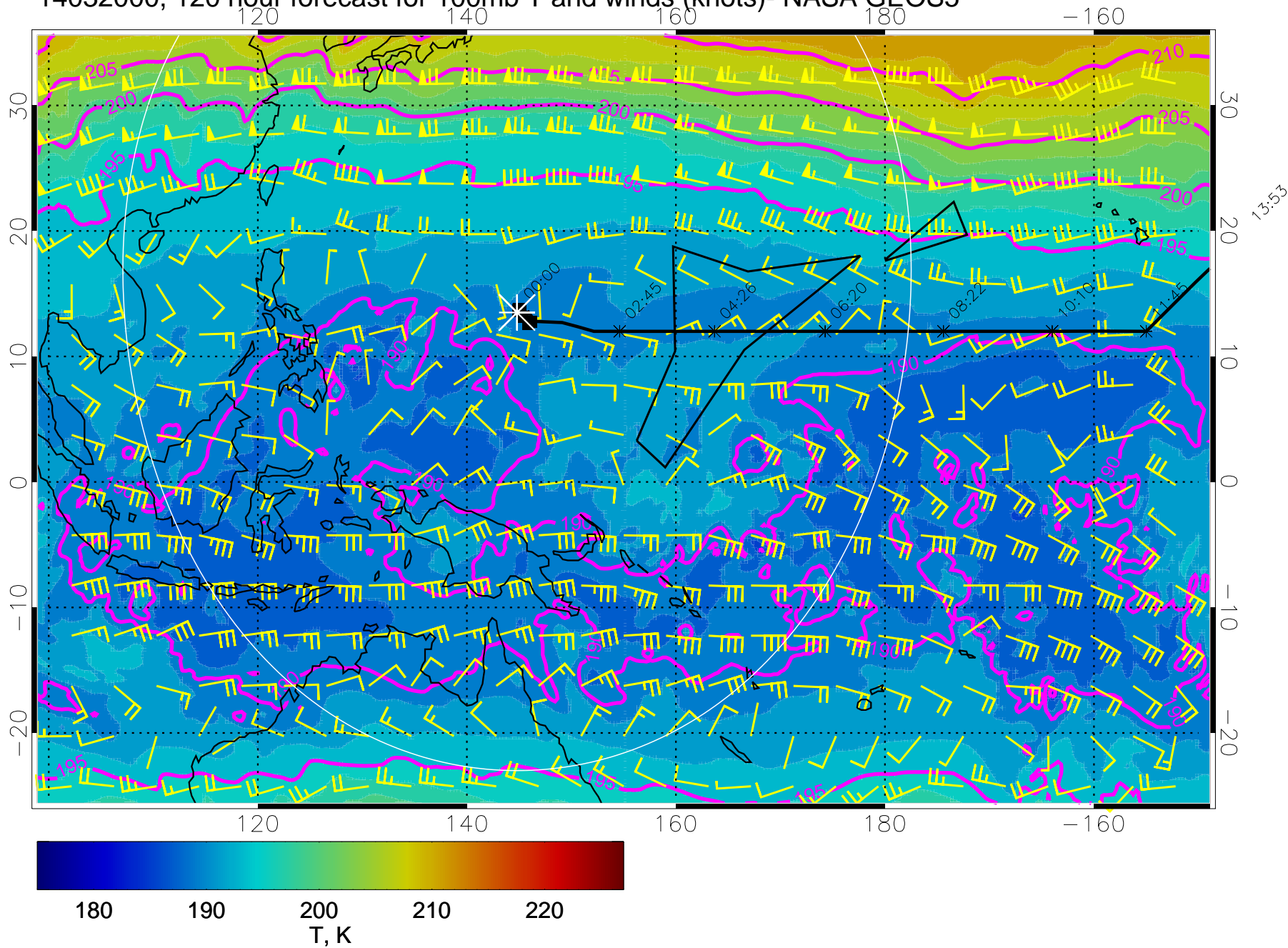
14032000, 120 hour forecast for 100mb T and winds (knots)- NASA GEOS5
