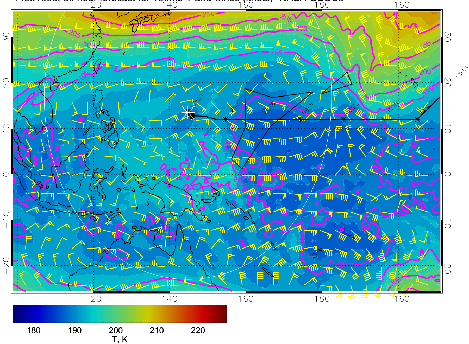
14031606, 30 hour forecast for 100mb T and winds (knots)- NASA GEOS5
