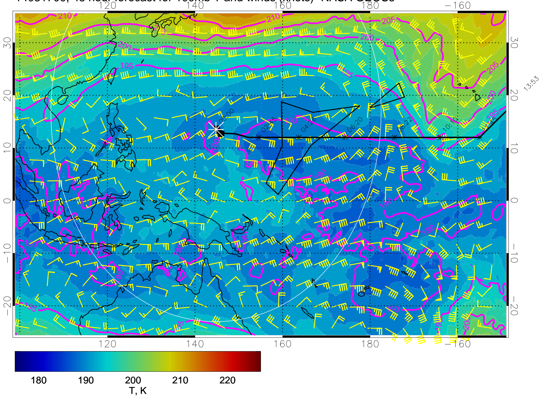
14031700, 48 hour forecast for 100mb T and winds (knots)- NASA GEOS5
