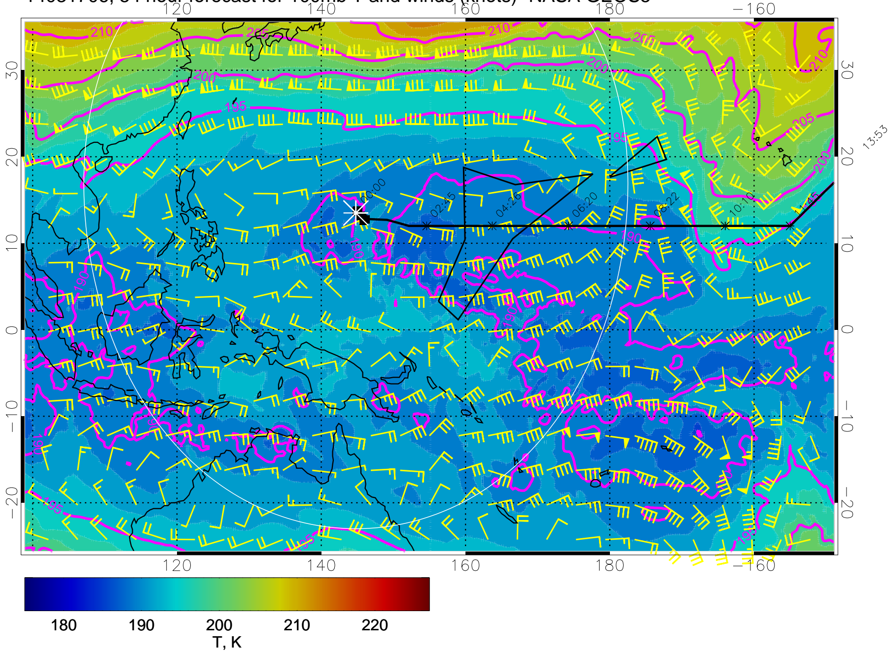
14031706, 54 hour forecast for 100mb T and winds (knots)- NASA GEOS5
