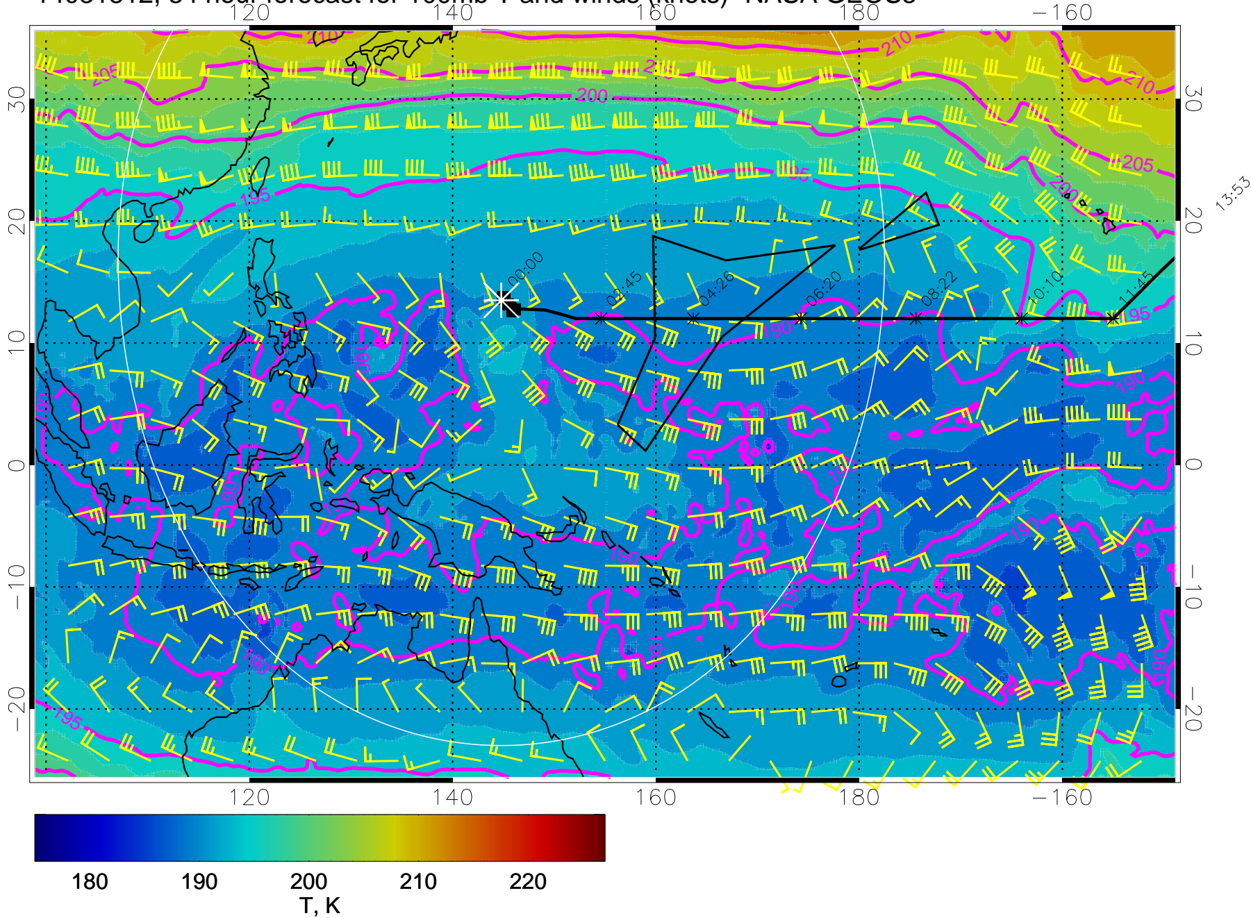
14031812, 84 hour forecast for 100mb T and winds (knots)- NASA GEOS5
