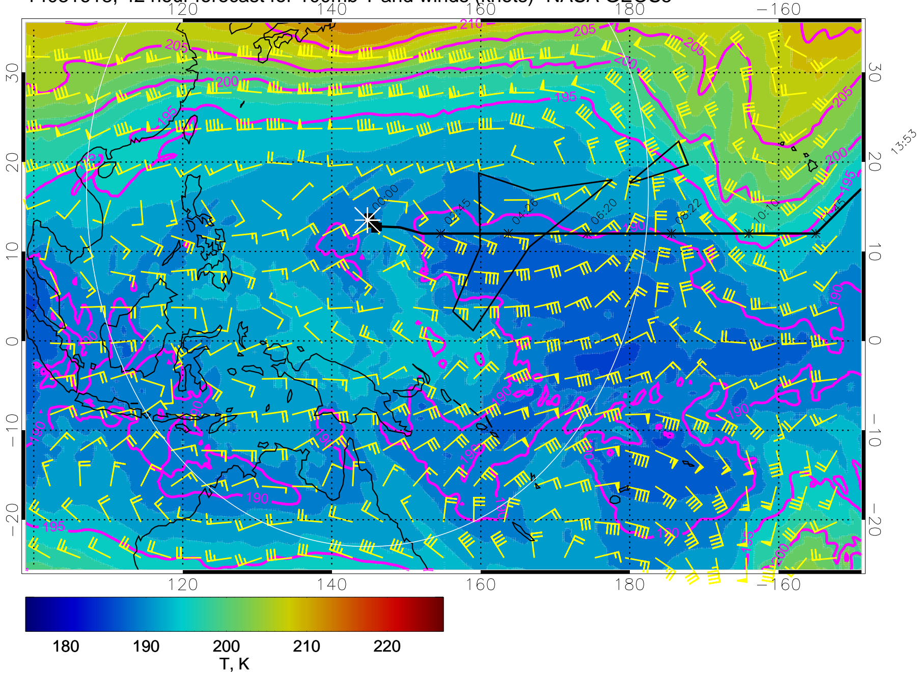
14031618, 42 hour forecast for 100mb T and winds (knots)- NASA GEOS5
