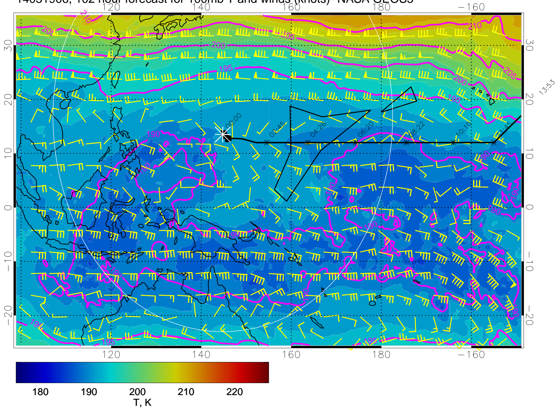
14031906, 102 hour forecast for 100mb T and winds (knots)- NASA GEOS5
