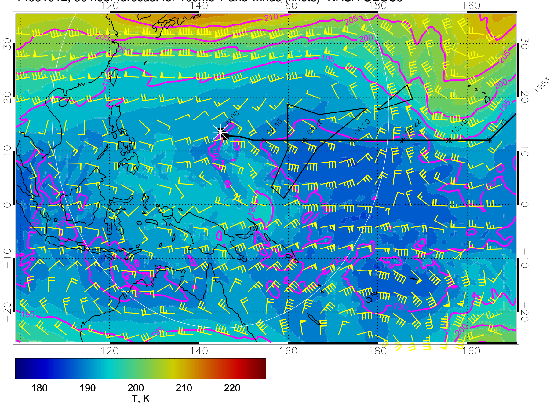
14031612, 36 hour forecast for 100mb T and winds (knots)- NASA GEOS5
