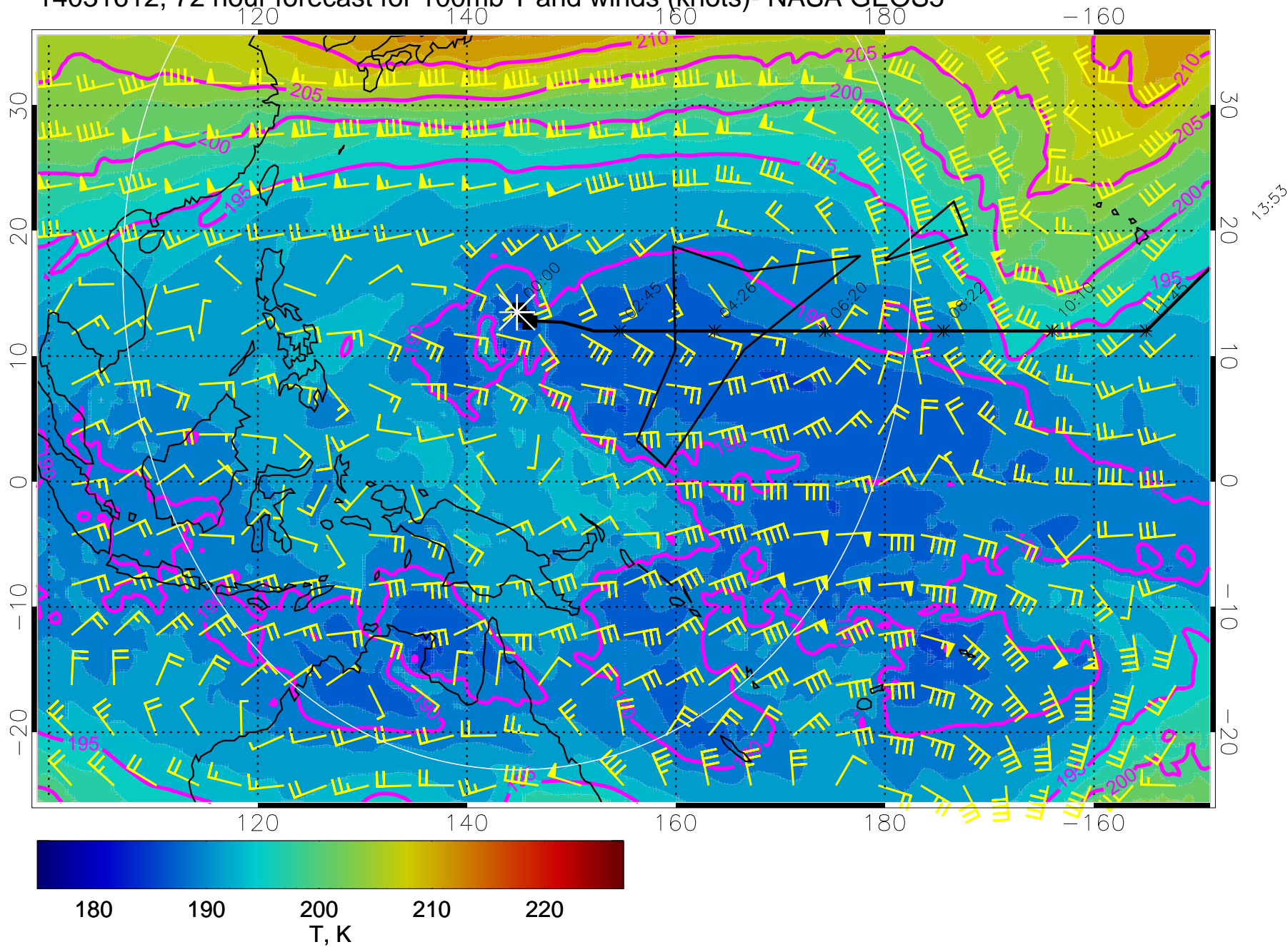
14031612, 72 hour forecast for 100mb T and winds (knots)- NASA GEOS5
