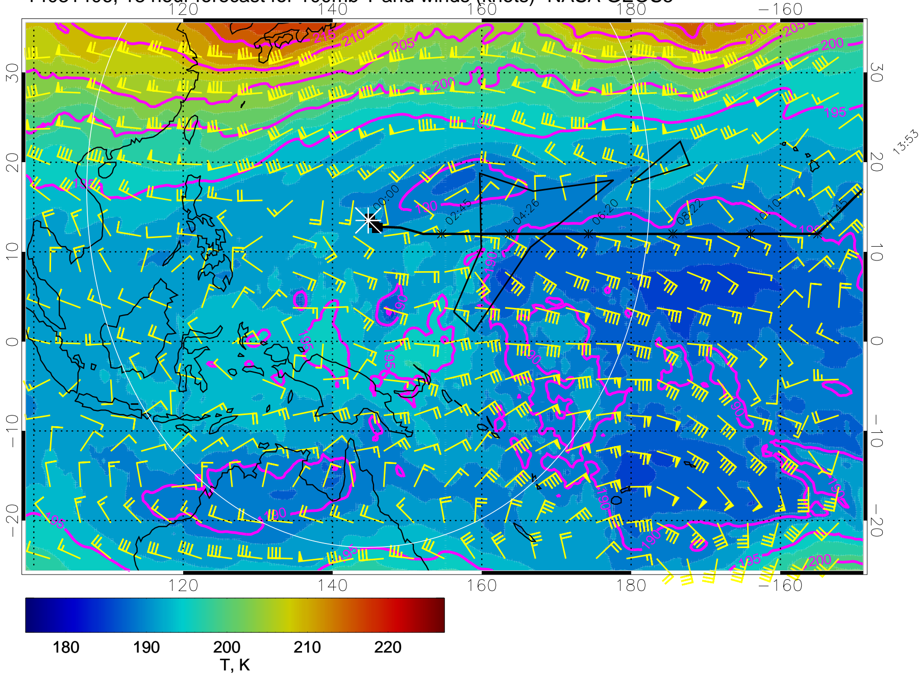
14031406, 18 hour forecast for 100mb T and winds (knots)- NASA GEOS5
