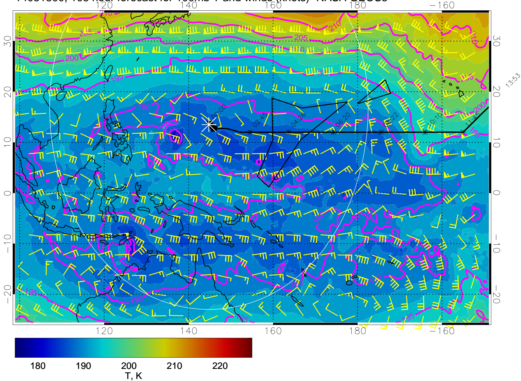
14031800, 108 hour forecast for 100mb T and winds (knots)- NASA GEOS5
