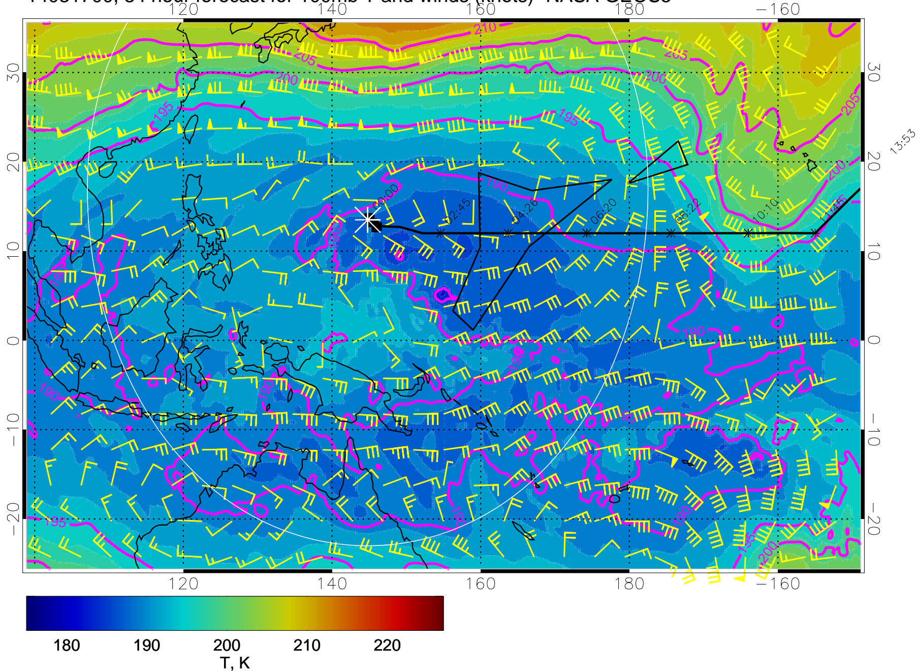
14031700, 84 hour forecast for 100mb T and winds (knots)- NASA GEOS5
