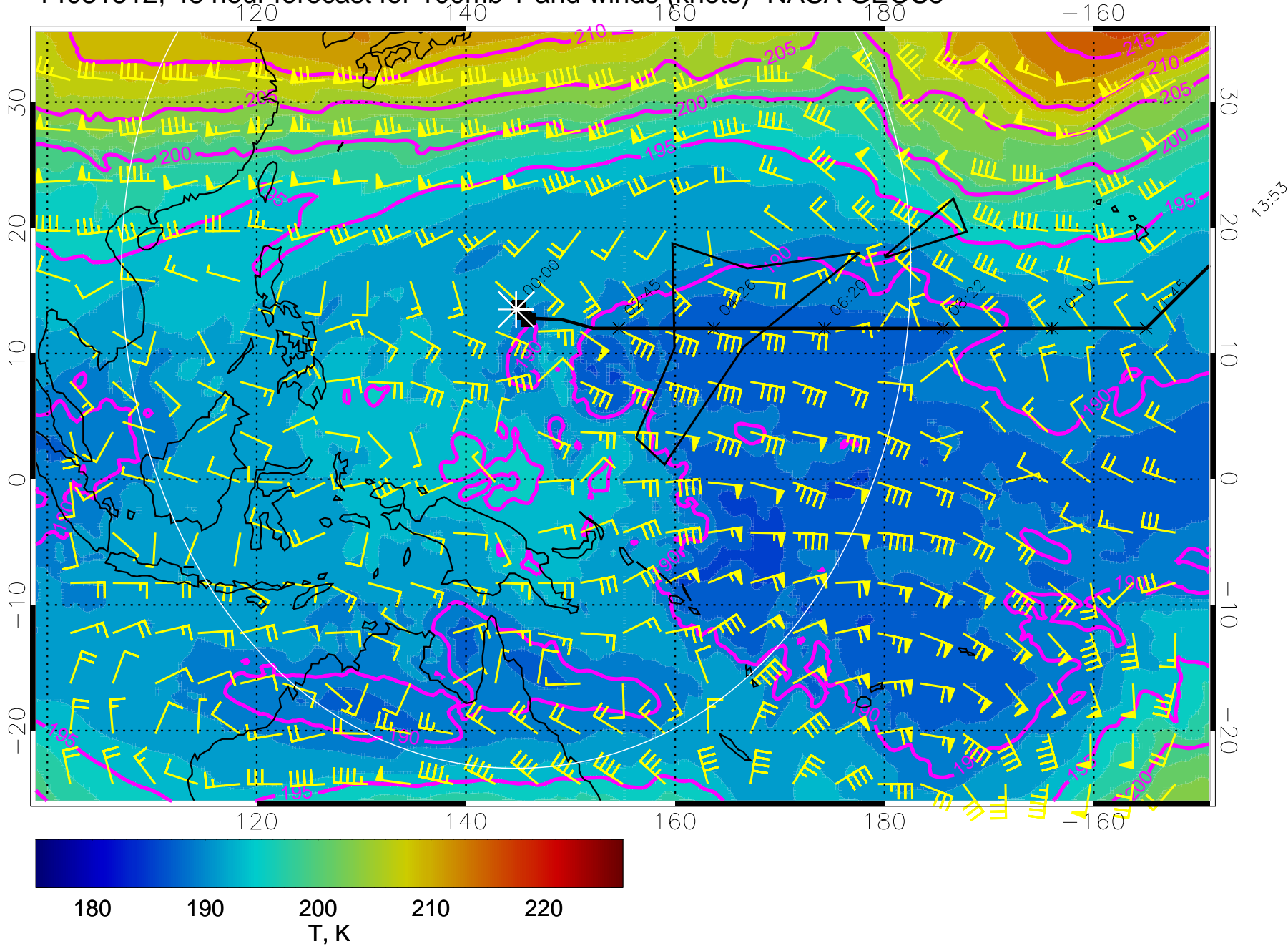
14031512, 48 hour forecast for 100mb T and winds (knots)- NASA GEOS5
