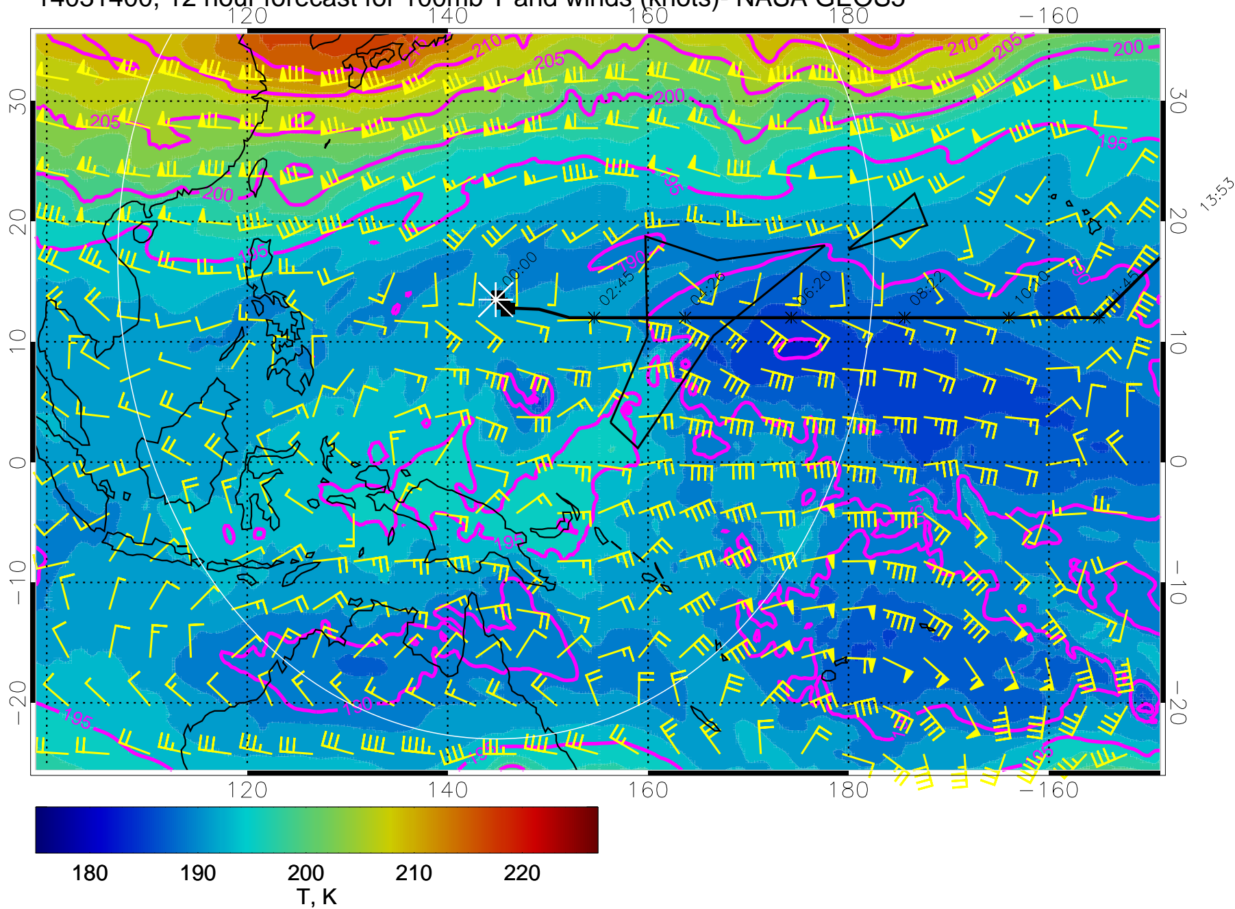
14031400, 12 hour forecast for 100mb T and winds (knots)- NASA GEOS5
