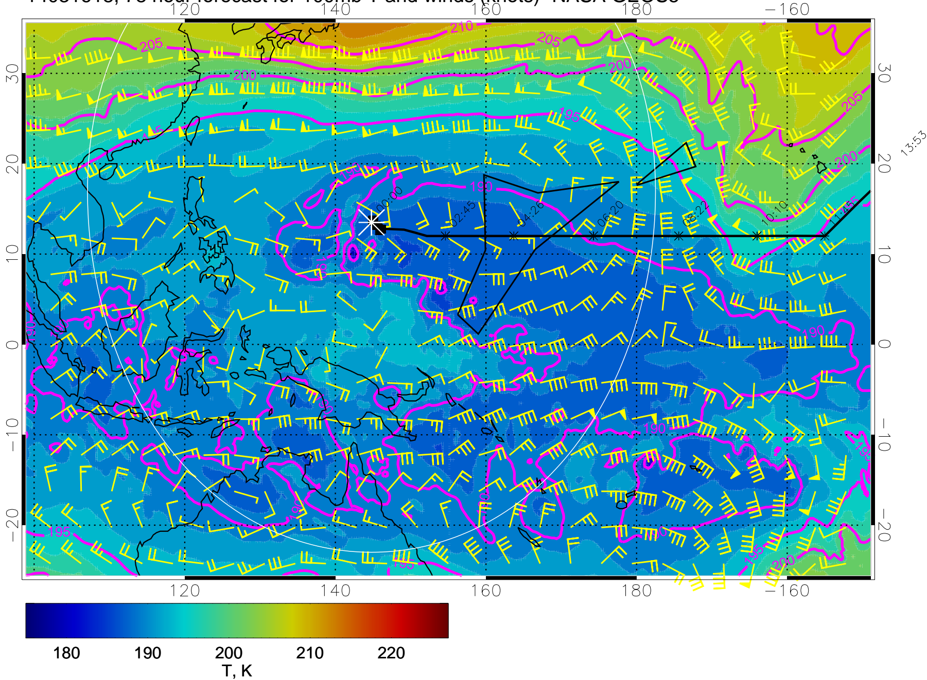
14031618, 78 hour forecast for 100mb T and winds (knots)- NASA GEOS5
