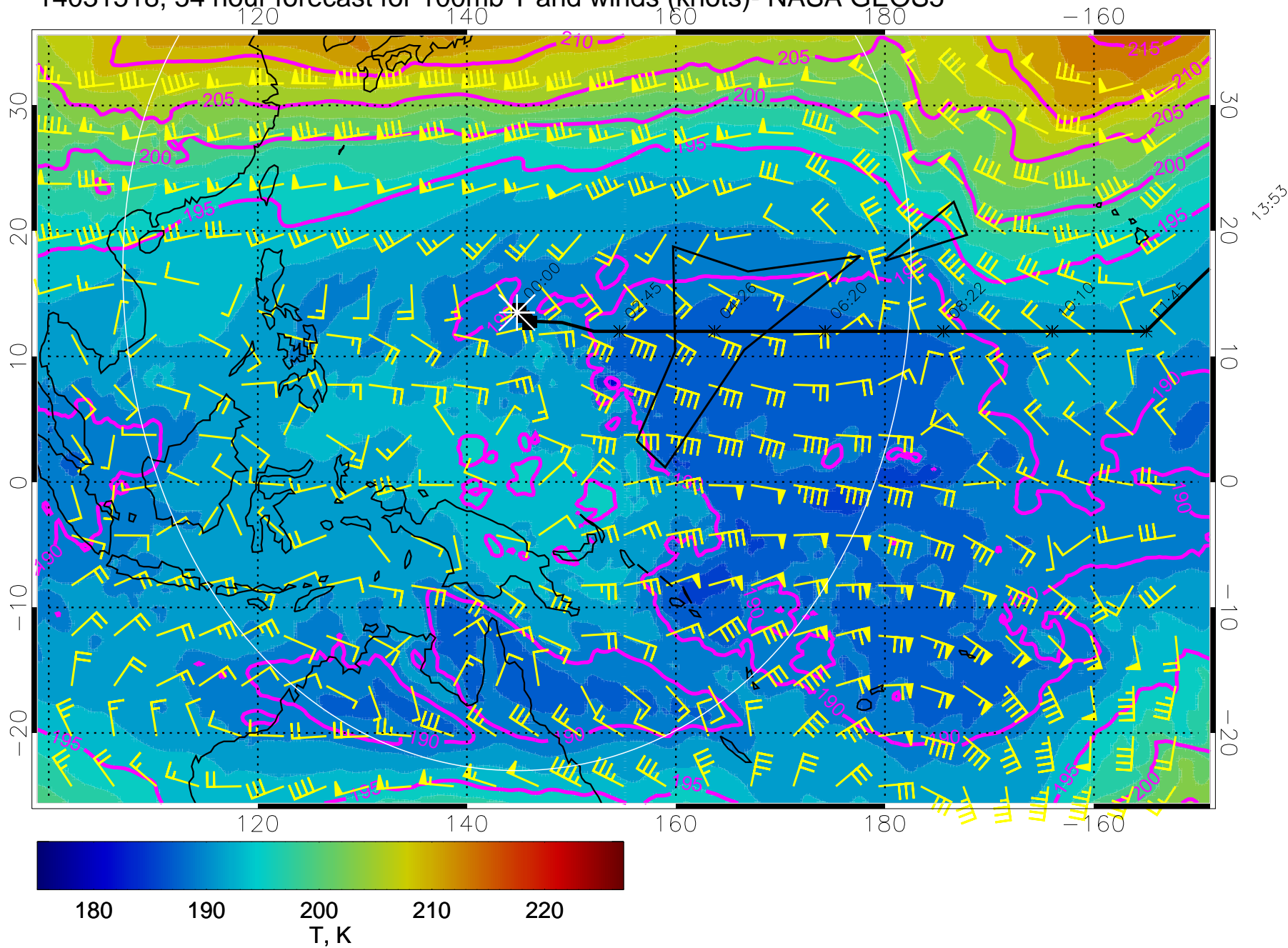
14031518, 54 hour forecast for 100mb T and winds (knots)- NASA GEOS5
