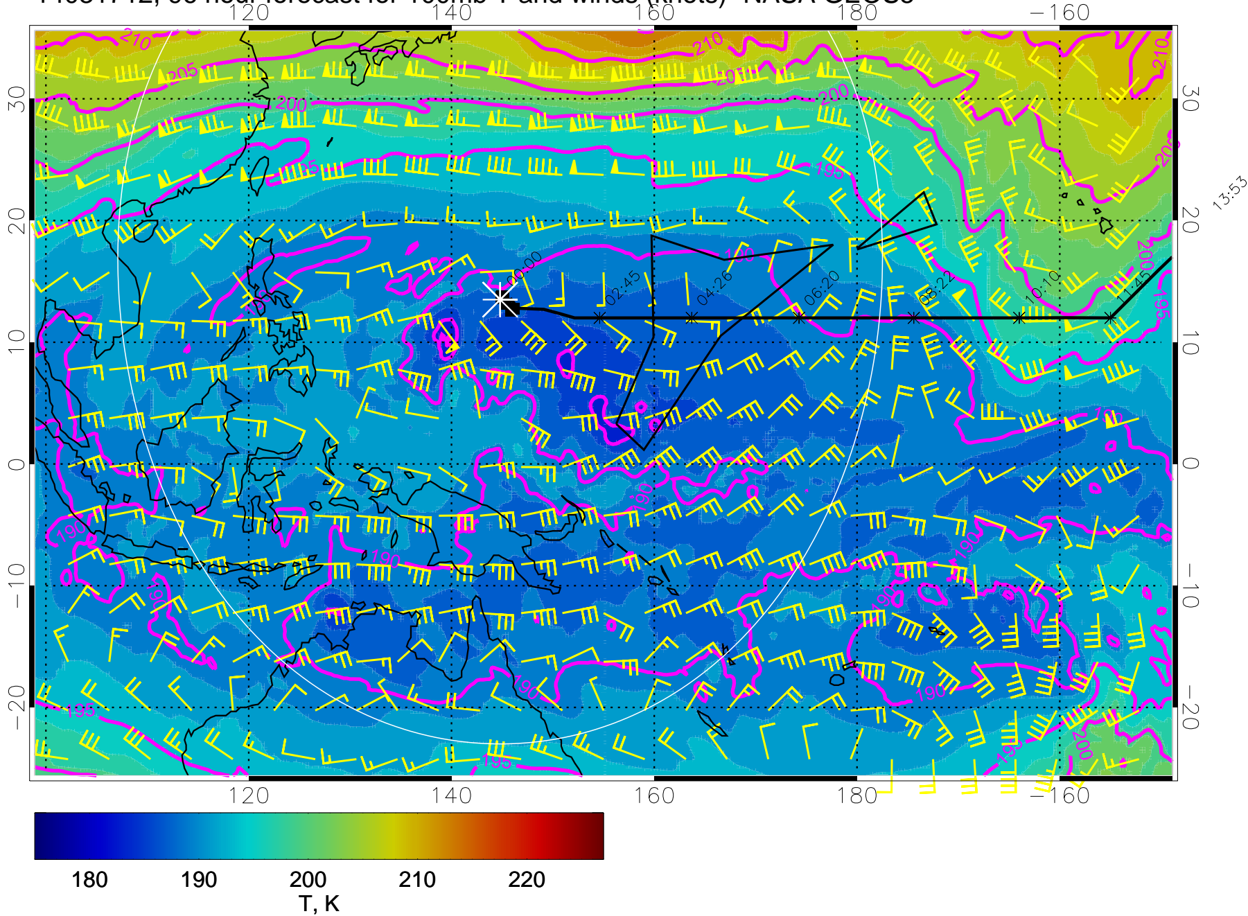
14031712, 96 hour forecast for 100mb T and winds (knots)- NASA GEOS5
