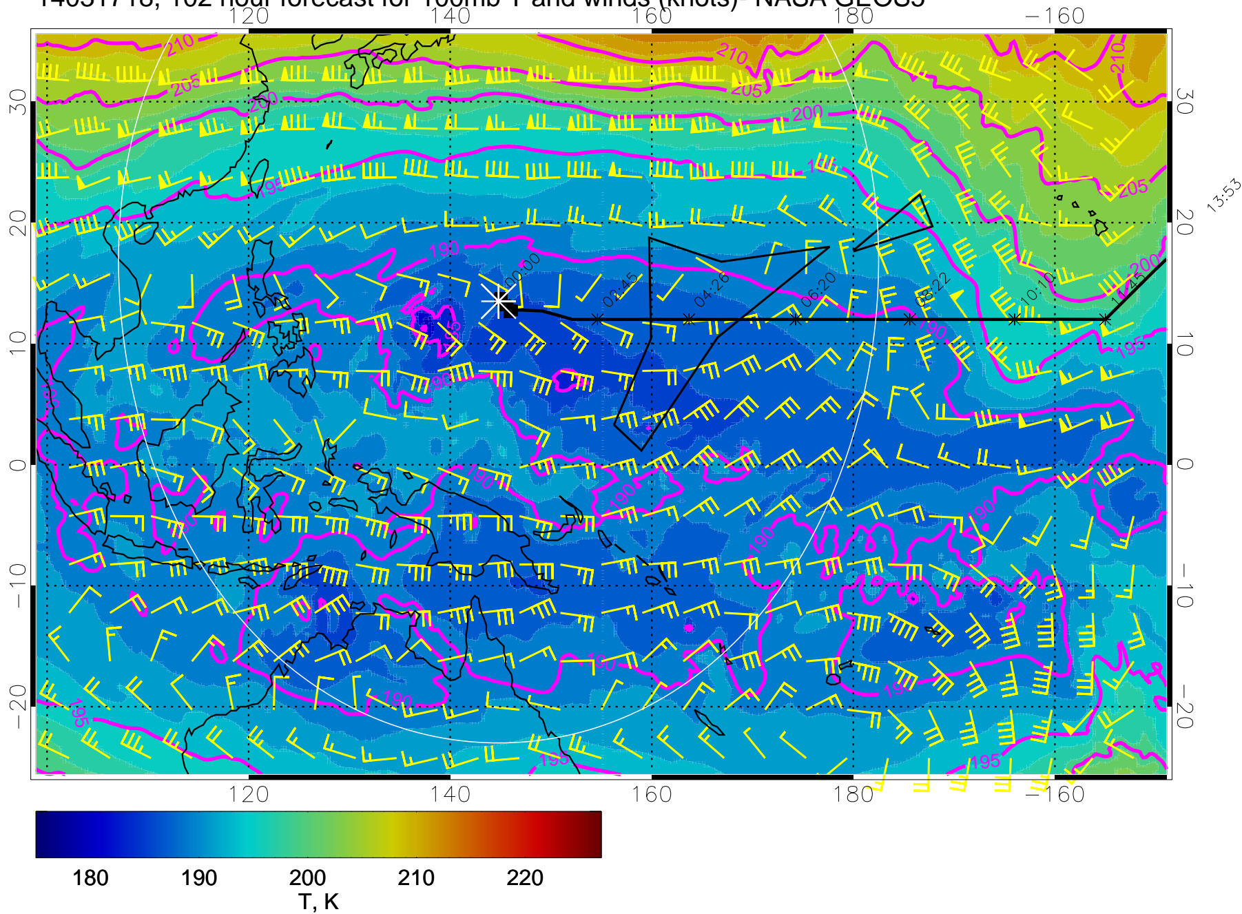
14031718, 102 hour forecast for 100mb T and winds (knots)- NASA GEOS5
