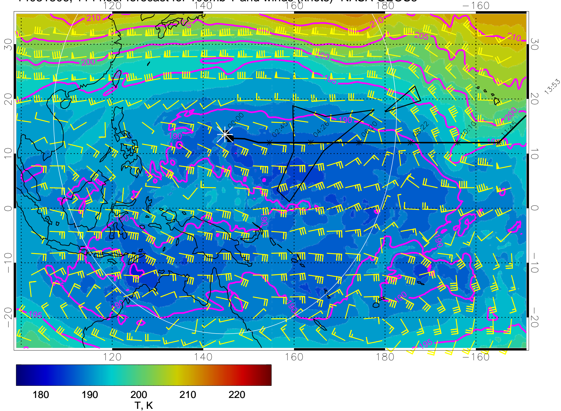
14031806, 114 hour forecast for 100mb T and winds (knots)- NASA GEOS5
