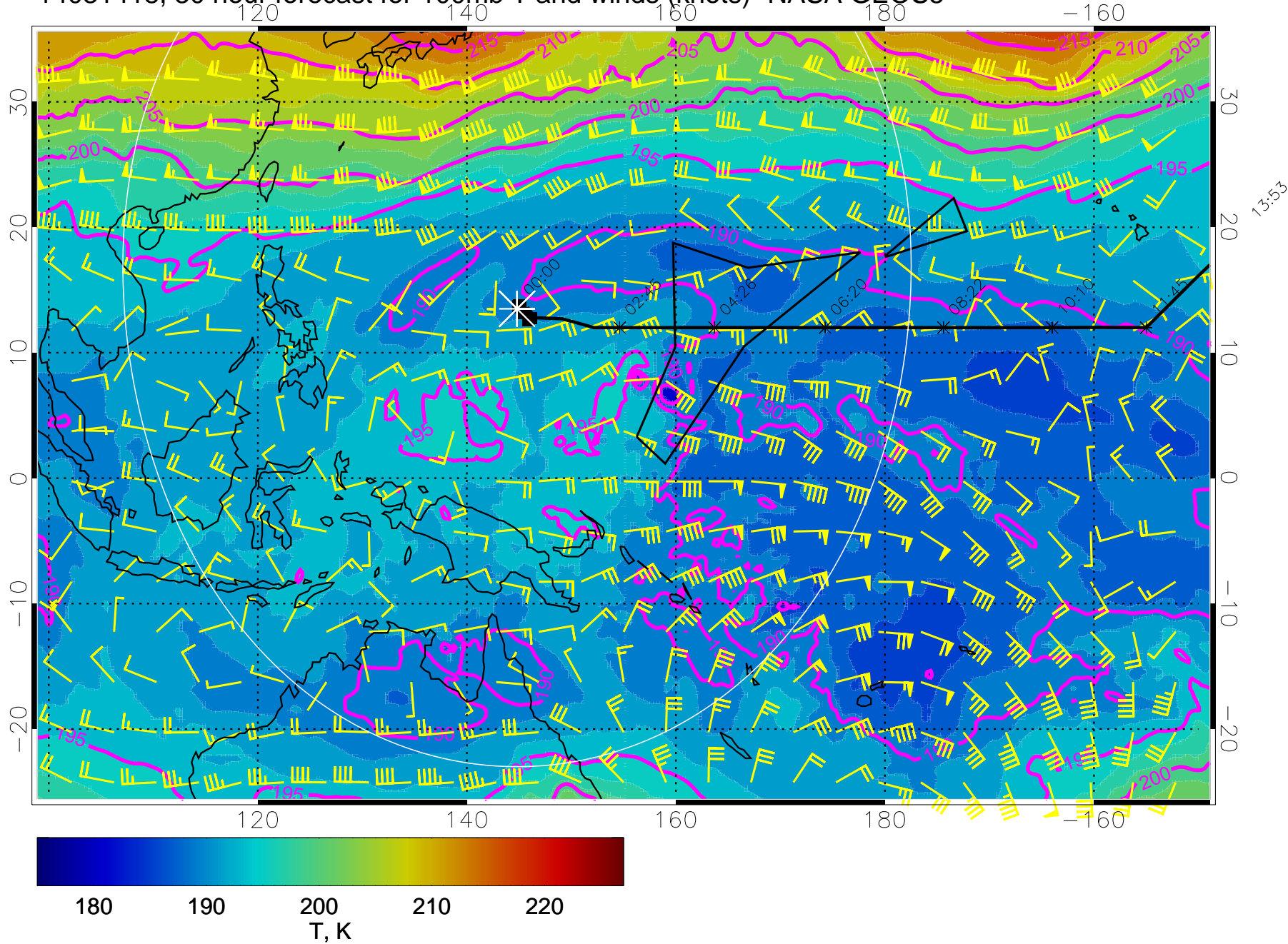
14031418, 30 hour forecast for 100mb T and winds (knots)- NASA GEOS5
