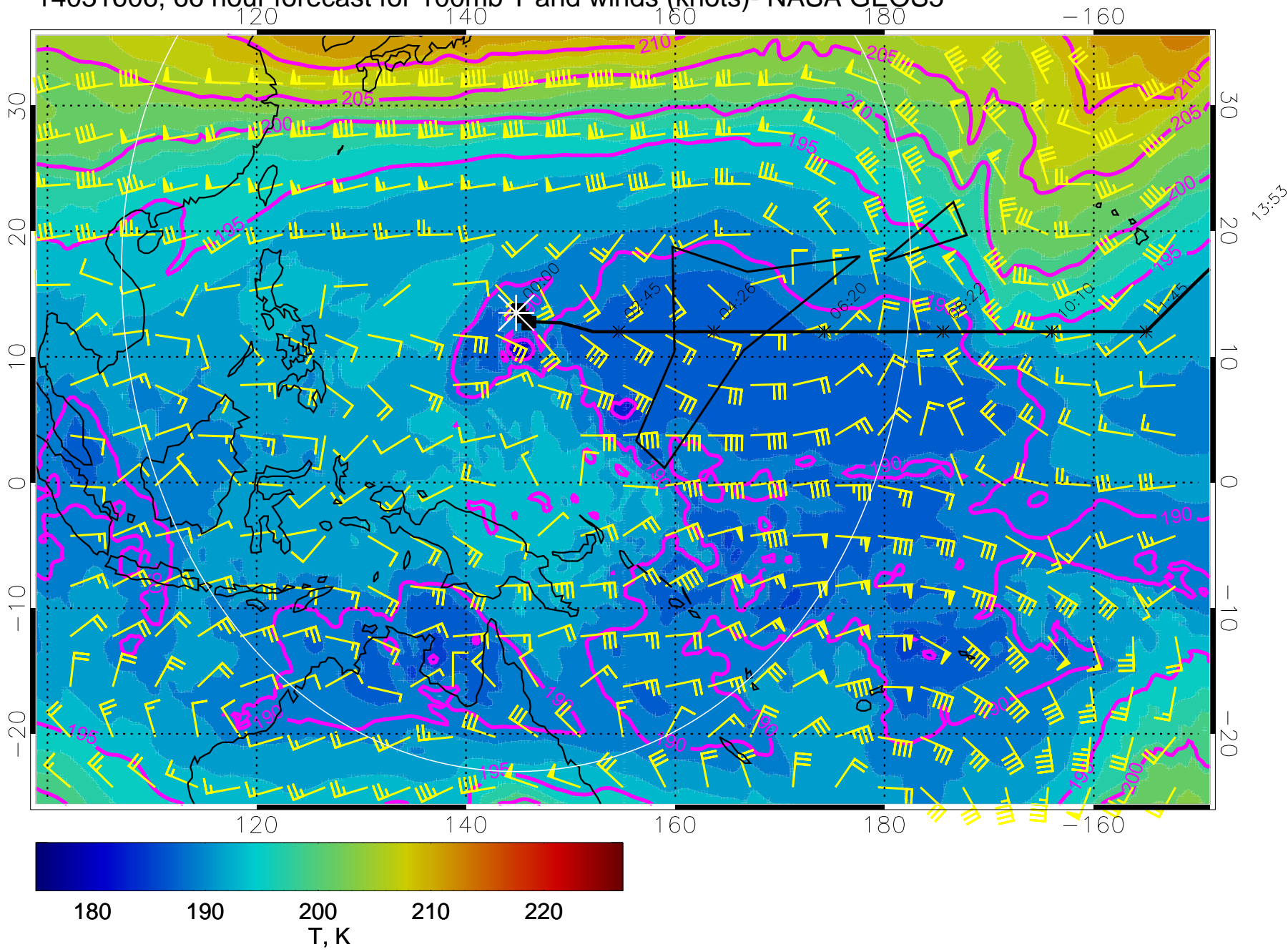
14031606, 66 hour forecast for 100mb T and winds (knots)- NASA GEOS5
