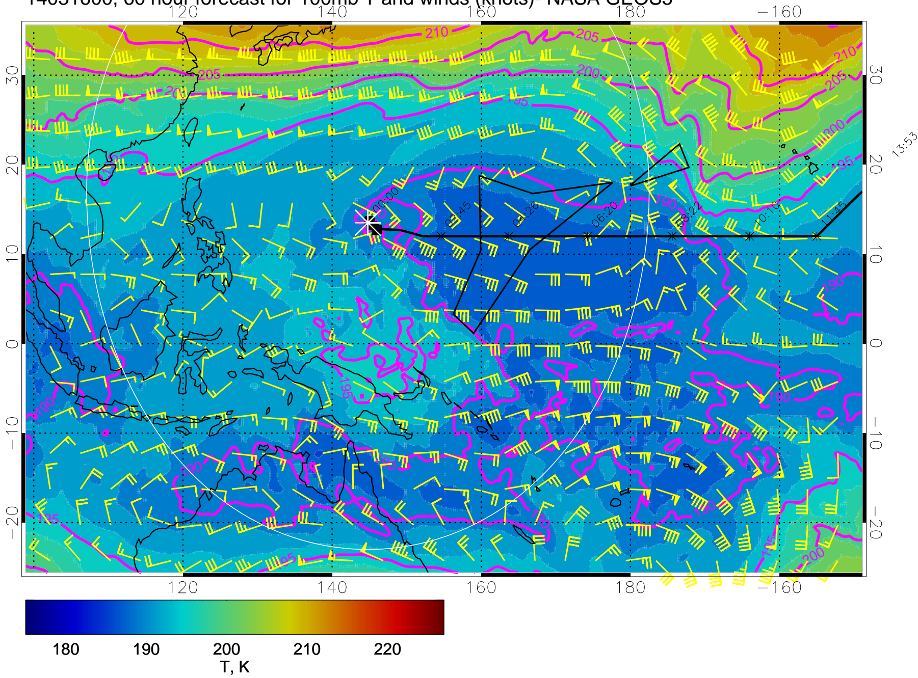
14031600, 60 hour forecast for 100mb T and winds (knots)- NASA GEOS5
