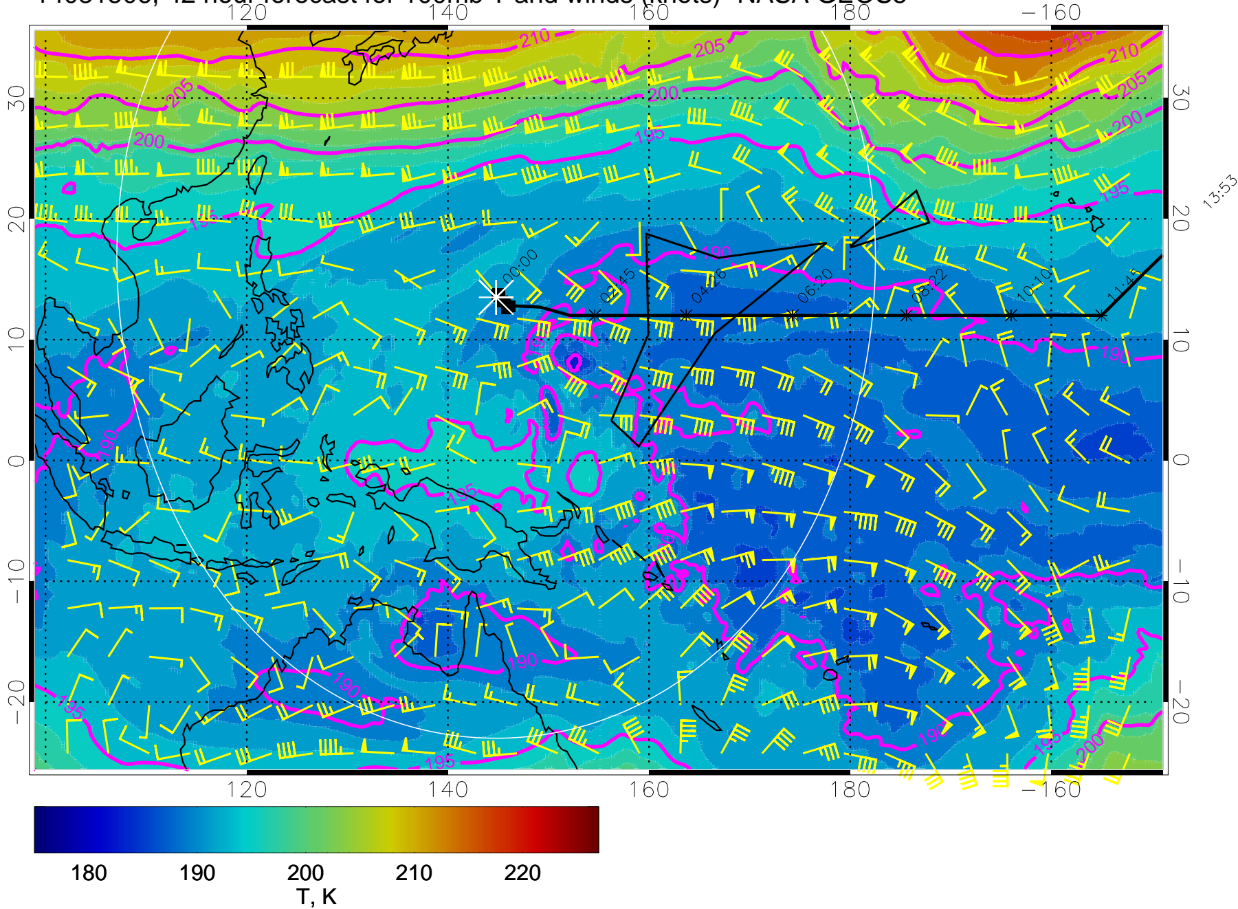
14031506, 42 hour forecast for 100mb T and winds (knots)- NASA GEOS5
