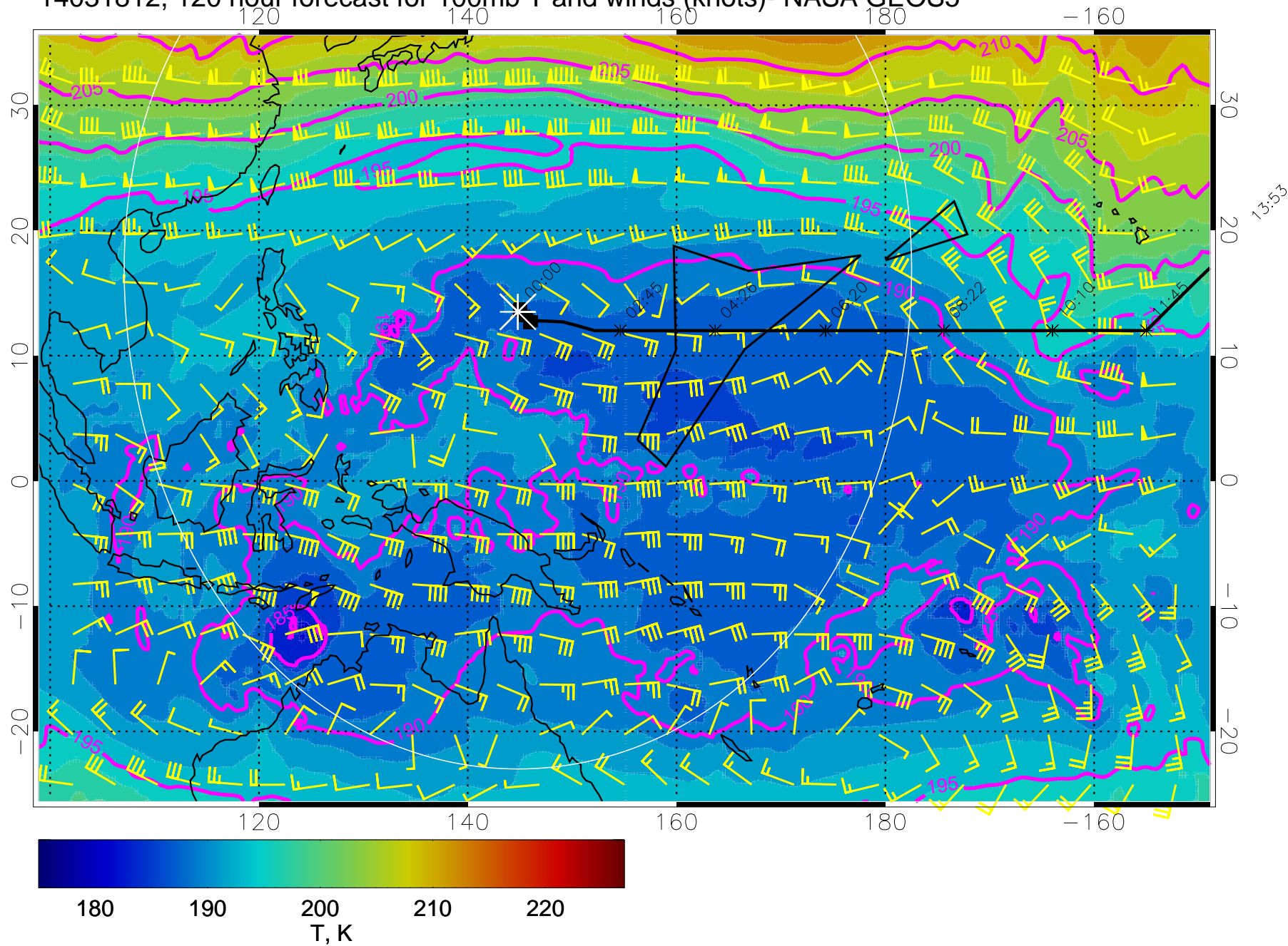
14031812, 120 hour forecast for 100mb T and winds (knots)- NASA GEOS5
