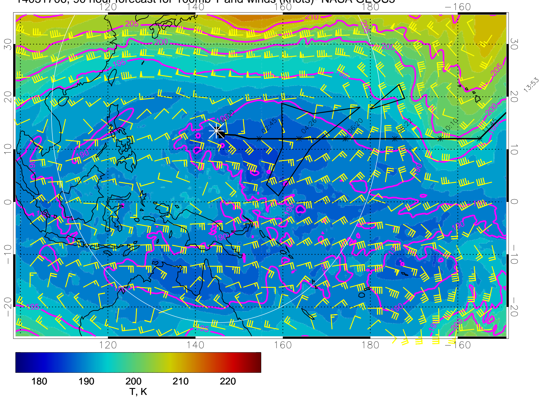
14031706, 90 hour forecast for 100mb T and winds (knots)- NASA GEOS5
