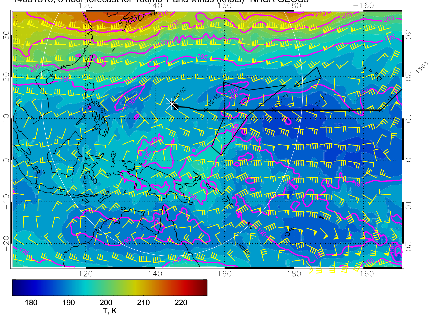
14031318, 6 hour forecast for 100mb T and winds (knots)- NASA GEOS5
