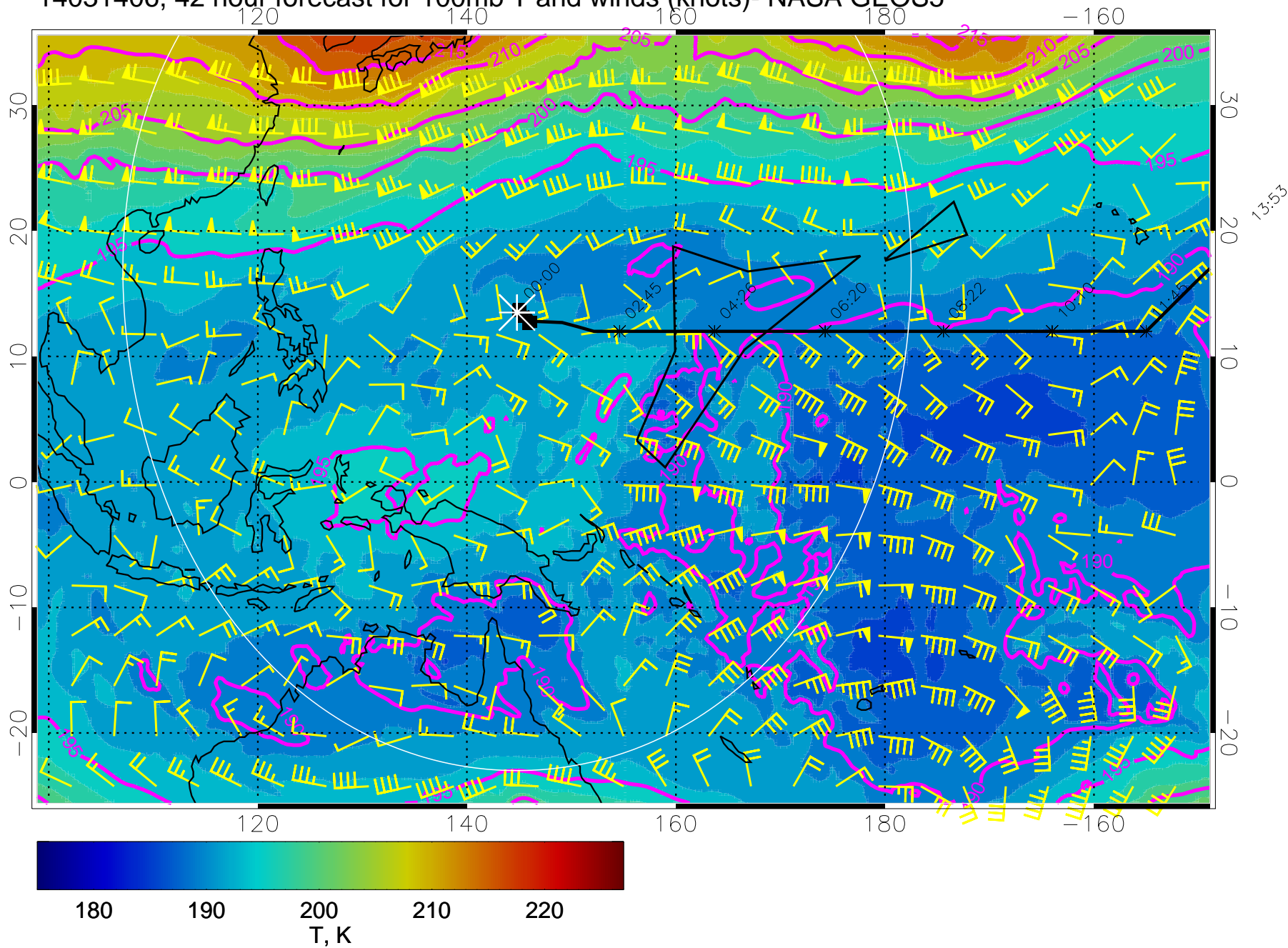
14031406, 42 hour forecast for 100mb T and winds (knots)- NASA GEOS5
