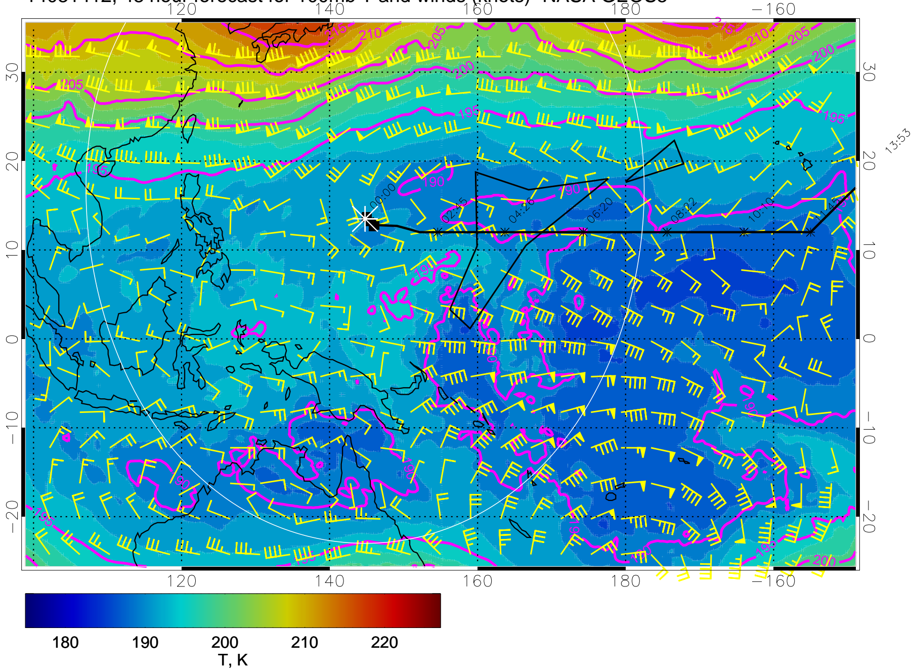
14031412, 48 hour forecast for 100mb T and winds (knots)- NASA GEOS5
