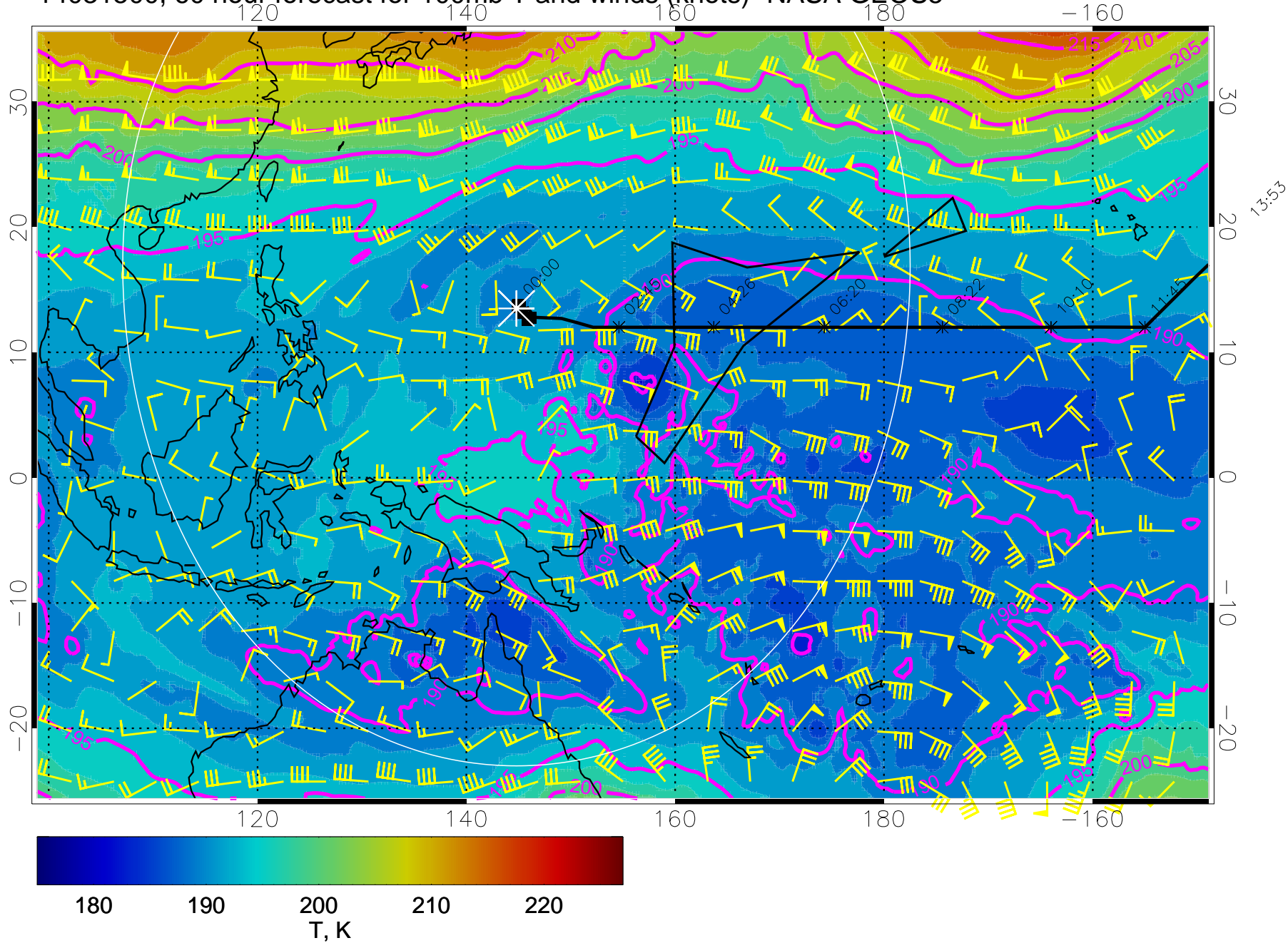
14031500, 60 hour forecast for 100mb T and winds (knots)- NASA GEOS5
