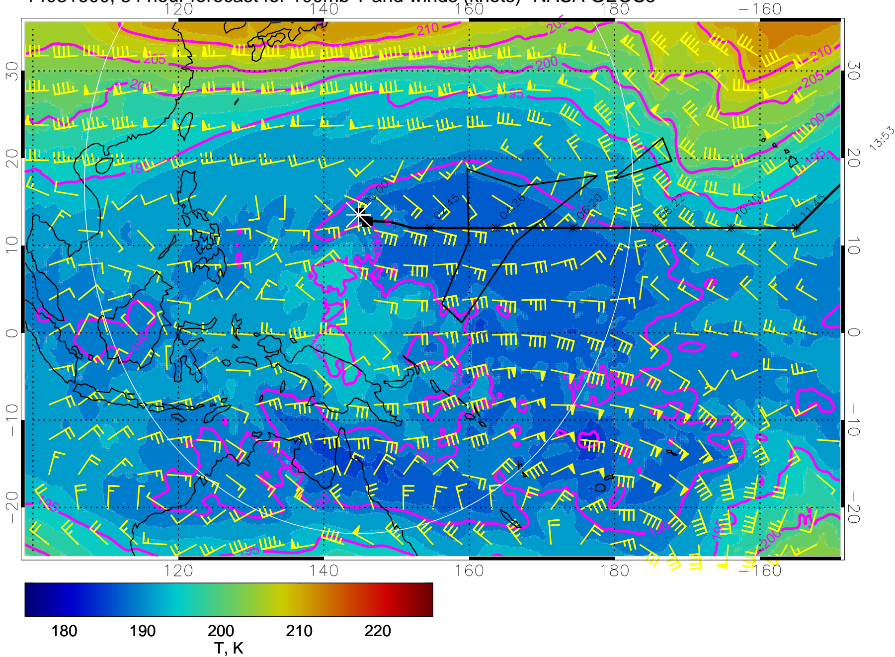
14031600, 84 hour forecast for 100mb T and winds (knots)- NASA GEOS5
