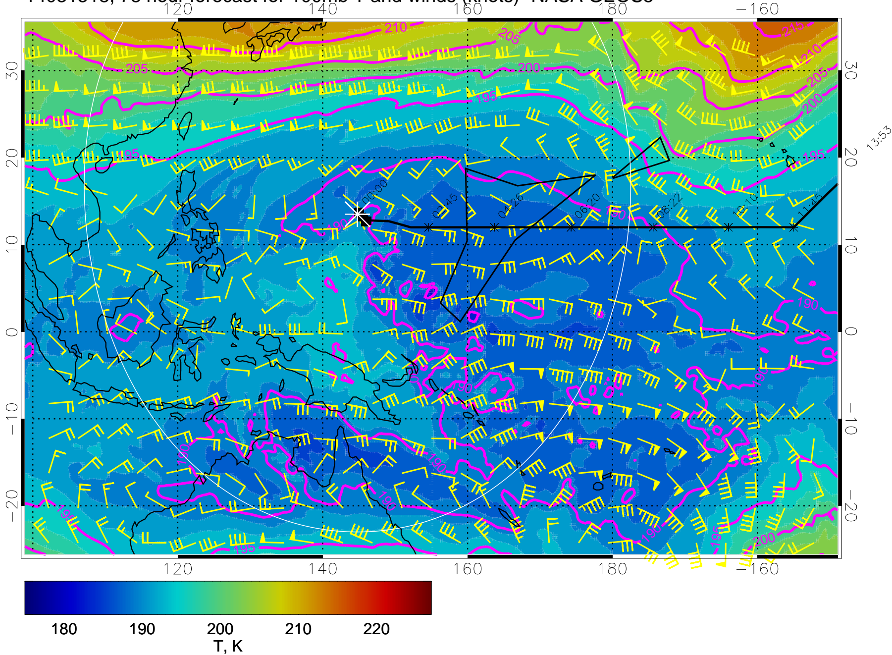
14031518, 78 hour forecast for 100mb T and winds (knots)- NASA GEOS5
