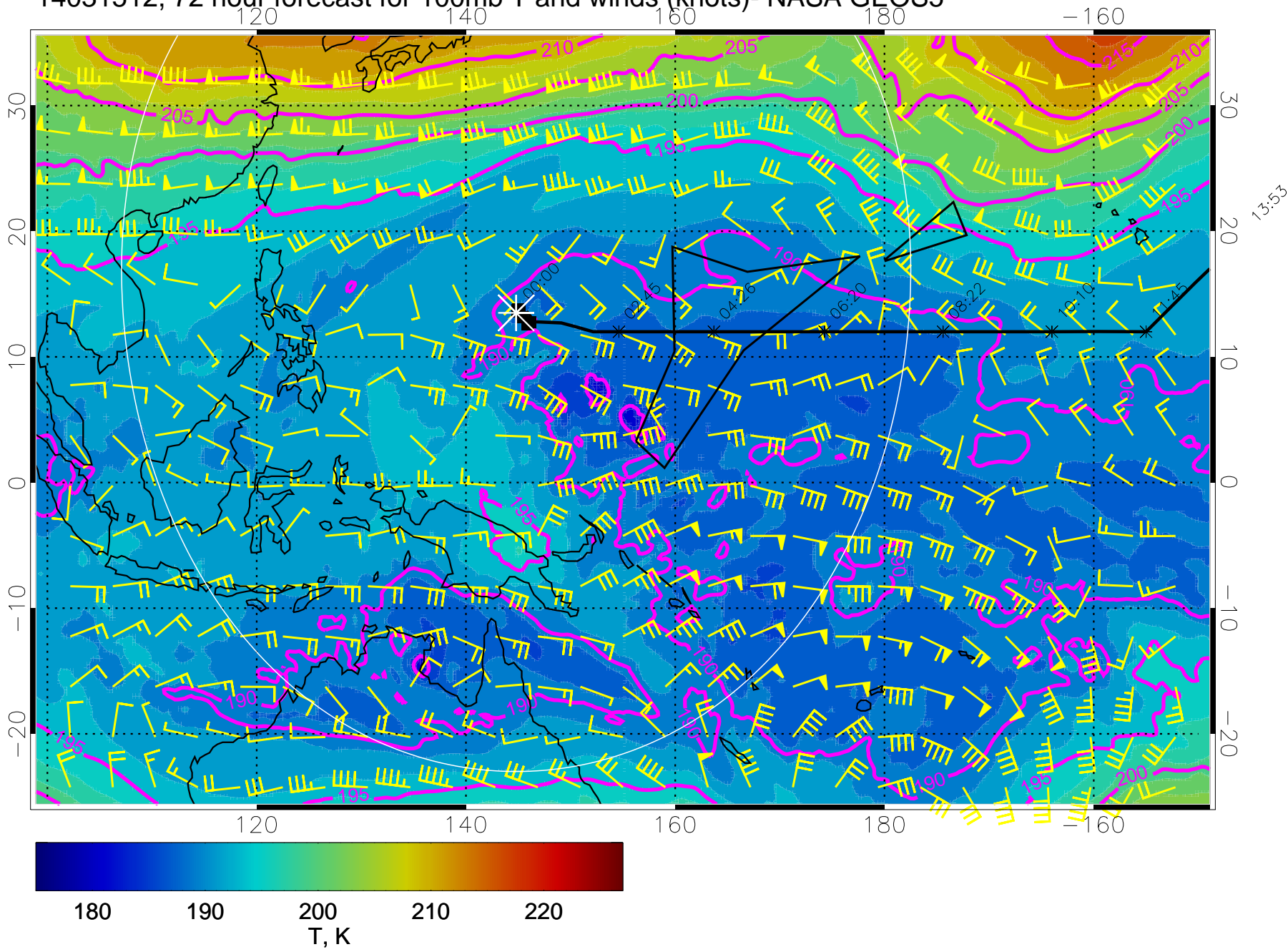
14031512, 72 hour forecast for 100mb T and winds (knots)- NASA GEOS5
