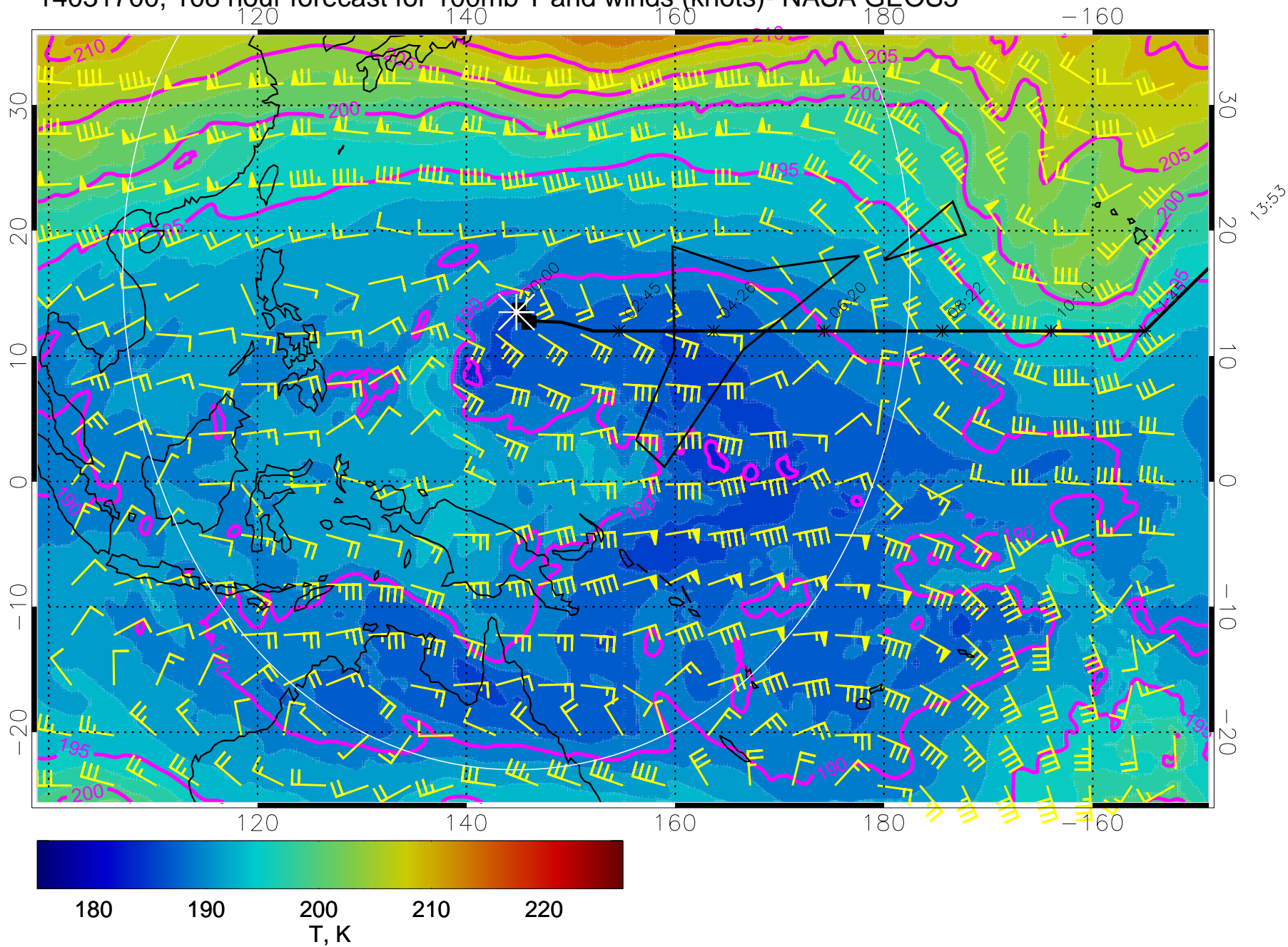
14031700, 108 hour forecast for 100mb T and winds (knots)- NASA GEOS5
