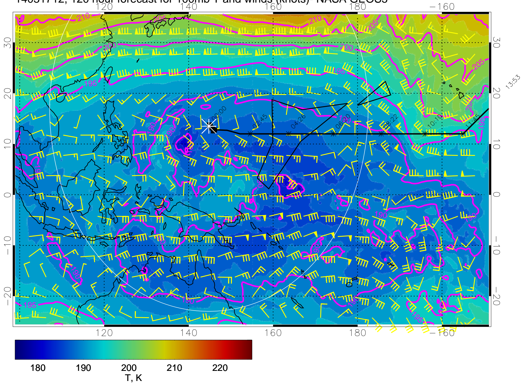
14031712, 120 hour forecast for 100mb T and winds (knots)- NASA GEOS5
