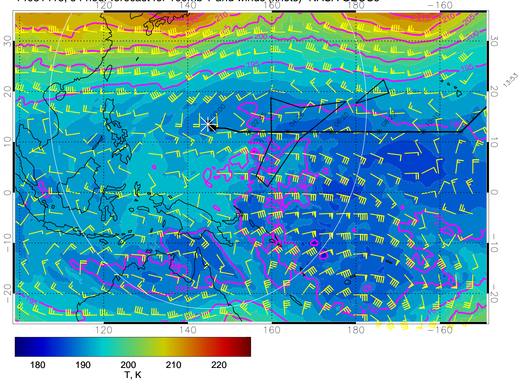
14031418, 54 hour forecast for 100mb T and winds (knots)- NASA GEOS5
