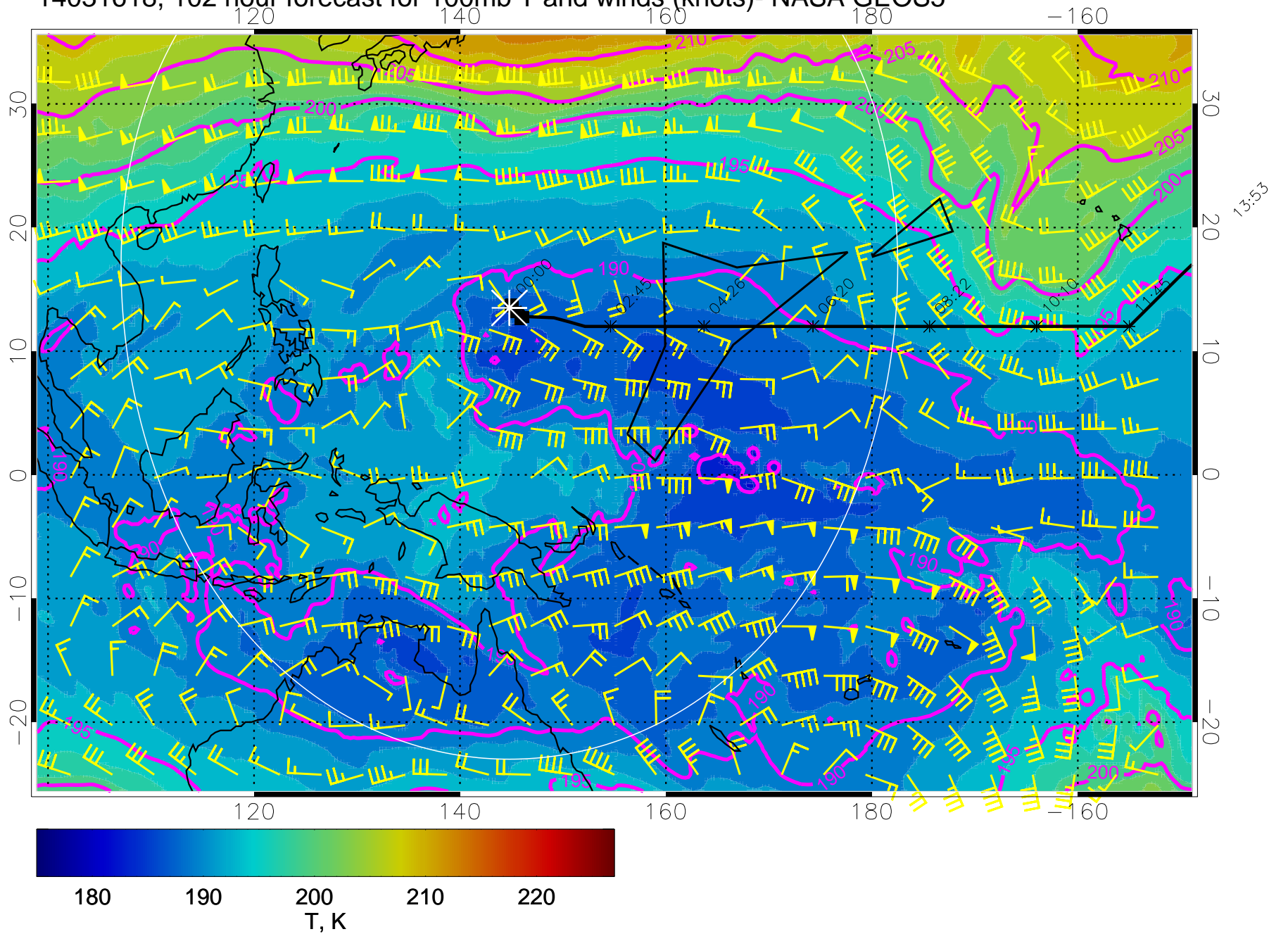
14031618, 102 hour forecast for 100mb T and winds (knots)- NASA GEOS5
