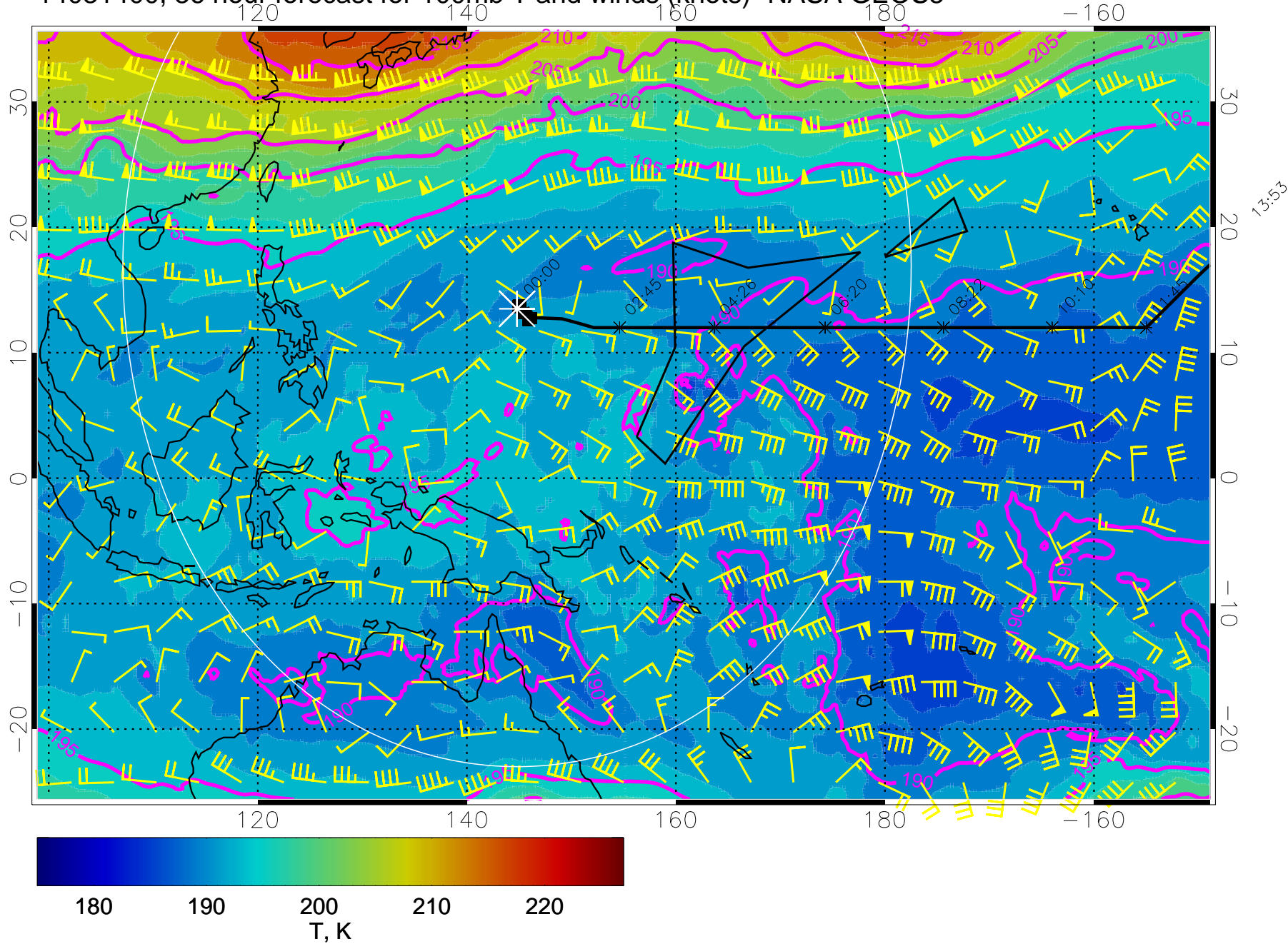
14031400, 36 hour forecast for 100mb T and winds (knots)- NASA GEOS5
