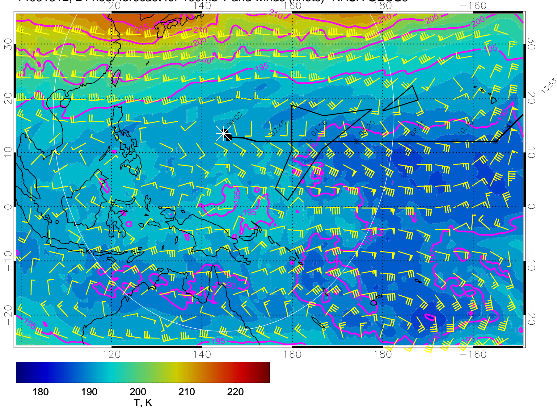
14031312, 24 hour forecast for 100mb T and winds (knots)- NASA GEOS5
