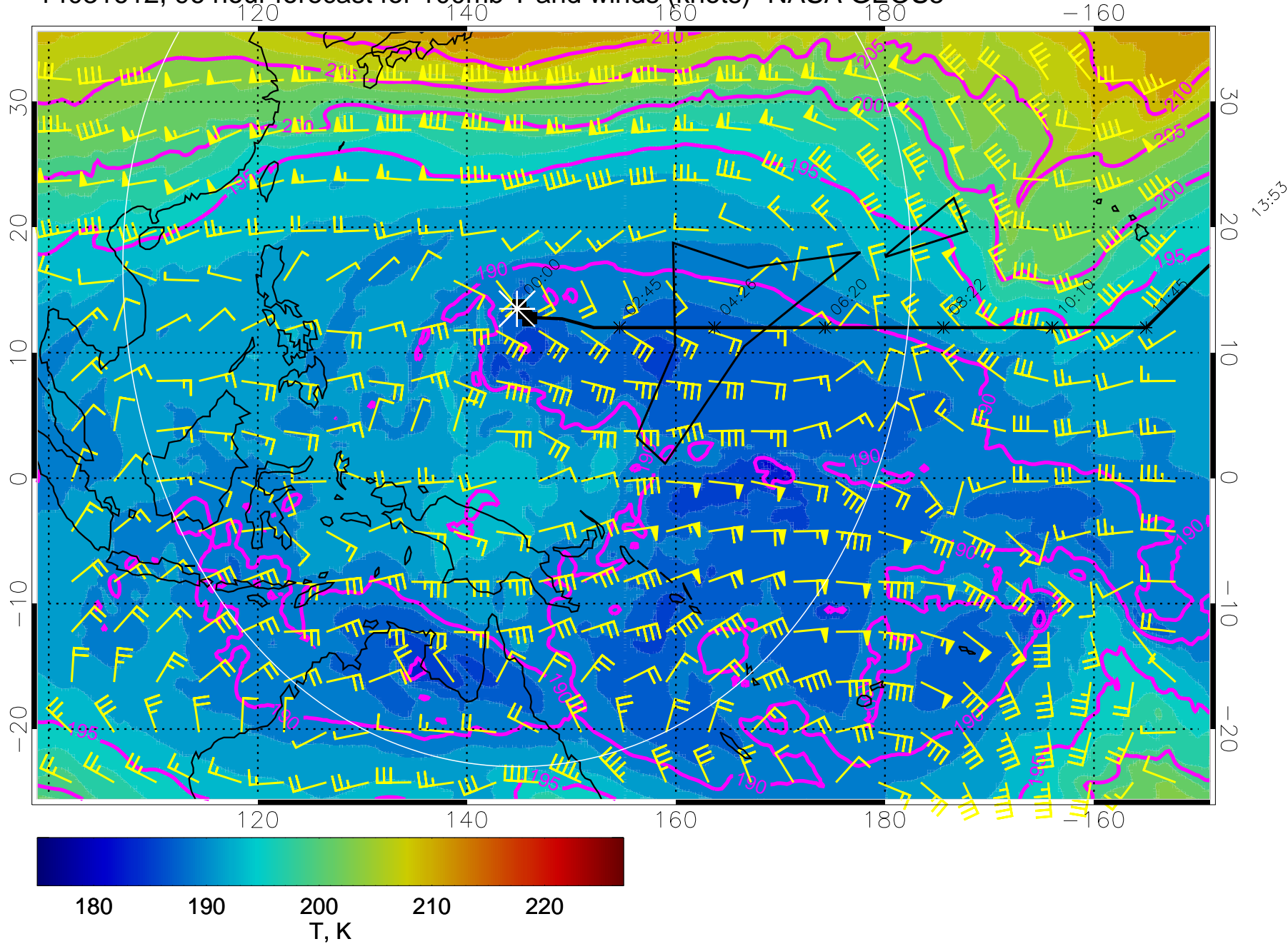
14031612, 96 hour forecast for 100mb T and winds (knots)- NASA GEOS5
