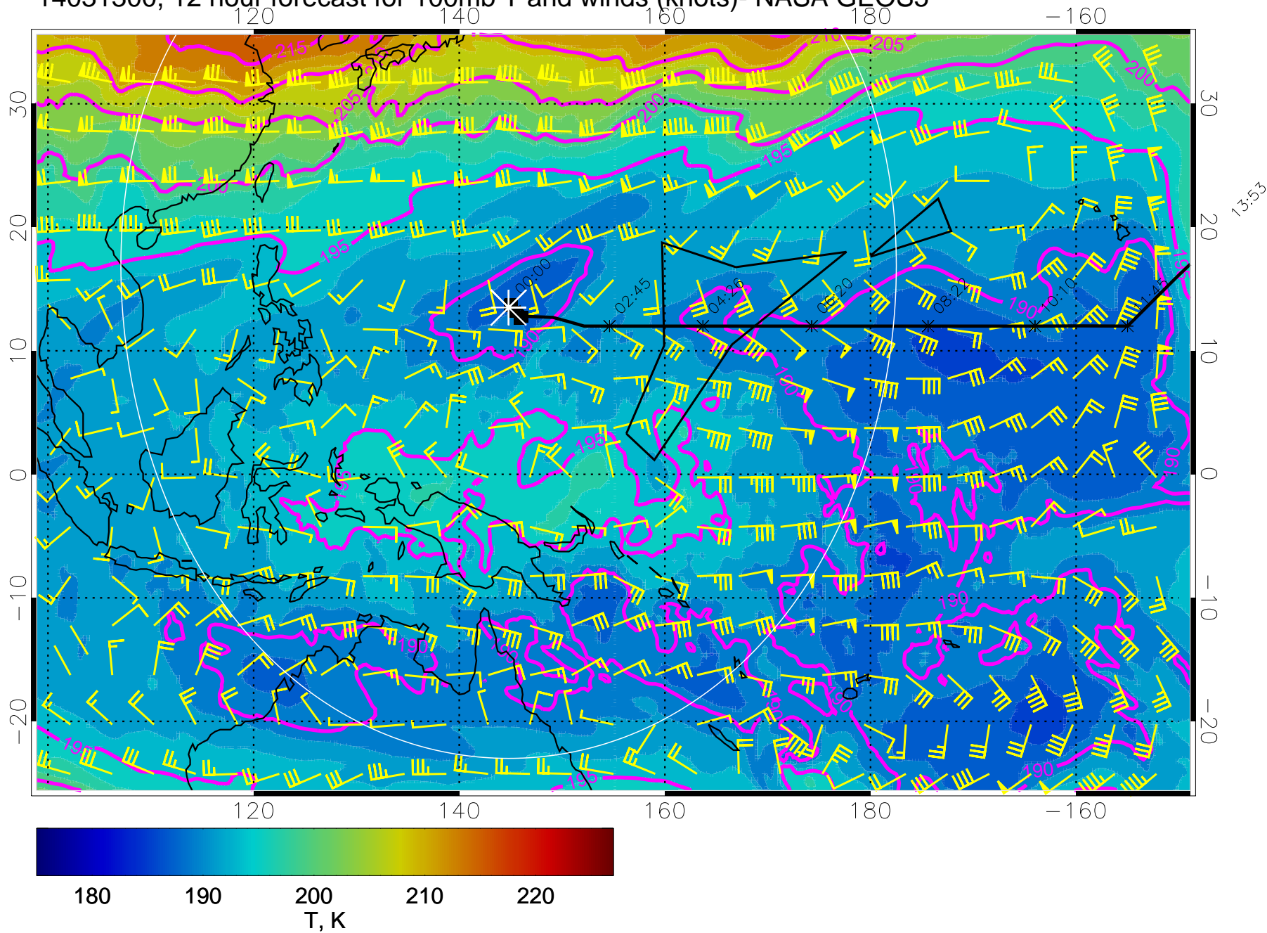
14031300, 12 hour forecast for 100mb T and winds (knots)- NASA GEOS5
