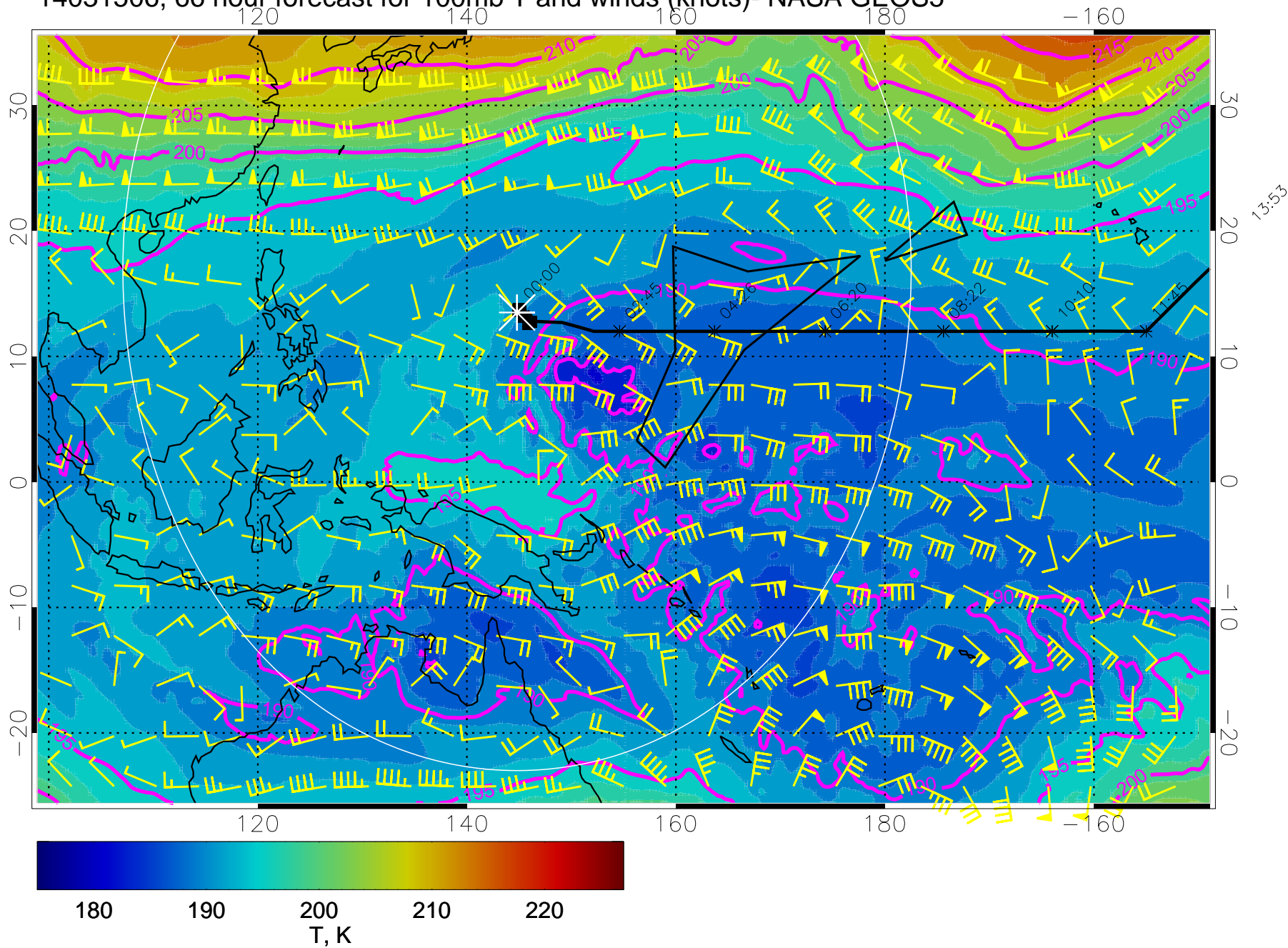
14031506, 66 hour forecast for 100mb T and winds (knots)- NASA GEOS5
