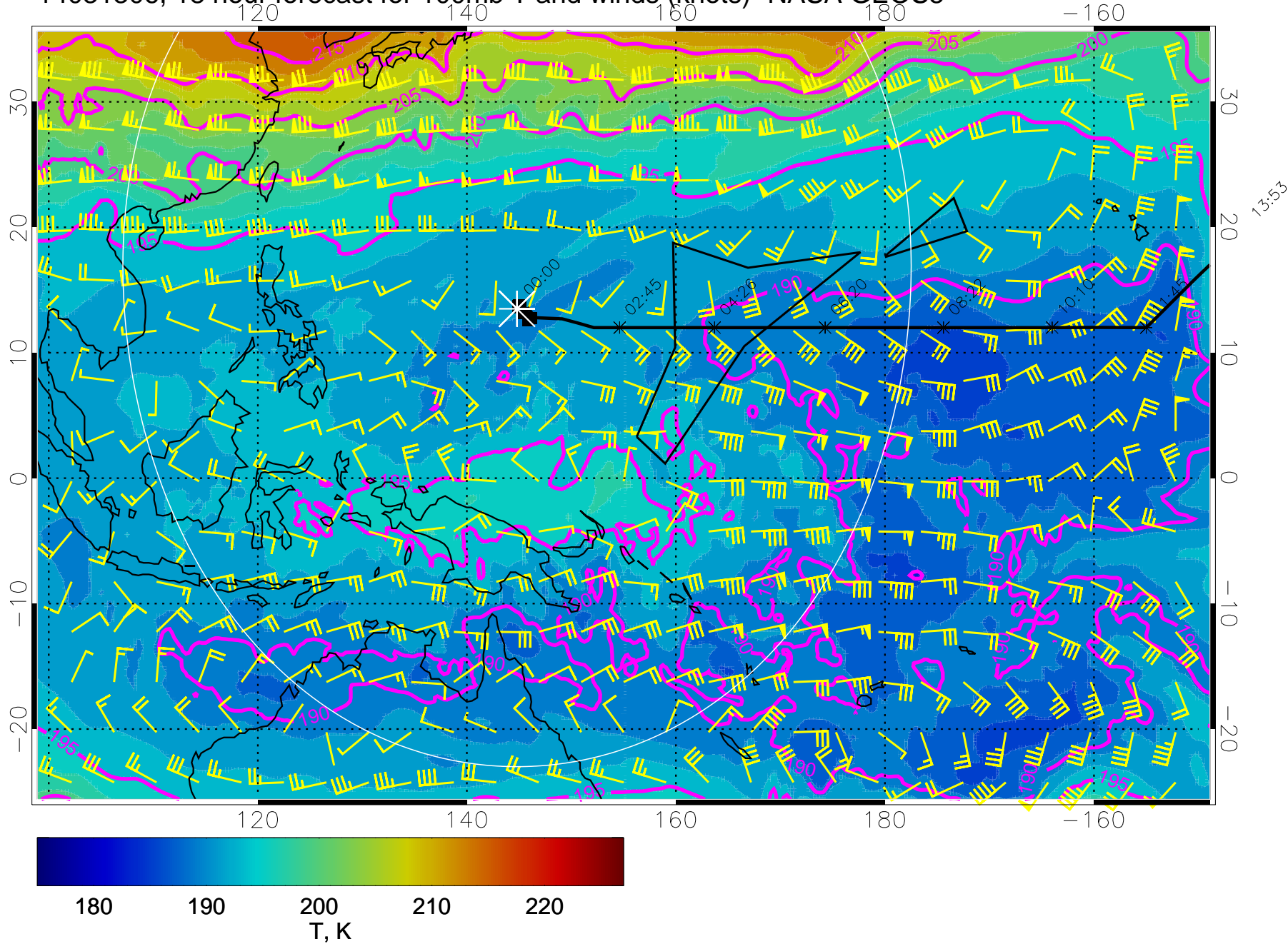
14031306, 18 hour forecast for 100mb T and winds (knots)- NASA GEOS5
