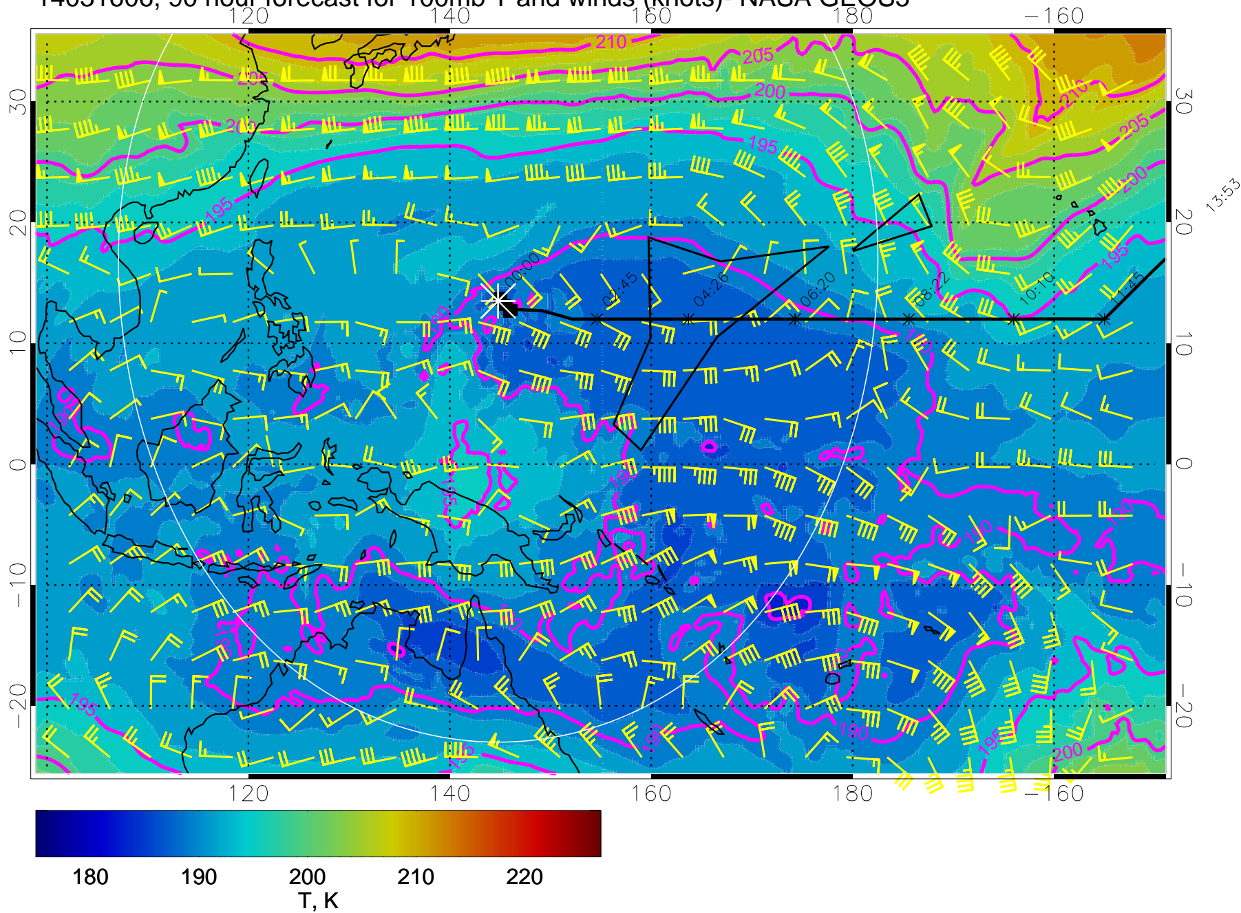
14031606, 90 hour forecast for 100mb T and winds (knots)- NASA GEOS5
