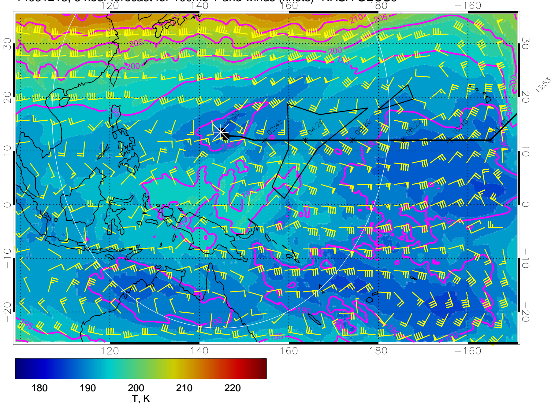
14031218, 6 hour forecast for 100mb T and winds (knots)- NASA GEOS5
