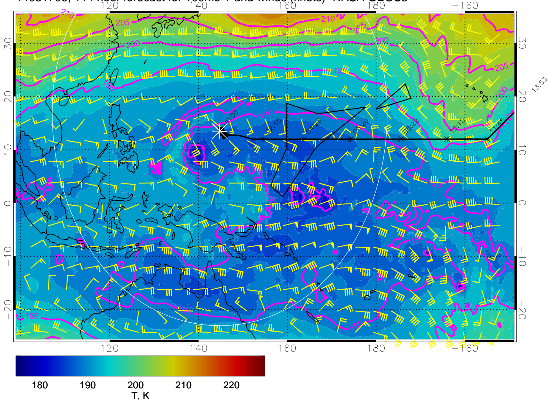
14031706, 114 hour forecast for 100mb T and winds (knots)- NASA GEOS5
