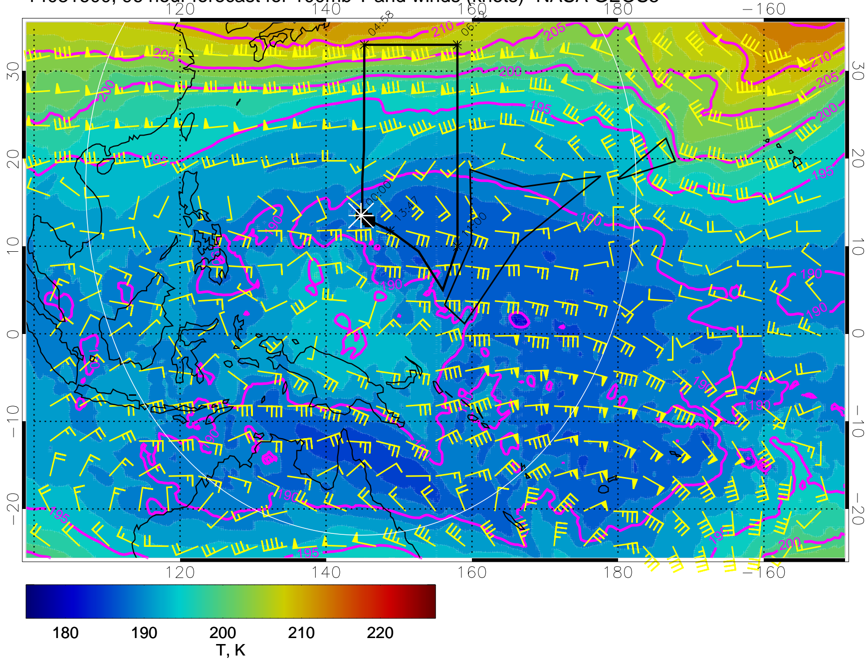
14031600, 96 hour forecast for 100mb T and winds (knots)- NASA GEOS5
