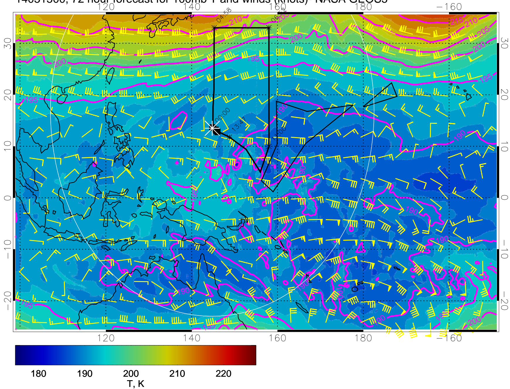
14031500, 72 hour forecast for 100mb T and winds (knots)- NASA GEOS5
