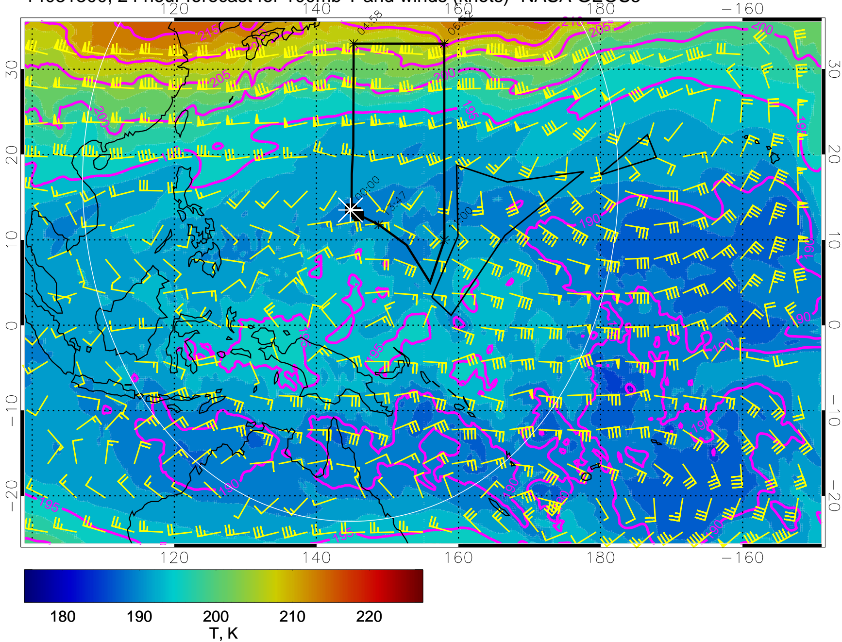
14031300, 24 hour forecast for 100mb T and winds (knots)- NASA GEOS5
