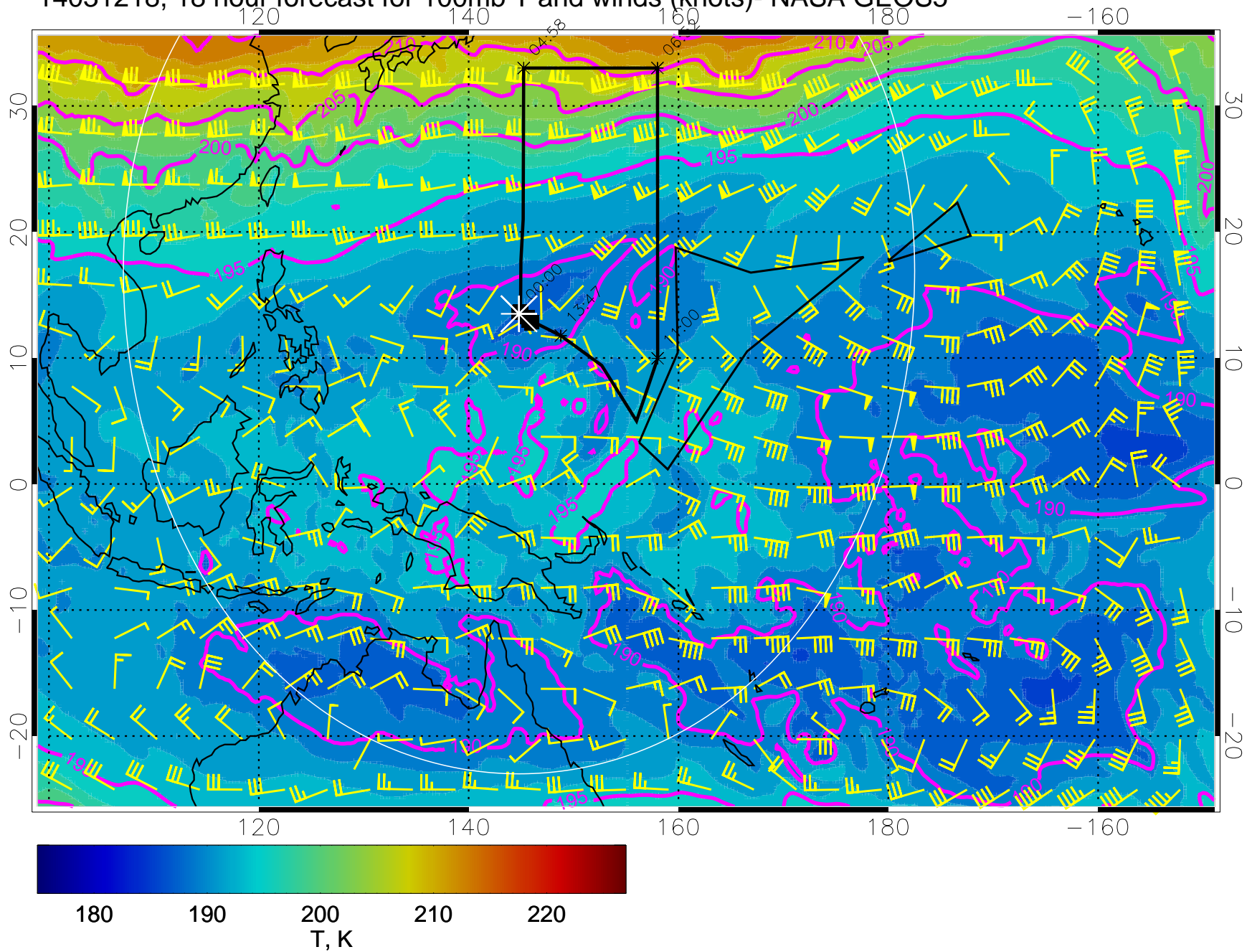
14031218, 18 hour forecast for 100mb T and winds (knots)- NASA GEOS5
