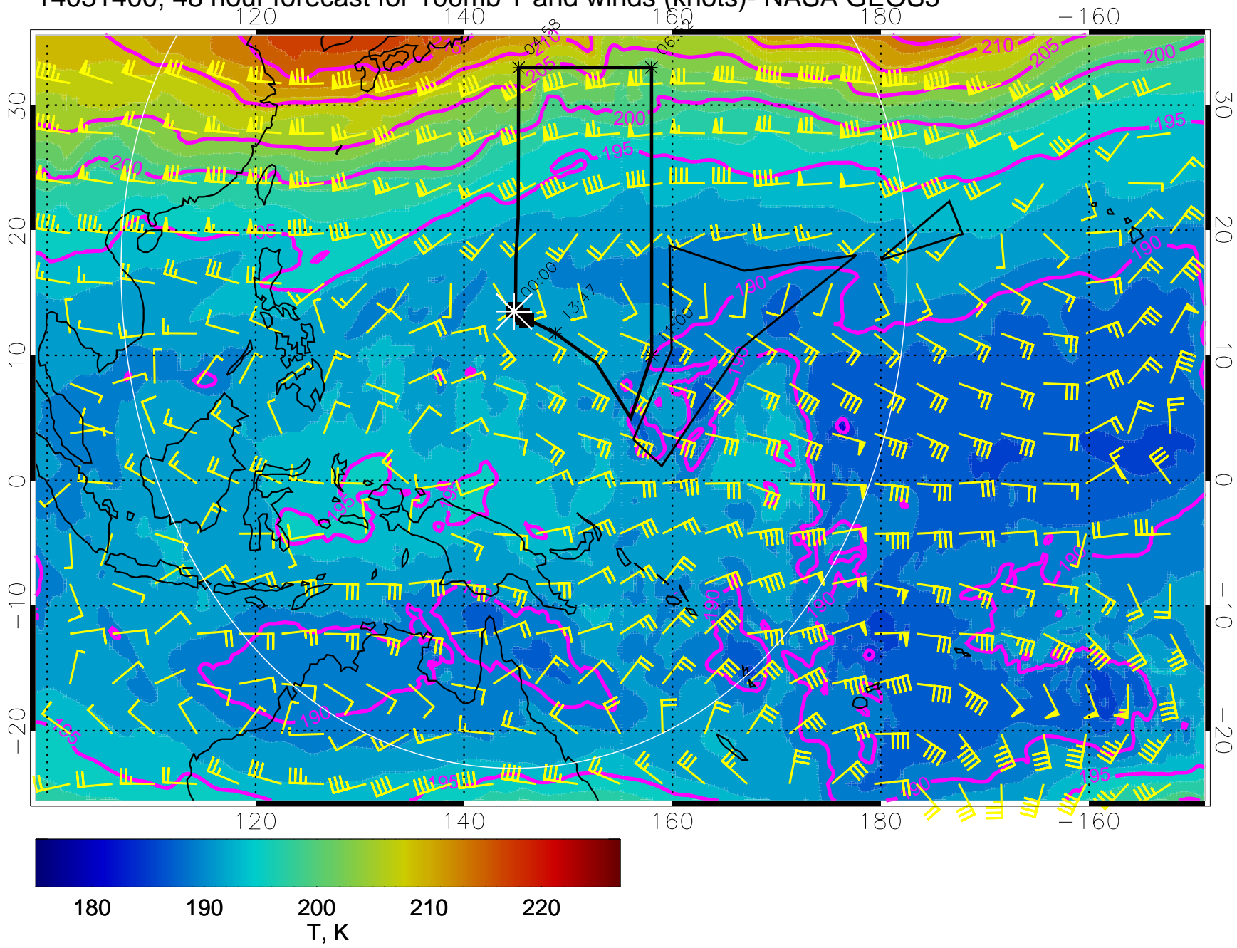
14031400, 48 hour forecast for 100mb T and winds (knots)- NASA GEOS5
