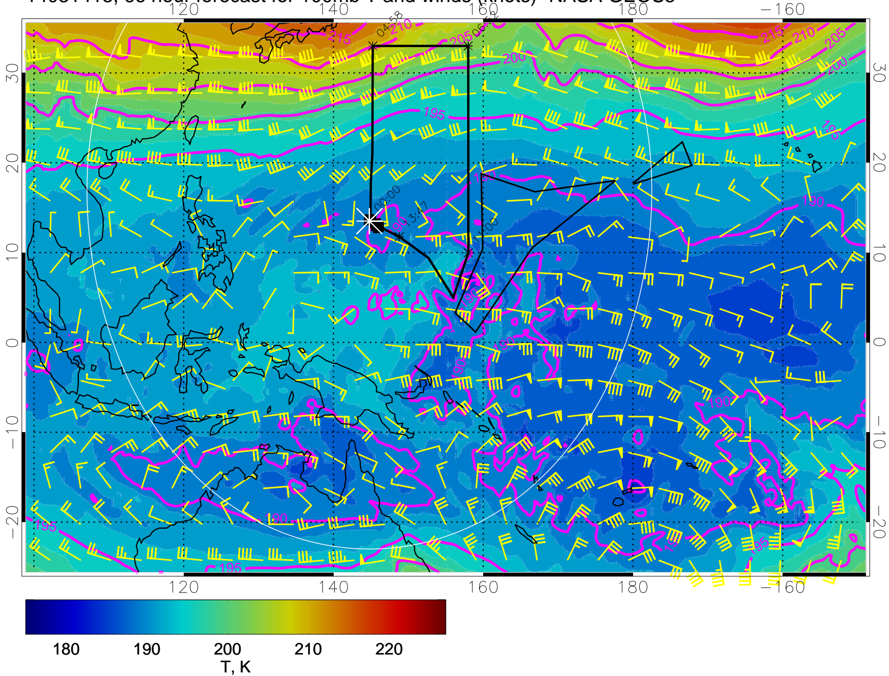
14031418, 66 hour forecast for 100mb T and winds (knots)- NASA GEOS5
