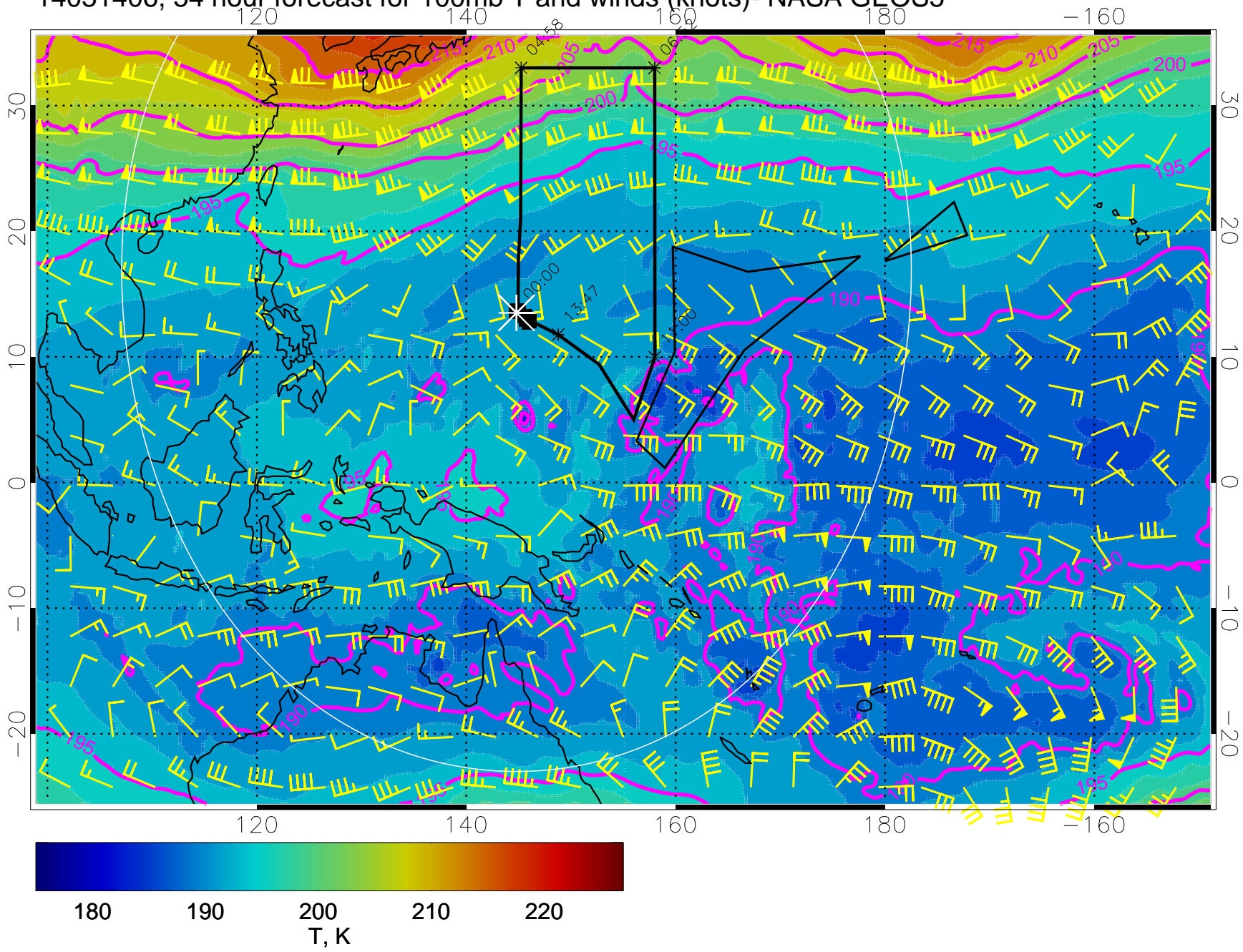
14031406, 54 hour forecast for 100mb T and winds (knots)- NASA GEOS5
