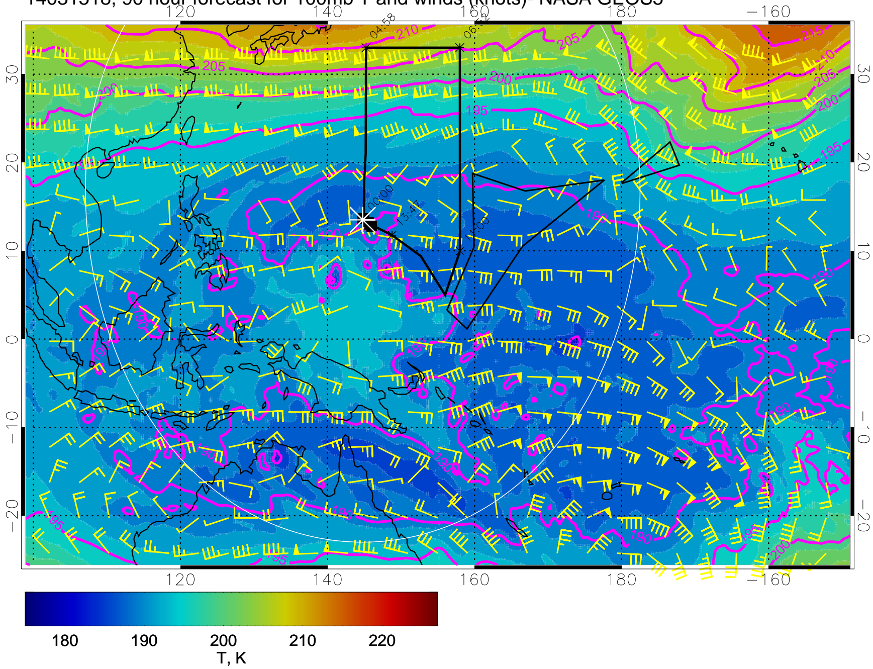
14031518, 90 hour forecast for 100mb T and winds (knots)- NASA GEOS5
