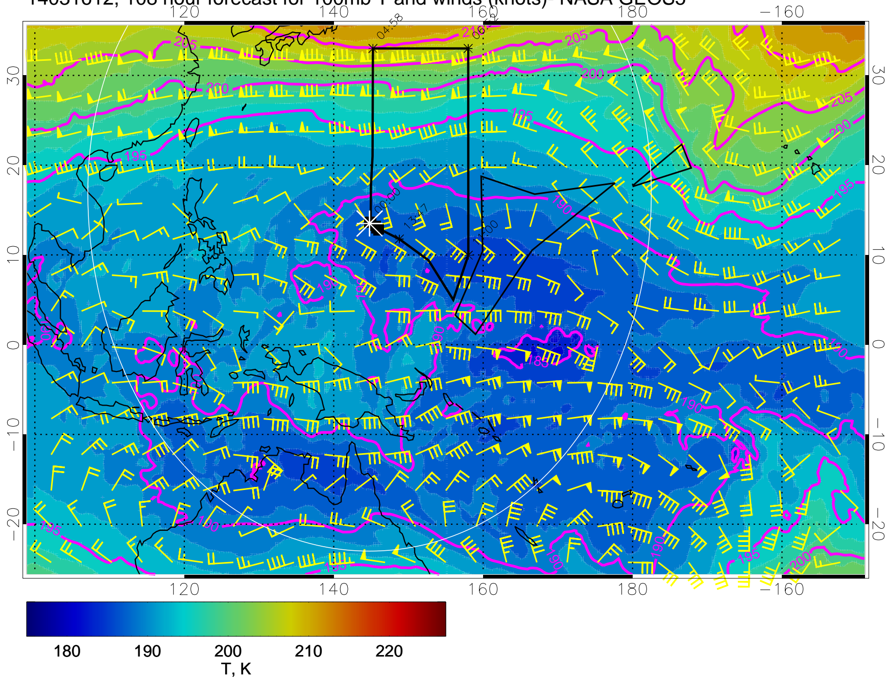
14031612, 108 hour forecast for 100mb T and winds (knots)- NASA GEOS5
