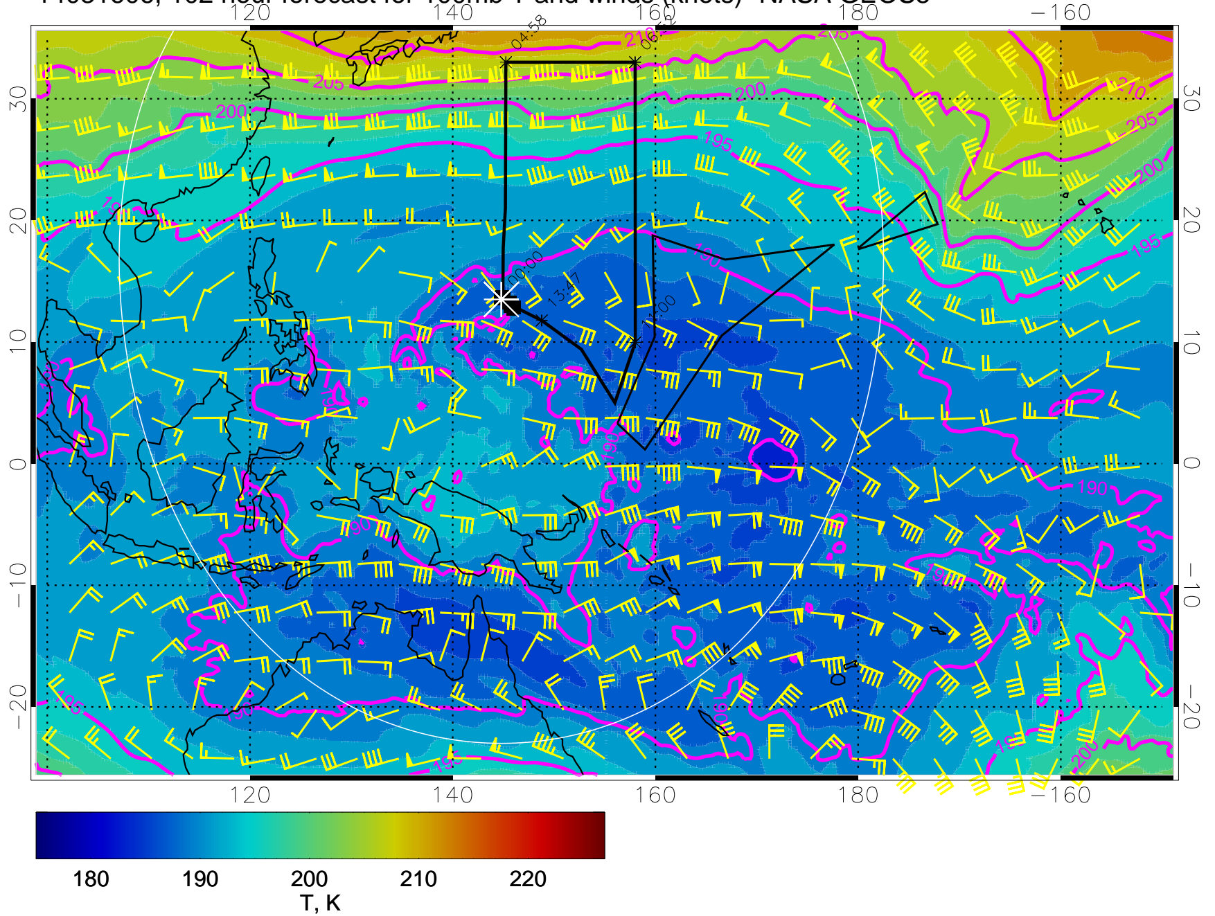
14031606, 102 hour forecast for 100mb T and winds (knots)- NASA GEOS5
