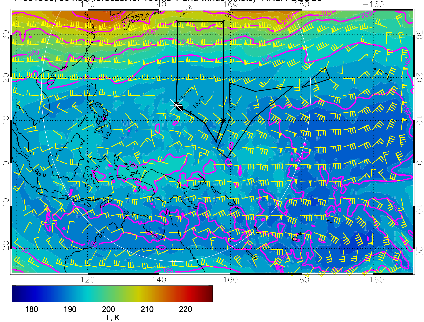
14031306, 30 hour forecast for 100mb T and winds (knots)- NASA GEOS5
