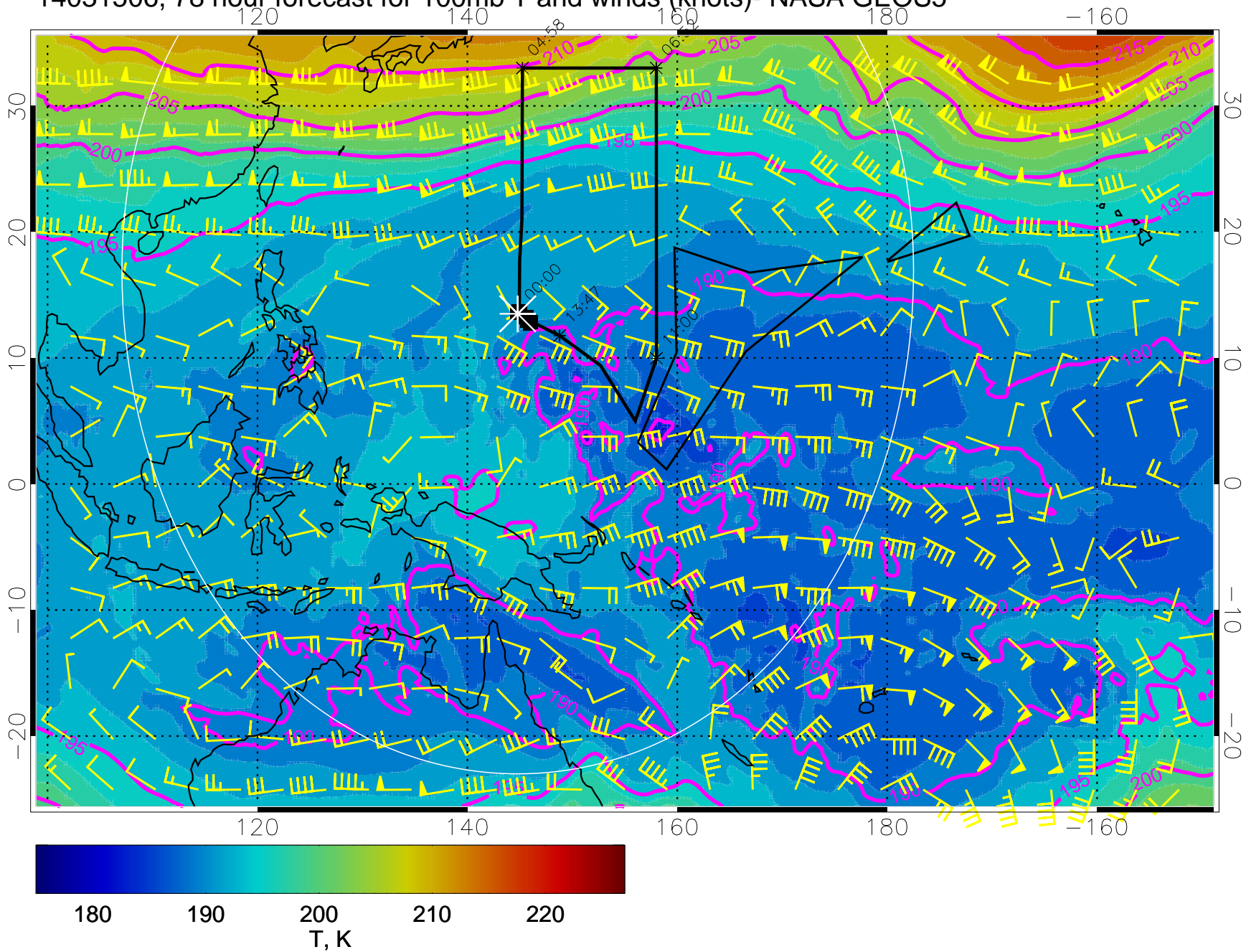
14031506, 78 hour forecast for 100mb T and winds (knots)- NASA GEOS5
