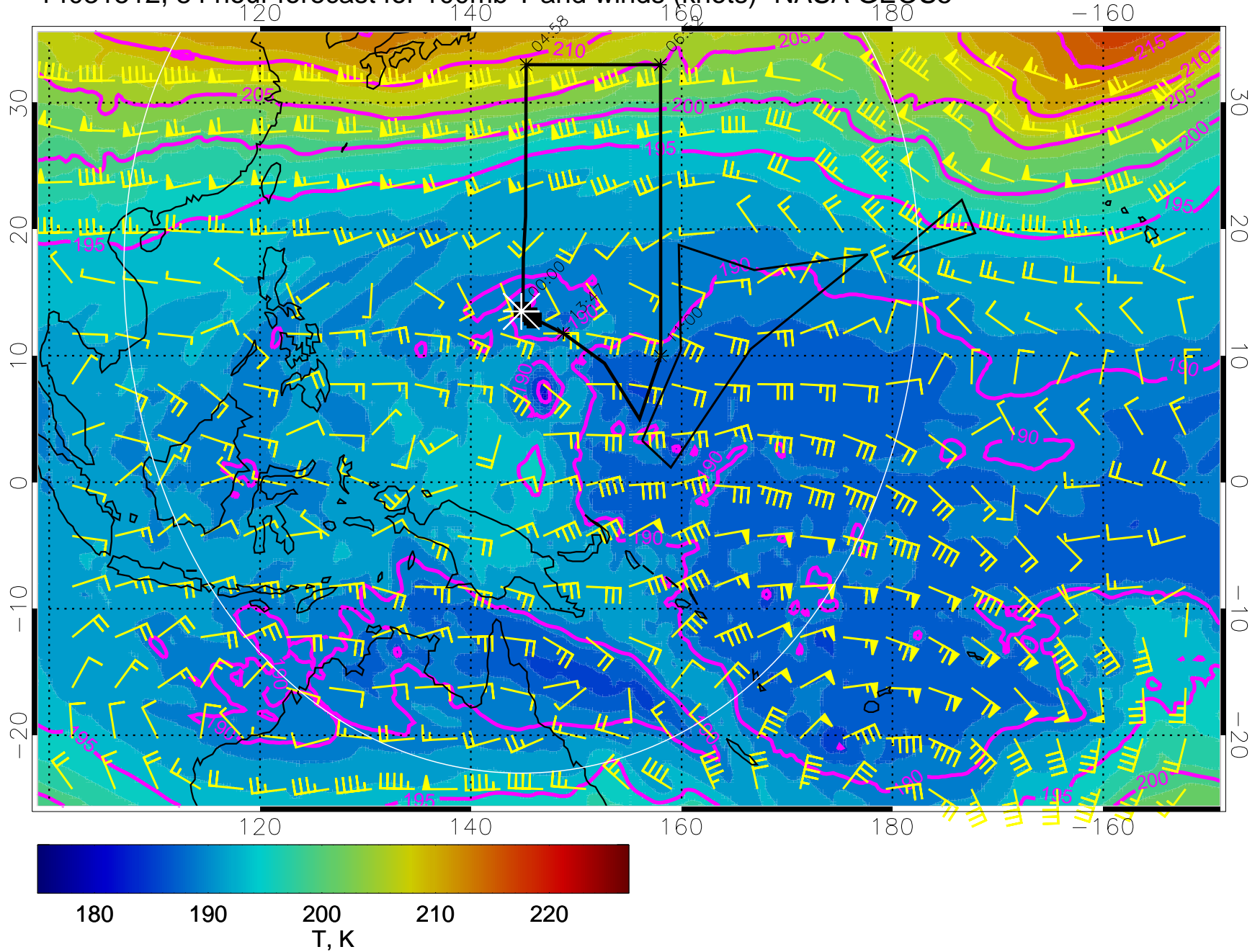
14031512, 84 hour forecast for 100mb T and winds (knots)- NASA GEOS5
