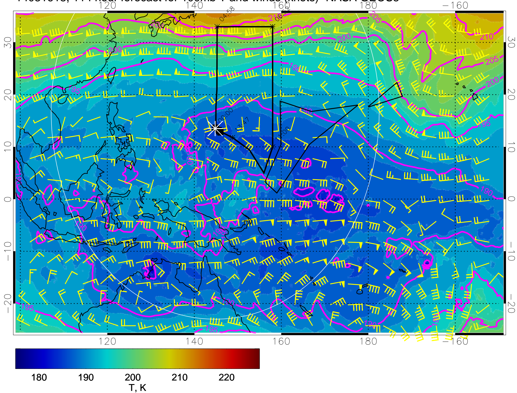
14031618, 114 hour forecast for 100mb T and winds (knots)- NASA GEOS5
