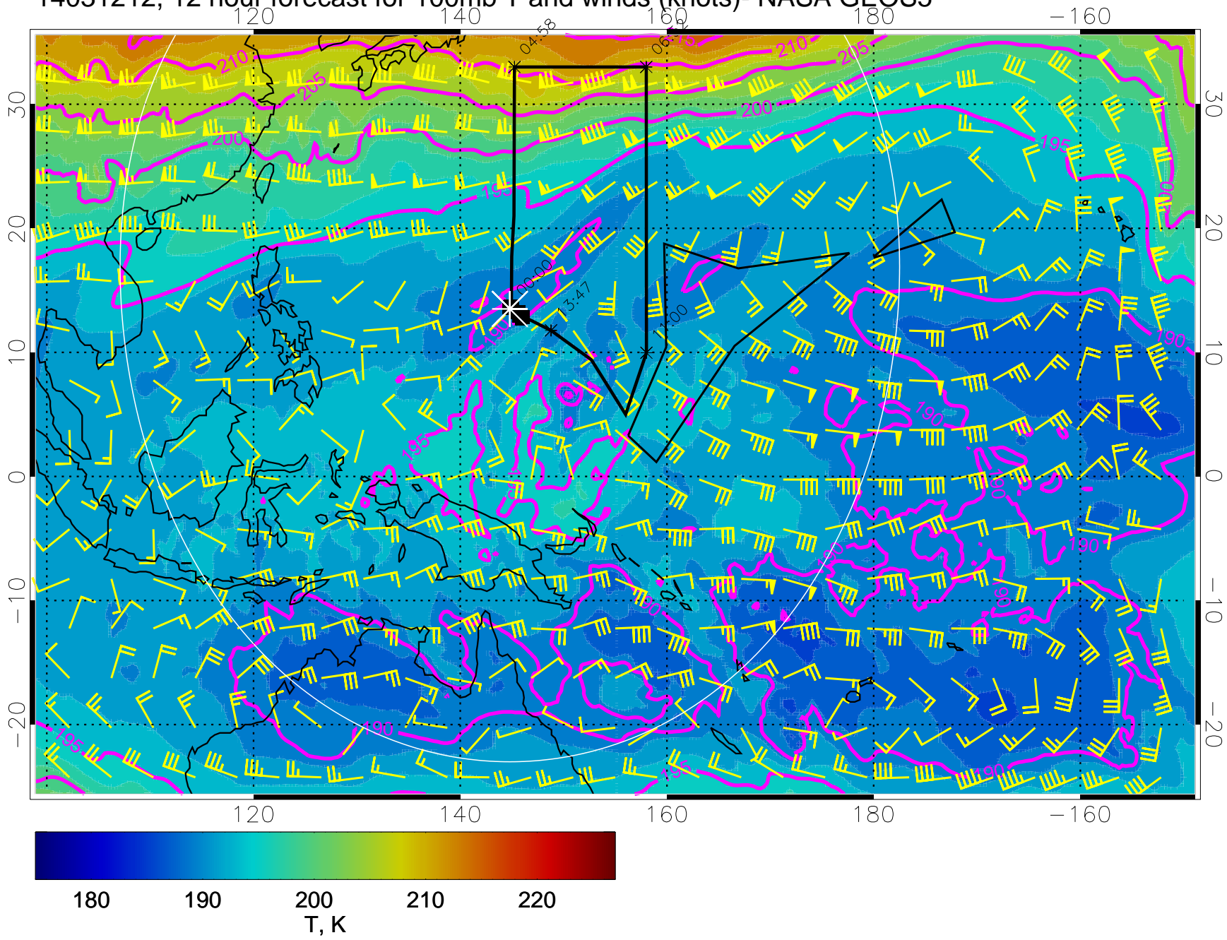
14031212, 12 hour forecast for 100mb T and winds (knots)- NASA GEOS5
