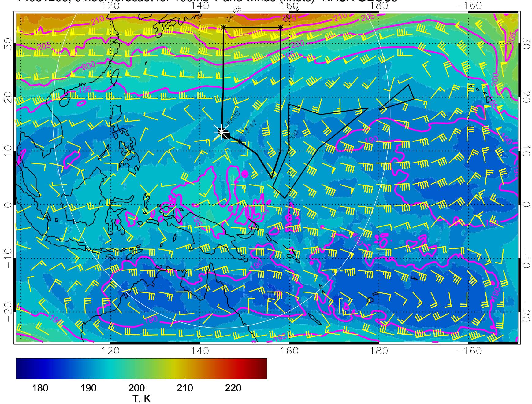
14031206, 6 hour forecast for 100mb T and winds (knots)- NASA GEOS5
