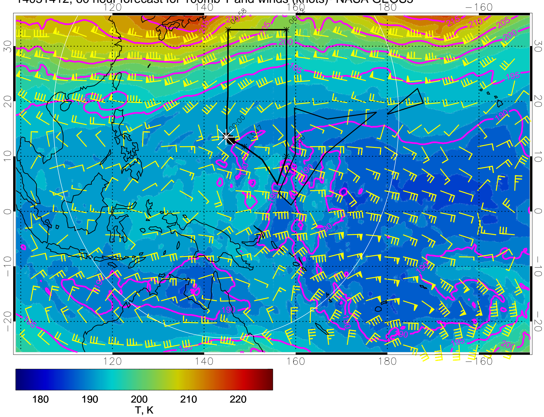
14031412, 60 hour forecast for 100mb T and winds (knots)- NASA GEOS5
