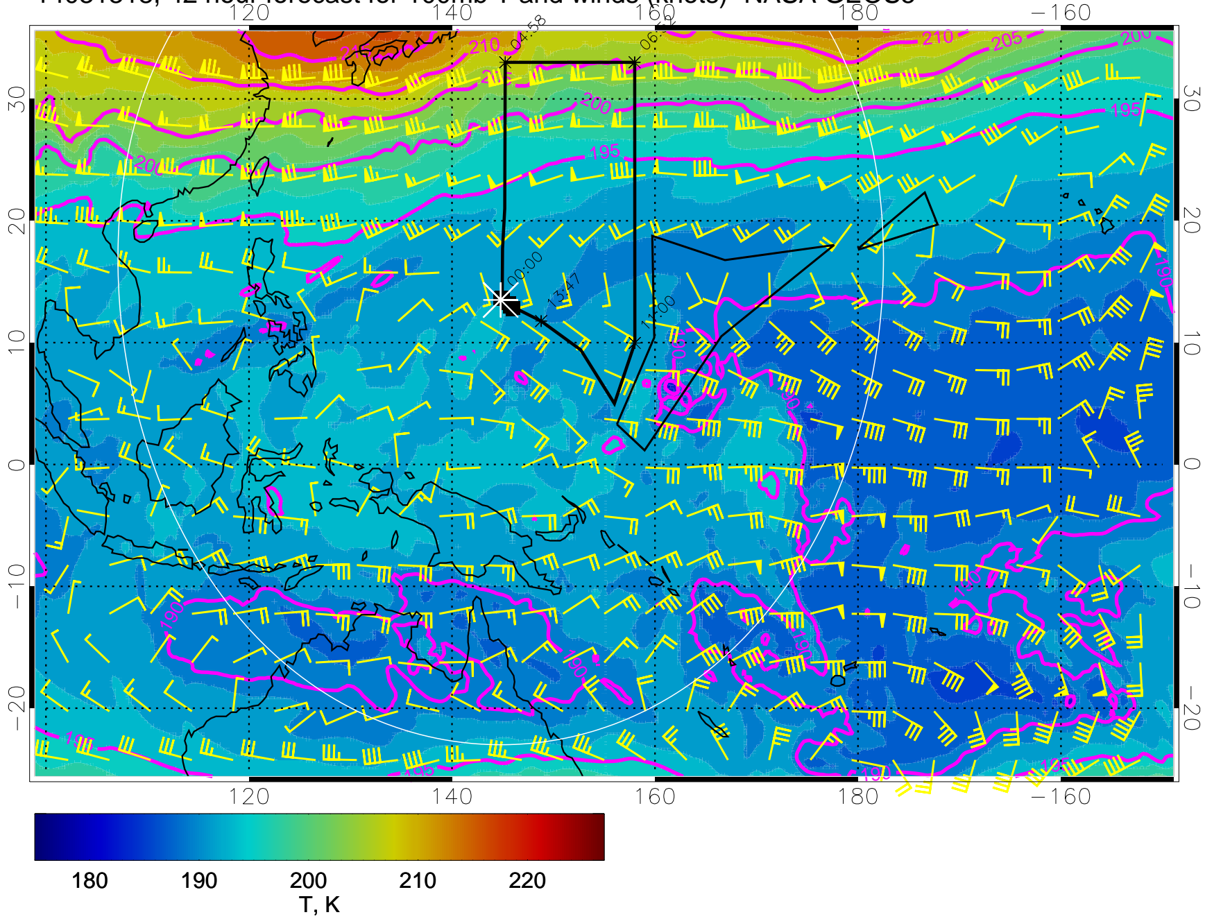
14031318, 42 hour forecast for 100mb T and winds (knots)- NASA GEOS5
