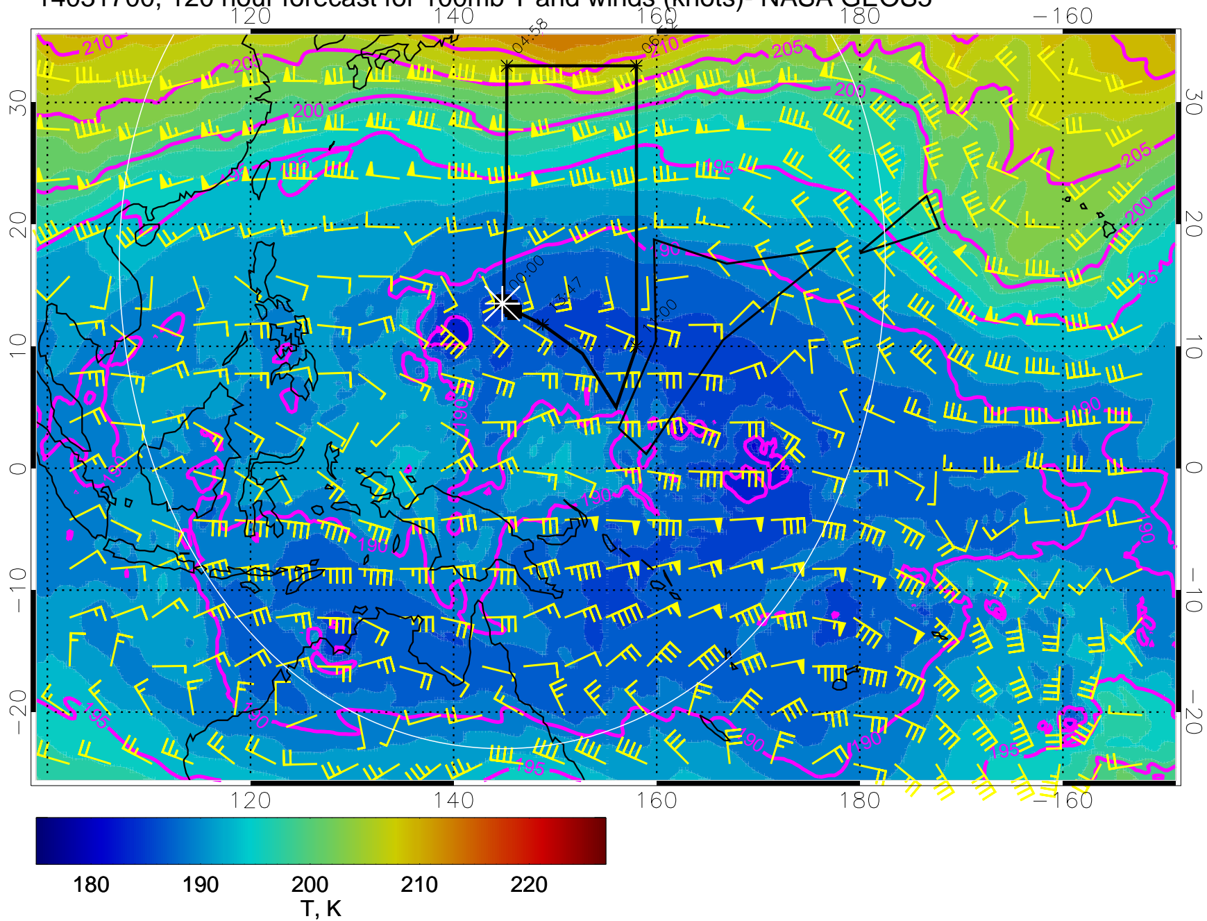
14031700, 120 hour forecast for 100mb T and winds (knots)- NASA GEOS5
