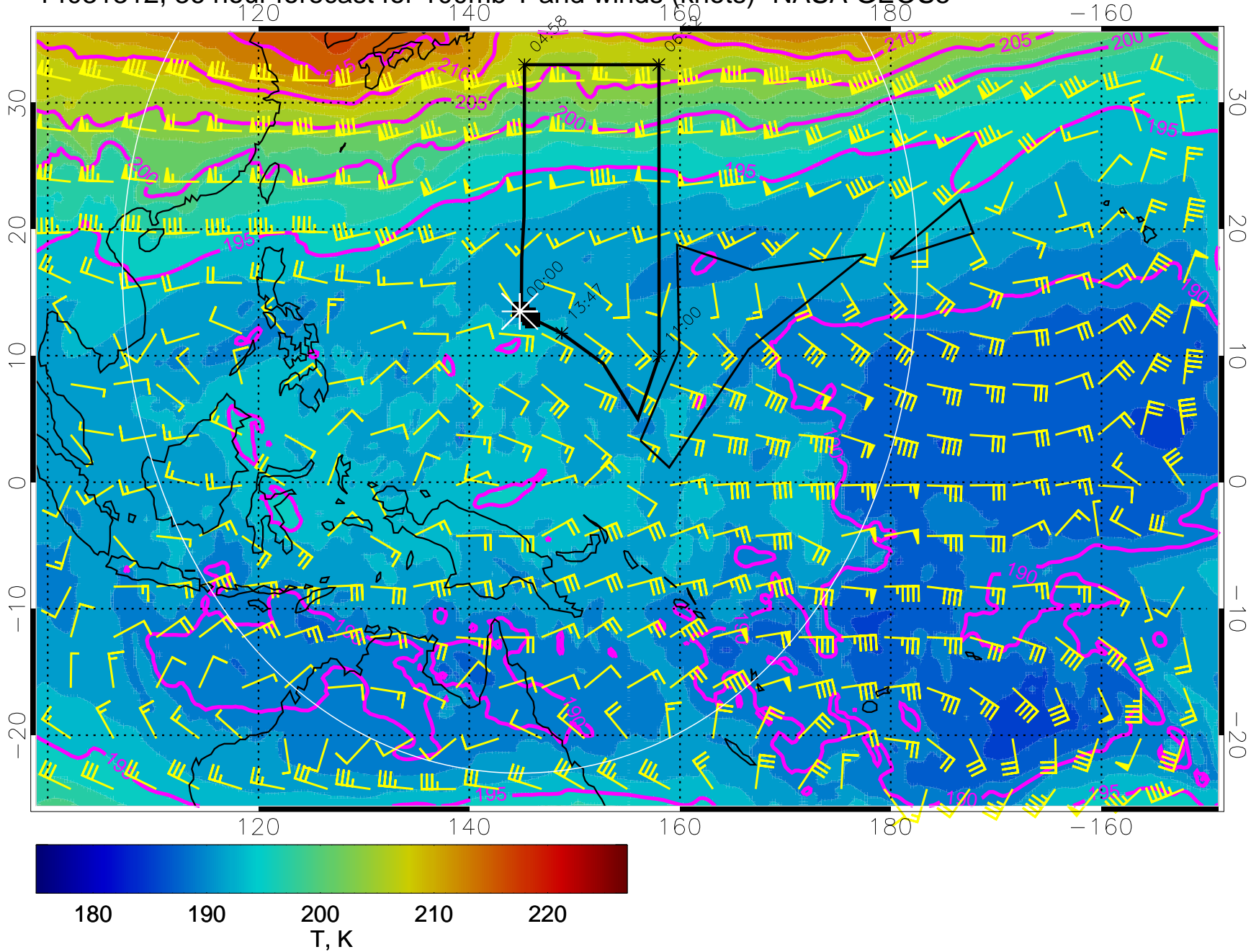
14031312, 36 hour forecast for 100mb T and winds (knots)- NASA GEOS5
