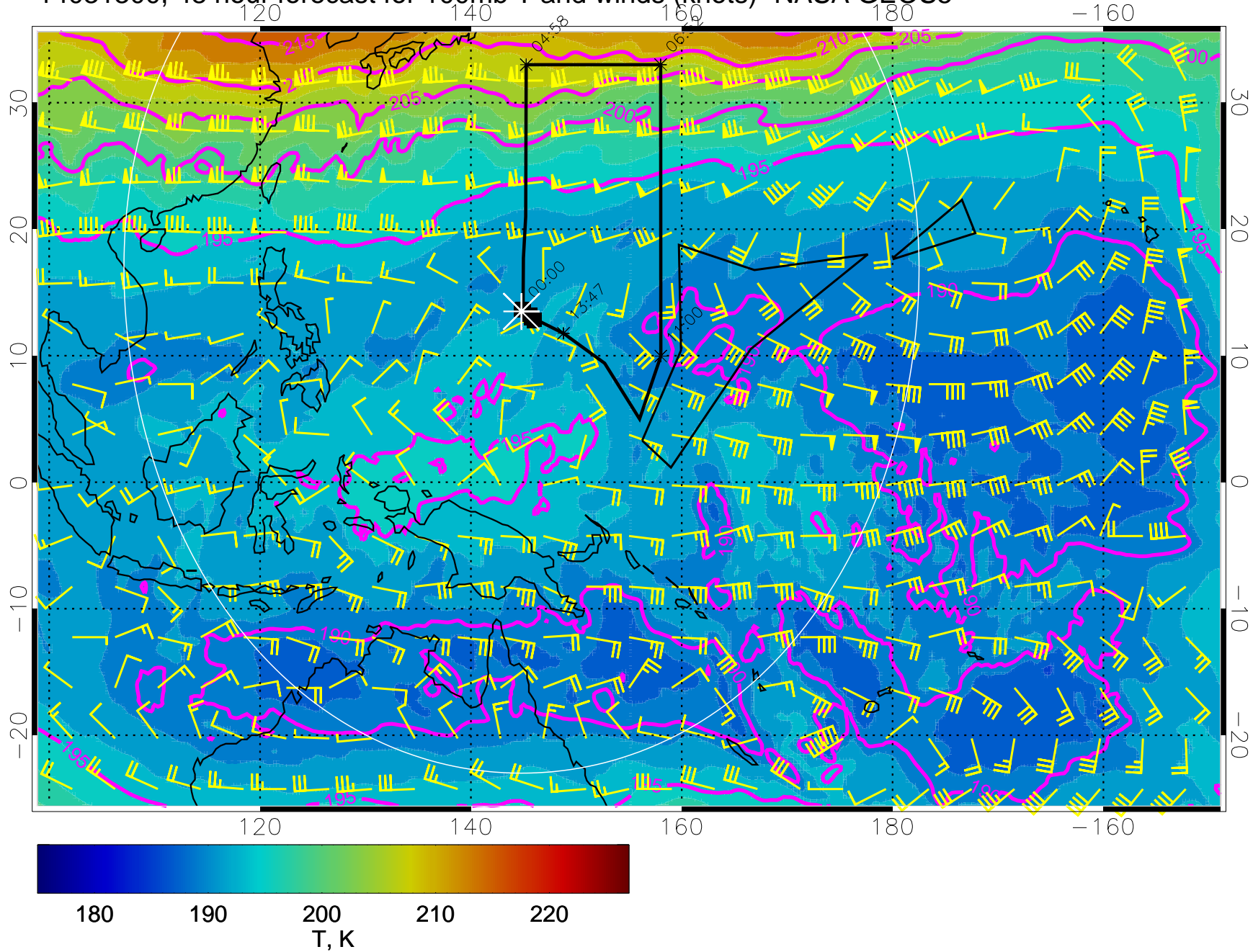
14031300, 48 hour forecast for 100mb T and winds (knots)- NASA GEOS5
