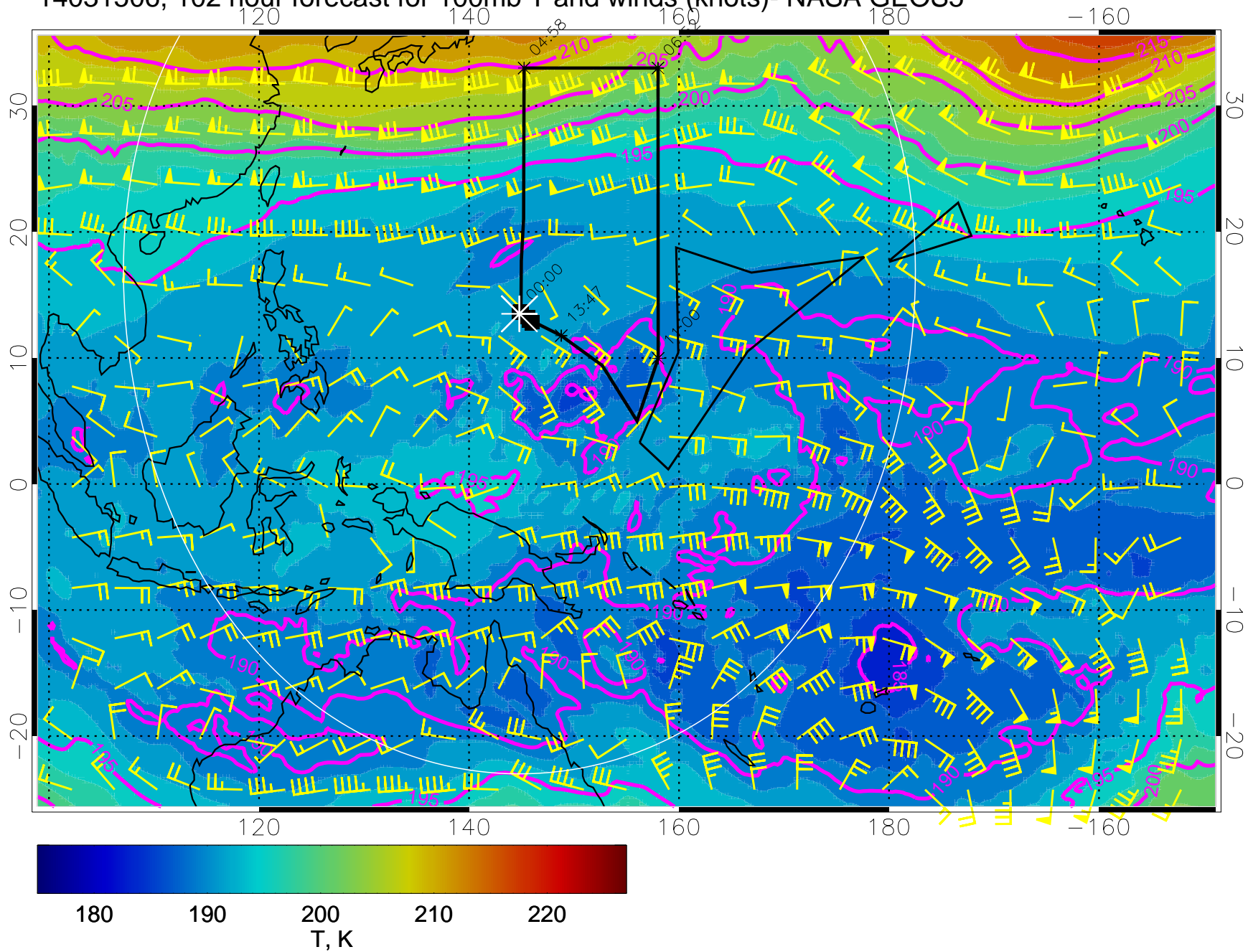
14031506, 102 hour forecast for 100mb T and winds (knots)- NASA GEOS5
