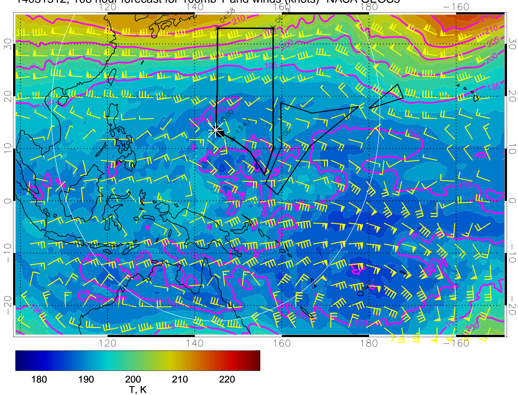
14031512, 108 hour forecast for 100mb T and winds (knots)- NASA GEOS5
