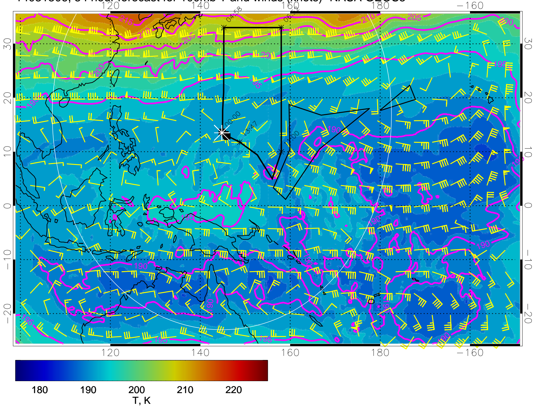
14031306, 54 hour forecast for 100mb T and winds (knots)- NASA GEOS5
