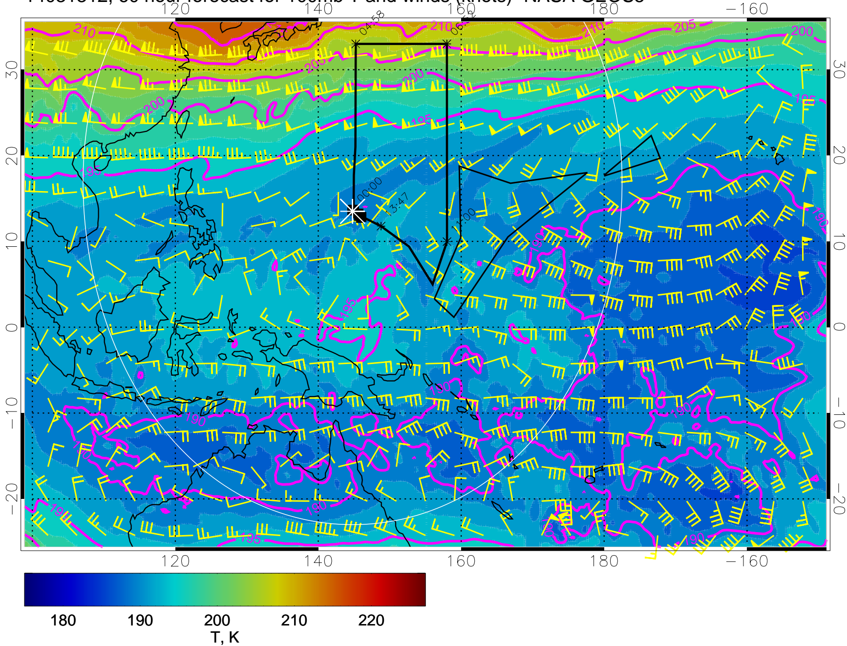
14031312, 60 hour forecast for 100mb T and winds (knots)- NASA GEOS5
