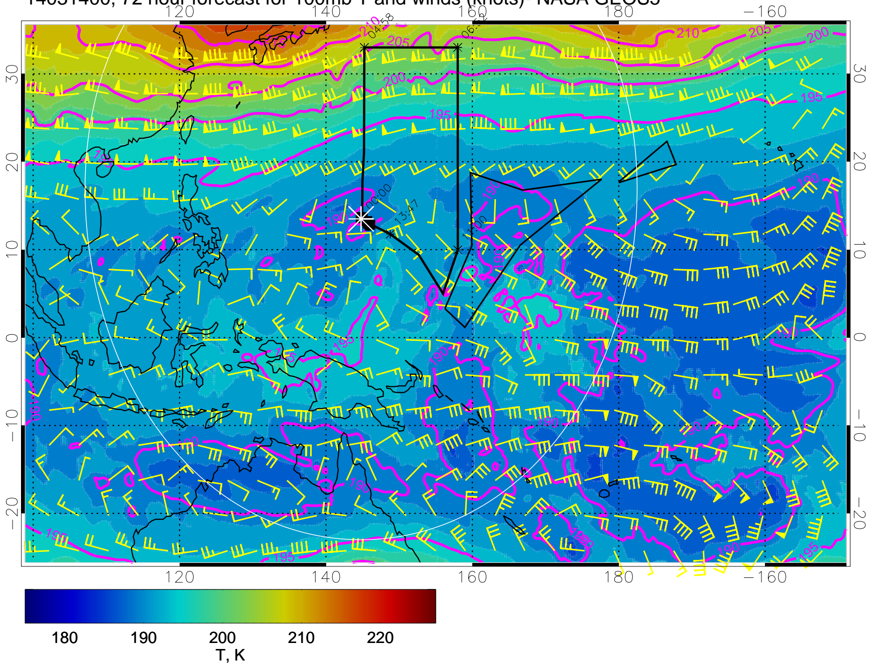
14031400, 72 hour forecast for 100mb T and winds (knots)- NASA GEOS5
