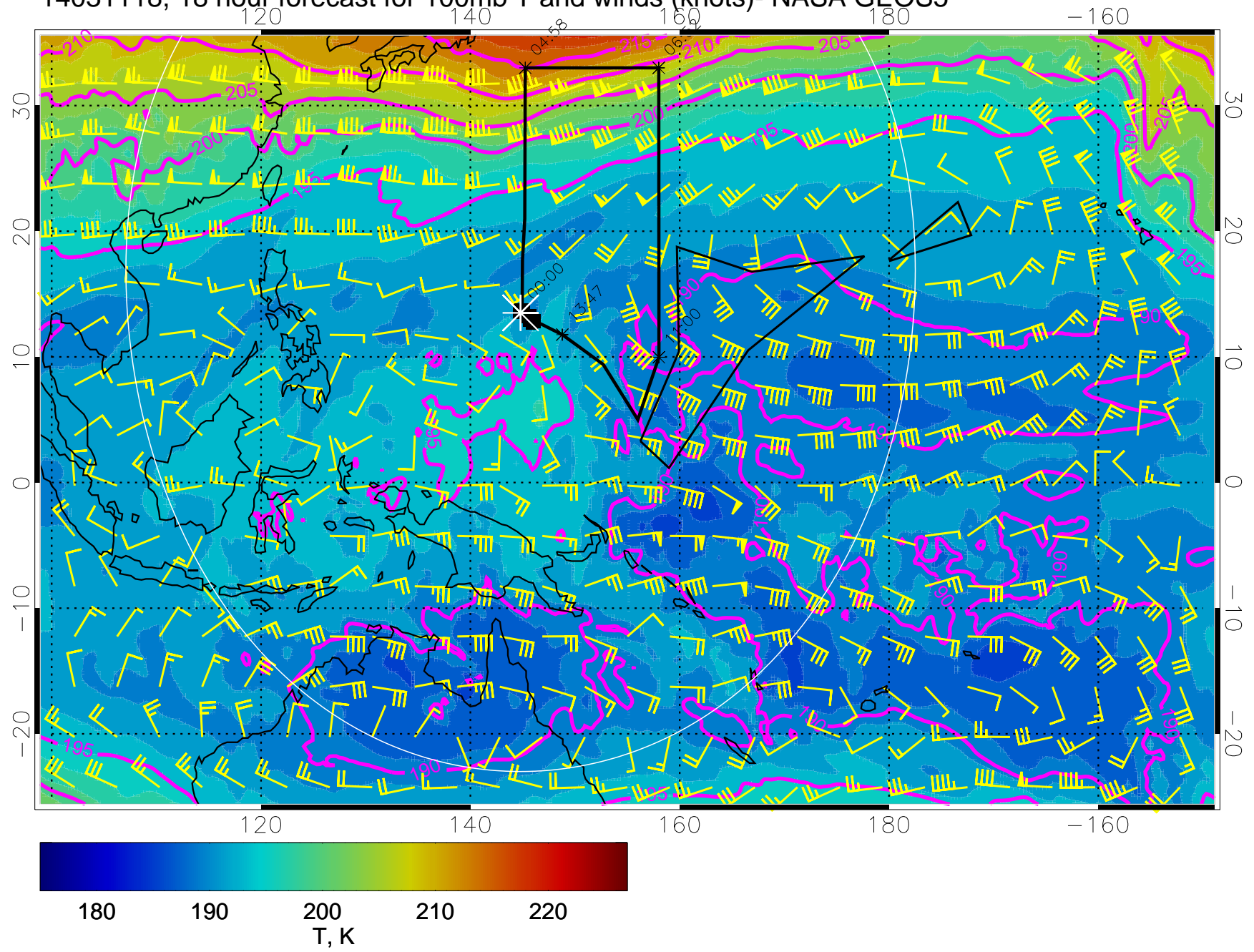
14031118, 18 hour forecast for 100mb T and winds (knots)- NASA GEOS5
