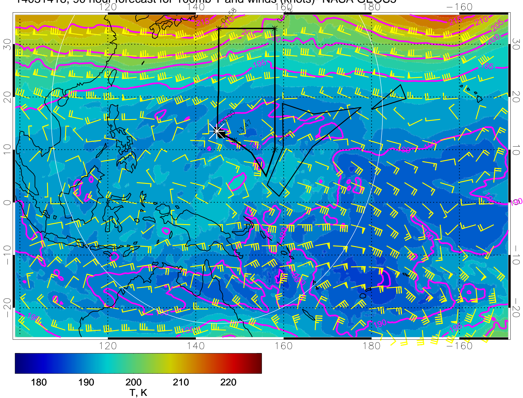
14031418, 90 hour forecast for 100mb T and winds (knots)- NASA GEOS5
