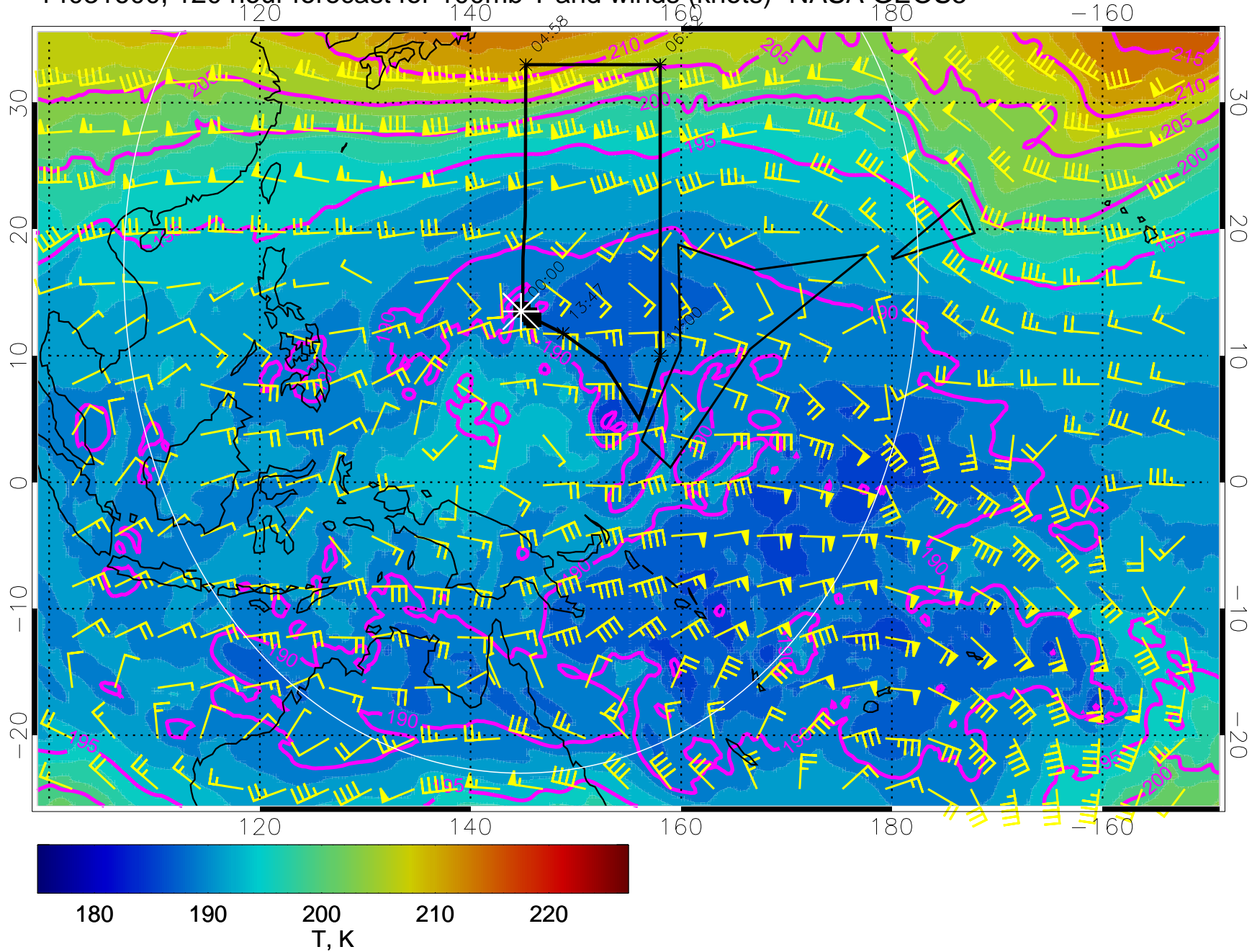
14031600, 120 hour forecast for 100mb T and winds (knots)- NASA GEOS5
