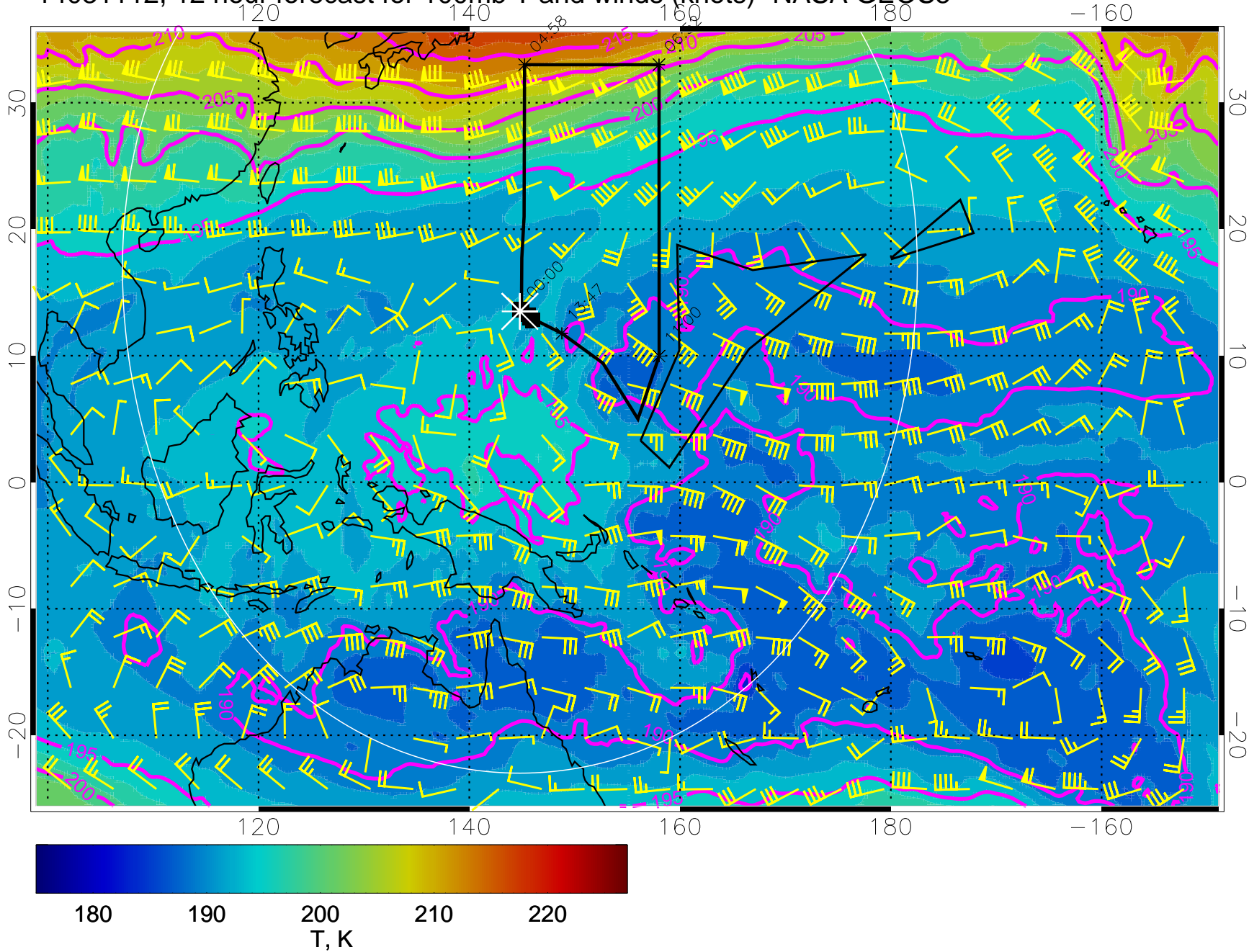
14031112, 12 hour forecast for 100mb T and winds (knots)- NASA GEOS5
