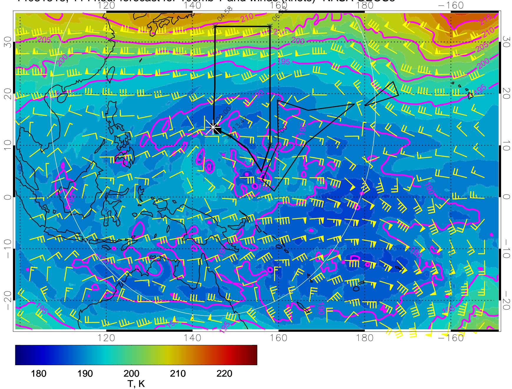
14031518, 114 hour forecast for 100mb T and winds (knots)- NASA GEOS5
