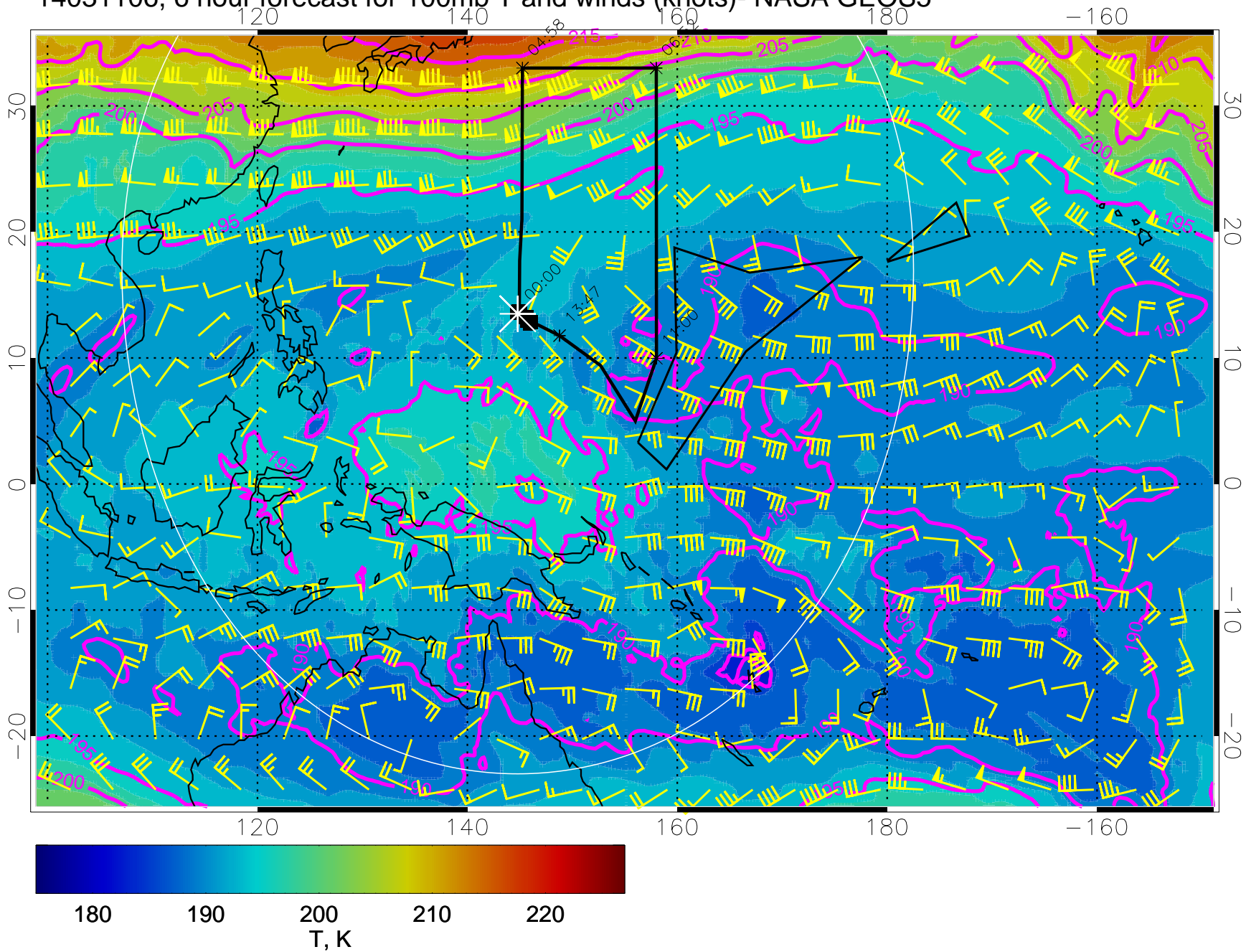
14031106, 6 hour forecast for 100mb T and winds (knots)- NASA GEOS5
