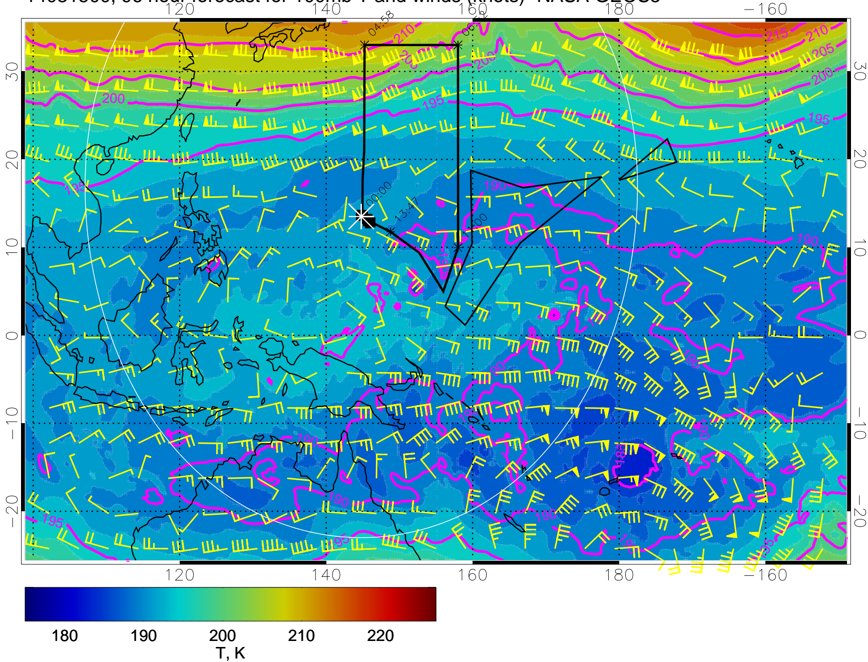
14031500, 96 hour forecast for 100mb T and winds (knots)- NASA GEOS5
