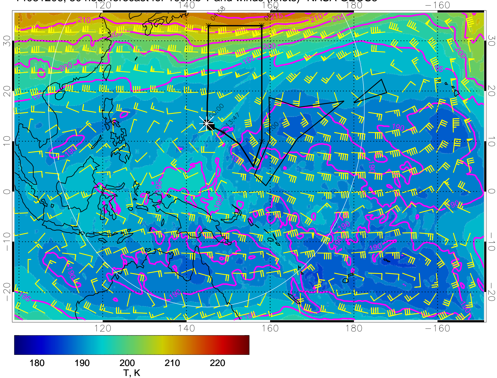
14031206, 30 hour forecast for 100mb T and winds (knots)- NASA GEOS5
