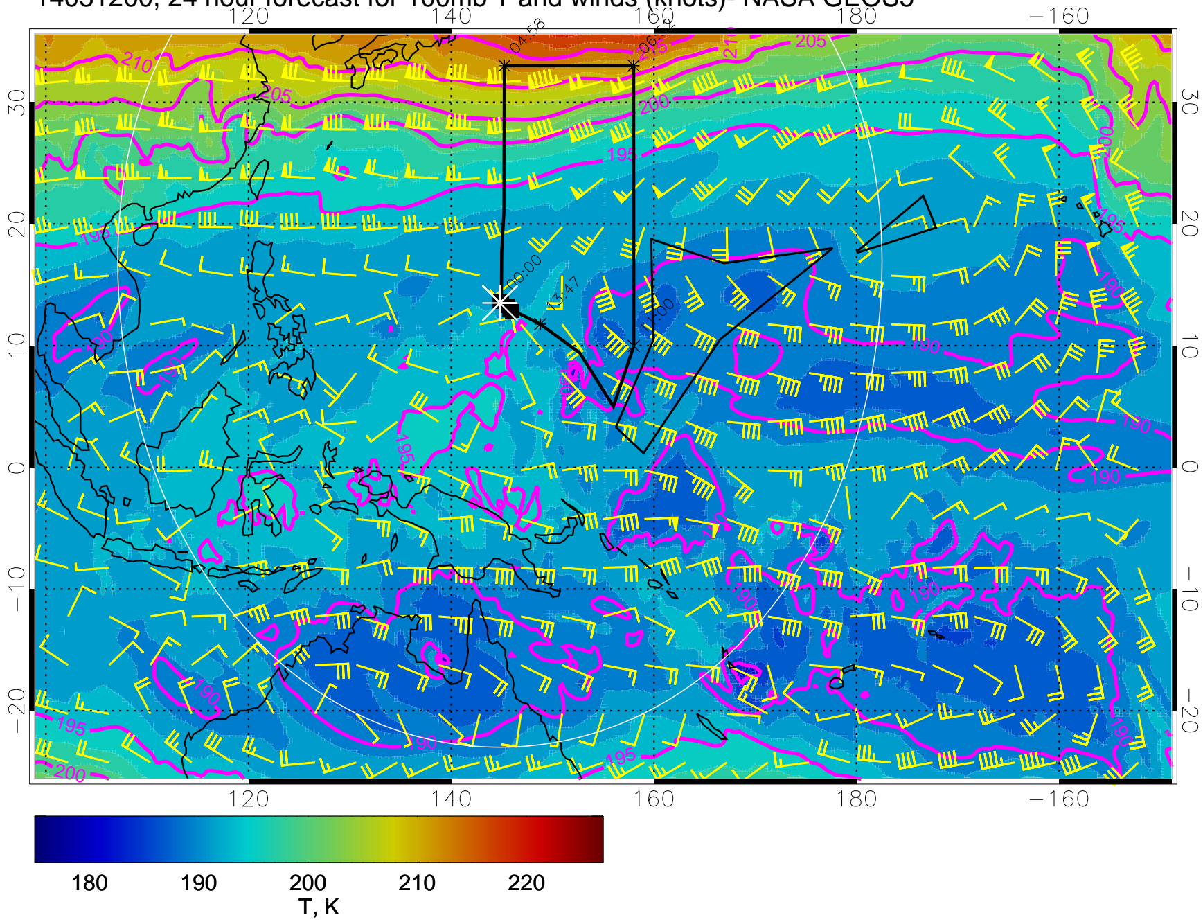
14031200, 24 hour forecast for 100mb T and winds (knots)- NASA GEOS5
