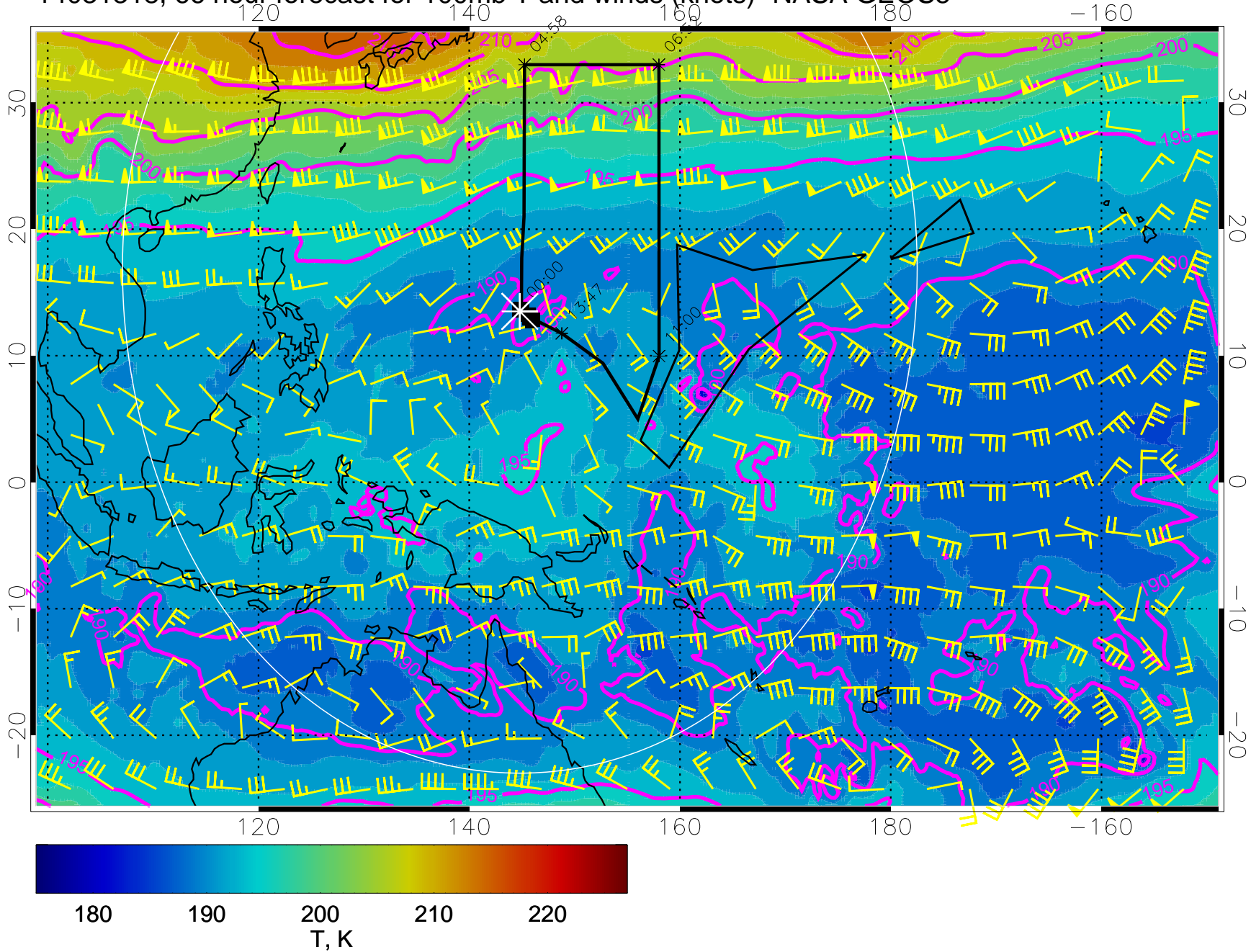
14031318, 66 hour forecast for 100mb T and winds (knots)- NASA GEOS5
