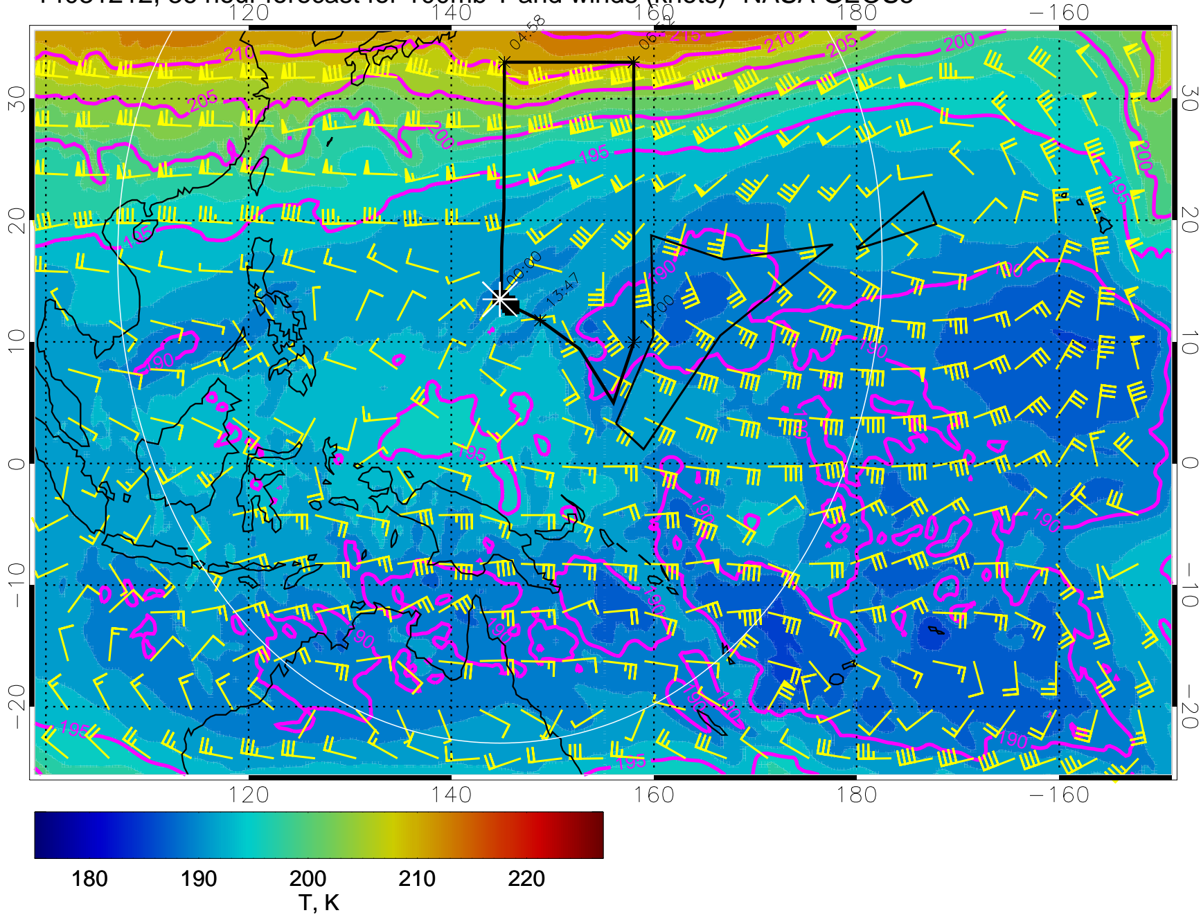
14031212, 36 hour forecast for 100mb T and winds (knots)- NASA GEOS5
