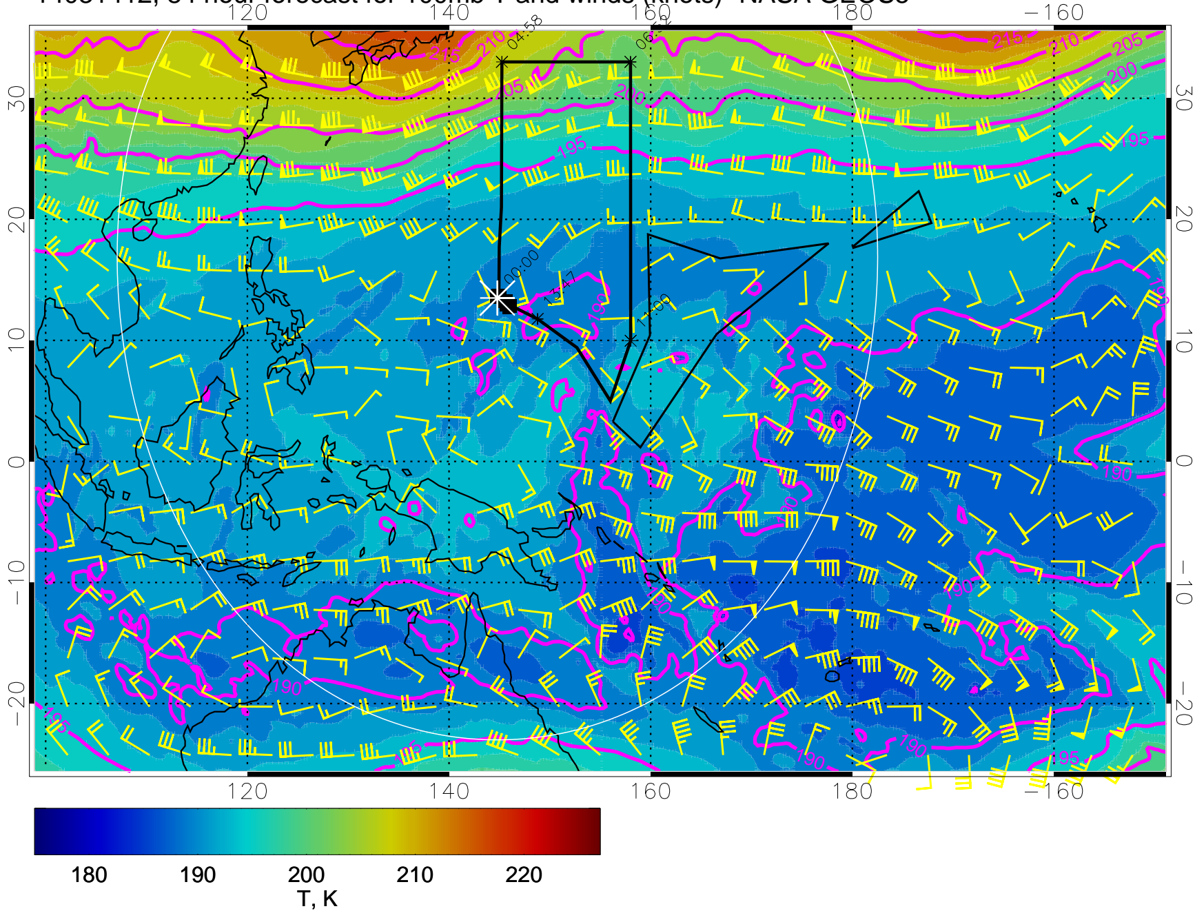
14031412, 84 hour forecast for 100mb T and winds (knots)- NASA GEOS5
