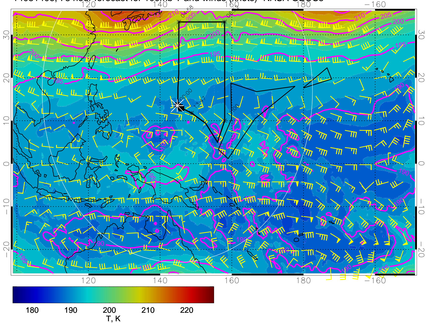
14031406, 78 hour forecast for 100mb T and winds (knots)- NASA GEOS5
