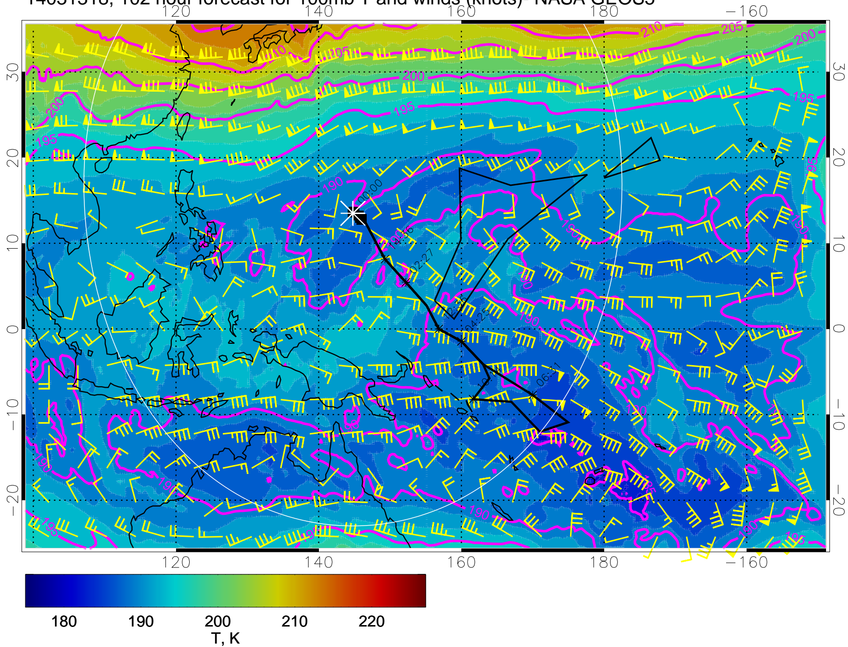
14031318, 102 hour forecast for 100mb T and winds (knots)- NASA GEOS5
