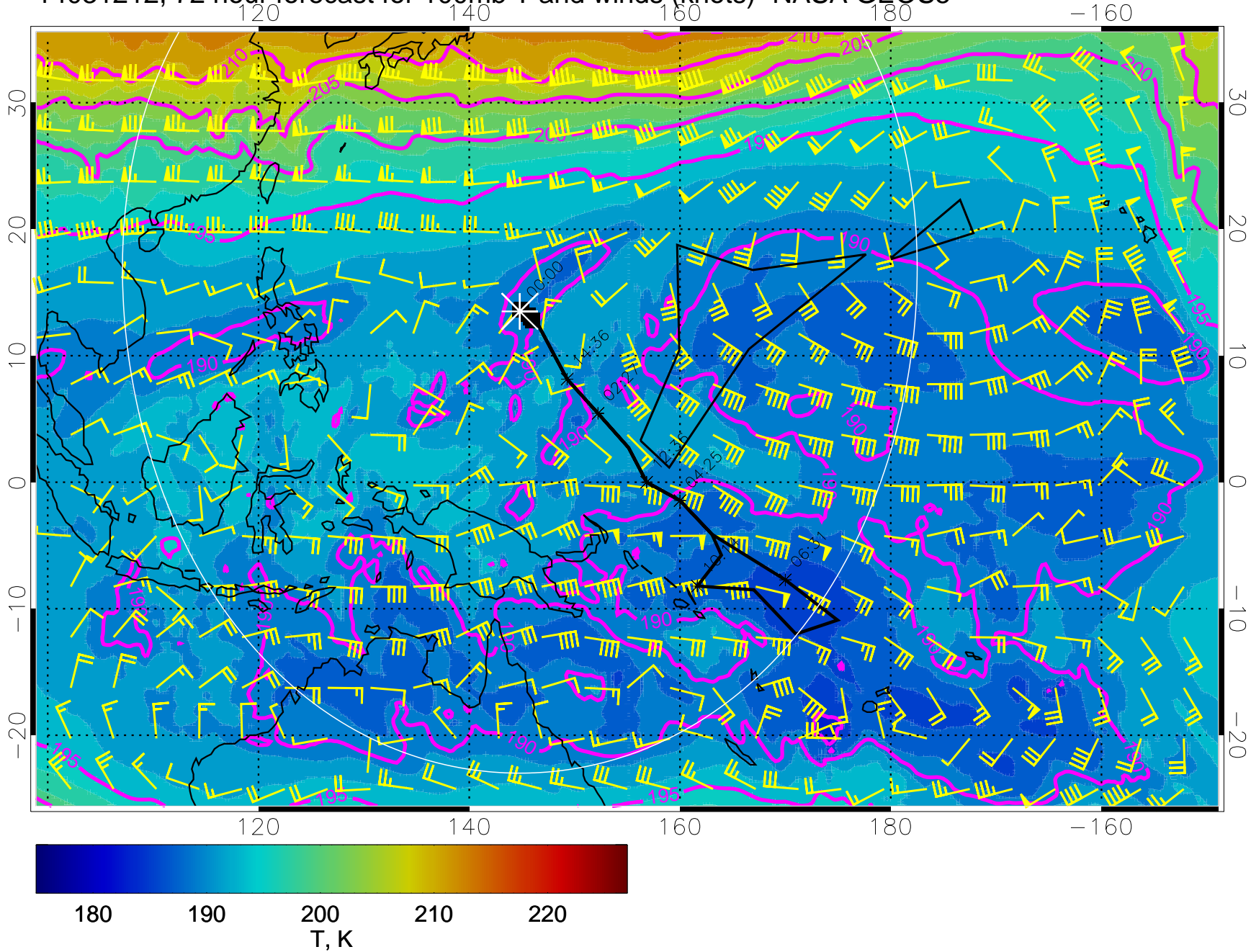
14031212, 72 hour forecast for 100mb T and winds (knots)- NASA GEOS5
