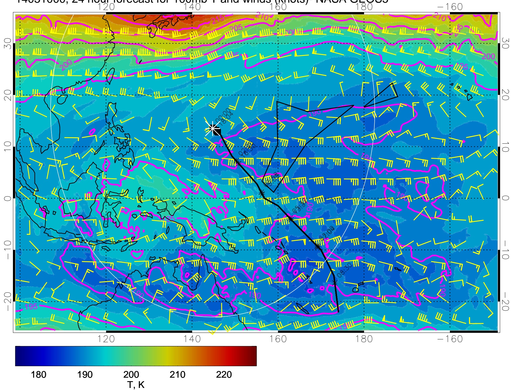
14031000, 24 hour forecast for 100mb T and winds (knots)- NASA GEOS5
