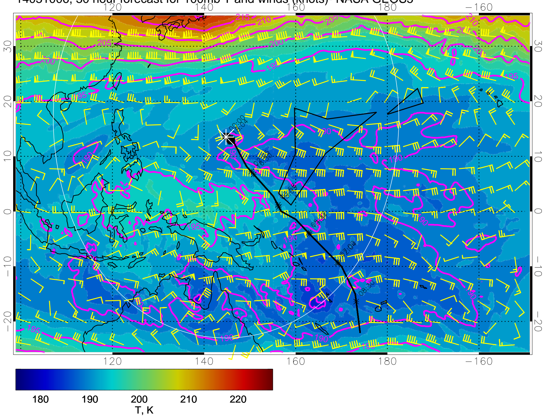
14031006, 30 hour forecast for 100mb T and winds (knots)- NASA GEOS5
