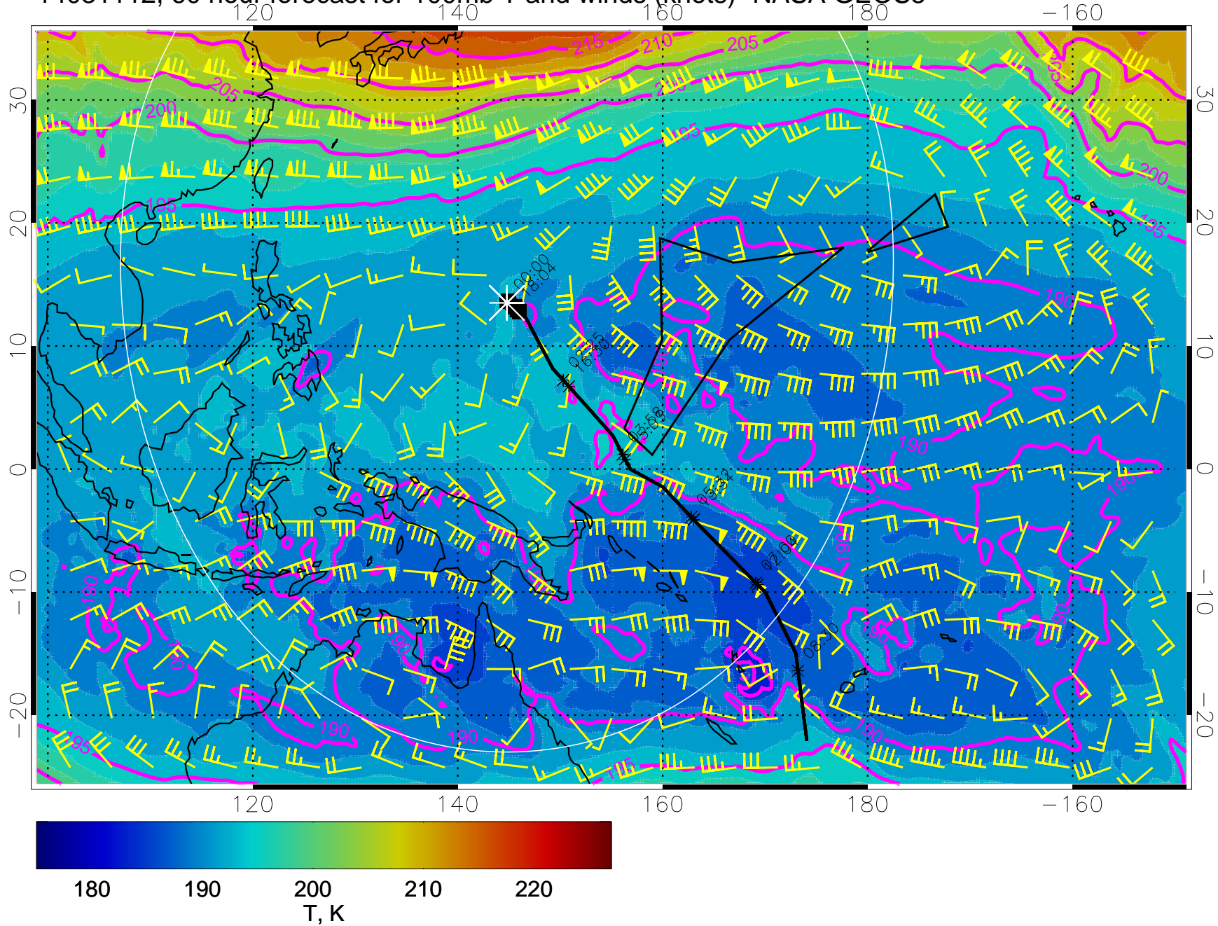
14031112, 60 hour forecast for 100mb T and winds (knots)- NASA GEOS5
